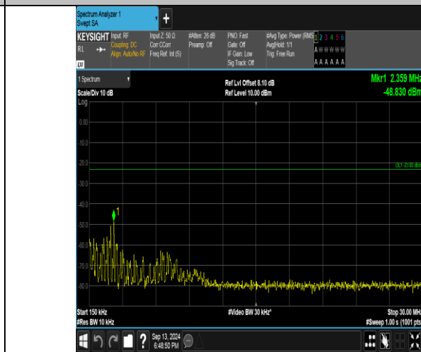
Band26_3MHz_QPSK_26805_15RB#0_0.15~30_0.15~30
