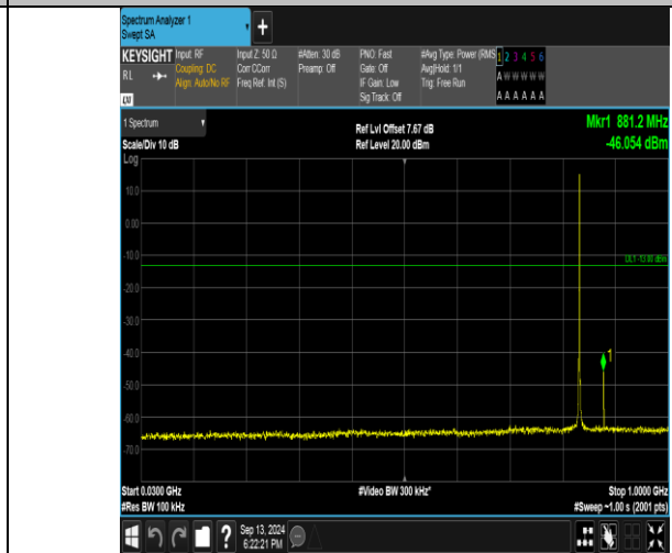
Band26_1.4MHz_16QAM_26915_1RB#5_30~1000_30~1000
