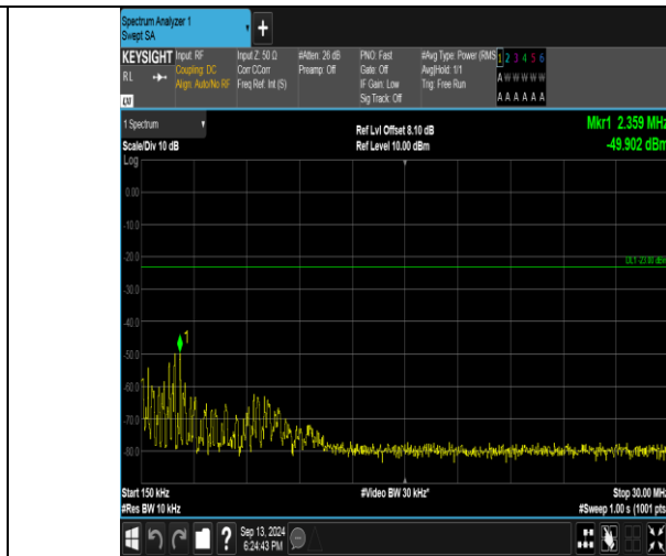
Band26_1.4MHz_QPSK_27033_1RB#0_0.15-30_0.15-30
