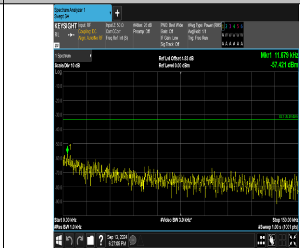
Band26_1.4MHz_16QAM_27033_1RB#5_0.009~0.15_0.009~0.15
