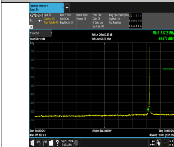
Band26_3MHz_QPSK_26805_1RB#0_30~1000_30~1000
