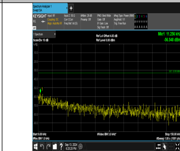
Band26_1.4MHz_16QAM_27033_1RB#0_0.009-0.15_0.009-0.15
