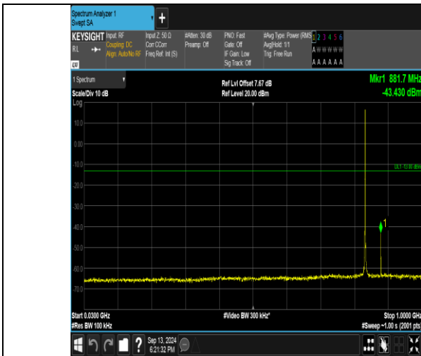
Band26_1.4MHz_QPSK_26915_1RB#5_30~1000_30~1000
