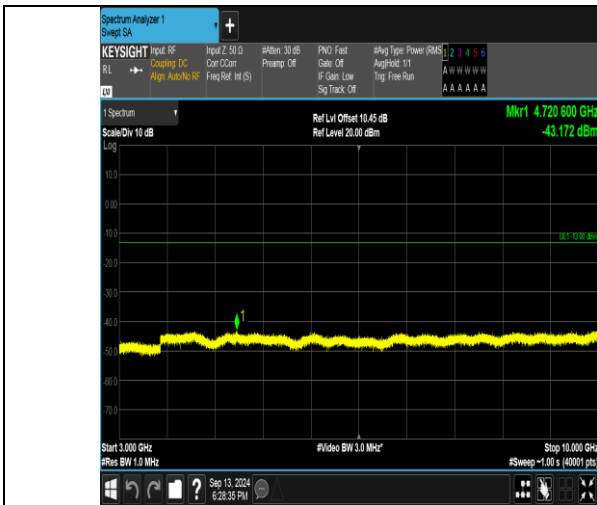
Band26_1.4MHz_QPSK_27033_6RB#0_3000~10000_3000~10000
