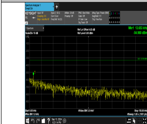
Band26_1.4MHz_QPSK_26915_1RB#5_0.009~0.15_0.009~0.15
