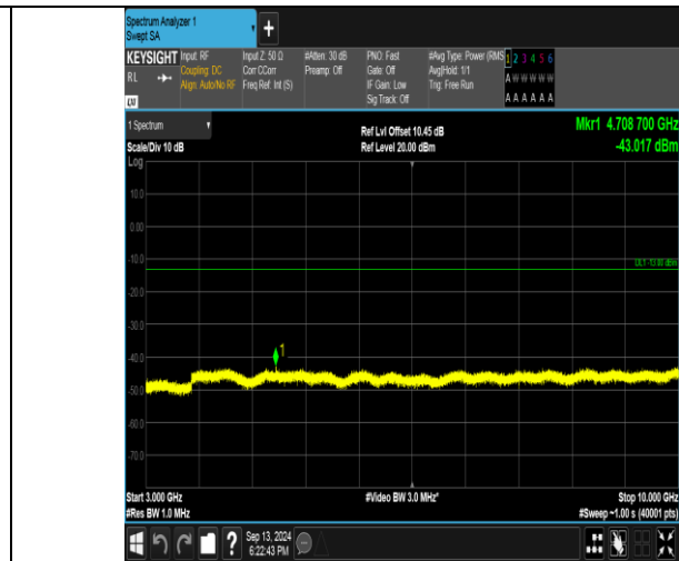
Band26_1.4MHz_16QAM_26915_1RB#5_3000~10000_3000~10000
