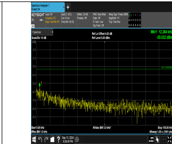
Band26_1.4MHz_16QAM_27033_6RB#0_0.009~0.15_0.009~0.15
