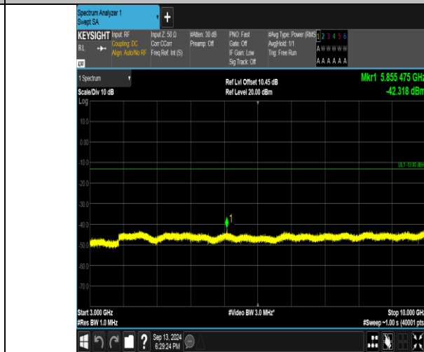
Band26_1.4MHz_16QAM_27033_6RB#0_3000~10000_3000~10000
