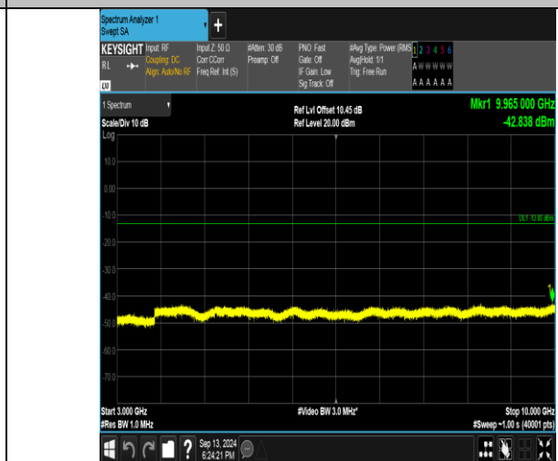
Band26_1.4MHz_16QAM_26915_6RB#0_3000~10000_3000~10000
