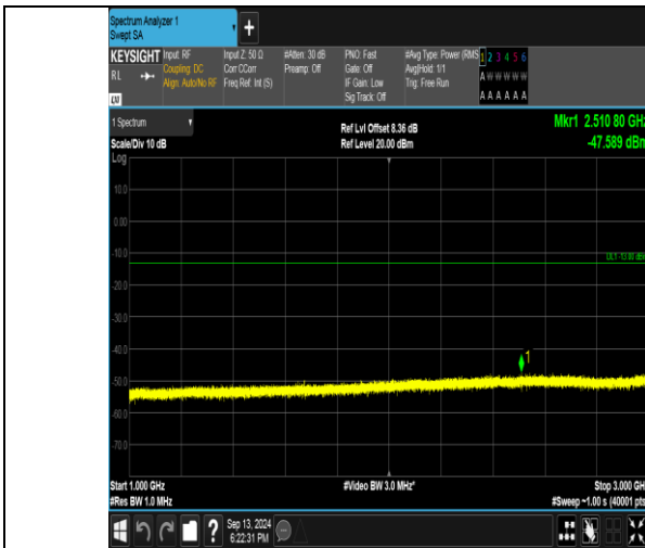
Band26_1.4MHz_16QAM_26915_1RB#5_1000~3000_1000~3000
