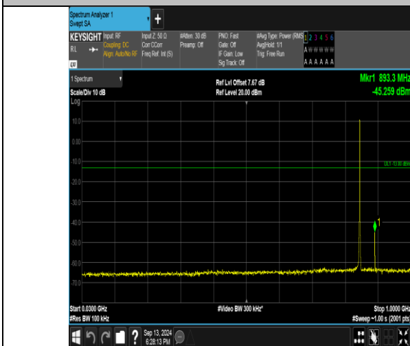
Band26_1.4MHz_QPSK_27033_6RB#0_30~1000_30~1000
