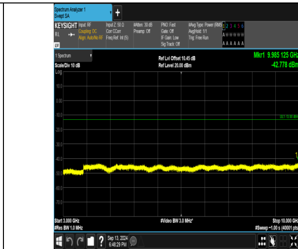
Band26_3MHz_16QAM_26805_1RB#14_3000~10000_3000~10000
