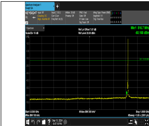
Band26_3MHz_QPSK_26805_1RB#14_30~1000_30~1000
