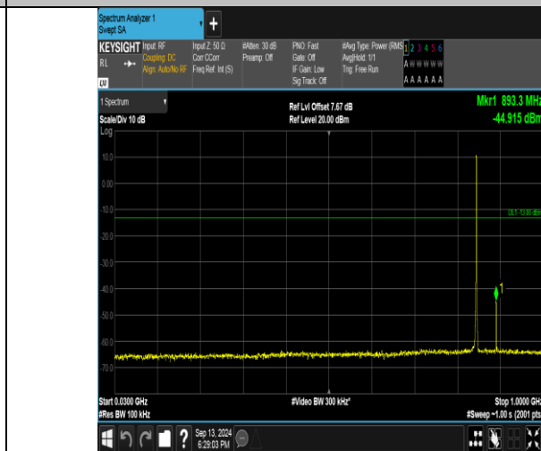
Band26_1.4MHz_16QAM_27033_6RB#0_30~1000_30~1000
