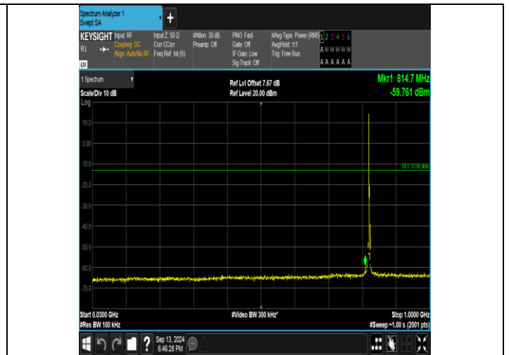
Band26_3MHz_16QAM_26805_1RB#0_30~1000_30~1000
