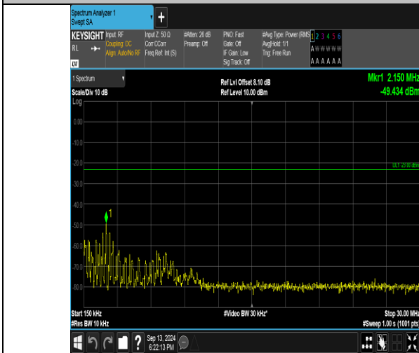
Band26_1.4MHz_16QAM_26915_1RB#5_0.15~30_0.15~30
