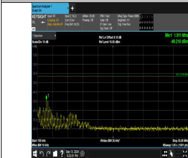
Band26_1.4MHz_16QAM_26915_6RB#0_0.15~30_0.15~30
