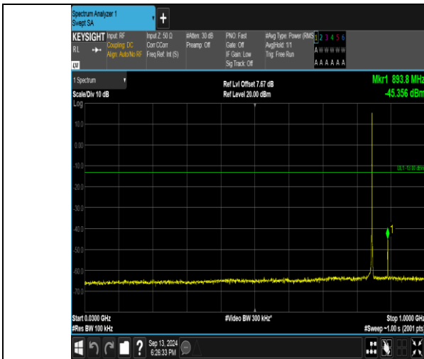
Band26_1.4MHz_QPSK_27033_1RB#5_30~1000_30~1000
