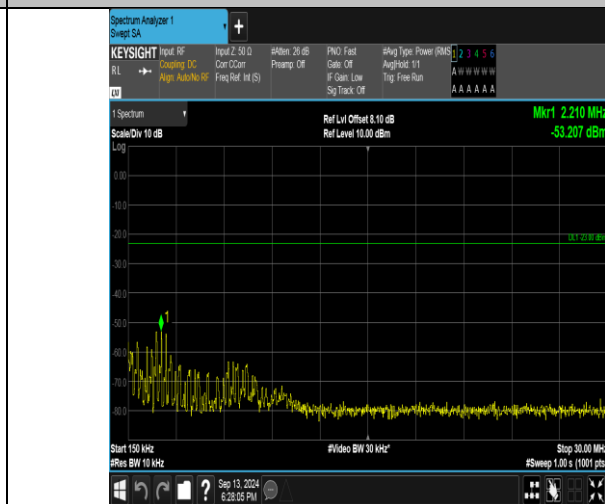
Band26_1.4MHz_QPSK_27033_6RB#0_0.15~30_0.15~30
