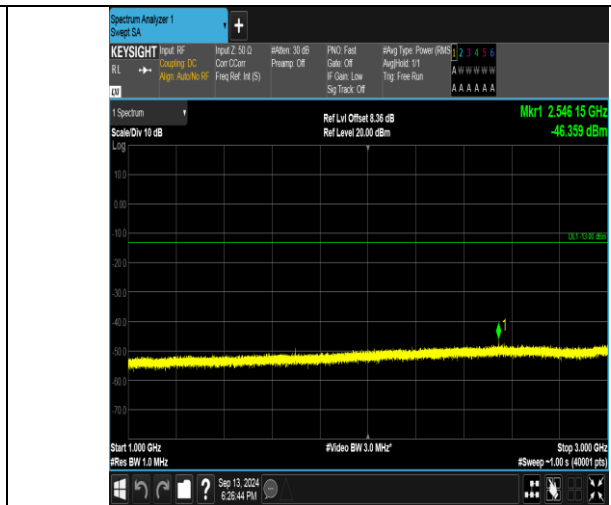
Band26_1.4MHz_QPSK_27033_1RB#5_1000~3000_1000~3000
