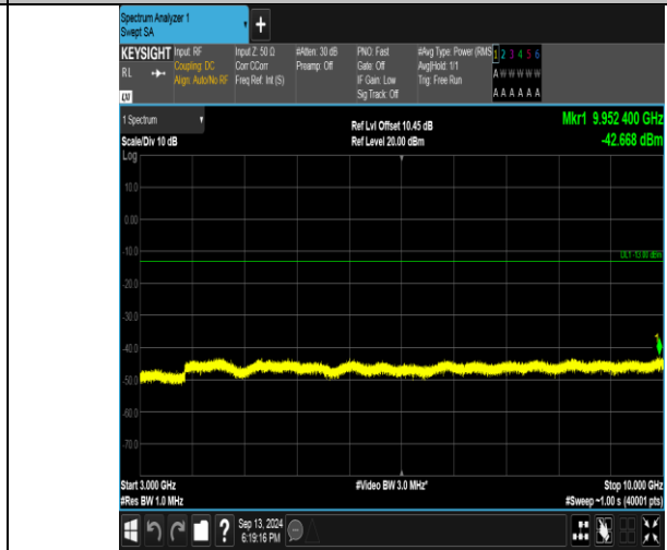
Band26_1.4MHz_16QAM_26797_6RB#0_3000~10000_3000~10000
