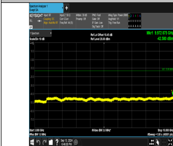
Band26_3MHz_QPSK_26805_1RB#0_3000~10000_3000~10000
