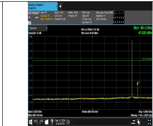
Band26_1.4MHz_16QAM_26915_1RB#0_30~1000_30~1000
