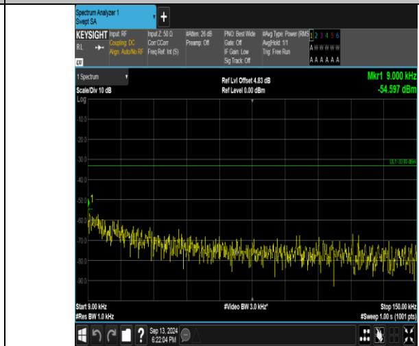
Band26_1.4MHz_16QAM_26915_1RB#5_0.009~0.15_0.009~0.15
