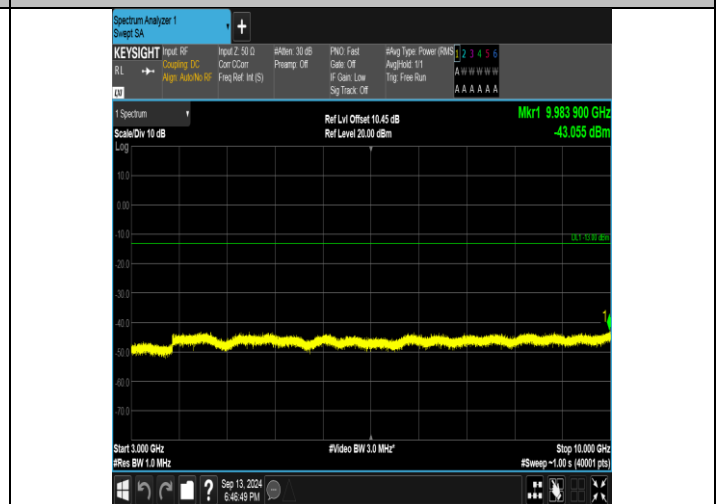
Band26_3MHz_16QAM_26805_1RB#0_3000~10000_3000~10000
