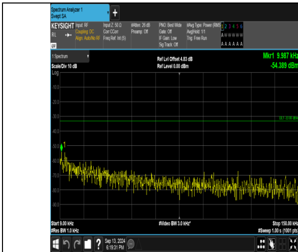
Band26_1.4MHz_QPSK_26915_1RB#0_0.009~0.15_0.009~0.15
