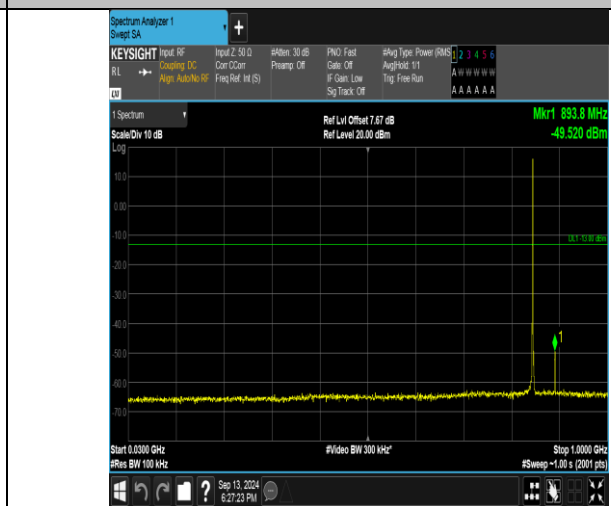
Band26_1.4MHz_16QAM_27033_1RB#5_30~1000_30~1000
