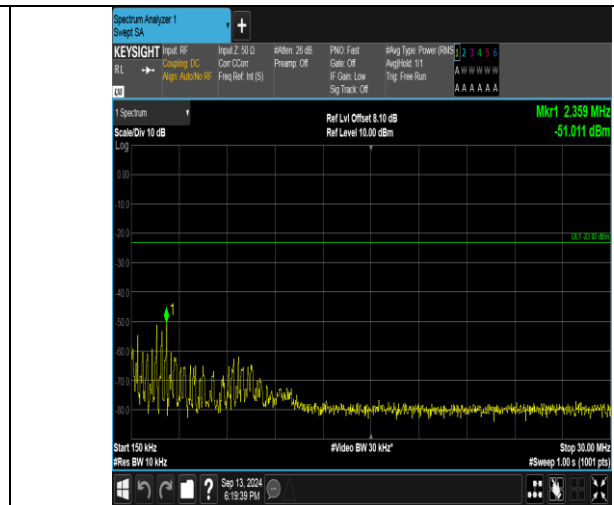
Band26_1.4MHz_QPSK_26915_1RB#0_0.15~30_0.15~30
