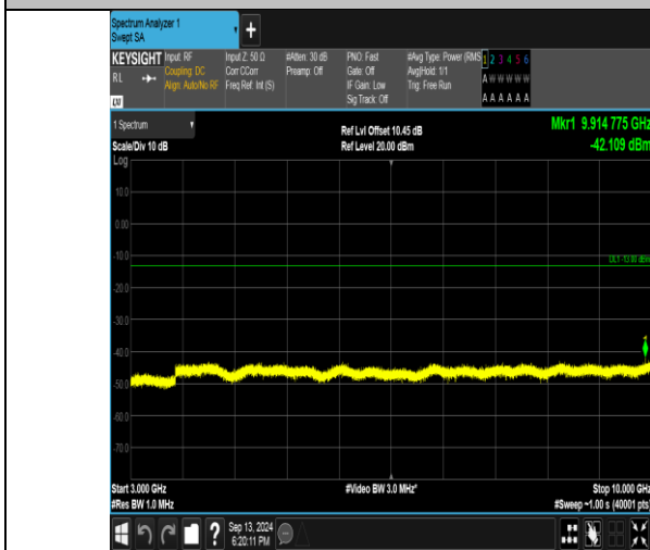
Band26_1.4MHz_QPSK_26915_1RB#0_3000~10000_3000~10000
