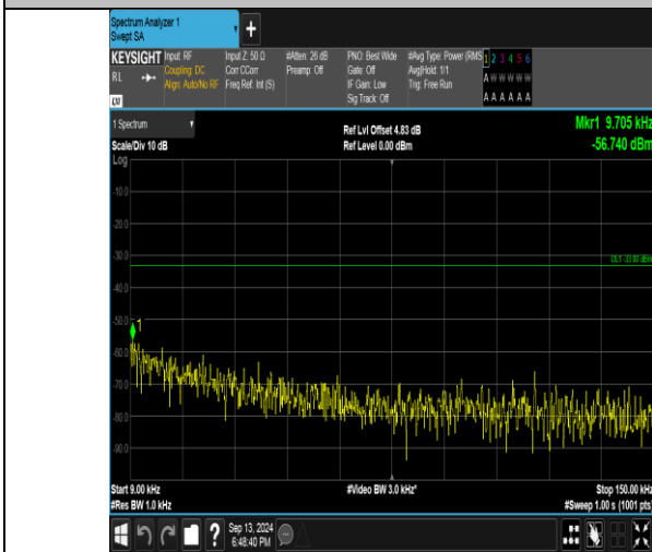
Band26_3MHz_QPSK_26805_15RB#0_0.009~0.15_0.009~0.15
