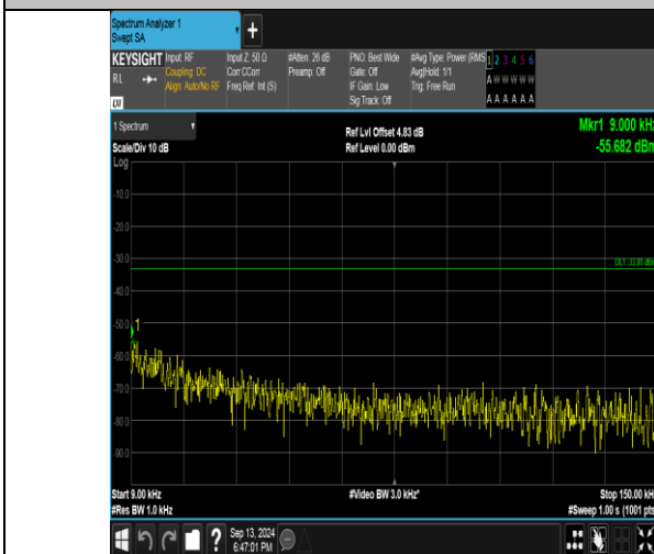
Band26_3MHz_QPSK_26805_1RB#14_0.009~0.15_0.009~0.15
