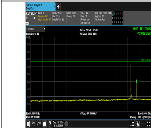
Band26_1.4MHz_QPSK_26915_1RB#0_30~1000_30~1000
