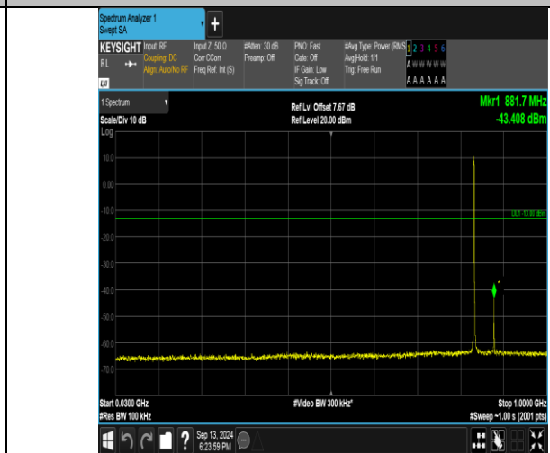
Band26_1.4MHz_16QAM_26915_6RB#0_30~1000_30~1000
