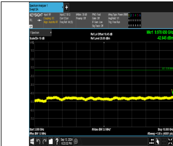
Band26_1.4MHz_QPSK_26915_6RB#0_3000~10000_3000~10000
