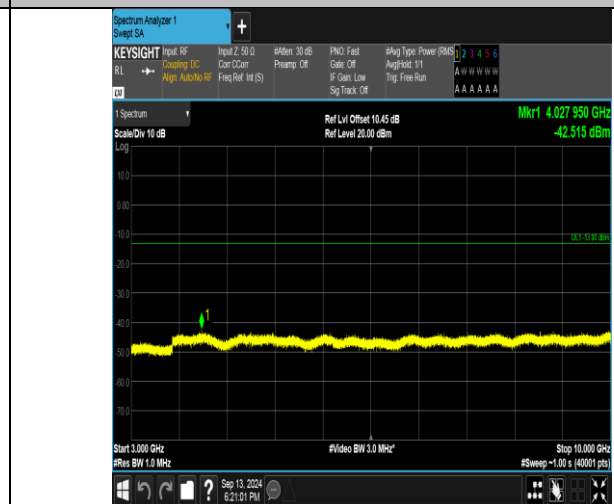
Band26_1.4MHz_16QAM_26915_1RB#0_3000~10000_3000~10000
