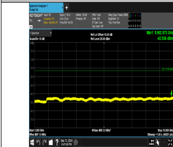
Band26_3MHz_QPSK_26805_1RB#14_3000~10000_3000~10000
