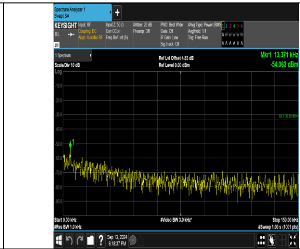
Band26_1.4MHz_16QAM_26797_6RB#0_0.009~0.15_0.009~0.15
