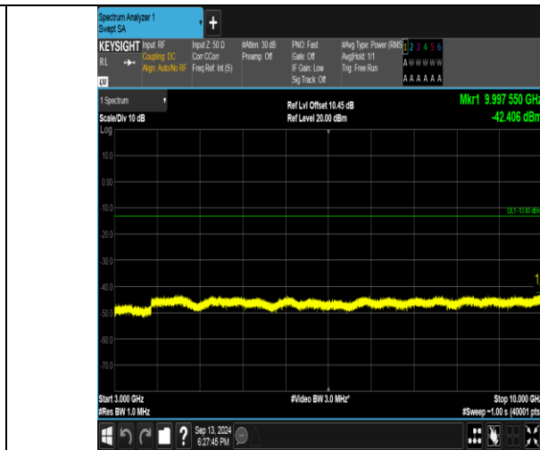
Band26_1.4MHz_16QAM_27033_1RB#5_3000~10000_3000~10000
