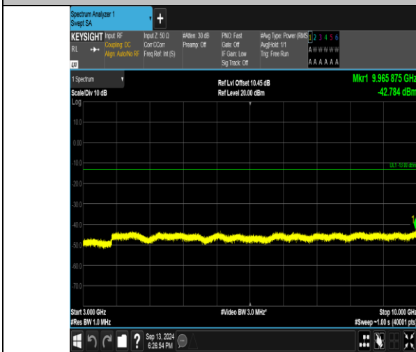
Band26_1.4MHz_QPSK_27033_1RB#5_3000~10000_3000~10000
