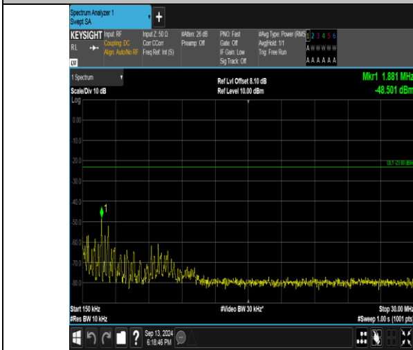
Band26_1.4MHz_16QAM_26797_6RB#0_0.15~30_0.15~30
