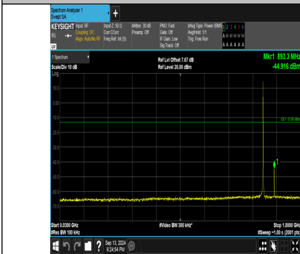
Band26_1.4MHz_QPSK_27033_1RB#0_30-1000_30-1000
