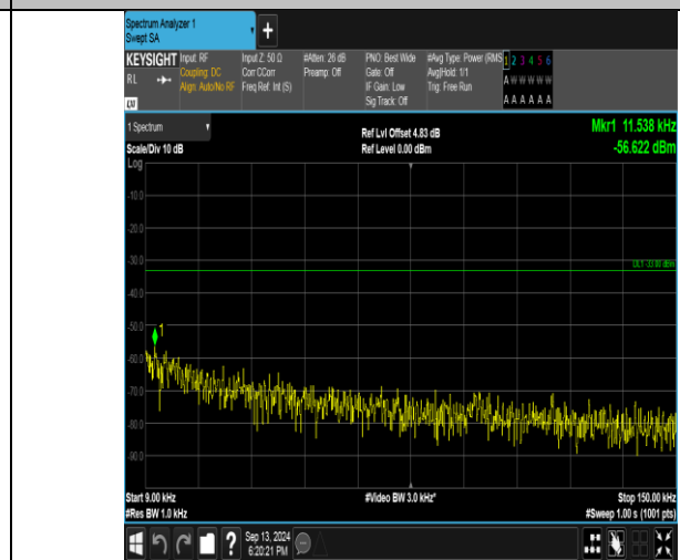
Band26_1.4MHz_16QAM_26915_1RB#0_0.009~0.15_0.009~0.15
