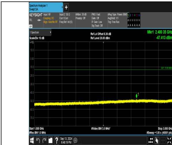
Band26_3MHz_16QAM_26805_1RB#14_1000~3000_1000~3000
