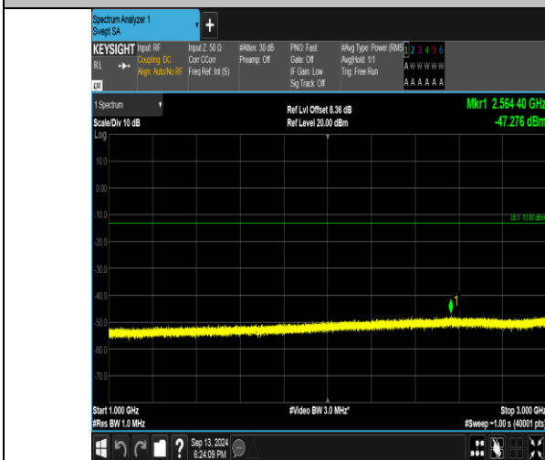
Band26_1.4MHz_16QAM_26915_6RB#0_1000~3000_1000~3000
