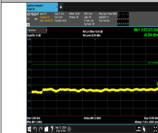
Band26_1.4MHz_QPSK_27033_1RB#0_3000-10000_3000-10000
