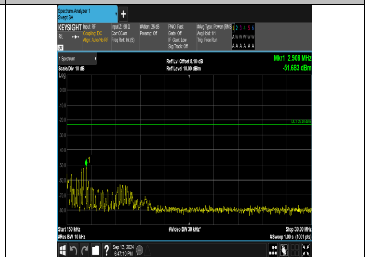
Band26_3MHz_QPSK_26805_1RB#14_0.15~30_0.15~30
