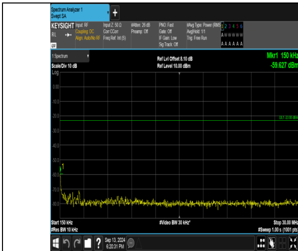
Band26_1.4MHz_16QAM_26915_1RB#0_0.15~30_0.15~30
