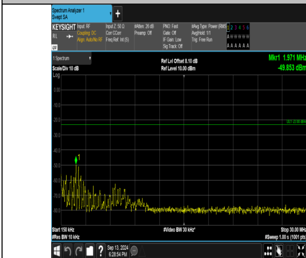
Band26_1.4MHz_16QAM_27033_6RB#0_0.15~30_0.15~30
