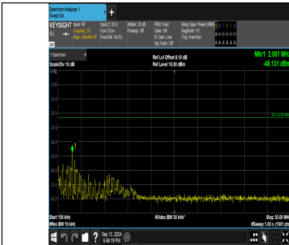
Band26_3MHz_16QAM_26805_1RB#0_0.15~30_0.15~30
