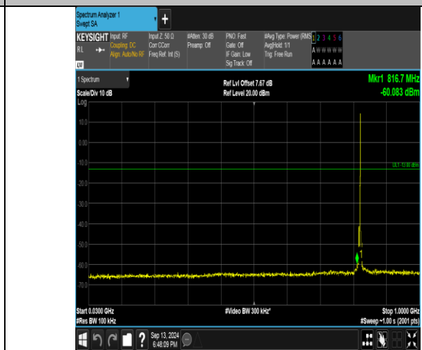
Band26_3MHz_16QAM_26805_1RB#14_30~1000_30~1000
