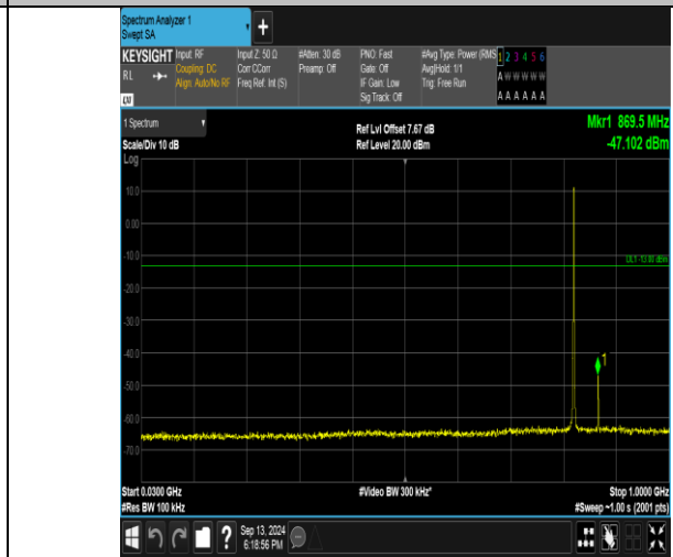
Band26_1.4MHz_16QAM_26797_6RB#0_30~1000_30~1000
