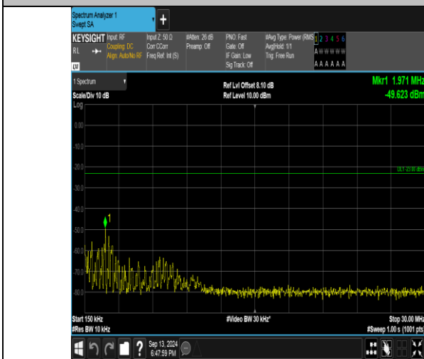
Band26_3MHz_16QAM_26805_1RB#14_0.15~30_0.15~30
