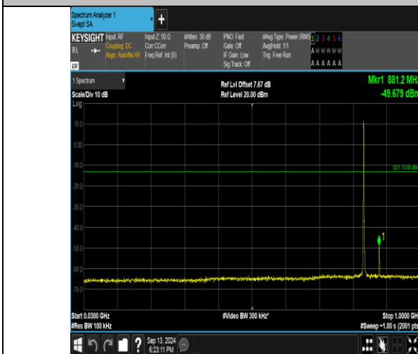
Band26_1.4MHz_QPSK_26915_6RB#0_30~1000_30~1000
