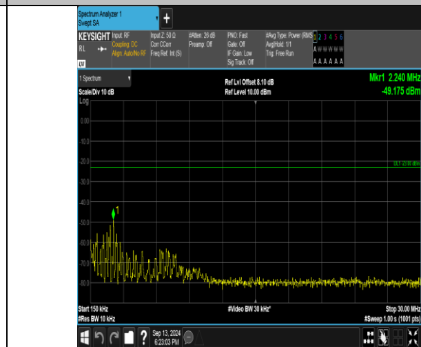
Band26_1.4MHz_QPSK_26915_6RB#0_0.15~30_0.15~30
