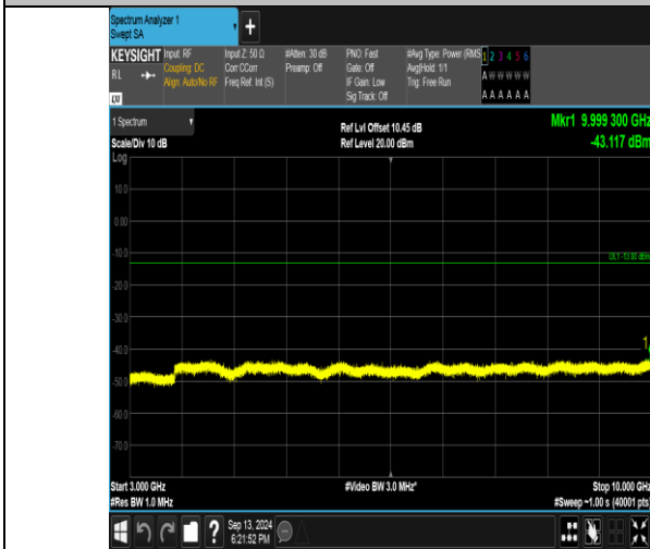
Band26_1.4MHz_QPSK_26915_1RB#5_3000~10000_3000~10000
