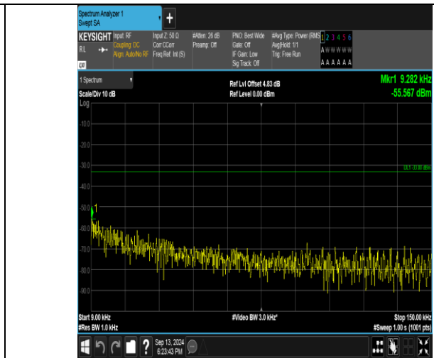
Band26_1.4MHz_16QAM_26915_6RB#0_0.009~0.15_0.009~0.15
