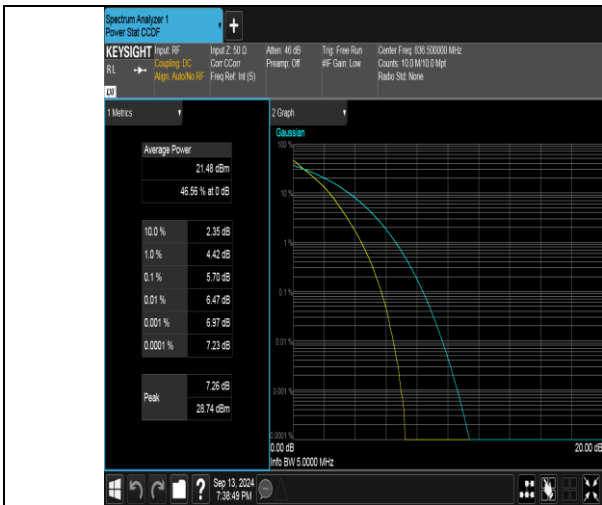
Band26(824-849)-5MHz-QPSK-26915-25RB#0-PASS
