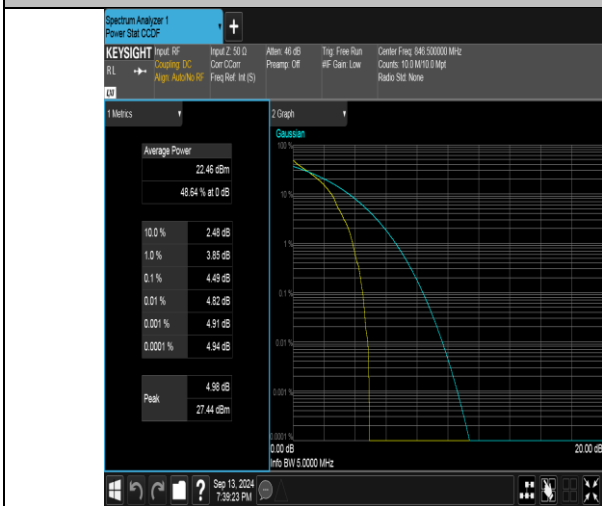
Band26(824-849)-5MHz-QPSK-27015-1RB#0-PASS
