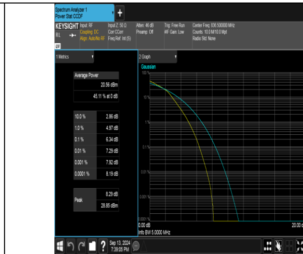
Band26(824-849)-5MHz-16QAM-26915-25RB#0-PASS
