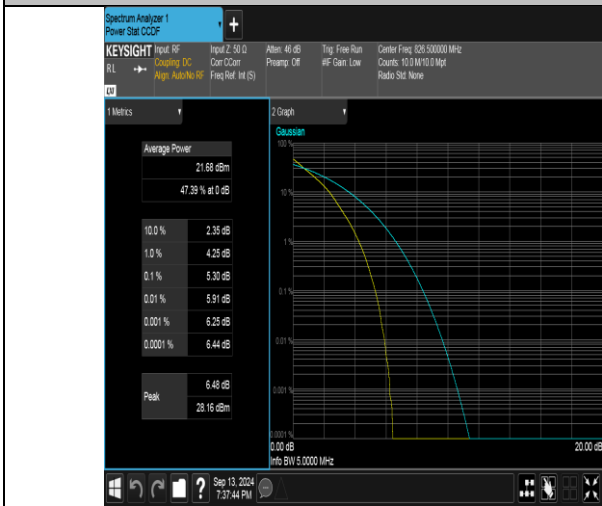
Band26(824-849)-5MHz-QPSK-26815-25RB#0-PASS
