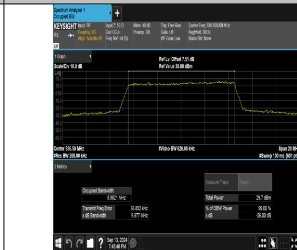
Band26(824-849)-10MHz-16QAM-26915-50RB#0-PASS
