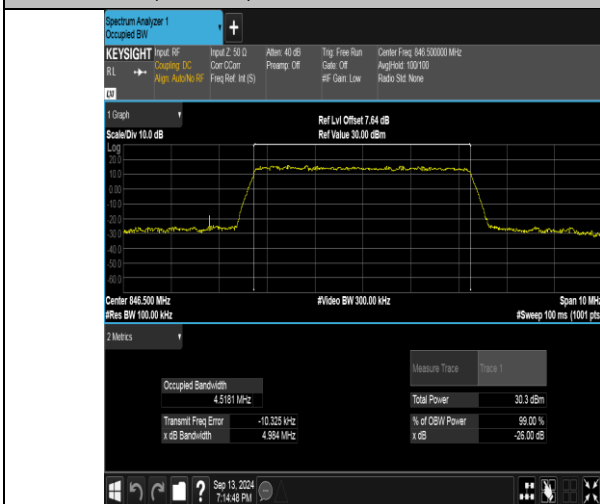
Band26(824-849)-5MHz-QPSK-27015-25RB#0-PASS
