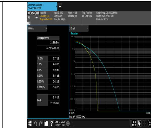
Band26(824-849)-10MHz-16QAM-26840-1RB#0-PASS
