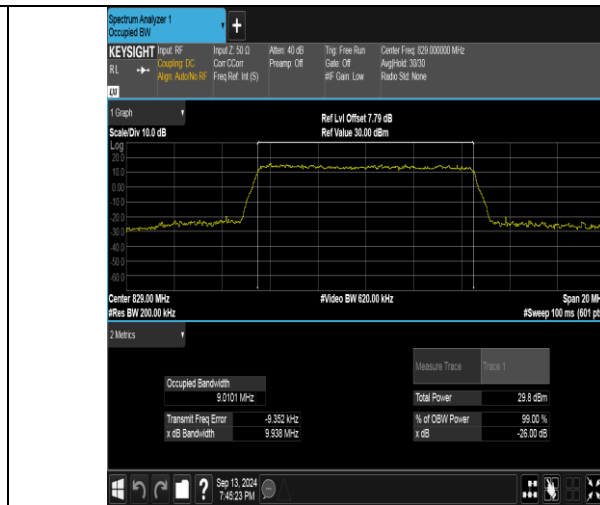
Band26(824-849)-10MHz-16QAM-26840-50RB#0-PASS
