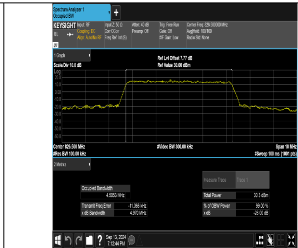
Band26(824-849)-5MHz-16QAM-26815-25RB#0-PASS
