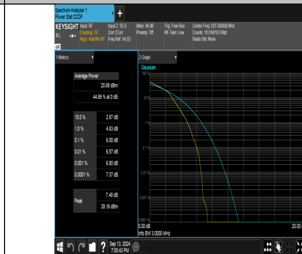
Band26(824-849)-3MHz-16QAM-26805-15RB#0-PASS
