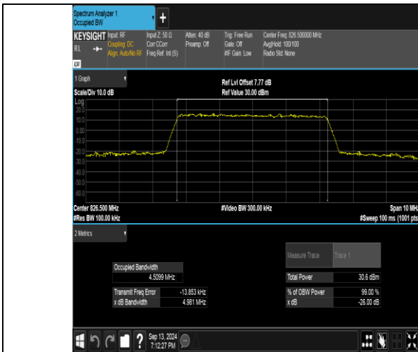
Band26(824-849)-5MHz-QPSK-26815-25RB#0-PASS
