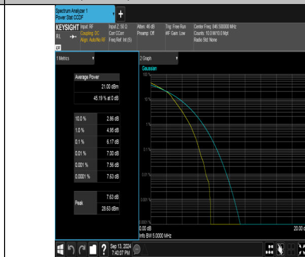
Band26(824-849)-5MHz-16QAM-27015-25RB#0-PASS
