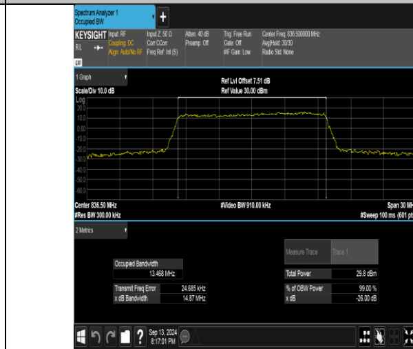
Band26(824-849)-15MHz-16QAM-26915-75RB#0-PASS
