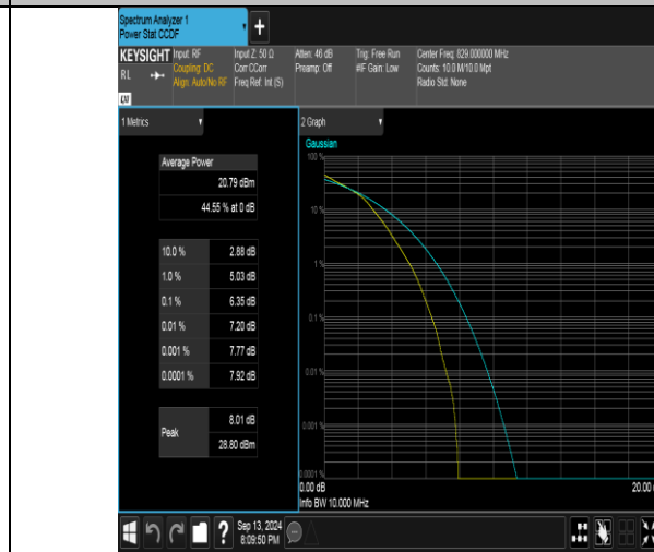
Band26(824-849)-10MHz-16QAM-26840-50RB#0-PASS
