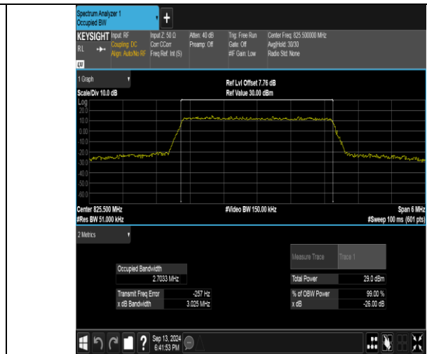
Band26(824-849)-3MHz-16QAM-26805-15RB#0-PASS
