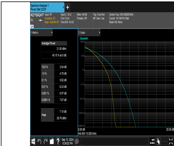
Band26(824-849)-15MHz-QPSK-26915-75RB#0-PASS
