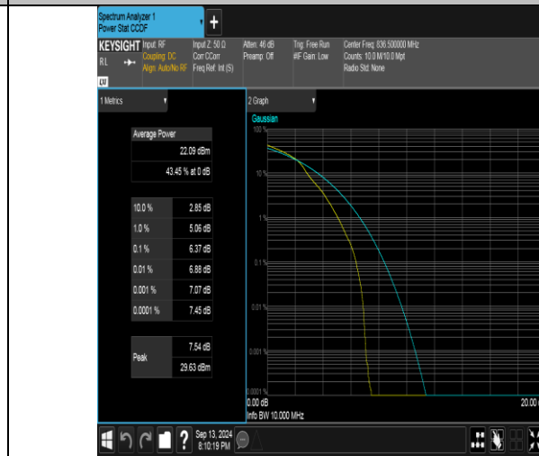
Band26(824-849)-10MHz-16QAM-26915-1RB#0-PASS
