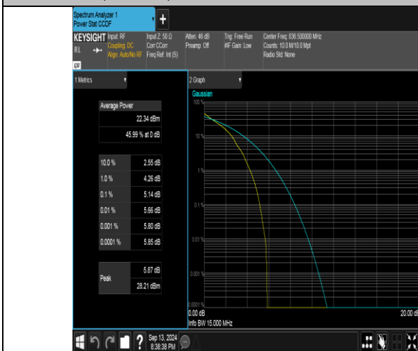
Band26(824-849)-15MHz-QPSK-26915-1RB#0-PASS
