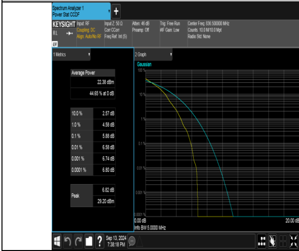
Band26(824-849)-5MHz-QPSK-26915-1RB#0-PASS
