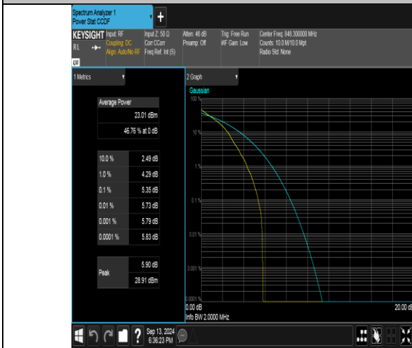
Band26(824-849)-1.4MHz-QPSK-27033-1RB#0-PASS
