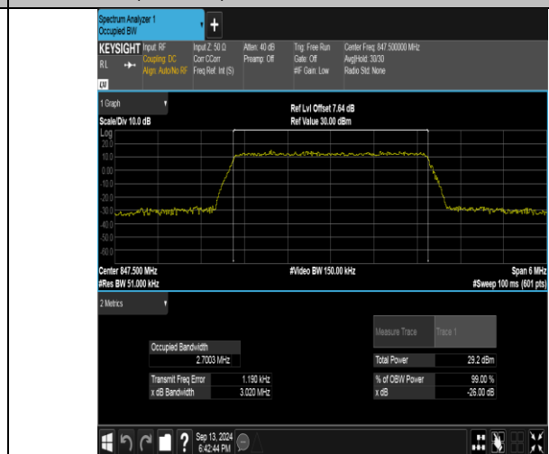
Band26(824-849)-3MHz-16QAM-27025-15RB#0-PASS
