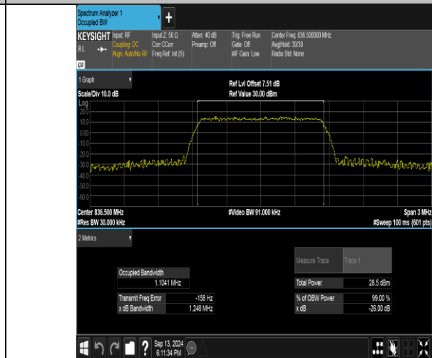
Band26(824-849)-1.4MHz-16QAM-26915-6RB#0-PASS
