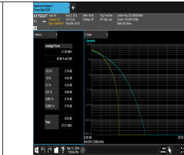
Band26(824-849)-3MHz-16QAM-26805-1RB#0-PASS
