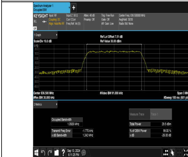
Band26(824-849)-1.4MHz-QPSK-26915-6RB#0-PASS
