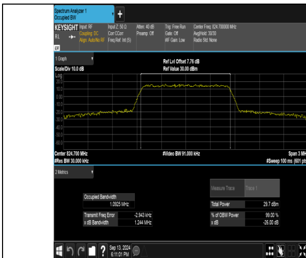
Band26(824-849)-1.4MHz-QPSK-26797-6RB#0-PASS
