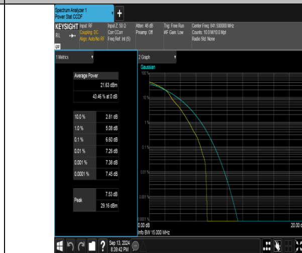
Band26(824-849)-15MHz-16QAM-26965-1RB#0-PASS
