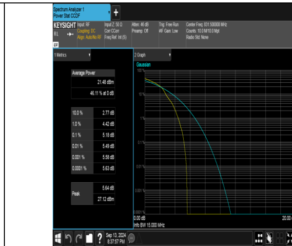
Band26(824-849)-15MHz-16QAM-26865-1RB#0-PASS
