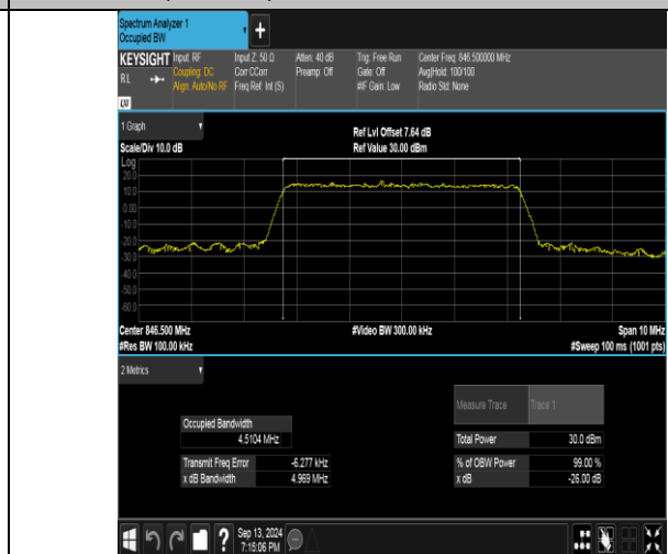
Band26(824-849)-5MHz-16QAM-27015-25RB#0-PASS
