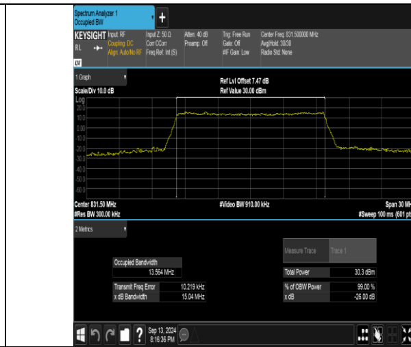
Band26(824-849)-15MHz-16QAM-26865-75RB#0-PASS
