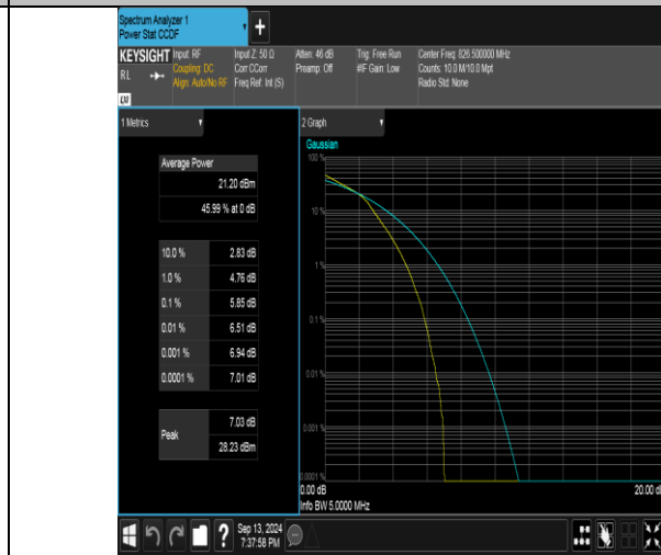
Band26(824-849)-5MHz-16QAM-26815-25RB#0-PASS
