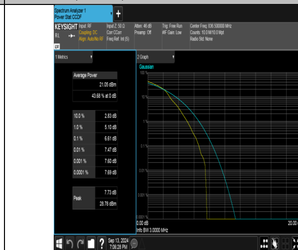
Band26(824-849)-3MHz-16QAM-26915-1RB#0-PASS
