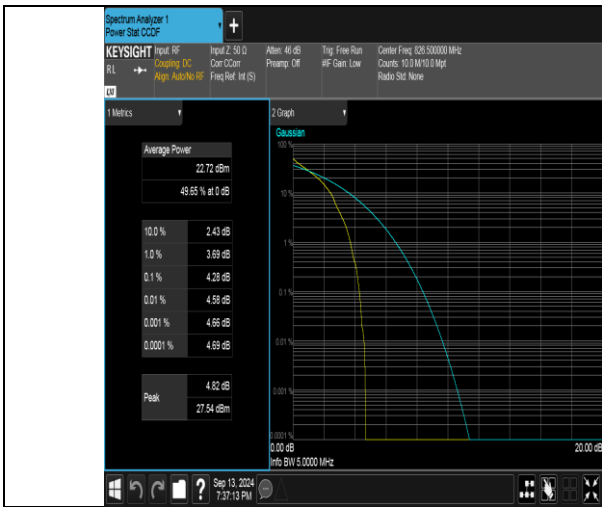
Band26(824-849)-5MHz-QPSK-26815-1RB#0-PASS
