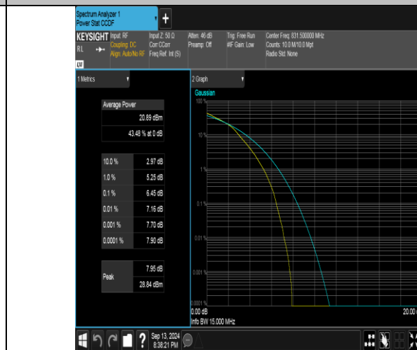
Band26(824-849)-15MHz-16QAM-26865-75RB#0-PASS
