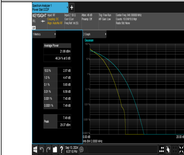
Band26(824-849)-1.4MHz-QPSK-27033-6RB#0-PASS
