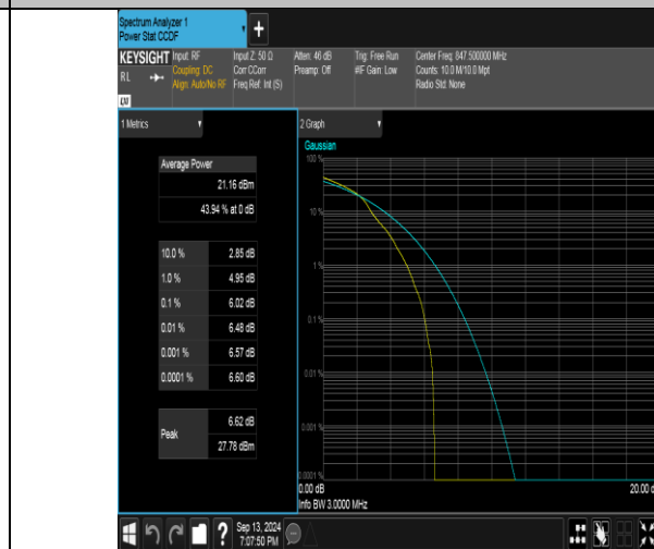
Band26(824-849)-3MHz-16QAM-27025-1RB#0-PASS
