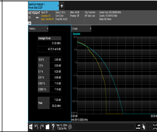
Band26(824-849)-5MHz-16QAM-26915-1RB#0-PASS
