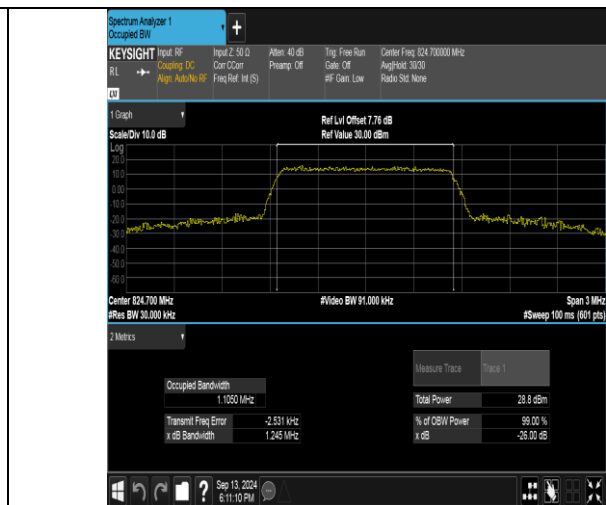
Band26(824-849)-1.4MHz-16QAM-26797-6RB#0-PASS
