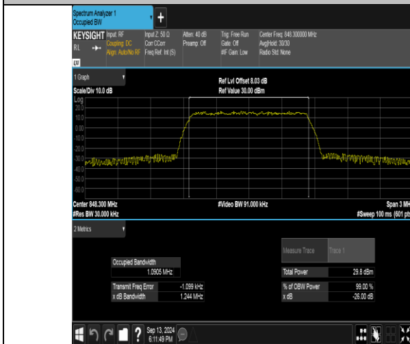
Band26(824-849)-1.4MHz-QPSK-27033-6RB#0-PASS
