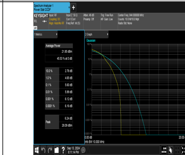
Band26(824-849)-10MHz-16QAM-26990-1RB#0-PASS
