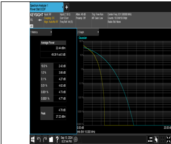
Band26(824-849)-15MHz-QPSK-26865-1RB#0-PASS
