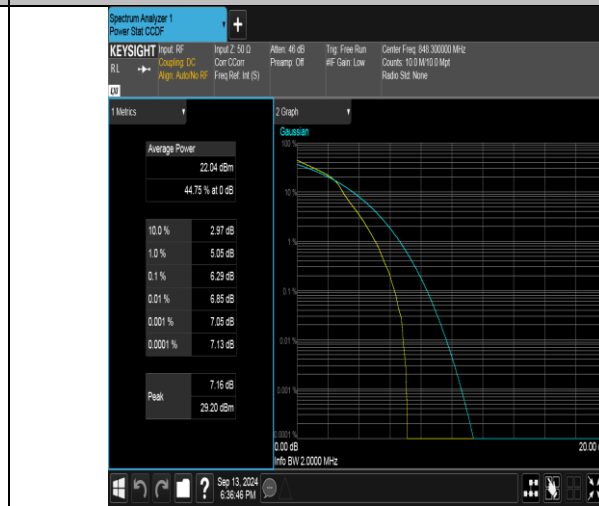
Band26(824-849)-1.4MHz-16QAM-27033-1RB#0-PASS
