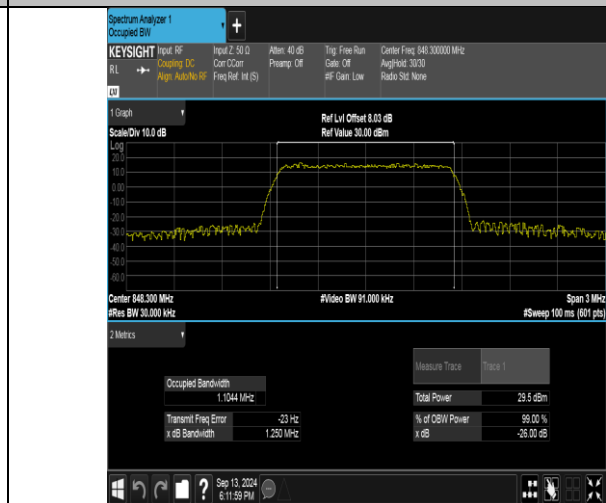
Band26(824-849)-1.4MHz-16QAM-27033-6RB#0-PASS
