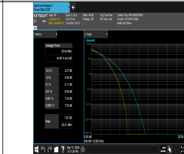
Band26(824-849)-10MHz-16QAM-26990-50RB#0-PASS
