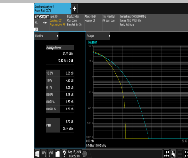
Band26(824-849)-15MHz-16QAM-26915-1RB#0-PASS
