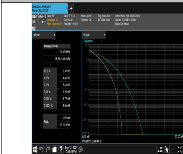
Band26(824-849)-5MHz-QPSK-27015-25RB#0-PASS
