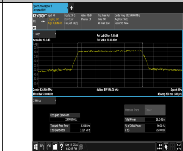
Band26(824-849)-3MHz-16QAM-26915-15RB#0-PASS
