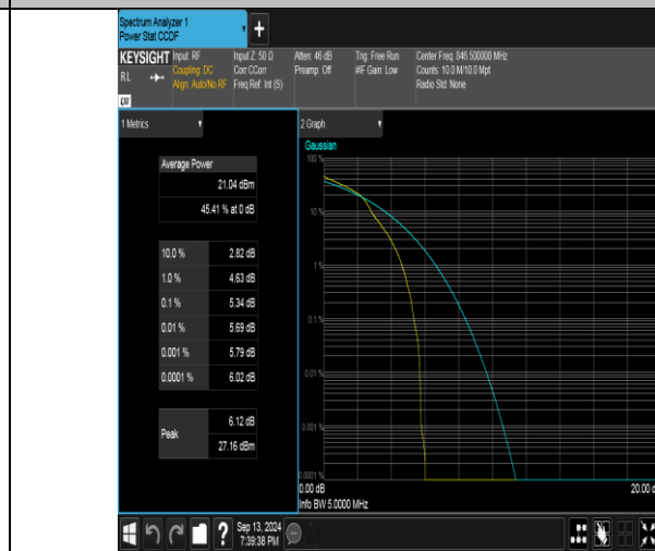
Band26(824-849)-5MHz-16QAM-27015-1RB#0-PASS
