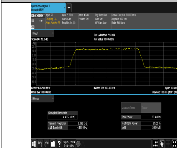
Band26(824-849)-5MHz-QPSK-26915-25RB#0-PASS
