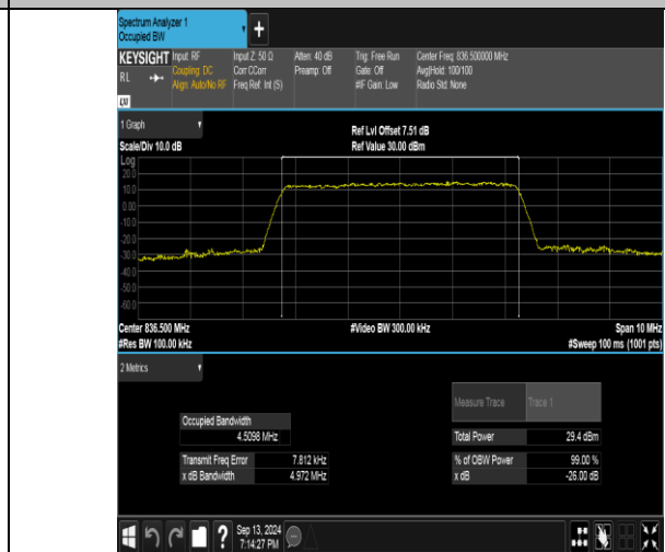
Band26(824-849)-5MHz-16QAM-26915-25RB#0-PASS
