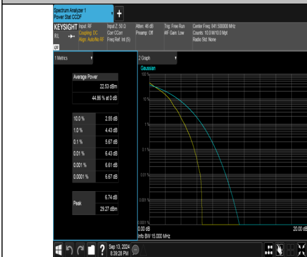
Band26(824-849)-15MHz-QPSK-26965-1RB#0-PASS
