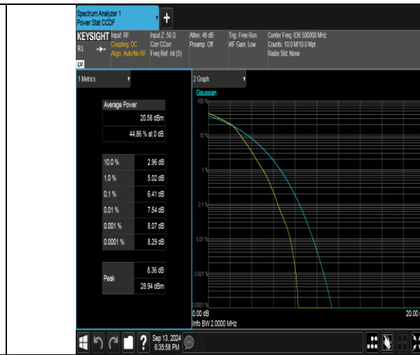
Band26(824-849)-1.4MHz-16QAM-26915-6RB#0-PASS
