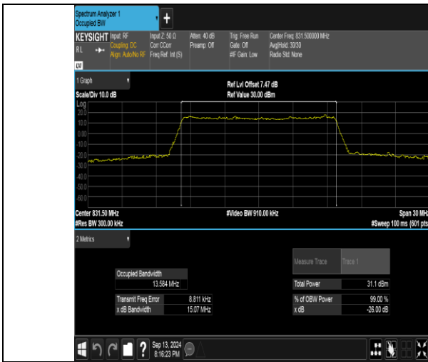
Band26(824-849)-15MHz-QPSK-26865-75RB#0-PASS
