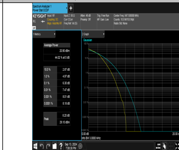
Band26(824-849)-3MHz-16QAM-27025-15RB#0-PASS
