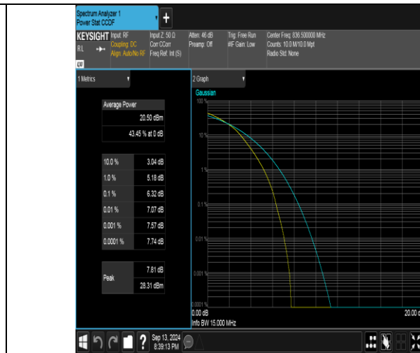
Band26(824-849)-15MHz-16QAM-26915-75RB#0-PASS
