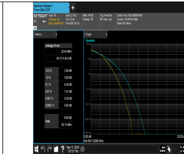
Band26(824-849)-3MHz-16QAM-26915-15RB#0-PASS
