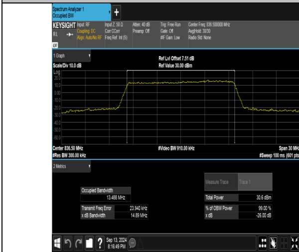
Band26(824-849)-15MHz-QPSK-26915-75RB#0-PASS
