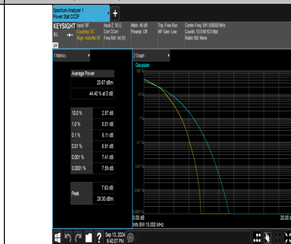
Band26(824-849)-15MHz-16QAM-26965-75RB#0-PASS
