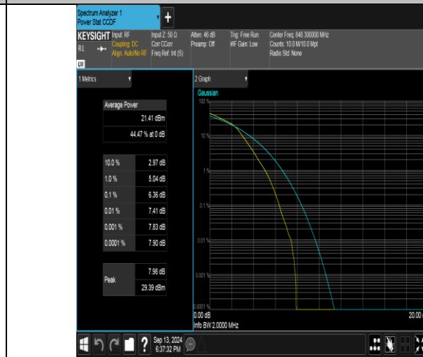
Band26(824-849)-1.4MHz-16QAM-27033-6RB#0-PASS
