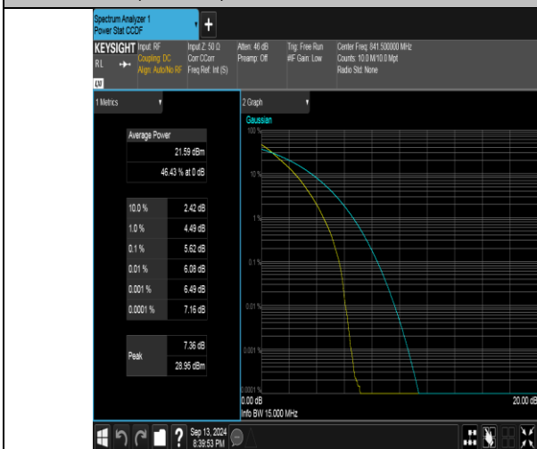
Band26(824-849)-15MHz-QPSK-26965-75RB#0-PASS
