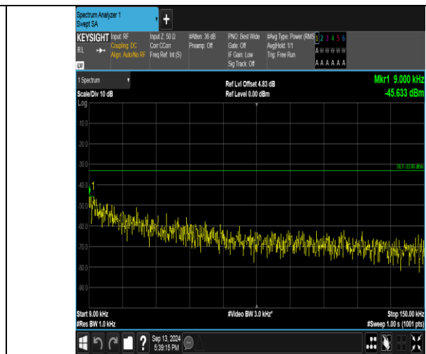
Band26_5MHz_16QAM_26715_25RB#0_0.009-0.15_0.009-0.15
