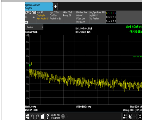
Band26_5MHz_QPSK_26715_1RB#24_0.009-0.15_0.009-0.15
