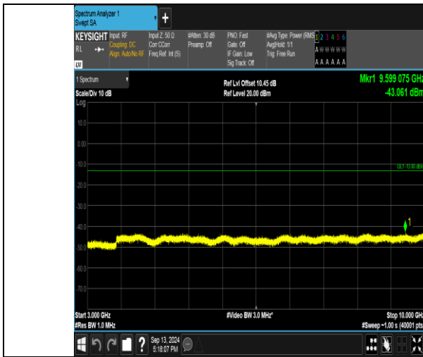
Band26_3MHz_QPSK_26775_15RB#0_3000-10000_3000-10000
