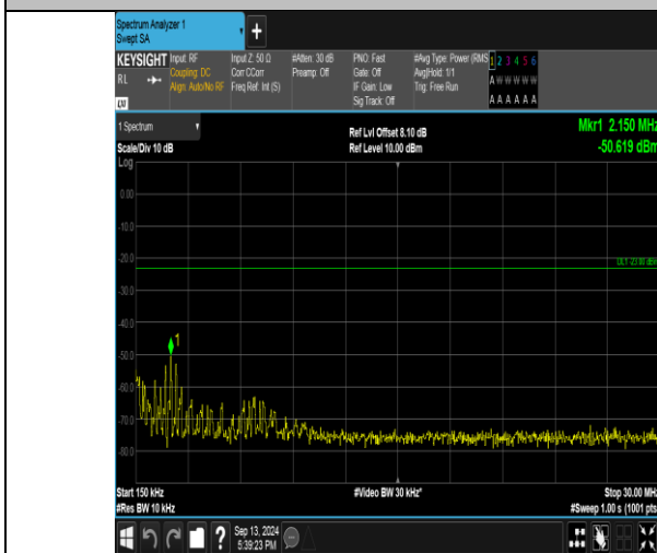
Band26_5MHz_16QAM_26715_25RB#0_0.15-30_0.15-30
