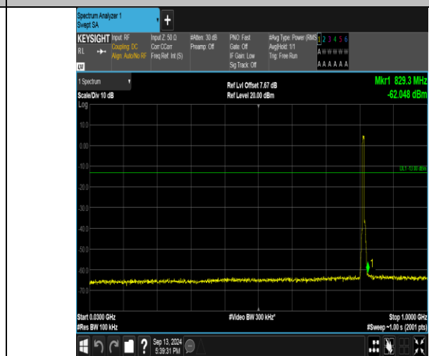
Band26_5MHz_16QAM_26715_25RB#0_30-1000_30-1000
