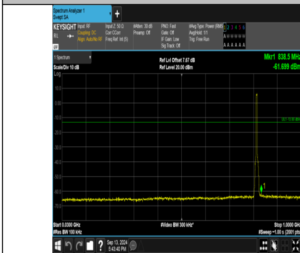
Band26_5MHz_QPSK_26740_25RB#0_30-1000_30-1000
