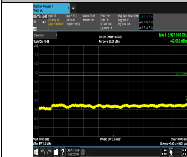
Band26_5MHz_QPSK_26740_1RB#24_3000~10000_3000~10000
