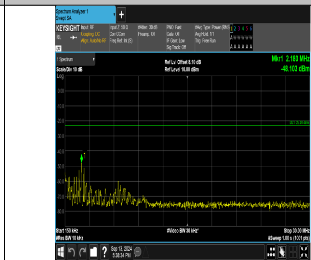
Band26_5MHz_QPSK_26715_25RB#0_0.15-30_0.15-30
