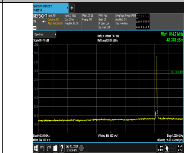
Band26_3MHz_16QAM_26775_15RB#0_30-1000_30-1000
