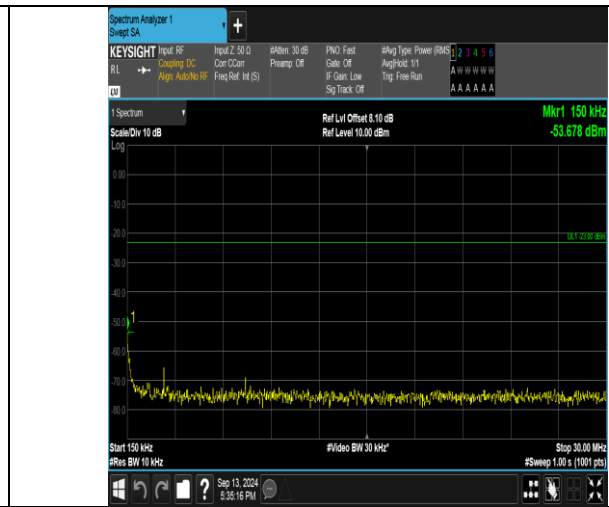
Band26_5MHz_QPSK_26715_1RB#0_0.15-30_0.15-30
