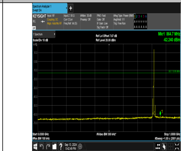
Band26_5MHz_16QAM_26740_1RB#24_30~1000_30~1000
