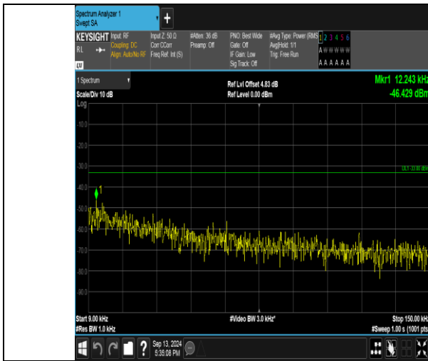
Band26_5MHz_QPSK_26715_1RB#0_0.009-0.15_0.009-0.15
