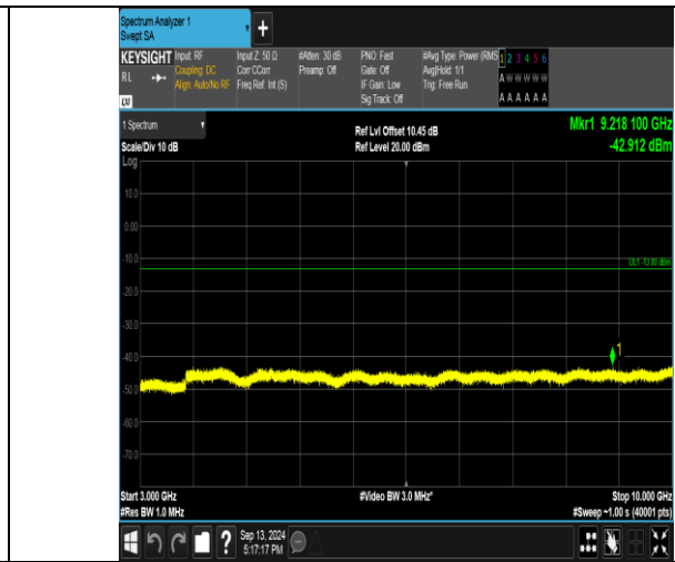
Band26_3MHz_16QAM_26775_1RB#14_3000-10000_3000-10000
