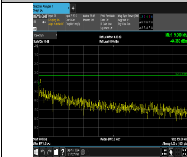
Band26_3MHz_QPSK_26775_15RB#0_0.009-0.15_0.009-0.15
