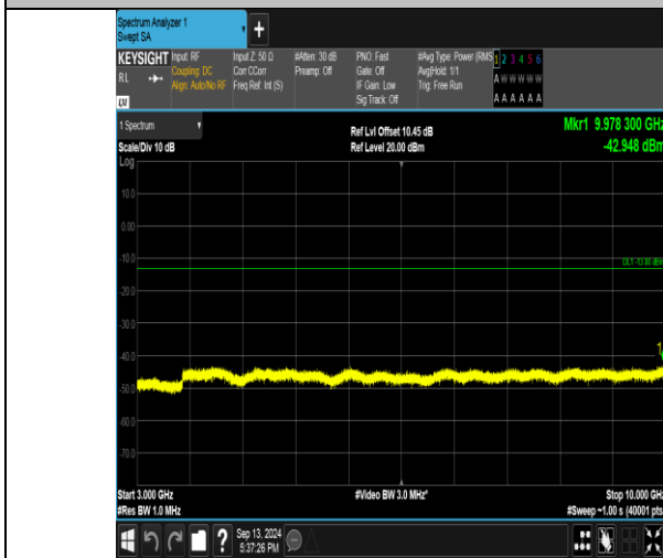
Band26_5MHz_QPSK_26715_1RB#24_3000~10000_3000~10000
