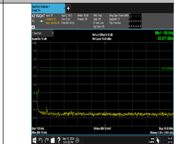
Band26_5MHz_QPSK_26740_1RB#24_0.15-30_0.15-30
