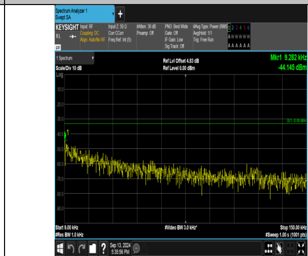
Band26_5MHz_16QAM_26715_1RB#0_0.009-0.15_0.009-0.15
