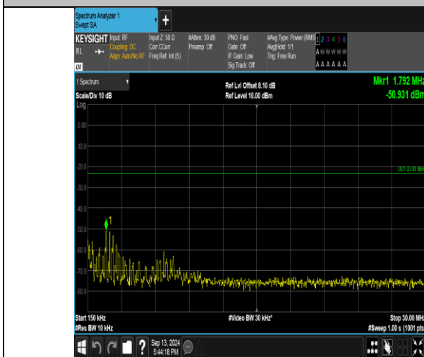
Band26_5MHz_16QAM_26740_25RB#0_0.15-30_0.15-30
