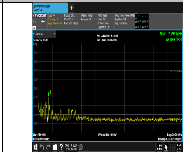
Band26_3MHz_QPSK_26775_15RB#0_0.15-30_0.15-30
