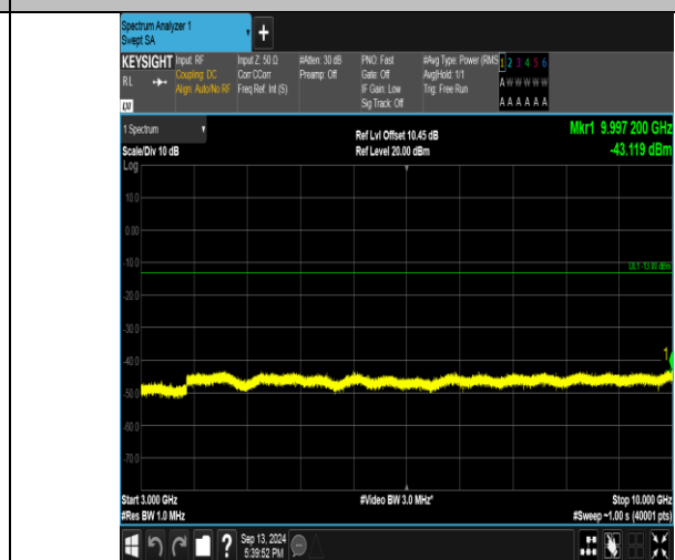
Band26_5MHz_16QAM_26715_25RB#0_3000-10000_3000-10000
