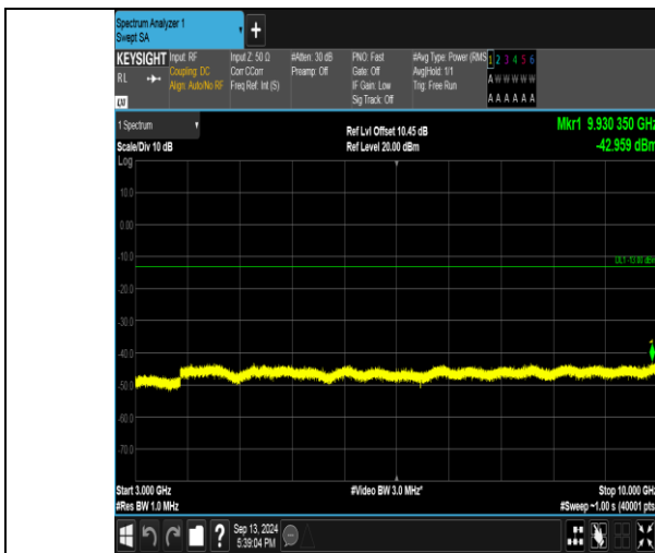
Band26_5MHz_QPSK_26715_25RB#0_3000-10000_3000-10000
