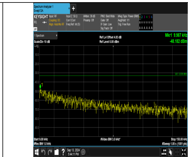
Band26_5MHz_16QAM_26740_25RB#0_0.009-0.15_0.009-0.15
