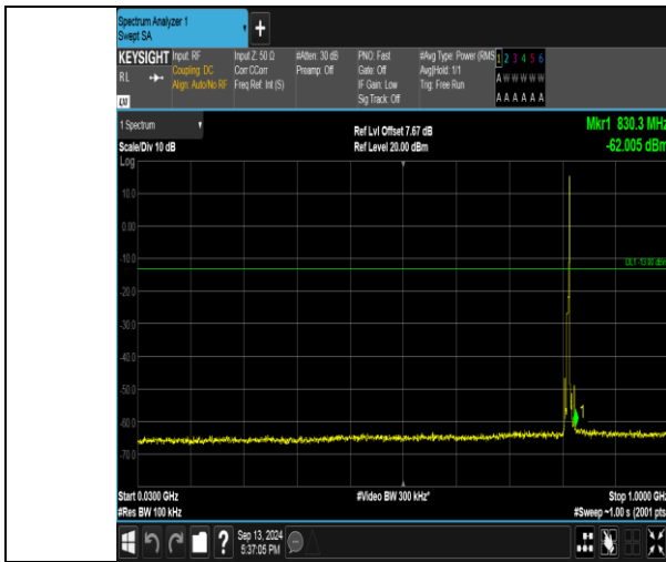
Band26_5MHz_QPSK_26715_1RB#24_30~1000_30~1000
