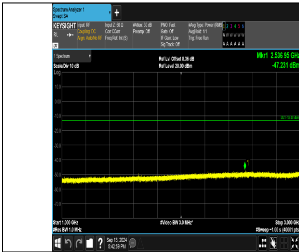
Band26_5MHz_16QAM_26740_1RB#24_1000-3000_1000-3000
