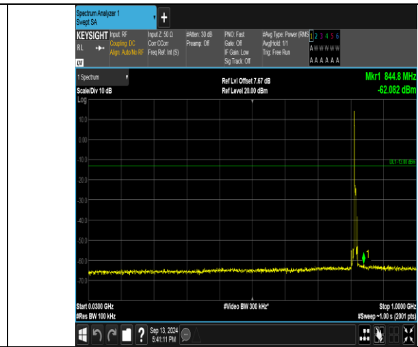
Band26_5MHz_16QAM_26740_1RB#0_30-1000_30-1000
