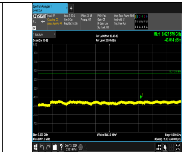
Band26_5MHz_16QAM_26715_1RB#24_3000-10000_3000-10000
