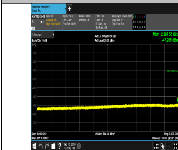
Band26_5MHz_16QAM_26715_25RB#0_1000-3000_1000-3000
