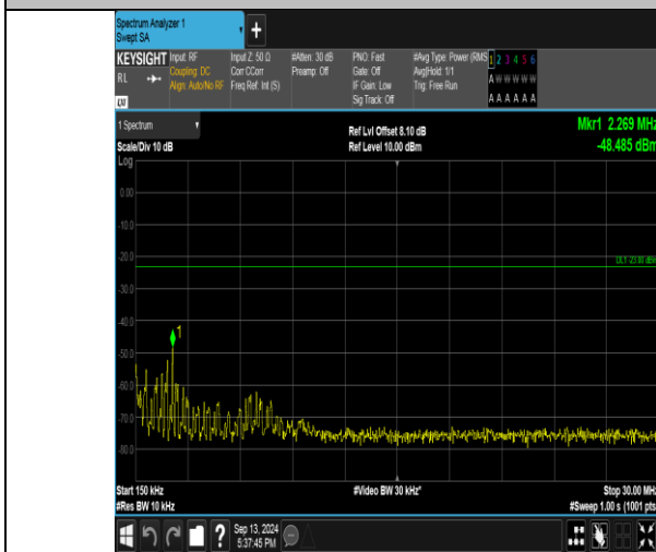
Band26_5MHz_16QAM_26715_1RB#24_0.15~30_0.15~30
