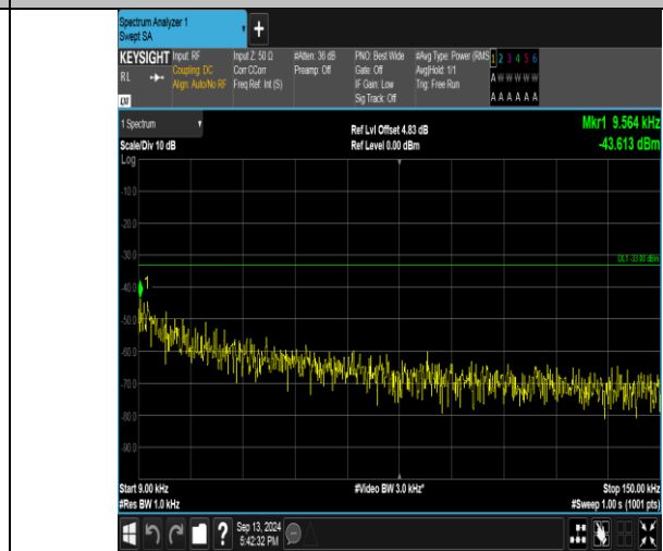
Band26_5MHz_16QAM_26740_1RB#24_0.009~0.15_0.009~0.15
