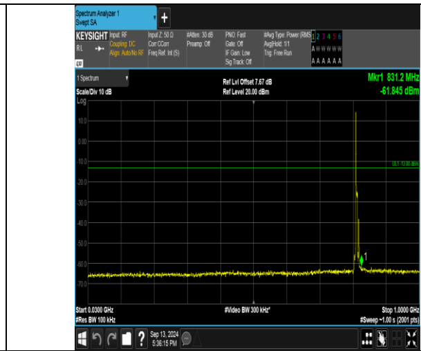
Band26_5MHz_16QAM_26715_1RB#0_30-1000_30-1000
