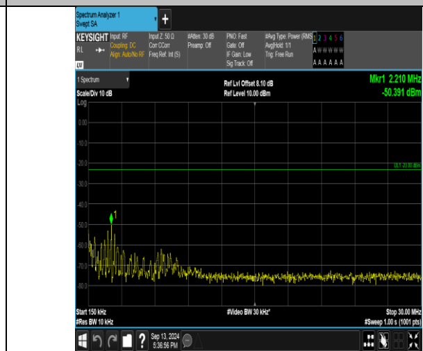
Band26_5MHz_QPSK_26715_1RB#24_0.15-30_0.15-30
