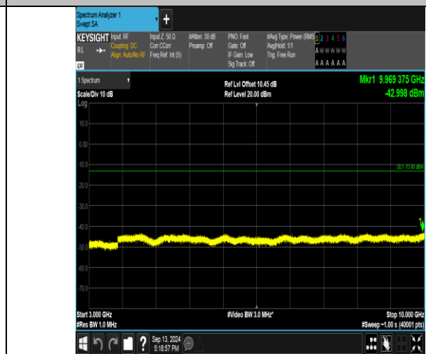
Band26_3MHz_16QAM_26775_15RB#0_3000-10000_3000-10000
