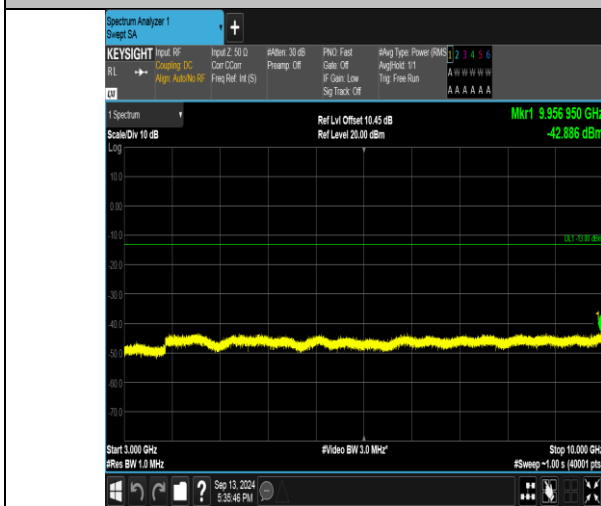
Band26_5MHz_QPSK_26715_1RB#0_3000-10000_3000-10000
