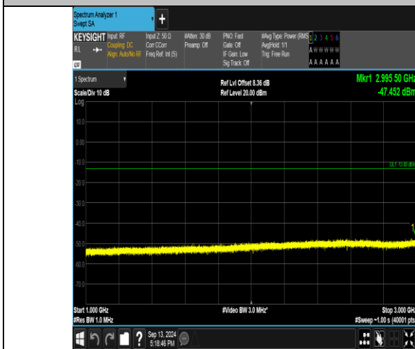
Band26_3MHz_16QAM_26775_15RB#0_1000-3000_1000-3000
