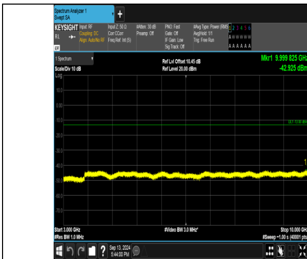
Band26_5MHz_QPSK_26740_25RB#0_3000-10000_3000-10000
