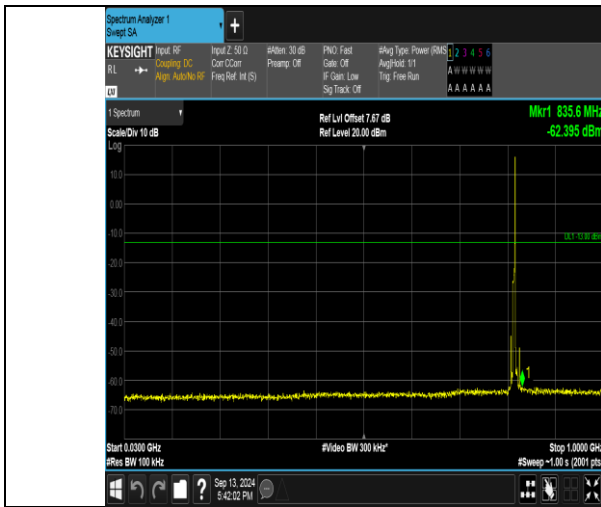
Band26_5MHz_QPSK_26740_1RB#24_30~1000_30~1000
