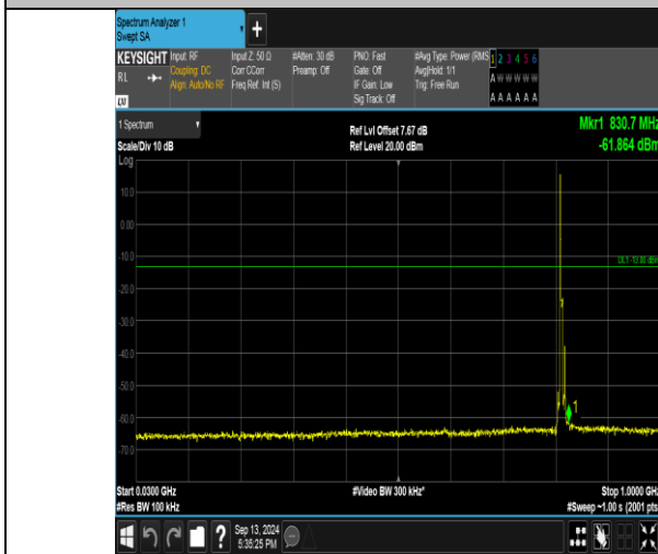
Band26_5MHz_QPSK_26715_1RB#0_30-1000_30-1000
