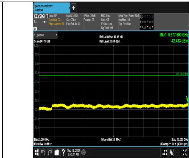
Band26_5MHz_16QAM_26740_1RB#24_3000-10000_3000-10000
