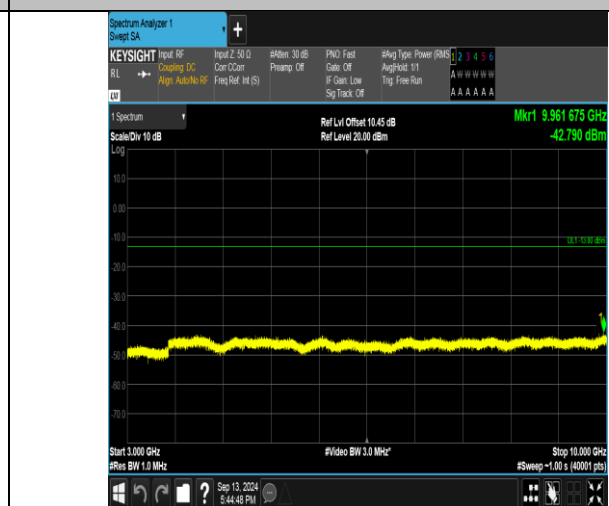
Band26_5MHz_16QAM_26740_25RB#0_3000-10000_3000-10000
