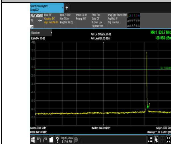
Band26_3MHz_QPSK_26775_15RB#0_30-1000_30-1000
