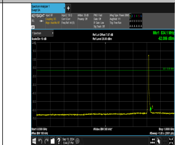
Band26_5MHz_16QAM_26740_25RB#0_30-1000_30-1000
