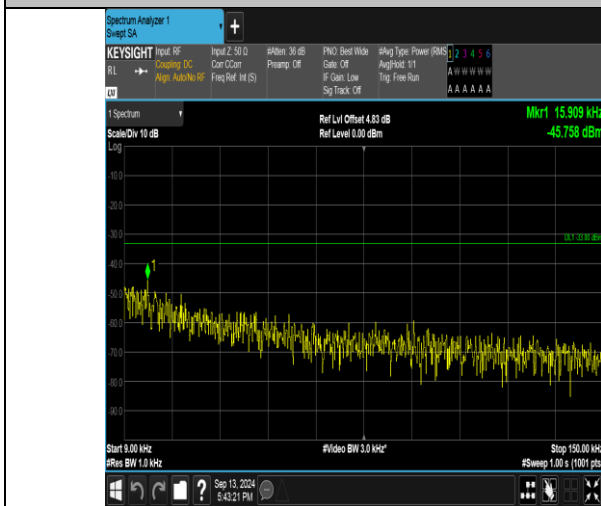
Band26_5MHz_QPSK_26740_25RB#0_0.009-0.15_0.009-0.15
