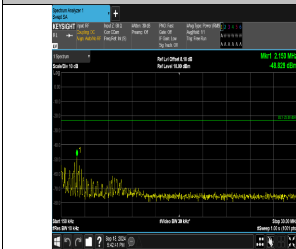
Band26_5MHz_16QAM_26740_1RB#24_0.15~30_0.15~30
