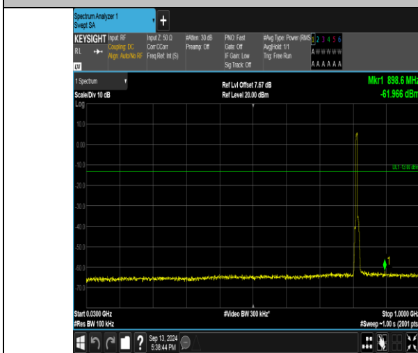
Band26_5MHz_QPSK_26715_25RB#0_30-1000_30-1000
