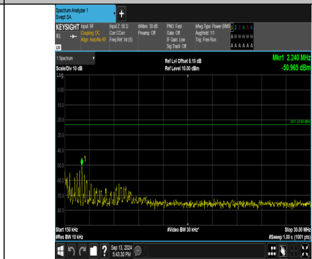
Band26_5MHz_QPSK_26740_25RB#0_0.15-30_0.15-30
