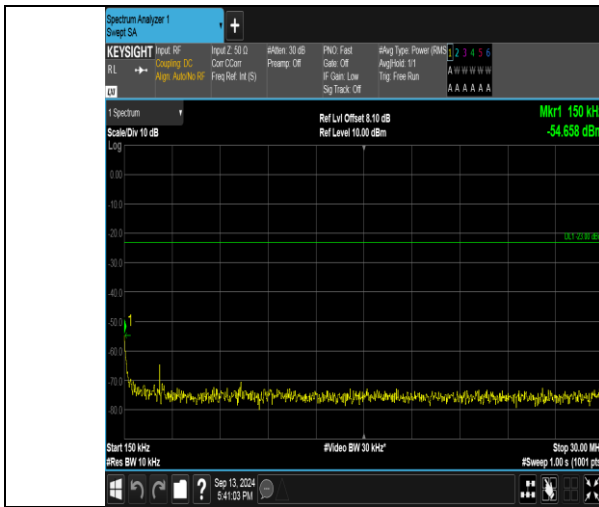
Band26_5MHz_16QAM_26740_1RB#0_0.15-30_0.15-30
