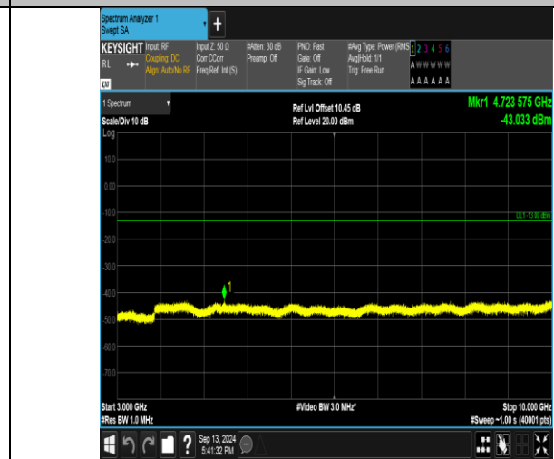
Band26_5MHz_16QAM_26740_1RB#0_3000-10000_3000-10000
