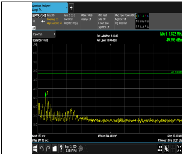
Band26_5MHz_16QAM_26715_1RB#0_0.15-30_0.15-30
