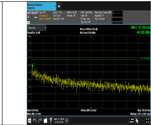
Band26_3MHz_16QAM_26775_15RB#0_0.009-0.15_0.009-0.15
