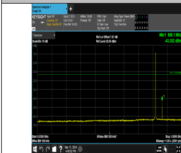
Band26_1.4MHz_QPSK_26783_6RB#0_30-1000_30-1000
