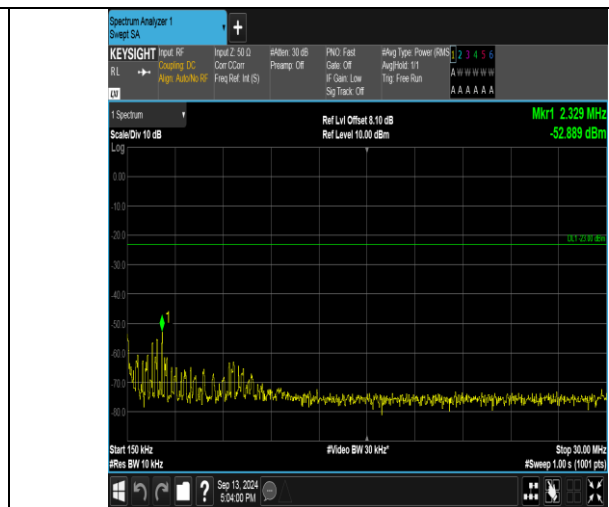
Band26_3MHz_QPSK_26705_1RB#0_0.15-30_0.15-30
