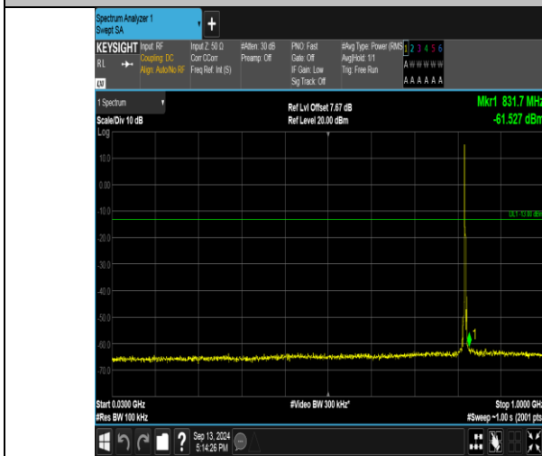
Band26_3MHz_QPSK_26775_1RB#0_30-1000_30-1000
