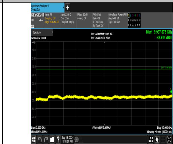
Band26_3MHz_16QAM_26740_1RB#0_3000-10000_3000-10000
