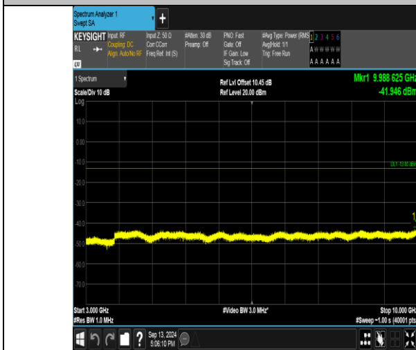
Band26_3MHz_QPSK_26705_1RB#14_3000~10000_3000~10000
