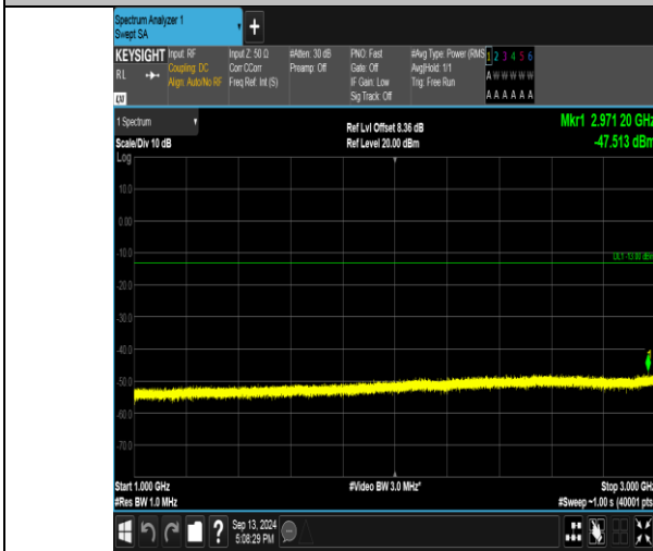
Band26_3MHz_16QAM_26705_15RB#0_1000-3000_1000-3000
