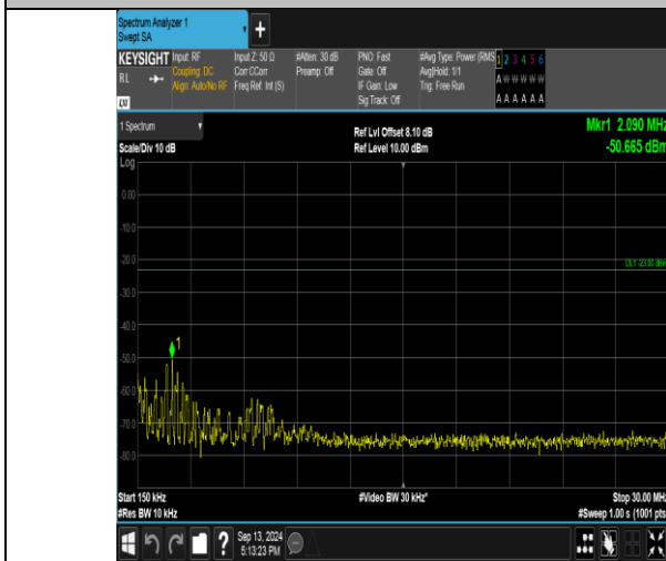
Band26_3MHz_16QAM_26740_15RB#0_0.15-30_0.15-30
