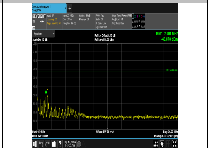
Band26_3MHz_QPSK_26740_15RB#0_0.15-30_0.15-30
