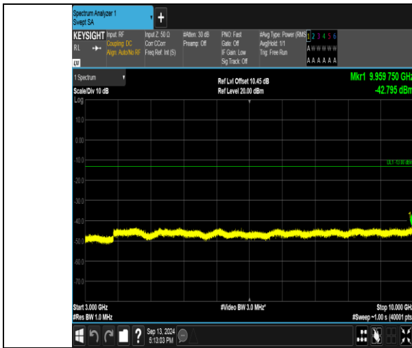
Band26_3MHz_QPSK_26740_15RB#0_3000-10000_3000-10000
