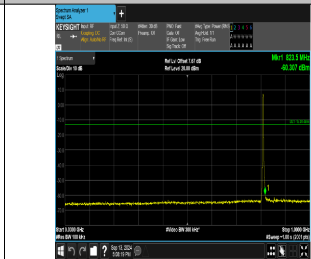
Band26_3MHz_16QAM_26705_15RB#0_30-1000_30-1000
