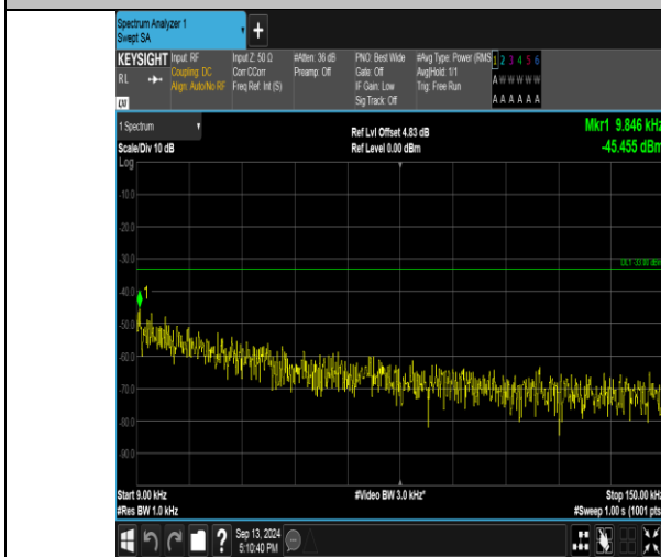
Band26_3MHz_QPSK_26740_1RB#14_0.009-0.15_0.009-0.15
