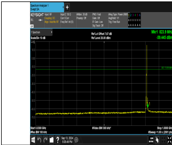
Band26_3MHz_QPSK_26705_1RB#14_30~1000_30~1000
