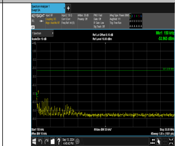
Band26_1.4MHz_QPSK_26783_6RB#0_0.15-30_0.15-30
