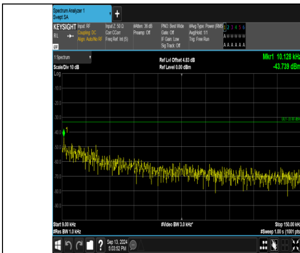
Band26_3MHz_QPSK_26705_1RB#0_0.009-0.15_0.009-0.15
