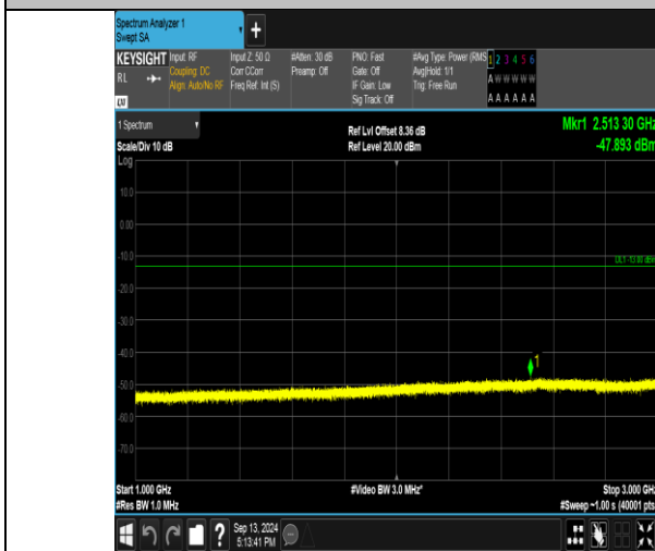
Band26_3MHz_16QAM_26740_15RB#0_1000-3000_1000-3000
