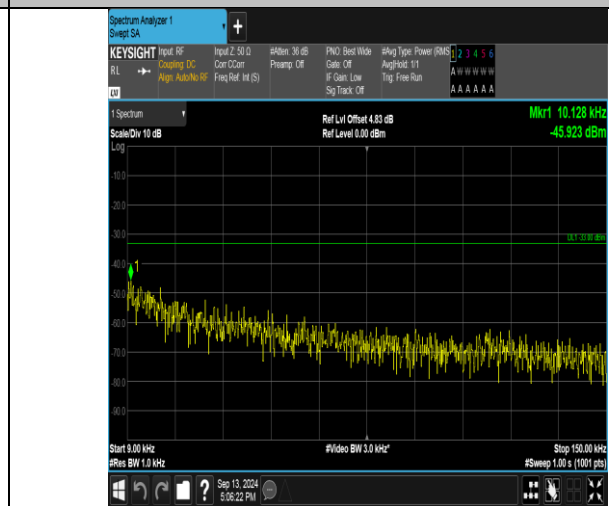
Band26_3MHz_16QAM_26705_1RB#14_0.009~0.15_0.009~0.15
