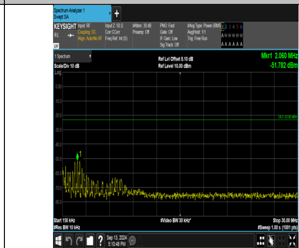
Band26_3MHz_QPSK_26740_1RB#14_0.15-30_0.15-30
