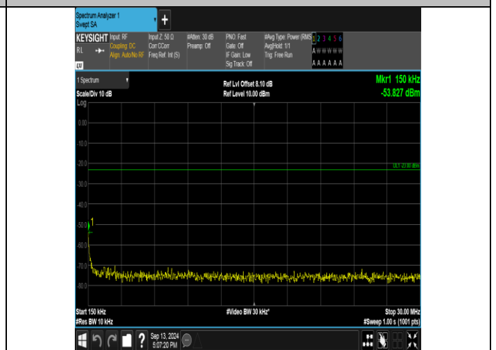
Band26_3MHz_QPSK_26705_15RB#0_0.15-30_0.15-30
