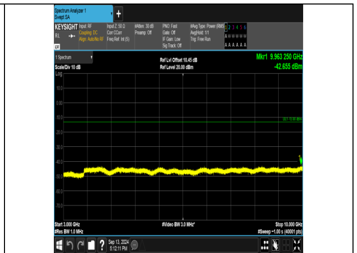
Band26_3MHz_16QAM_26740_1RB#14_3000-10000_3000-10000
