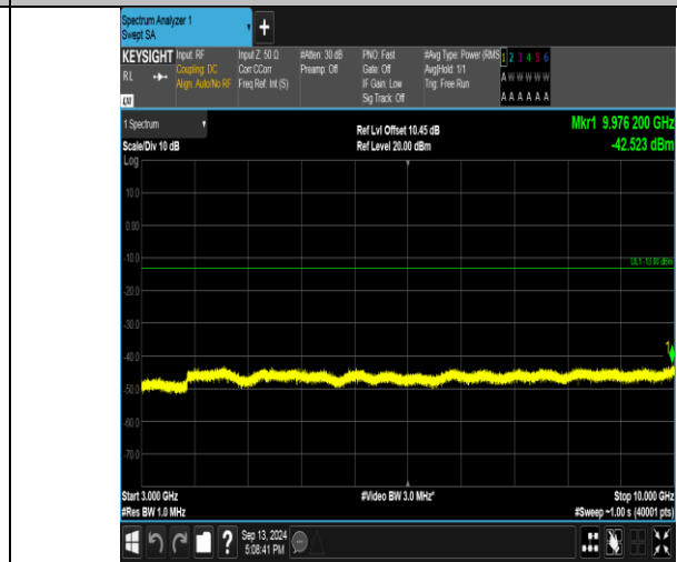
Band26_3MHz_16QAM_26705_15RB#0_3000-10000_3000-10000
