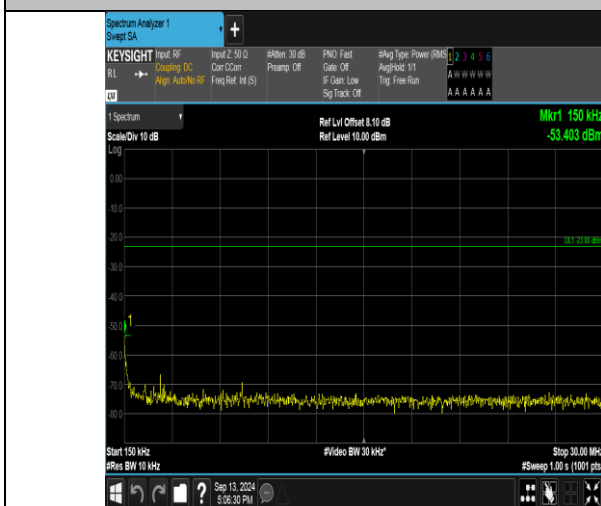
Band26_3MHz_16QAM_26705_1RB#14_0.15~30_0.15~30
