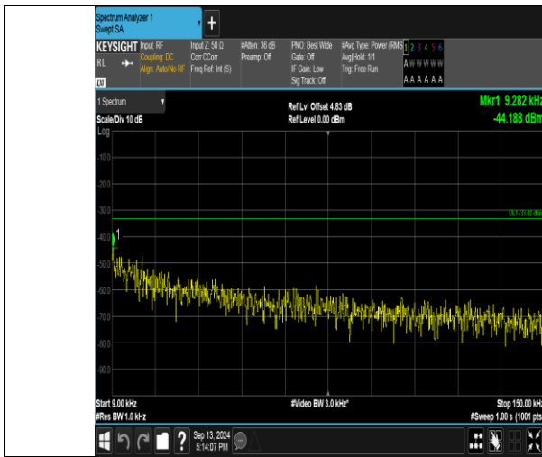
Band26_3MHz_QPSK_26775_1RB#0_0.009-0.15_0.009-0.15
