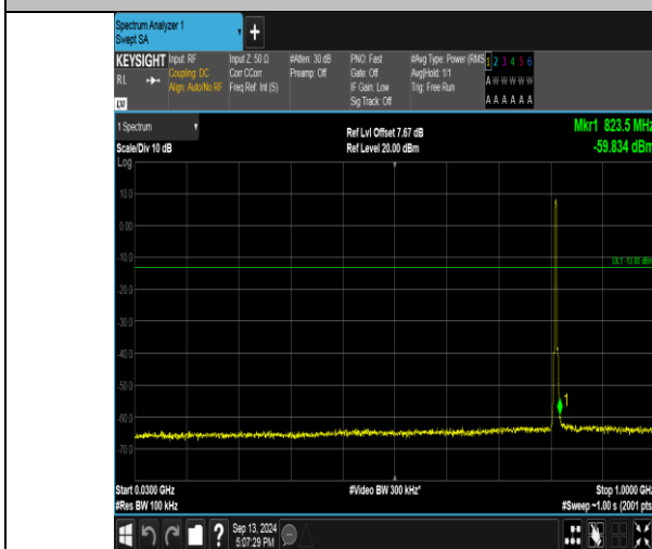
Band26_3MHz_QPSK_26705_15RB#0_30-1000_30-1000
