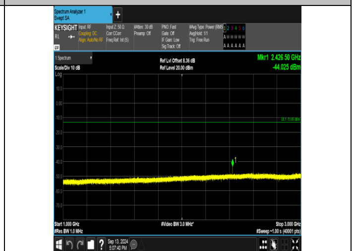
Band26_3MHz_QPSK_26705_15RB#0_1000-3000_1000-3000
