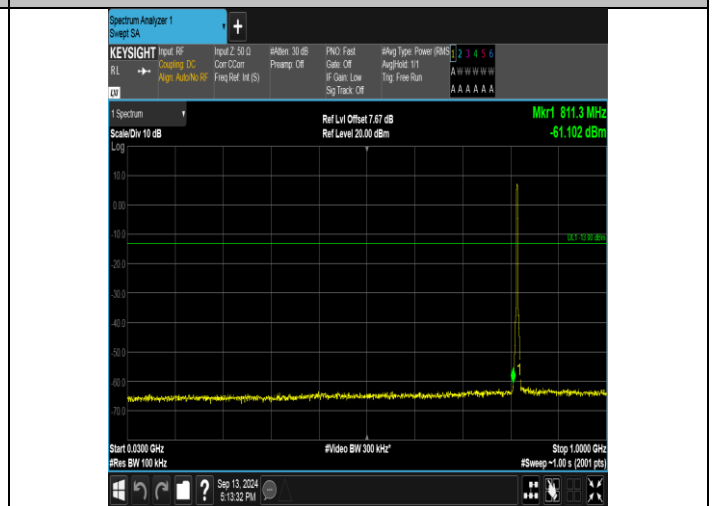
Band26_3MHz_16QAM_26740_15RB#0_30-1000_30-1000
