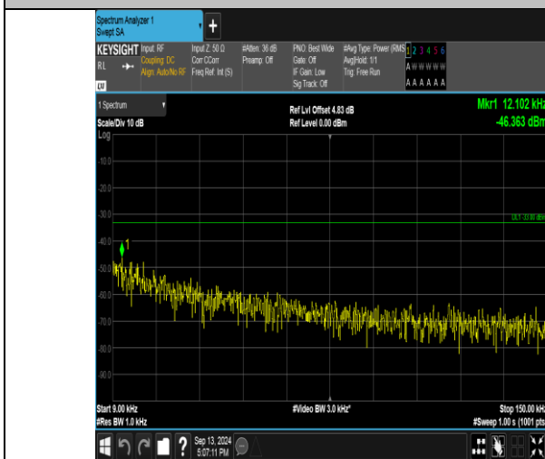
Band26_3MHz_QPSK_26705_15RB#0_0.009-0.15_0.009-0.15
