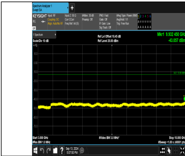
Band26_3MHz_QPSK_26705_15RB#0_3000-10000_3000-10000
