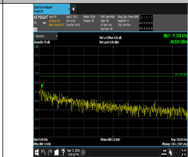
Band26_3MHz_16QAM_26705_1RB#0_0.009-0.15_0.009-0.15
