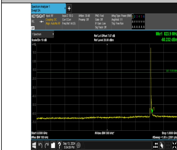
Band26_3MHz_QPSK_26705_1RB#0_30-1000_30-1000
