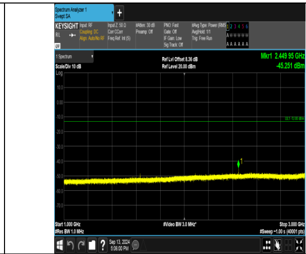
Band26_3MHz_QPSK_26705_1RB#14_1000~3000_1000~3000
