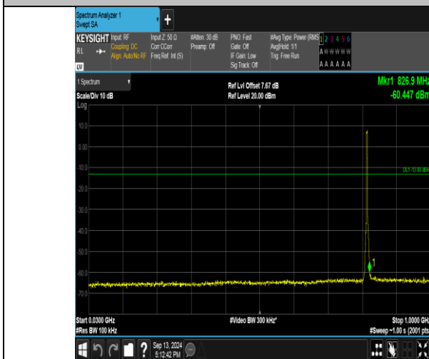
Band26_3MHz_QPSK_26740_15RB#0_30-1000_30-1000
