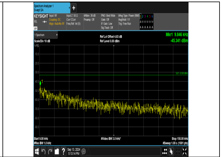
Band26_3MHz_16QAM_26740_15RB#0_0.009-0.15_0.009-0.15
