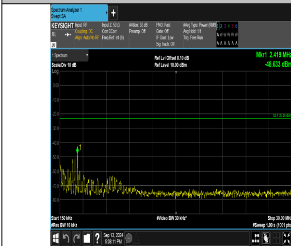
Band26_3MHz_16QAM_26705_15RB#0_0.15-30_0.15-30
