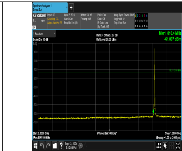
Band26_3MHz_16QAM_26740_1RB#0_30-1000_30-1000
