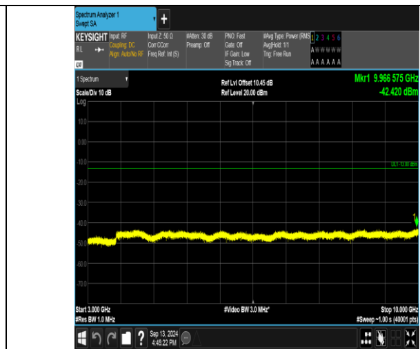
Band26_1.4MHz_16QAM_26783_1RB#5_3000-10000_3000-10000
