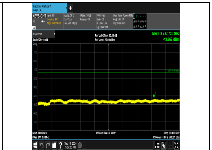
Band26_3MHz_16QAM_26705_1RB#14_3000-10000_3000-10000
