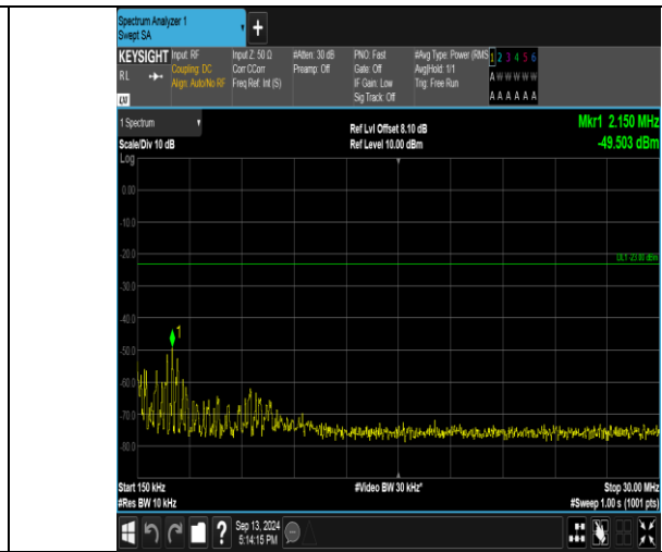
Band26_3MHz_QPSK_26775_1RB#0_0.15-30_0.15-30
