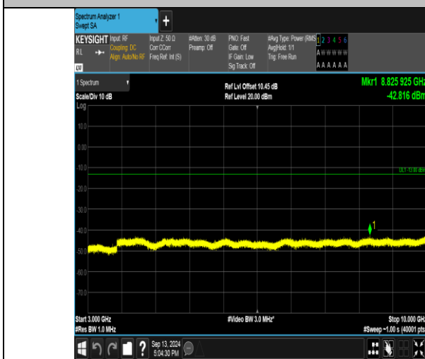
Band26_3MHz_QPSK_26705_1RB#0_3000-10000_3000-10000
