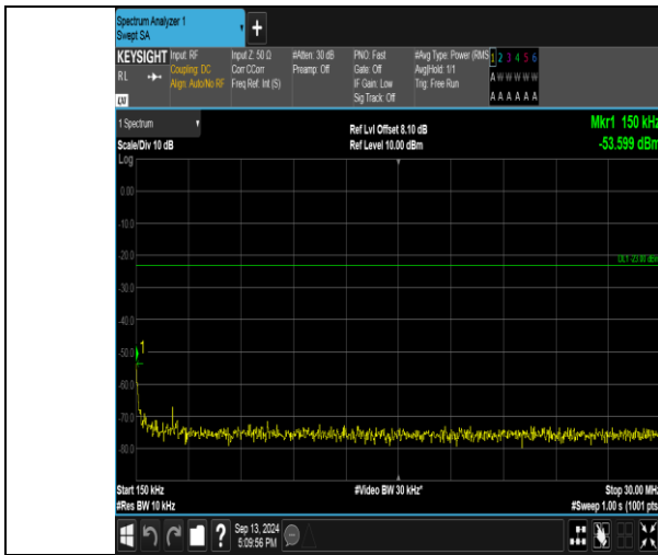
Band26_3MHz_16QAM_26740_1RB#0_0.15-30_0.15-30
