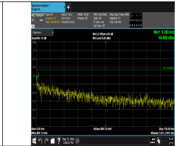
Band26_3MHz_16QAM_26705_15RB#0_0.009-0.15_0.009-0.15
