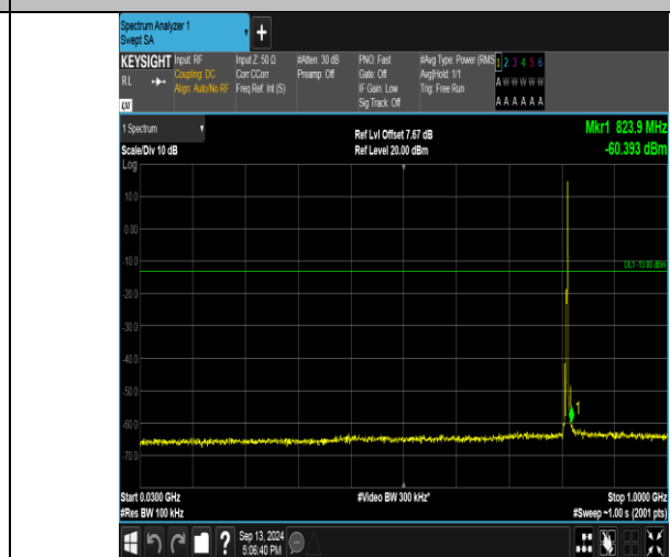
Band26_3MHz_16QAM_26705_1RB#14_30~1000_30~1000
