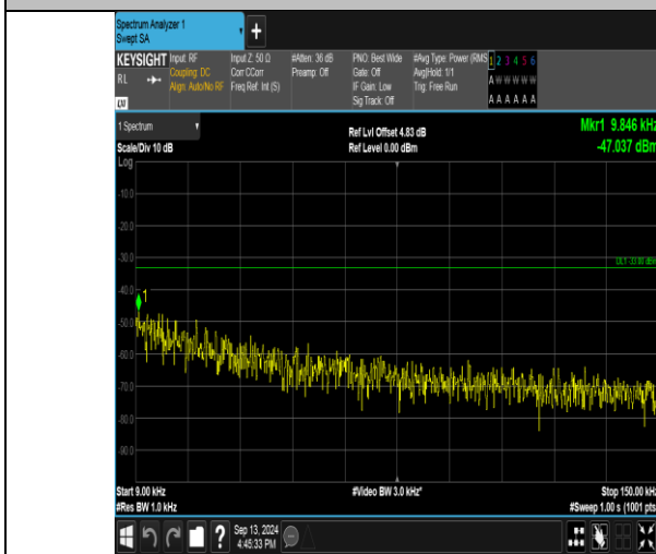
Band26_1.4MHz_QPSK_26783_6RB#0_0.009-0.15_0.009-0.15
