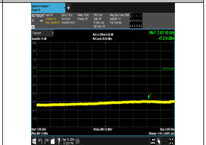
Band26_3MHz_QPSK_26740_15RB#0_1000-3000_1000-3000
