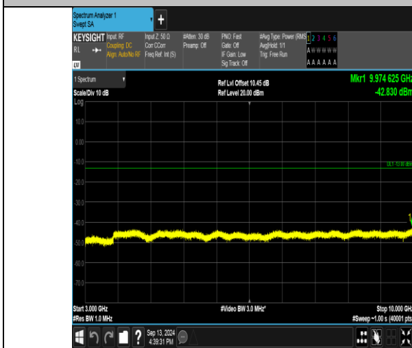
Band26_1.4MHz_QPSK_26740_1RB#5_3000~10000_3000~10000
