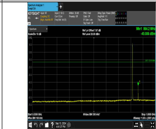
Band26_1.4MHz_16QAM_26740_6RB#0_30~1000_30~1000
