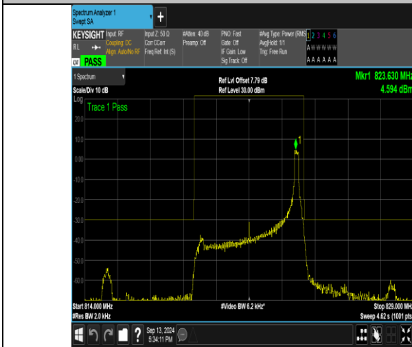
Band26_5MHz_QPSK_26765_1RB#24
