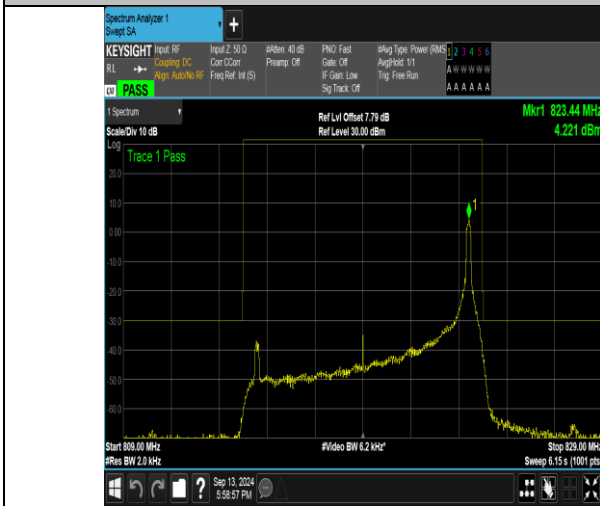
Band26_10MHz_QPSK_26740_1RB#49
