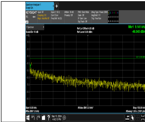
Band26_1.4MHz_QPSK_26783_1RB#0_0.009-0.15_0.009-0.15
