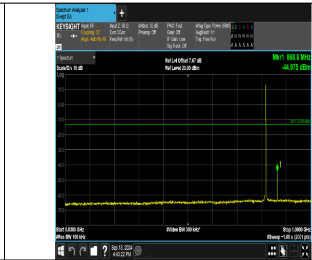
Band26_1.4MHz_16QAM_26783_1RB#0_30~1000_30~1000
