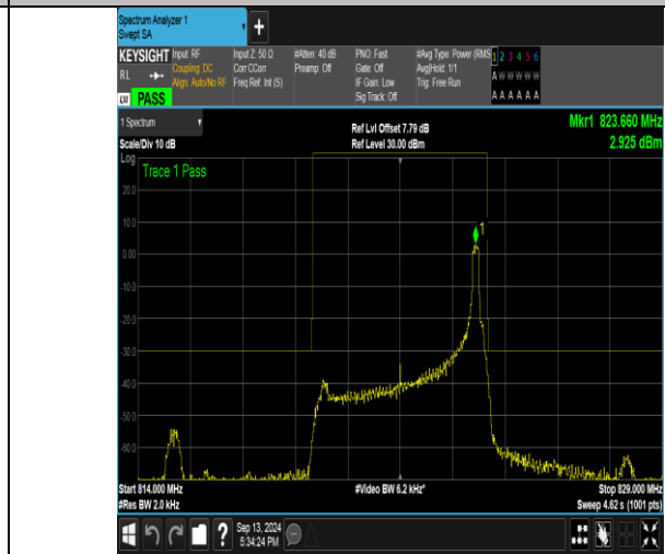
Band26_5MHz_16QAM_26765_1RB#24
