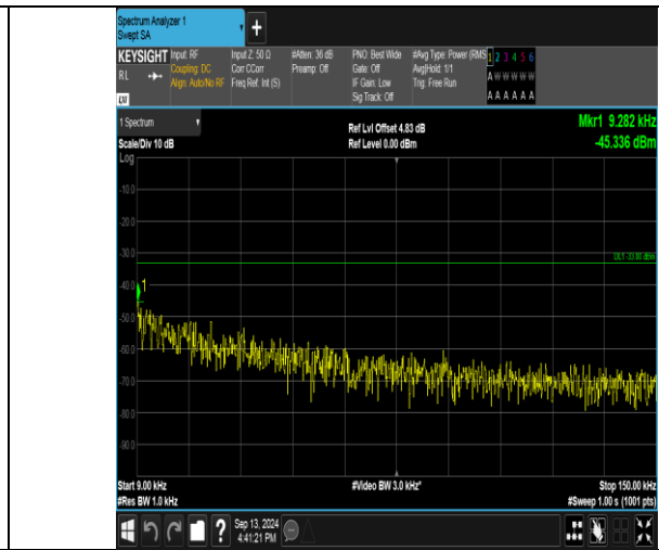
Band26_1.4MHz_16QAM_26740_6RB#0_0.009~0.15_0.009~0.15
