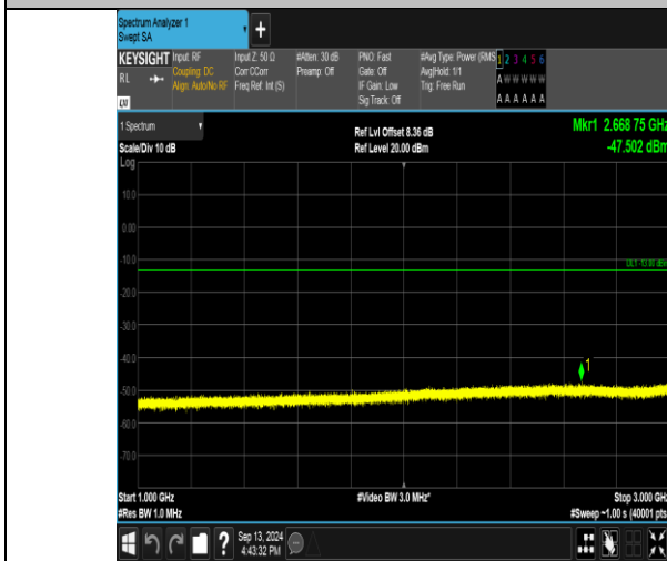
Band26_1.4MHz_16QAM_26783_1RB#0_1000~3000_1000~3000
