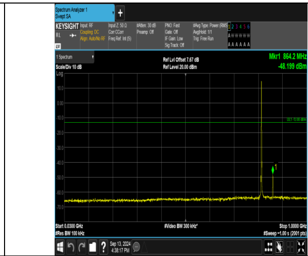
Band26_1.4MHz_16QAM_26740_1RB#0_30~1000_30~1000
