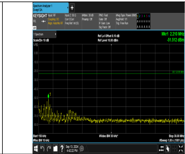
Band26_1.4MHz_QPSK_26783_1RB#0_0.15-30_0.15-30
