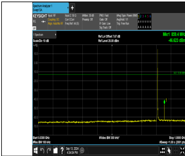
Band26_1.4MHz_QPSK_26697_1RB#5_30-1000_30-1000
