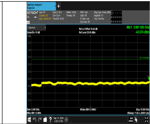
Band26_1.4MHz_16QAM_26697_1RB#5_3000-10000_3000-10000
