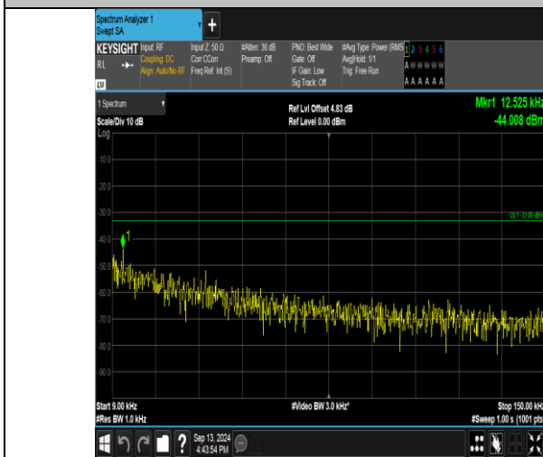
Band26_1.4MHz_QPSK_26783_1RB#5_0.009~0.15_0.009~0.15
