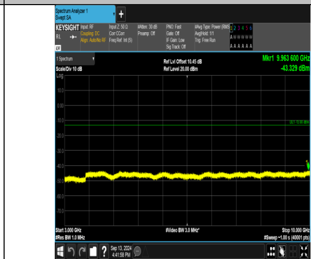
Band26_1.4MHz_16QAM_26740_6RB#0_3000~10000_3000~10000
