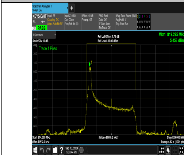
Band26_5MHz_QPSK_26765_1RB#0
