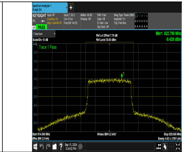
Band26_5MHz_16QAM_26765_25RB#0
