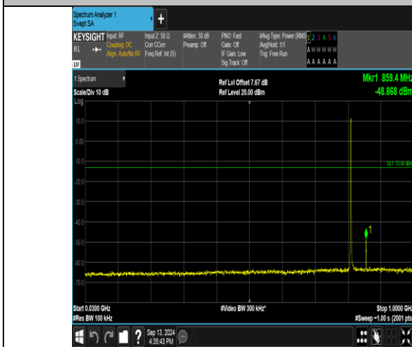
Band26_1.4MHz_QPSK_26697_6RB#0_30-1000_30-1000
