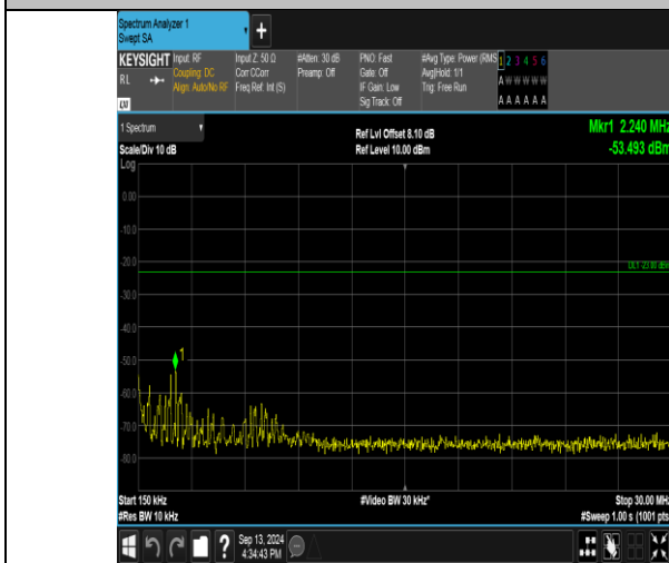
Band26_1.4MHz_16QAM_26697_1RB#5_0.15-30_0.15-30
