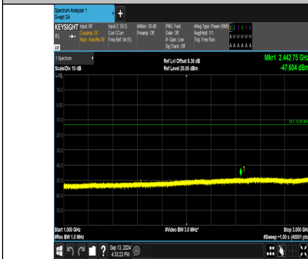
Band26_1.4MHz_16QAM_26697_1RB#0_1000~3000_1000~3000
