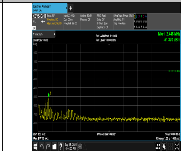
Band26_1.4MHz_QPSK_26783_1RB#5_0.15~30_0.15~30
