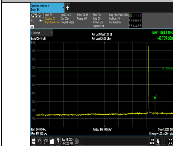
Band26_1.4MHz_QPSK_26783_1RB#0_30-1000_30-1000
