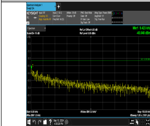
Band26_1.4MHz_QPSK_26697_6RB#0_0.009-0.15_0.009-0.15
