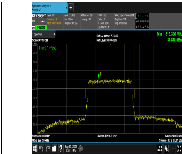
Band26_5MHz_QPSK_26715_25RB#0
