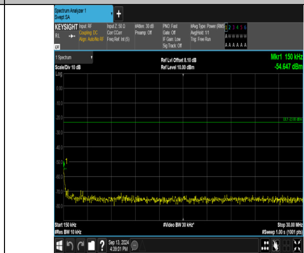
Band26_1.4MHz_QPSK_26740_1RB#5_0.15~30_0.15~30
