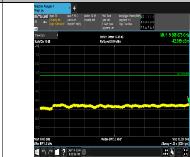
Band26_1.4MHz_16QAM_26740_1RB#0_3000~10000_3000~10000
