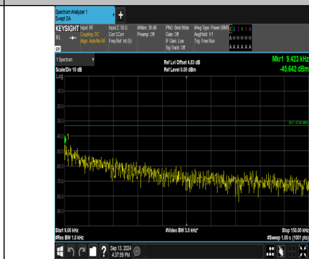
Band26_1.4MHz_16QAM_26740_1RB#0_0.009-0.15_0.009-0.15
