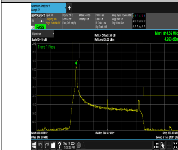
Band26_10MHz_QPSK_26740_1RB#0
