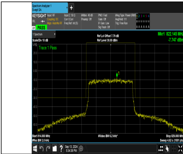
Band26_5MHz_QPSK_26765_25RB#0
