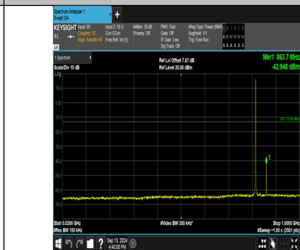
Band26_1.4MHz_16QAM_26740_1RB#5_30~1000_30~1000
