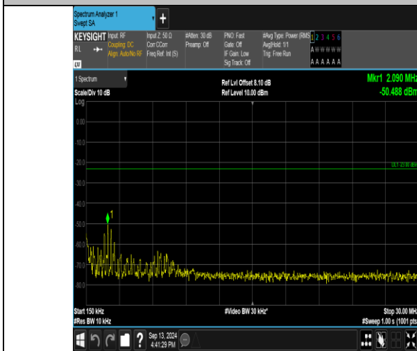
Band26_1.4MHz_16QAM_26740_6RB#0_0.15~30_0.15~30
