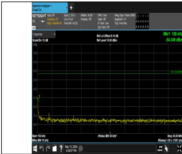
Band26_1.4MHz_16QAM_26740_1RB#0_0.15~30_0.15~30
