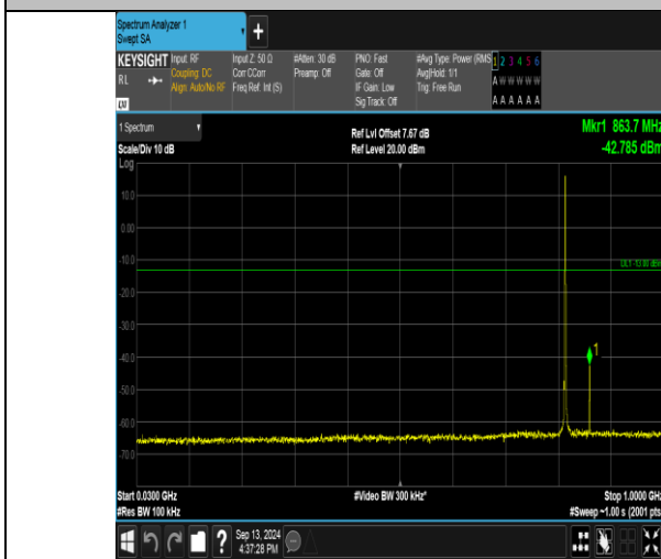
Band26_1.4MHz_QPSK_26740_1RB#0_30-1000_30-1000
