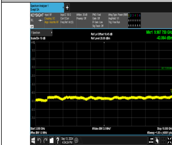
Band26_1.4MHz_QPSK_26697_1RB#5_3000-10000_3000-10000
