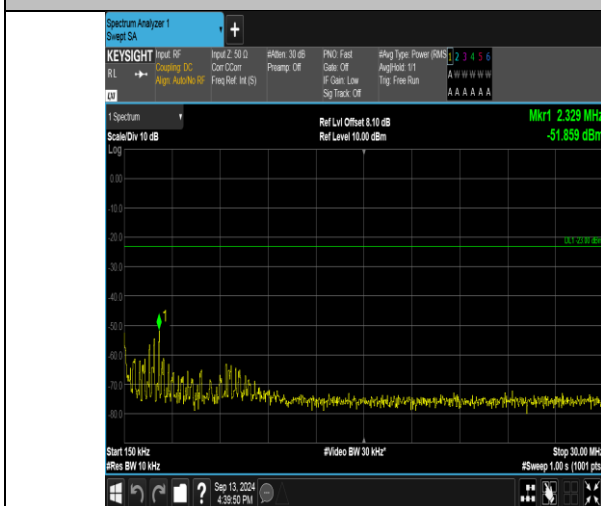
Band26_1.4MHz_16QAM_26740_1RB#5_0.15~30_0.15~30
