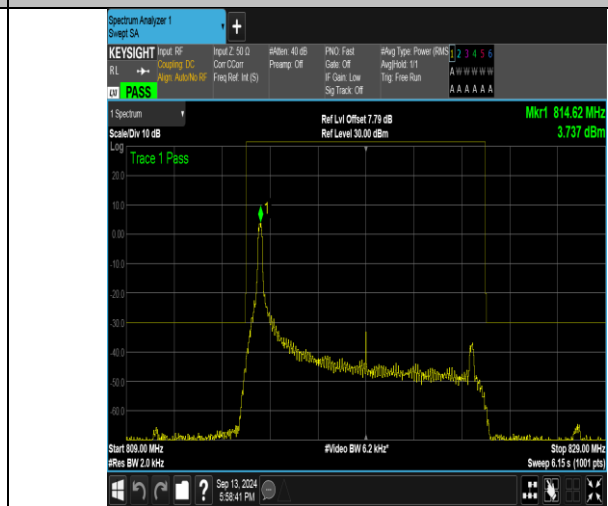
Band26_10MHz_16QAM_26740_1RB#0
