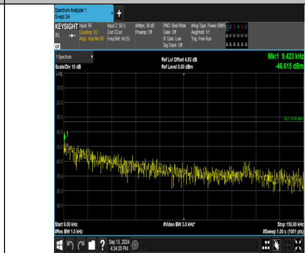
Band26_1.4MHz_16QAM_26697_1RB#5_0.009-0.15_0.009-0.15
