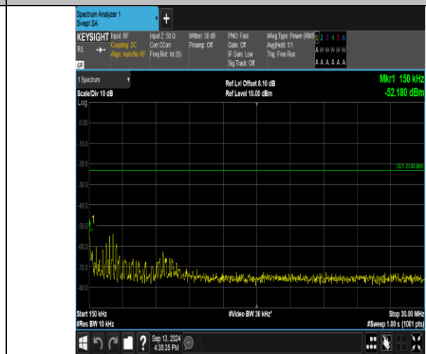
Band26_1.4MHz_QPSK_26697_6RB#0_0.15-30_0.15-30
