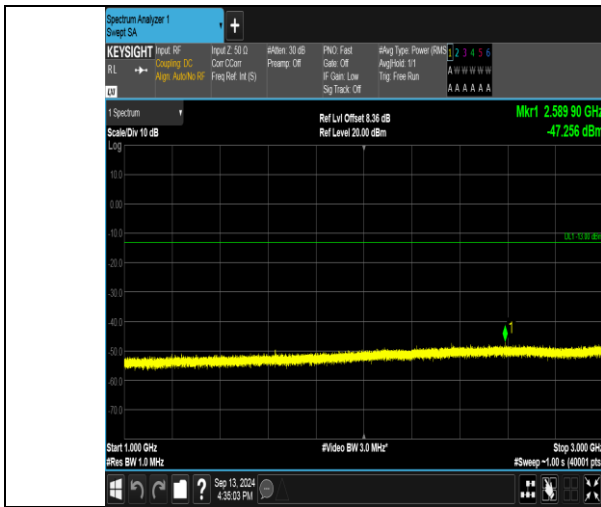
Band26_1.4MHz_16QAM_26697_1RB#5_1000-3000_1000-3000
