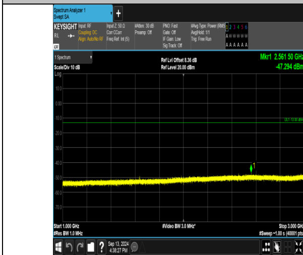
Band26_1.4MHz_16QAM_26740_1RB#0_1000~3000_1000~3000
