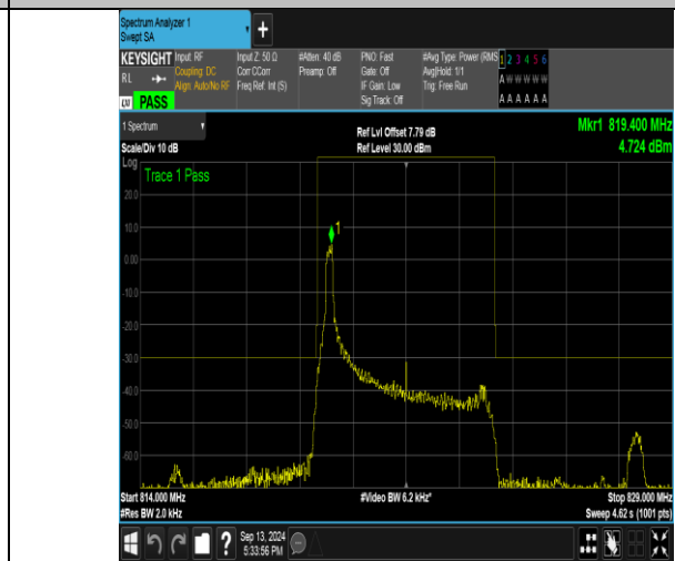
Band26_5MHz_16QAM_26765_1RB#0
