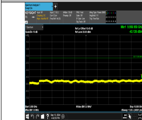
Band26_1.4MHz_QPSK_26783_1RB#0_3000-10000_3000-10000
