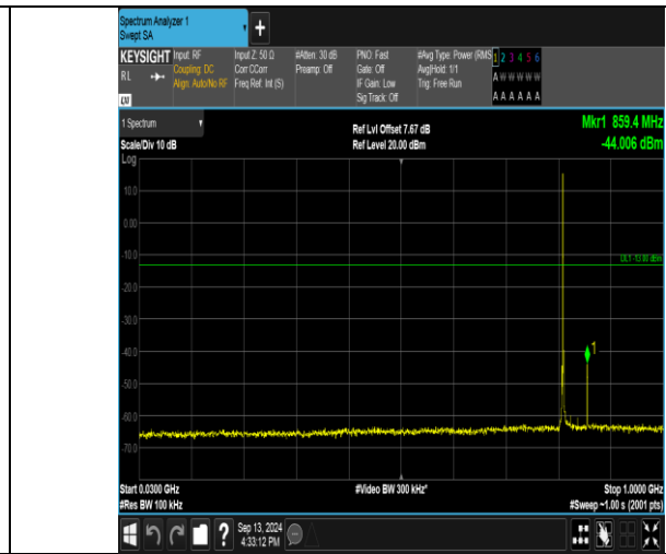
Band26_1.4MHz_16QAM_26697_1RB#0_30~1000_30~1000
