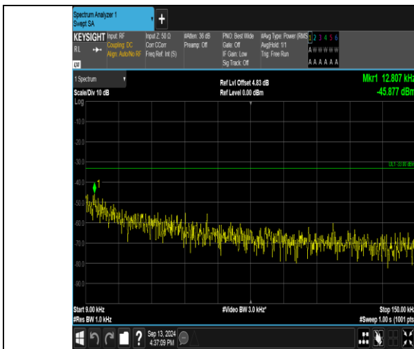
Band26_1.4MHz_QPSK_26740_1RB#0_0.009-0.15_0.009-0.15
