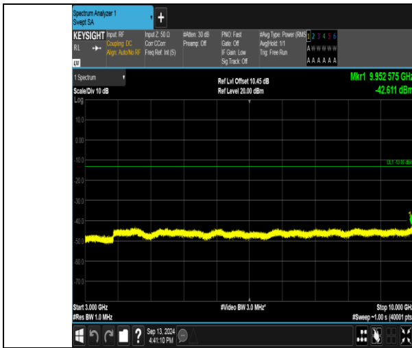
Band26_1.4MHz_QPSK_26740_6RB#0_3000~10000_3000~10000
