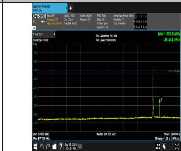
Band26_1.4MHz_16QAM_26697_1RB#5_30-1000_30-1000
