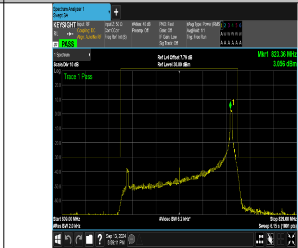
Band26_10MHz_16QAM_26740_1RB#49
