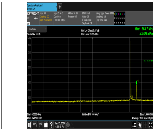
Band26_1.4MHz_QPSK_26740_1RB#5_30~1000_30~1000
