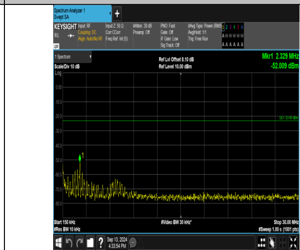
Band26_1.4MHz_QPSK_26697_1RB#5_0.15~30_0.15~30
