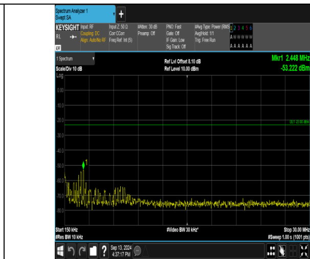
Band26_1.4MHz_QPSK_26740_1RB#0_0.15-30_0.15-30
