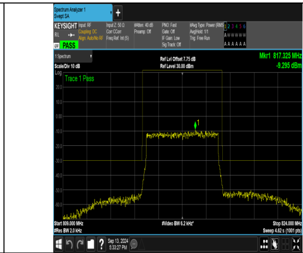
Band26_5MHz_16QAM_26715_25RB#0
