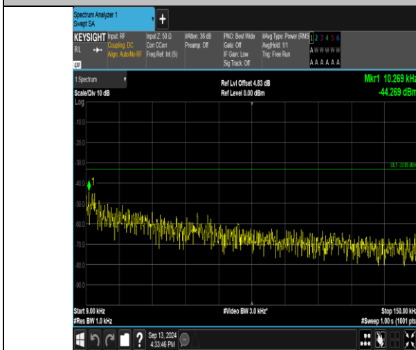
Band26_1.4MHz_QPSK_26697_1RB#5_0.009~0.15_0.009~0.15
