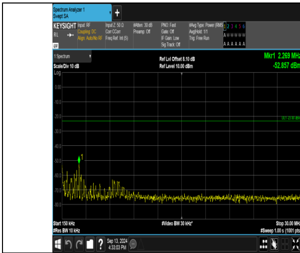
Band26_1.4MHz_16QAM_26697_1RB#0_0.15~30_0.15~30
