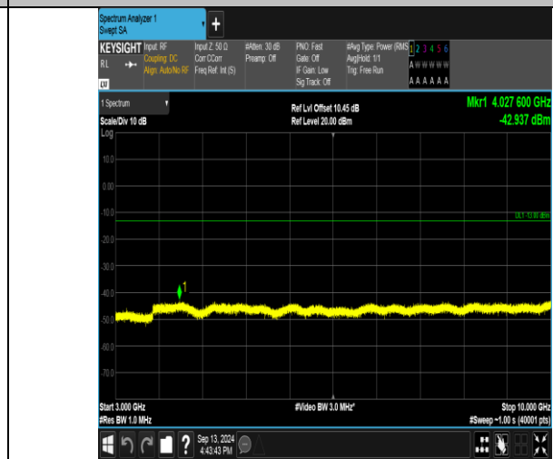
Band26_1.4MHz_16QAM_26783_1RB#0_3000~10000_3000~10000
