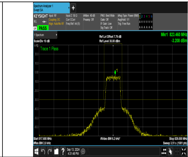
Band26_1.4MHz_16QAM_26783_6RB#0
