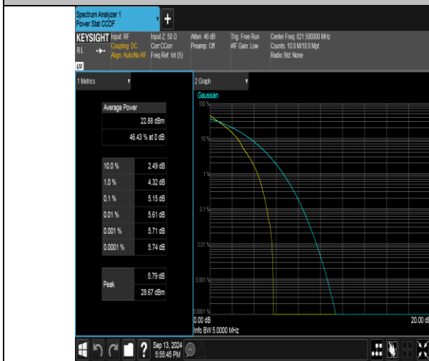
Band26(814-824)-5MHz-QPSK-26765-1RB#0-PASS
