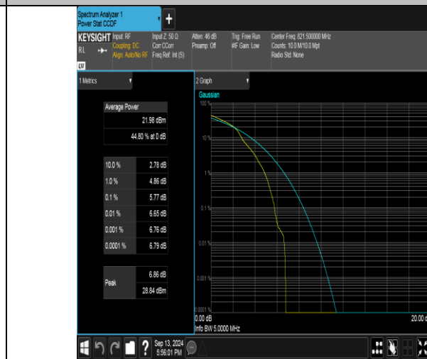
Band26(814-824)-5MHz-16QAM-26765-1RB#0-PASS
