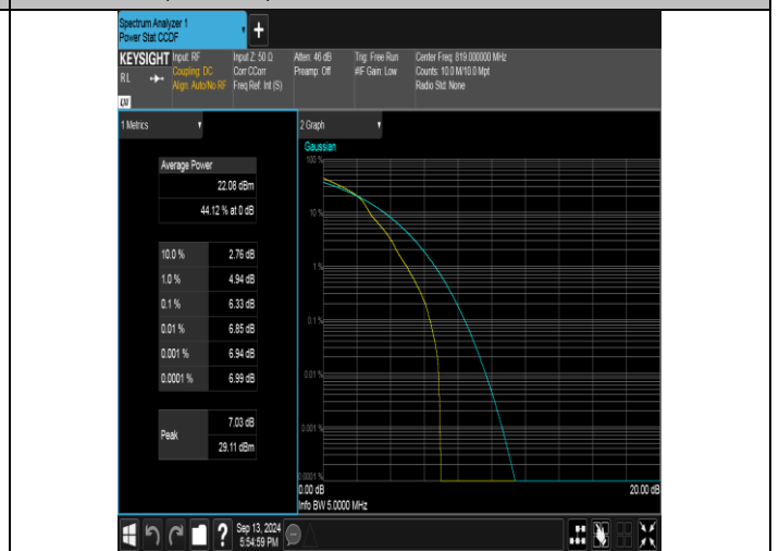
Band26(814-824)-5MHz-16QAM-26740-1RB#0-PASS
