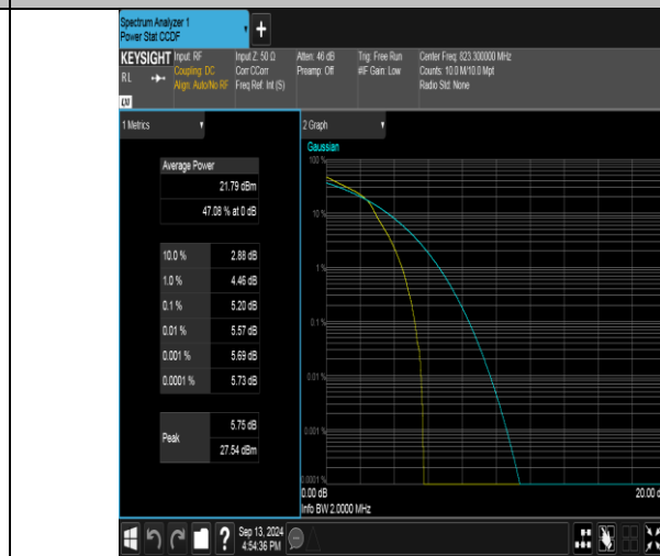
Band26(814-824)-1.4MHz-16QAM-26783-1RB#0-PASS
