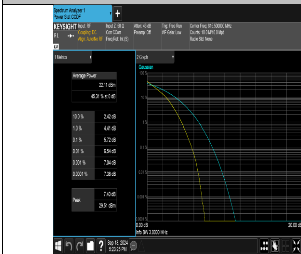
Band26(814-824)-3MHz-QPSK-26705-15RB#0-PASS
