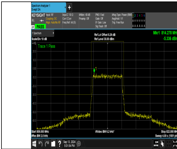
Band26_3MHz_QPSK_26705_15RB#0
