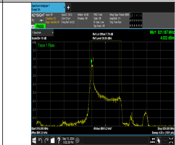
Band26_3MHz_16QAM_26775_1RB#0
