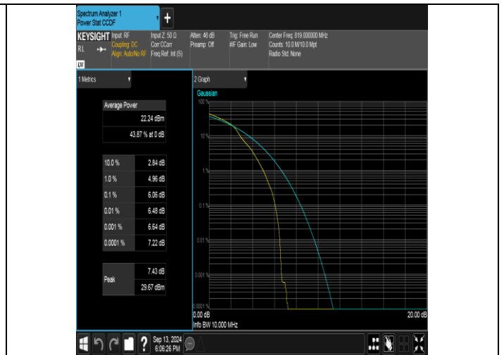
Band26(814-824)-10MHz-16QAM-26740-1RB#0-PASS
