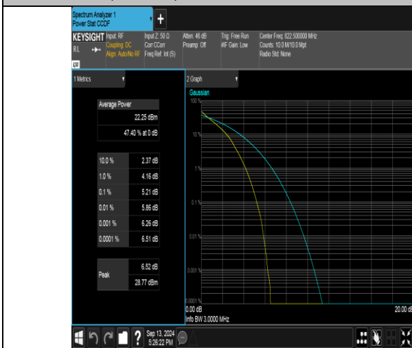
Band26(814-824)-3MHz-QPSK-26775-15RB#0-PASS
