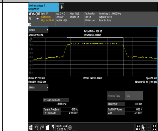
Band26(814-824)-5MHz-16QAM-26765-25RB#0-PASS
