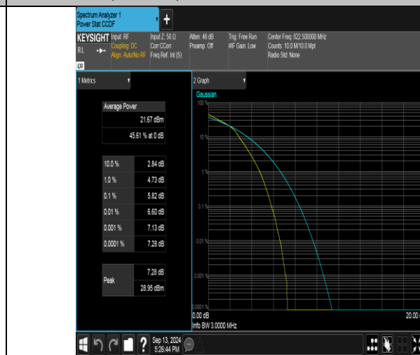
Band26(814-824)-3MHz-16QAM-26775-15RB#0-PASS
