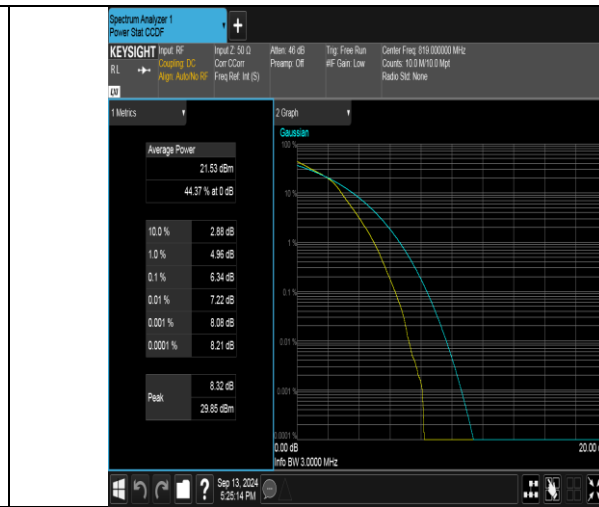
Band26(814-824)-3MHz-16QAM-26740-15RB#0-PASS
