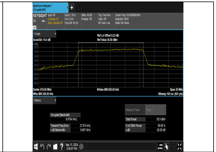
Band26(814-824)-10MHz-16QAM-26740-50RB#0-PASS
