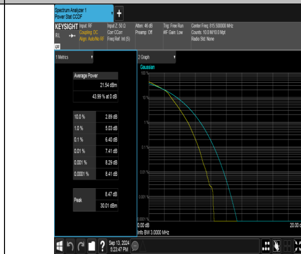
Band26(814-824)-3MHz-16QAM-26705-15RB#0-PASS
