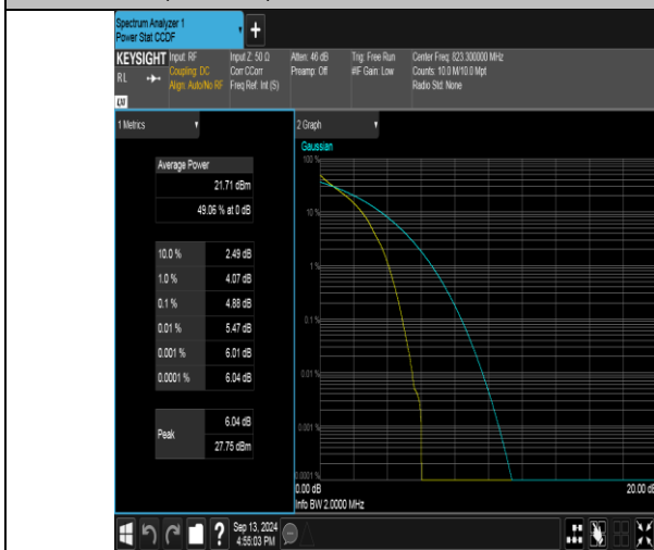
Band26(814-824)-1.4MHz-QPSK-26783-6RB#0-PASS
