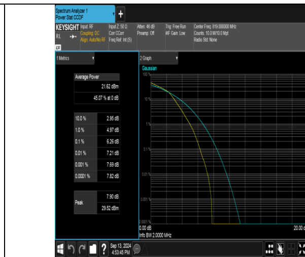
Band26(814-824)-1.4MHz-16QAM-26740-6RB#0-PASS
