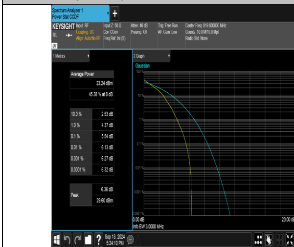
Band26(814-824)-3MHz-QPSK-26740-1RB#0-PASS
