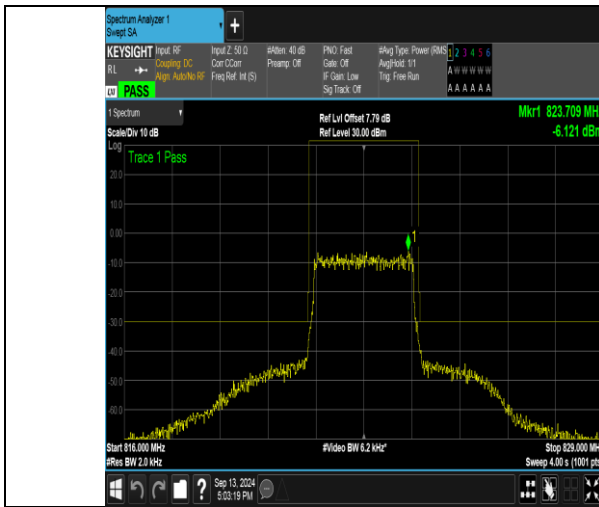
Band26_3MHz_QPSK_26775_15RB#0
