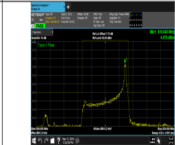
Band26_5MHz_16QAM_26715_1RB#24
