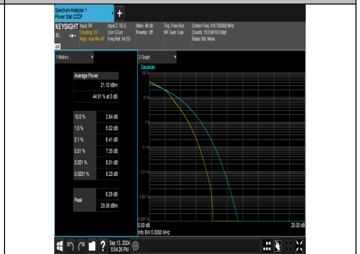
Band26(814-824)-5MHz-16QAM-26715-25RB#0-PASS
