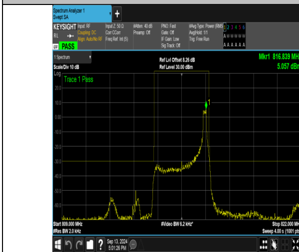
Band26_3MHz_QPSK_26705_1RB#14
