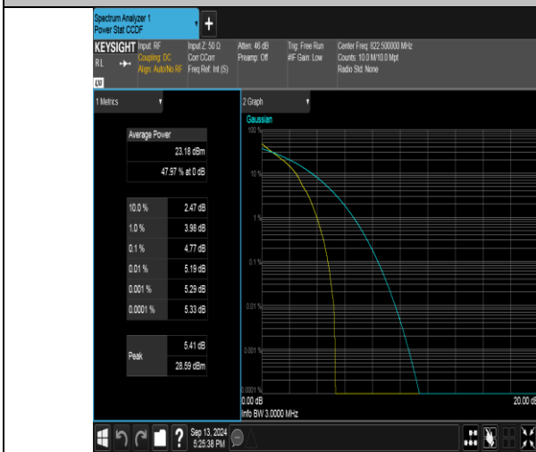
Band26(814-824)-3MHz-QPSK-26775-1RB#0-PASS
