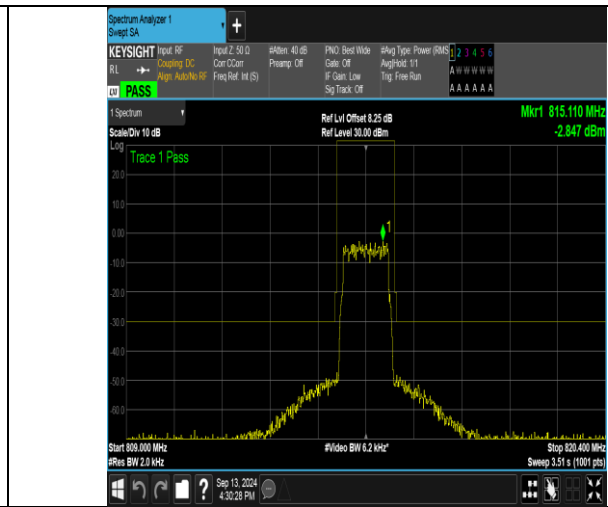
Band26_1.4MHz_16QAM_26697_6RB#0
