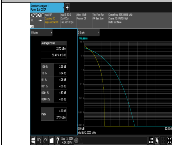
Band26(814-824)-1.4MHz-QPSK-26783-1RB#0-PASS
