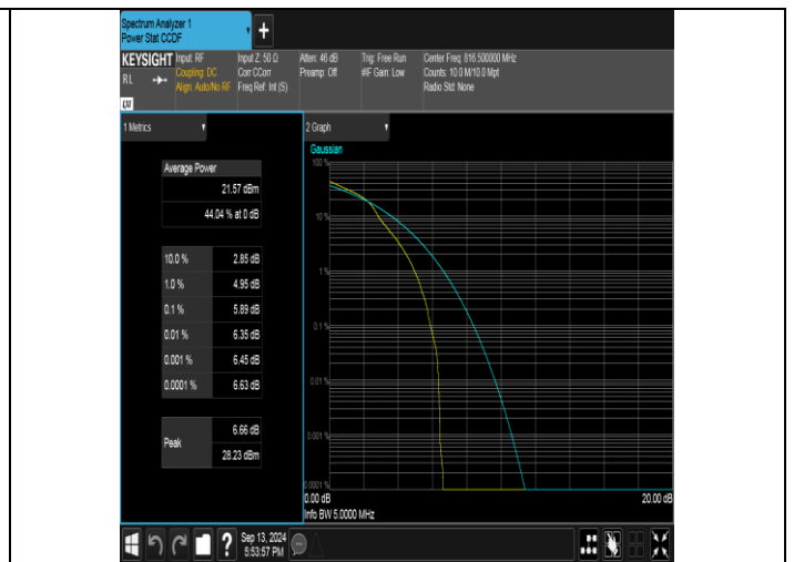
Band26(814-824)-5MHz-16QAM-26715-1RB#0-PASS
