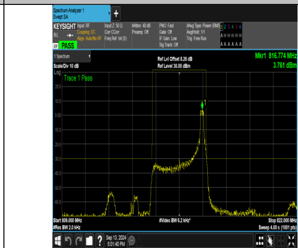
Band26_3MHz_16QAM_26705_1RB#14
