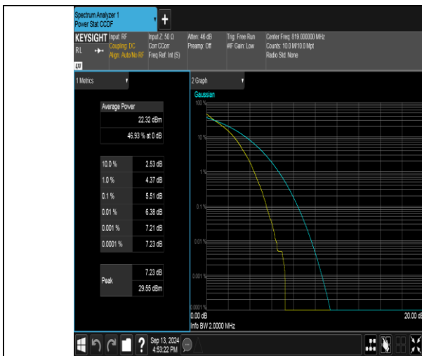
Band26(814-824)-1.4MHz-QPSK-26740-6RB#0-PASS
