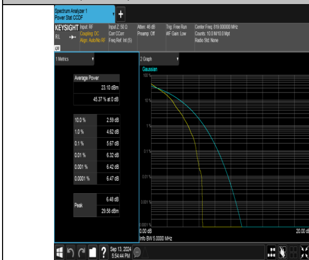
Band26(814-824)-5MHz-QPSK-26740-1RB#0-PASS
