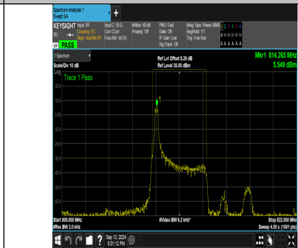
Band26_3MHz_16QAM_26705_1RB#0
