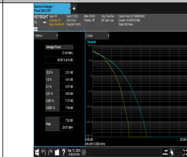
Band26(814-824)-5MHz-16QAM-26765-25RB#0-PASS
