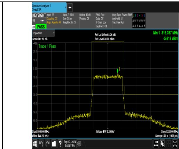
Band26_3MHz_16QAM_26705_15RB#0
