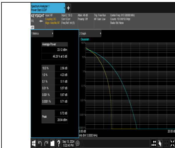
Band26(814-824)-3MHz-QPSK-26705-1RB#0-PASS
