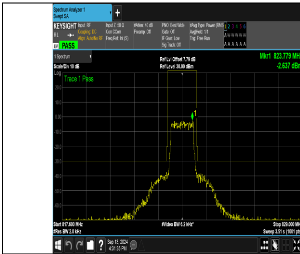
Band26_1.4MHz_QPSK_26783_6RB#0
