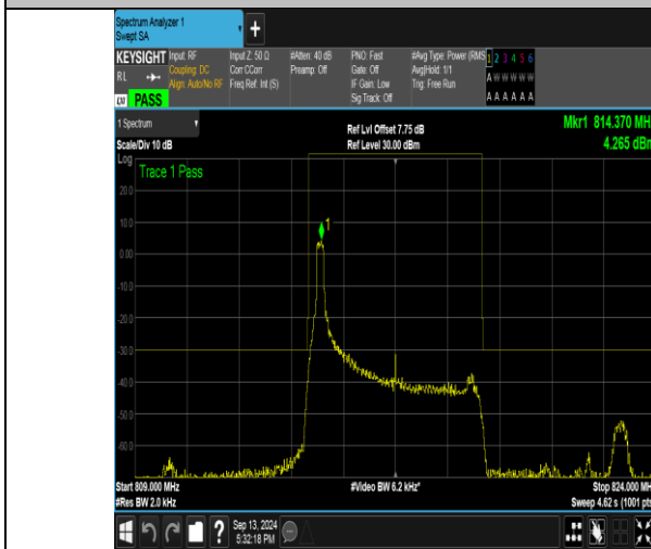
Band26_5MHz_QPSK_26715_1RB#0
