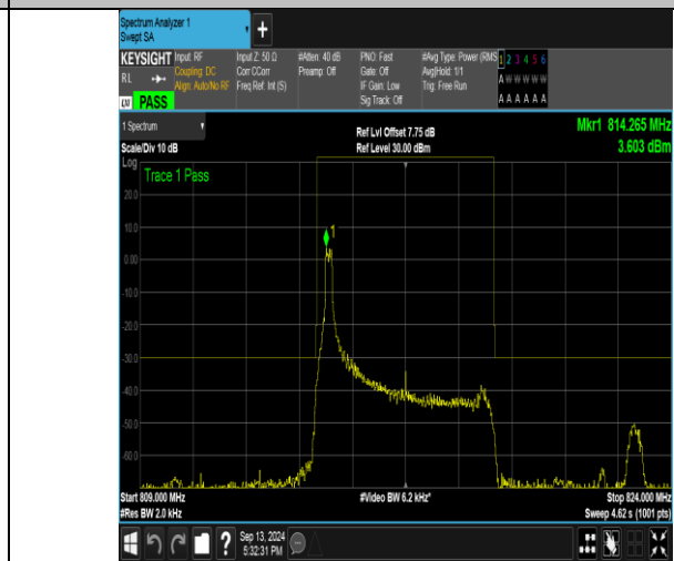
Band26_5MHz_16QAM_26715_1RB#0
