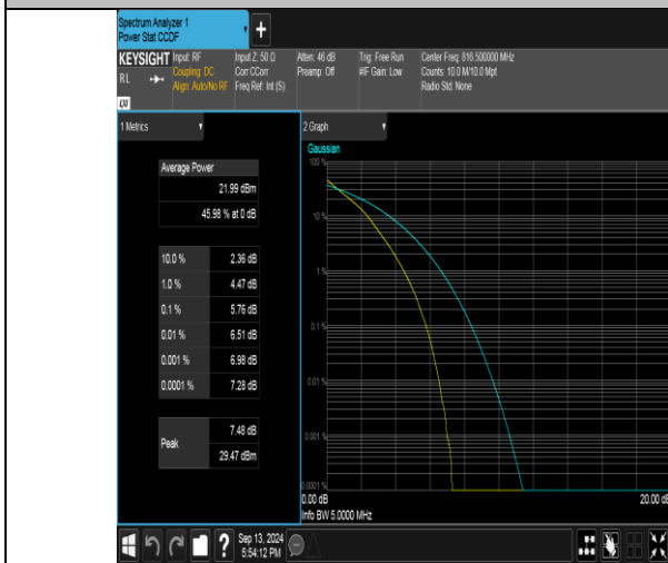
Band26(814-824)-5MHz-QPSK-26715-25RB#0-PASS
