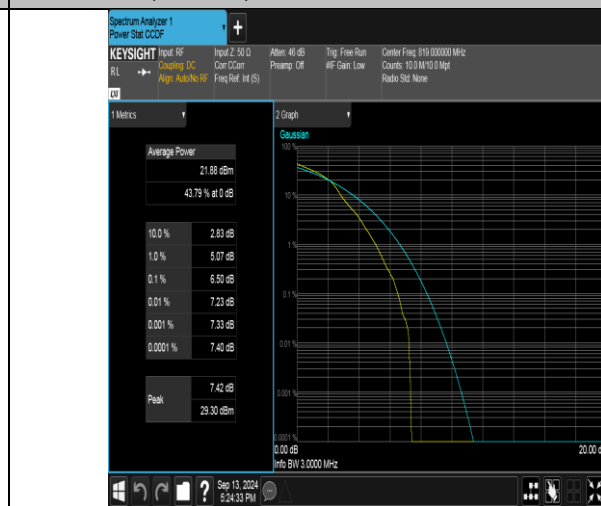
Band26(814-824)-3MHz-16QAM-26740-1RB#0-PASS
