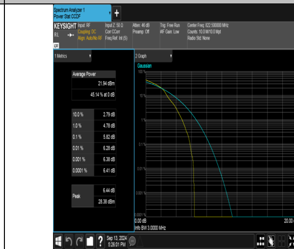
Band26(814-824)-3MHz-16QAM-26775-1RB#0-PASS
