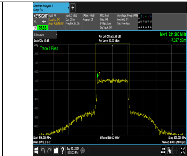
Band26_3MHz_16QAM_26775_15RB#0
