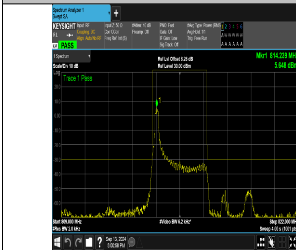
Band26_3MHz_QPSK_26705_1RB#0
