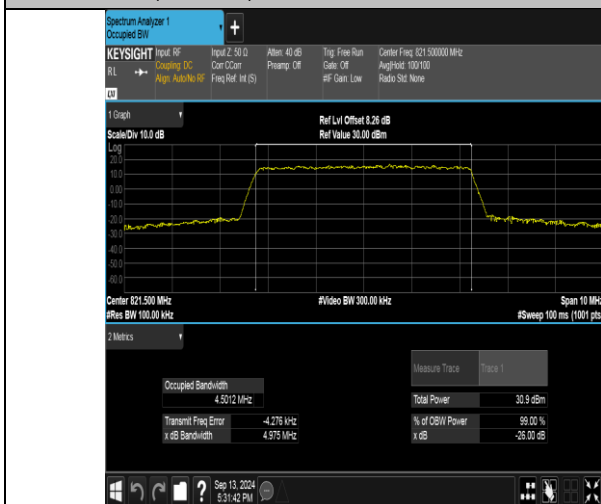
Band26(814-824)-5MHz-QPSK-26765-25RB#0-PASS
