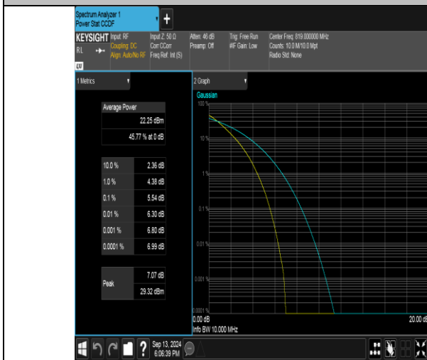
Band26(814-824)-10MHz-QPSK-26740-50RB#0-PASS
