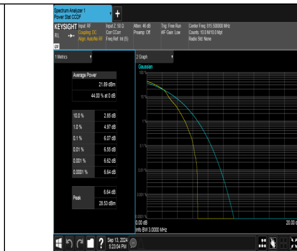
Band26(814-824)-3MHz-16QAM-26705-1RB#0-PASS
