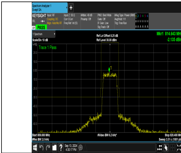
Band26_1.4MHz_QPSK_26697_6RB#0
