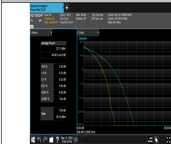
Band26(814-824)-5MHz-QPSK-26765-25RB#0-PASS
