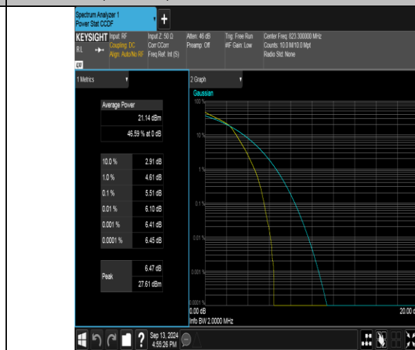
Band26(814-824)-1.4MHz-16QAM-26783-6RB#0-PASS
