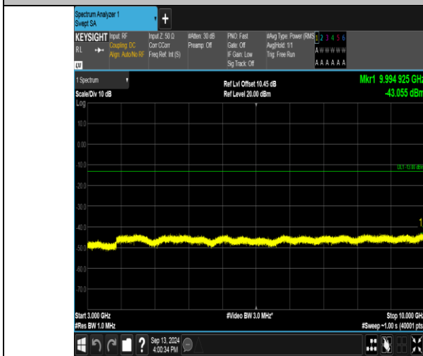
Band17_10MHz_QPSK_23800_1RB#49_3000~10000_3000~10000
