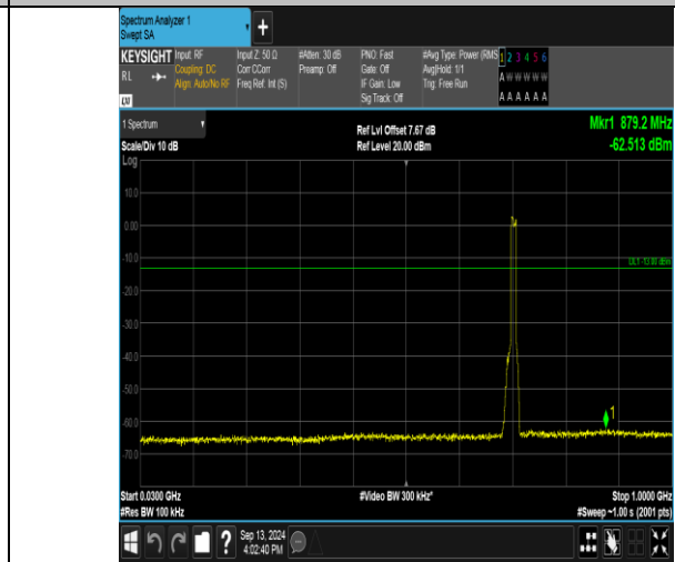
Band17_10MHz_16QAM_23800_50RB#0_30~1000_30~1000
