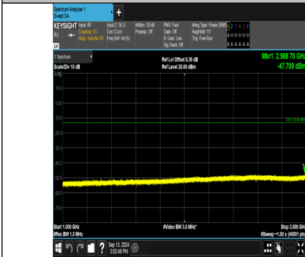
Band17_10MHz_16QAM_23780_50RB#0_1000~3000_1000~3000
