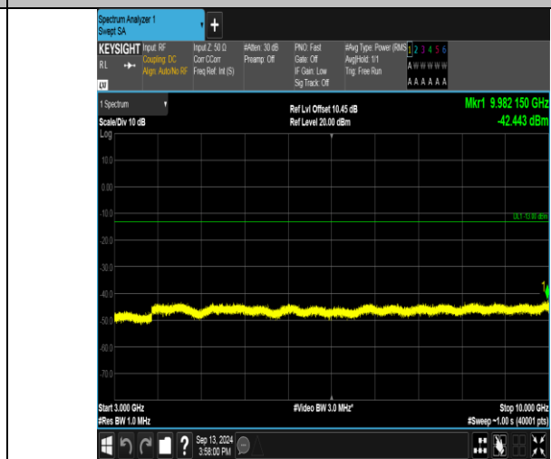
Band17_10MHz_16QAM_23790_50RB#0_3000~10000_3000~10000
