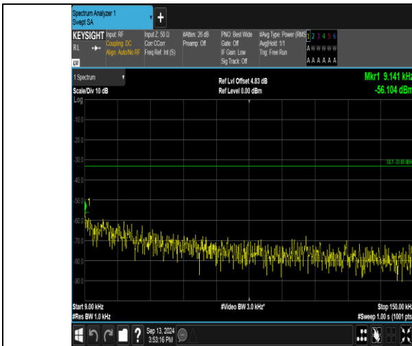
Band17_10MHz_QPSK_23790_1RB#0_0.009-0.15_0.009-0.15
