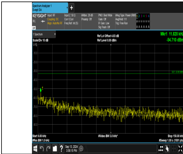
Band17_10MHz_QPSK_23800_1RB#0_0.009-0.15_0.009-0.15
