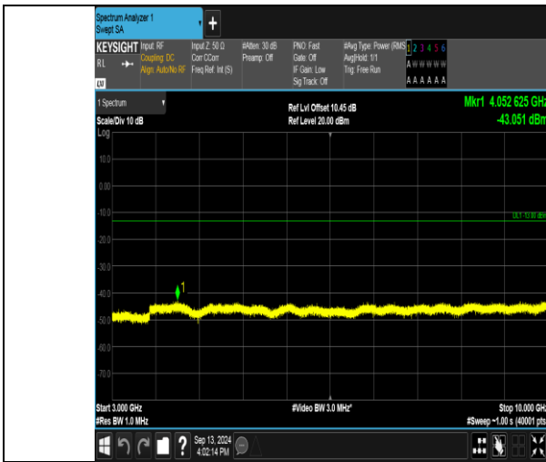
Band17_10MHz_QPSK_23800_50RB#0_3000~10000_3000~10000
