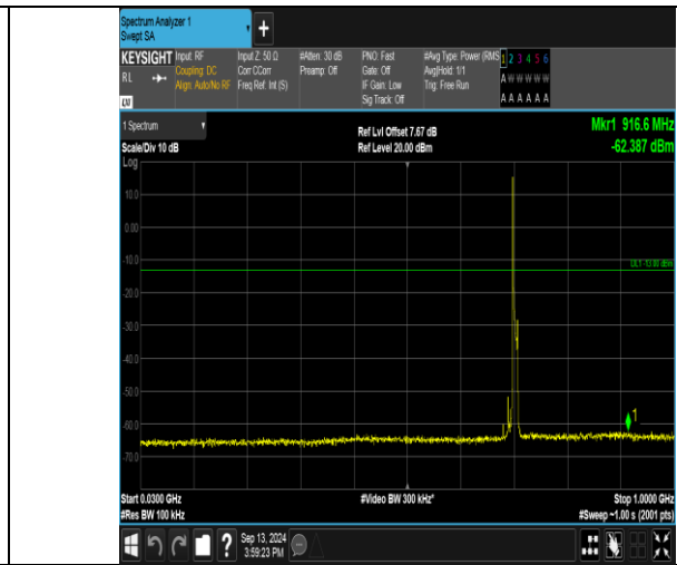
Band17_10MHz_16QAM_23800_1RB#0_30~1000_30~1000
