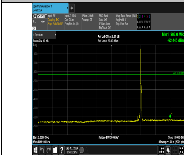
Band17_10MHz_QPSK_23800_1RB#0_30-1000_30-1000
