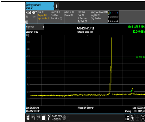
Band17_10MHz_QPSK_23800_1RB#49_30~1000_30~1000
