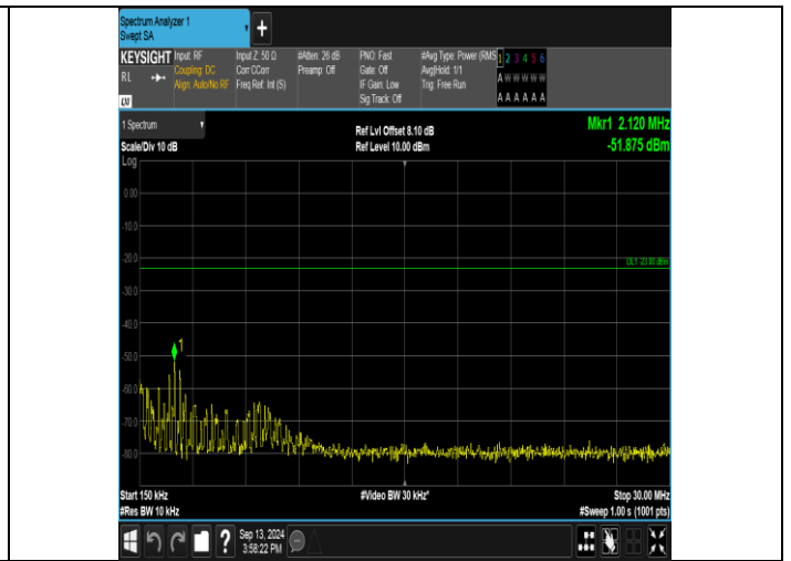
Band17_10MHz_QPSK_23800_1RB#0_0.15-30_0.15-30
