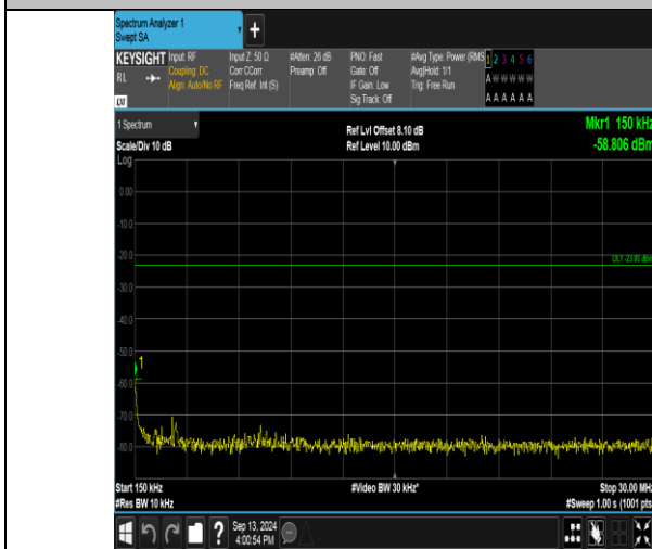
Band17_10MHz_16QAM_23800_1RB#49_0.15~30_0.15~30
