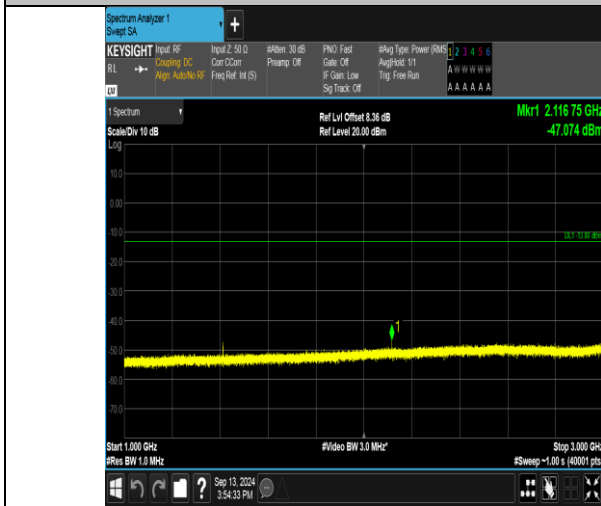
Band17_10MHz_16QAM_23790_1RB#0.1000-3000_1000-3000
