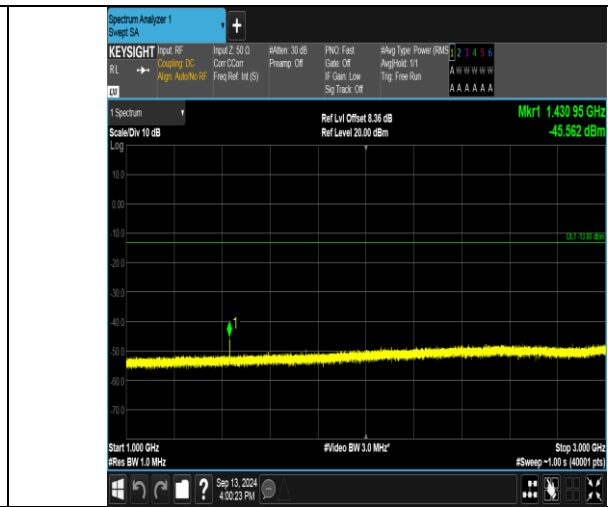
Band17_10MHz_QPSK_23800_1RB#49_1000~3000_1000~3000
