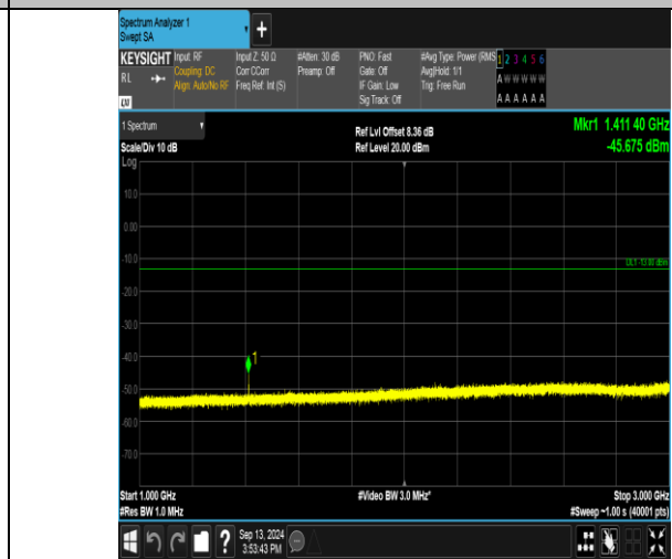
Band17_10MHz_QPSK_23790_1RB#0_1000-3000_1000-3000
