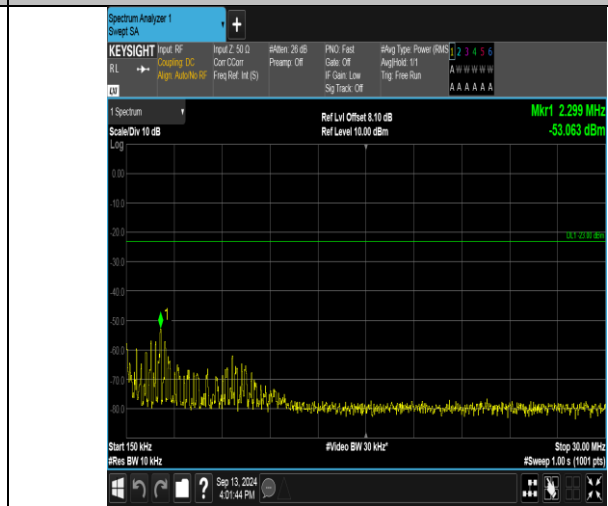
Band17_10MHz_QPSK_23800_50RB#0_0.15~30_0.15~30
