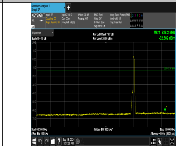
Band17_10MHz_16QAM_23790_50RB#0_30~1000_30~1000
