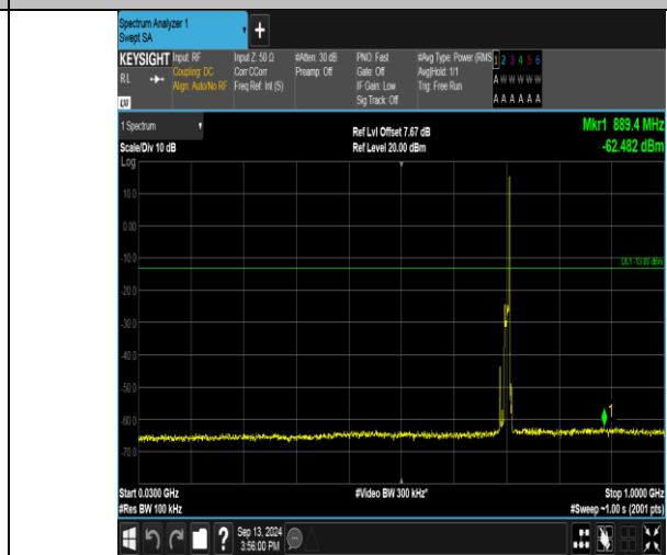
Band17_10MHz_16QAM_23790_1RB#49_30~1000_30~1000
