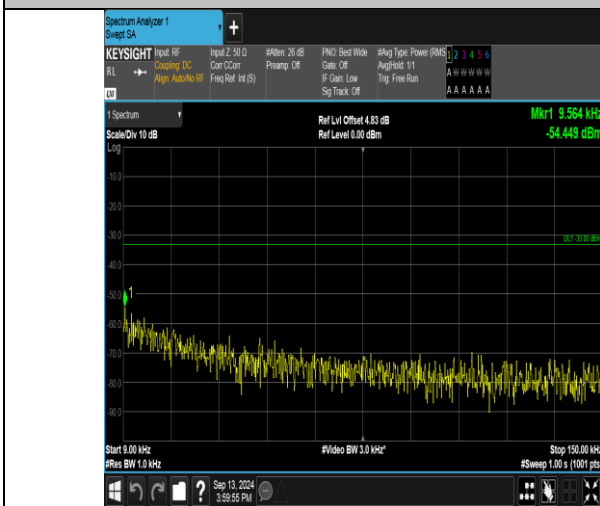
Band17_10MHz_QPSK_23800_1RB#49_0.009~0.15_0.009~0.15
