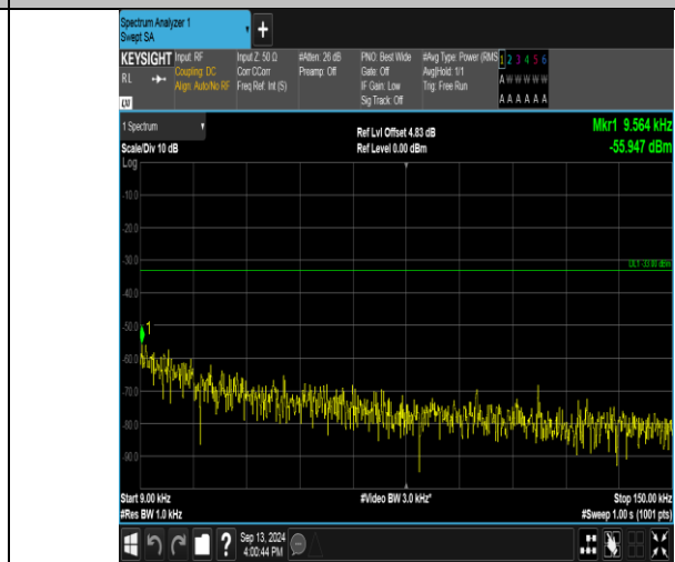
Band17_10MHz_16QAM_23800_1RB#49_0.009~0.15_0.009~0.15
