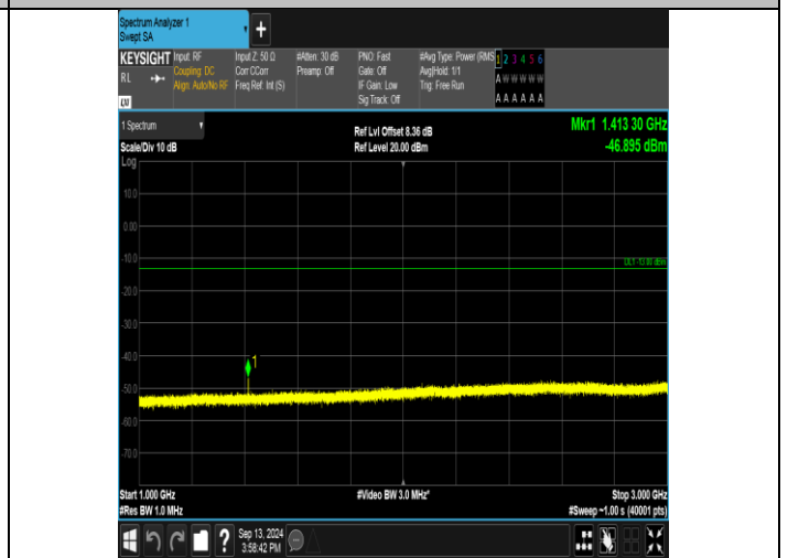
Band17_10MHz_QPSK_23800_1RB#0_1000-3000_1000-3000
