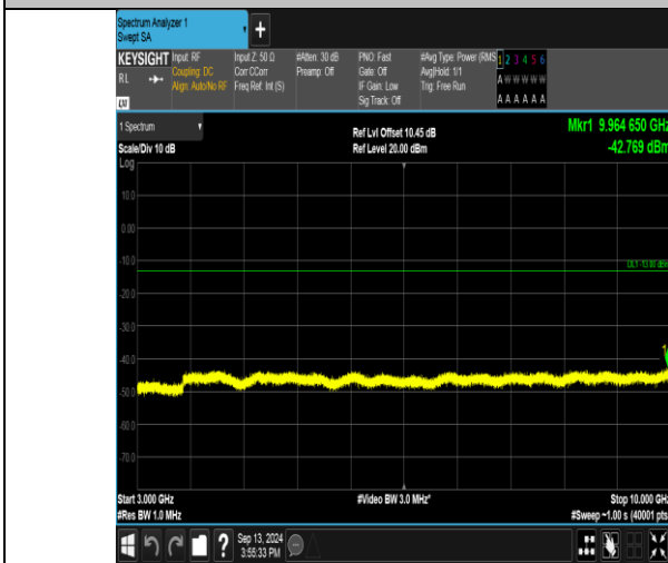
Band17_10MHz_QPSK_23790_1RB#49_3000~10000_3000~10000
