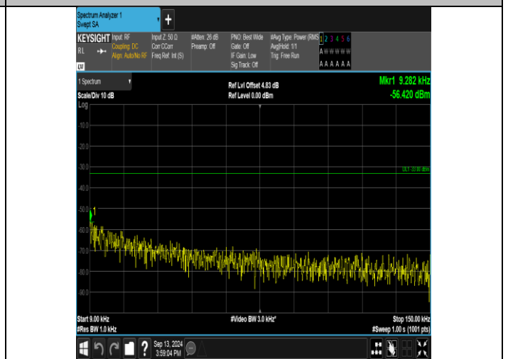
Band17_10MHz_16QAM_23800_1RB#0_0.009-0.15_0.009-0.15
