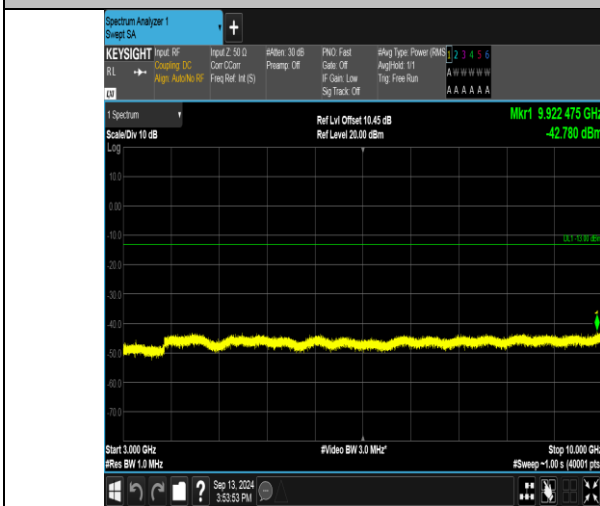
Band17_10MHz_QPSK_23790_1RB#0_3000-10000_3000-10000
