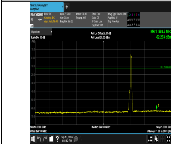
Band17_10MHz_QPSK_23800_50RB#0_30~1000_30~1000
