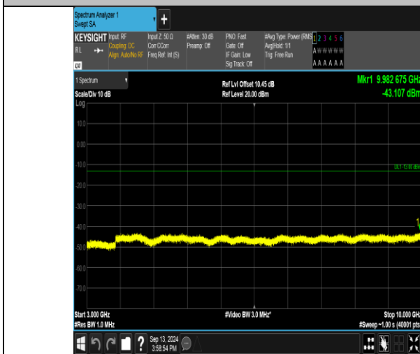
Band17_10MHz_QPSK_23800_1RB#0_3000-10000_3000-10000
