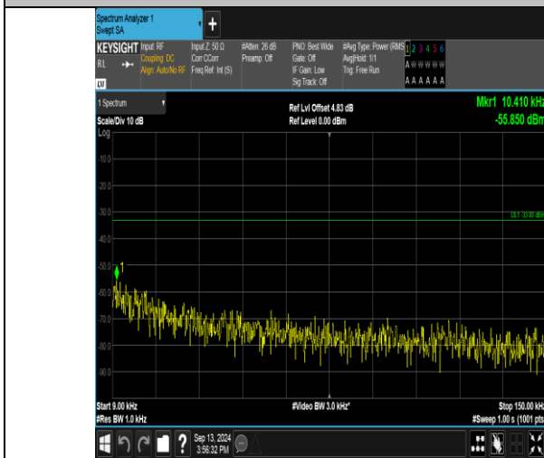
Band17_10MHz_QPSK_23790_50RB#0_0.009-0.15_0.009-0.15
