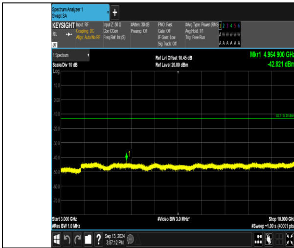
Band17_10MHz_QPSK_23790_50RB#0_3000~10000_3000~10000
