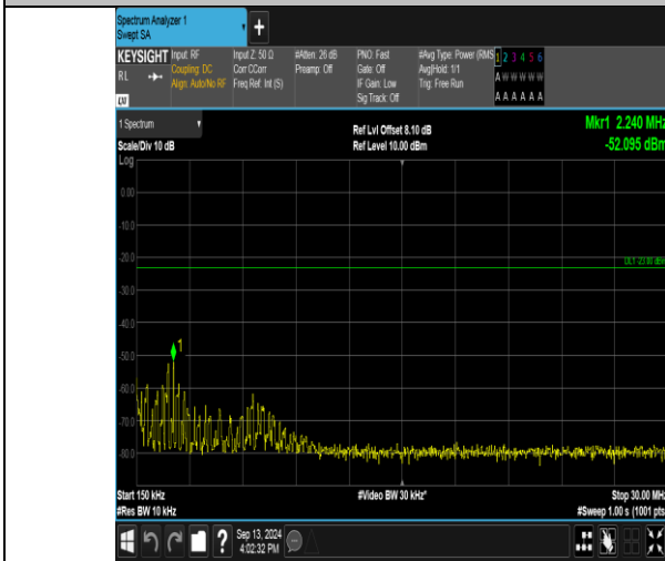
Band17_10MHz_16QAM_23800_50RB#0_0.15~30_0.15~30
