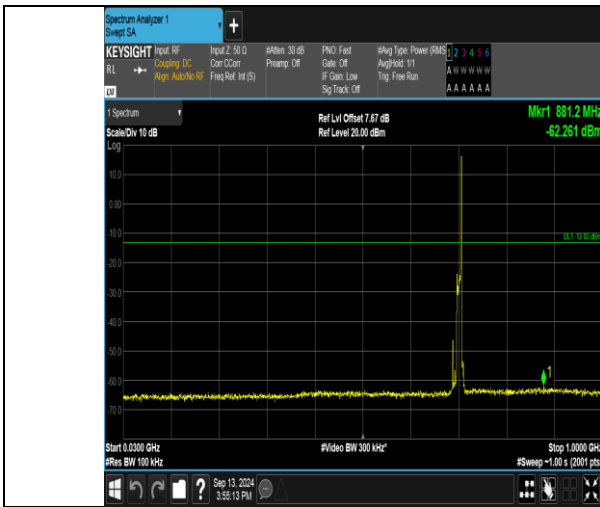
Band17_10MHz_QPSK_23790_1RB#49_30~1000_30~1000
