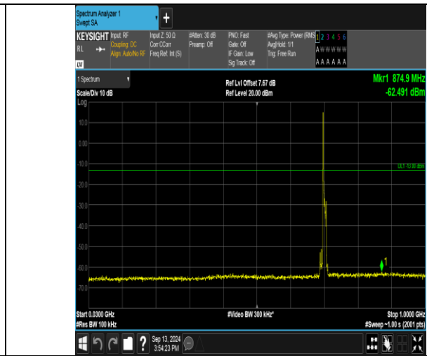
Band17_10MHz_16QAM_23790_1RB#0.30-1000_30-1000
