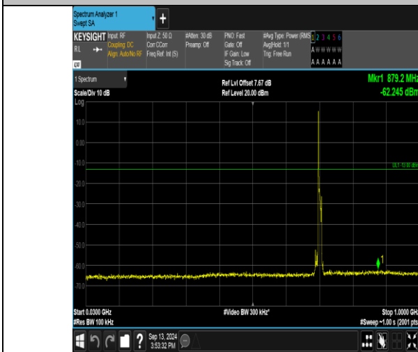
Band17_10MHz_QPSK_23790_1RB#0_30-1000_30-1000
