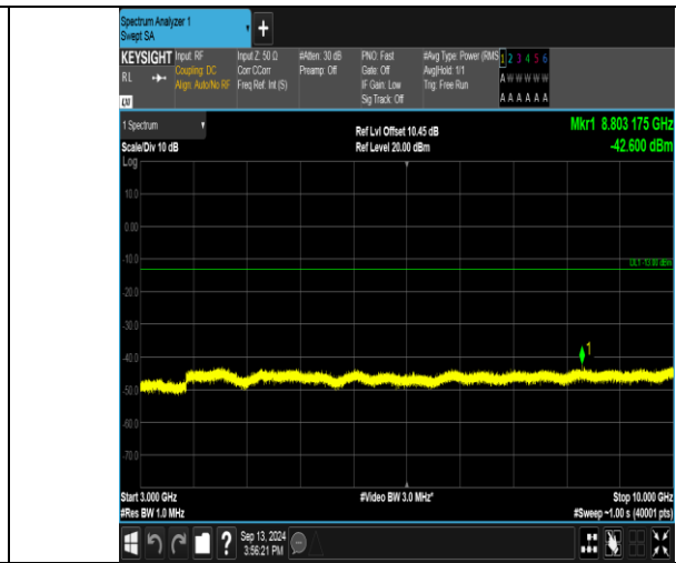
Band17_10MHz_16QAM_23790_1RB#49_3000-10000_3000-10000
