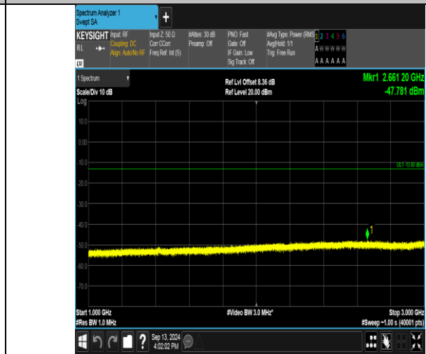
Band17_10MHz_QPSK_23800_50RB#0_1000~3000_1000~3000
