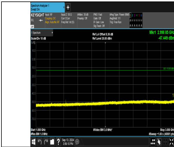
Band17_10MHz_16QAM_23790_1RB#49_1000-3000_1000-3000
