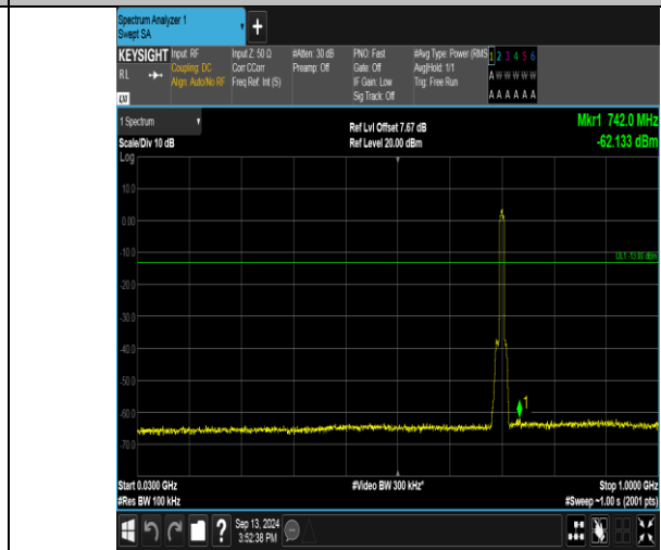
Band17_10MHz_16QAM_23780_50RB#0_30~1000_30~1000
