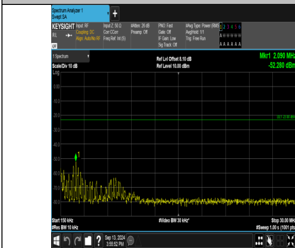
Band17_10MHz_16QAM_23790_1RB#49_0.15~30_0.15~30
