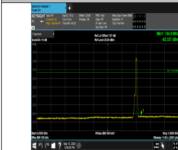
Band17_10MHz_QPSK_23790_50RB#0_30-1000_30-1000
