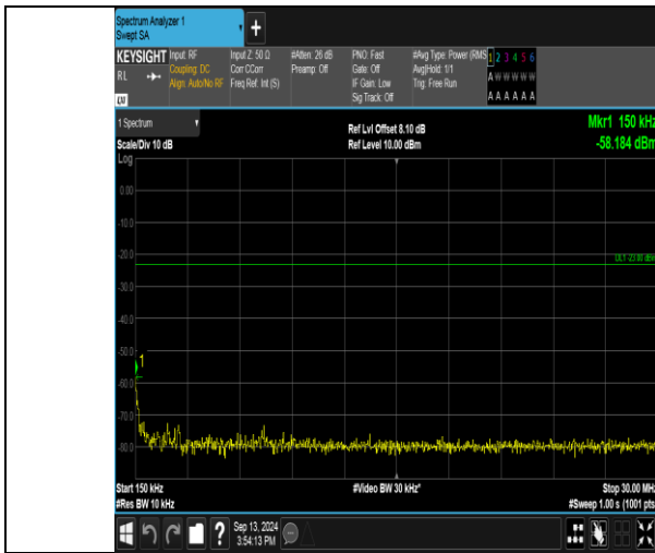
Band17_10MHz_16QAM_23790_1RB#0.015-30_0.15-30
