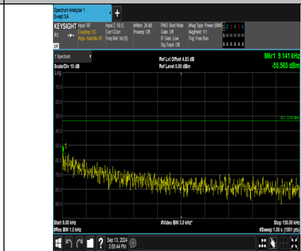
Band17_10MHz_16QAM_23790_1RB#49_0.009~0.15_0.009~0.15
