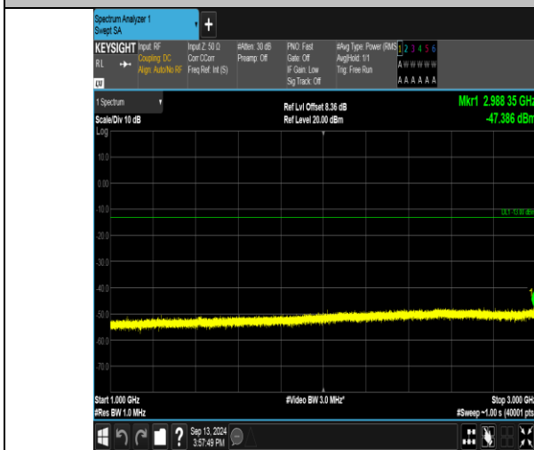
Band17_10MHz_16QAM_23790_50RB#0_1000~3000_1000~3000
