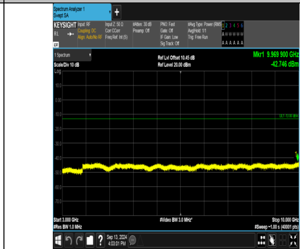
Band17_10MHz_16QAM_23800_50RB#0_3000~10000_3000~10000
