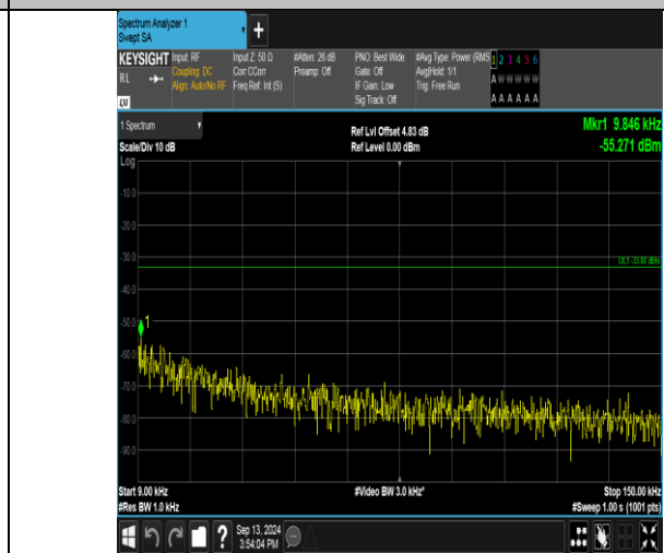
Band17_10MHz_16QAM_23790_1RB#0_0.009-0.15_0.009-0.15
