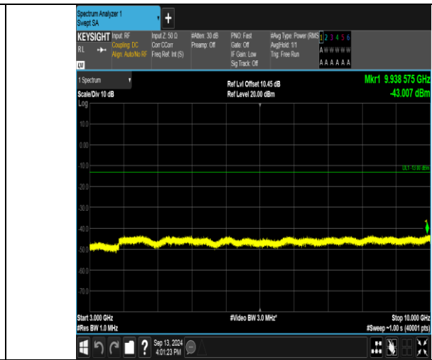
Band17_10MHz_16QAM_23800_1RB#49_3000~10000_3000~10000
