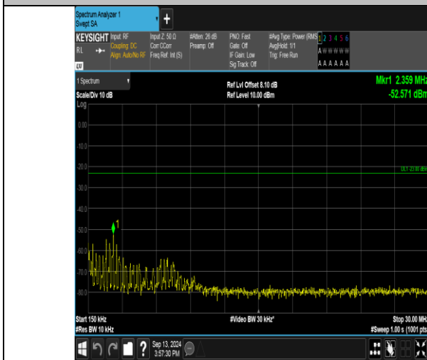
Band17_10MHz_16QAM_23790_50RB#0_0.15~30_0.15~30
