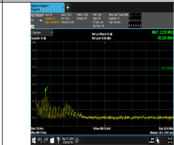
Band17_10MHz_QPSK_23790_50RB#0_0.15-30_0.15-30
