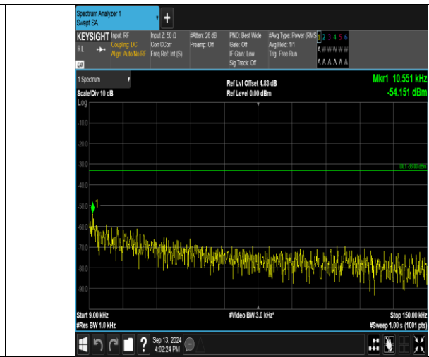
Band17_10MHz_16QAM_23800_50RB#0_0.009~0.15_0.009~0.15
