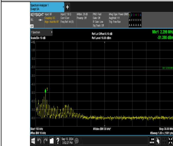
Band17_10MHz_16QAM_23780_50RB#0_0.15~30_0.15~30
