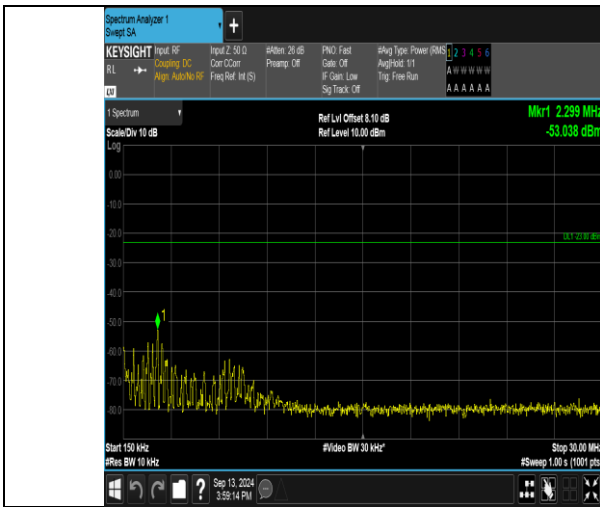
Band17_10MHz_16QAM_23800_1RB#0_0.15~30_0.15~30
