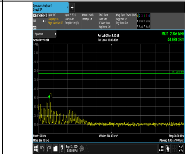
Band17_10MHz_QPSK_23790_1RB#49.015-30_0.15-30
