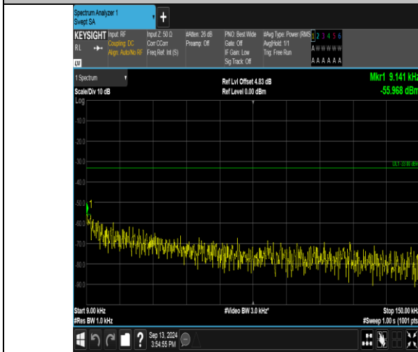
Band17_10MHz_QPSK_23790_1RB#49.0009-0.15_0.009-0.15
