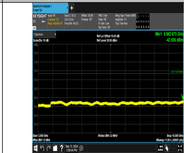
Band17_10MHz_16QAM_23800_1RB#0_3000~10000_3000~10000
