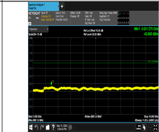
Band17_10MHz_16QAM_23790_1RB#0.3000-10000_3000-10000
