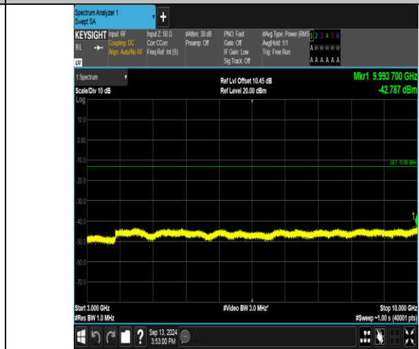
Band17_10MHz_16QAM_23780_50RB#0_3000~10000_3000~10000
