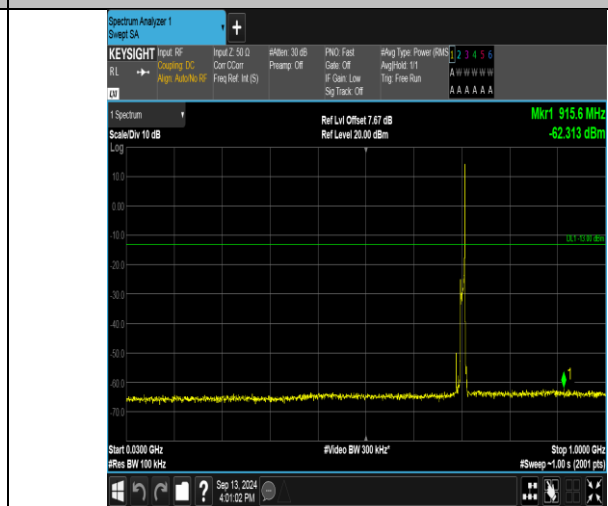
Band17_10MHz_16QAM_23800_1RB#49_30~1000_30~1000
