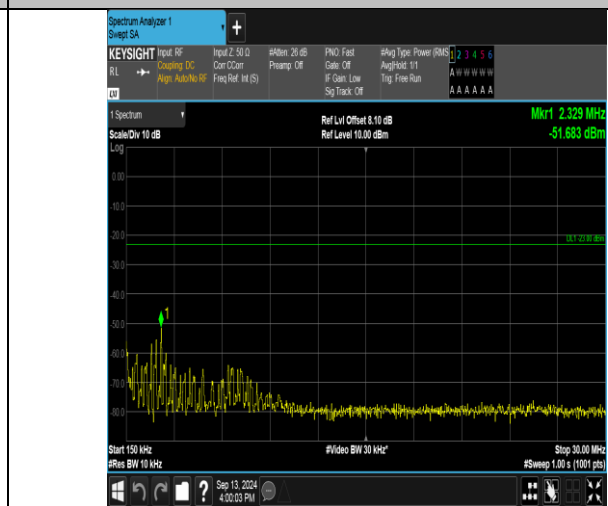
Band17_10MHz_QPSK_23800_1RB#49_0.15~30_0.15~30
