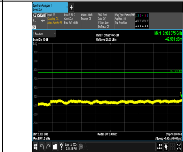
Band17_5MHz_16QAM_23790_25RB#0_3000~10000_3000~10000
