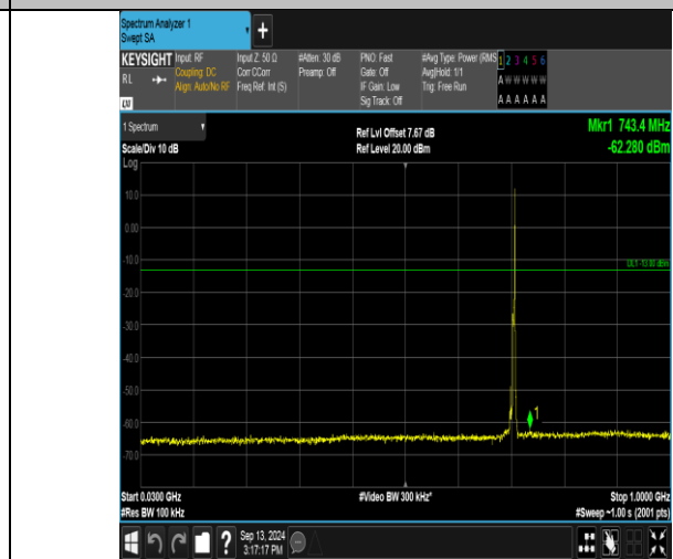
Band17_5MHz_16QAM_23825_1RB#24_30~1000_30~1000
