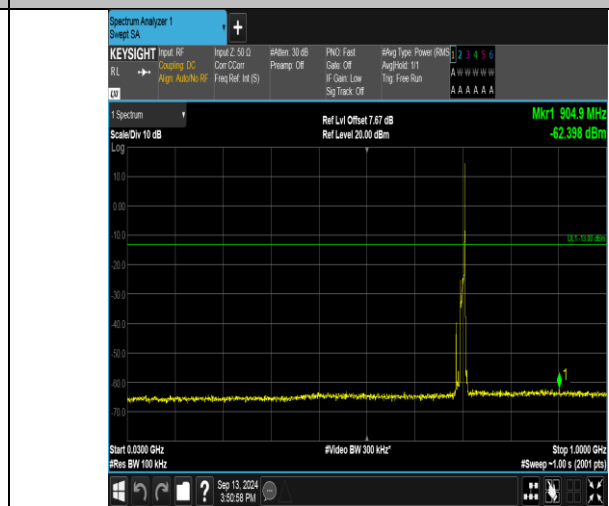
Band17_10MHz_16QAM_23780_1RB#49_30~1000_30~1000
