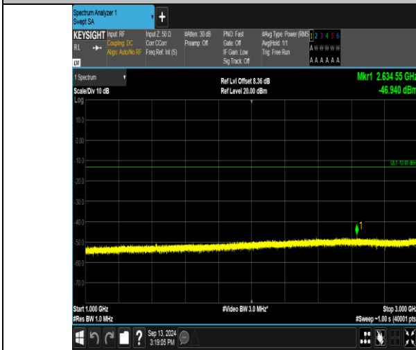
Band17_5MHz_16QAM_23825_25RB#0_1000~3000_1000~3000
