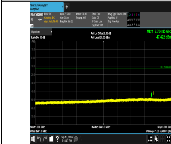
Band17_5MHz_16QAM_23790_25RB#0_1000~3000_1000~3000
