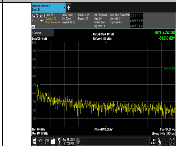
Band17_5MHz_16QAM_23825_1RB#24_0.009~0.15_0.009~0.15
