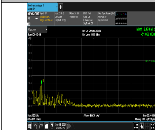
Band17_10MHz_16QAM_23780_1RB#49_0.15~30_0.15~30
