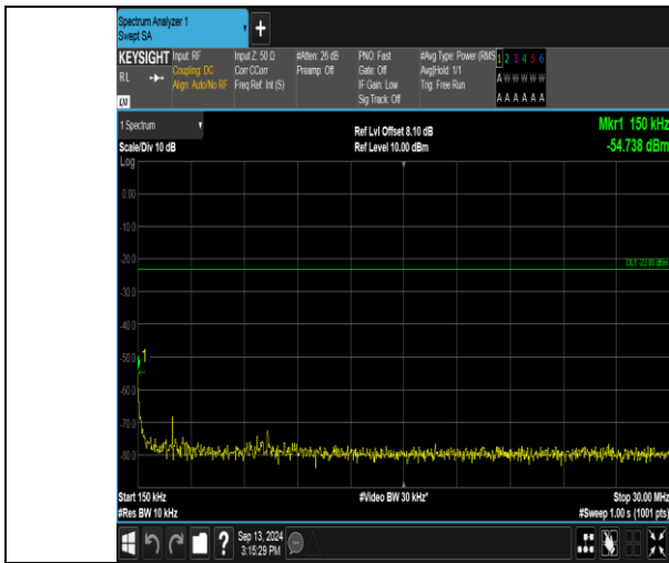
Band17_5MHz_16QAM_23825_1RB#0_0.15~30_0.15~30
