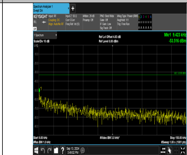
Band17_10MHz_16QAM_23780_1RB#0_0.009-0.15_0.009-0.15
