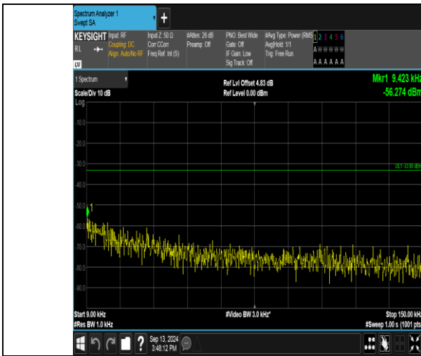
Band17_10MHz_QPSK_23780_1RB#0_0.009-0.15_0.009-0.15
