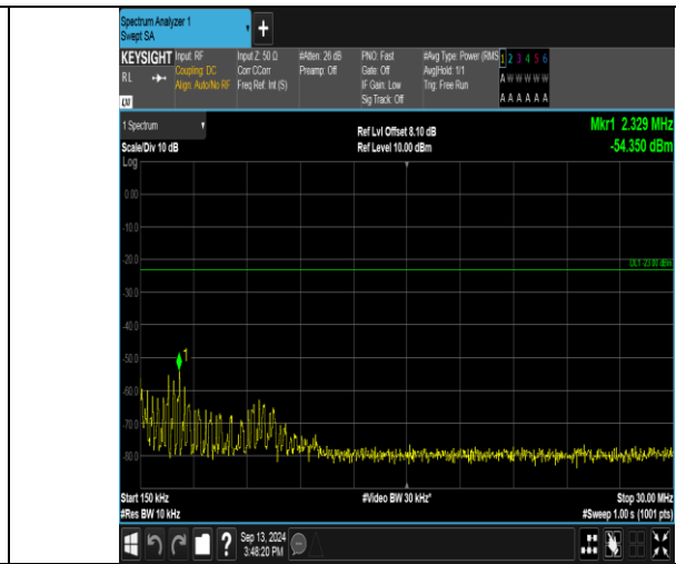
Band17_10MHz_QPSK_23780_1RB#0_0.15-30_0.15-30
