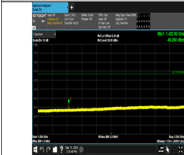
Band17_5MHz_16QAM_23825_1RB#0_1000~3000_1000~3000
