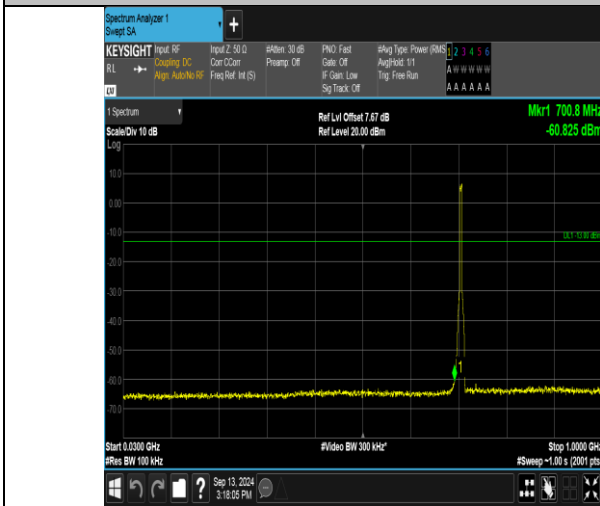
Band17_5MHz_QPSK_23825_25RB#0_30-1000_30-1000
