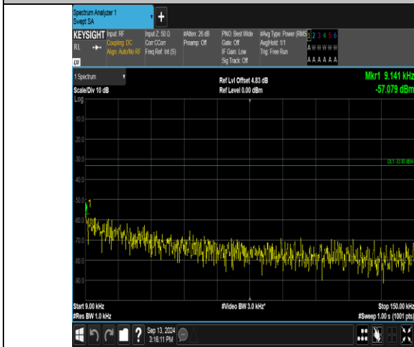
Band17_5MHz_QPSK_23825_1RB#24_0.009~0.15_0.009~0.15
