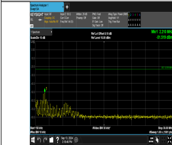
Band17_5MHz_16QAM_23825_25RB#0_0.15~30_0.15~30
