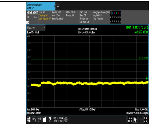
Band17_5MHz_16QAM_23825_1RB#24_3000-10000_3000-10000
