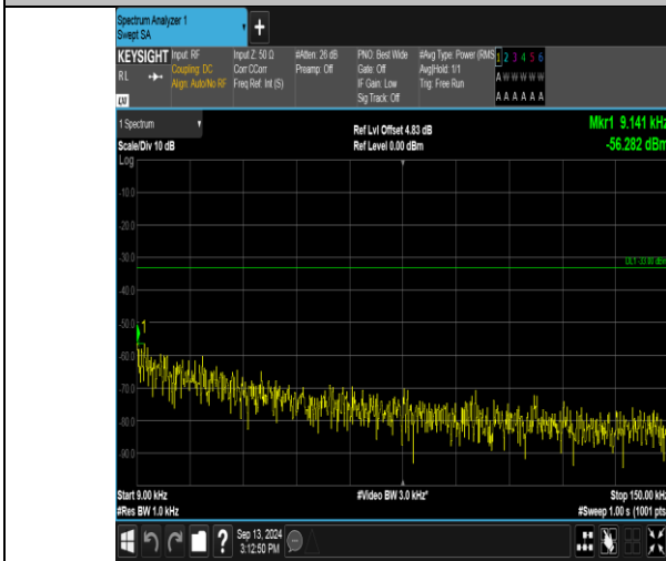
Band17_5MHz_QPSK_23790_25RB#0_0.009-0.15_0.009-0.15
