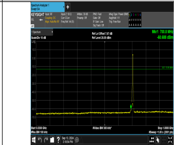
Band17_5MHz_16QAM_23825_25RB#0_30~1000_30~1000
