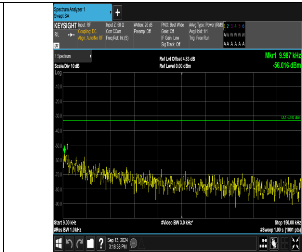
Band17_5MHz_16QAM_23825_25RB#0_0.009~0.15_0.009~0.15
