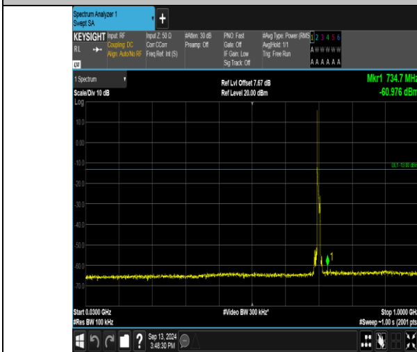
Band17_10MHz_QPSK_23780_1RB#0_30-1000_30-1000
