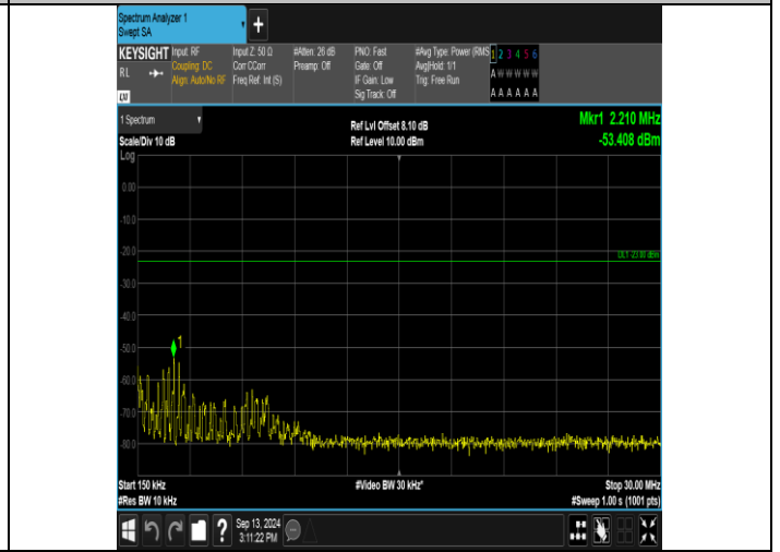
Band17_5MHz_QPSK_23790_1RB#24_0.15~30_0.15~30
