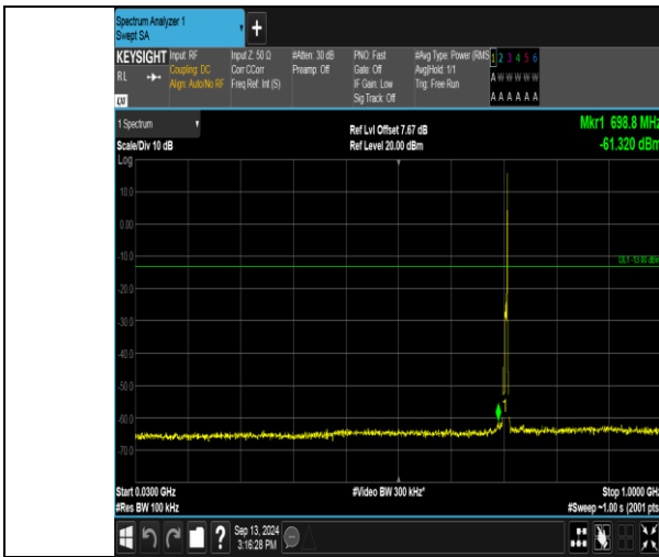
Band17_5MHz_QPSK_23825_1RB#24_30~1000_30~1000
