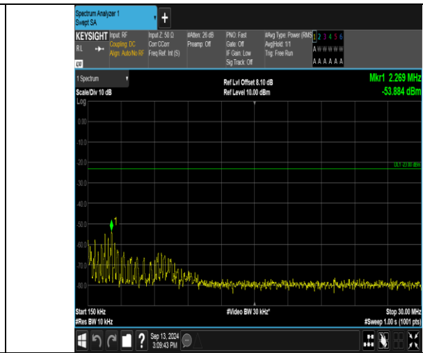
Band17_5MHz_QPSK_23790_1RB#0_0.15-30_0.15-30
