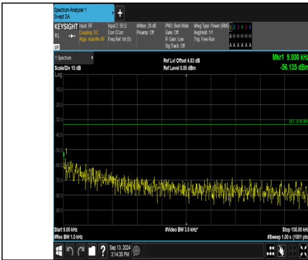
Band17_5MHz_QPSK_23825_1RB#0_0.009-0.15_0.009-0.15
