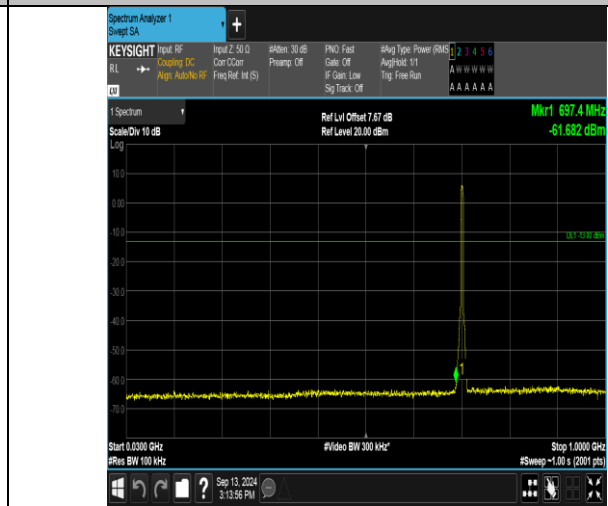
Band17_5MHz_16QAM_23790_25RB#0_30~1000_30~1000
