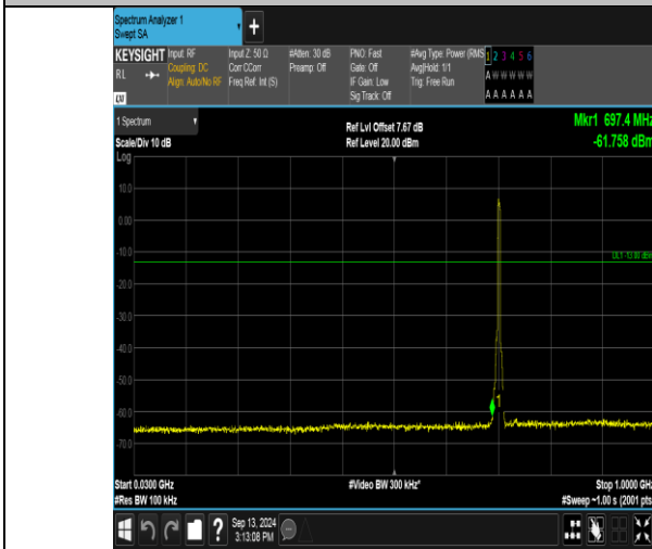
Band17_5MHz_QPSK_23790_25RB#0_30-1000_30-1000
