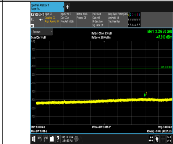
Band17_10MHz_QPSK_23780_50RB#0_1000-3000_1000-3000
