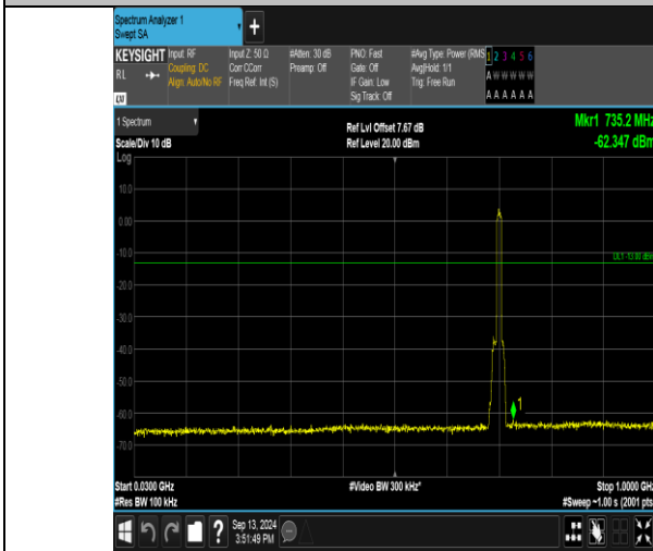
Band17_10MHz_QPSK_23780_50RB#0_30-1000_30-1000
