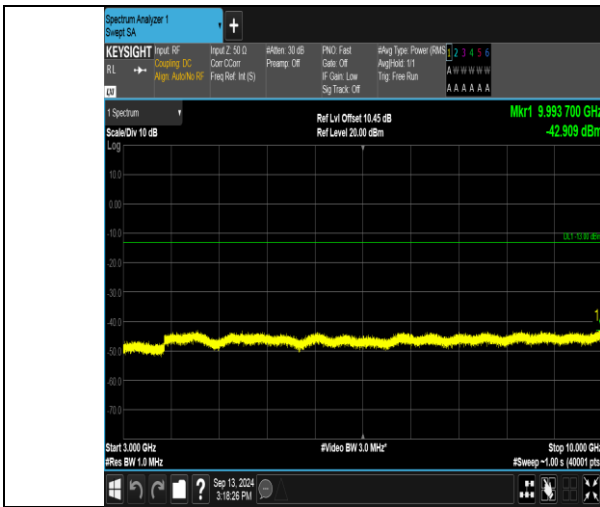
Band17_5MHz_QPSK_23825_25RB#0_3000~10000_3000~10000
