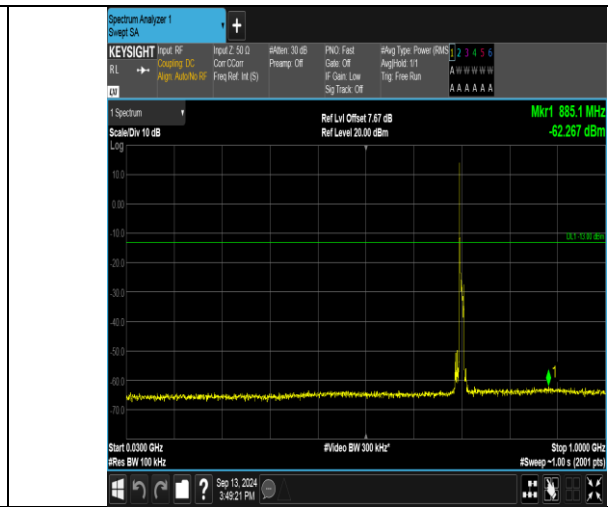
Band17_10MHz_16QAM_23780_1RB#0.30-1000_30-1000
