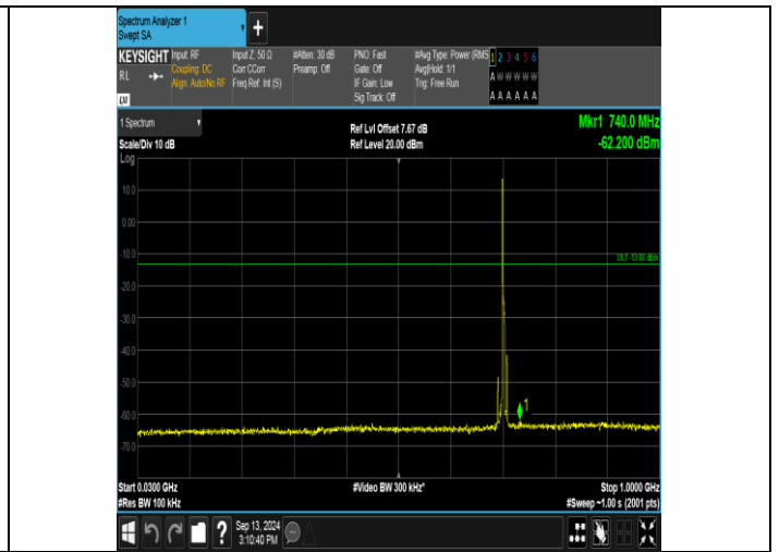
Band17_5MHz_16QAM_23790_1RB#0_30~1000_30~1000
