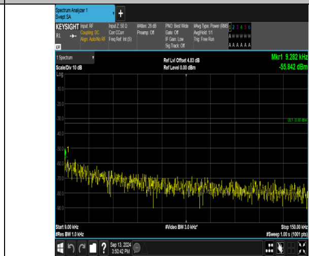
Band17_10MHz_16QAM_23780_1RB#49_0.009~0.15_0.009~0.15
