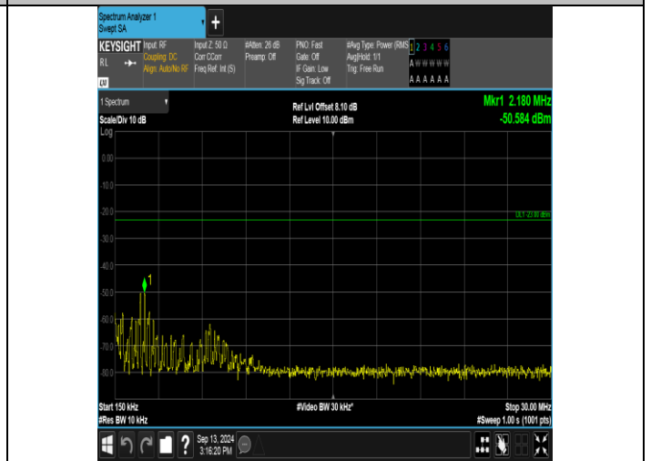
Band17_5MHz_QPSK_23825_1RB#24_0.15~30_0.15~30
