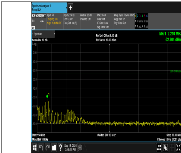
Band17_10MHz_16QAM_23780_1RB#0.015-30_0.15-30
