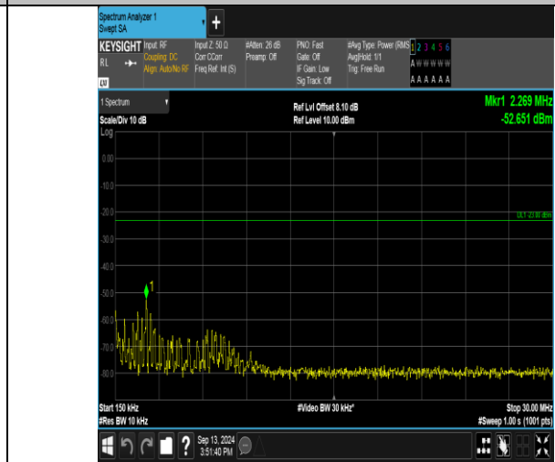
Band17_10MHz_QPSK_23780_50RB#0_0.15-30_0.15-30
