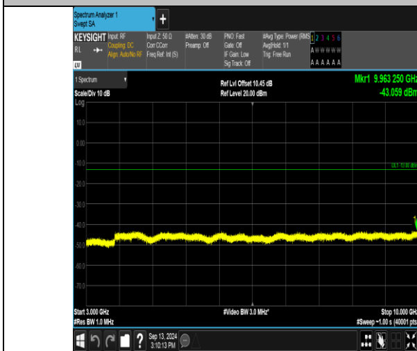
Band17_5MHz_QPSK_23790_1RB#0_3000-10000_3000-10000
