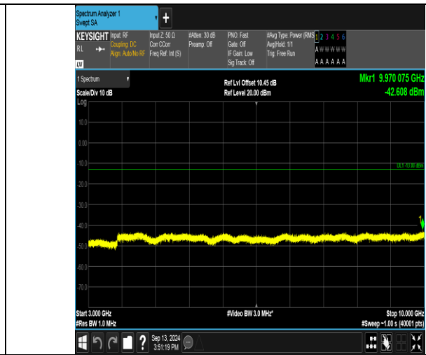
Band17_10MHz_16QAM_23780_1RB#49_3000-10000_3000-10000
