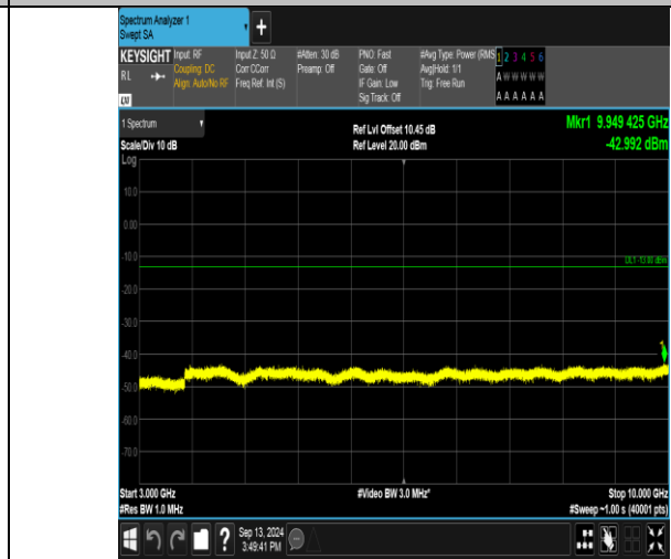
Band17_10MHz_16QAM_23780_1RB#0.3000-10000_3000-10000
