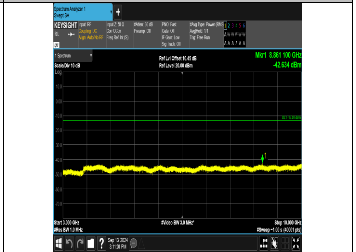
Band17_5MHz_16QAM_23790_1RB#0_3000~10000_3000~10000
