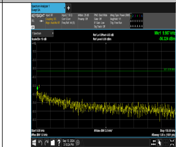
Band17_5MHz_16QAM_23790_1RB#0_0.009-0.15_0.009-0.15
