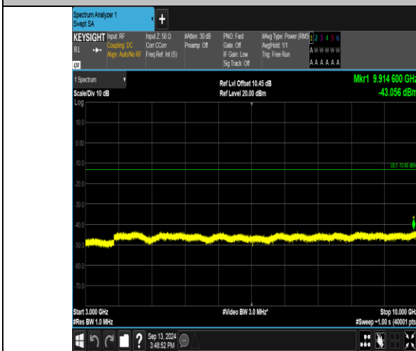
Band17_10MHz_QPSK_23780_1RB#0_3000-10000_3000-10000
