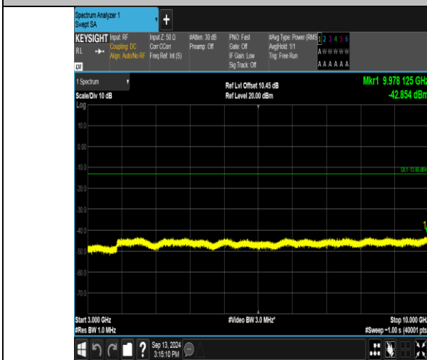
Band17_5MHz_QPSK_23825_1RB#0_3000-10000_3000-10000
