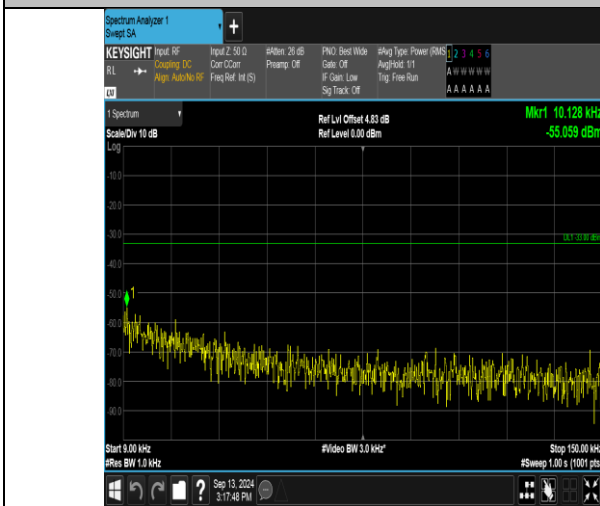
Band17_5MHz_QPSK_23825_25RB#0_0.009-0.15_0.009-0.15
