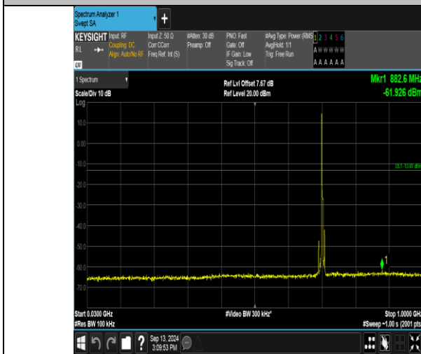
Band17_5MHz_QPSK_23790_1RB#0_30-1000_30-1000
