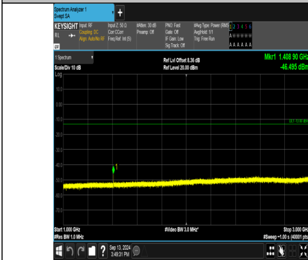
Band17_10MHz_16QAM_23780_1RB#0.1000-3000_1000-3000
