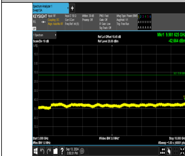
Band17_10MHz_QPSK_23780_1RB#49_3000~10000_3000~10000
