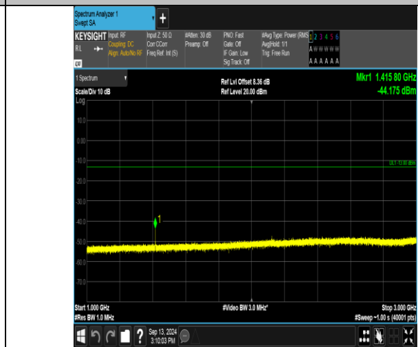
Band17_5MHz_QPSK_23790_1RB#0_1000-3000_1000-3000
