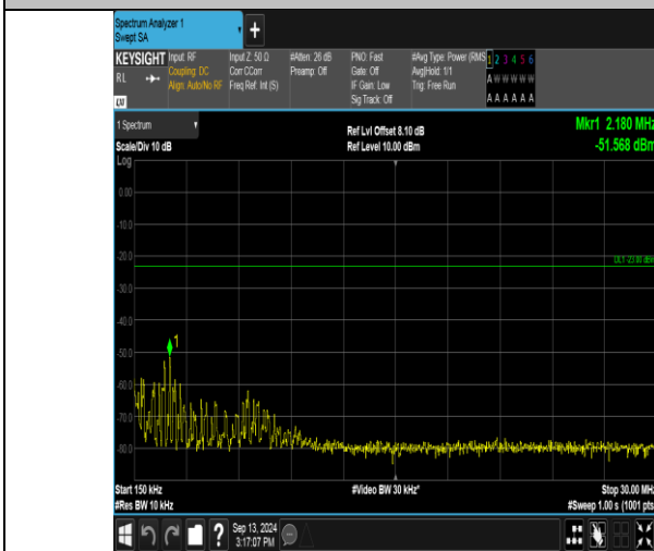
Band17_5MHz_16QAM_23825_1RB#24_0.15~30_0.15~30
