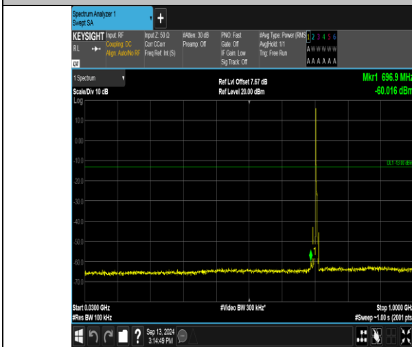
Band17_5MHz_QPSK_23825_1RB#0_30-1000_30-1000
