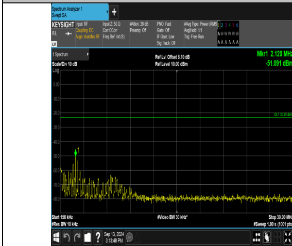
Band17_5MHz_16QAM_23790_25RB#0_0.15~30_0.15~30
