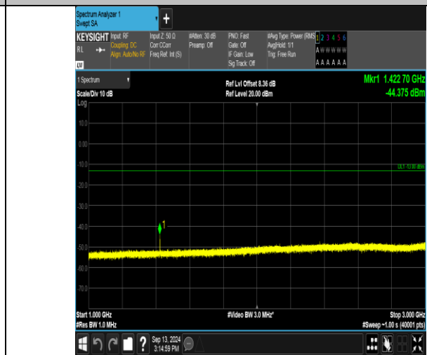
Band17_5MHz_QPSK_23825_1RB#0_1000-3000_1000-3000
