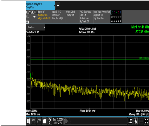
Band17_5MHz_QPSK_23790_1RB#24_0.009~0.15_0.009~0.15
