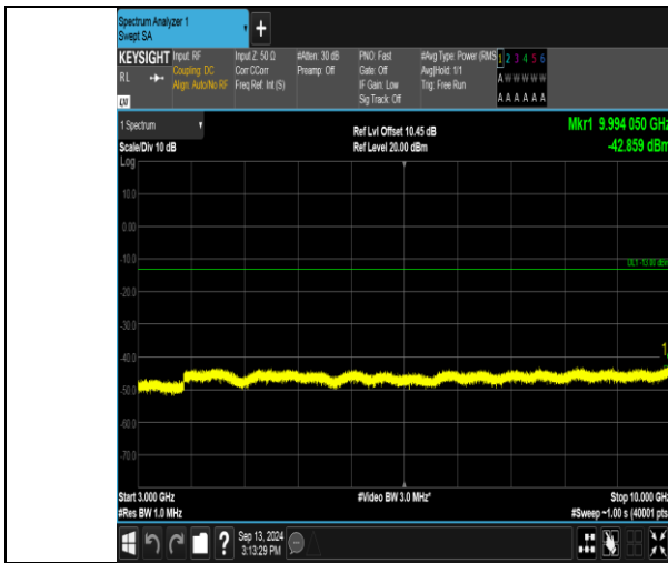
Band17_5MHz_QPSK_23790_25RB#0_3000~10000_3000~10000
