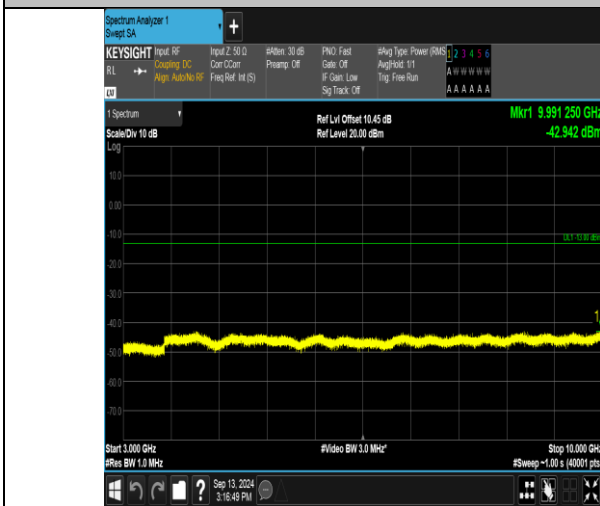
Band17_5MHz_QPSK_23825_1RB#24_3000~10000_3000~10000
