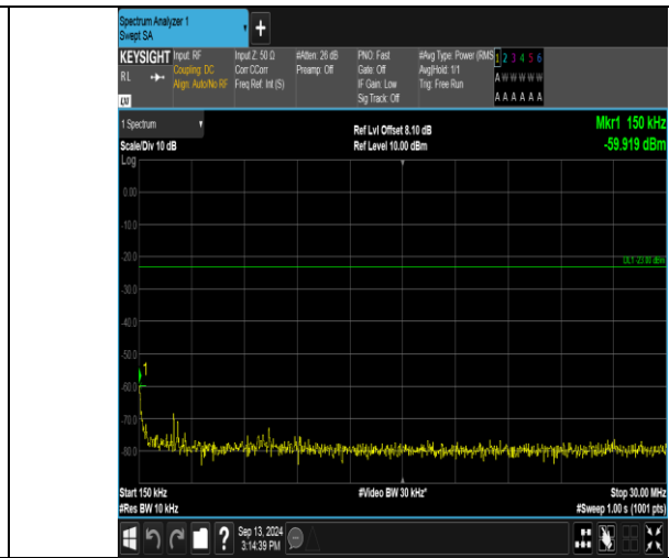
Band17_5MHz_QPSK_23825_1RB#0_0.15-30_0.15-30
