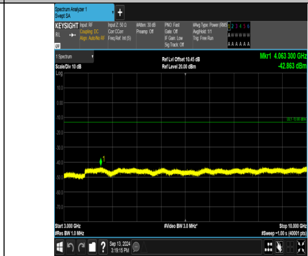
Band17_5MHz_16QAM_23825_25RB#0_3000~10000_3000~10000
