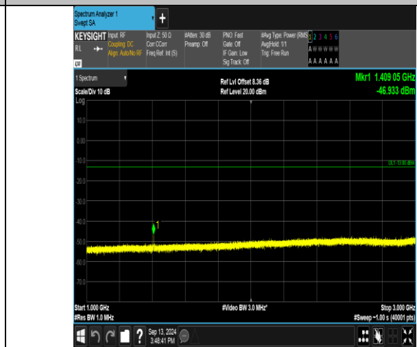
Band17_10MHz_QPSK_23780_1RB#0_1000-3000_1000-3000
