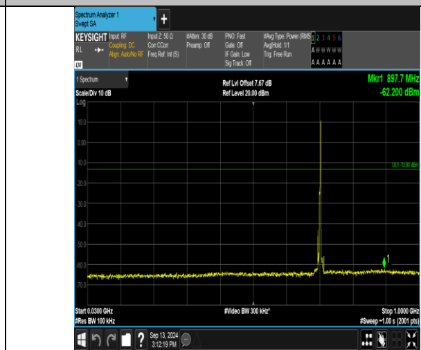
Band17_5MHz_16QAM_23790_1RB#24_30~1000_30~1000
