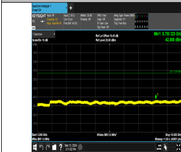
Band17_5MHz_QPSK_23790_1RB#24_3000~10000_3000~10000
