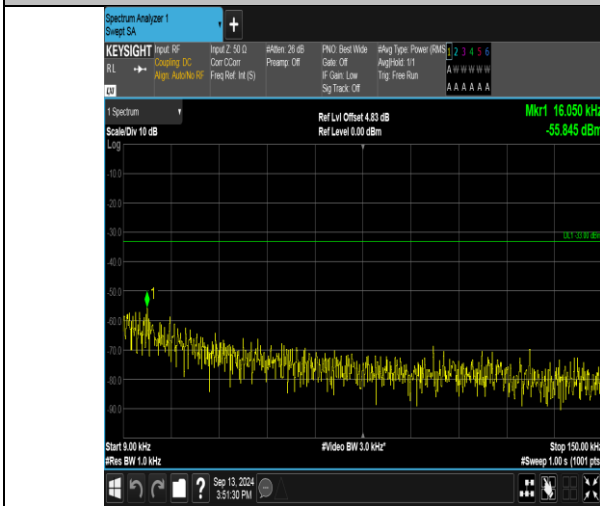
Band17_10MHz_QPSK_23780_50RB#0_0.009-0.15_0.009-0.15
