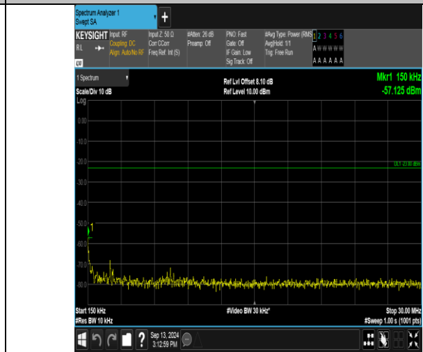
Band17_5MHz_QPSK_23790_25RB#0_0.15-30_0.15-30
