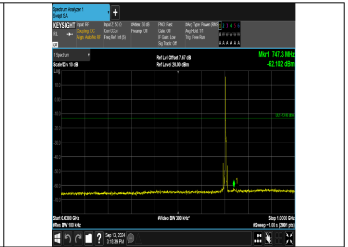
Band17_5MHz_16QAM_23825_1RB#0_30~1000_30~1000
