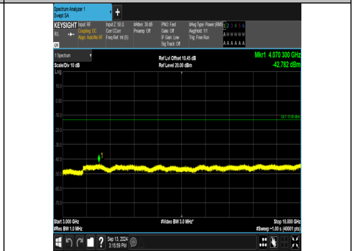
Band17_5MHz_16QAM_23825_1RB#0_3000~10000_3000~10000
