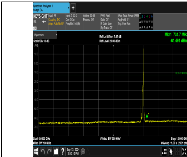
Band17_10MHz_QPSK_23780_1RB#49_30~1000_30~1000
