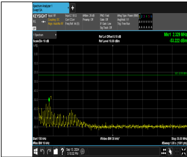
Band17_5MHz_16QAM_23790_1RB#0_0.15~30_0.15~30
