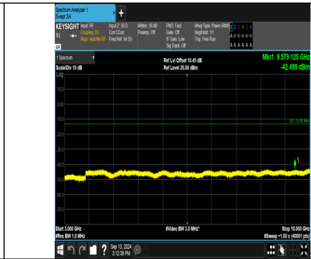
Band17_5MHz_16QAM_23790_1RB#24_3000-10000_3000-10000
