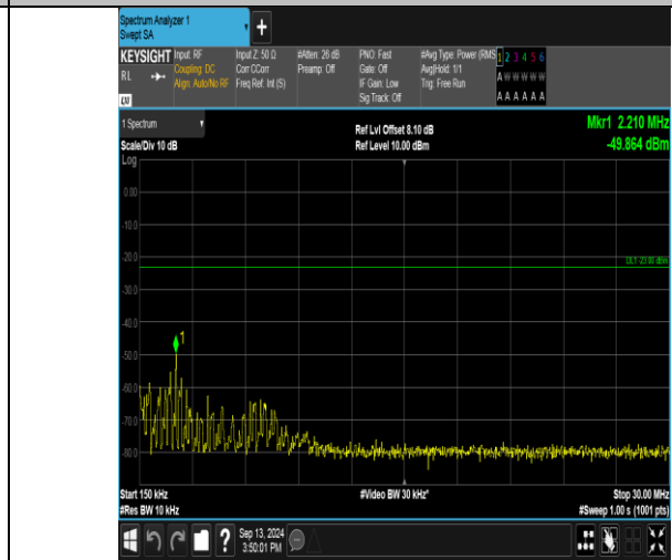
Band17_10MHz_QPSK_23780_1RB#49.015-30_0.15-30
