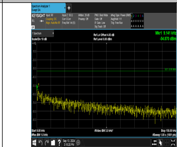
Band17_5MHz_16QAM_23825_1RB#0_0.009-0.15_0.009-0.15
