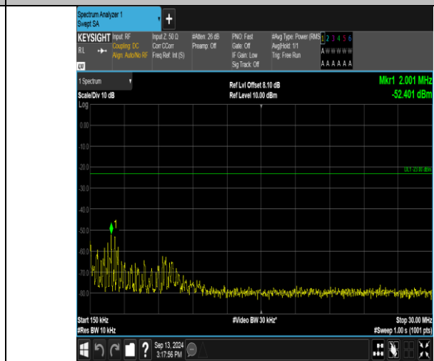
Band17_5MHz_QPSK_23825_25RB#0_0.15-30_0.15-30
