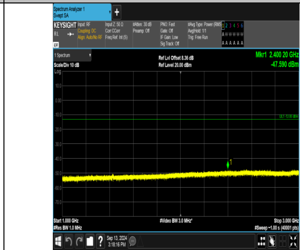
Band17_5MHz_QPSK_23825_25RB#0_1000-3000_1000-3000
