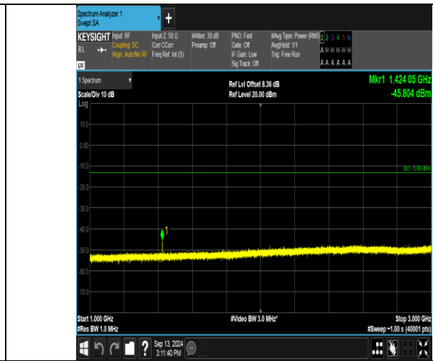
Band17_5MHz_QPSK_23790_1RB#24_1000~3000_1000~3000
