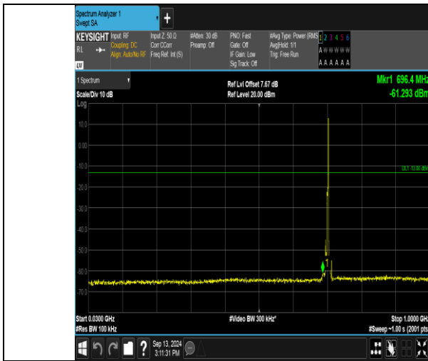
Band17_5MHz_QPSK_23790_1RB#24_30~1000_30~1000
