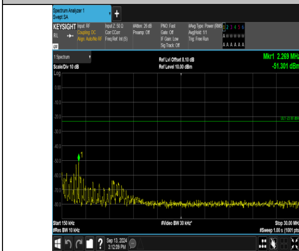
Band17_5MHz_16QAM_23790_1RB#24_0.15~30_0.15~30
