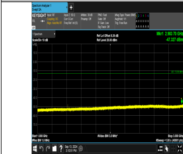
Band17_5MHz_16QAM_23790_1RB#0_1000~3000_1000~3000
