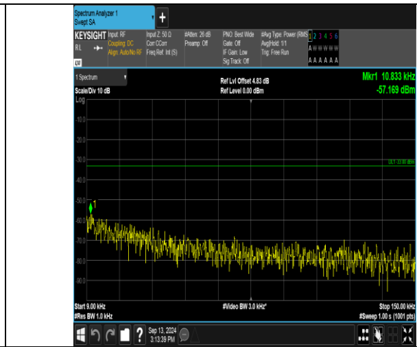
Band17_5MHz_16QAM_23790_25RB#0_0.009~0.15_0.009~0.15
