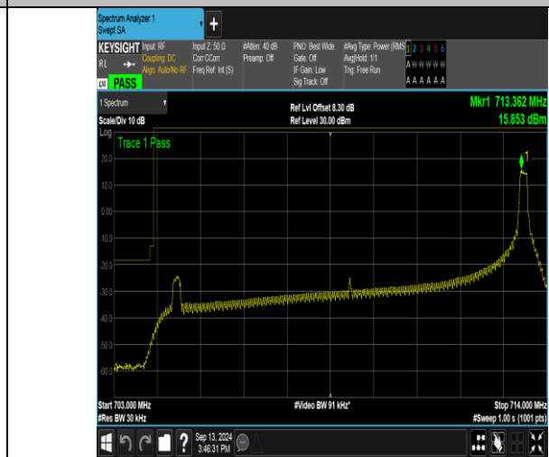
Band17_10MHz_16QAM_23780_1RB#49
