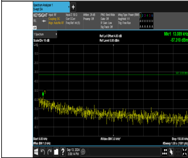
Band17_5MHz_QPSK_23755_1RB#24_0.009~0.15_0.009~0.15
