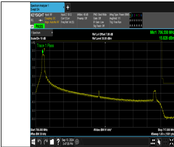
Band17_10MHz_QPSK_23800_1RB#0
