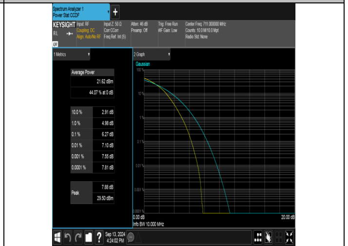
Band17-10MHz-16QAM-23800-50RB#0-PASS
