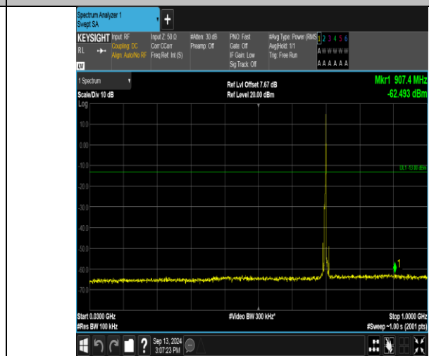
Band17_5MHz_16QAM_23755_1RB#24_30~1000_30~1000
