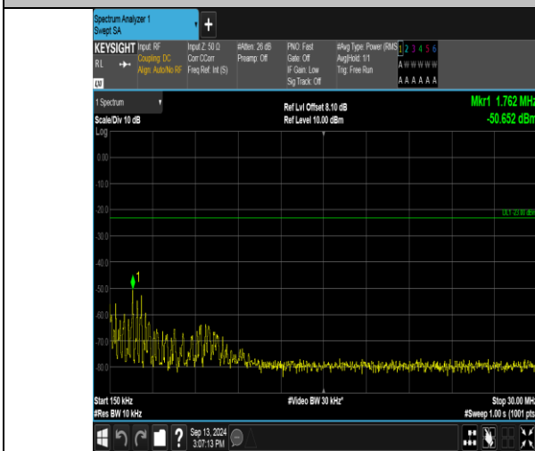
Band17_5MHz_16QAM_23755_1RB#24_0.15~30_0.15~30
