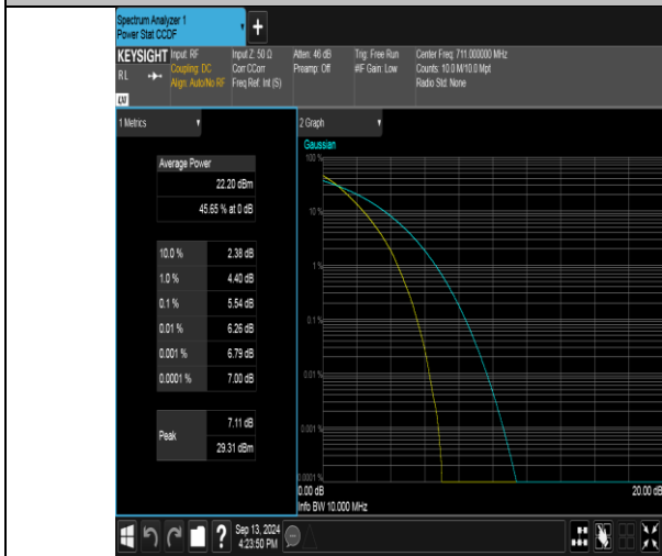
Band17-10MHz-QPSK-23800-50RB#0-PASS
