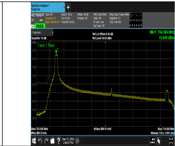
Band17_10MHz_16QAM_23780_1RB#0
