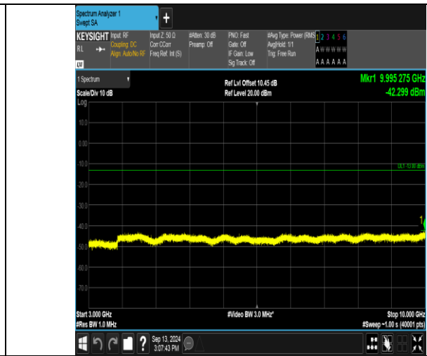
Band17_5MHz_16QAM_23755_1RB#24_3000-10000_3000-10000
