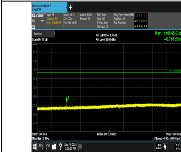
Band17_5MHz_16QAM_23755_1RB#0_1000~3000_1000~3000
