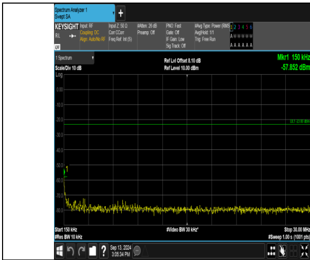
Band17_5MHz_16QAM_23755_1RB#0_0.15~30_0.15~30
