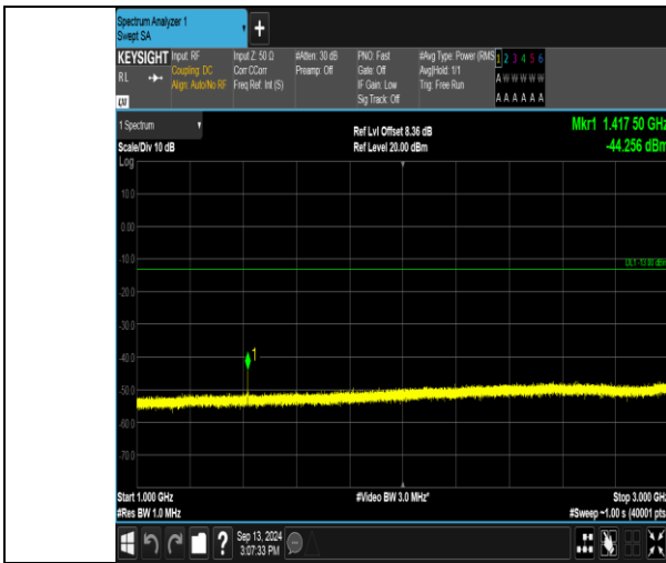
Band17_5MHz_16QAM_23755_1RB#24_1000-3000_1000-3000
