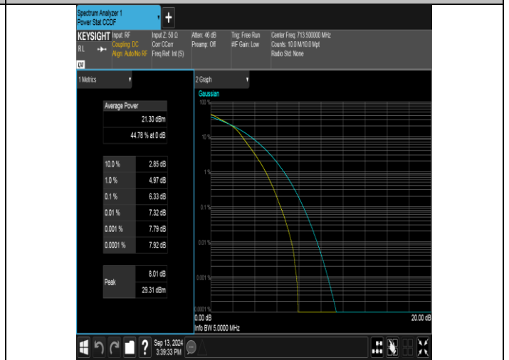
Band17-5MHz-16QAM-23825-25RB#0-PASS
