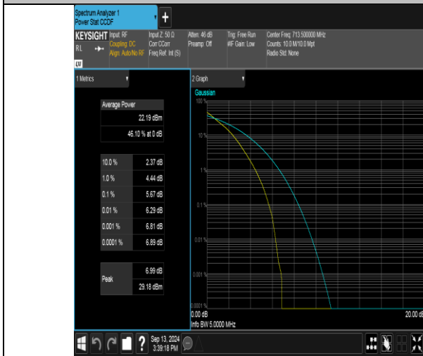
Band17-5MHz-QPSK-23825-25RB#0-PASS
