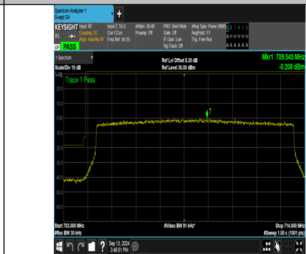
Band17_10MHz_16QAM_23780_50RB#0
