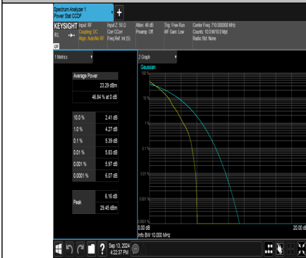
Band17-10MHz-QPSK-23790-1RB#0-PASS
