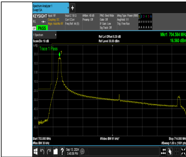
Band17_10MHz_QPSK_23780_1RB#0
