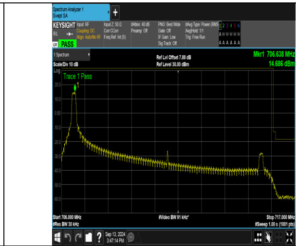
Band17_10MHz_16QAM_23800_1RB#0
