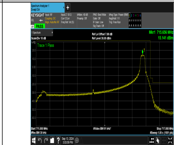
Band17_5MHz_16QAM_23825_1RB#24
