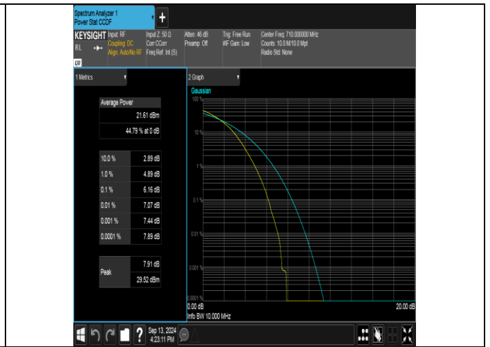
Band17-10MHz-16QAM-23790-50RB#0-PASS
