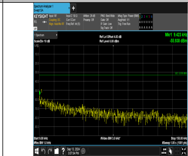
Band17_5MHz_16QAM_23755_1RB#24_0.009~0.15_0.009~0.15
