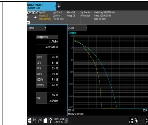
Band17-10MHz-16QAM-23780-1RB#0-PASS
