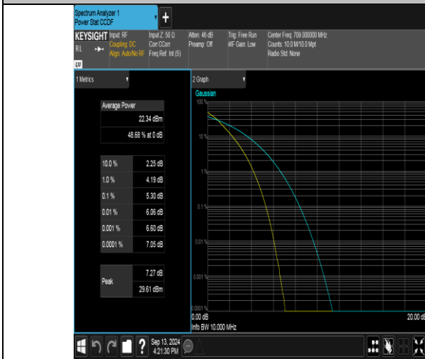
Band17-10MHz-QPSK-23780-50RB#0-PASS
