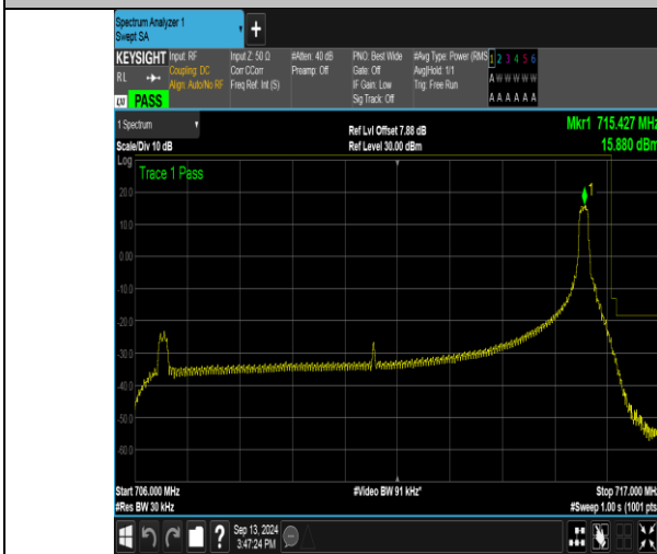
Band17_10MHz_QPSK_23800_1RB#49
