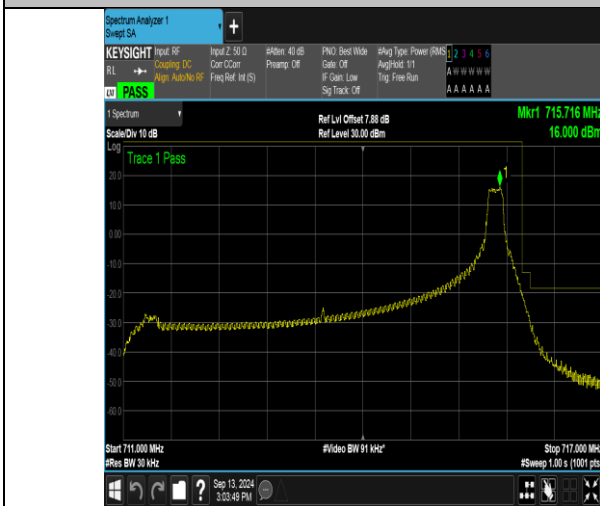
Band17_5MHz_QPSK_23825_1RB#24
