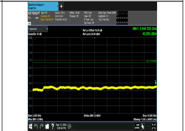
Band17_5MHz_16QAM_23755_1RB#0_3000~10000_3000~10000
