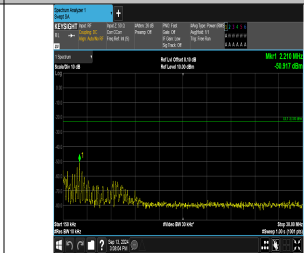
Band17_5MHz_QPSK_23755_25RB#0_0.15-30_0.15-30
