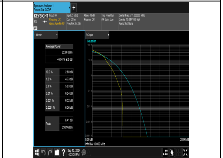
Band17-10MHz-16QAM-23800-1RB#0-PASS
