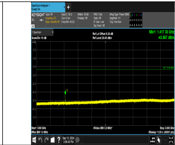
Band17_5MHz_QPSK_23755_1RB#24_1000~3000_1000~3000
