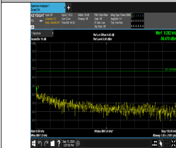
Band17_5MHz_QPSK_23755_25RB#0_0.009-0.15_0.009-0.15
