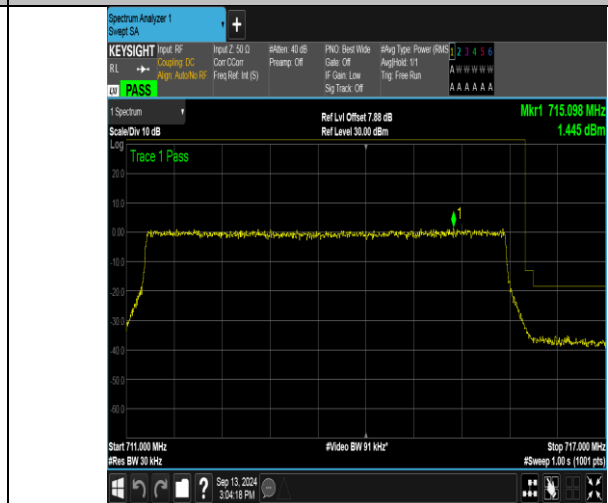
Band17_5MHz_16QAM_23825_25RB#0
