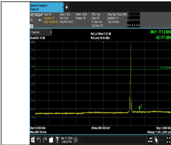
Band17_5MHz_QPSK_23755_1RB#24_30~1000_30~1000
