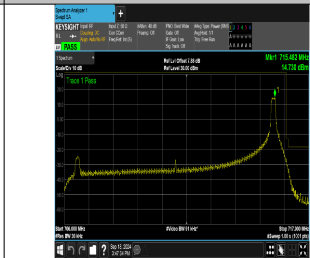
Band17_10MHz_16QAM_23800_1RB#49
