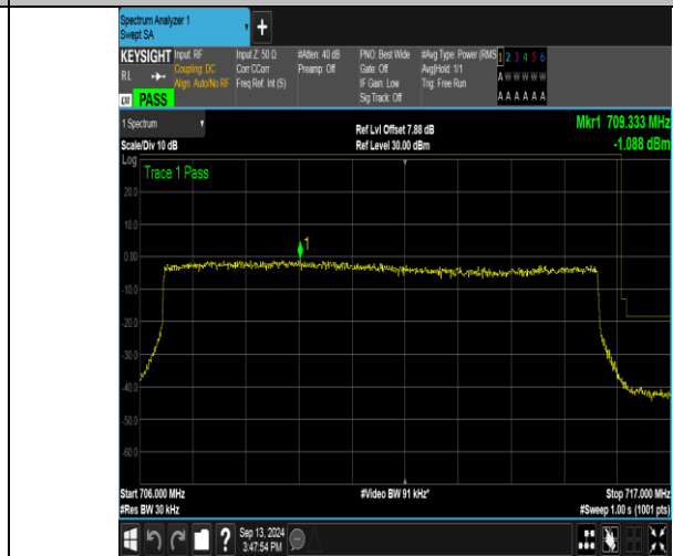
Band17_10MHz_16QAM_23800_50RB#0
