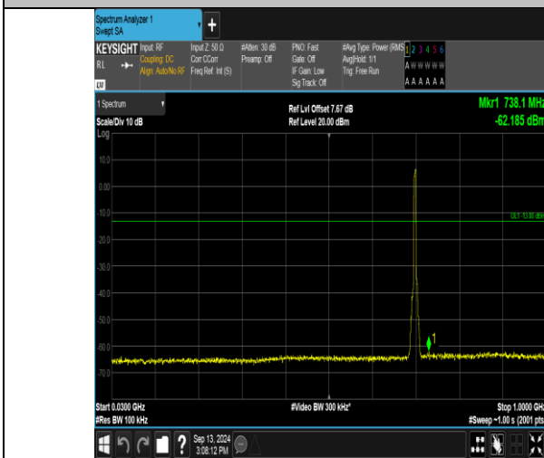
Band17_5MHz_QPSK_23755_25RB#0_30-1000_30-1000
