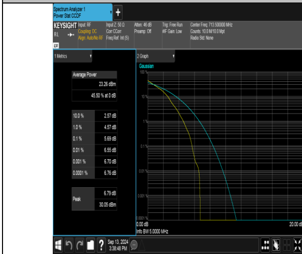
Band17-5MHz-QPSK-23825-1RB#0-PASS
