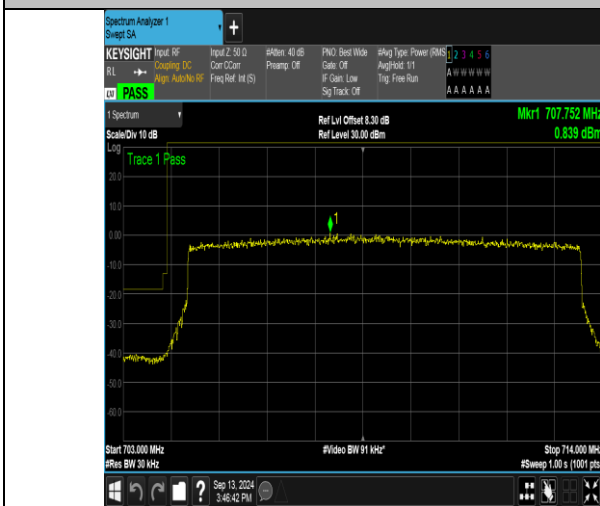
Band17_10MHz_QPSK_23780_50RB#0
