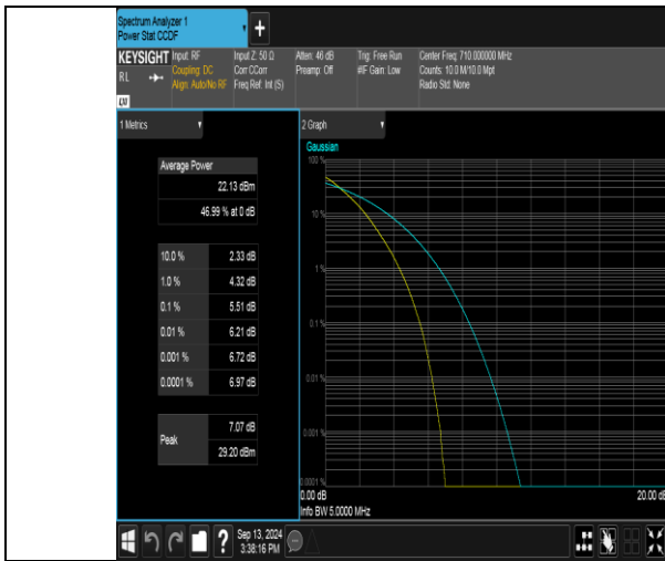
Band17-5MHz-QPSK-23790-25RB#0-PASS
