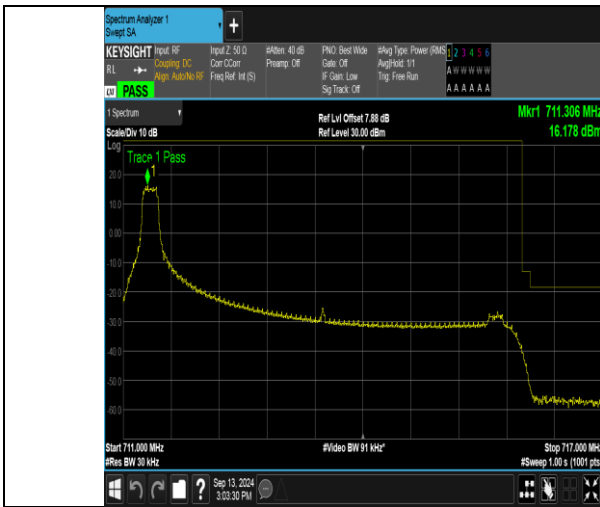
Band17_5MHz_QPSK_23825_1RB#0
