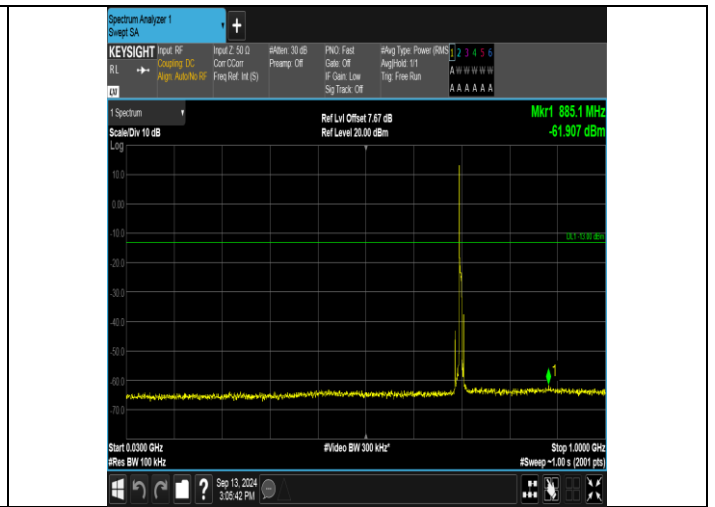
Band17_5MHz_16QAM_23755_1RB#0_30~1000_30~1000
