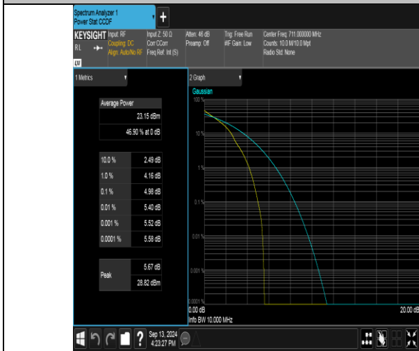
Band17-10MHz-QPSK-23800-1RB#0-PASS
