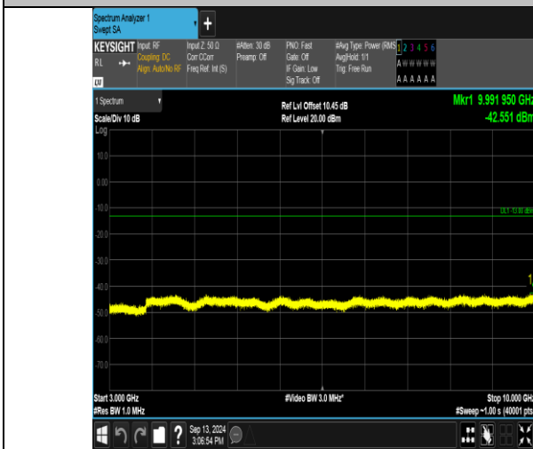
Band17_5MHz_QPSK_23755_1RB#24_3000~10000_3000~10000
