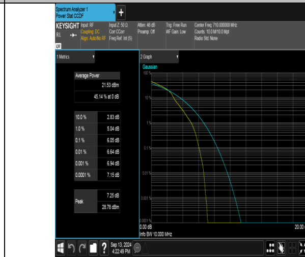
Band17-10MHz-16QAM-23790-1RB#0-PASS
