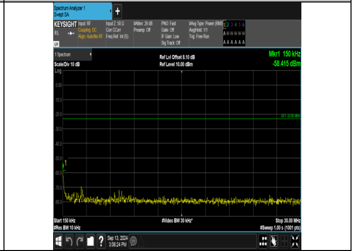
Band17_5MHz_QPSK_23755_1RB#24_0.15~30_0.15~30
