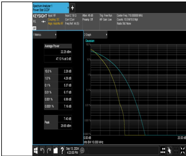
Band17-10MHz-QPSK-23790-50RB#0-PASS
