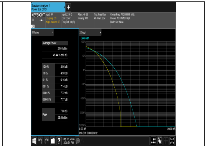
Band17-5MHz-16QAM-23790-25RB#0-PASS
