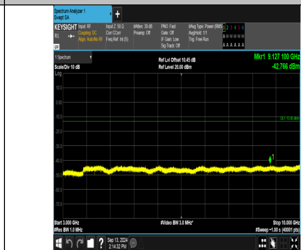
Band13_5MHz_16QAM_23230_1RB#24_3000~10000_3000~10000
