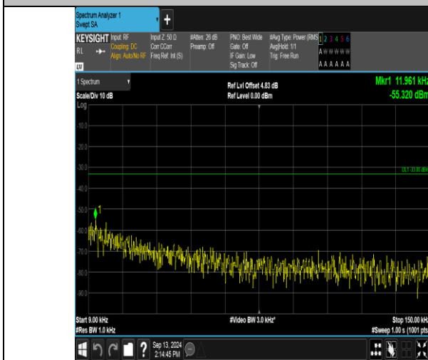
Band13_5MHz_QPSK_23230_25RB#0_0.009~0.15_0.009~0.15
