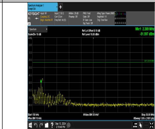
Band13_5MHz_QPSK_23255_25RB#0_0.15~30_0.15~30
