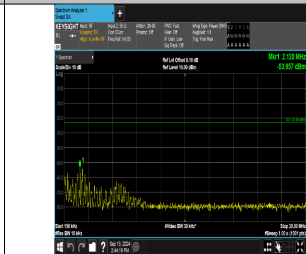
Band13_10MHz_QPSK_23230_1RB#0_0.15-30_0.15-30
