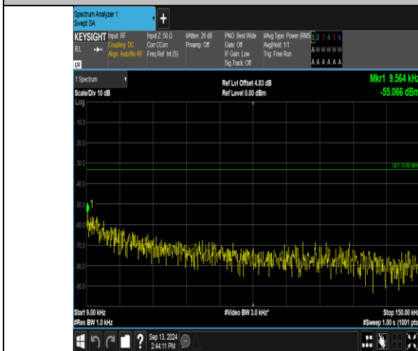
Band13_10MHz_QPSK_23230_1RB#0_0.009-0.15_0.009-0.15
