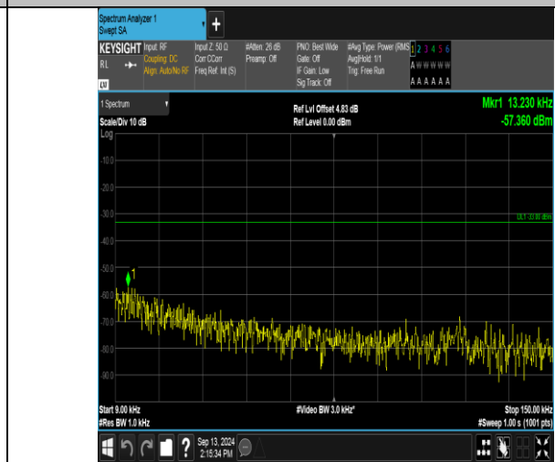
Band13_5MHz_16QAM_23230_25RB#0_0.009~0.15_0.009~0.15
