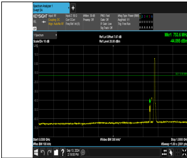
Band13_5MHz_QPSK_23255_25RB#0_30~1000_30~1000
