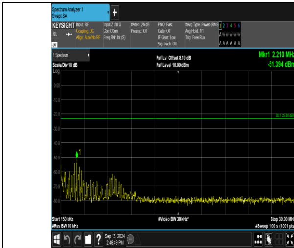
Band13_10MHz_16QAM_23230_1RB#49_0.15-30_0.15-30
