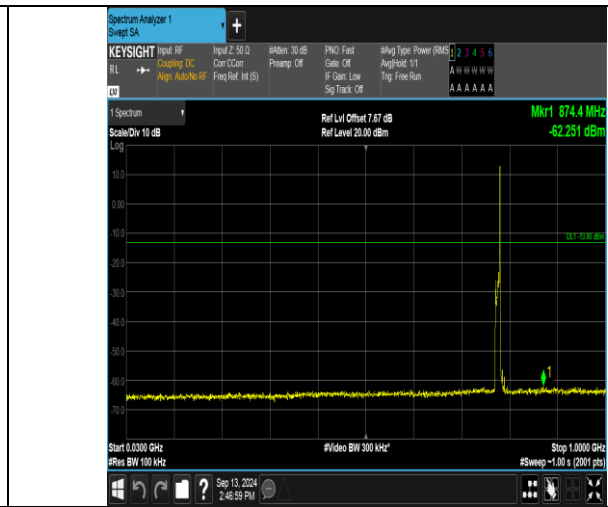
Band13_10MHz_16QAM_23230_1RB#49_30-1000_30-1000
