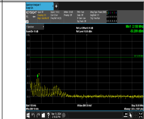
Band13_5MHz_QPSK_23255_1RB#0_0.15~30_0.15~30
