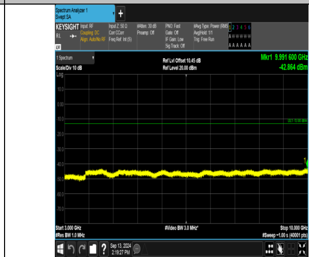
Band13_5MHz_16QAM_23255_1RB#24_3000~10000_3000~10000
