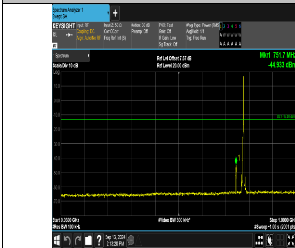
Band13_5MHz_QPSK_23230_1RB#24_30-1000_30-1000
