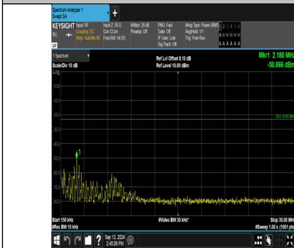
Band13_10MHz_16QAM_23230_1RB#0_0.15~30_0.15~30
