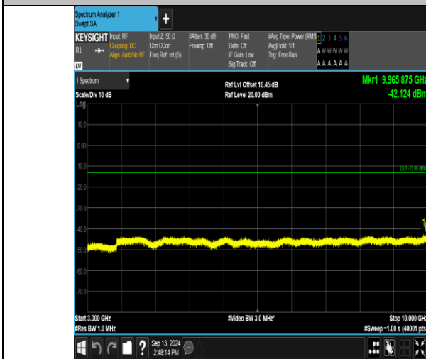
Band13_10MHz_QPSK_23230_50RB#0_3000~10000_3000~10000
