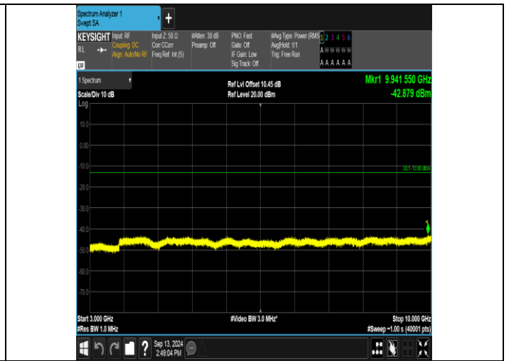
Band13_10MHz_16QAM_23230_50RB#0_3000~10000_3000~10000
