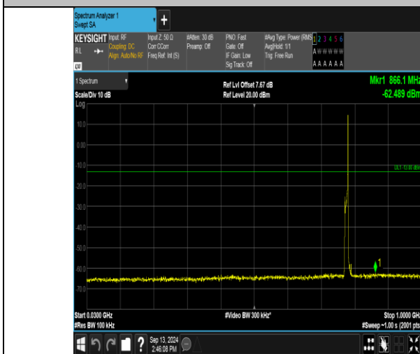
Band13_10MHz_QPSK_23230_1RB#49_30~1000_30~1000
