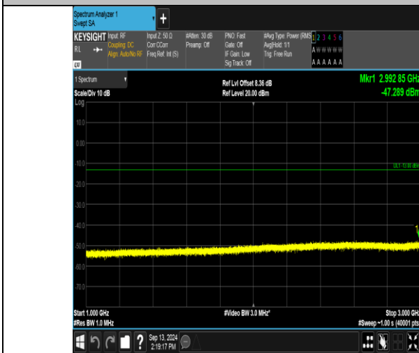
Band13_5MHz_16QAM_23255_1RB#24_1000~3000_1000~3000
