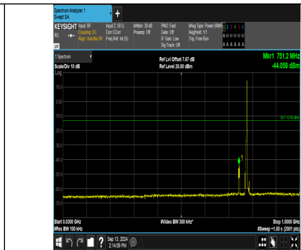
Band13_5MHz_16QAM_23230_1RB#24_30~1000_30~1000
