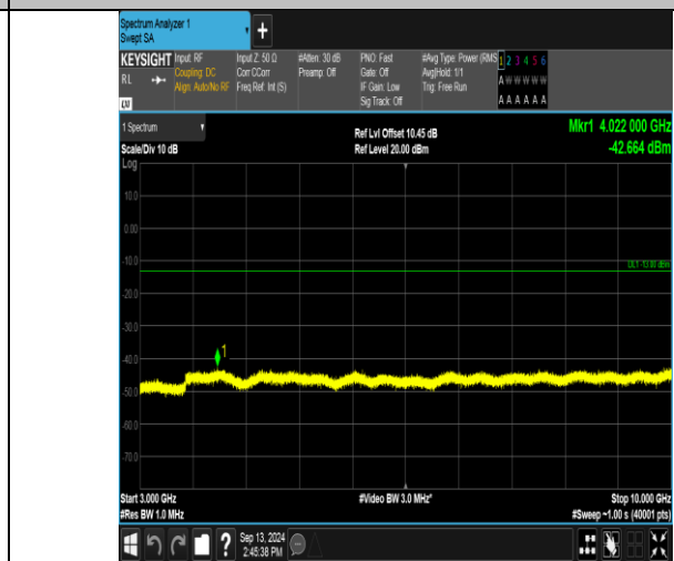
Band13_10MHz_16QAM_23230_1RB#0_3000~10000_3000~10000
