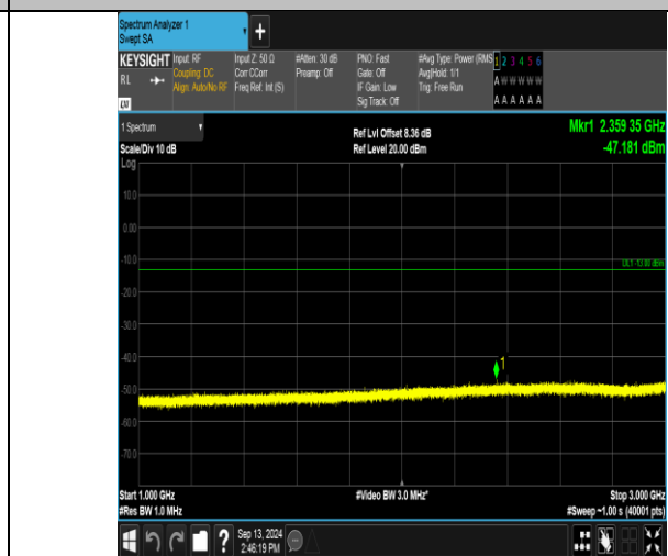
Band13_10MHz_QPSK_23230_1RB#49_1000~3000_1000~3000
