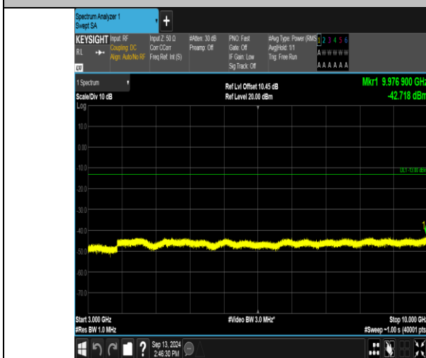
Band13_10MHz_QPSK_23230_1RB#49_3000~10000_3000~10000
