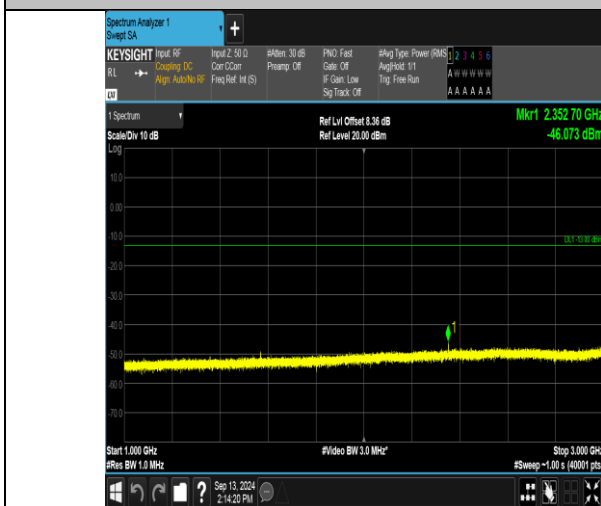
Band13_5MHz_16QAM_23230_1RB#24_1000~3000_1000~3000
