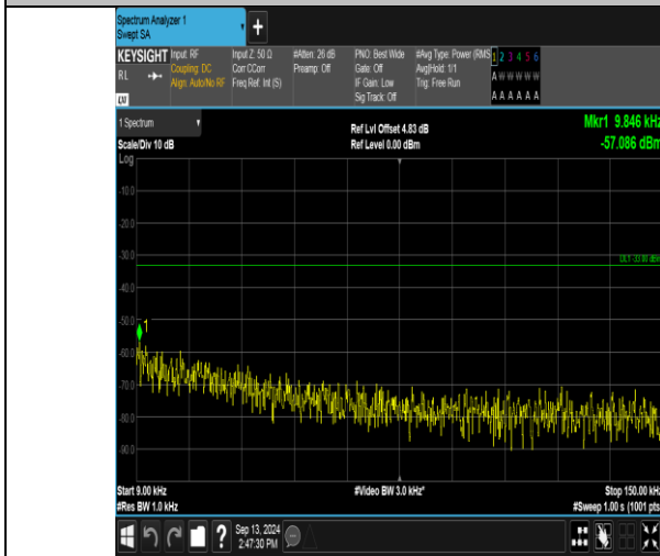
Band13_10MHz_QPSK_23230_50RB#0_0.009-0.15_0.009-0.15
