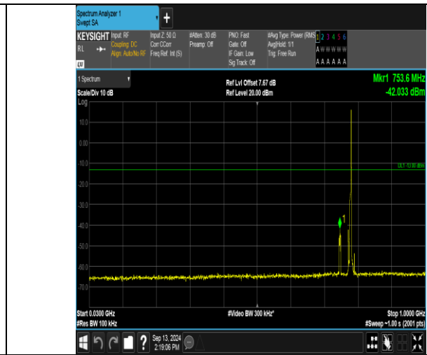
Band13_5MHz_16QAM_23255_1RB#24_30~1000_30~1000
