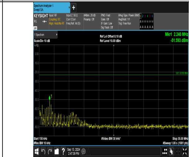
Band13_10MHz_QPSK_23230_50RB#0_0.15-30_0.15-30
