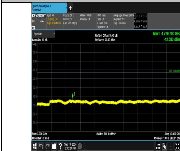
Band13_5MHz_QPSK_23230_25RB#0_3000~10000_3000~10000
