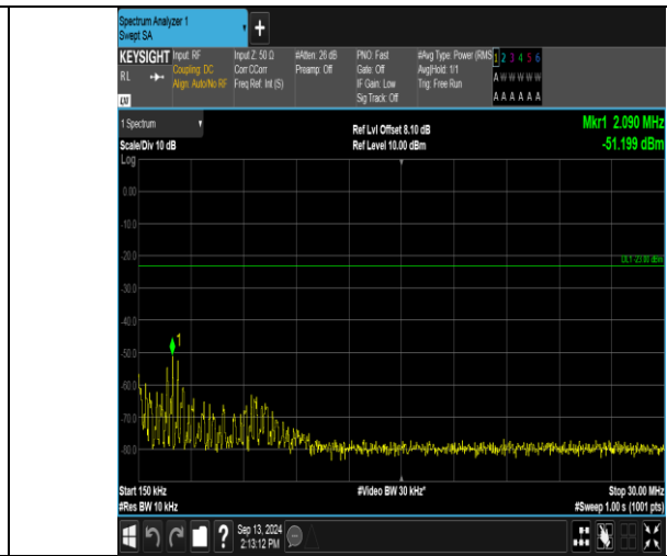
Band13_5MHz_QPSK_23230_1RB#24_0.15-30_0.15-30
