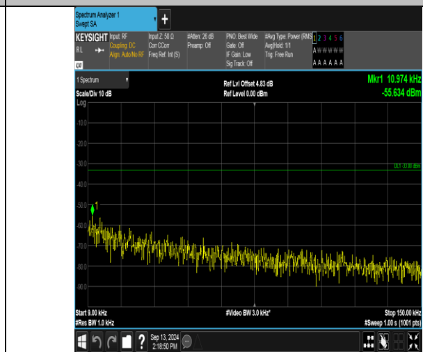
Band13_5MHz_16QAM_23255_1RB#24_0.009-0.15_0.009-0.15
