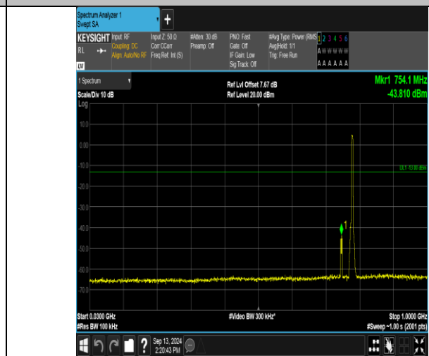
Band13_5MHz_16QAM_23255_25RB#0_30~1000_30~1000
