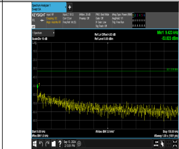
Band13_5MHz_16QAM_23230_1RB#24_0.009-0.15_0.009-0.15
