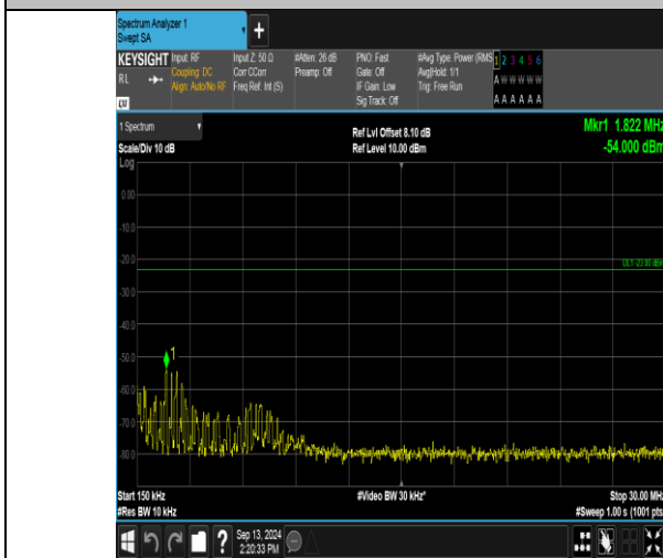
Band13_5MHz_16QAM_23255_25RB#0_0.15~30_0.15~30
