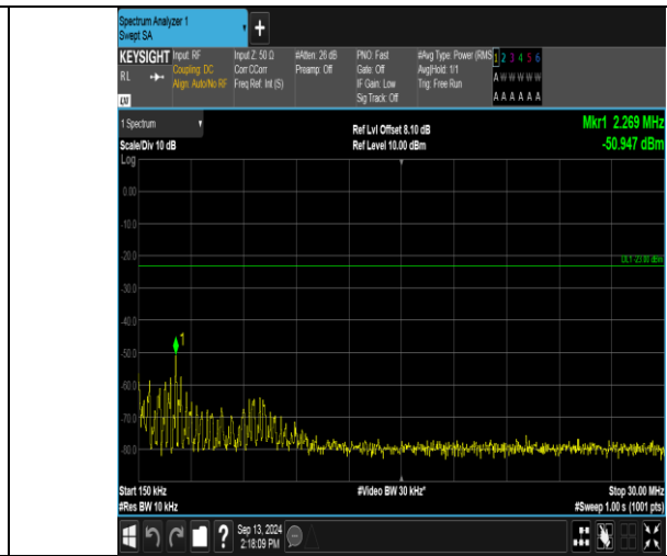
Band13_5MHz_QPSK_23255_1RB#24_0.15-30_0.15-30
