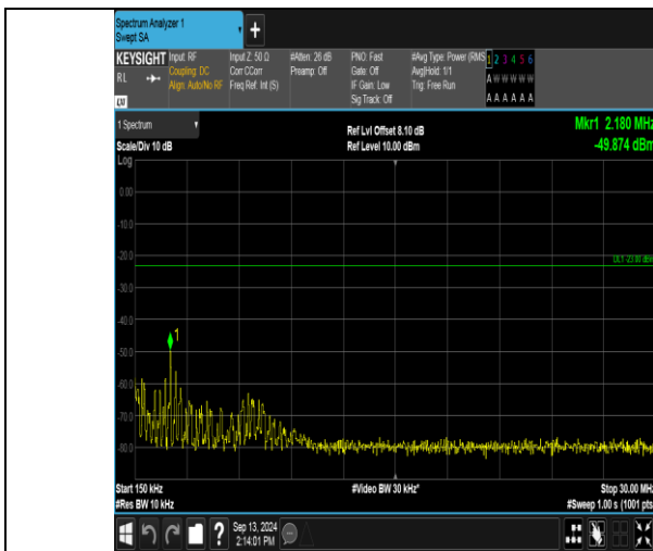
Band13_5MHz_16QAM_23230_1RB#24_0.15~30_0.15~30
