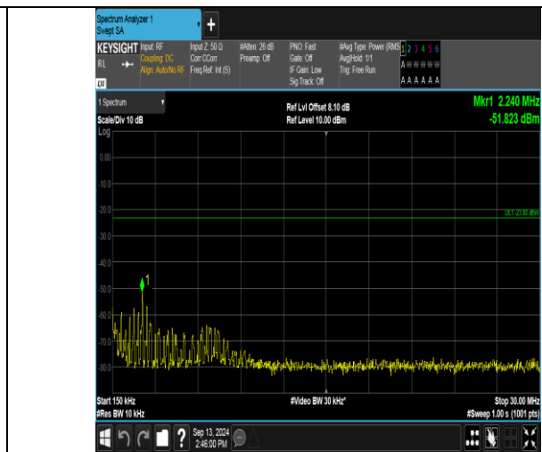
Band13_10MHz_QPSK_23230_1RB#49_0.15~30_0.15~30
