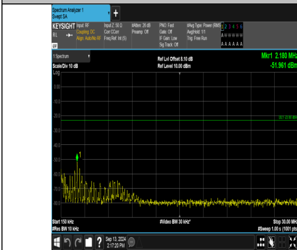
Band13_5MHz_16QAM_23255_1RB#0_0.15~30_0.15~30
