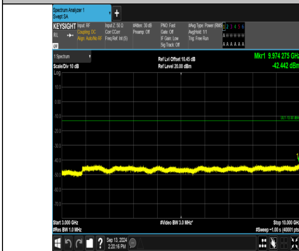
Band13_5MHz_QPSK_23255_25RB#0_3000~10000_3000~10000
