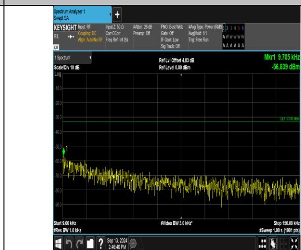
Band13_10MHz_16QAM_23230_1RB#49_0.009~0.15_0.009~0.15
