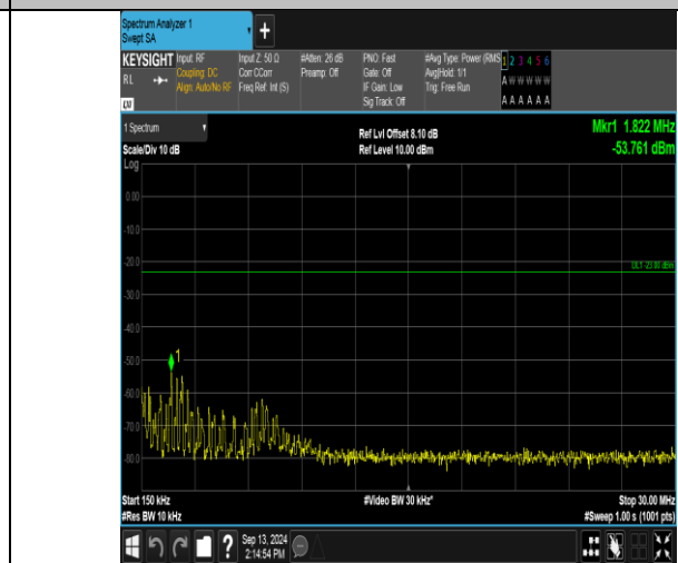
Band13_5MHz_QPSK_23230_25RB#0_0.15~30_0.15~30
