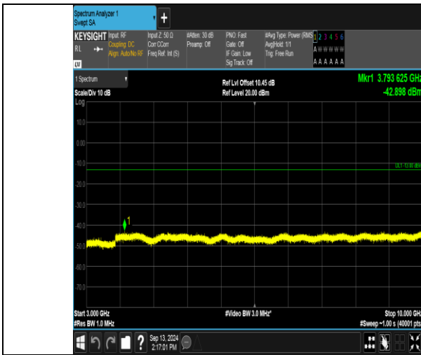
Band13_5MHz_QPSK_23255_1RB#0_3000~10000_3000~10000
