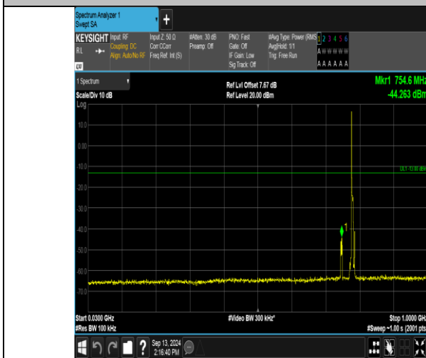
Band13_5MHz_QPSK_23255_1RB#0_30~1000_30~1000
