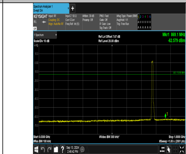
Band13_10MHz_16QAM_23230_50RB#0_30~1000_30~1000
