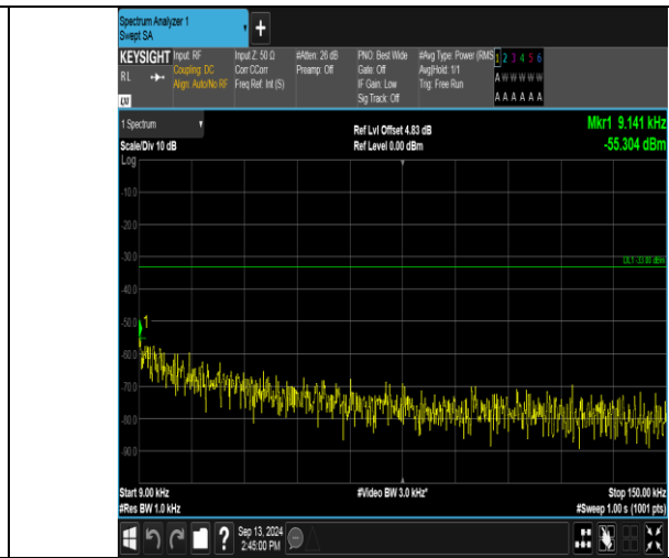
Band13_10MHz_16QAM_23230_1RB#0_0.009~0.15_0.009~0.15
