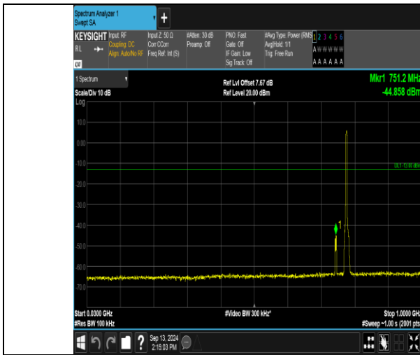
Band13_5MHz_QPSK_23230_25RB#0_30~1000_30~1000
