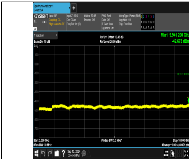
Band13_10MHz_QPSK_23230_1RB#0_3000~10000_3000~10000
