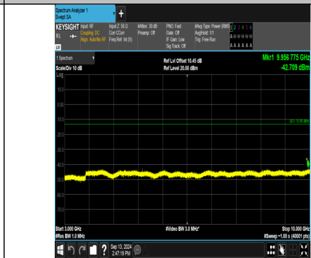
Band13_10MHz_16QAM_23230_1RB#49_3000-10000_3000-10000
