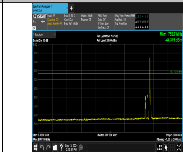
Band13_5MHz_16QAM_23230_25RB#0_30~1000_30~1000
