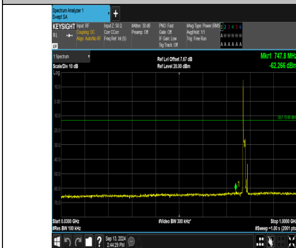
Band13_10MHz_QPSK_23230_1RB#0_30-1000_30-1000
