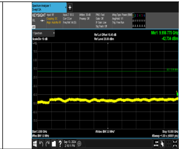
Band13_5MHz_16QAM_23230_25RB#0_3000~10000_3000~10000
