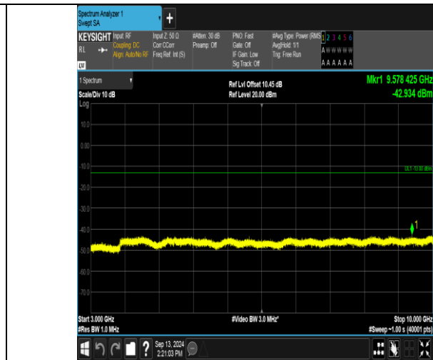
Band13_5MHz_16QAM_23255_25RB#0_3000-10000_3000-10000
