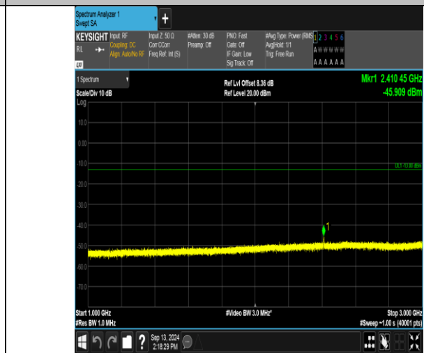
Band13_5MHz_QPSK_23255_1RB#24_1000-3000_1000-3000
