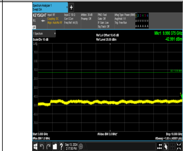
Band13_5MHz_16QAM_23255_1RB#0_3000~10000_3000~10000
