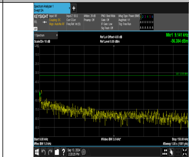
Band13_5MHz_16QAM_23255_25RB#0_0.009~0.15_0.009~0.15
