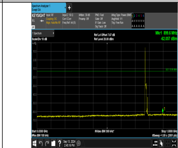
Band13_10MHz_16QAM_23230_1RB#0_30~1000_30~1000
