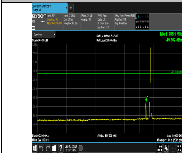
Band13_5MHz_QPSK_23255_1RB#24_30-1000_30-1000
