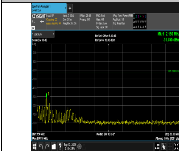
Band13_5MHz_16QAM_23230_25RB#0_0.15~30_0.15~30
