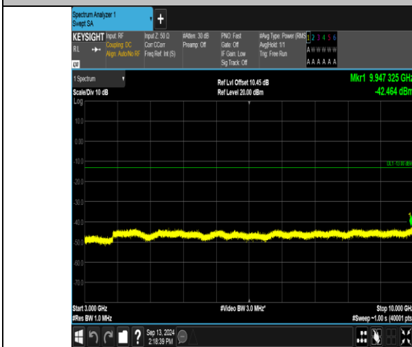
Band13_5MHz_QPSK_23255_1RB#24_3000-10000_3000-10000
