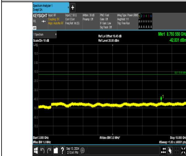
Band13_5MHz_QPSK_23230_1RB#24_3000-10000_3000-10000
