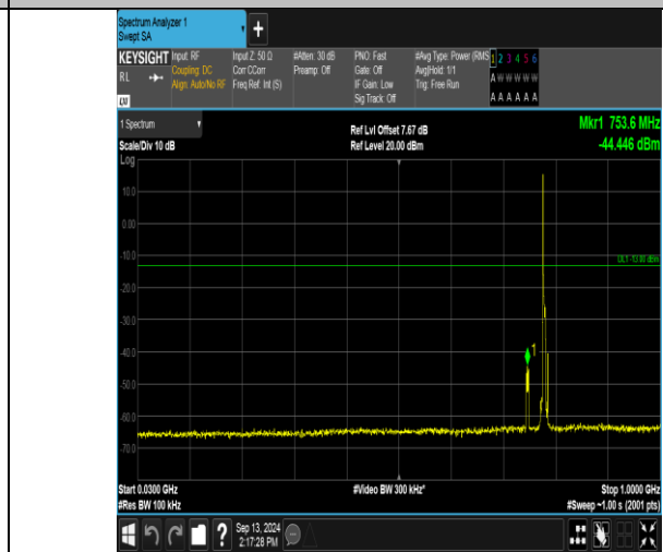
Band13_5MHz_16QAM_23255_1RB#0_30~1000_30~1000
