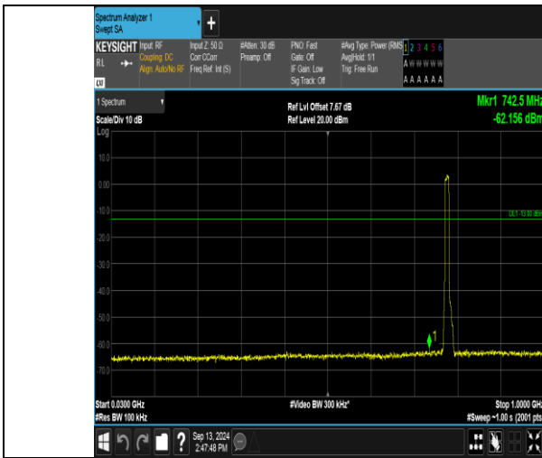
Band13_10MHz_QPSK_23230_50RB#0_30~1000_30~1000
