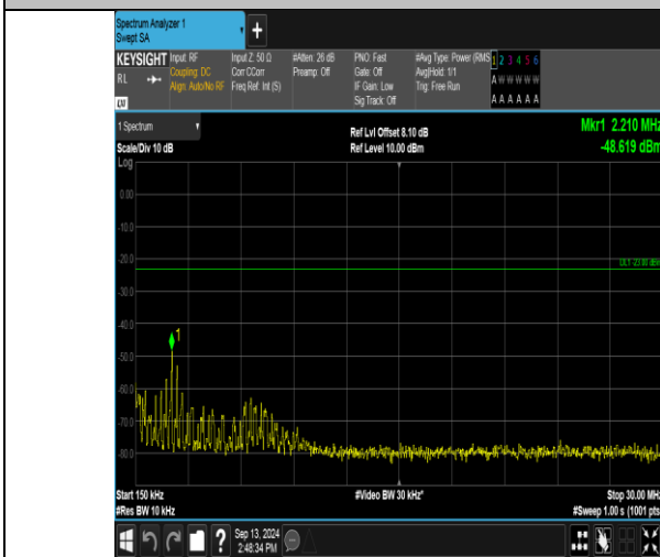
Band13_10MHz_16QAM_23230_50RB#0_0.15~30_0.15~30
