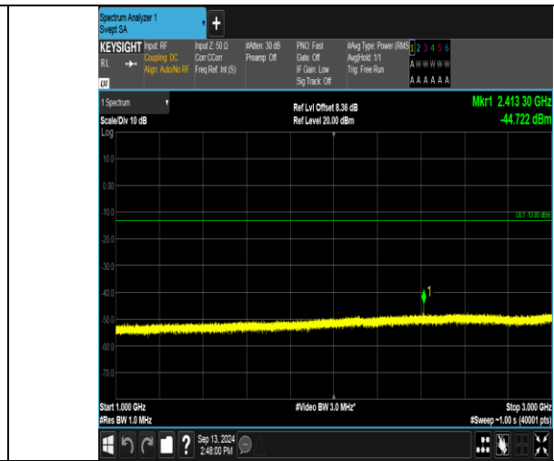
Band13_10MHz_QPSK_23230_50RB#0_1000~3000_1000~3000
