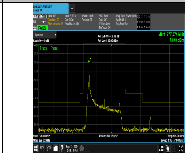
Band13_10MHz_16QAM_23230_1RB#0
