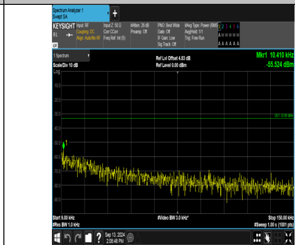
Band13_5MHz_16QAM_23205_1RB#24_0.009-0.15_0.009-0.15
