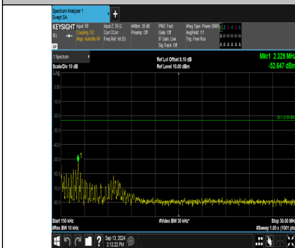
Band13_5MHz_16QAM_23230_1RB#0_0.15~30_0.15~30
