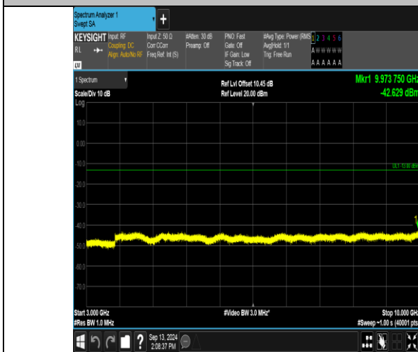
Band13_5MHz_QPSK_23205_1RB#24_3000-10000_3000-10000
