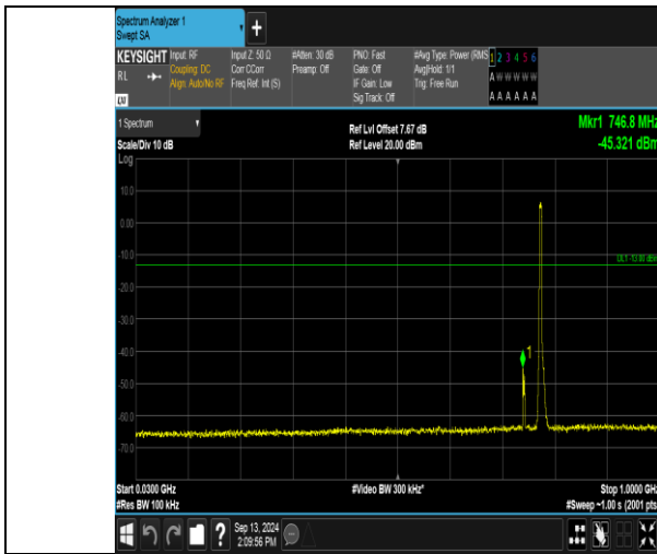
Band13_5MHz_QPSK_23205_25RB#0_30~1000_30~1000
