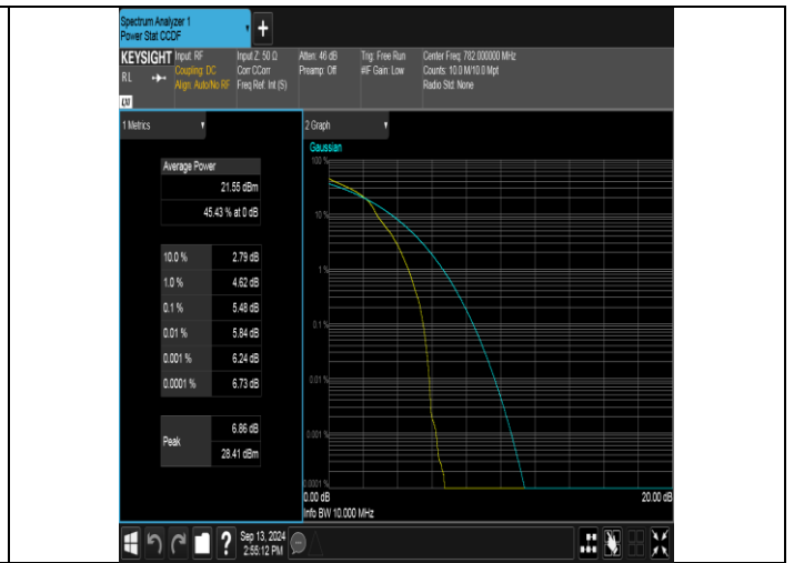
Band13-10MHz-16QAM-23230-1RB#0-PASS
