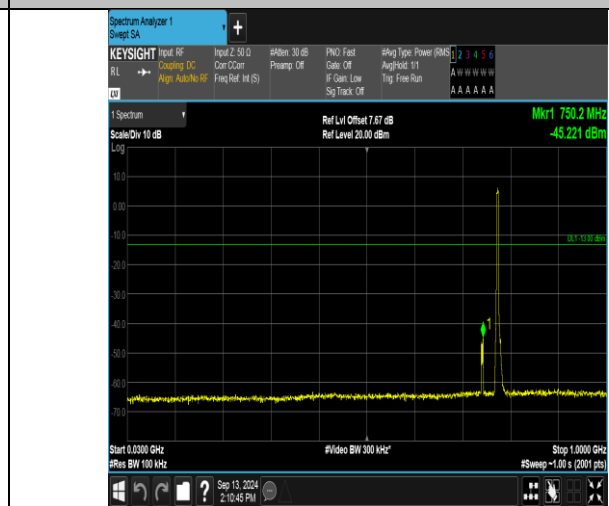
Band13_5MHz_16QAM_23205_25RB#0_30~1000_30~1000
