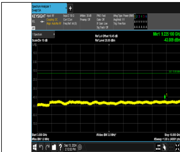
Band13_5MHz_QPSK_23230_1RB#0_3000~10000_3000~10000
