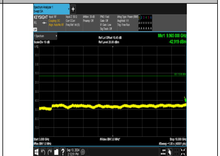
Band13_5MHz_16QAM_23230_1RB#0_3000~10000_3000~10000
