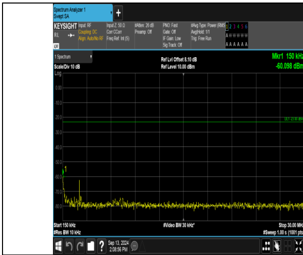
Band13_5MHz_16QAM_23205_1RB#24_0.15~30_0.15~30
