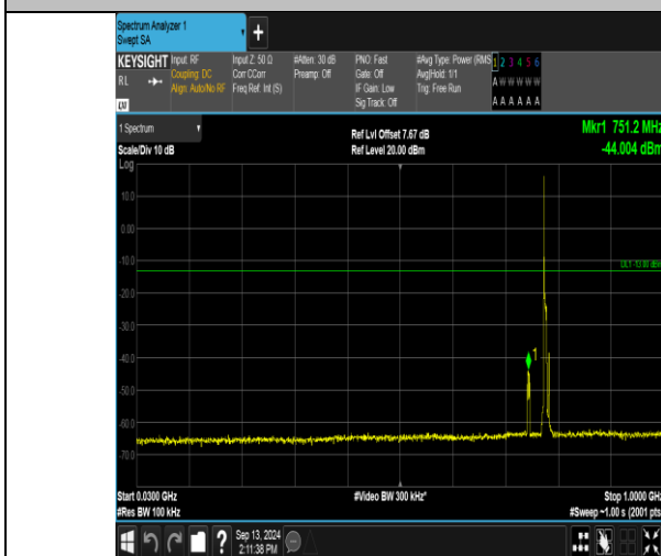
Band13_5MHz_QPSK_23230_1RB#0_30~1000_30~1000
