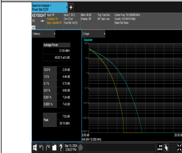
Band13-10MHz-QPSK-23230-50RB#0-PASS
