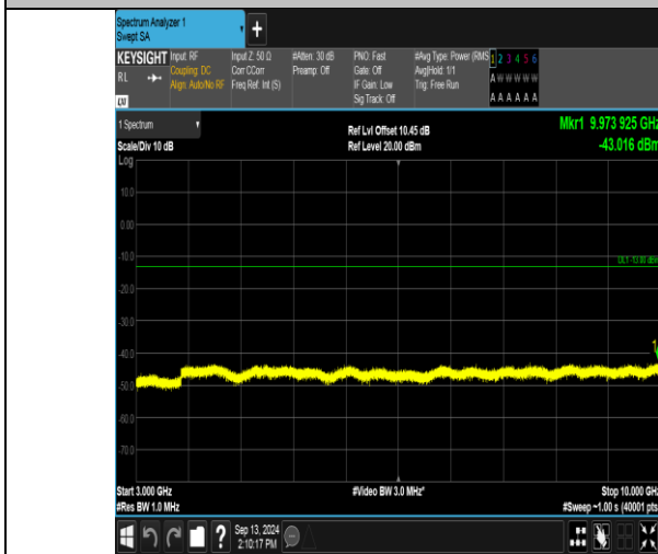
Band13_5MHz_QPSK_23205_25RB#0_3000~10000_3000~10000
