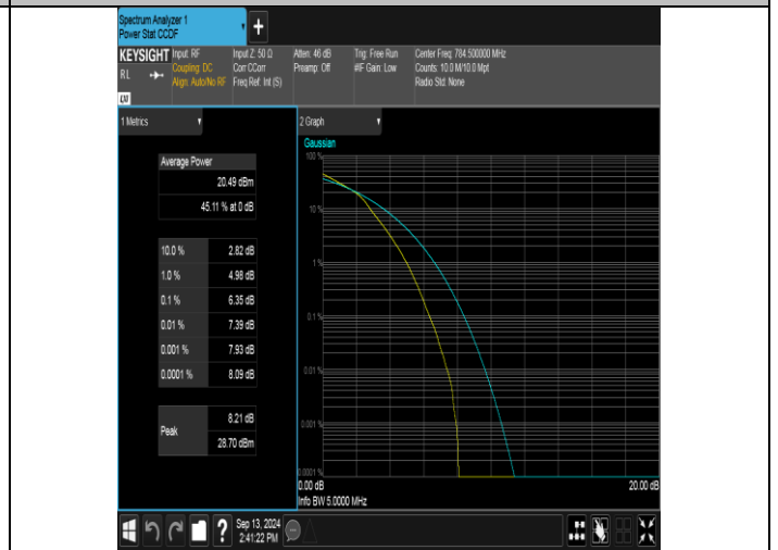
Band13-5MHz-16QAM-23255-25RB#0-PASS
