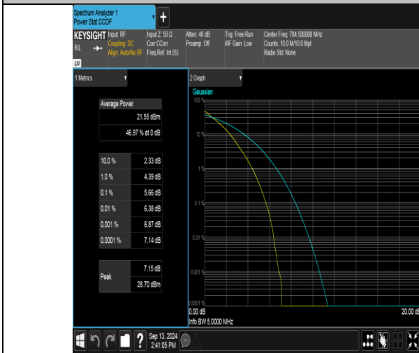
Band13-5MHz-QPSK-23255-25RB#0-PASS
