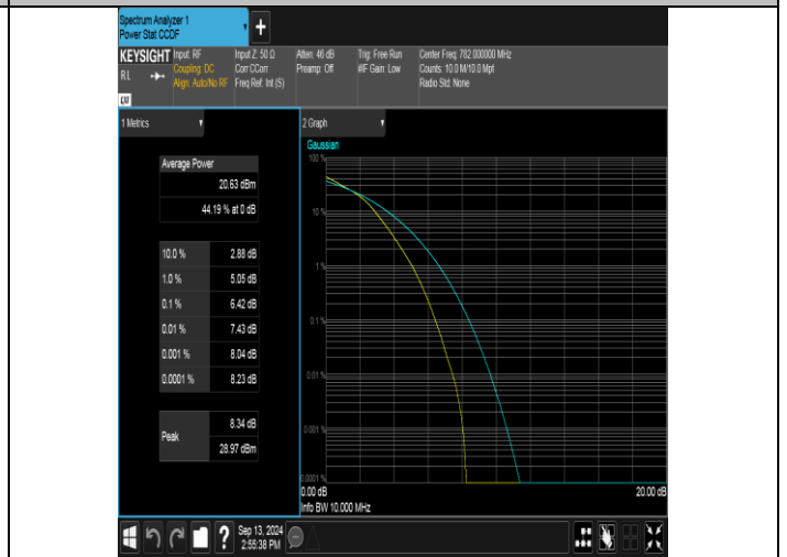
Band13-10MHz-16QAM-23230-50RB#0-PASS
