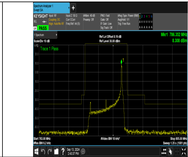
Band13_10MHz_16QAM_23230_1RB#49
