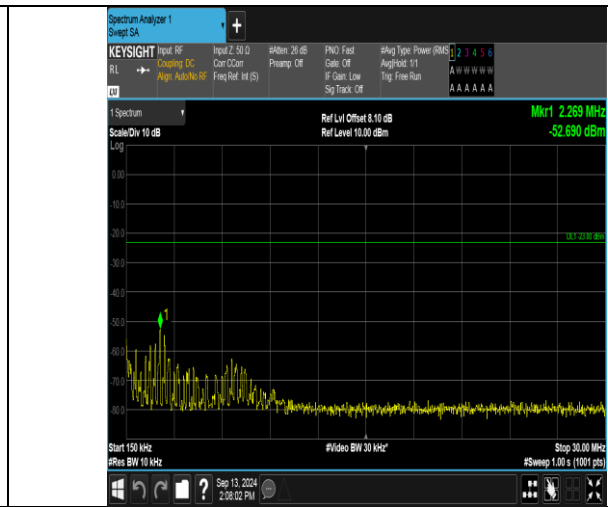
Band13_5MHz_QPSK_23205_1RB#24_0.15-30_0.15-30
