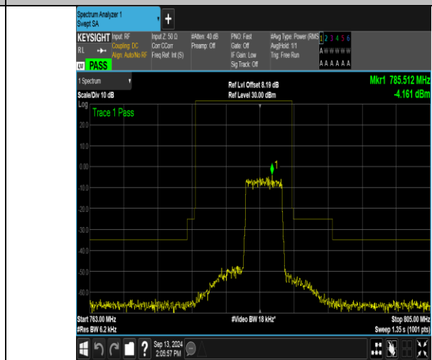
Band13_5MHz_16QAM_23255_25RB#0
