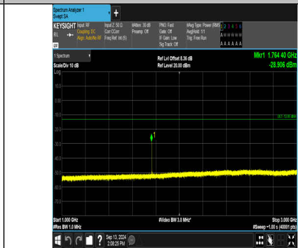
Band13_5MHz_QPSK_23205_1RB#24_1000-3000_1000-3000
