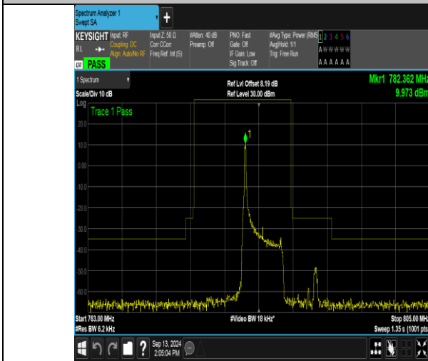
Band13_5MHz_QPSK_23255_1RB#0
