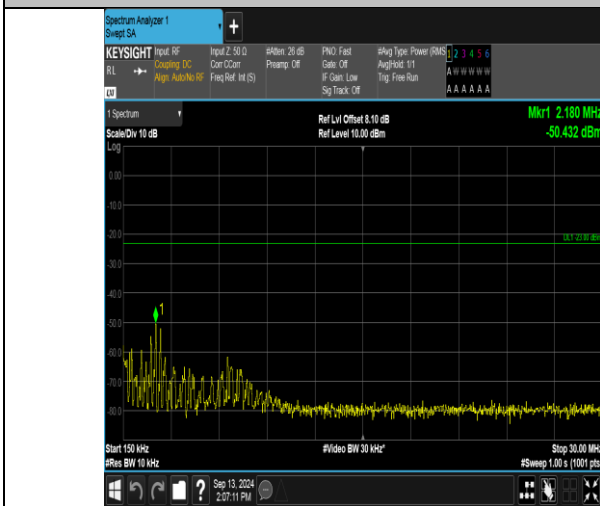
Band13_5MHz_16QAM_23205_1RB#0_0.15~30_0.15~30
