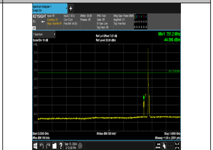
Band13_5MHz_16QAM_23230_1RB#0_30~1000_30~1000
