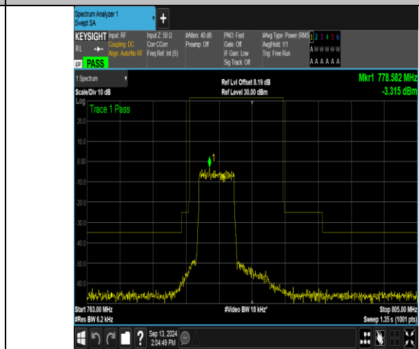
Band13_5MHz_16QAM_23205_25RB#0
