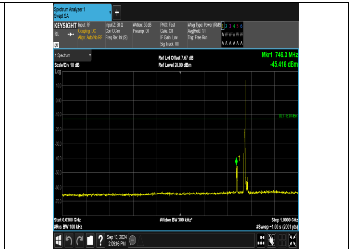
Band13_5MHz_16QAM_23205_1RB#24_30~1000_30~1000
