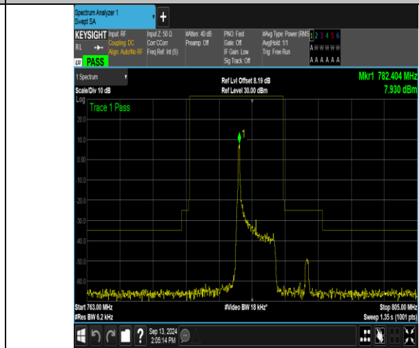
Band13_5MHz_16QAM_23255_1RB#0
