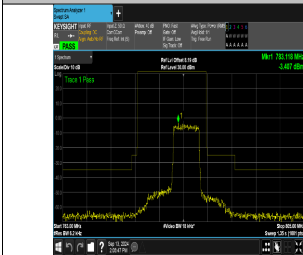
Band13_5MHz_QPSK_23255_25RB#0
