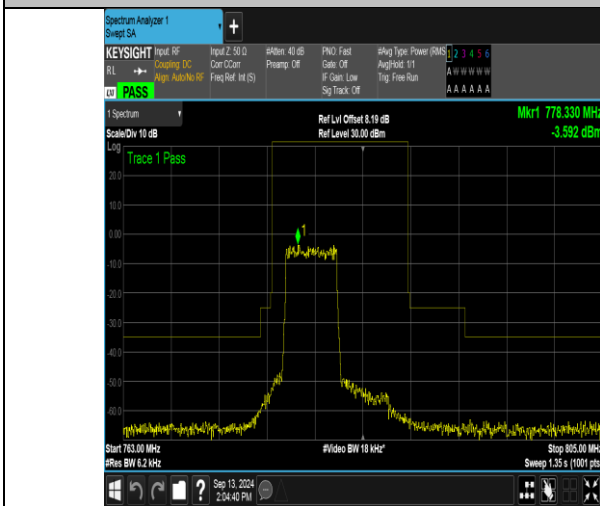
Band13_5MHz_QPSK_23205_25RB#0
