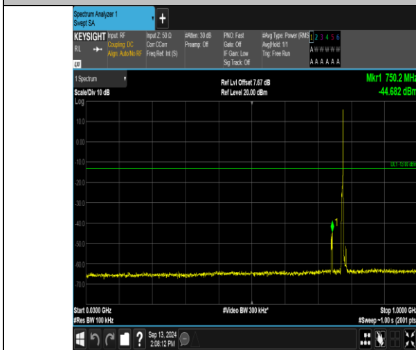
Band13_5MHz_QPSK_23205_1RB#24_30-1000_30-1000
