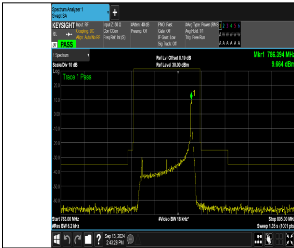
Band13_10MHz_QPSK_23230_1RB#49
