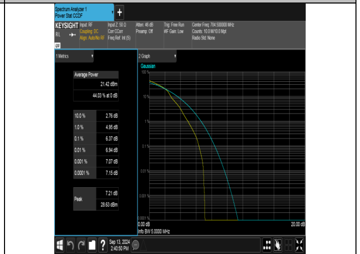
Band13-5MHz-16QAM-23255-1RB#0-PASS
