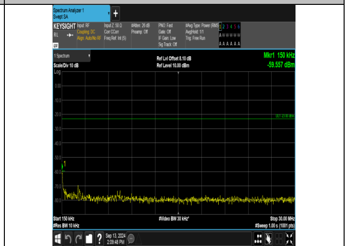
Band13_5MHz_QPSK_23205_25RB#0_0.15~30_0.15~30
