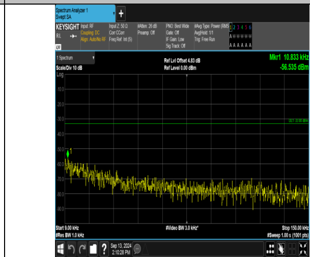
Band13_5MHz_16QAM_23205_25RB#0_0.009~0.15_0.009~0.15
