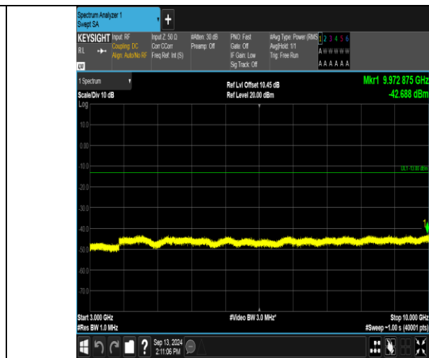
Band13_5MHz_16QAM_23205_25RB#0_3000~10000_3000~10000
