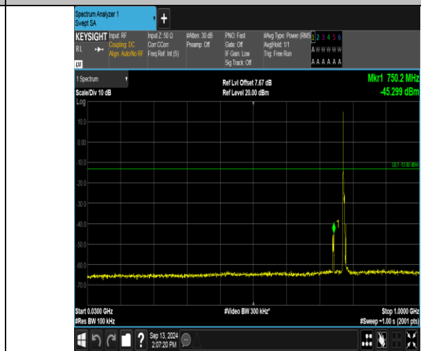
Band13_5MHz_16QAM_23205_1RB#0_30~1000_30~1000
