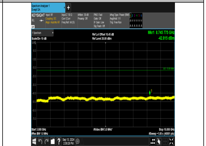
Band13_5MHz_16QAM_23205_1RB#24_3000~10000_3000~10000
