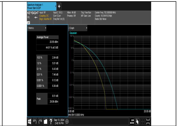
Band13-5MHz-16QAM-23230-25RB#0-PASS
