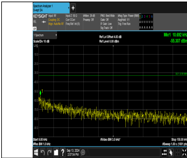
Band13_5MHz_QPSK_23205_1RB#24_0.009-0.15_0.009-0.15
