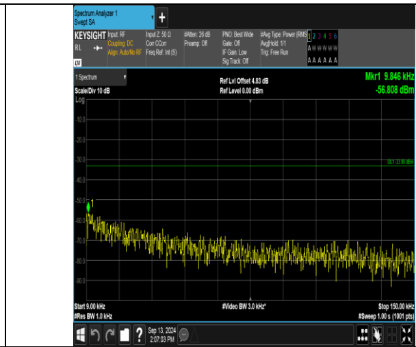
Band13_5MHz_16QAM_23205_1RB#0_0.009~0.15_0.009~0.15
