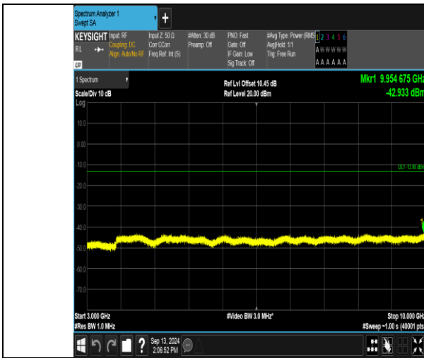
Band13_5MHz_QPSK_23205_1RB#0_3000~10000_3000~10000
