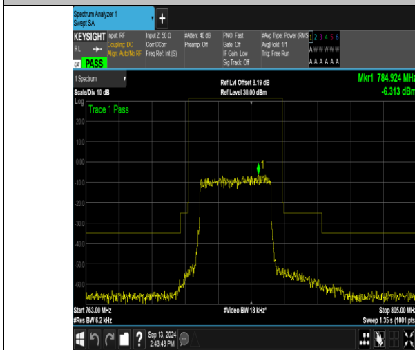
Band13_10MHz_QPSK_23230_50RB#0
