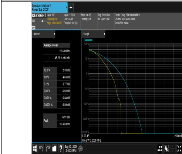
Band13-5MHz-QPSK-23255-1RB#0-PASS
