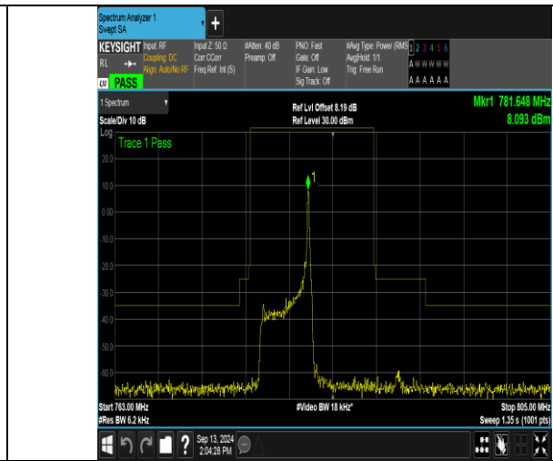
Band13_5MHz_16QAM_23205_1RB#24
