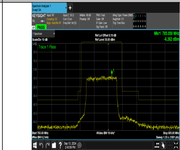
Band13_10MHz_16QAM_23230_50RB#0
