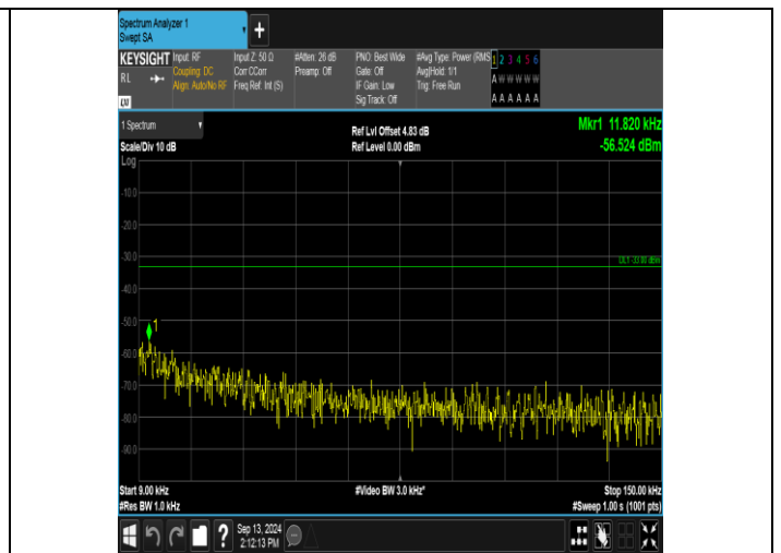
Band13_5MHz_16QAM_23230_1RB#0_0.009~0.15_0.009~0.15
