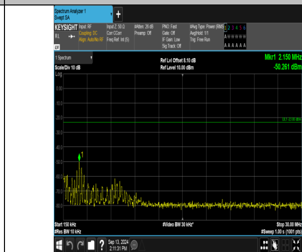
Band13_5MHz_QPSK_23230_1RB#0_0.15~30_0.15~30
