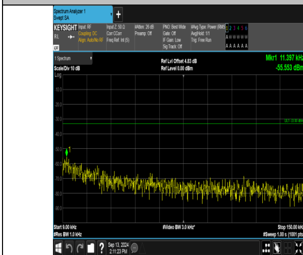
Band13_5MHz_QPSK_23230_1RB#0_0.009~0.15_0.009~0.15
