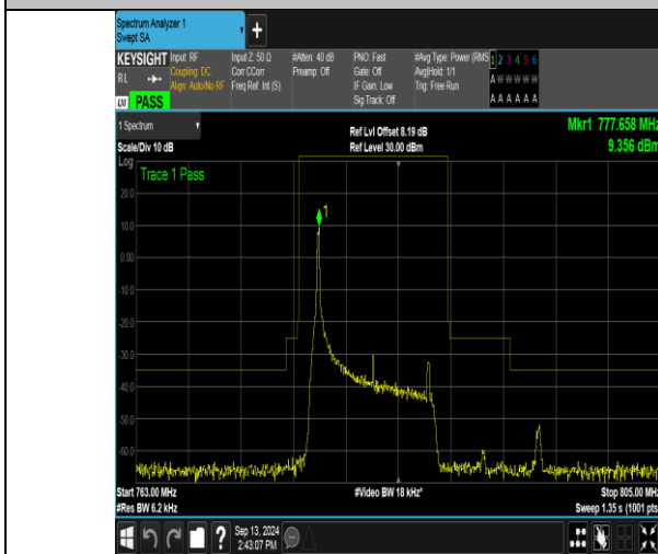
Band13_10MHz_QPSK_23230_1RB#0
