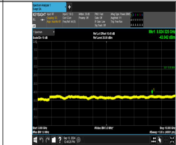
Band12_5MHz_16QAM_23035_25RB#0_3000~10000_3000~10000
