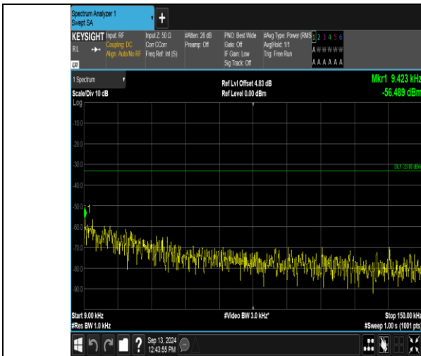
Band12_5MHz_QPSK_23035_25RB#0_0.009-0.15_0.009-0.15
