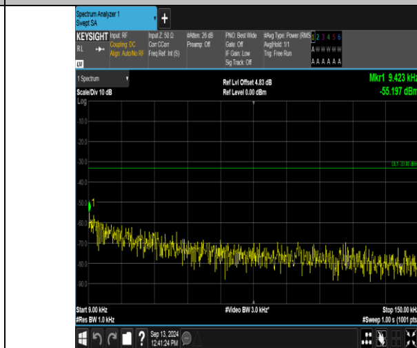
Band12_5MHz_16QAM_23035_1RB#0_0.009~0.15_0.009~0.15
