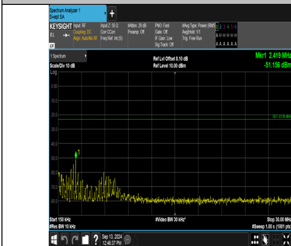
Band12_5MHz_16QAM_23095_1RB#0_0.15~30_0.15~30
