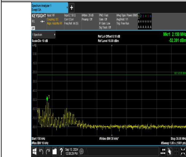
Band12_3MHz_16QAM_23165_1RB#0_0.15~30_0.15~30
