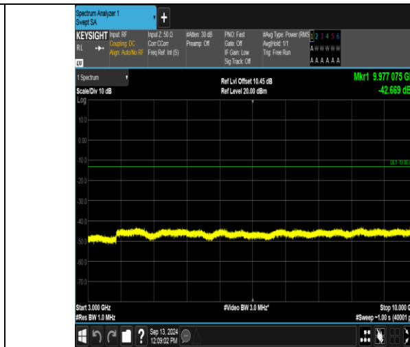
Band12_3MHz_16QAM_23165_1RB#0_3000~10000_3000~10000
