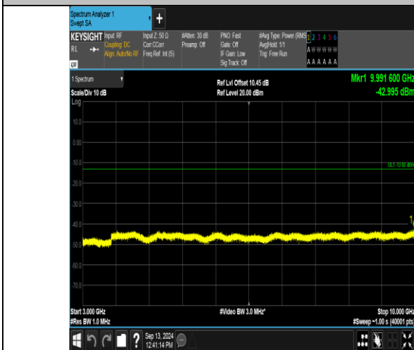
Band12_5MHz_QPSK_23035_1RB#0_3000~10000_3000~10000
