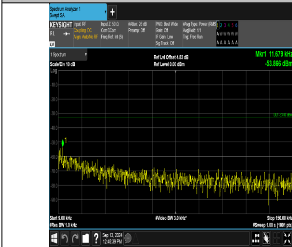
Band12_5MHz_QPSK_23095_1RB#0_0.009~0.15_0.009~0.15
