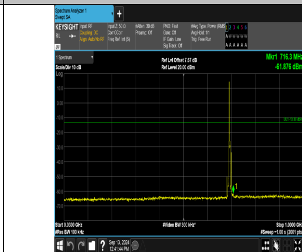
Band12_5MHz_16QAM_23035_1RB#0_30~1000_30~1000
