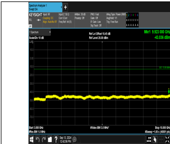
Band12_5MHz_QPSK_23035_1RB#24_3000~10000_3000~10000
