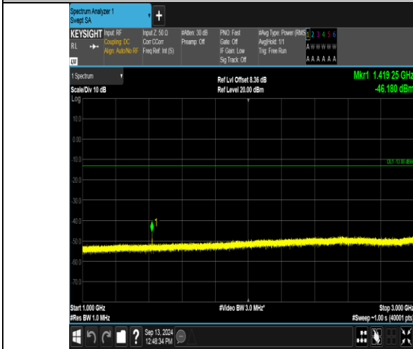
Band12_5MHz_16QAM_23095_1RB#24_1000~3000_1000~3000
