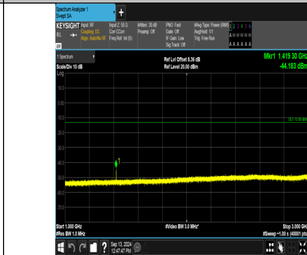
Band12_5MHz_QPSK_23095_1RB#24_1000~3000_1000~3000
