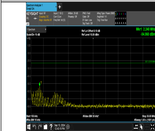
Band12_5MHz_16QAM_23035_1RB#24_0.15~30_0.15~30
