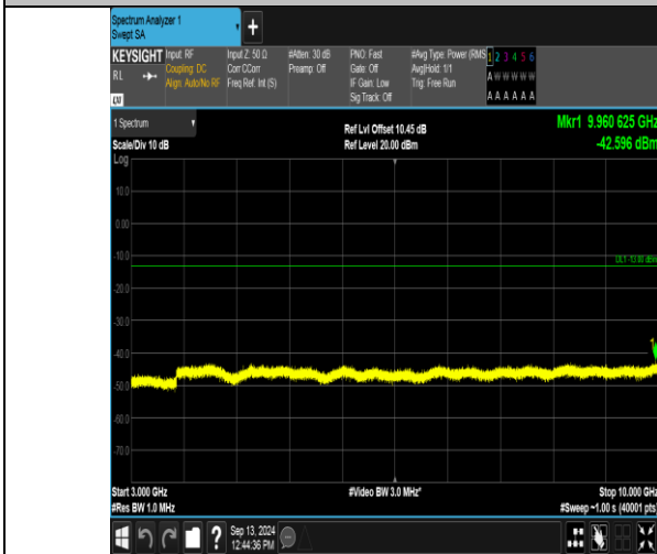
Band12_5MHz_QPSK_23035_25RB#0_3000-10000_3000-10000
