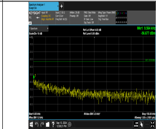
Band12_3MHz_16QAM_23165_1RB#0_0.009~0.15_0.009~0.15
