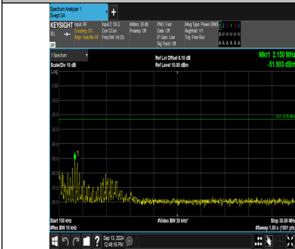
Band12_5MHz_16QAM_23095_1RB#24_0.15~30_0.15~30
