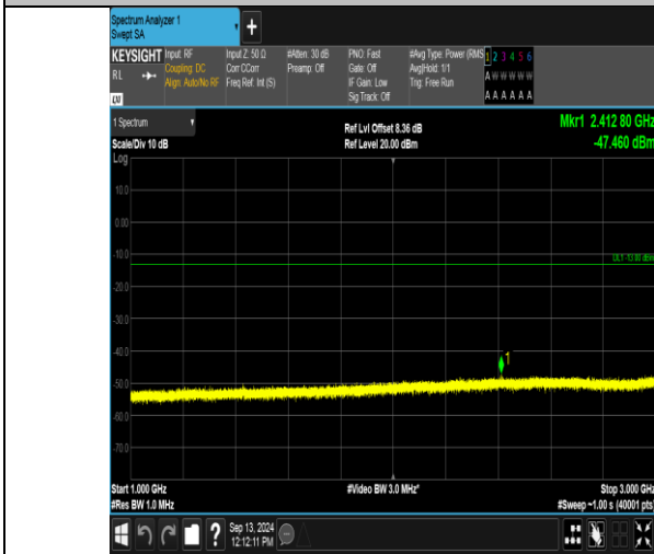
Band12_3MHz_16QAM_23165_15RB#0_1000~3000_1000~3000
