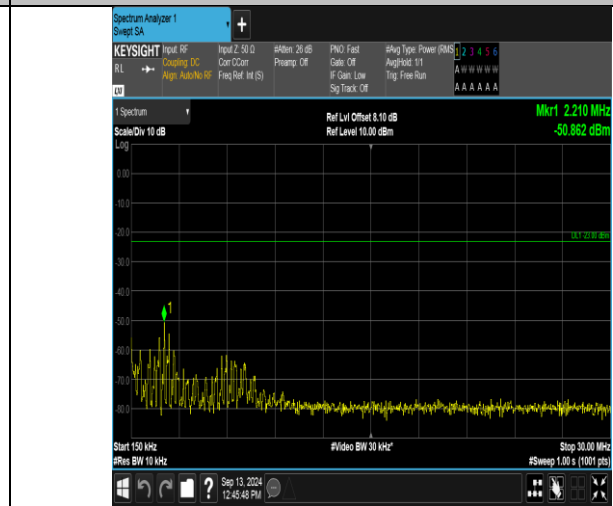
Band12_5MHz_QPSK_23095_1RB#0_0.15~30_0.15~30
