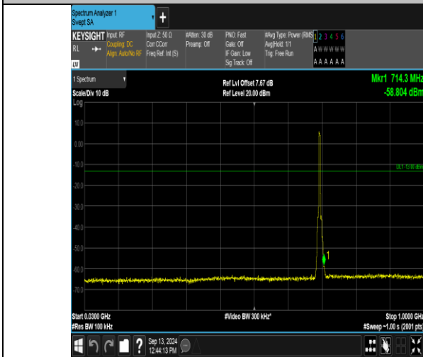
Band12_5MHz_QPSK_23035_25RB#0_30-1000_30-1000
