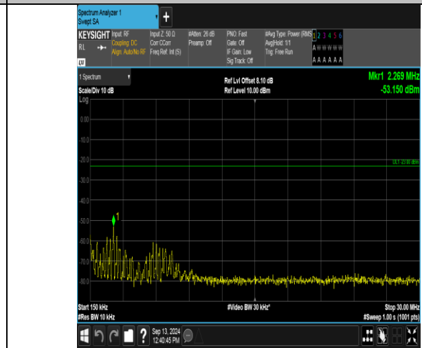
Band12_5MHz_QPSK_23035_1RB#0_0.15~30_0.15~30
