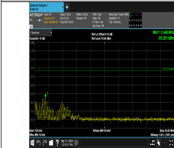
Band12_3MHz_16QAM_23165_1RB#14_0.15~30_0.15~30
