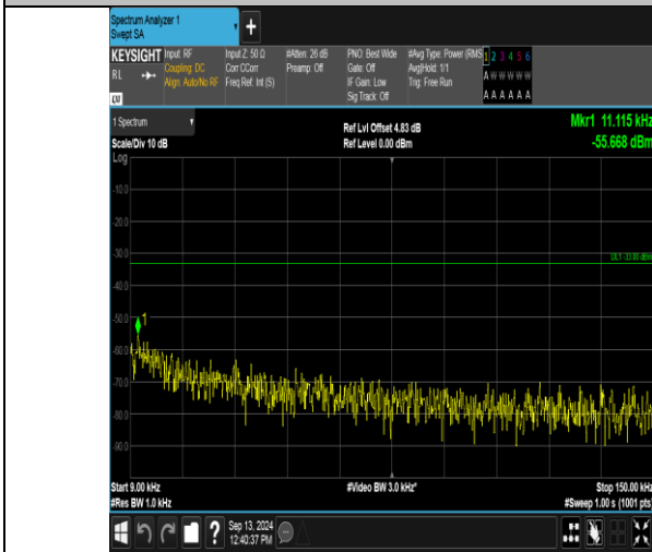
Band12_5MHz_QPSK_23035_1RB#0_0.009~0.15_0.009~0.15
