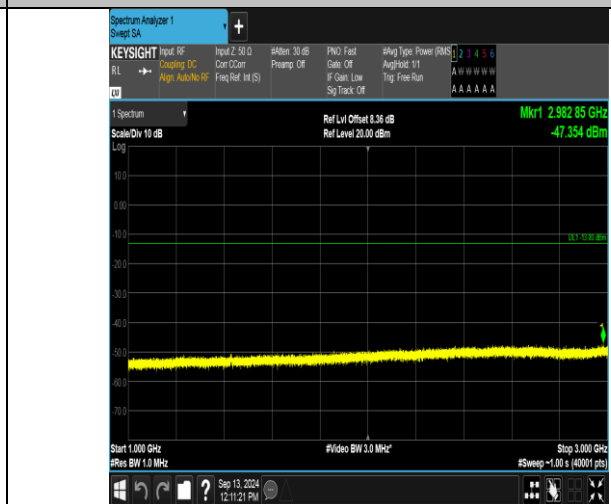
Band12_3MHz_QPSK_23165_15RB#0_1000-3000_1000-3000
