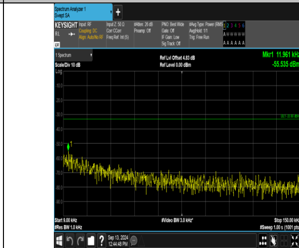
Band12_5MHz_16QAM_23035_25RB#0_0.009-0.15_0.009-0.15
