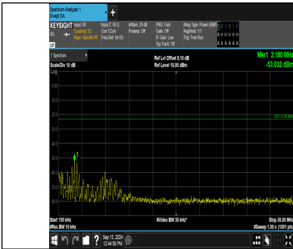
Band12_5MHz_16QAM_23035_25RB#0_0.15~30_0.15~30
