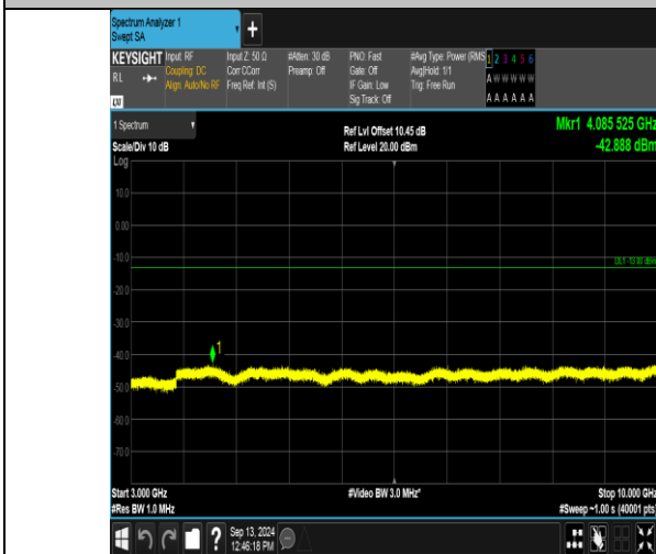
Band12_5MHz_QPSK_23095_1RB#0_3000~10000_3000~10000
