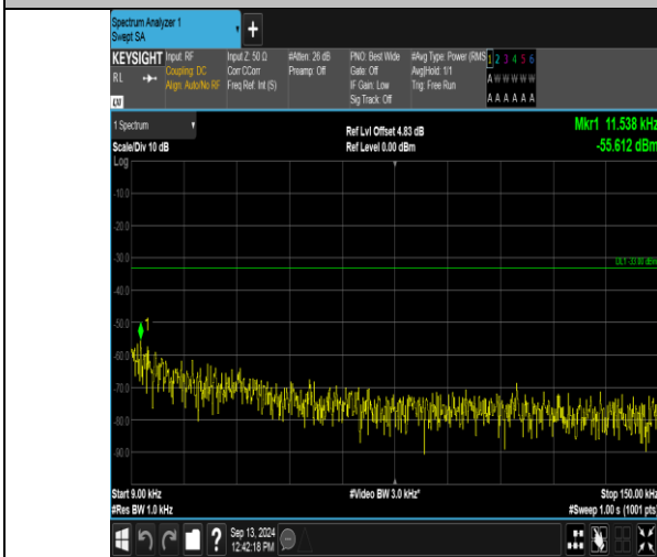
Band12_5MHz_QPSK_23035_1RB#24_0.009~0.15_0.009~0.15
