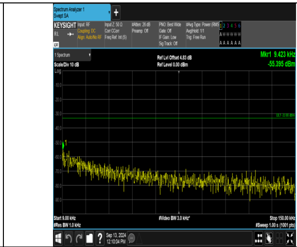
Band12_3MHz_16QAM_23165_1RB#14_0.009~0.15_0.009~0.15
