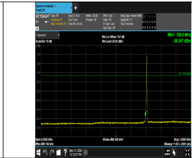
Band12_3MHz_16QAM_23165_15RB#0_30~1000_30~1000
