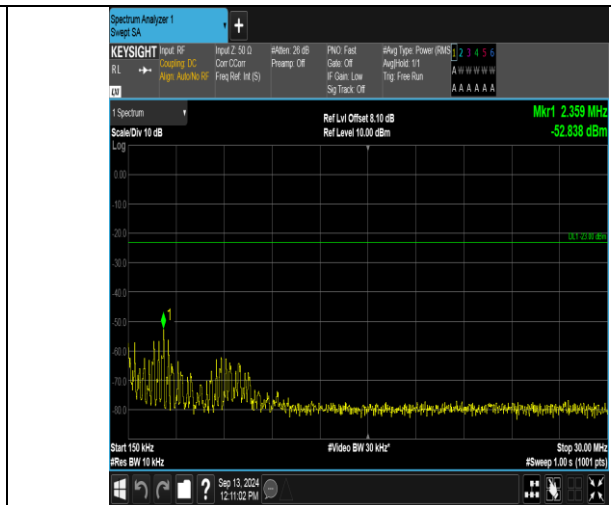
Band12_3MHz_QPSK_23165_15RB#0_0.15-30_0.15-30
