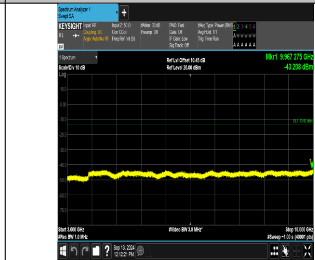
Band12_3MHz_16QAM_23165_15RB#0_3000~10000_3000~10000
