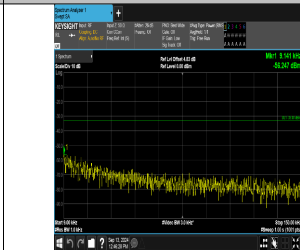
Band12_5MHz_16QAM_23095_1RB#0_0.009~0.15_0.009~0.15
