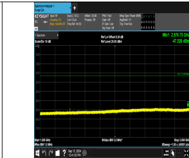
Band12_5MHz_QPSK_23035_1RB#0_1000~3000_1000~3000
