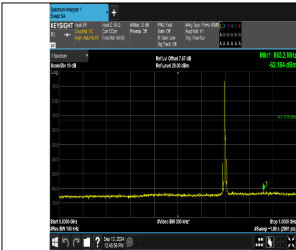
Band12_5MHz_QPSK_23095_1RB#0_30~1000_30~1000
