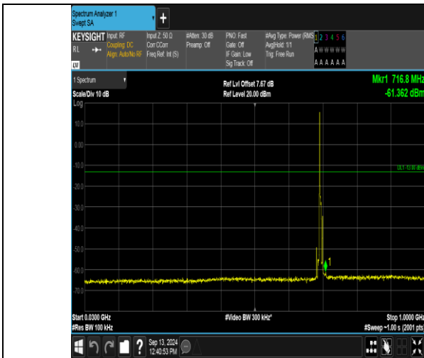
Band12_5MHz_QPSK_23035_1RB#0_30~1000_30~1000
