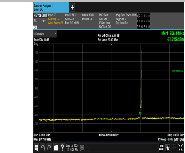
Band12_3MHz_16QAM_23165_1RB#14_30~1000_30~1000
