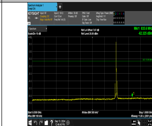
Band12_5MHz_16QAM_23095_1RB#0_30~1000_30~1000
