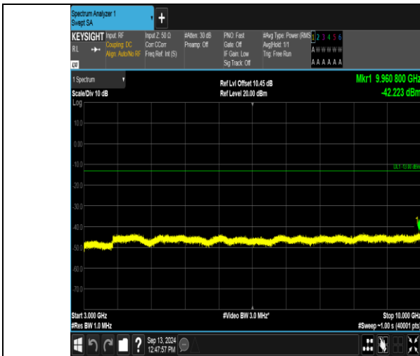
Band12_5MHz_QPSK_23095_1RB#24_3000~10000_3000~10000
