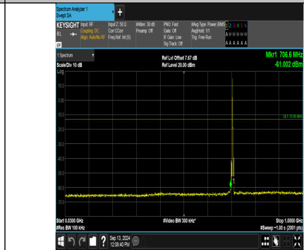
Band12_3MHz_16QAM_23165_1RB#0_30~1000_30~1000
