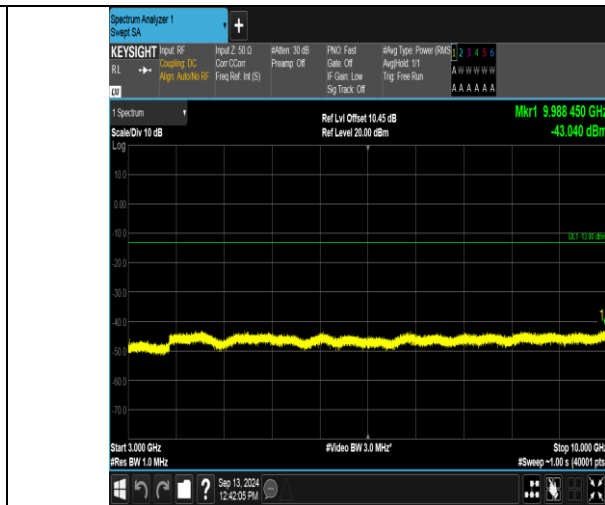
Band12_5MHz_16QAM_23035_1RB#0_3000~10000_3000~10000
