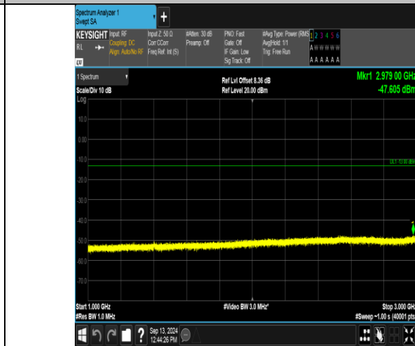
Band12_5MHz_QPSK_23035_25RB#0_1000-3000_1000-3000
