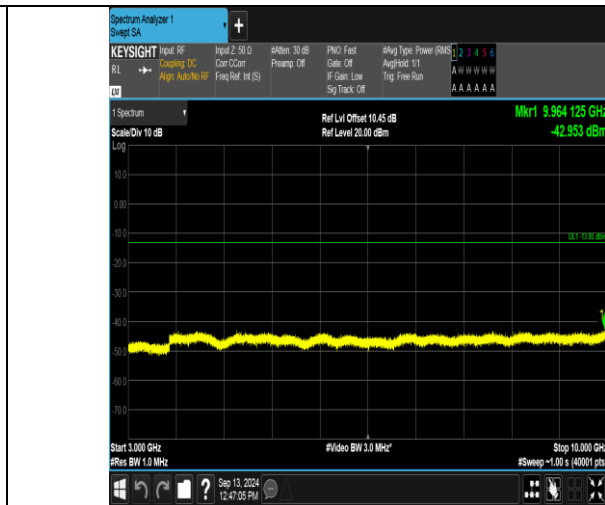
Band12_5MHz_16QAM_23095_1RB#0_3000~10000_3000~10000
