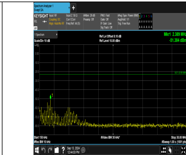
Band12_5MHz_QPSK_23035_25RB#0_0.15-30_0.15-30
