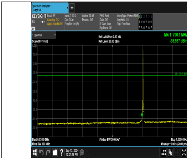
Band12_3MHz_QPSK_23165_1RB#0_30~1000_30~1000
