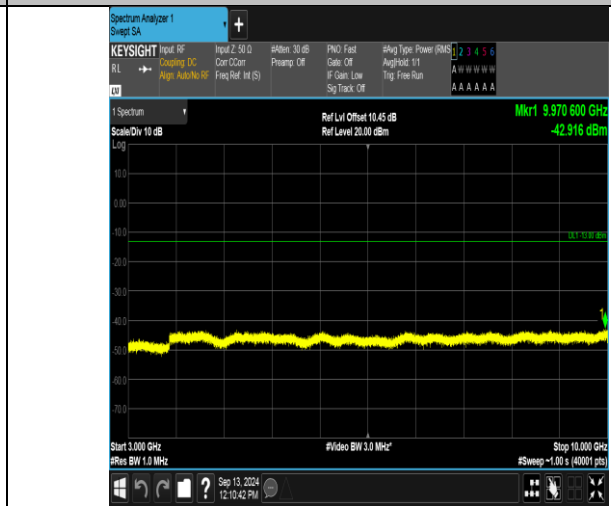
Band12_3MHz_16QAM_23165_1RB#14_3000~10000_3000~10000
