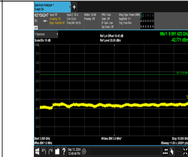
Band12_5MHz_16QAM_23095_1RB#24_3000~10000_3000~10000
