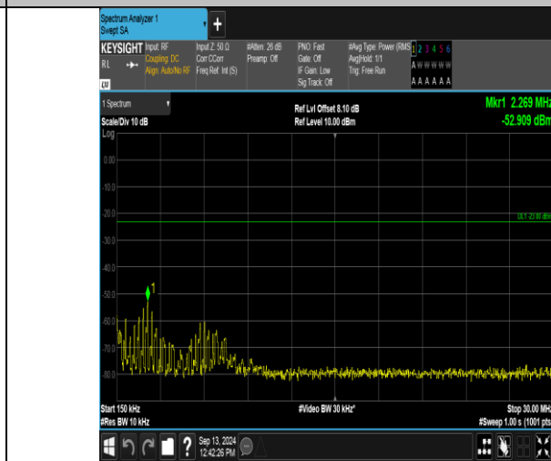
Band12_5MHz_QPSK_23035_1RB#24_0.15~30_0.15~30
