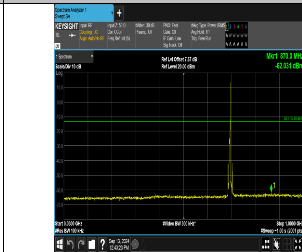
Band12_5MHz_16QAM_23035_1RB#24_30~1000_30~1000
