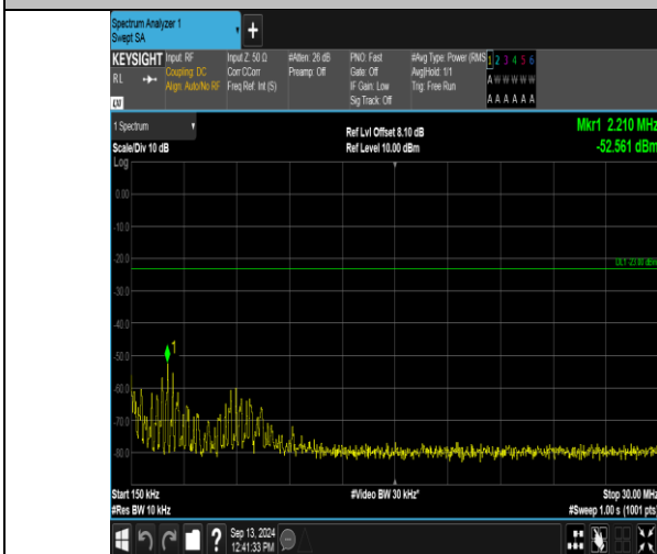
Band12_5MHz_16QAM_23035_1RB#0_0.15~30_0.15~30
