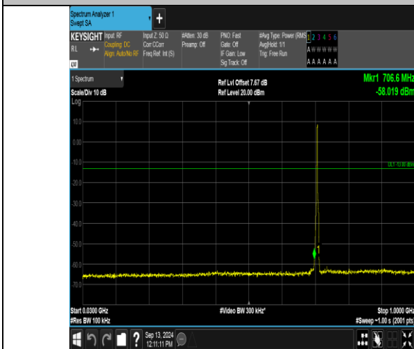
Band12_3MHz_QPSK_23165_15RB#0_30-1000_30-1000
