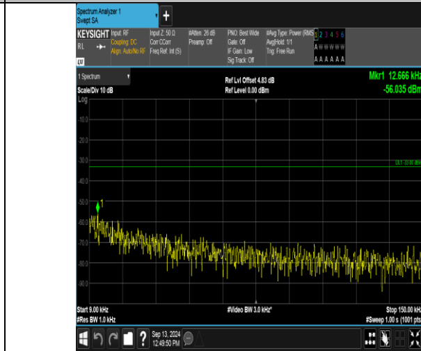
Band12_5MHz_16QAM_23095_25RB#0_0.009-0.15_0.009-0.15
