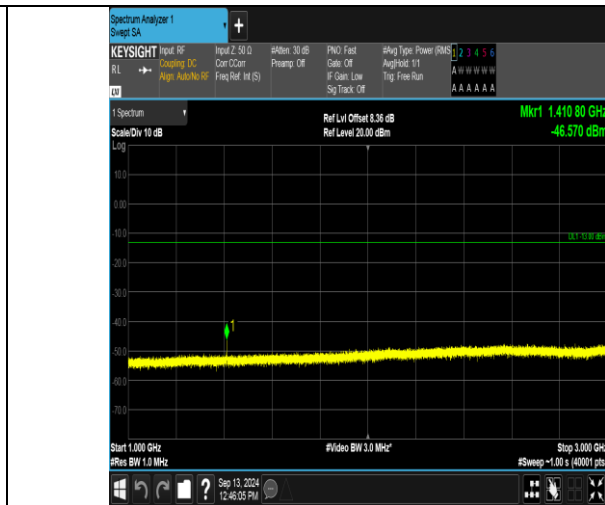
Band12_5MHz_QPSK_23095_1RB#0_1000~3000_1000~3000
