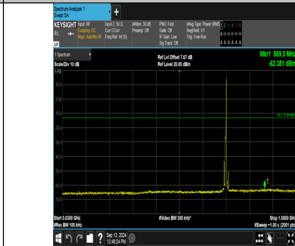
Band12_5MHz_16QAM_23095_1RB#24_30~1000_30~1000
