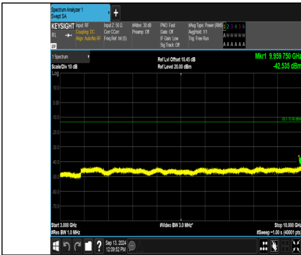
Band12_3MHz_QPSK_23165_1RB#14_3000~10000_3000~10000
