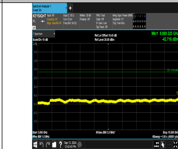
Band12_5MHz_16QAM_23035_1RB#24_3000~10000_3000~10000
