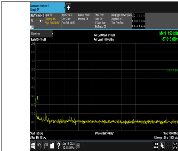
Band12_3MHz_16QAM_23165_15RB#0_0.15~30_0.15~30
