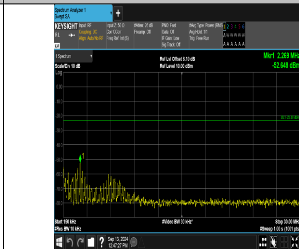
Band12_5MHz_QPSK_23095_1RB#24_0.15~30_0.15~30
