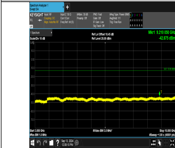
Band12_3MHz_QPSK_23165_1RB#0_3000~10000_3000~10000
