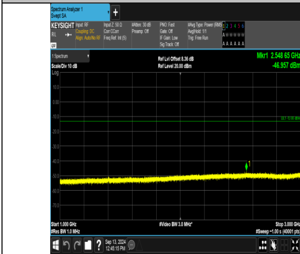
Band12_5MHz_16QAM_23035_25RB#0_1000~3000_1000~3000
