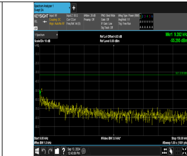
Band12_5MHz_16QAM_23035_1RB#24_0.009~0.15_0.009~0.15
