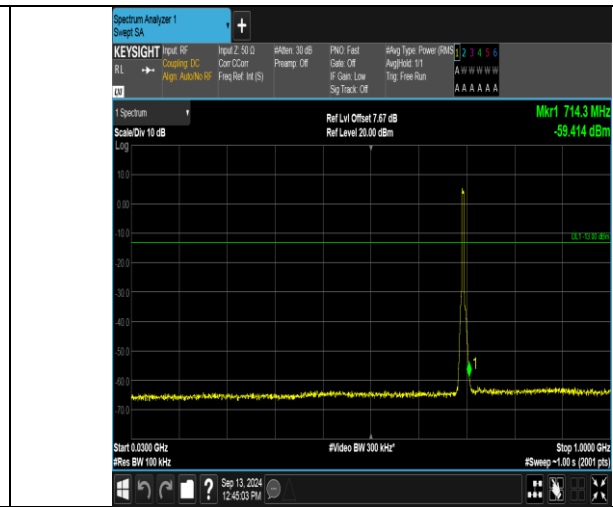
Band12_5MHz_16QAM_23035_25RB#0_30~1000_30~1000
