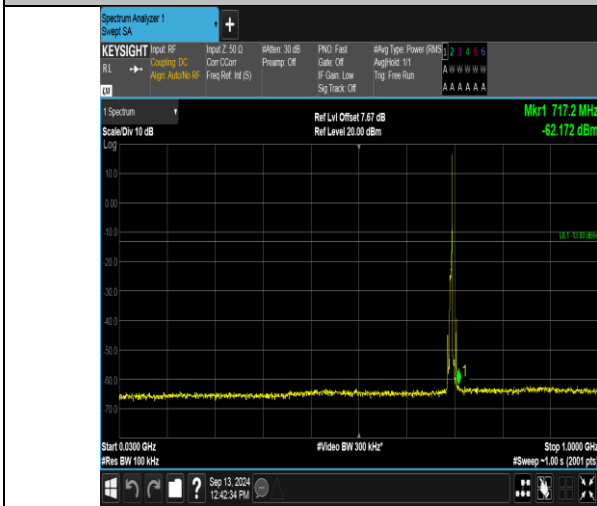
Band12_5MHz_QPSK_23035_1RB#24_30~1000_30~1000
