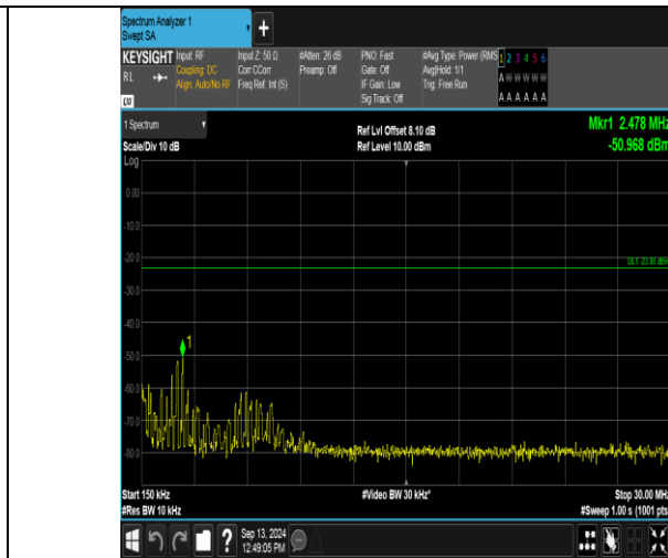
Band12_5MHz_QPSK_23095_25RB#0_0.15-30_0.15-30
