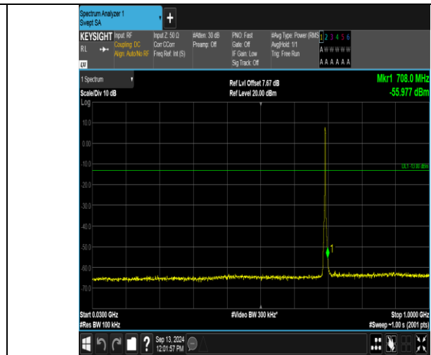
Band12_3MHz_16QAM_23025_15RB#0_30~1000_30~1000
