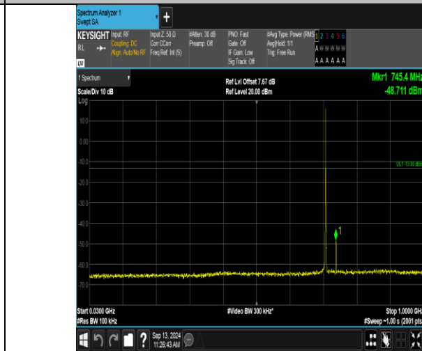
Band12_1.4MHz_16QAM_23173_1RB#5_30~1000_30~1000
