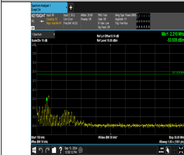
Band12_3MHz_16QAM_23025_1RB#14_0.15~30_0.15~30
