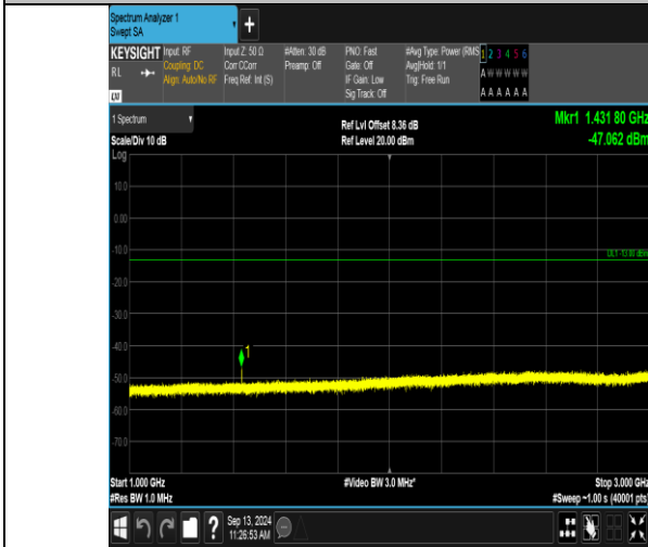
Band12_1.4MHz_16QAM_23173_1RB#5_1000~3000_1000~3000
