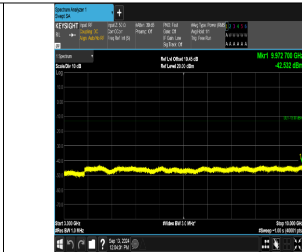
Band12_3MHz_16QAM_23095_1RB#0_3000~10000_3000~10000
