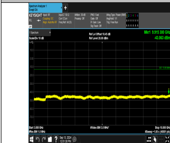
Band12_3MHz_QPSK_23025_15RB#0_3000-10000_3000-10000
