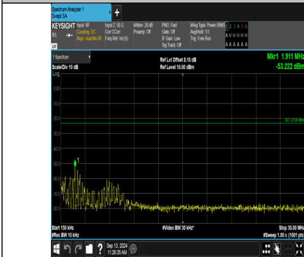
Band12_1.4MHz_16QAM_23173_1RB#5_0.15~30_0.15~30
