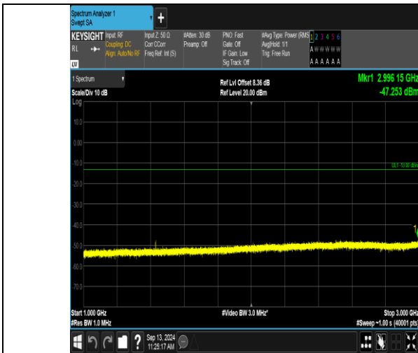
Band12_1.4MHz_16QAM_23173_1RB#0_1000-3000_1000-3000
