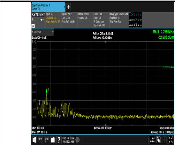
Band12_3MHz_QPSK_23025_1RB#14_0.15~30_0.15~30
