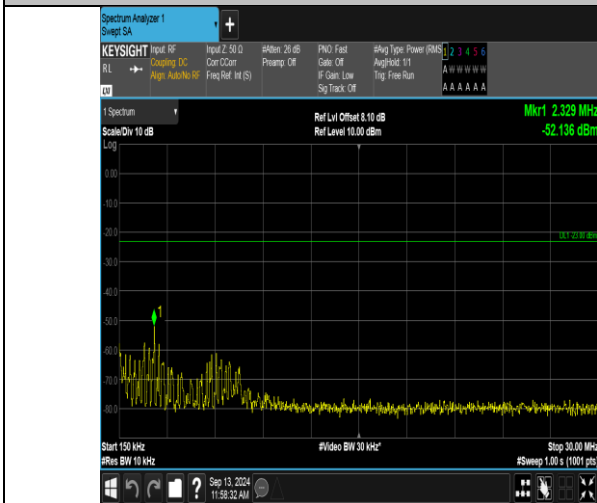
Band12_3MHz_16QAM_23025_1RB#0_0.15~30_0.15~30
