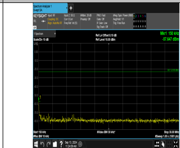
Band12_1.4MHz_QPSK_23173_1RB#0_0.15~30_0.15~30
