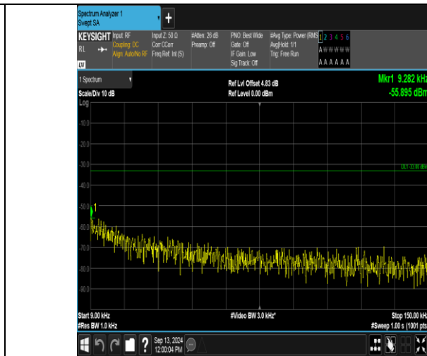
Band12_3MHz_16QAM_23025_1RB#14_0.009~0.15_0.009~0.15
