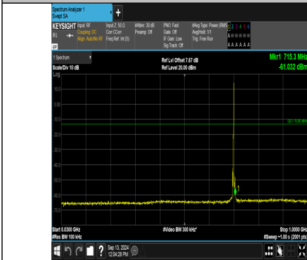
Band12_3MHz_QPSK_23095_1RB#14_30~1000_30~1000
