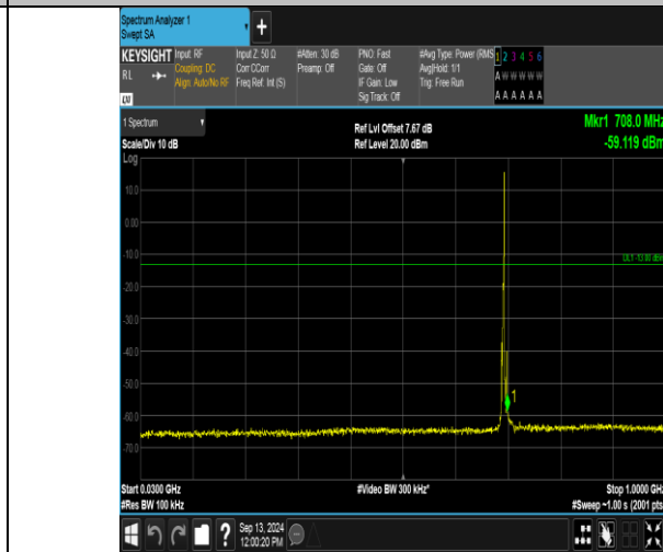
Band12_3MHz_16QAM_23025_1RB#14_30~1000_30~1000
