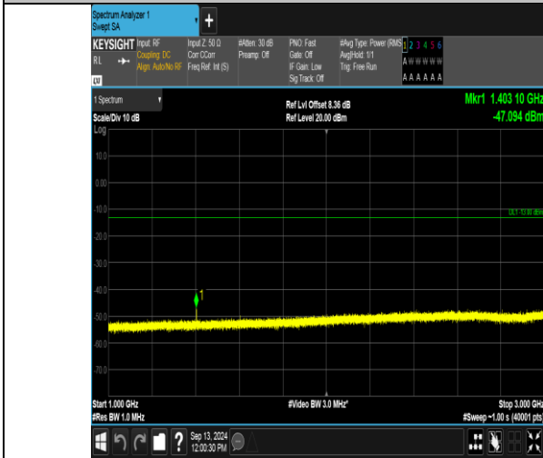
Band12_3MHz_16QAM_23025_1RB#14_1000~3000_1000~3000
