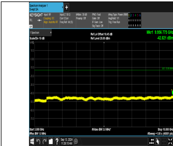
Band12_1.4MHz_QPSK_23173_1RB#5_3000~10000_3000~10000
