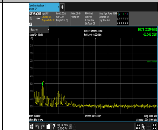
Band12_3MHz_QPSK_23095_1RB#0_0.15~30_0.15~30
