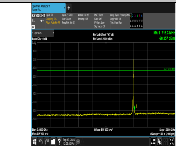
Band12_3MHz_16QAM_23095_1RB#0_30~1000_30~1000
