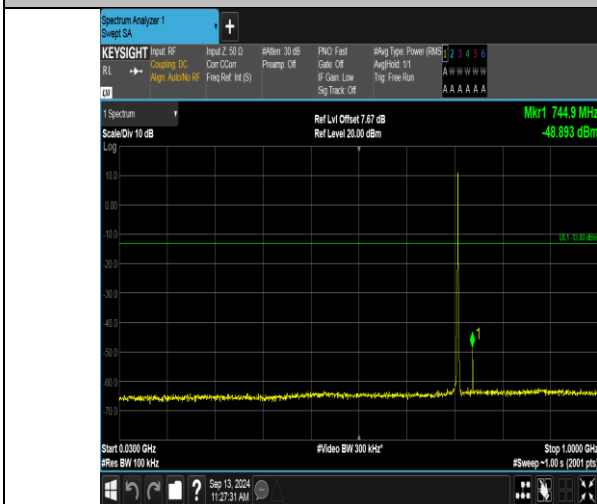
Band12_1.4MHz_QPSK_23173_6RB#0_30~1000_30~1000
