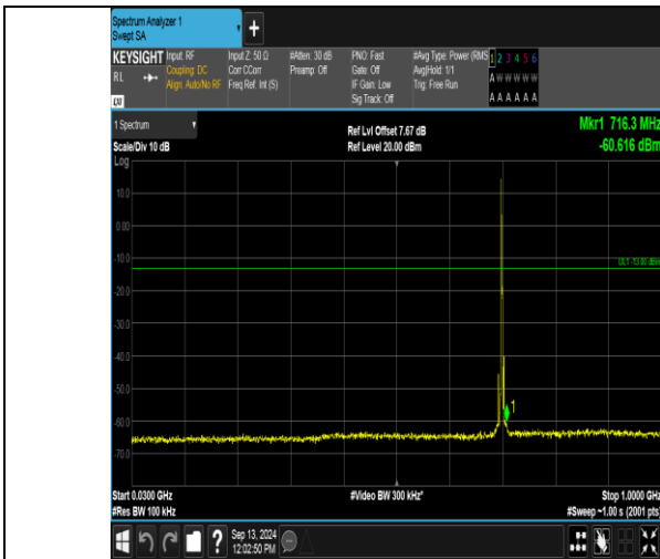
Band12_3MHz_QPSK_23095_1RB#0_30~1000_30~1000
