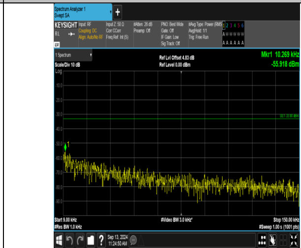
Band12_1.4MHz_16QAM_23173_1RB#0_0.009~0.15_0.009~0.15
