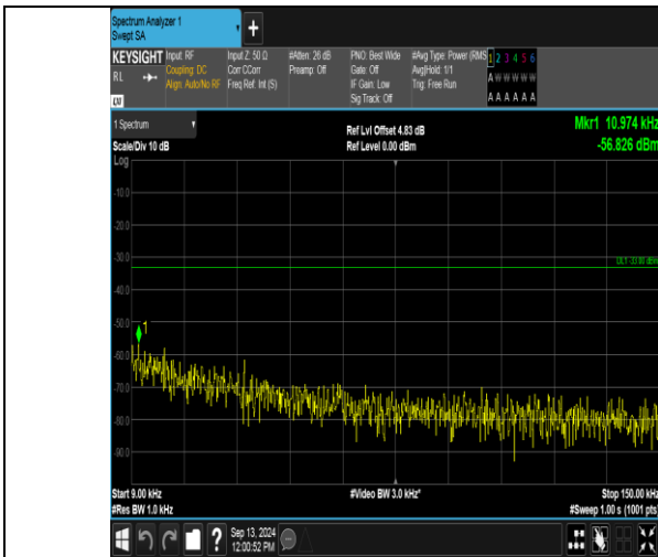
Band12_3MHz_QPSK_23025_15RB#0_0.009-0.15_0.009-0.15
