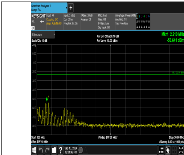
Band12_3MHz_16QAM_23025_15RB#0_0.15~30_0.15~30
