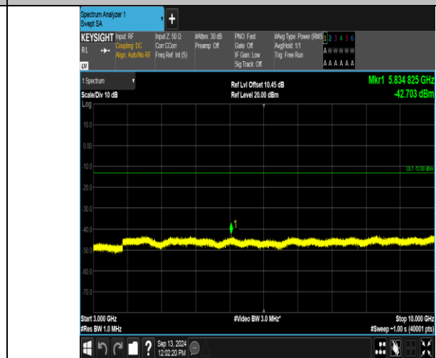
Band12_3MHz_16QAM_23025_15RB#0_3000~10000_3000~10000
