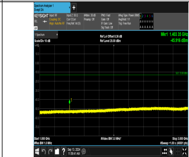
Band12_3MHz_QPSK_23025_1RB#14_1000~3000_1000~3000
