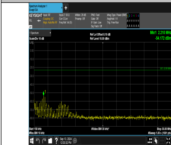
Band12_3MHz_16QAM_23095_1RB#0_0.15~30_0.15~30
