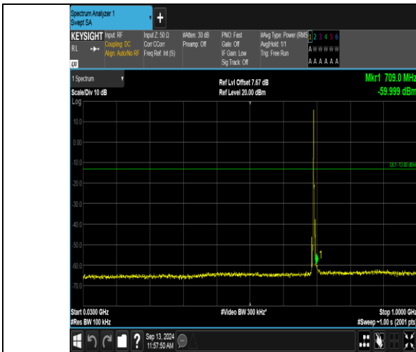
Band12_3MHz_QPSK_23025_1RB#0_30~1000_30~1000
