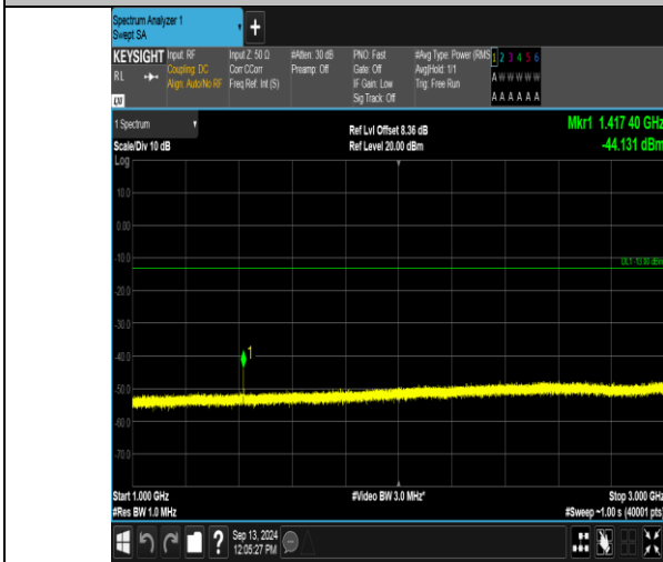
Band12_3MHz_16QAM_23095_1RB#14_1000~3000_1000~3000
