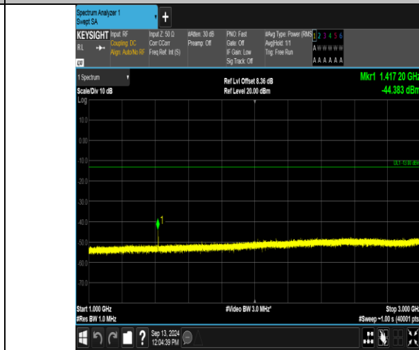
Band12_3MHz_QPSK_23095_1RB#14_1000~3000_1000~3000
