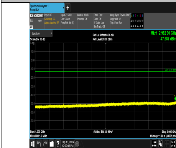
Band12_3MHz_16QAM_23025_15RB#0_1000~3000_1000~3000
