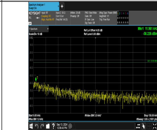
Band12_3MHz_16QAM_23095_15RB#0_0.009-0.15_0.009-0.15
