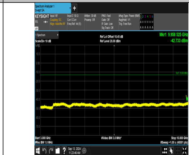
Band12_1.4MHz_16QAM_23095_6RB#0_3000~10000_3000~10000
