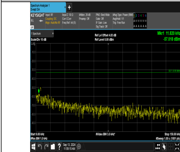
Band12_3MHz_QPSK_23025_1RB#14_0.009~0.15_0.009~0.15
