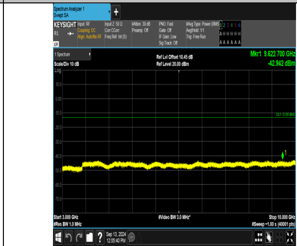
Band12_3MHz_16QAM_23095_1RB#14_3000~10000_3000~10000
