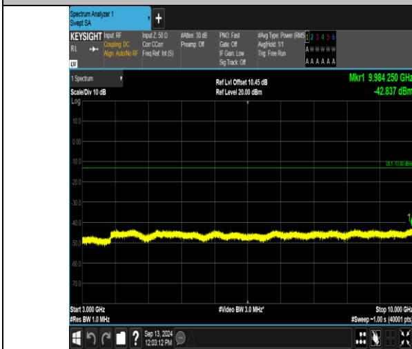
Band12_3MHz_QPSK_23095_1RB#0_3000~10000_3000~10000
