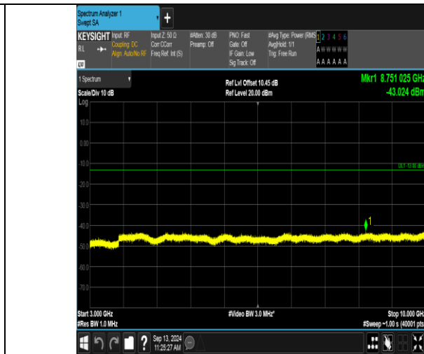
Band12_1.4MHz_16QAM_23173_1RB#0_3000-10000_3000-10000
