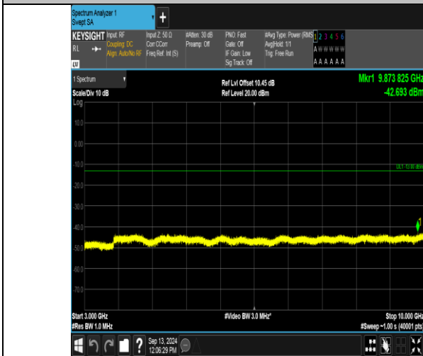
Band12_3MHz_QPSK_23095_15RB#0_3000-10000_3000-10000
