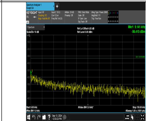
Band12_3MHz_16QAM_23095_1RB#0_0.009~0.15_0.009~0.15
