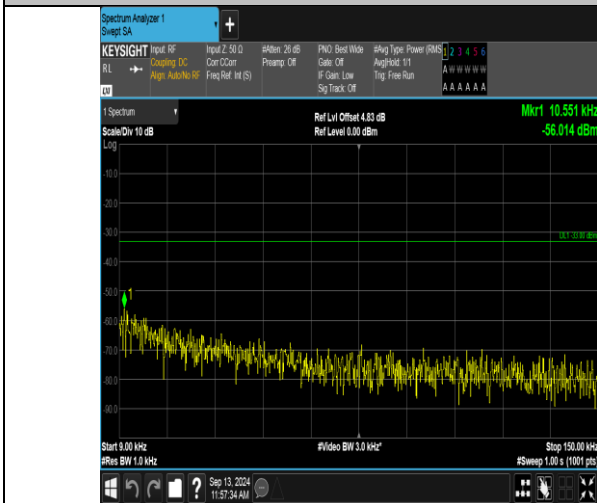
Band12_3MHz_QPSK_23025_1RB#0_0.009~0.15_0.009~0.15
