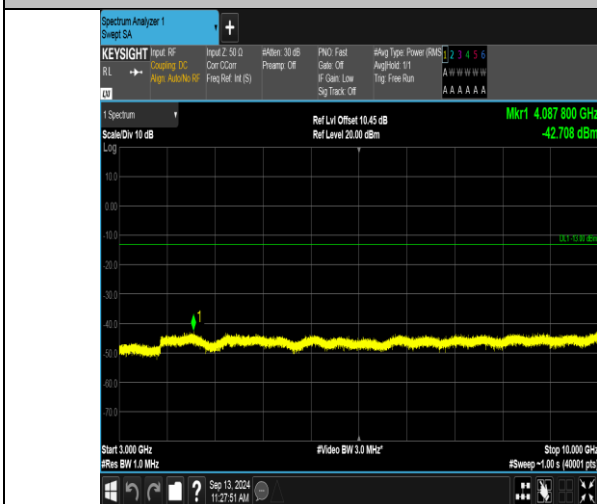
Band12_1.4MHz_QPSK_23173_6RB#0_3000~10000_3000~10000
