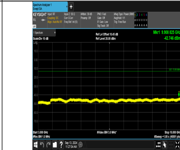
Band12_1.4MHz_16QAM_23173_1RB#5_3000~10000_3000~10000
