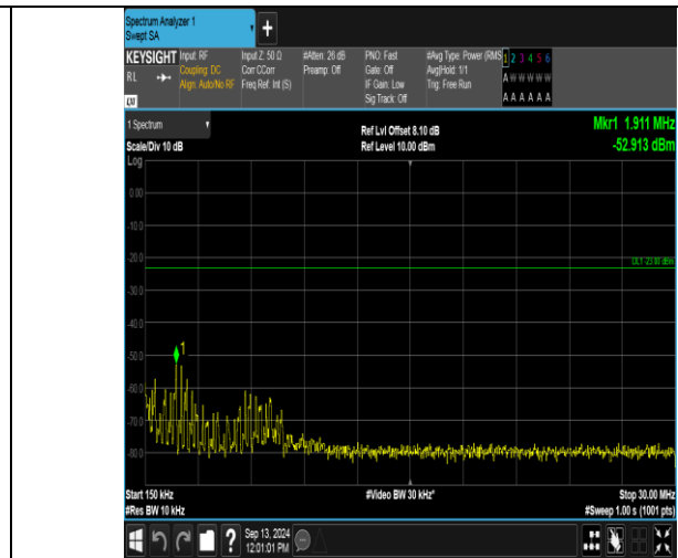
Band12_3MHz_QPSK_23025_15RB#0_0.15-30_0.15-30
