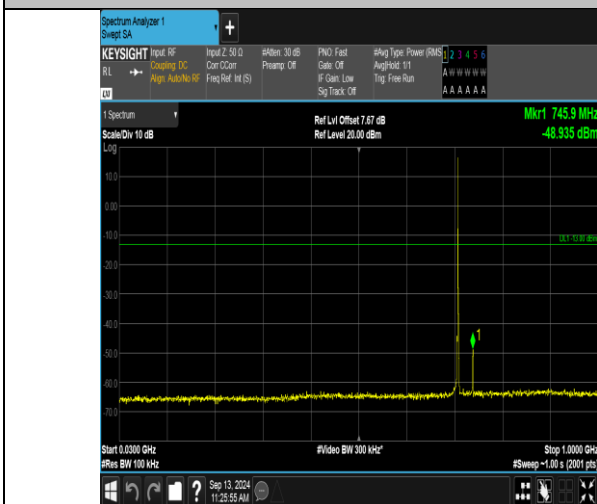
Band12_1.4MHz_QPSK_23173_1RB#5_30-1000_30-1000
