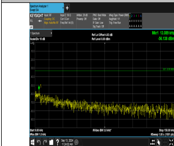
Band12_1.4MHz_QPSK_23173_1RB#0_0.009~0.15_0.009~0.15
