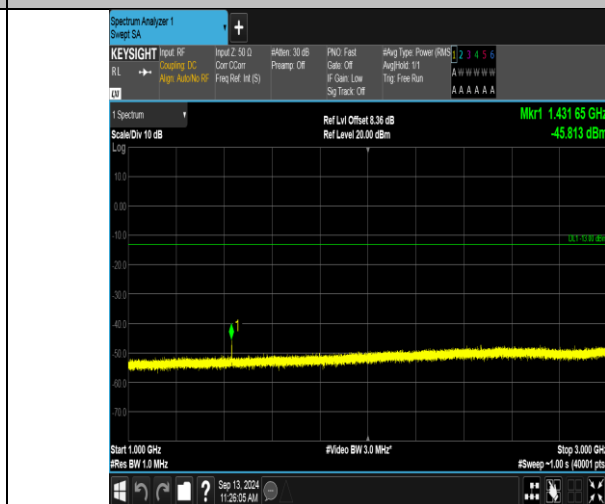
Band12_1.4MHz_QPSK_23173_1RB#5_1000-3000_1000-3000
