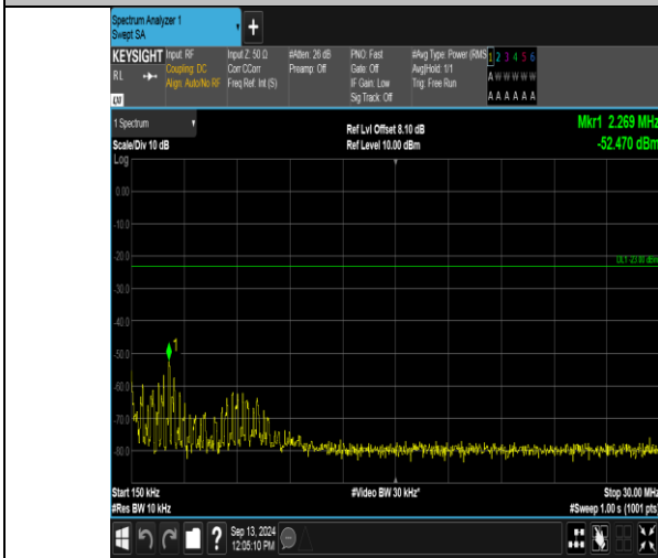
Band12_3MHz_16QAM_23095_1RB#14_0.15~30_0.15~30
