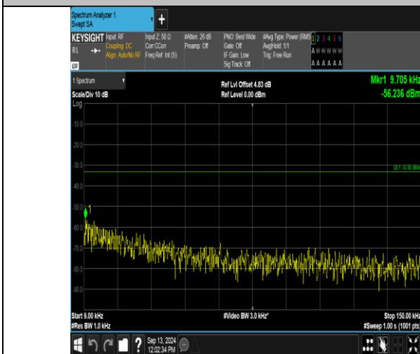
Band12_3MHz_QPSK_23095_1RB#0_0.009~0.15_0.009~0.15
