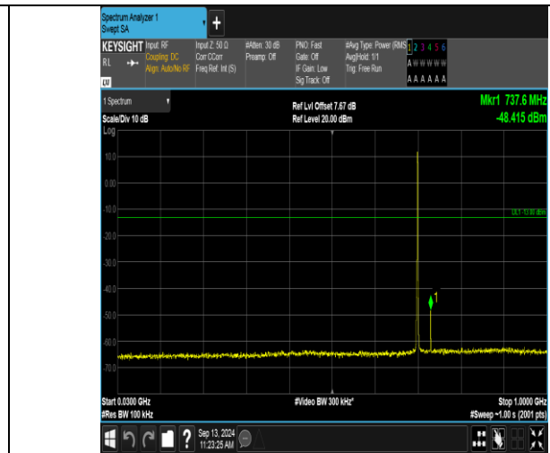
Band12_1.4MHz_16QAM_23095_6RB#0_30~1000_30~1000
