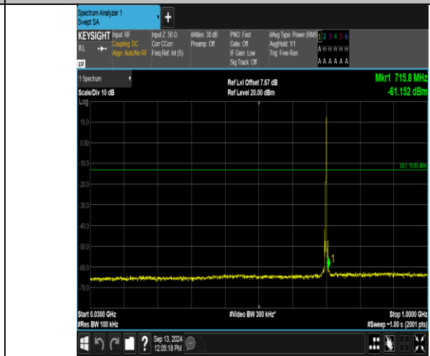
Band12_3MHz_16QAM_23095_1RB#14_30~1000_30~1000
