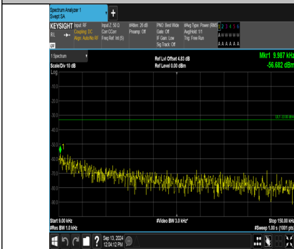
Band12_3MHz_QPSK_23095_1RB#14_0.009~0.15_0.009~0.15
