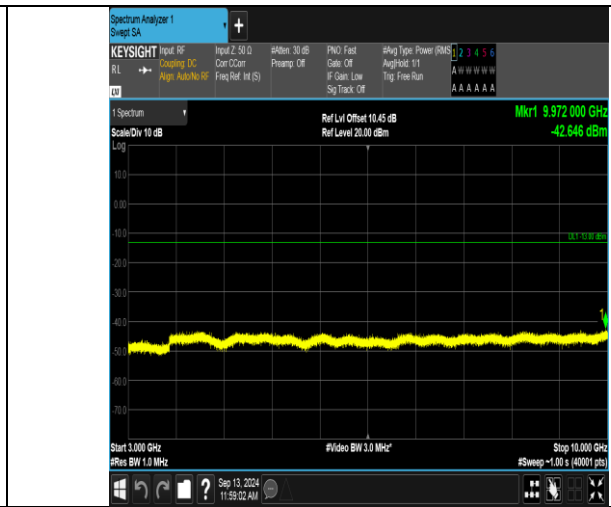
Band12_3MHz_16QAM_23025_1RB#0_3000~10000_3000~10000
