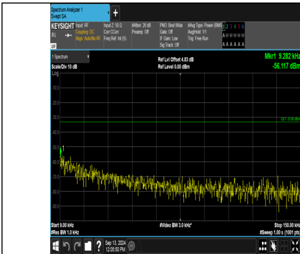
Band12_3MHz_QPSK_23095_15RB#0_0.009-0.15_0.009-0.15
