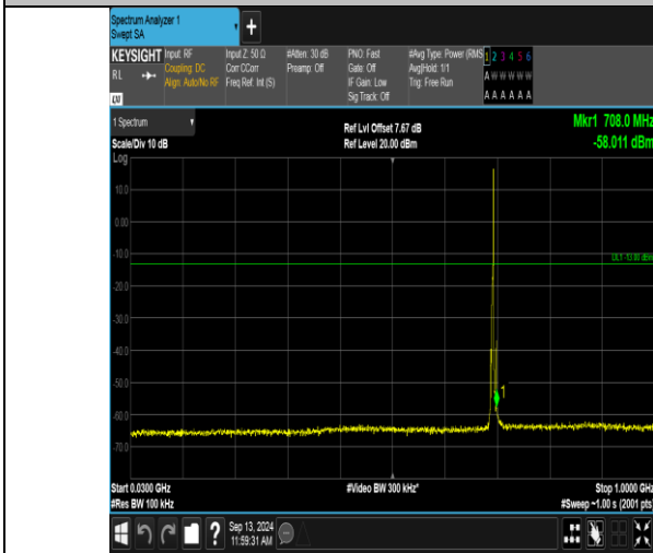
Band12_3MHz_QPSK_23025_1RB#14_30~1000_30~1000
