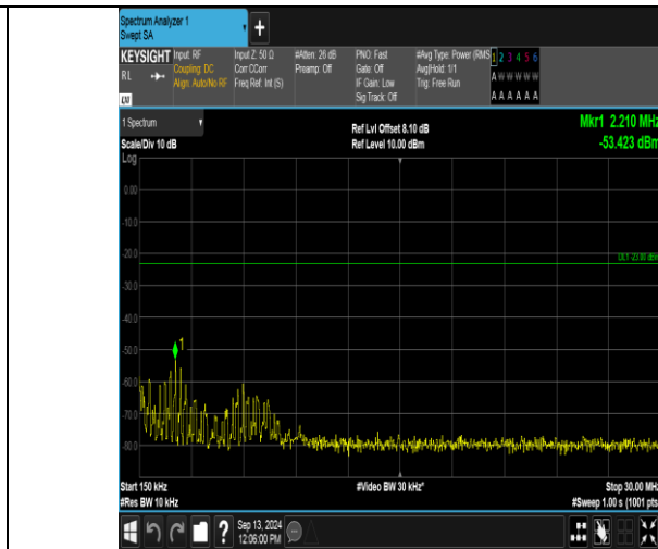
Band12_3MHz_QPSK_23095_15RB#0_0.15-30_0.15-30
