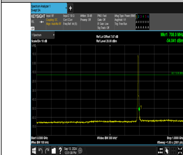
Band12_3MHz_QPSK_23025_15RB#0_30-1000_30-1000
