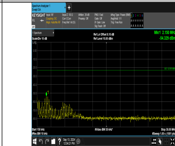
Band12_3MHz_QPSK_23095_1RB#14_0.15~30_0.15~30
