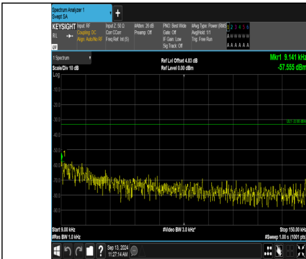
Band12_1.4MHz_QPSK_23173_6RB#0_0.009~0.15_0.009~0.15
