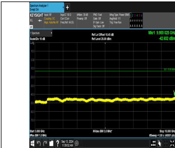
Band12_3MHz_QPSK_23025_1RB#14_3000~10000_3000~10000
