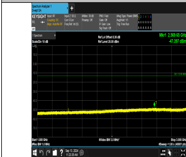
Band12_1.4MHz_16QAM_23095_6RB#0_1000~3000_1000~3000
