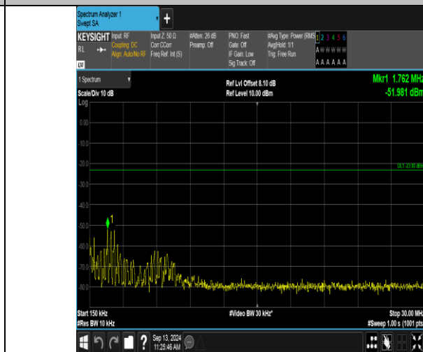
Band12_1.4MHz_QPSK_23173_1RB#5_0.15-30_0.15-30
