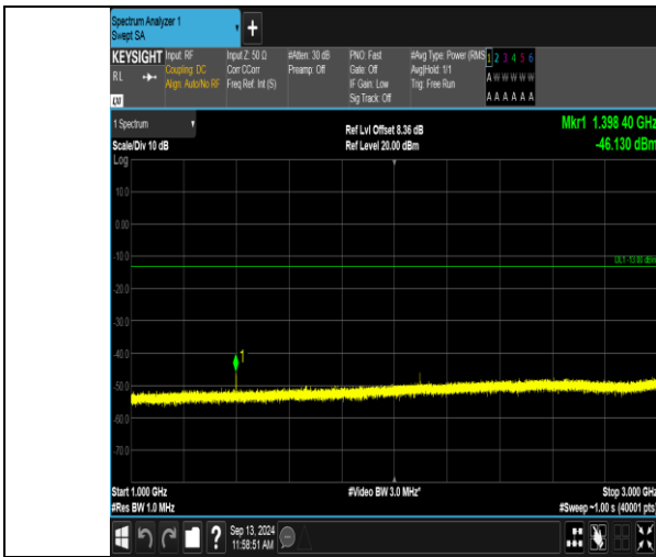
Band12_3MHz_16QAM_23025_1RB#0_1000~3000_1000~3000
