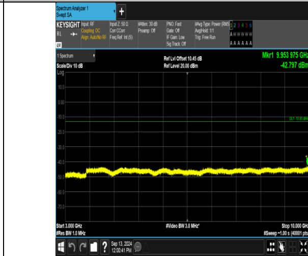
Band12_3MHz_16QAM_23025_1RB#14_3000~10000_3000~10000
