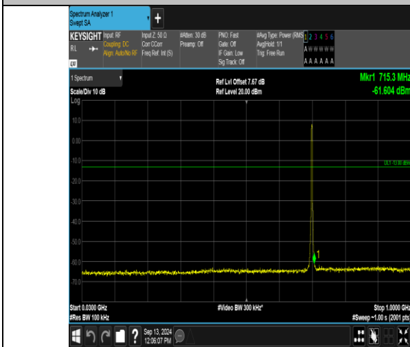
Band12_3MHz_QPSK_23095_15RB#0_30-1000_30-1000
