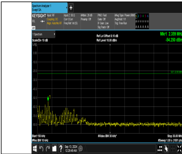
Band5_10MHz_16QAM_20450_50RB#0_0.15~30_0.15~30
