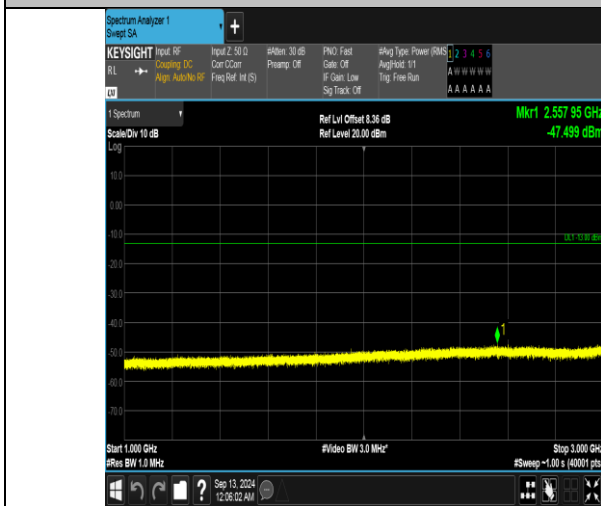
Band5_5MHz_16QAM_20525_25RB#0_1000~3000_1000~3000
