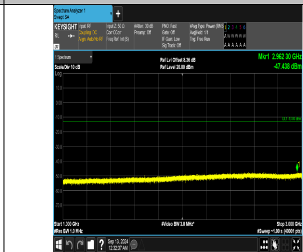
Band5_10MHz_QPSK_20525_1RB#49_1000-3000_1000-3000
