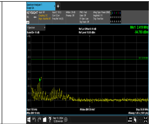
Band5_5MHz_QPSK_20625_25RB#0_0.15-30_0.15-30
