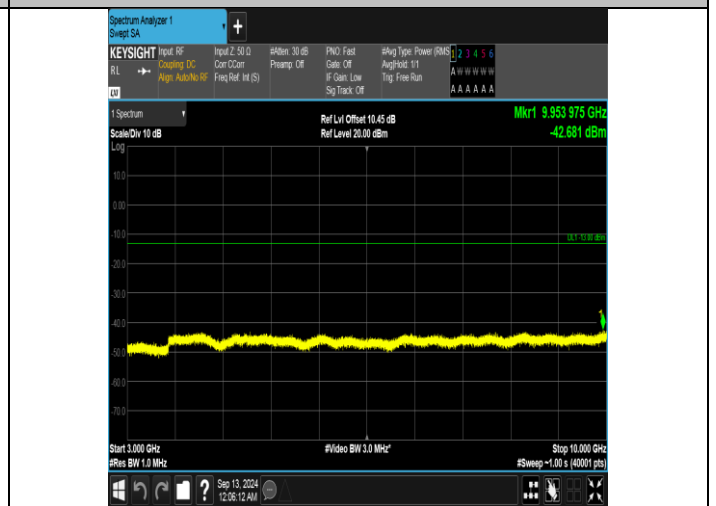
Band5_5MHz_16QAM_20525_25RB#0_3000~10000_3000~10000
