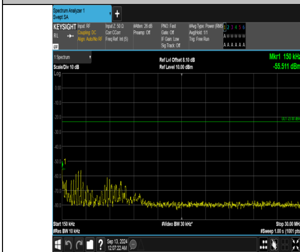
Band5_5MHz_16QAM_20625_1RB#0_0.15~30_0.15~30
