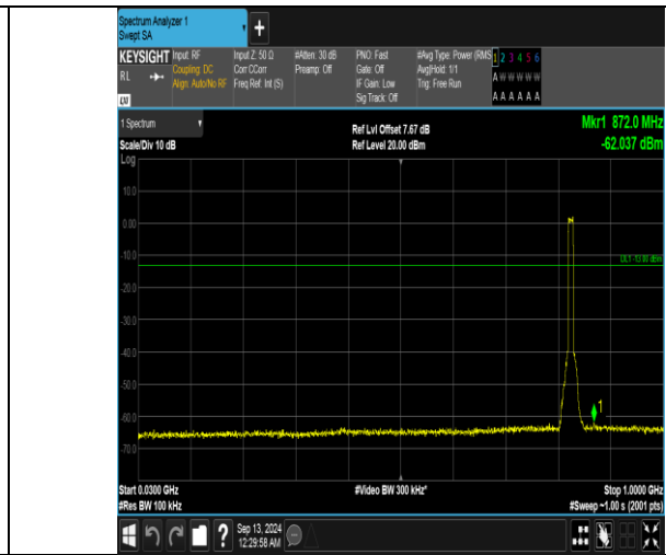
Band5_10MHz_16QAM_20450_50RB#0_30~1000_30~1000
