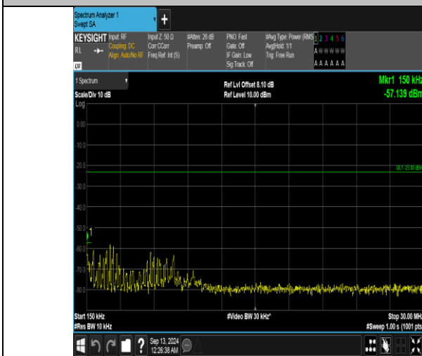
Band5_10MHz_16QAM_20450_1RB#0_0.15~30_0.15~30
