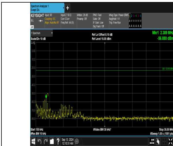
Band5_5MHz_16QAM_20625_25RB#0_0.15~30_0.15~30
