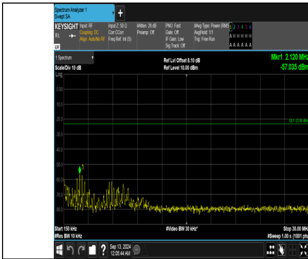
Band5_5MHz_16QAM_20525_25RB#0_0.15~30_0.15~30
