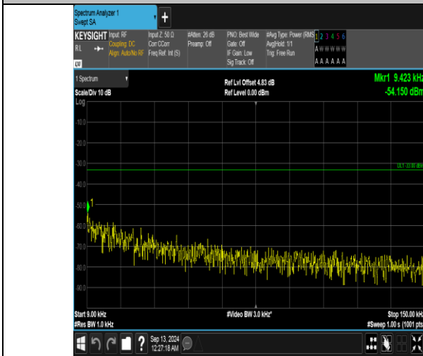
Band5_10MHz_QPSK_20450_1RB#49_0.009-0.15_0.009-0.15
