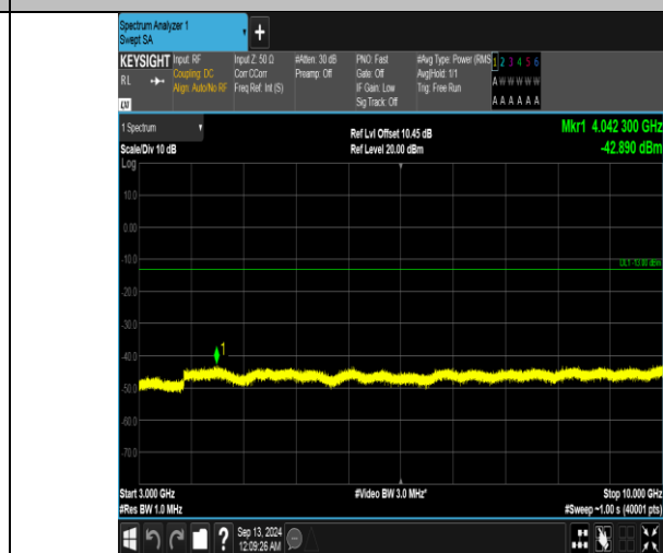
Band5_5MHz_16QAM_20625_1RB#24_3000~10000_3000~10000
