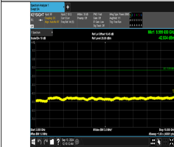
Band5_5MHz_QPSK_20625_25RB#0_3000-10000_3000-10000
