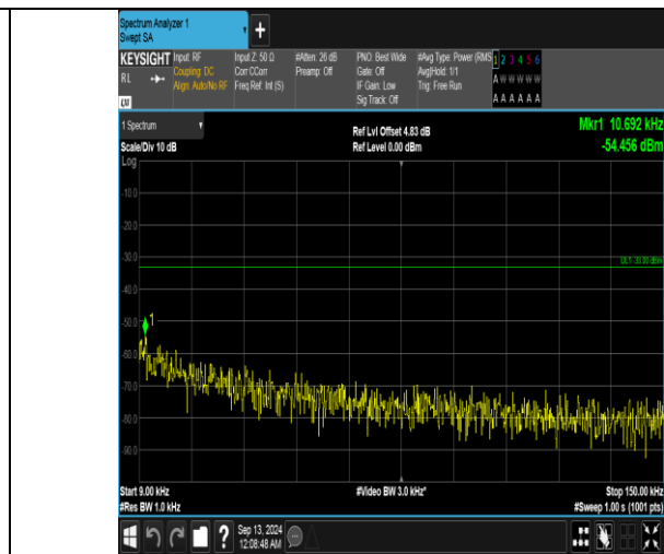
Band5_5MHz_16QAM_20625_1RB#24_0.009~0.15_0.009~0.15
