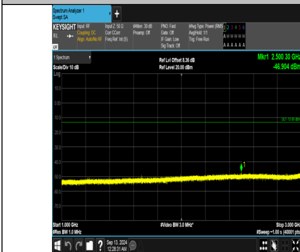
Band5_10MHz_16QAM_20450_1RB#49_1000~3000_1000~3000
