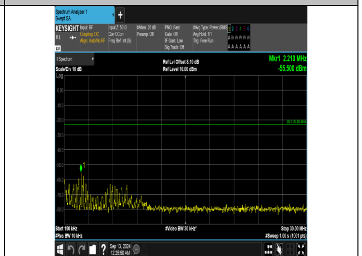
Band5_10MHz_QPSK_20450_1RB#0_0.15~30_0.15~30
