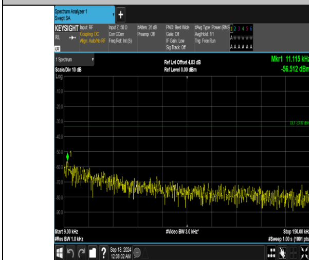
Band5_5MHz_QPSK_20625_1RB#24_0.009-0.15_0.009-0.15
