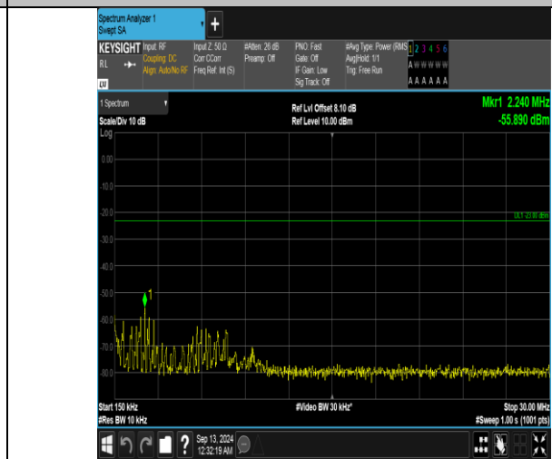
Band5_10MHz_QPSK_20525_1RB#49_0.15-30_0.15-30
