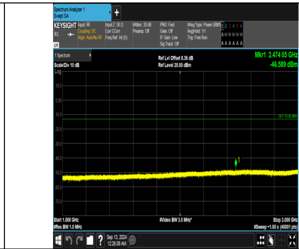
Band5_10MHz_QPSK_20450_1RB#0_1000~3000_1000~3000
