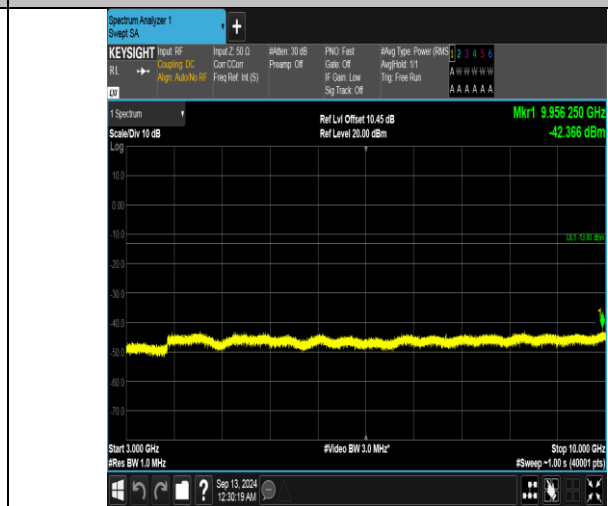
Band5_10MHz_16QAM_20450_50RB#0_3000~10000_3000~10000
