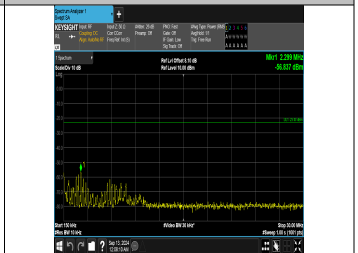
Band5_5MHz_QPSK_20625_1RB#24_0.15-30_0.15-30
