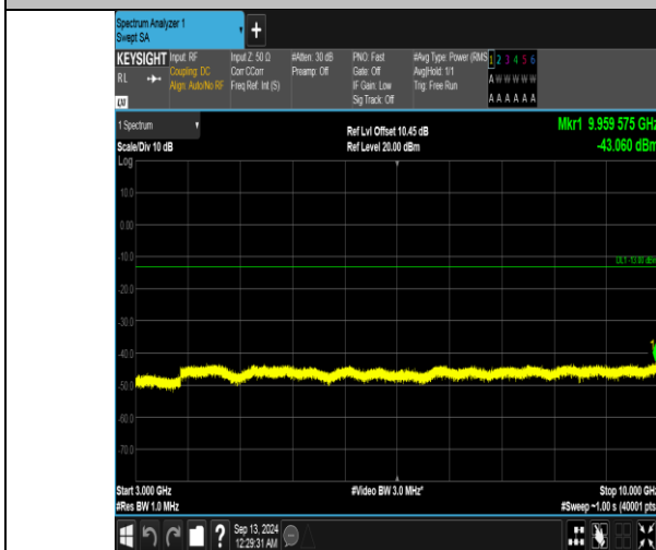
Band5_10MHz_QPSK_20450_50RB#0_3000-10000_3000-10000
