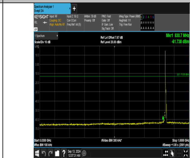
Band5_5MHz_16QAM_20625_1RB#0_30~1000_30~1000
