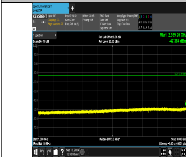
Band5_10MHz_16QAM_20450_50RB#0_1000~3000_1000~3000
