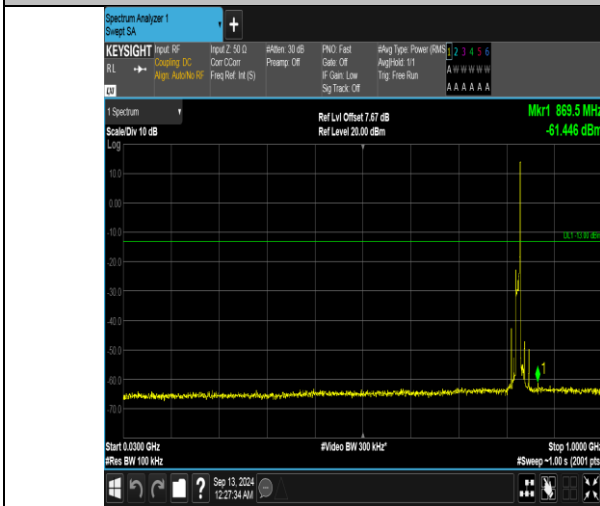
Band5_10MHz_QPSK_20450_1RB#49_30-1000_30-1000
