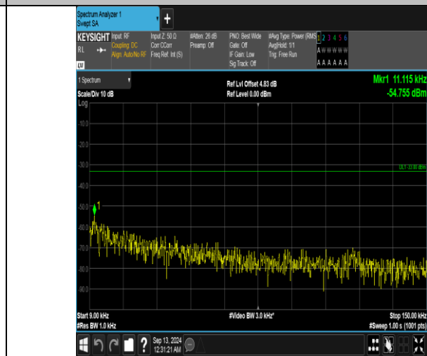
Band5_10MHz_16QAM_20525_1RB#0_0.009~0.15_0.009~0.15
