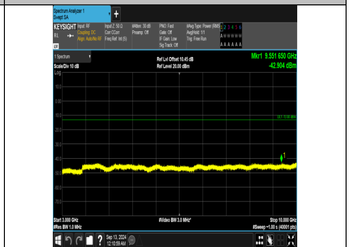
Band5_5MHz_16QAM_20625_25RB#0_3000~10000_3000~10000
