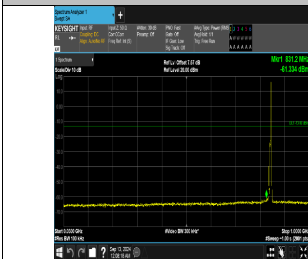
Band5_5MHz_QPSK_20625_1RB#24_30-1000_30-1000
