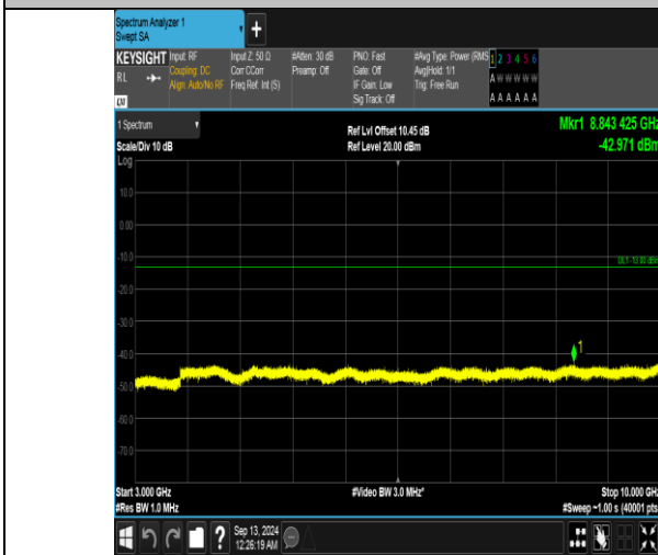
Band5_10MHz_QPSK_20450_1RB#0_3000~10000_3000~10000
