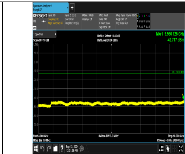
Band5_10MHz_16QAM_20525_1RB#0_3000-10000_3000-10000
