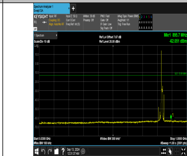
Band5_10MHz_16QAM_20525_1RB#0_30~1000_30~1000
