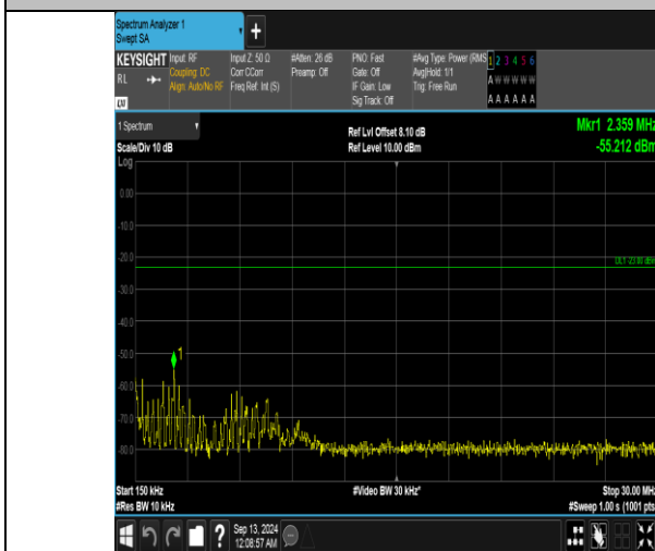
Band5_5MHz_16QAM_20625_1RB#24_0.15~30_0.15~30
