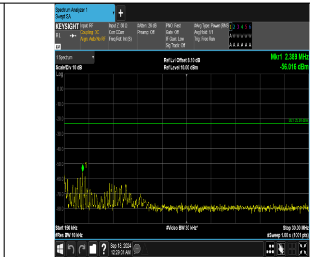
Band5_10MHz_QPSK_20450_50RB#0_0.15-30_0.15-30
