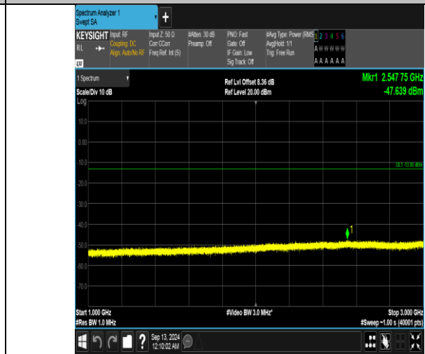
Band5_5MHz_QPSK_20625_25RB#0_1000-3000_1000-3000
