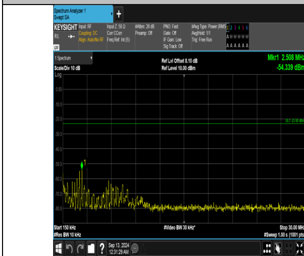
Band5_10MHz_16QAM_20525_1RB#0_0.15~30_0.15~30
