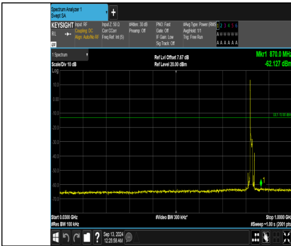
Band5_10MHz_QPSK_20450_1RB#0_30~1000_30~1000
