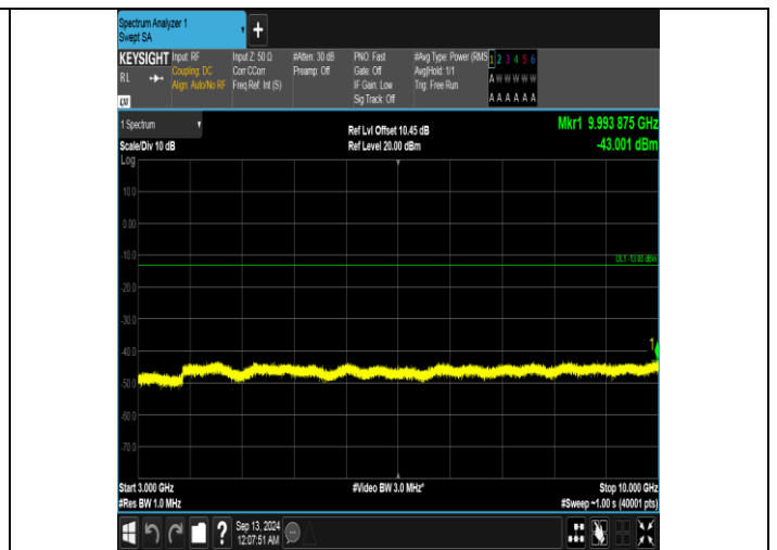
Band5_5MHz_16QAM_20625_1RB#0_3000-10000_3000-10000
