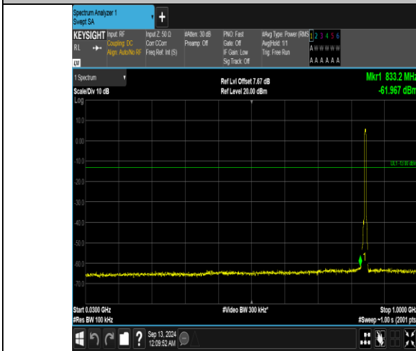
Band5_5MHz_QPSK_20625_25RB#0_30-1000_30-1000
