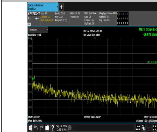
Band5_10MHz_QPSK_20525_1RB#49_0.009-0.15_0.009-0.15
