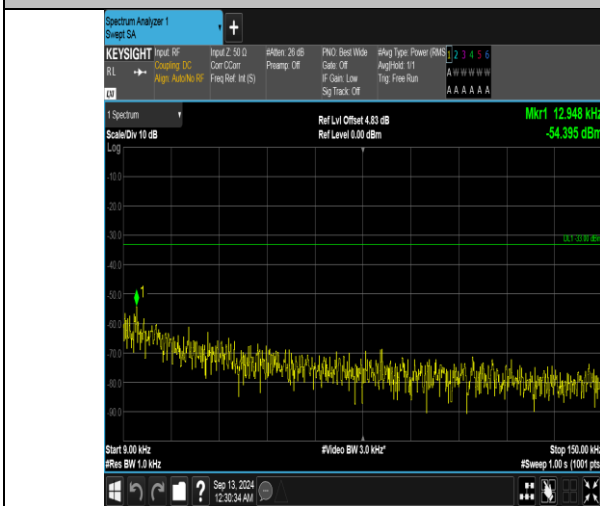
Band5_10MHz_QPSK_20525_1RB#0_0.009~0.15_0.009~0.15
