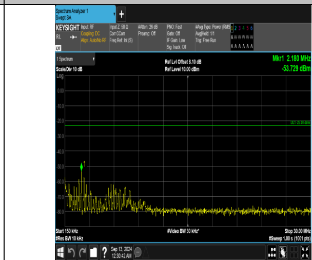
Band5_10MHz_QPSK_20525_1RB#0_0.15~30_0.15~30
