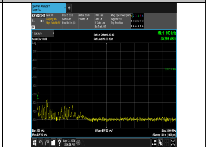
Band5_5MHz_QPSK_20625_1RB#0_0.15~30_0.15~30
