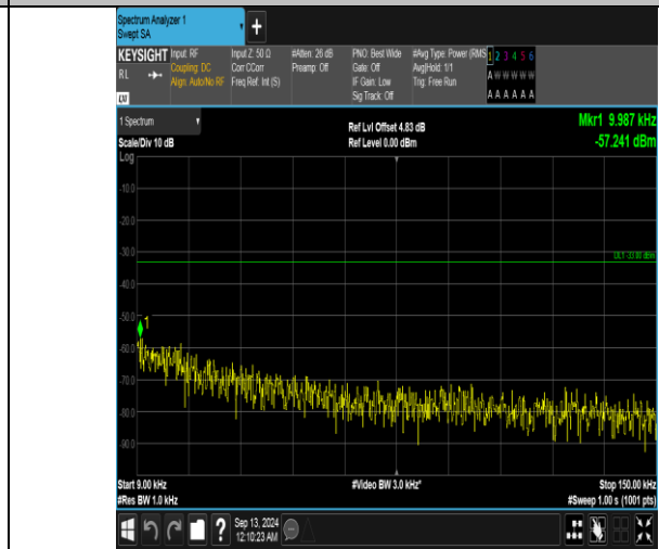
Band5_5MHz_16QAM_20625_25RB#0_0.009-0.15_0.009-0.15
