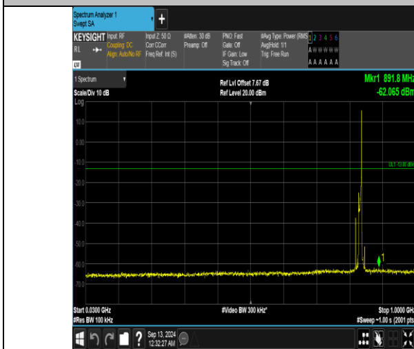
Band5_10MHz_QPSK_20525_1RB#49_30-1000_30-1000
