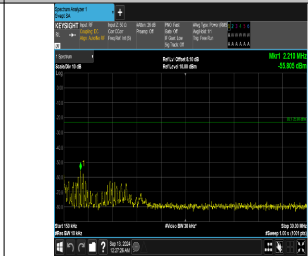
Band5_10MHz_QPSK_20450_1RB#49_0.15-30_0.15-30
