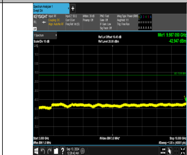
Band5_10MHz_16QAM_20450_1RB#49_3000~10000_3000~10000
