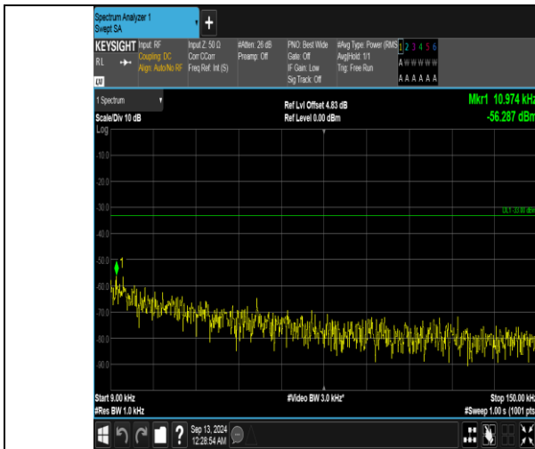
Band5_10MHz_QPSK_20450_50RB#0_0.009-0.15_0.009-0.15
