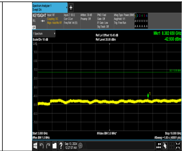
Band5_10MHz_16QAM_20450_1RB#0_3000-10000_3000-10000
