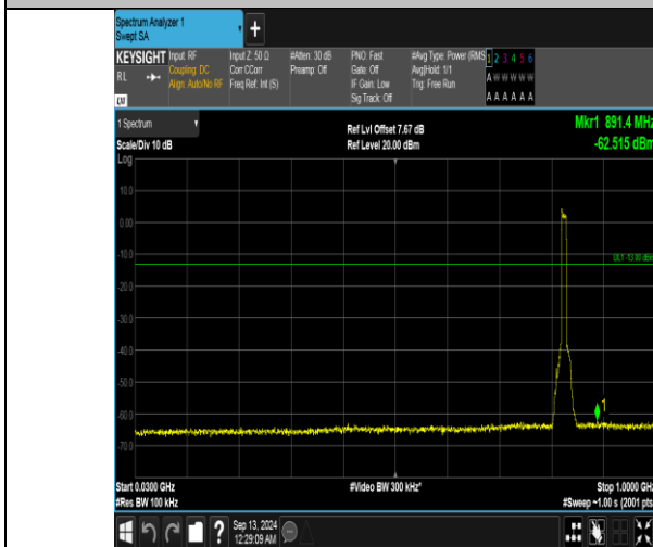
Band5_10MHz_QPSK_20450_50RB#0_30-1000_30-1000
