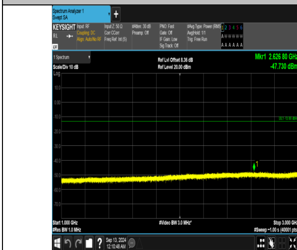
Band5_5MHz_16QAM_20625_25RB#0_1000~3000_1000~3000
