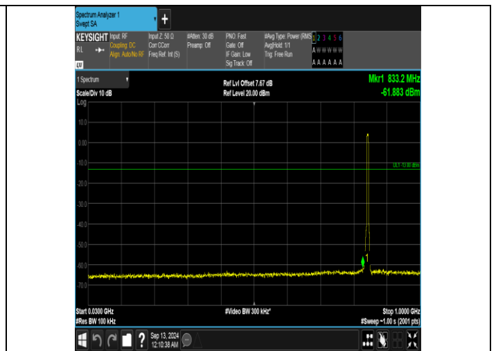
Band5_5MHz_16QAM_20625_25RB#0_30~1000_30~1000
