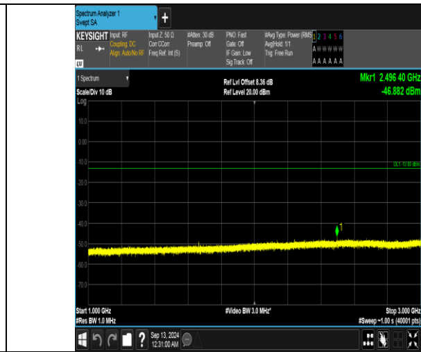
Band5_10MHz_QPSK_20525_1RB#0_1000~3000_1000~3000
