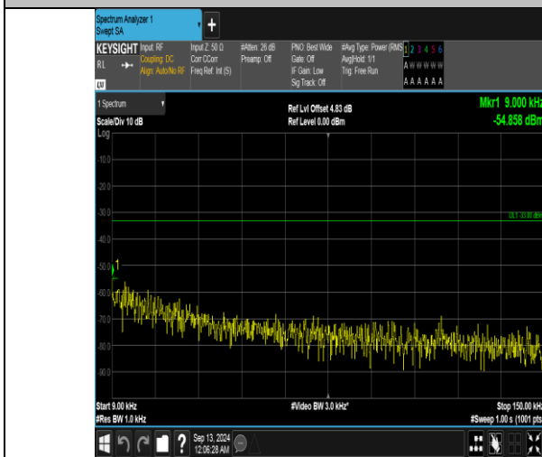
Band5_5MHz_QPSK_20625_1RB#0_0.009~0.15_0.009~0.15
