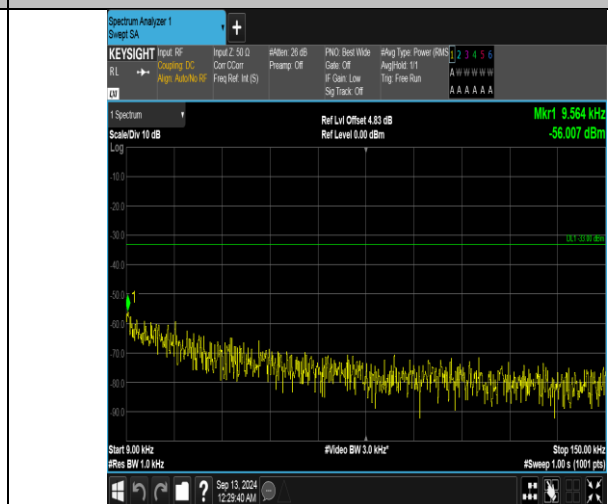
Band5_10MHz_16QAM_20450_50RB#0_0.009-0.15_0.009-0.15
