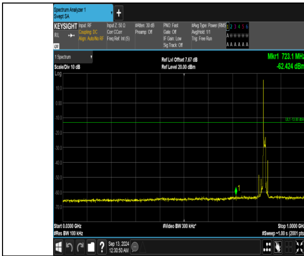
Band5_10MHz_QPSK_20525_1RB#0_30~1000_30~1000
