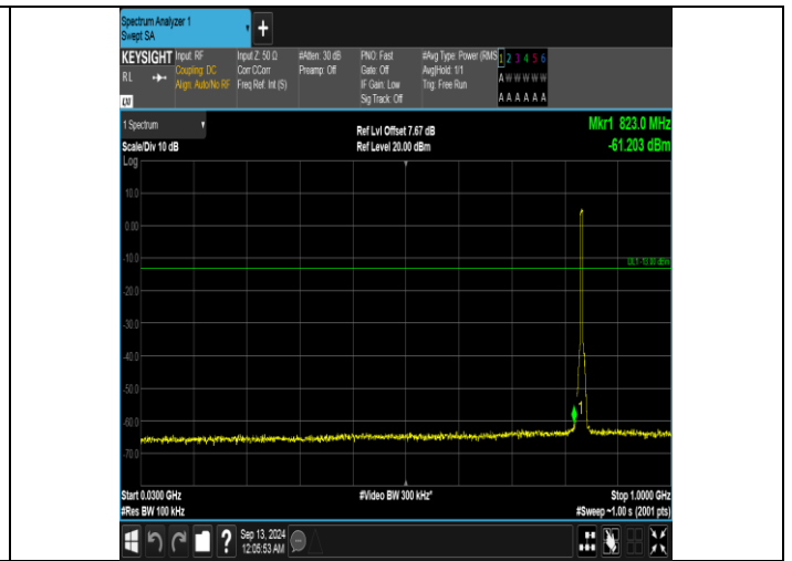
Band5_5MHz_16QAM_20525_25RB#0_30~1000_30~1000
