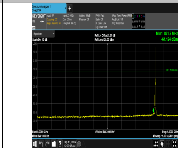
Band5_5MHz_16QAM_20625_1RB#24_30~1000_30~1000
