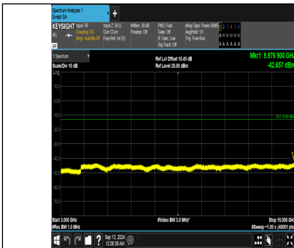
Band5_5MHz_QPSK_20625_1RB#24_3000~10000_3000~10000
