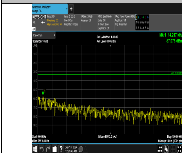
Band5_10MHz_QPSK_20450_1RB#0_0.009~0.15_0.009~0.15
