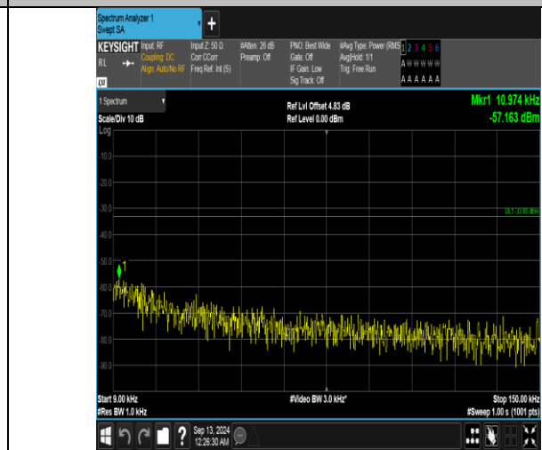
Band5_10MHz_16QAM_20450_1RB#0_0.009~0.15_0.009~0.15
