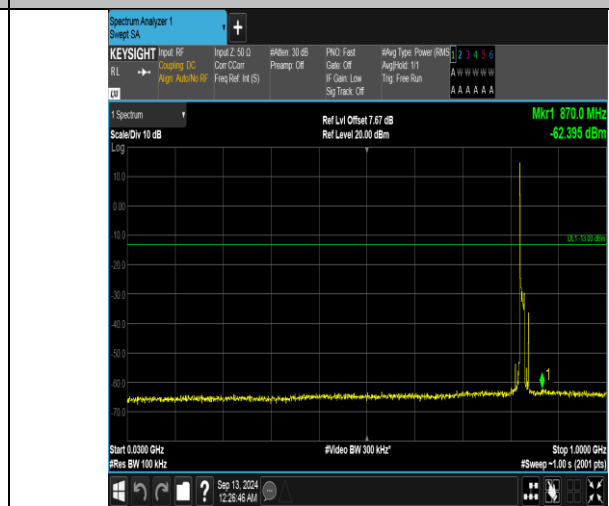
Band5_10MHz_16QAM_20450_1RB#0_30~1000_30~1000
