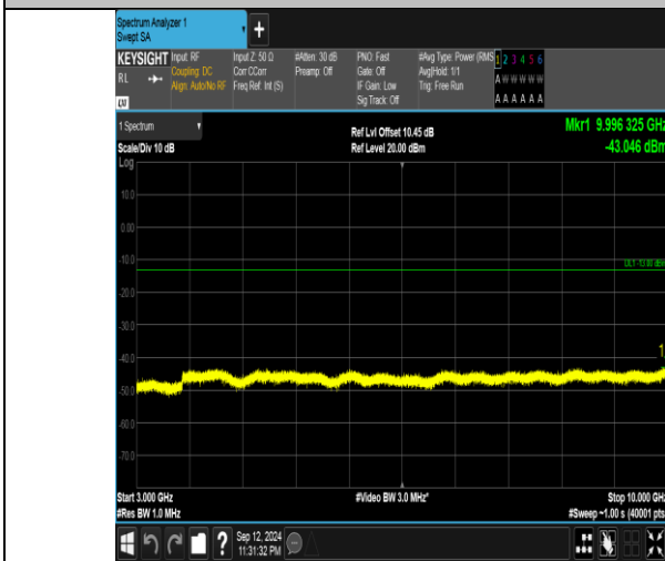
Band5_3MHz_QPSK_20525_1RB#0_3000~10000_3000~10000
