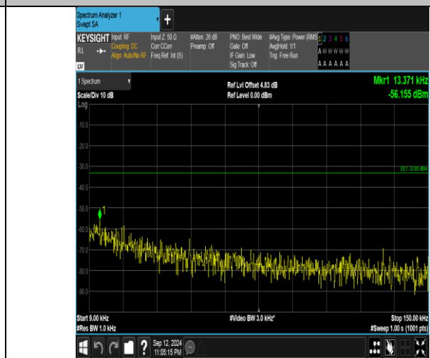
Band5_1.4MHz_16QAM_20525_6RB#0_0.009~0.15_0.009~0.15
