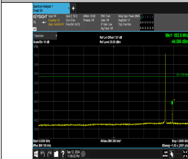
Band5_1.4MHz_QPSK_20643_6RB#0_30~1000_30~1000
