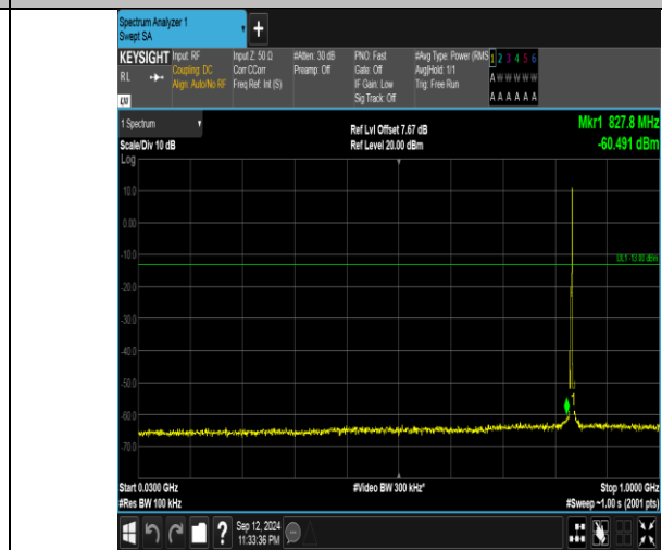
Band5_3MHz_16QAM_20525_1RB#14_30~1000_30~1000
