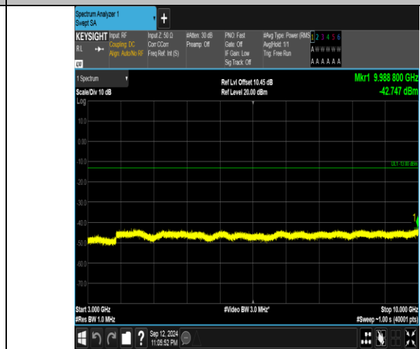
Band5_1.4MHz_16QAM_20525_6RB#0_3000~10000_3000~10000
