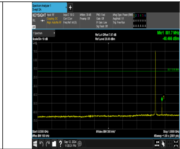
Band5_1.4MHz_16QAM_20525_6RB#0_30~1000_30~1000
