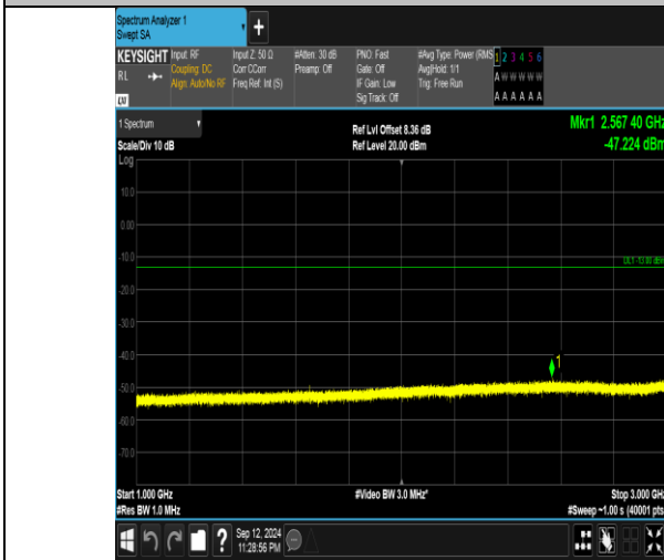
Band5_3MHz_16QAM_20415_1RB#14_1000~3000_1000~3000
