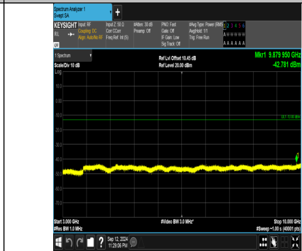
Band5_3MHz_16QAM_20415_1RB#14_3000~10000_3000~10000
