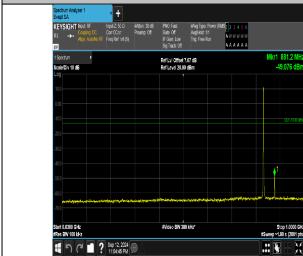
Band5_1.4MHz_QPSK_20525_6RB#0_30~1000_30~1000
