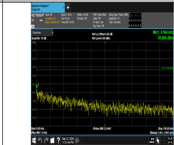
Band5_3MHz_16QAM_20525_1RB#0_0.009~0.15_0.009~0.15
