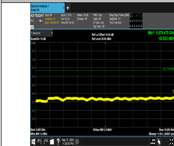
Band5_3MHz_QPSK_20415_15RB#0_3000-10000_3000-10000
