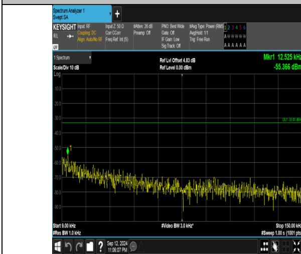
Band5_1.4MHz_QPSK_20643_1RB#0_0.009~0.15_0.009~0.15
