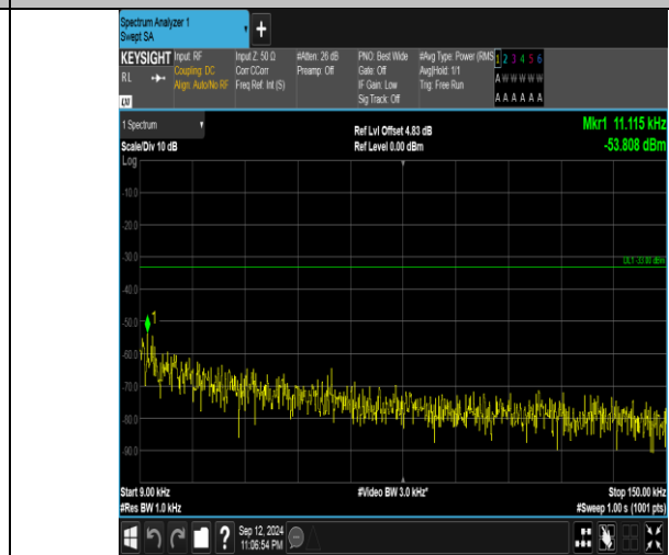
Band5_1.4MHz_16QAM_20643_1RB#0_0.009~0.15_0.009~0.15
