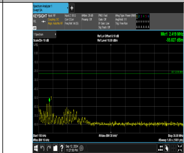
Band5_3MHz_QPSK_20415_1RB#14_0.15~30_0.15~30
