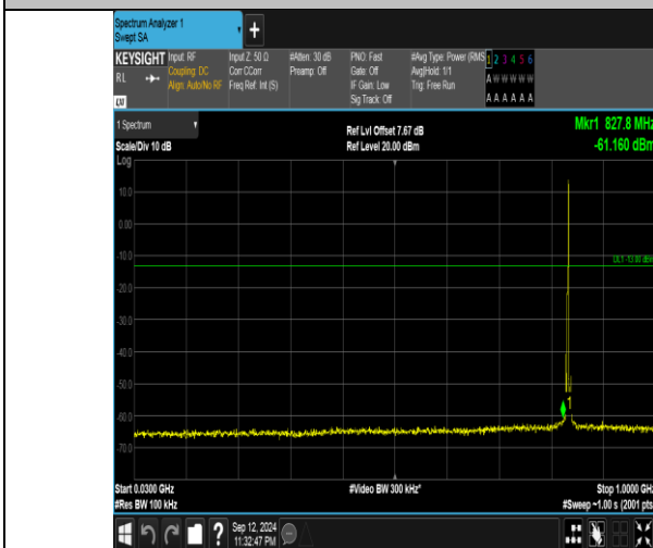
Band5_3MHz_QPSK_20525_1RB#14_30~1000_30~1000
