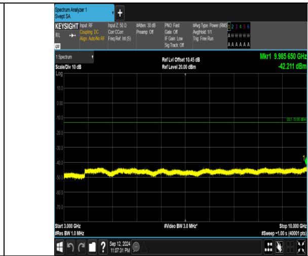
Band5_1.4MHz_16QAM_20643_1RB#0_3000~10000_3000~10000
