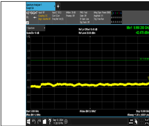
Band5_3MHz_QPSK_20415_1RB#14_3000~10000_3000~10000
