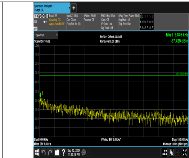
Band5_3MHz_16QAM_20525_1RB#14_0.009~0.15_0.009~0.15
