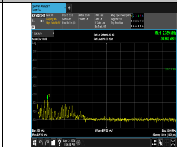
Band5_1.4MHz_QPSK_20643_1RB#0_0.15~30_0.15~30
