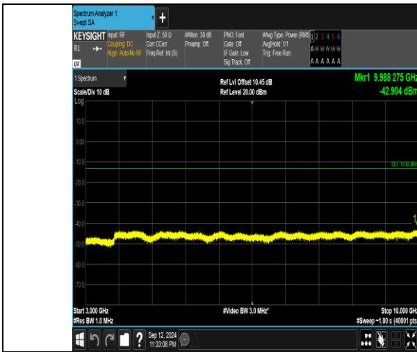
Band5_3MHz_QPSK_20525_1RB#14_3000~10000_3000~10000
