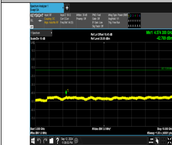
Band5_1.4MHz_QPSK_20643_6RB#0_3000~10000_3000~10000
