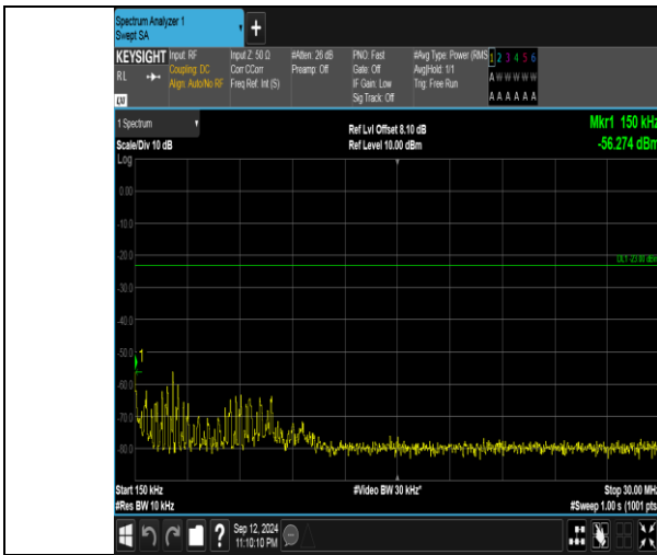
Band5_1.4MHz_16QAM_20643_6RB#0_0.15~30_0.15~30
