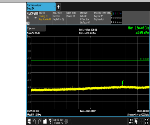
Band5_1.4MHz_QPSK_20643_1RB#5_1000~3000_1000~3000
