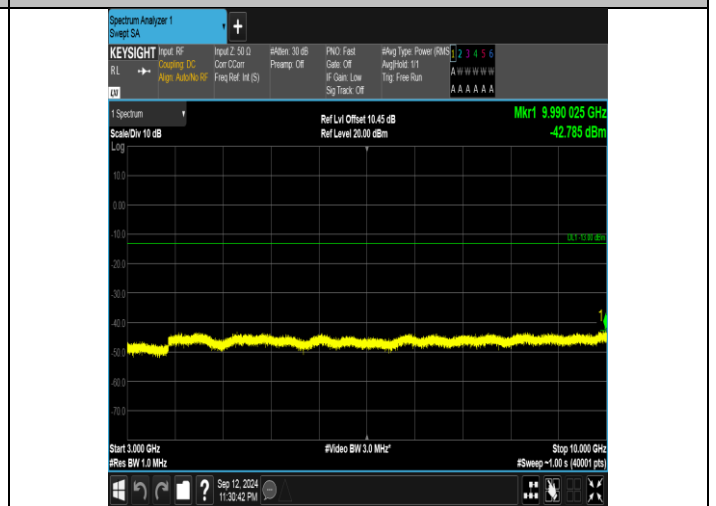
Band5_3MHz_16QAM_20415_15RB#0_3000~10000_3000~10000
