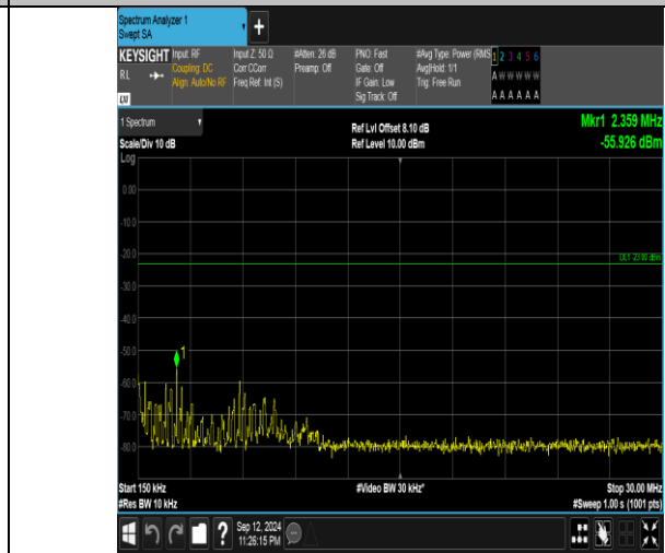
Band5_3MHz_QPSK_20415_1RB#0_0.15~30_0.15~30
