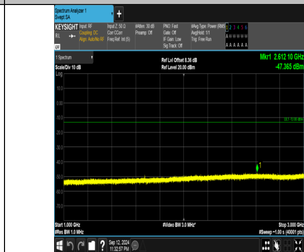
Band5_3MHz_QPSK_20525_1RB#14_1000~3000_1000~3000
