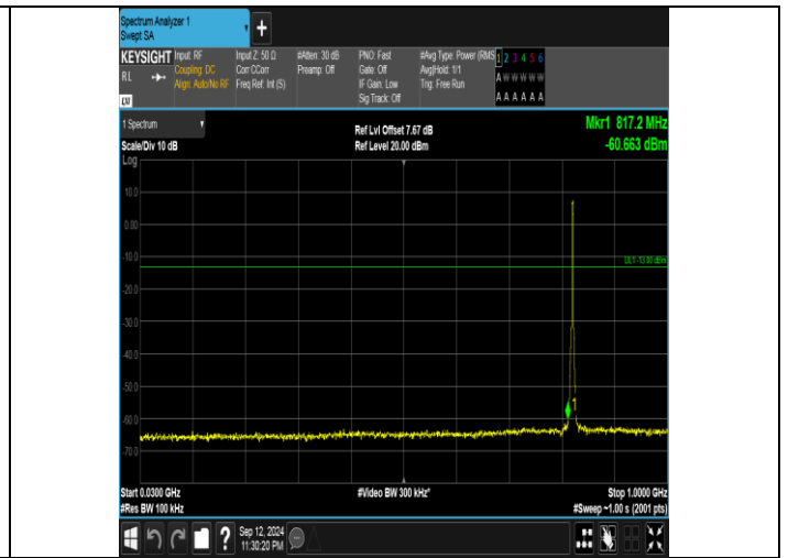
Band5_3MHz_16QAM_20415_15RB#0_30~1000_30~1000
