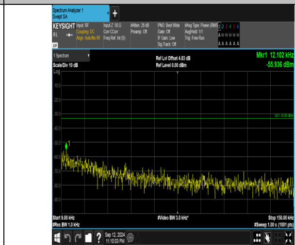
Band5_1.4MHz_16QAM_20643_6RB#0_0.009~0.15_0.009~0.15
