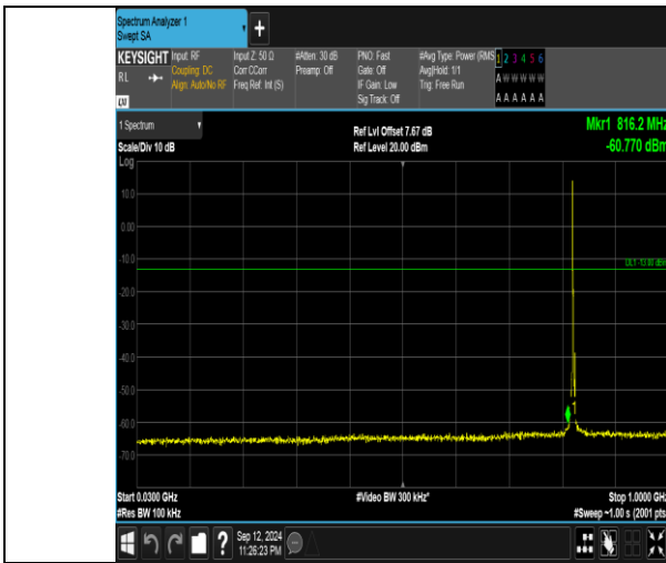
Band5_3MHz_QPSK_20415_1RB#0_30~1000_30~1000
