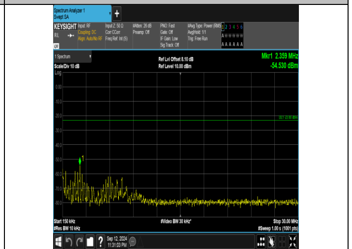
Band5_3MHz_QPSK_20525_1RB#0_0.15~30_0.15~30
