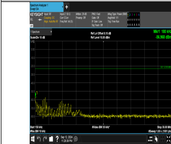
Band5_3MHz_16QAM_20415_1RB#14_0.15~30_0.15~30
