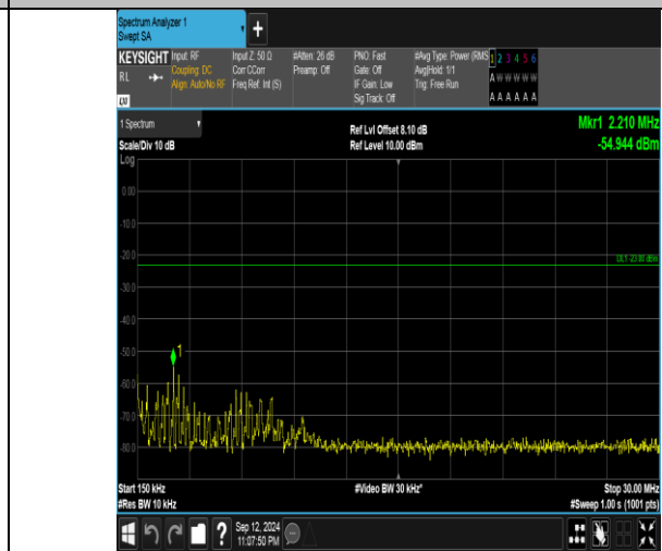
Band5_1.4MHz_QPSK_20643_1RB#5_0.15~30_0.15~30
