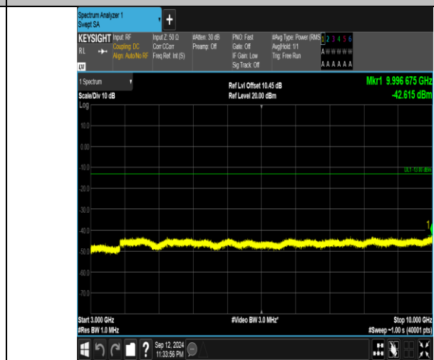
Band5_3MHz_16QAM_20525_1RB#14_3000~10000_3000~10000
