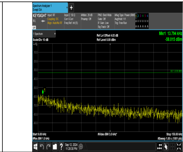
Band5_3MHz_16QAM_20415_1RB#14_0.009~0.15_0.009~0.15
