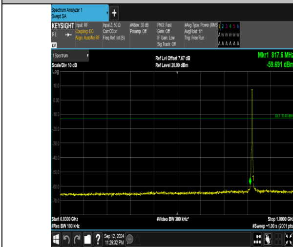
Band5_3MHz_QPSK_20415_15RB#0_30-1000_30-1000
