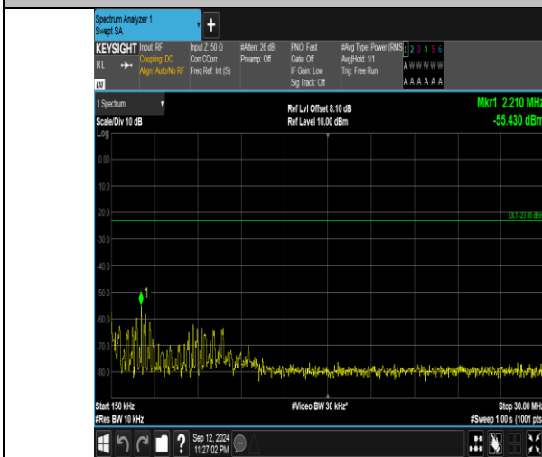
Band5_3MHz_16QAM_20415_1RB#0_0.15~30_0.15~30
