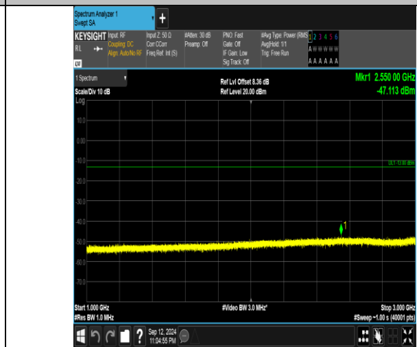
Band5_1.4MHz_QPSK_20525_6RB#0_1000~3000_1000~3000
