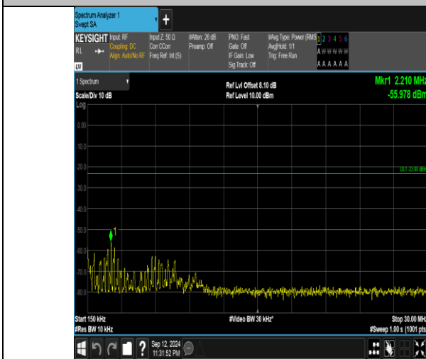
Band5_3MHz_16QAM_20525_1RB#0_0.15~30_0.15~30
