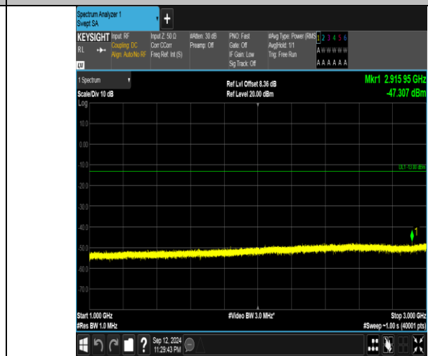
Band5_3MHz_QPSK_20415_15RB#0_1000-3000_1000-3000
