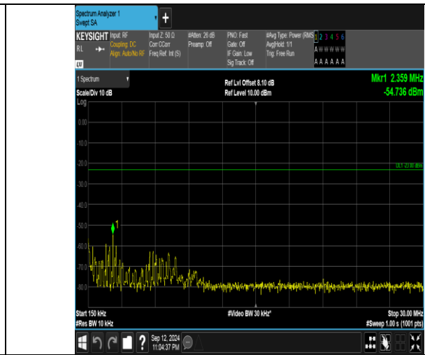
Band5_1.4MHz_QPSK_20525_6RB#0_0.15~30_0.15~30
