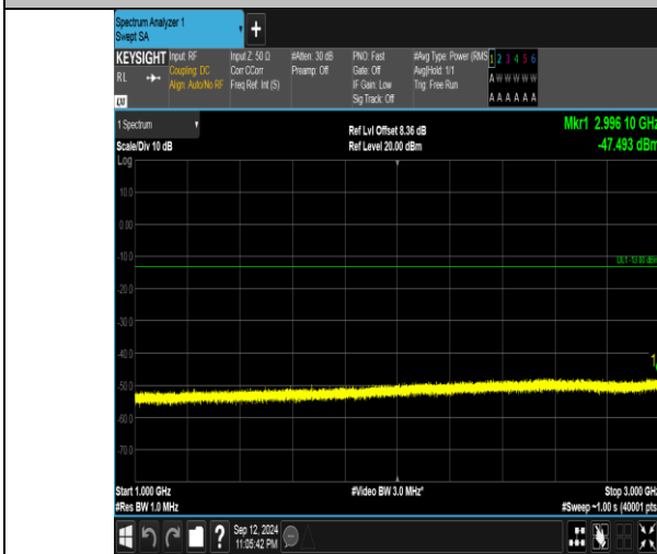
Band5_1.4MHz_16QAM_20525_6RB#0_1000~3000_1000~3000
