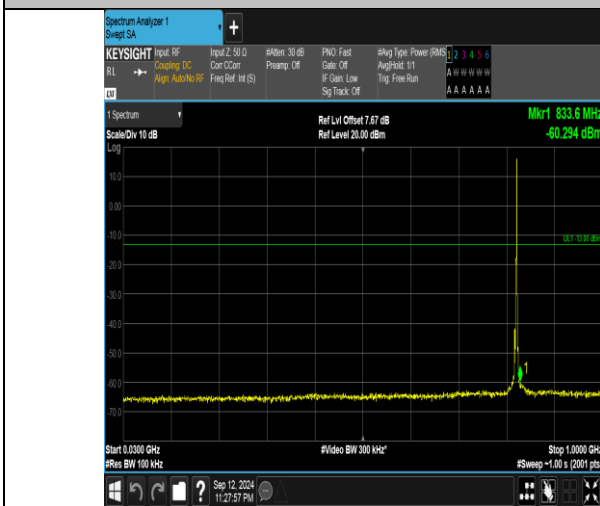
Band5_3MHz_QPSK_20415_1RB#14_30~1000_30~1000
