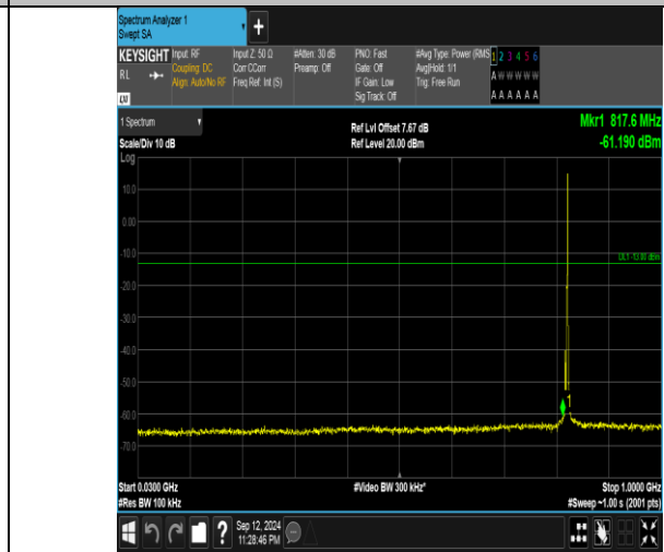
Band5_3MHz_16QAM_20415_1RB#14_30~1000_30~1000
