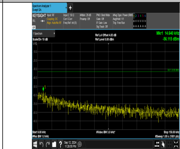
Band5_3MHz_16QAM_20415_1RB#0_0.009~0.15_0.009~0.15
