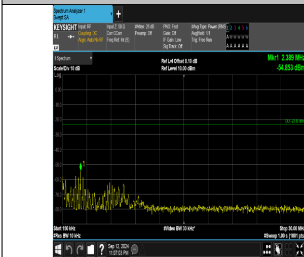
Band5_1.4MHz_16QAM_20643_1RB#0_0.15~30_0.15~30
