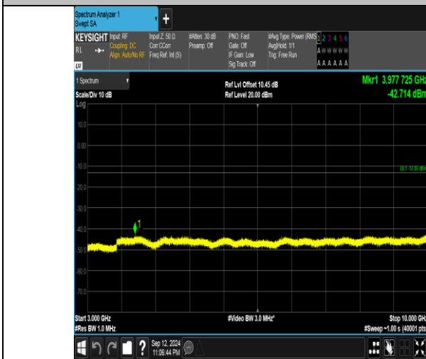
Band5_1.4MHz_QPSK_20643_1RB#0_3000~10000_3000~10000
