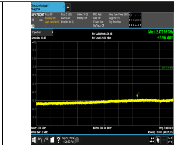
Band5_3MHz_QPSK_20415_1RB#0_1000~3000_1000~3000
