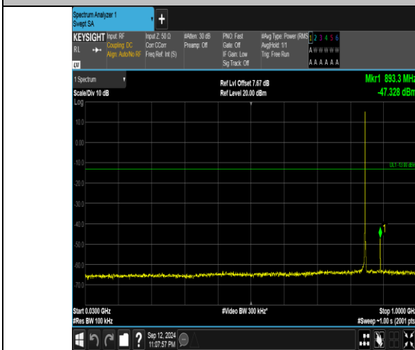
Band5_1.4MHz_QPSK_20643_1RB#5_30~1000_30~1000
