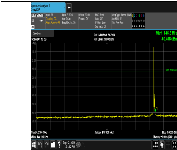
Band5_3MHz_QPSK_20525_1RB#0_30~1000_30~1000
