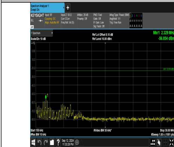
Band5_3MHz_16QAM_20525_1RB#14_0.15~30_0.15~30
