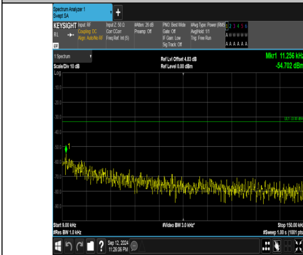
Band5_3MHz_QPSK_20415_1RB#0_0.009~0.15_0.009~0.15
