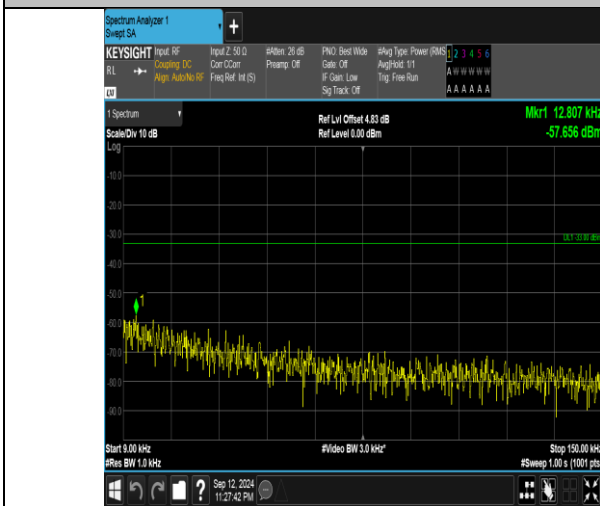
Band5_3MHz_QPSK_20415_1RB#14_0.009~0.15_0.009~0.15
