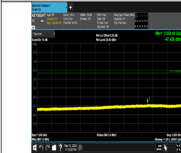
Band5_1.4MHz_16QAM_20643_6RB#0_1000~3000_1000~3000
