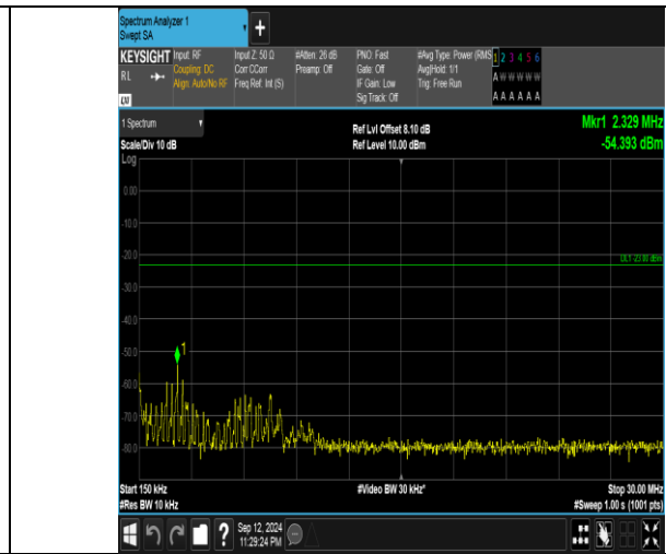
Band5_3MHz_QPSK_20415_15RB#0_0.15-30_0.15-30
