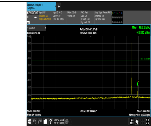
Band5_1.4MHz_16QAM_20643_6RB#0_30~1000_30~1000
