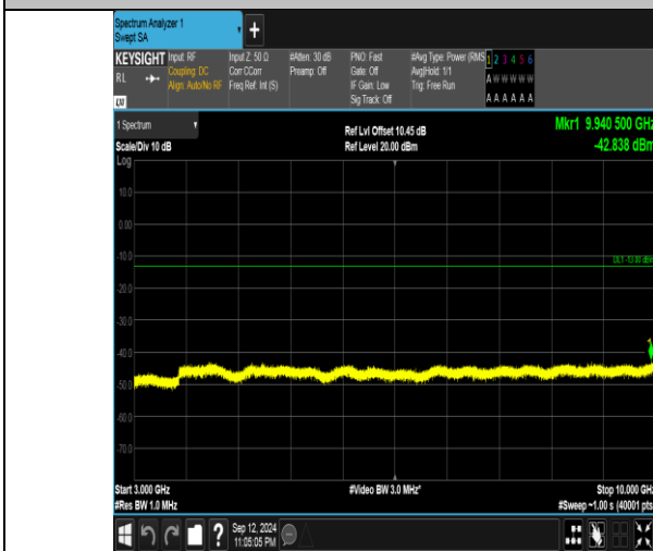
Band5_1.4MHz_QPSK_20525_6RB#0_3000~10000_3000~10000
