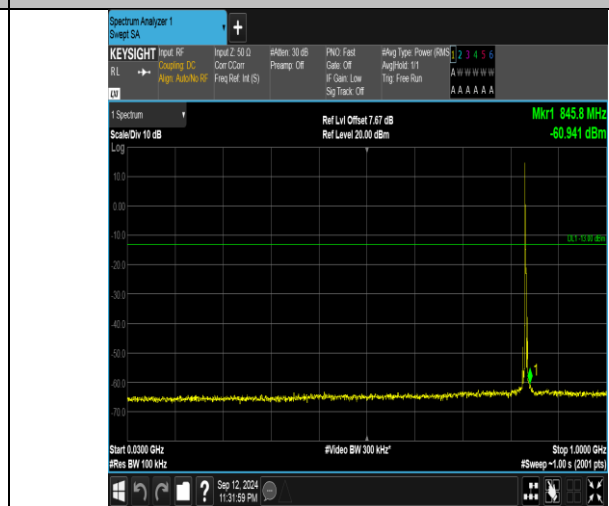
Band5_3MHz_16QAM_20525_1RB#0_30~1000_30~1000
