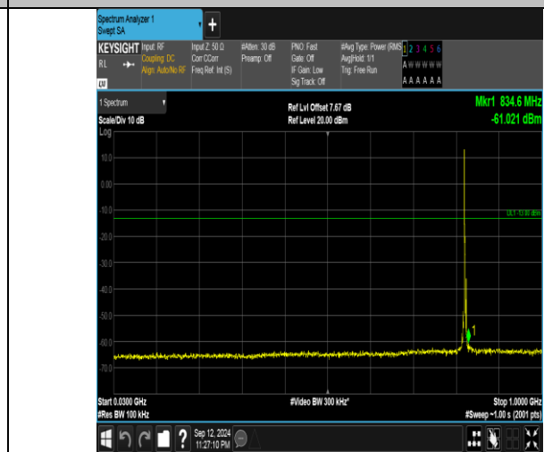
Band5_3MHz_16QAM_20415_1RB#0_30~1000_30~1000
