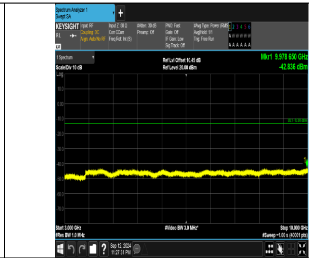
Band5_3MHz_16QAM_20415_1RB#0_3000~10000_3000~10000
