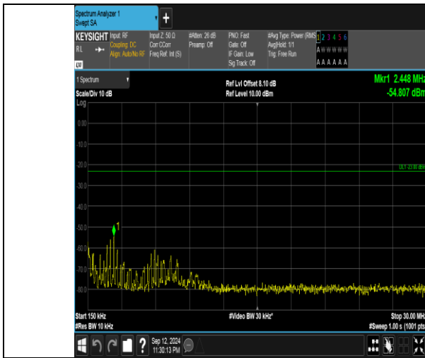
Band5_3MHz_16QAM_20415_15RB#0_0.15~30_0.15~30
