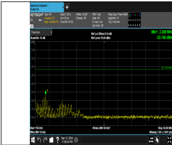
Band5_1.4MHz_16QAM_20525_6RB#0_0.15~30_0.15~30
