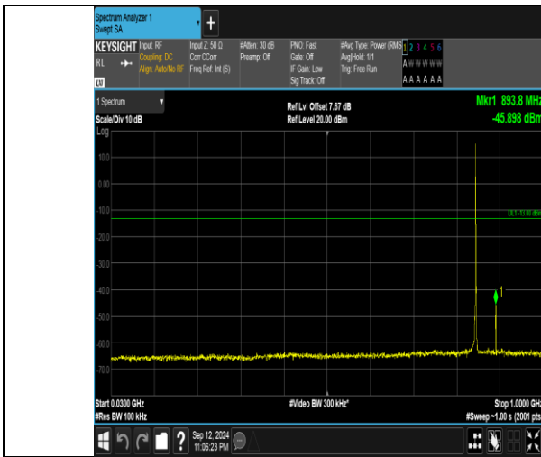
Band5_1.4MHz_QPSK_20643_1RB#0_30~1000_30~1000
