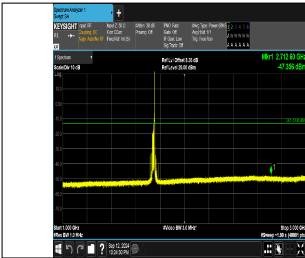
Band4_20MHz_16QAM_20300_1RB#99_1000-3000_1000-3000
