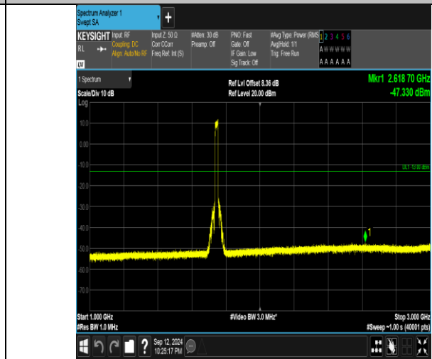
Band4_20MHz_QPSK_20300_100RB#0_1000-3000_1000-3000
