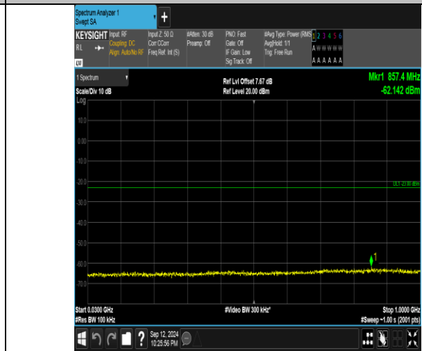
Band4_20MHz_16QAM_20300_100RB#0_30~1000_30~1000
