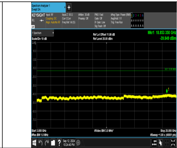
Band4_20MHz_16QAM_20300_1RB#99_3000-20000_3000-20000
