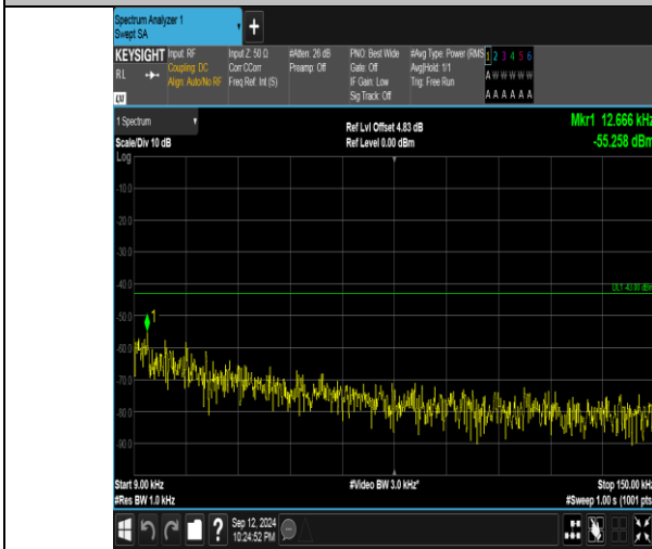
Band4_20MHz_QPSK_20300_100RB#0_0.009-0.15_0.009-0.15
