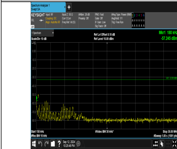
Band4_20MHz_16QAM_20300_100RB#0_0.15~30_0.15~30
