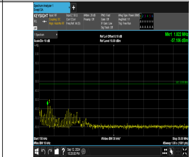
Band4_20MHz_QPSK_20300_100RB#0_0.15-30_0.15-30
