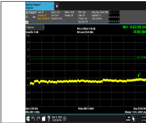
Band4_20MHz_QPSK_20300_100RB#0_3000~20000_3000~20000
