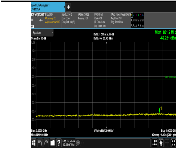
Band4_20MHz_QPSK_20300_100RB#0_30-1000_30-1000
