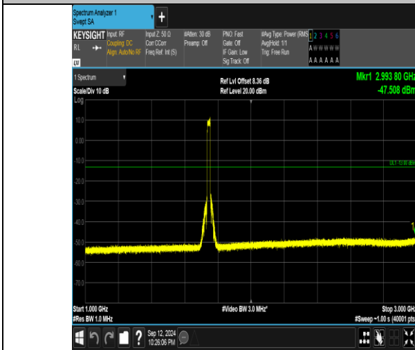
Band4_20MHz_16QAM_20300_100RB#0_1000~3000_1000~3000
