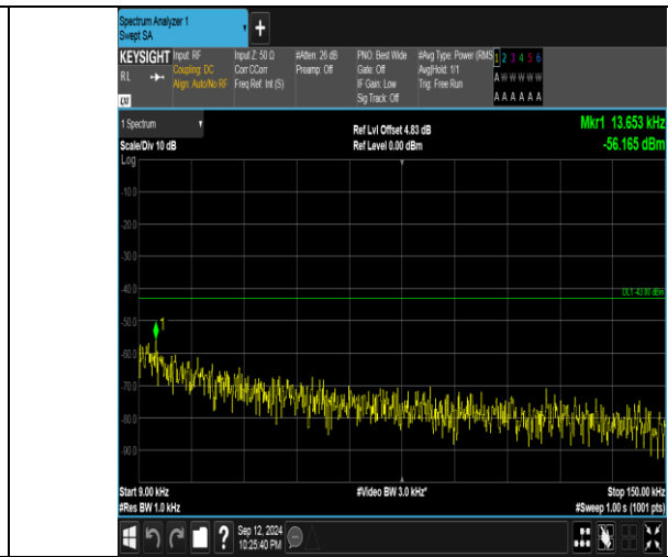
Band4_20MHz_16QAM_20300_100RB#0_0.009~0.15_0.009~0.15
