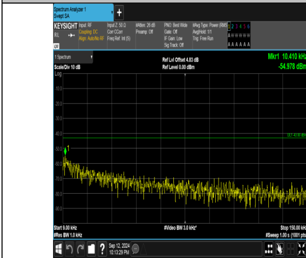
Band4_20MHz_QPSK_20050_1RB#99_0.009~0.15_0.009~0.15
