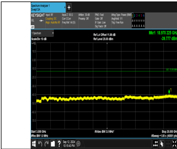
Band4_20MHz_QPSK_20050_100RB#0_3000~20000_3000~20000
