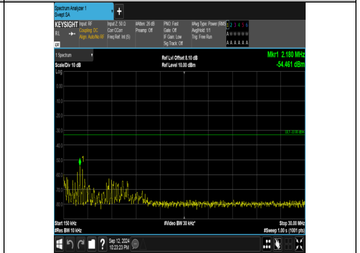
Band4_20MHz_QPSK_20300_1RB#99_0.15~30_0.15~30
