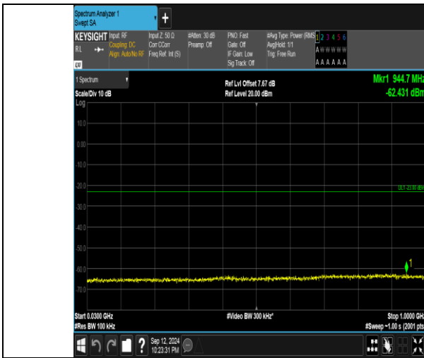
Band4_20MHz_QPSK_20300_1RB#99_30~1000_30~1000
