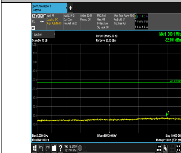
Band4_20MHz_QPSK_20175_1RB#0_30-1000_30-1000
