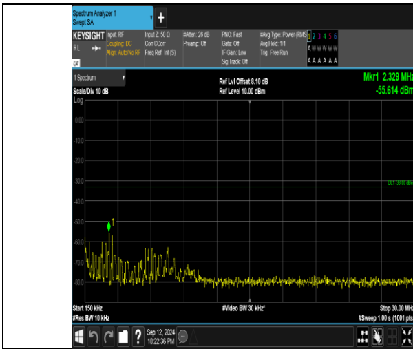
Band4_20MHz_16QAM_20300_1RB#0_0.15~30_0.15~30
