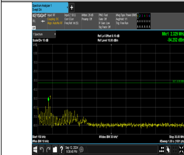
Band4_15MHz_16QAM_20325_75RB#0_0.15~30_0.15~30
