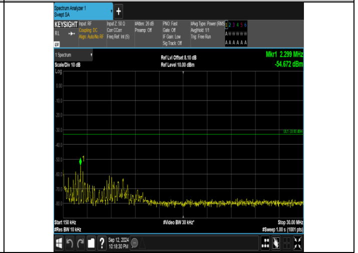
Band4_20MHz_QPSK_20175_1RB#99_0.15~30_0.15~30
