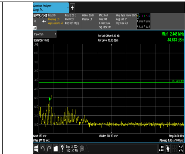
Band4_20MHz_QPSK_20300_1RB#0_0.15-30_0.15-30
