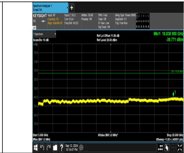
Band4_20MHz_16QAM_20175_1RB#99_3000-20000_3000-20000
