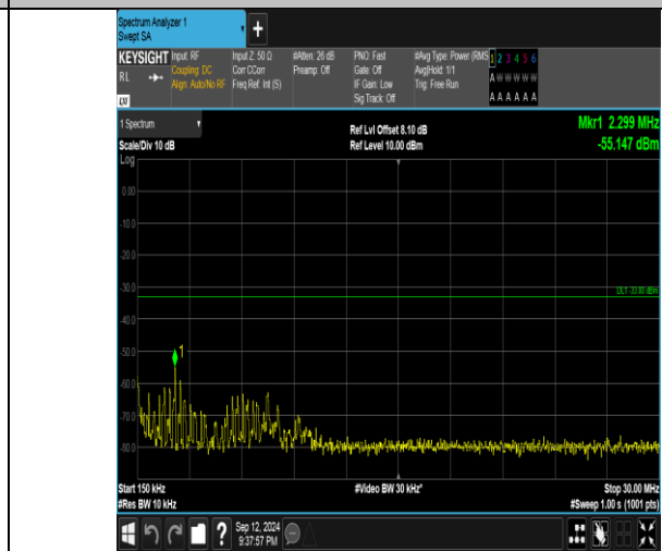
Band4_15MHz_QPSK_20325_75RB#0_0.15-30_0.15-30
