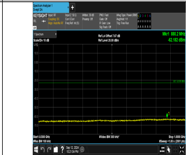
Band4_20MHz_16QAM_20175_100RB#0_30~1000_30~1000
