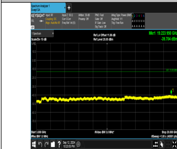
Band4_20MHz_QPSK_20300_1RB#99_3000~20000_3000~20000
