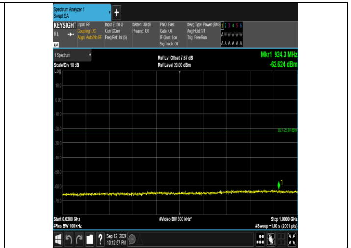
Band4_20MHz_16QAM_20050_1RB#0_30~1000_30~1000
