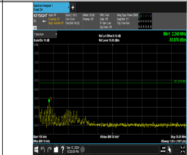
Band4_20MHz_QPSK_20175_100RB#0_0.15-30_0.15-30
