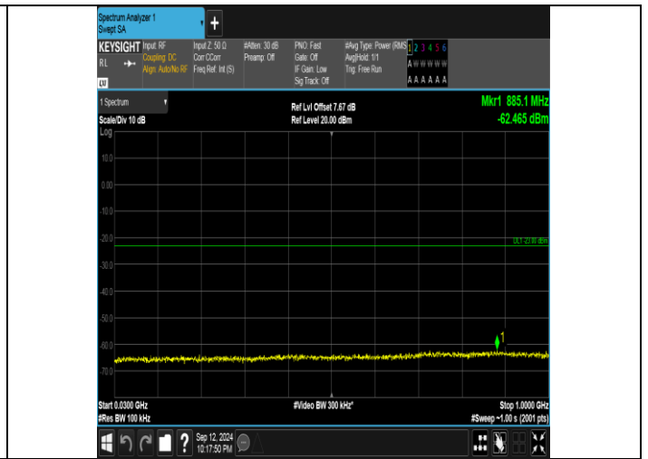
Band4_20MHz_16QAM_20175_1RB#0_30~1000_30~1000
