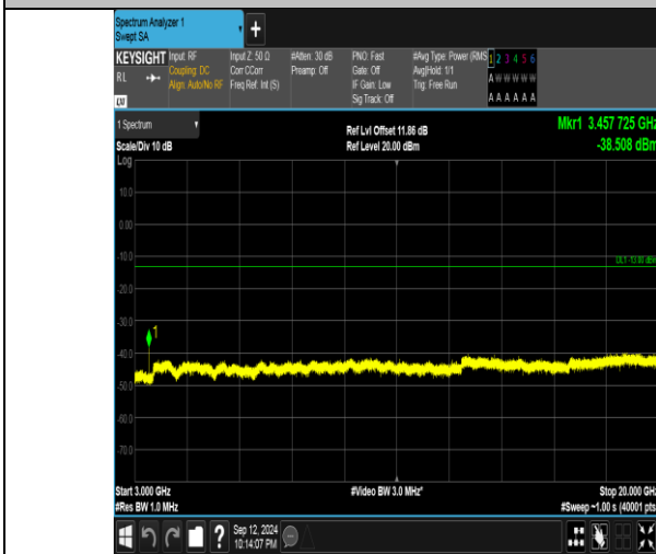
Band4_20MHz_QPSK_20050_1RB#99_3000~20000_3000~20000
