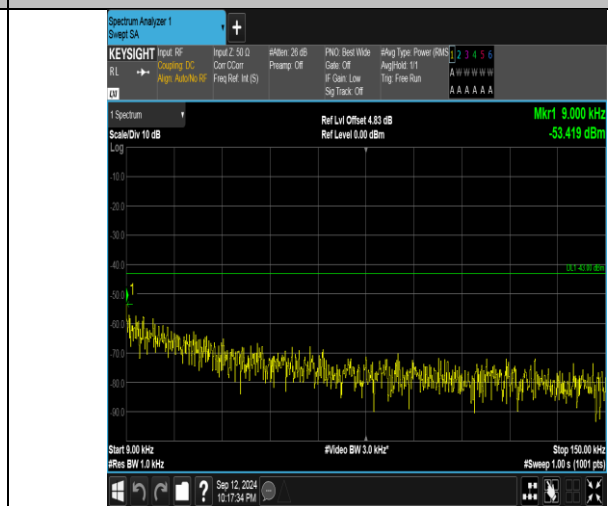
Band4_20MHz_16QAM_20175_1RB#0_0.009-0.15_0.009-0.15
