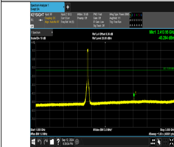
Band4_15MHz_16QAM_20325_75RB#0_1000~3000_1000~3000
