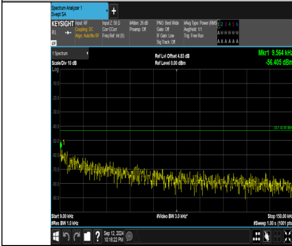
Band4_20MHz_QPSK_20175_1RB#99_0.009~0.15_0.009~0.15
