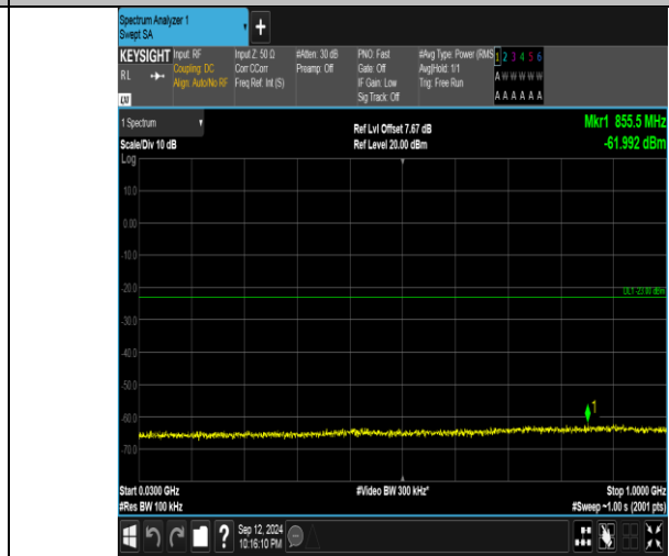
Band4_20MHz_16QAM_20050_100RB#0_30~1000_30~1000
