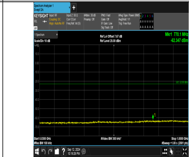
Band4_20MHz_16QAM_20175_1RB#99_30~1000_30~1000
