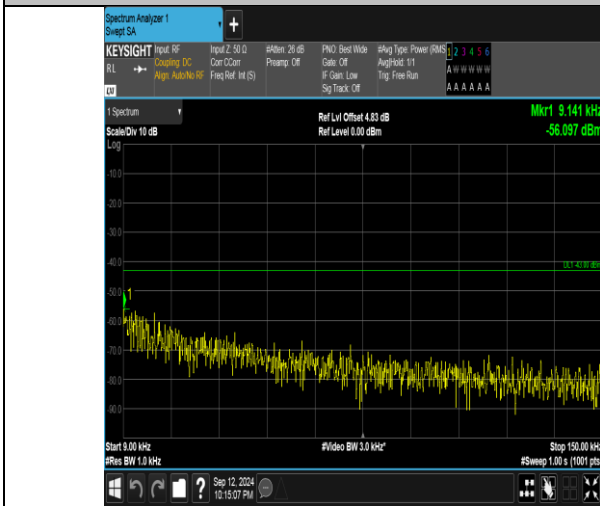
Band4_20MHz_QPSK_2050_100RB#0_0.009-0.15_0.009-0.15
