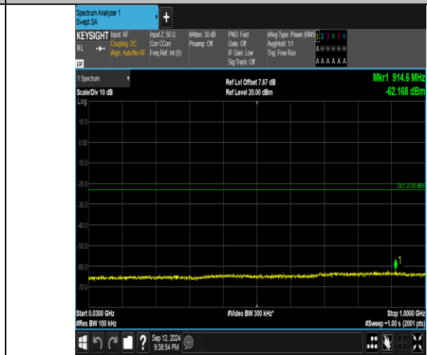
Band4_15MHz_16QAM_20325_75RB#0_30~1000_30~1000
