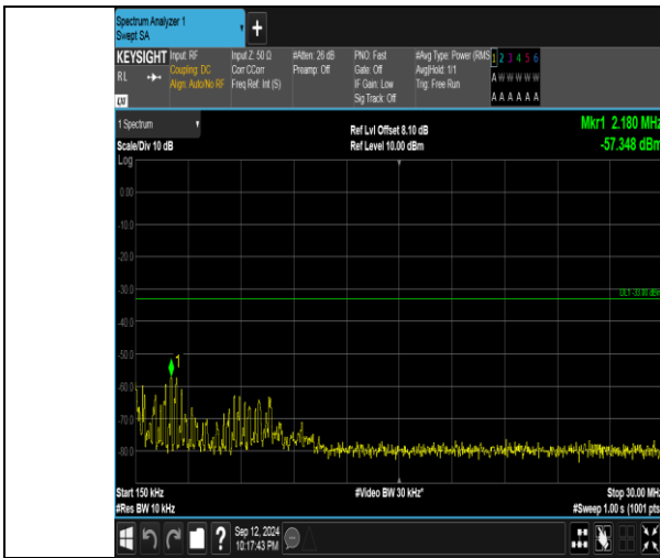
Band4_20MHz_16QAM_20175_1RB#0_0.15~30_0.15~30
