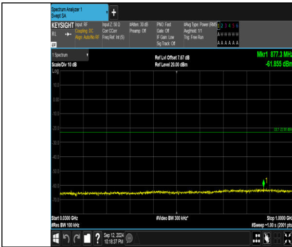
Band4_20MHz_QPSK_20175_1RB#99_30~1000_30~1000
