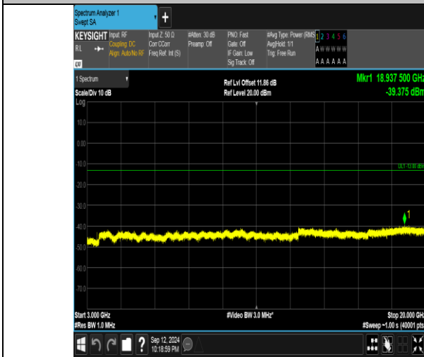
Band4_20MHz_QPSK_20175_1RB#99_3000~20000_3000~20000
