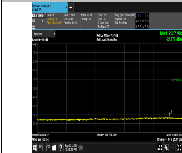
Band4_20MHz_QPSK_2050_100RB#0_30-1000_30-1000
