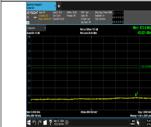
Band4_20MHz_QPSK_20300_1RB#0_30-1000_30-1000
