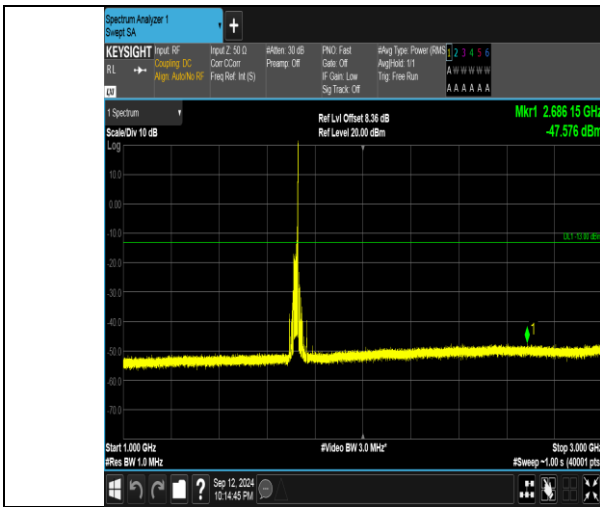
Band4_20MHz_16QAM_2050_1RB#99_1000-3000_1000-3000
