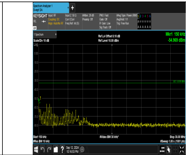
Band4_20MHz_QPSK_20175_1RB#0_0.15-30_0.15-30
