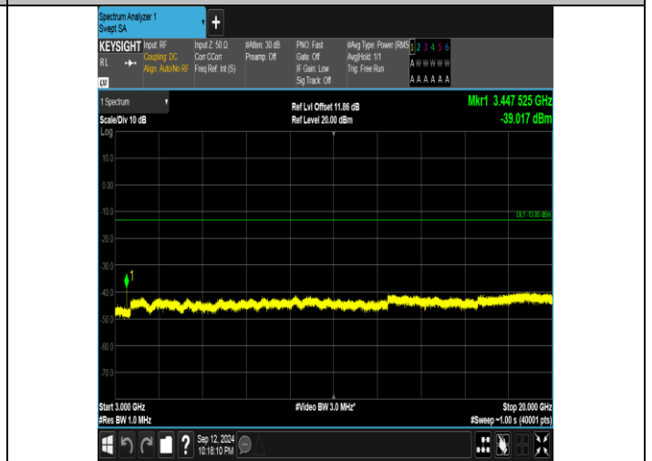
Band4_20MHz_16QAM_20175_1RB#0_3000~20000_3000~20000
