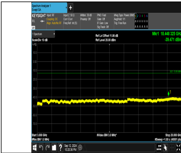
Band4_20MHz_QPSK_20175_100RB#0_3000~20000_3000~20000
