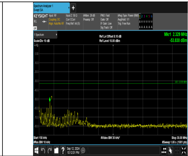
Band4_20MHz_QPSK_20050_1RB#0_0.15-30_0.15-30
