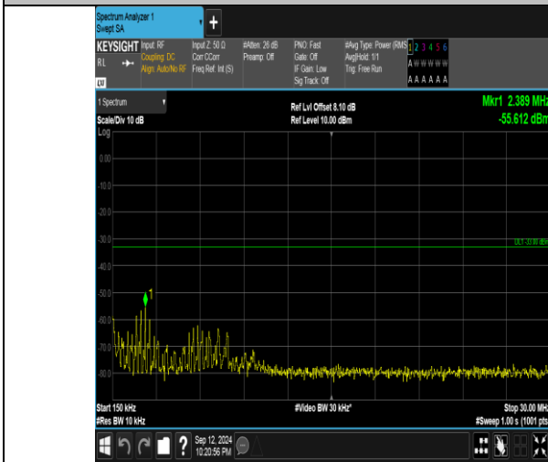
Band4_20MHz_16QAM_20175_100RB#0_0.15~30_0.15~30
