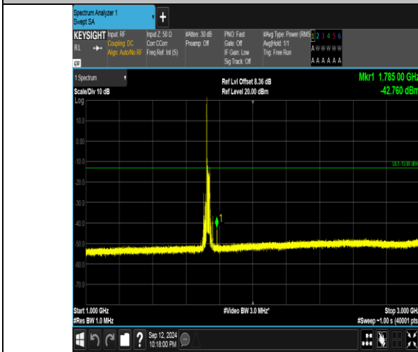
Band4_20MHz_16QAM_20175_1RB#0_1000~3000_1000~3000
