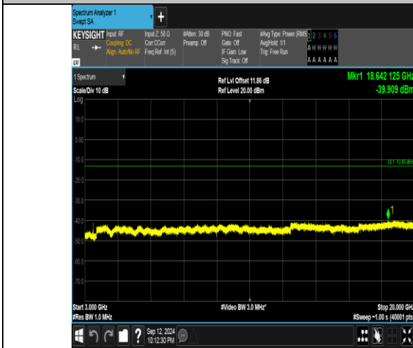
Band4_20MHz_QPSK_20050_1RB#0_3000-20000_3000-20000
