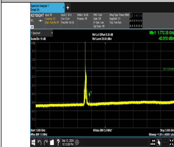
Band4_20MHz_16QAM_20050_1RB#0_1000~3000_1000~3000
