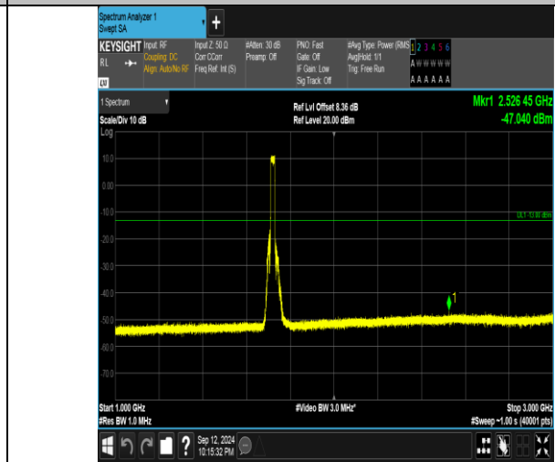
Band4_20MHz_QPSK_2050_100RB#0_1000-3000_1000-3000
