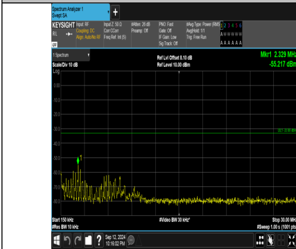
Band4_20MHz_16QAM_20050_100RB#0_0.15~30_0.15~30
