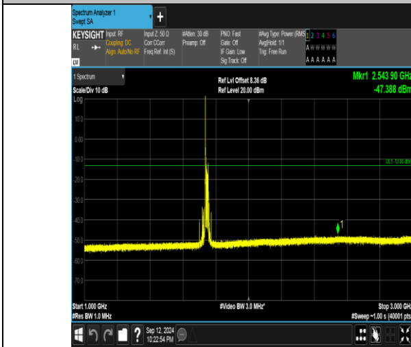
Band4_20MHz_16QAM_20300_1RB#0_1000~3000_1000~3000
