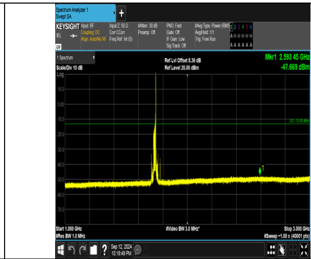
Band4_20MHz_QPSK_20175_1RB#99_1000~3000_1000~3000
