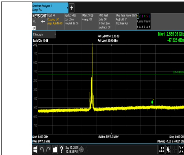
Band4_20MHz_16QAM_20175_1RB#99_1000-3000_1000-3000
