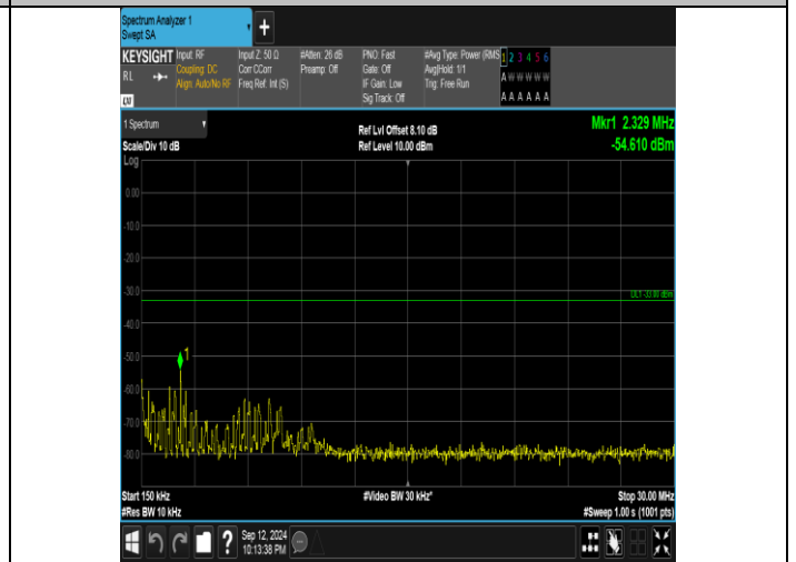
Band4_20MHz_QPSK_20050_1RB#99_0.15~30_0.15~30
