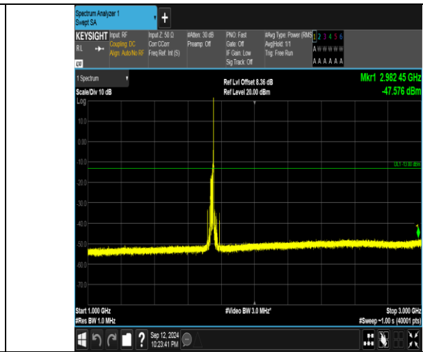
Band4_20MHz_QPSK_20300_1RB#99_1000~3000_1000~3000
