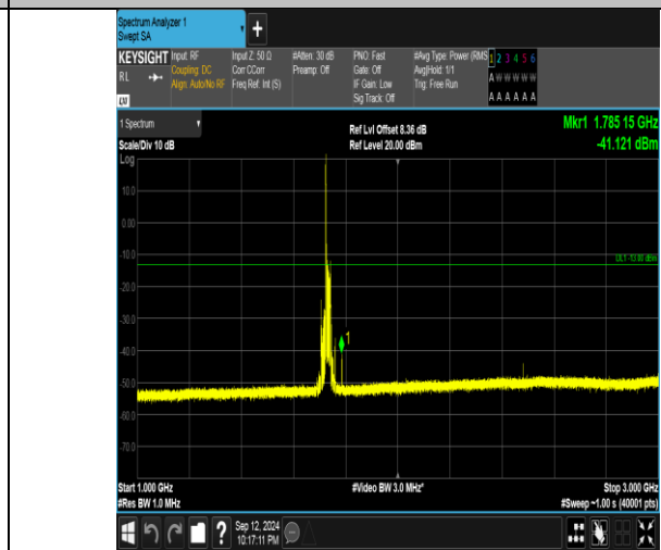
Band4_20MHz_QPSK_20175_1RB#0_1000-3000_1000-3000
