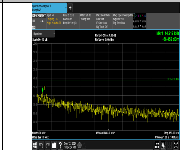
Band4_20MHz_16QAM_20300_1RB#99_0.009~0.15_0.009~0.15
