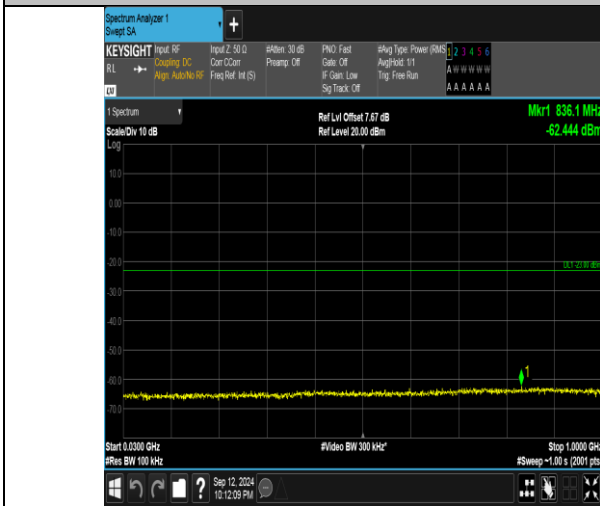
Band4_20MHz_QPSK_20050_1RB#0_30-1000_30-1000
