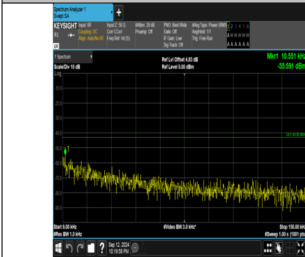
Band4_20MHz_QPSK_20175_100RB#0_0.009-0.15_0.009-0.15
