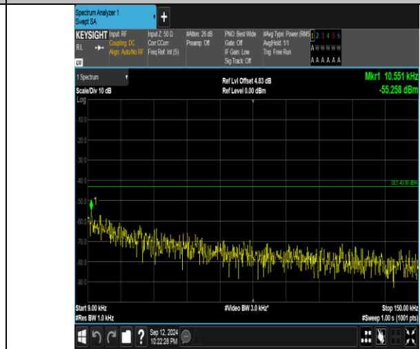
Band4_20MHz_16QAM_20300_1RB#0_0.009-0.15_0.009-0.15
