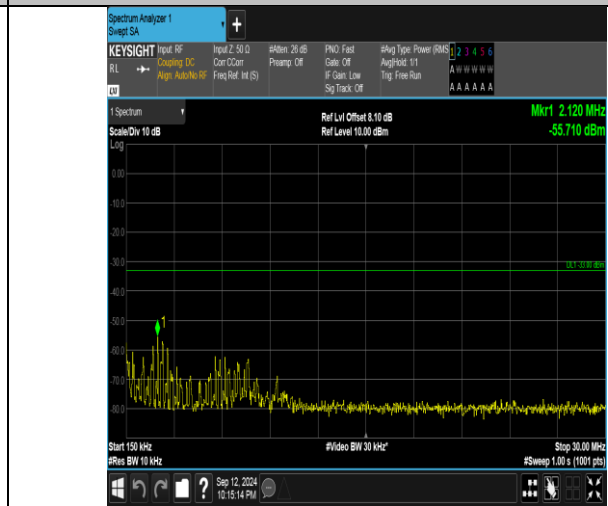
Band4_20MHz_QPSK_2050_100RB#0_0.15-30_0.15-30
