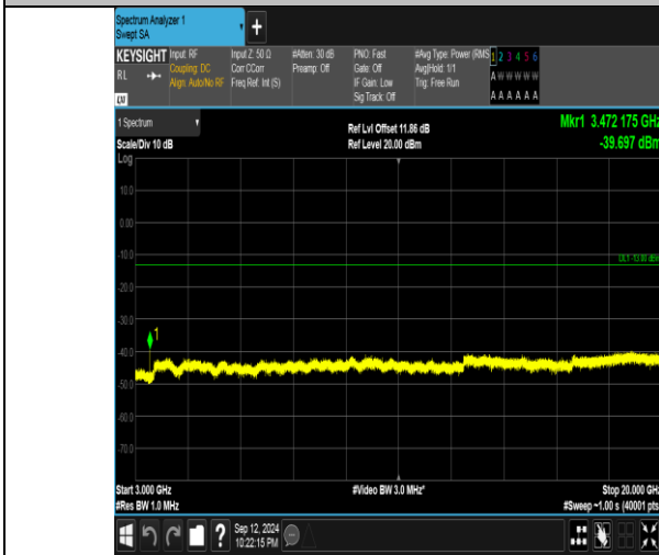
Band4_20MHz_QPSK_20300_1RB#0_3000-20000_3000-20000
