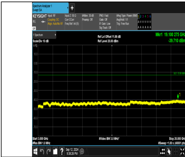
Band4_15MHz_QPSK_20325_75RB#0_3000~20000_3000~20000
