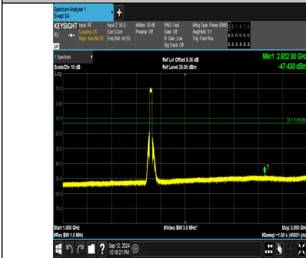
Band4_20MHz_16QAM_20050_100RB#0_1000~3000_1000~3000
