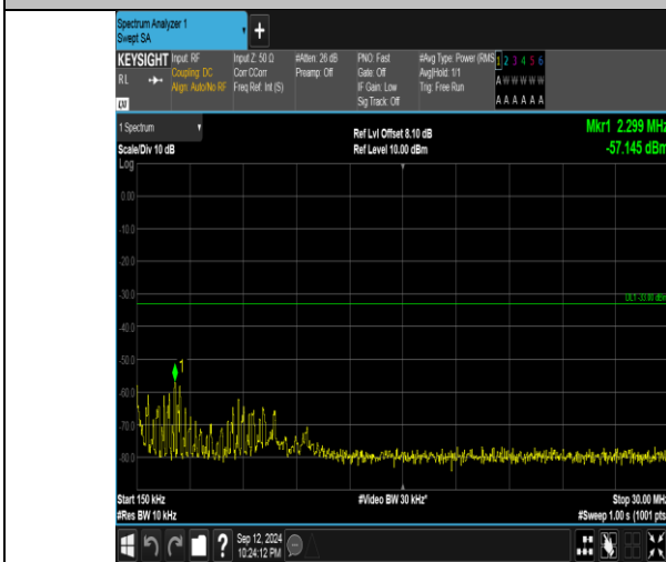
Band4_20MHz_16QAM_20300_1RB#99_0.15~30_0.15~30
