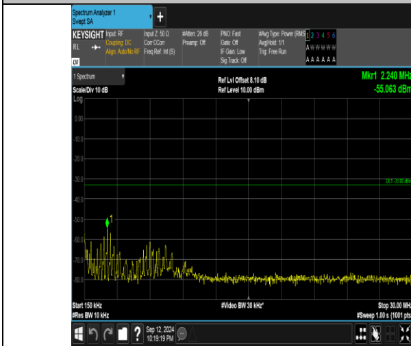
Band4_20MHz_16QAM_20175_1RB#99_0.15~30_0.15~30
