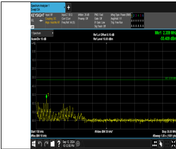
Band4_20MHz_16QAM_20050_1RB#0_0.15~30_0.15~30
