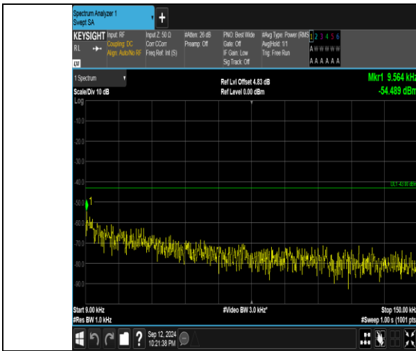
Band4_20MHz_QPSK_20300_1RB#0_0.009-0.15_0.009-0.15
