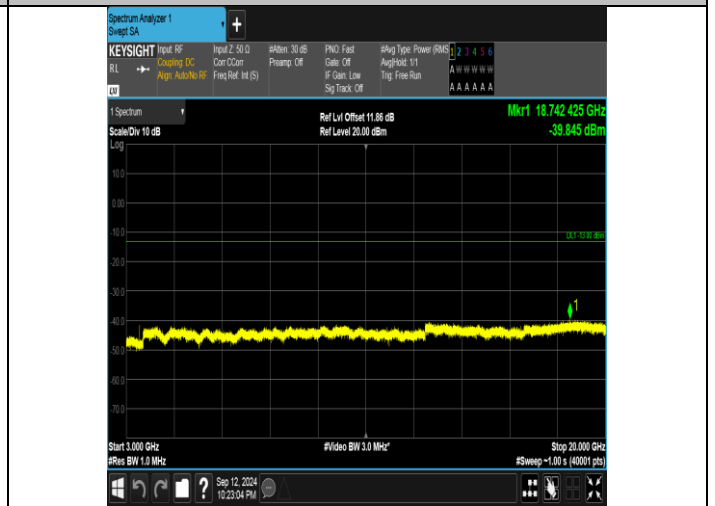
Band4_20MHz_16QAM_20300_1RB#0_3000~20000_3000~20000
