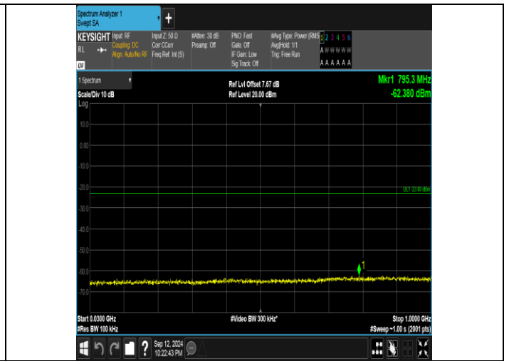
Band4_20MHz_16QAM_20300_1RB#0_30~1000_30~1000
