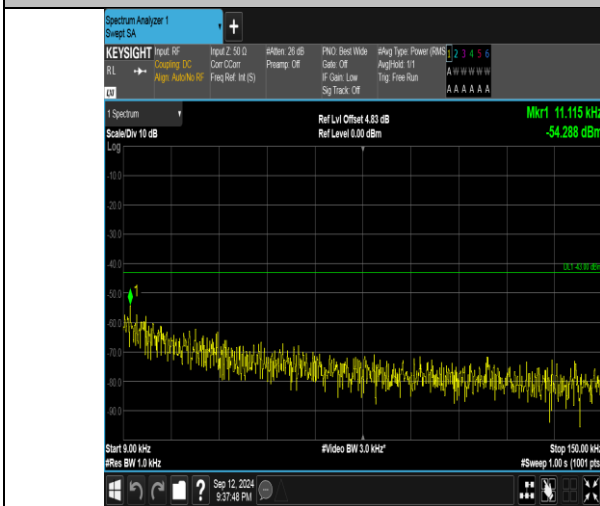
Band4_15MHz_QPSK_20325_75RB#0_0.009-0.15_0.009-0.15
