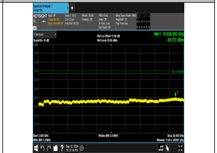
Band4_20MHz_16QAM_20050_1RB#0_3000~20000_3000~20000
