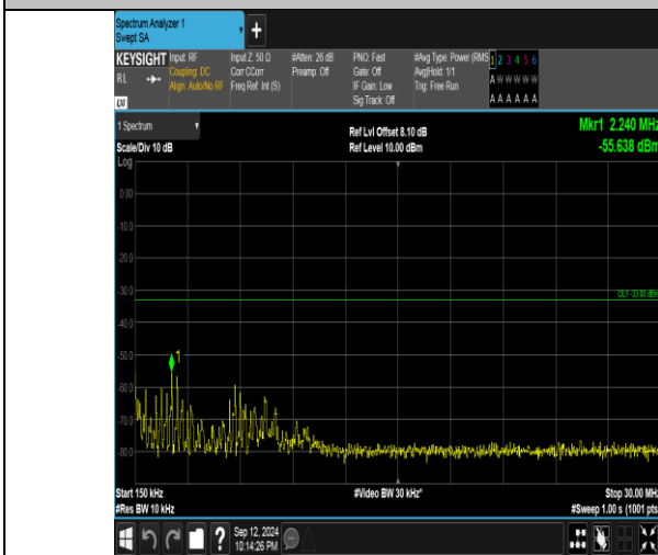
Band4_20MHz_16QAM_20050_1RB#99_0.15~30_0.15~30
