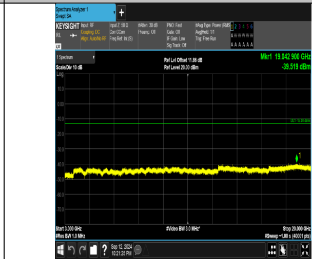
Band4_20MHz_16QAM_20175_100RB#0_3000~20000_3000~20000
