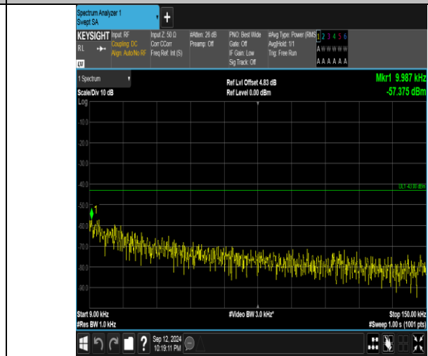
Band4_20MHz_16QAM_20175_1RB#99_0.009~0.15_0.009~0.15
