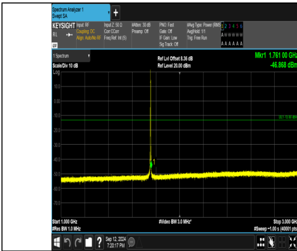
Band4_3MHz_16QAM_20385_1RB#14_1000-3000_1000-3000
