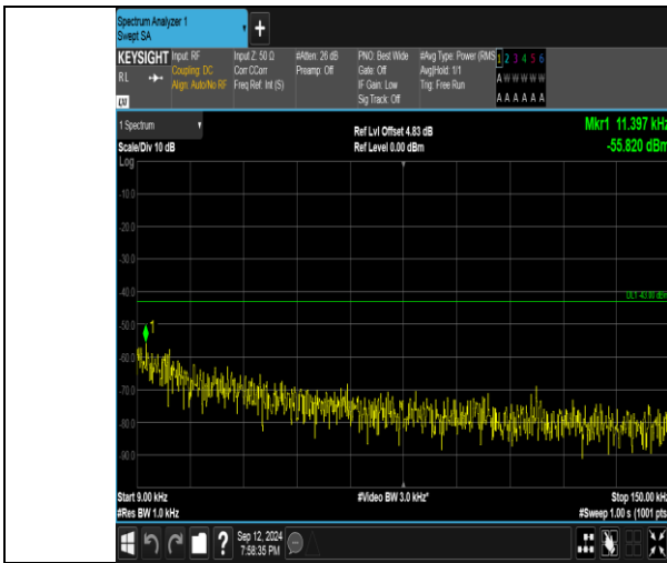
Band4_5MHz_QPSK_20175_1RB#0_0.009~0.15_0.009~0.15
