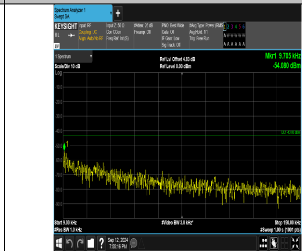
Band4_5MHz_16QAM_19975_1RB#24_0.009~0.15_0.009~0.15
