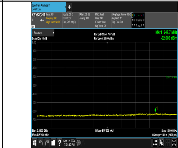
Band4_3MHz_16QAM_20385_15RB#0_30~1000_30~1000
