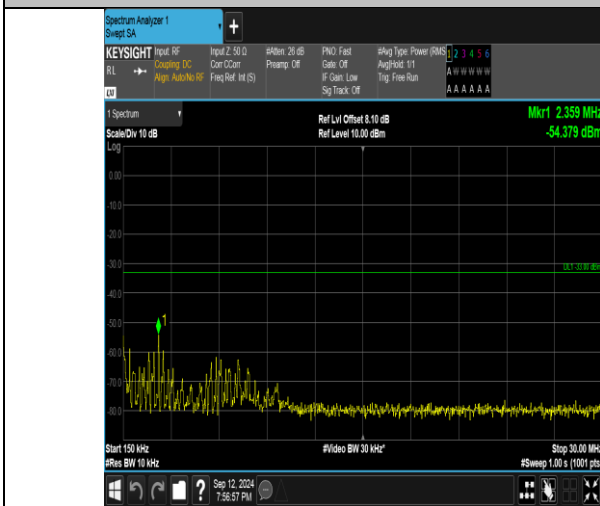
Band4_5MHz_16QAM_19975_25RB#0_0.15~30_0.15~30
