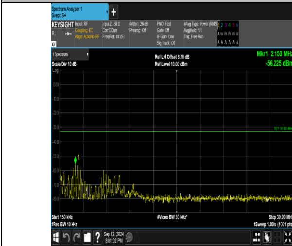
Band4_5MHz_16QAM_20175_1RB#24_0.15~30_0.15~30
