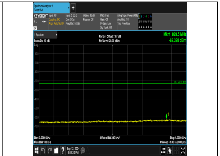
Band4_5MHz_16QAM_20375_1RB#0_30~1000_30~1000
