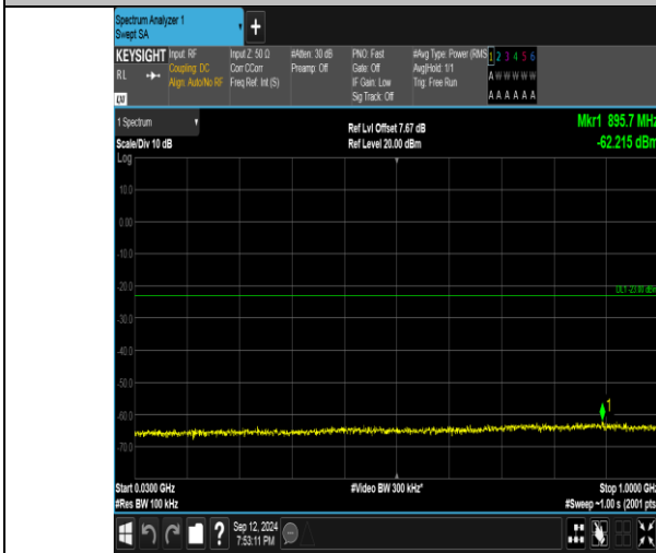
Band4_5MHz_QPSK_19975_1RB#0_30~1000_30~1000
