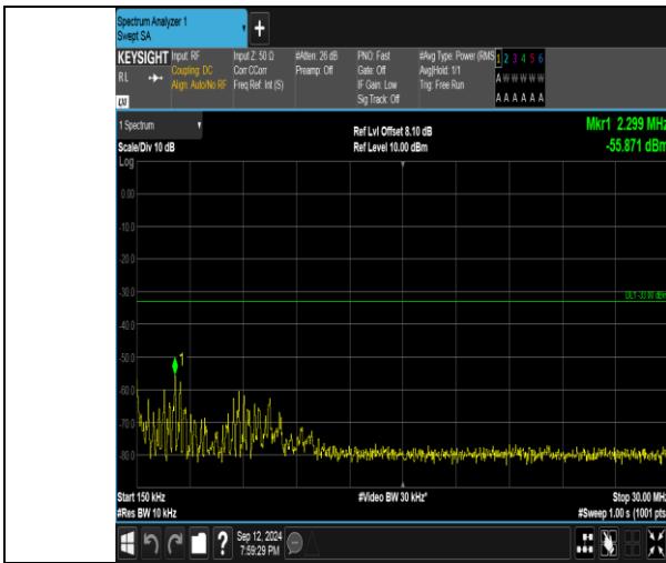
Band4_5MHz_16QAM_20175_1RB#0_0.15~30_0.15~30
