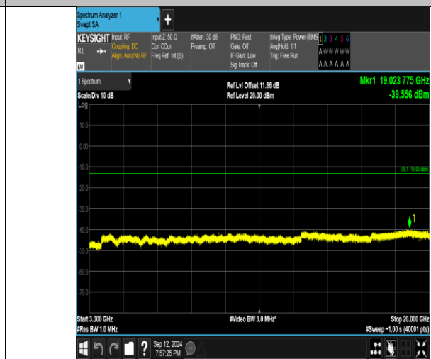
Band4_5MHz_16QAM_19975_25RB#0_3000~20000_3000~20000
