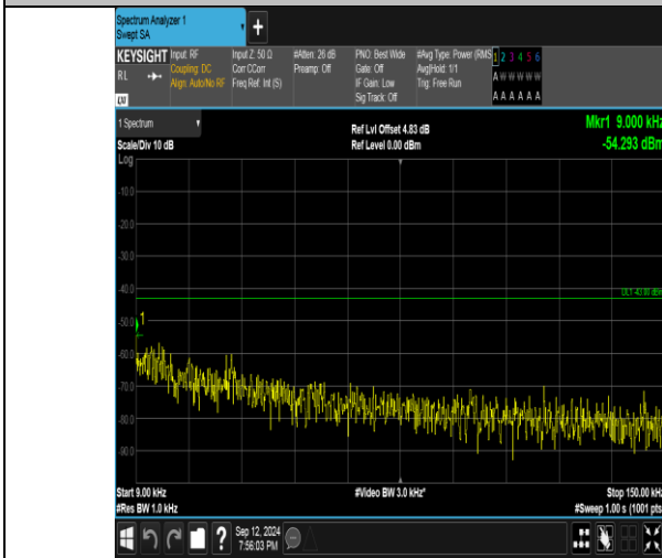
Band4_5MHz_QPSK_19975_25RB#0_0.009-0.15_0.009-0.15
