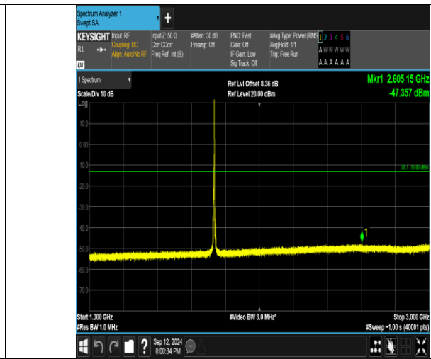
Band4_5MHz_QPSK_20175_1RB#24_1000~3000_1000~3000
