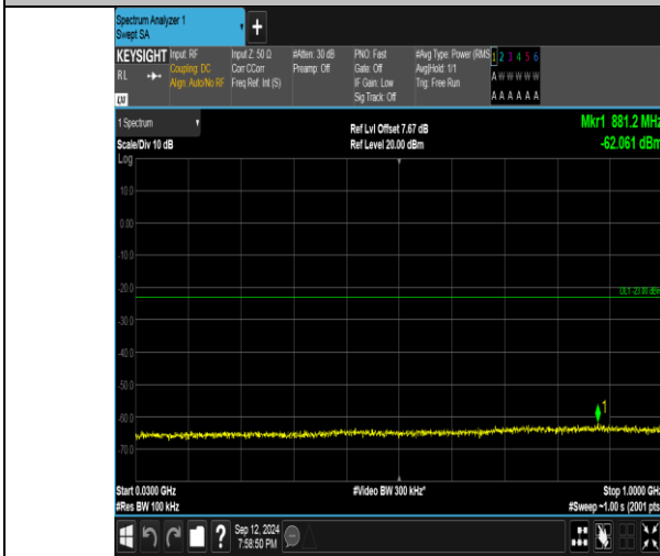
Band4_5MHz_QPSK_20175_1RB#0_30~1000_30~1000
