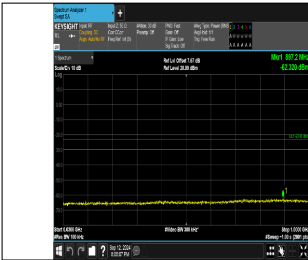
Band4_5MHz_QPSK_20375_1RB#24_30~1000_30~1000
