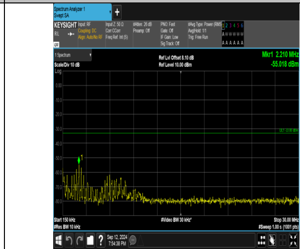
Band4_5MHz_QPSK_19975_1RB#24_0.15-30_0.15-30
