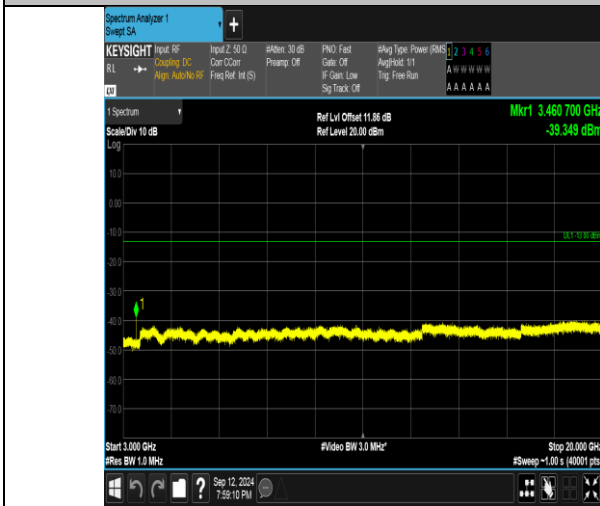
Band4_5MHz_QPSK_20175_1RB#0_3000~20000_3000~20000
