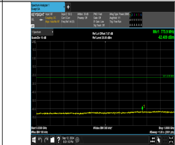
Band4_5MHz_16QAM_20175_1RB#24_30~1000_30~1000
