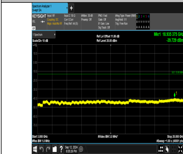
Band4_5MHz_QPSK_20375_1RB#24_3000~20000_3000~20000
