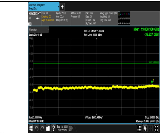
Band4_3MHz_16QAM_20385_1RB#14_3000-20000_3000-20000
