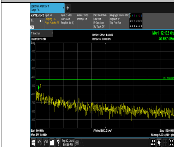
Band4_5MHz_QPSK_20375_1RB#24_0.009~0.15_0.009~0.15
