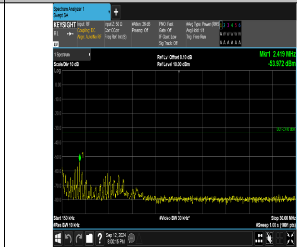
Band4_5MHz_QPSK_20175_1RB#24_0.15~30_0.15~30
