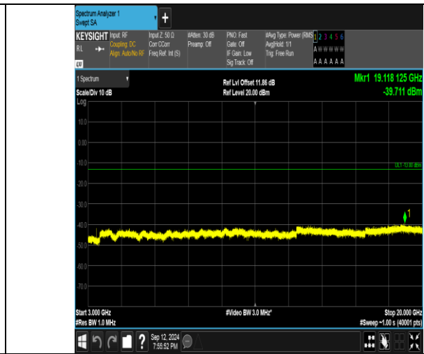
Band4_5MHz_16QAM_19975_1RB#24_3000-20000_3000-20000
