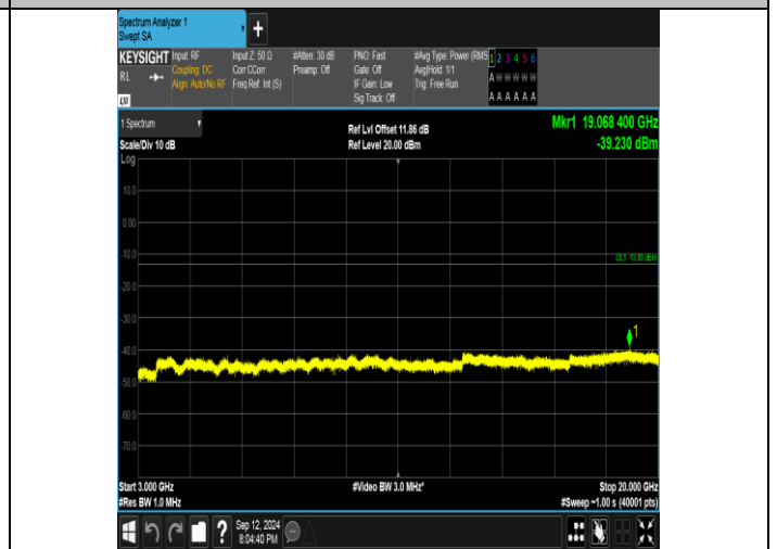
Band4_5MHz_16QAM_20375_1RB#0_3000~20000_3000~20000
