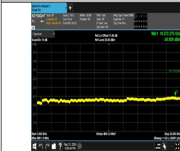
Band4_5MHz_QPSK_20175_1RB#24_3000~20000_3000~20000
