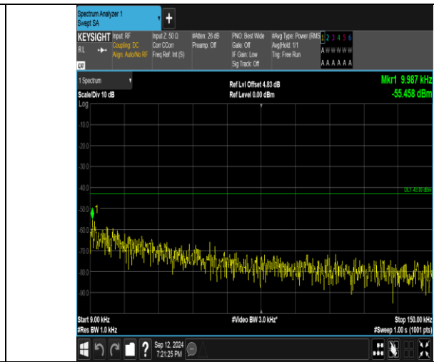
Band4_3MHz_16QAM_20385_15RB#0_0.009~0.15_0.009~0.15
