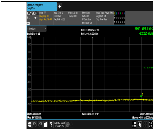
Band4_5MHz_QPSK_19975_1RB#24_30~1000_30~1000
