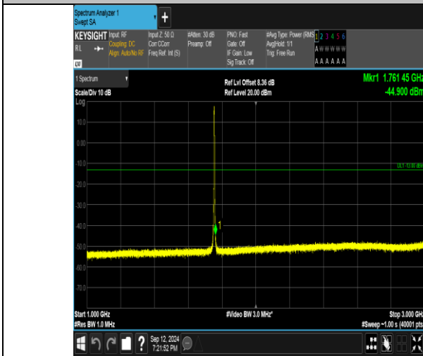
Band4_3MHz_16QAM_20385_15RB#0_1000~3000_1000~3000
