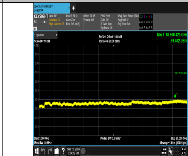
Band4_5MHz_16QAM_19975_1RB#0_3000-20000_3000-20000
