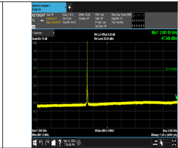
Band4_5MHz_QPSK_19975_1RB#24_1000~3000_1000~3000
