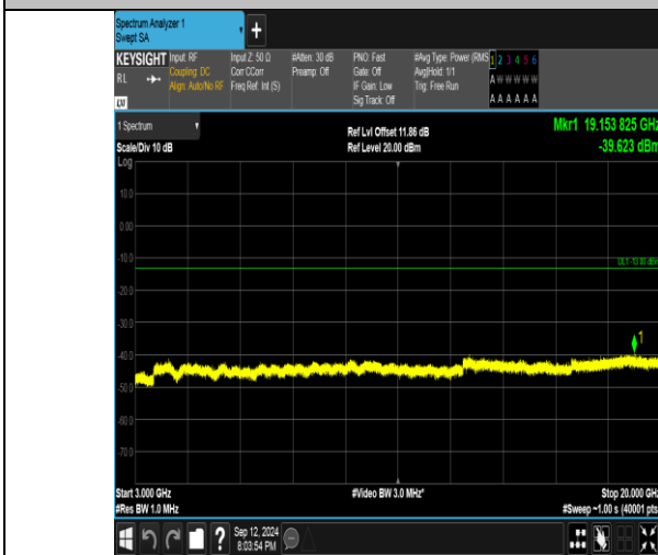
Band4_5MHz_QPSK_20375_1RB#0_3000~20000_3000~20000
