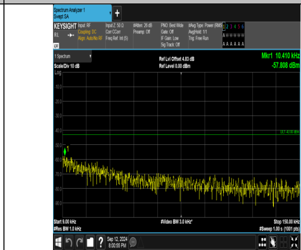
Band4_5MHz_16QAM_20175_1RB#24_0.009~0.15_0.009~0.15
