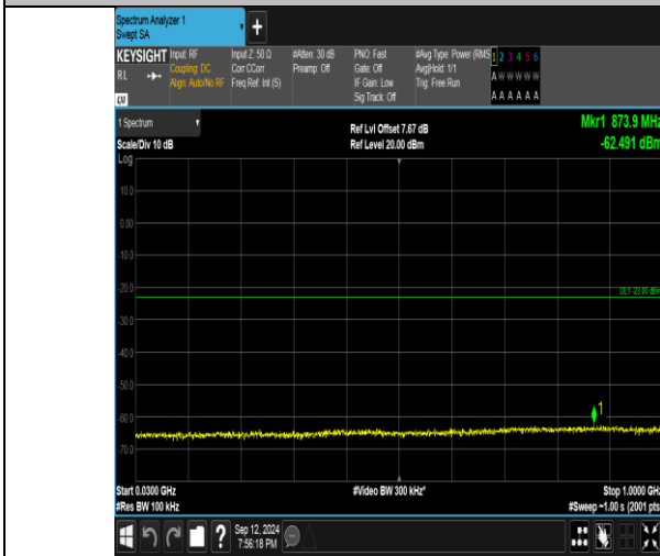
Band4_5MHz_QPSK_19975_25RB#0_30-1000_30-1000
