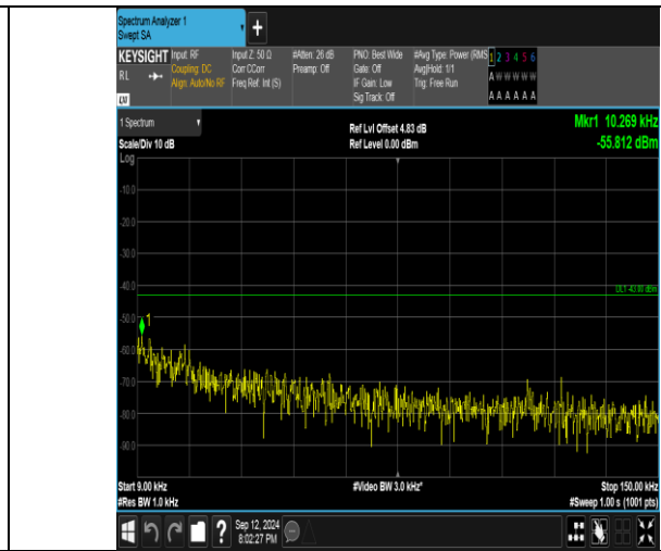
Band4_5MHz_16QAM_20175_25RB#0_0.009-0.15_0.009-0.15
