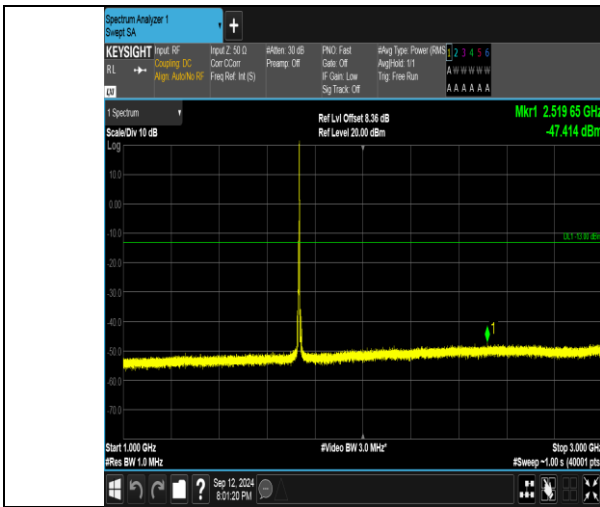
Band4_5MHz_16QAM_20175_1RB#24_1000-3000_1000-3000
