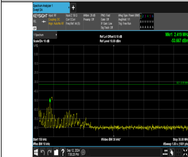
Band4_5MHz_16QAM_19975_1RB#24_0.15~30_0.15~30
