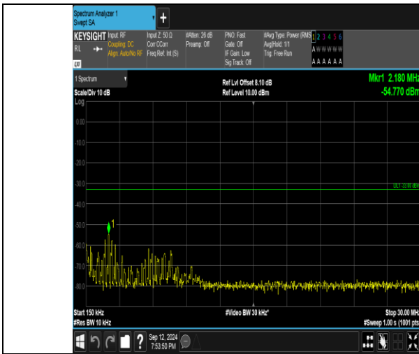
Band4_5MHz_16QAM_19975_1RB#0_0.15-30_0.15-30
