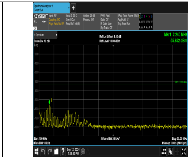
Band4_5MHz_QPSK_20175_1RB#0_0.15~30_0.15~30
