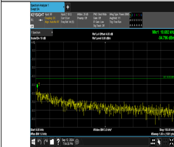
Band4_5MHz_QPSK_19975_1RB#24_0.009-0.15_0.009-0.15
