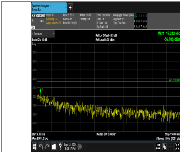
Band4_5MHz_QPSK_20375_1RB#0_0.009~0.15_0.009~0.15
