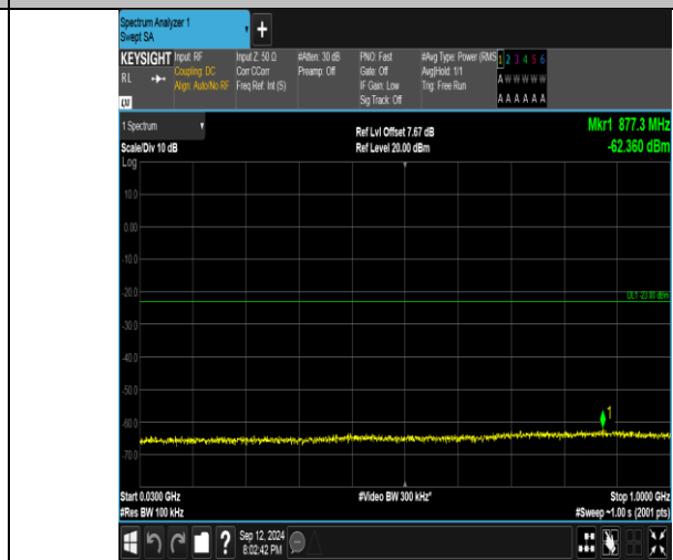
Band4_5MHz_16QAM_20175_25RB#0_30-1000_30-1000
