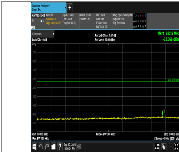
Band4_5MHz_QPSK_20175_1RB#24_30~1000_30~1000
