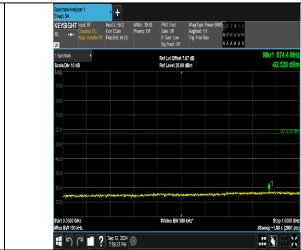
Band4_5MHz_16QAM_20175_1RB#0_30~1000_30~1000
