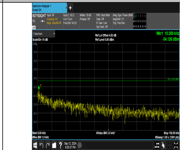
Band4_5MHz_16QAM_20375_1RB#24_0.009~0.15_0.009~0.15
