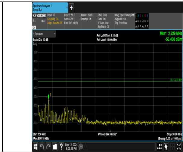
Band4_5MHz_QPSK_20375_1RB#0_0.15~30_0.15~30
