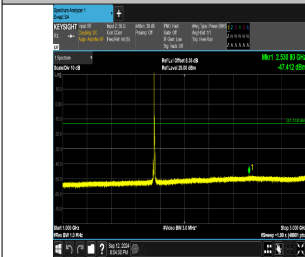
Band4_5MHz_16QAM_20375_1RB#0_1000~3000_1000~3000
