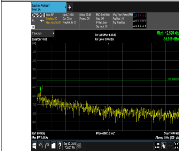
Band4_3MHz_QPSK_20385_15RB#0_0.009-0.15_0.009-0.15
