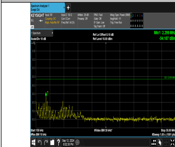
Band4_5MHz_16QAM_20175_25RB#0_0.15-30_0.15-30
