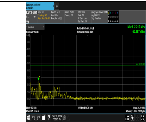
Band4_5MHz_QPSK_19975_1RB#0_0.15~30_0.15~30
