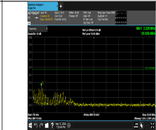
Band4_3MHz_QPSK_20385_15RB#0_0.15-30_0.15-30
