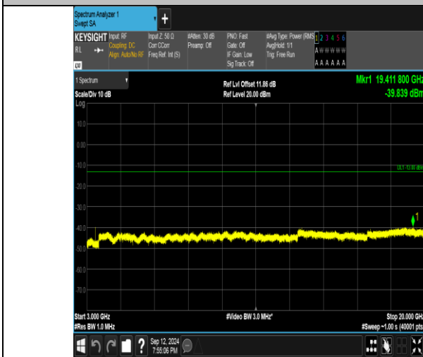
Band4_5MHz_QPSK_19975_1RB#24_3000~20000_3000~20000
