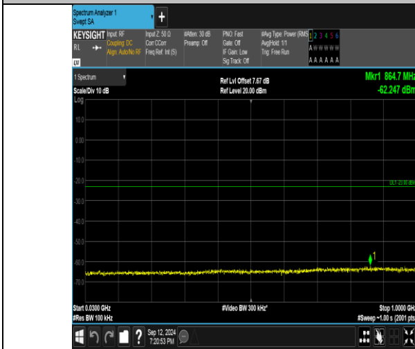
Band4_3MHz_QPSK_20385_15RB#0_30-1000_30-1000
