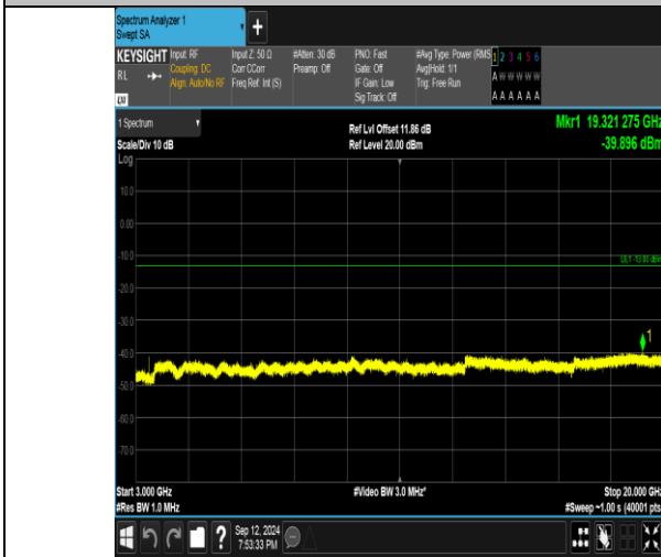
Band4_5MHz_QPSK_19975_1RB#0_3000~20000_3000~20000
