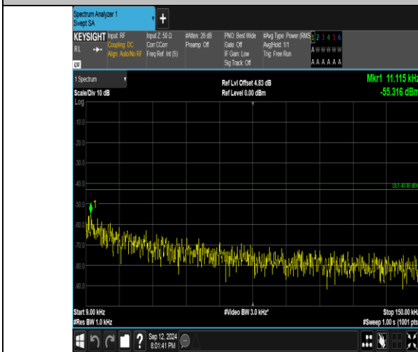
Band4_5MHz_QPSK_20175_25RB#0_0.009-0.15_0.009-0.15
