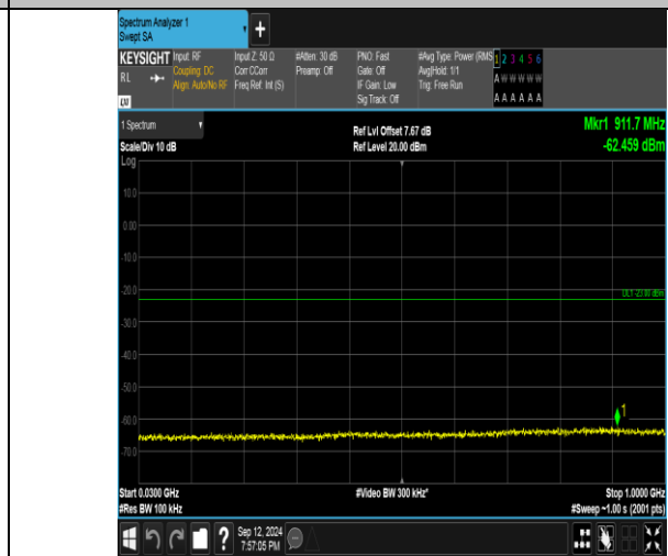
Band4_5MHz_16QAM_19975_25RB#0_30~1000_30~1000
