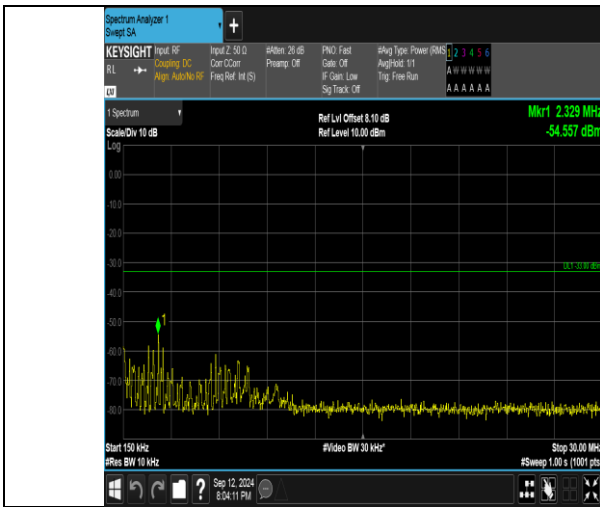
Band4_5MHz_16QAM_20375_1RB#0_0.15~30_0.15~30
