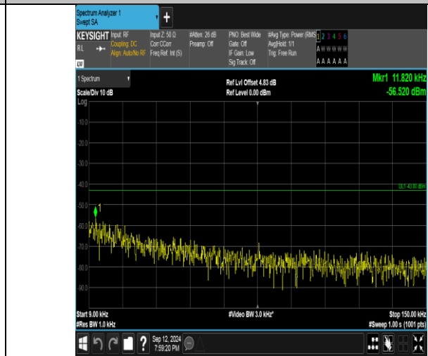
Band4_5MHz_16QAM_20175_1RB#0_0.009~0.15_0.009~0.15
