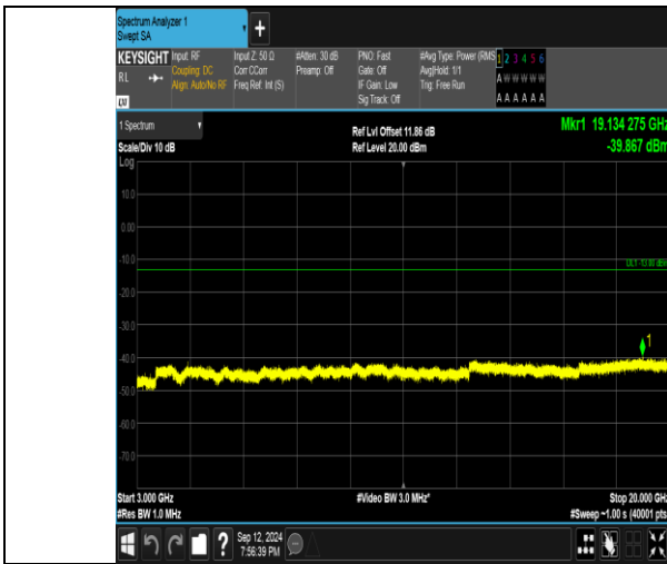
Band4_5MHz_QPSK_19975_25RB#0_3000~20000_3000~20000
