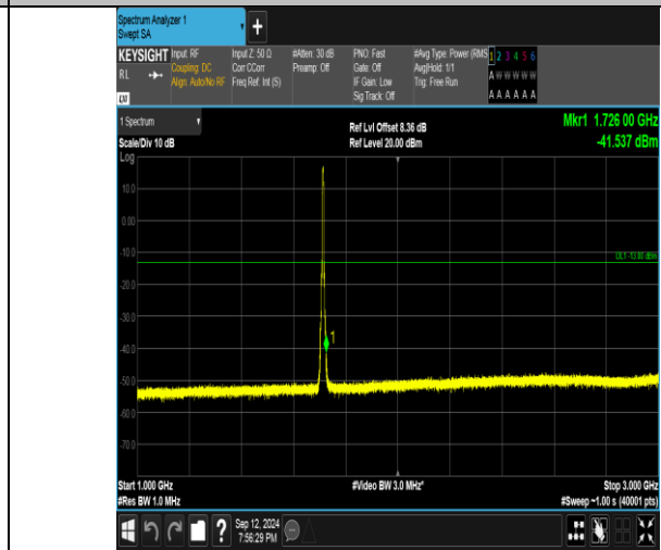
Band4_5MHz_QPSK_19975_25RB#0_1000-3000_1000-3000
