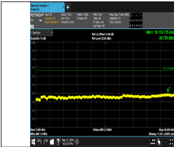
Band4_5MHz_QPSK_20175_25RB#0_3000-20000_3000-20000
