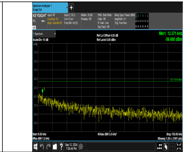
Band4_5MHz_16QAM_19975_25RB#0_0.009~0.15_0.009~0.15
