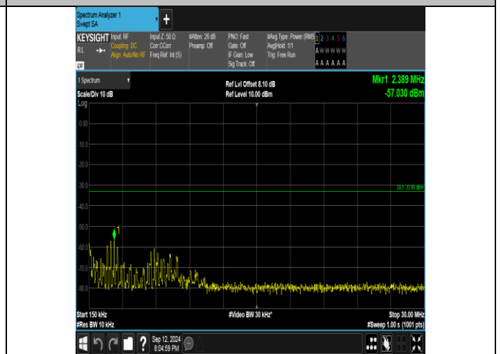
Band4_5MHz_QPSK_20375_1RB#24_0.15~30_0.15~30
