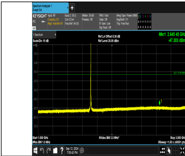
Band4_5MHz_16QAM_19975_1RB#24_1000-3000_1000-3000
