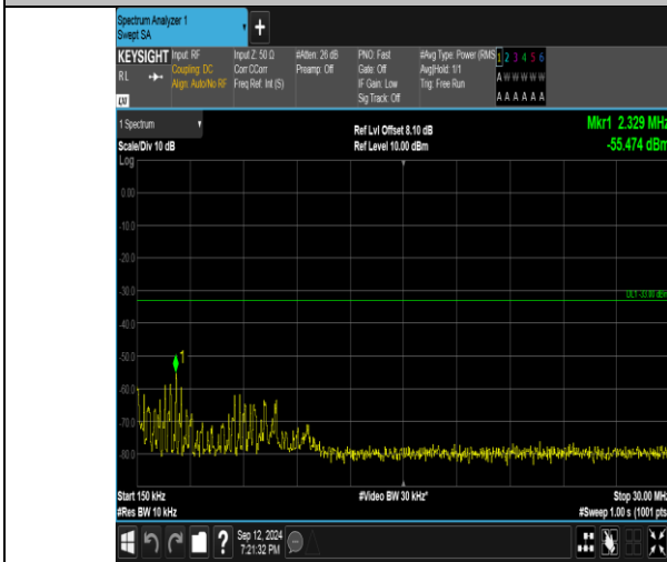
Band4_3MHz_16QAM_20385_15RB#0_0.15~30_0.15~30
