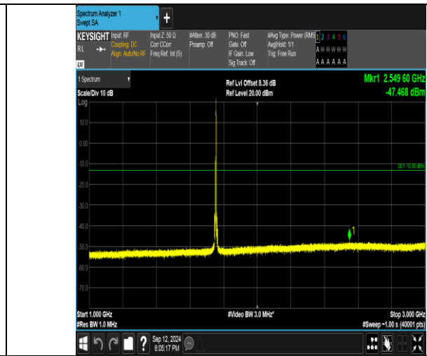
Band4_5MHz_QPSK_20375_1RB#24_1000~3000_1000~3000
