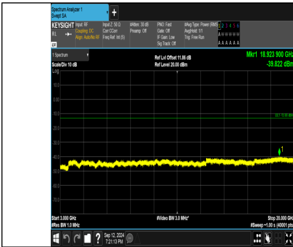
Band4_3MHz_QPSK_20385_15RB#0_3000~20000_3000~20000
