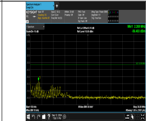
Band4_5MHz_QPSK_19975_25RB#0_0.15-30_0.15-30
