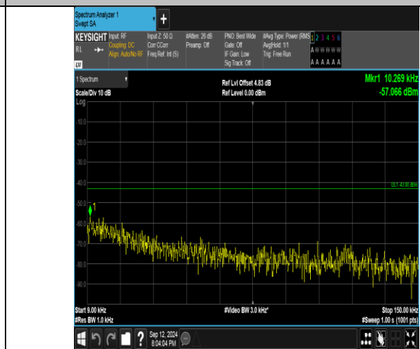
Band4_5MHz_16QAM_20375_1RB#0_0.009~0.15_0.009~0.15
