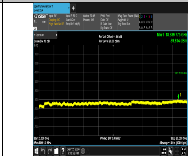
Band4_3MHz_16QAM_20385_1RB#0_3000-20000_3000-20000
