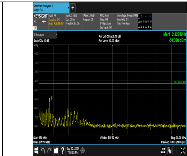
Band4_3MHz_QPSK_19965_1RB#0_0.15~30_0.15~30
