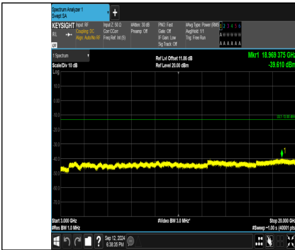
Band4_1.4MHz_QPSK_20393_6RB#0_3000~20000_3000~20000
