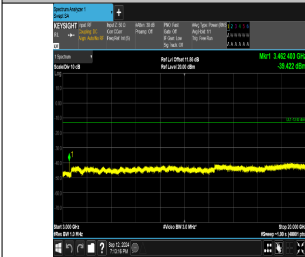
Band4_3MHz_QPSK_20175_1RB#0_3000~20000_3000~20000
