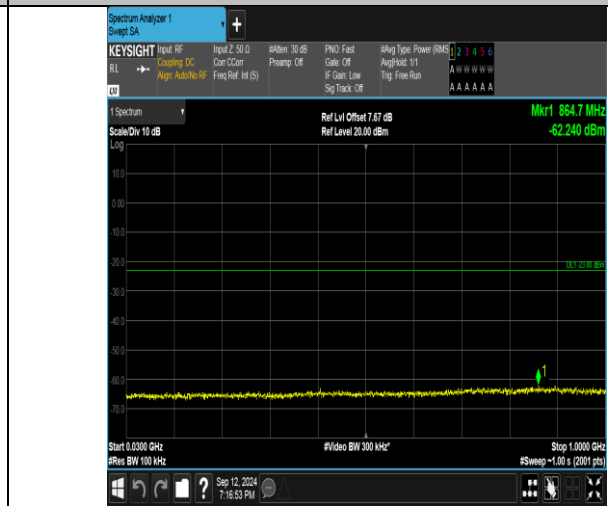
Band4_3MHz_16QAM_20175_15RB#0_30~1000_30~1000
