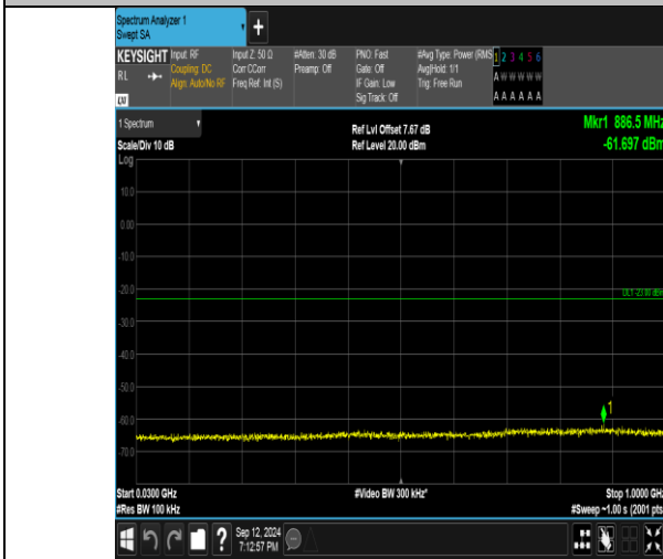
Band4_3MHz_QPSK_20175_1RB#0_30~1000_30~1000
