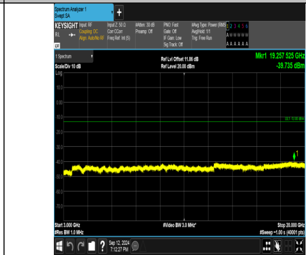
Band4_3MHz_16QAM_19965_15RB#0_3000~20000_3000~20000
