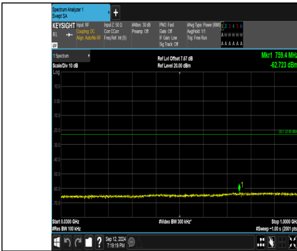
Band4_3MHz_QPSK_20385_1RB#14_30~1000_30~1000
