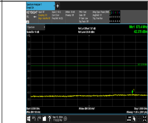
Band4_3MHz_16QAM_19965_1RB#14_30~1000_30~1000
