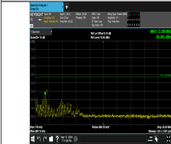
Band4_3MHz_16QAM_19965_15RB#0_0.15~30_0.15~30
