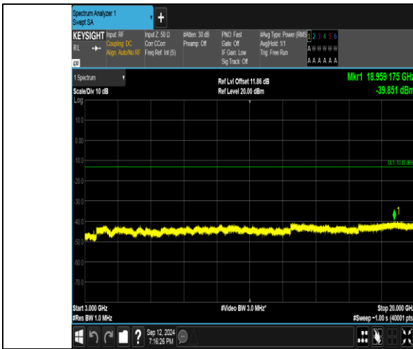
Band4_3MHz_QPSK_20175_15RB#0_3000~20000_3000~20000
