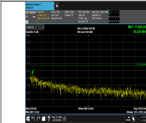
Band4_1.4MHz_QPSK_20393_6RB#0_0.009~0.15_0.009~0.15
