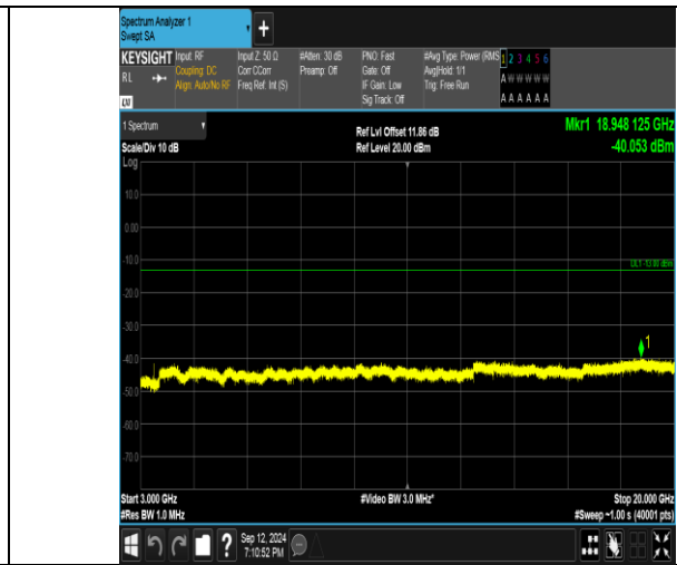
Band4_3MHz_16QAM_19965_1RB#14_3000-20000_3000-20000
