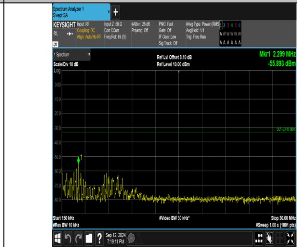
Band4_3MHz_QPSK_20385_1RB#14_0.15-30_0.15-30
