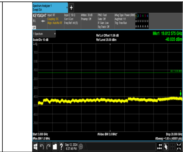
Band4_1.4MHz_16QAM_20393_1RB#5_3000~20000_3000~20000
