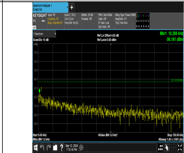
Band4_3MHz_16QAM_19965_1RB#14_0.009~0.15_0.009~0.15
