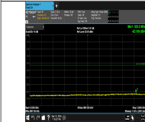
Band4_3MHz_QPSK_20175_15RB#0_30-1000_30-1000
