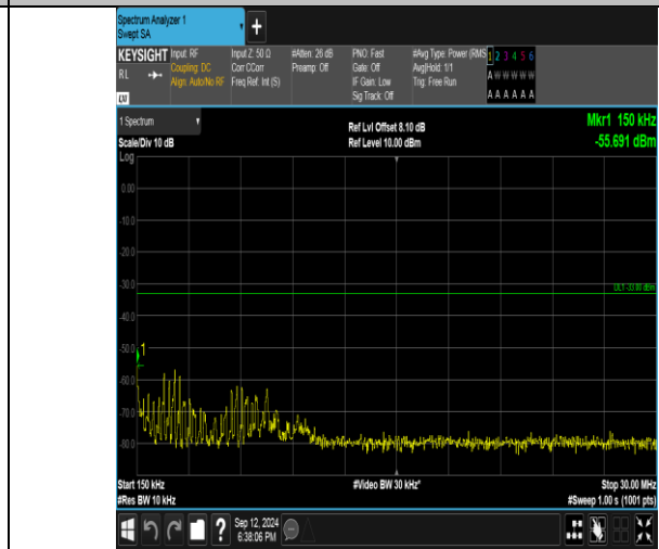
Band4_1.4MHz_QPSK_20393_6RB#0_0.15~30_0.15~30
