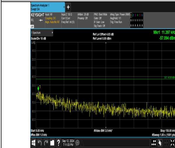
Band4_3MHz_QPSK_19965_15RB#0_0.009-0.15_0.009-0.15
