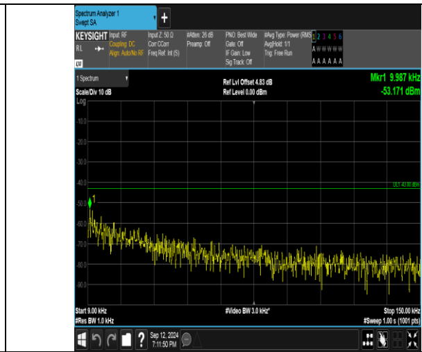
Band4_3MHz_16QAM_19965_15RB#0_0.009~0.15_0.009~0.15
