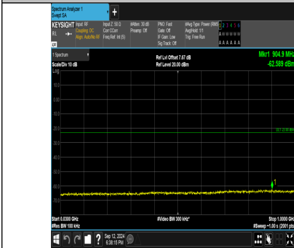
Band4_1.4MHz_QPSK_20393_6RB#0_30~1000_30~1000
