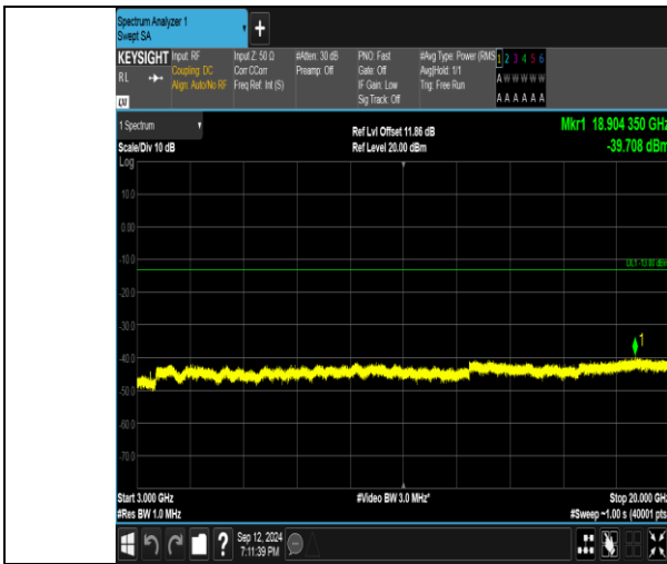
Band4_3MHz_QPSK_19965_15RB#0_3000~20000_3000~20000
