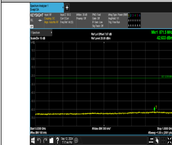
Band4_3MHz_QPSK_20385_1RB#0_30~1000_30~1000
