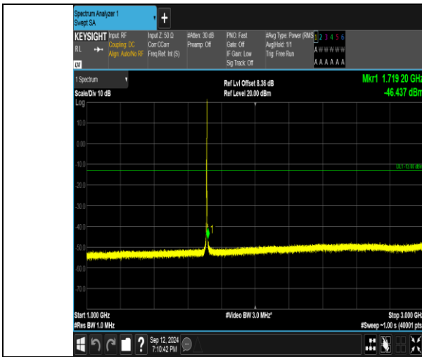
Band4_3MHz_16QAM_19965_1RB#14_1000-3000_1000-3000
