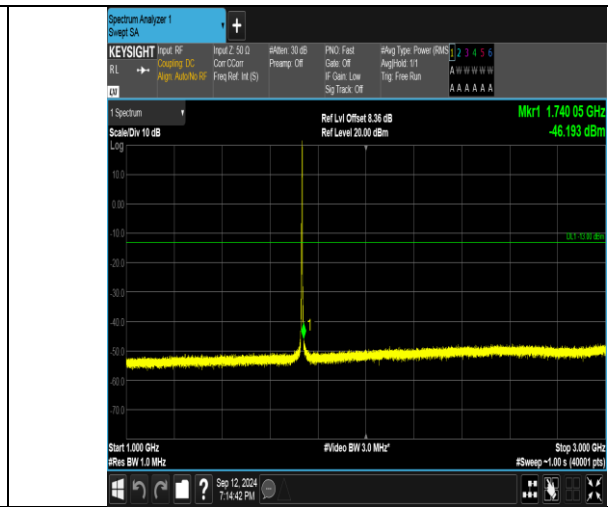
Band4_3MHz_QPSK_20175_1RB#14_1000~3000_1000~3000
