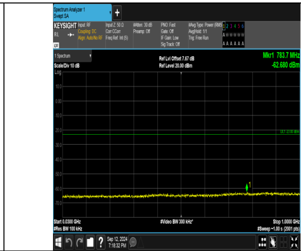
Band4_3MHz_16QAM_20385_1RB#0_30-1000_30-1000
