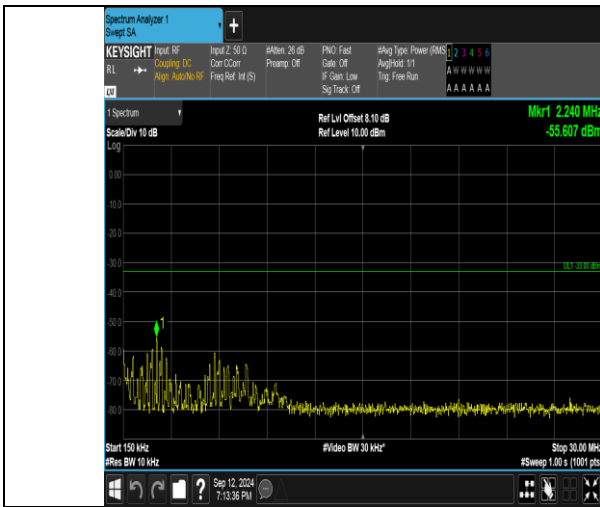
Band4_3MHz_16QAM_20175_1RB#0_0.15-30_0.15-30
