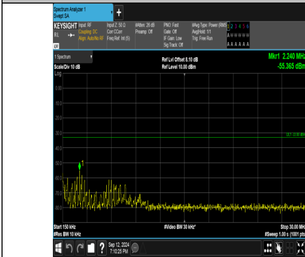
Band4_3MHz_16QAM_19965_1RB#14_0.15~30_0.15~30
