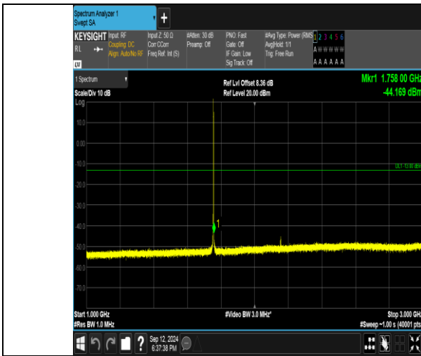
Band4_1.4MHz_16QAM_20393_1RB#5_1000~3000_1000~3000
