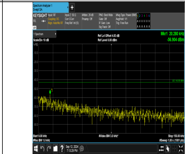
Band4_3MHz_16QAM_20175_1RB#0_0.009~0.15_0.009~0.15
