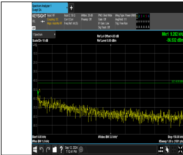
Band4_3MHz_QPSK_20175_1RB#0_0.009~0.15_0.009~0.15
