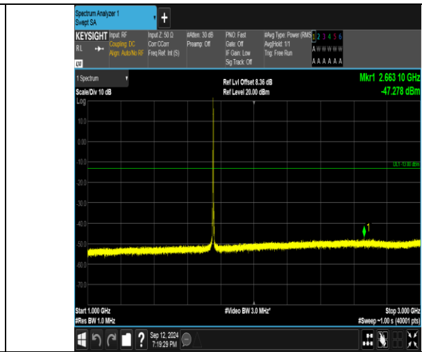
Band4_3MHz_QPSK_20385_1RB#14_1000~3000_1000~3000
