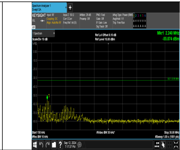
Band4_3MHz_QPSK_20385_1RB#0_0.15~30_0.15~30
