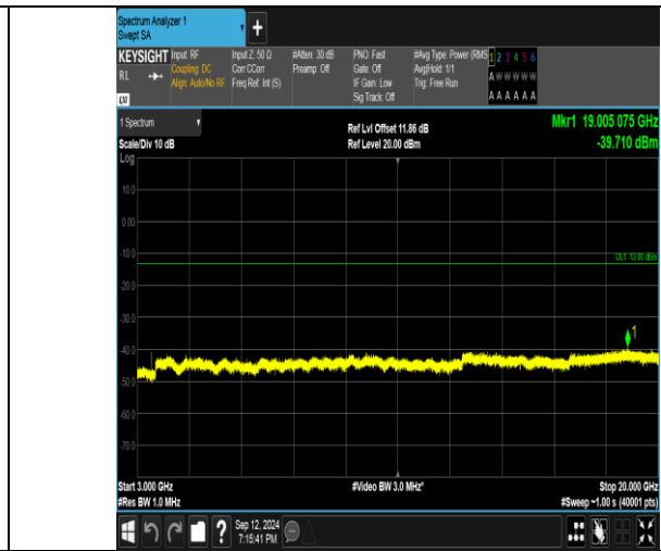
Band4_3MHz_16QAM_20175_1RB#14_3000-20000_3000-20000
