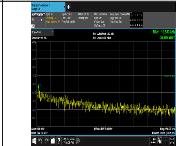
Band4_3MHz_16QAM_20175_1RB#14_0.009~0.15_0.009~0.15
