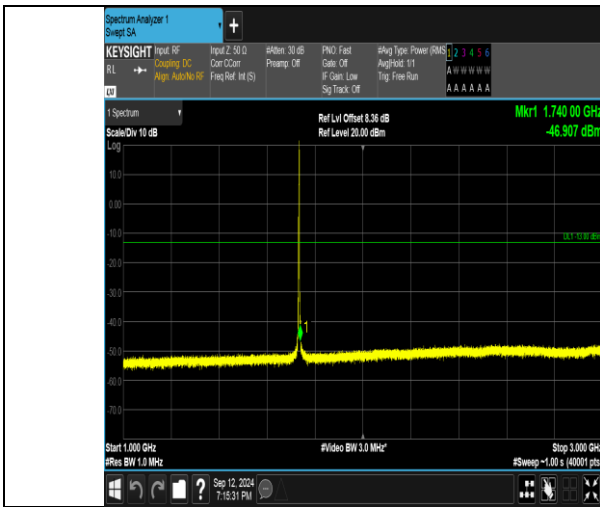
Band4_3MHz_16QAM_20175_1RB#14_1000-3000_1000-3000
