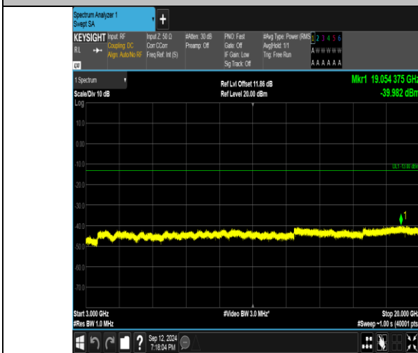
Band4_3MHz_QPSK_20385_1RB#0_3000~20000_3000~20000
