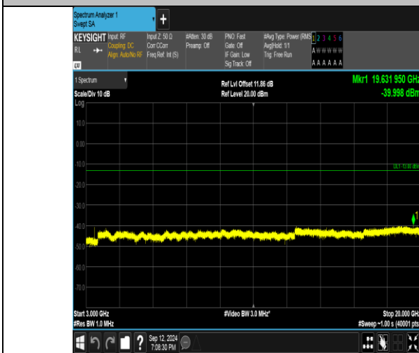
Band4_3MHz_QPSK_19965_1RB#0_3000~20000_3000~20000
