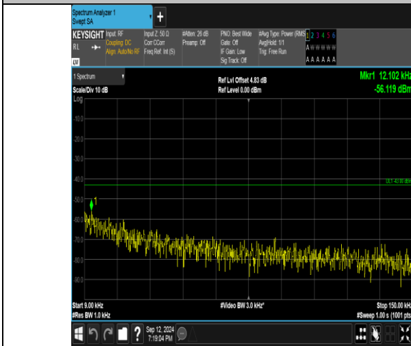
Band4_3MHz_QPSK_20385_1RB#14_0.009-0.15_0.009-0.15
