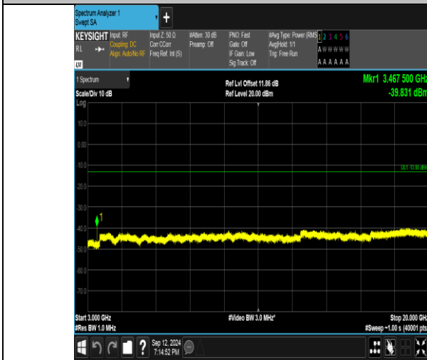
Band4_3MHz_QPSK_20175_1RB#14_3000~20000_3000~20000
