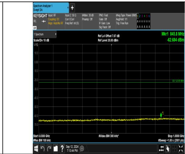
Band4_3MHz_16QAM_20175_1RB#0_30-1000_30-1000
