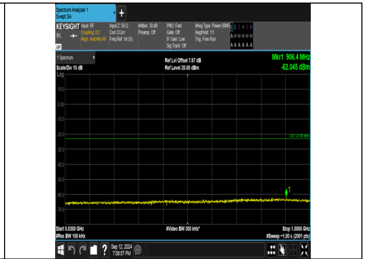
Band4_3MHz_16QAM_19965_1RB#0_30-1000_30-1000
