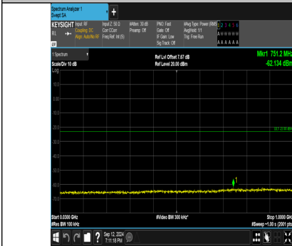
Band4_3MHz_QPSK_19965_15RB#0_30-1000_30-1000
