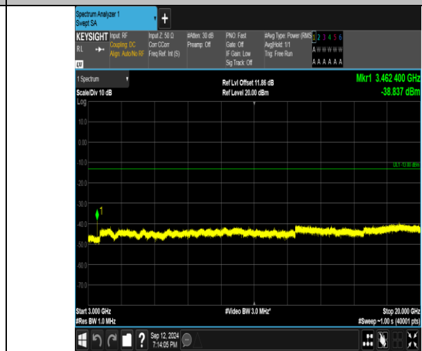
Band4_3MHz_16QAM_20175_1RB#0_3000-20000_3000-20000
