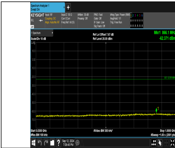
Band4_3MHz_QPSK_19965_1RB#14_30~1000_30~1000
