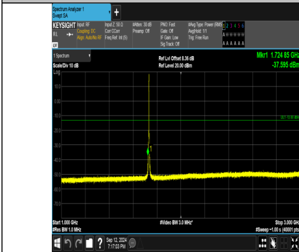
Band4_3MHz_16QAM_20175_15RB#0_1000~3000_1000~3000
