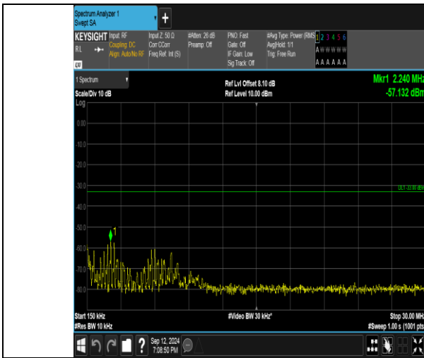
Band4_3MHz_16QAM_19965_1RB#0_0.15-30_0.15-30
