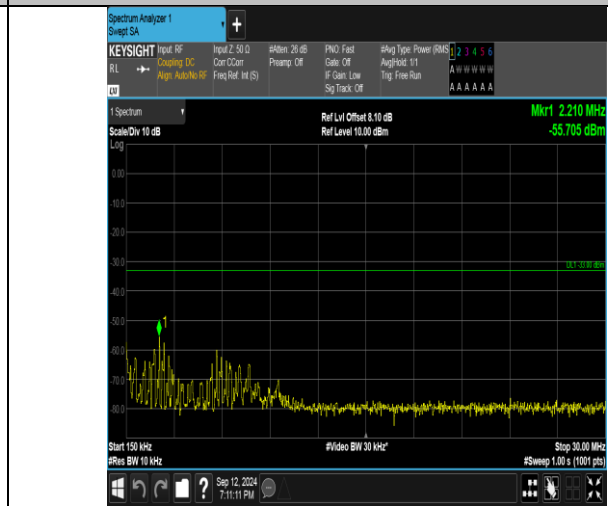
Band4_3MHz_QPSK_19965_15RB#0_0.15-30_0.15-30
