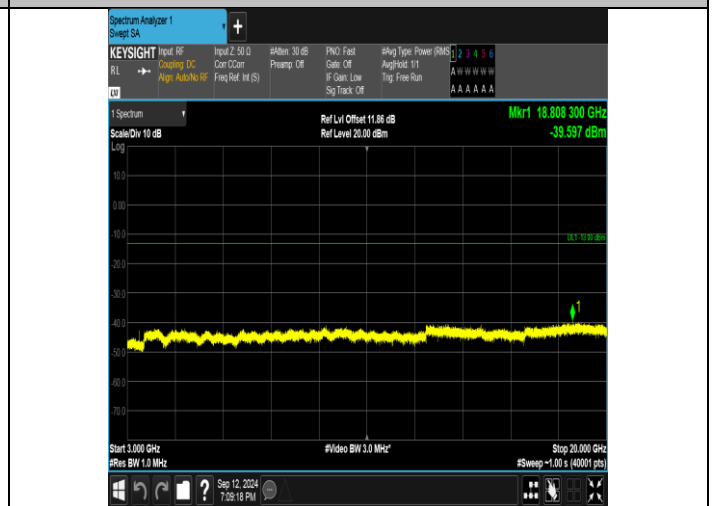
Band4_3MHz_16QAM_19965_1RB#0_3000-20000_3000-20000
