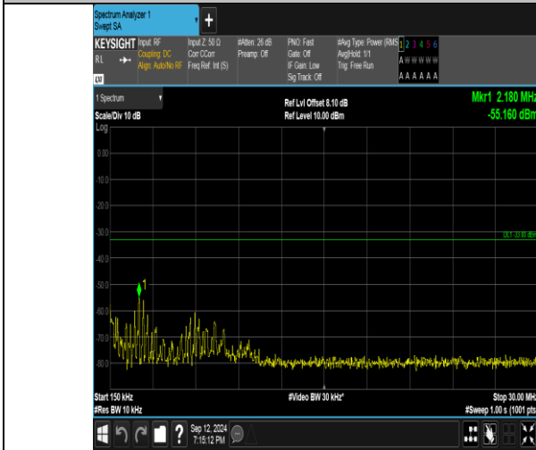
Band4_3MHz_16QAM_20175_1RB#14_0.15~30_0.15~30
