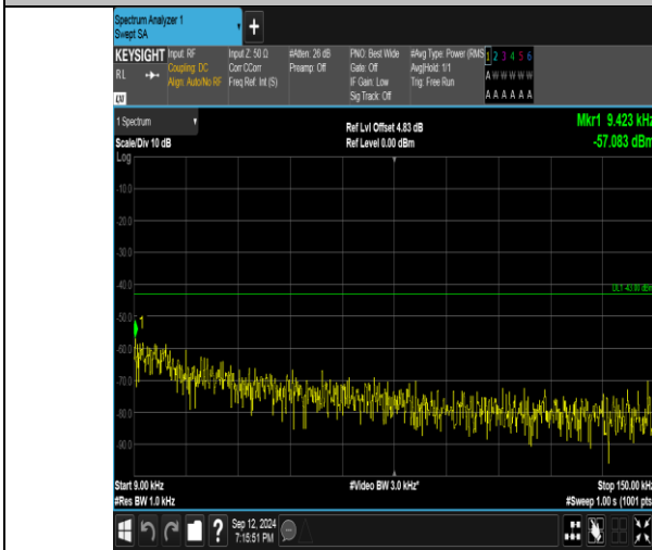
Band4_3MHz_QPSK_20175_15RB#0_0.009-0.15_0.009-0.15
