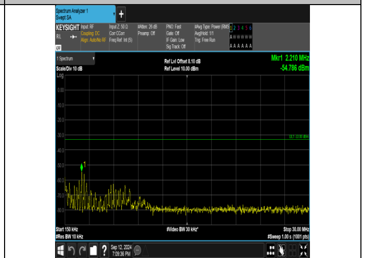
Band4_3MHz_QPSK_19965_1RB#14_0.15-30_0.15-30
