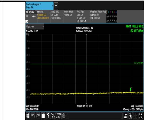
Band4_3MHz_16QAM_19965_15RB#0_30~1000_30~1000
