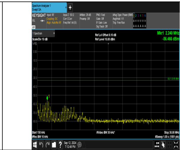
Band4_3MHz_QPSK_20175_1RB#0_0.15~30_0.15~30
