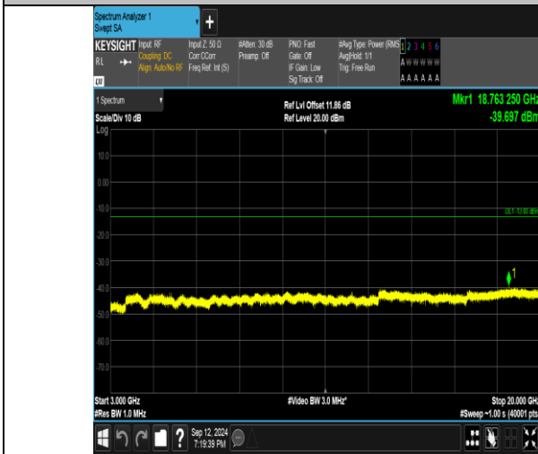
Band4_3MHz_QPSK_20385_1RB#14_3000~20000_3000~20000
