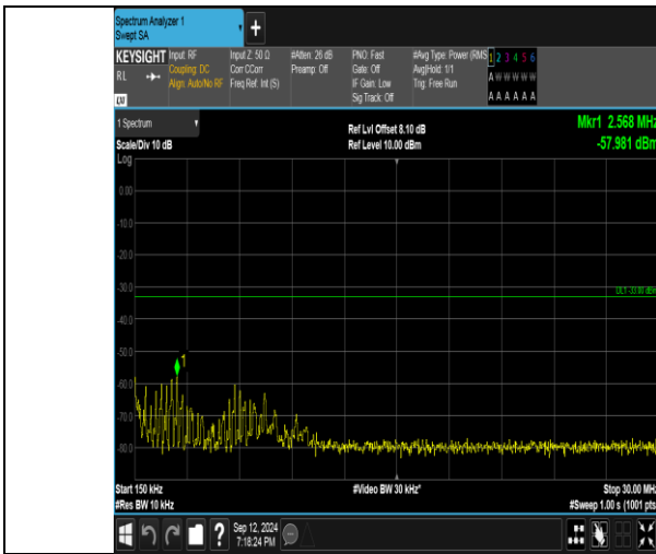
Band4_3MHz_16QAM_20385_1RB#0_0.15-30_0.15-30
