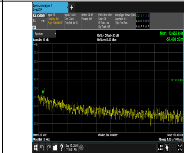
Band4_3MHz_16QAM_20385_1RB#14_0.009~0.15_0.009~0.15
