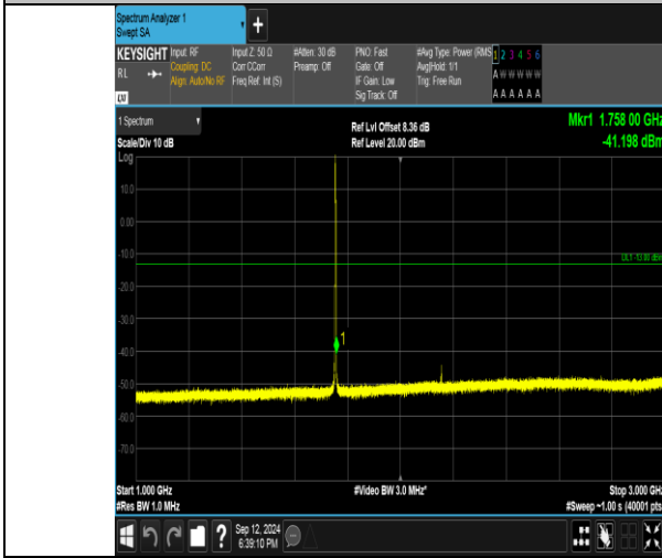
Band4_1.4MHz_16QAM_20393_6RB#0_1000~3000_1000~3000
