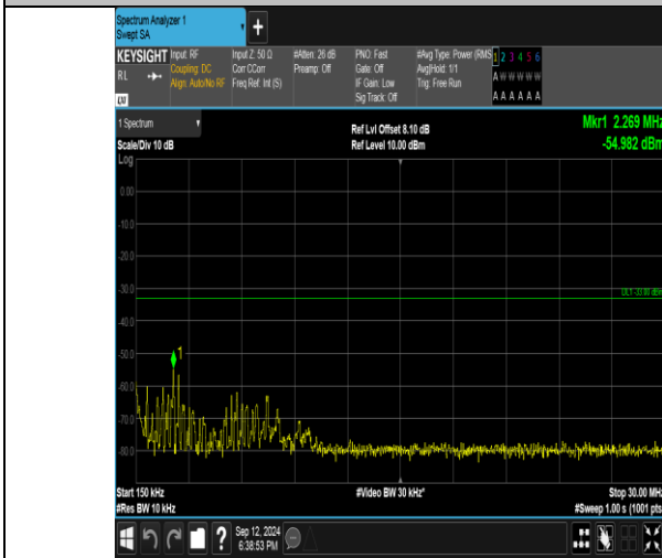
Band4_1.4MHz_16QAM_20393_6RB#0_0.15~30_0.15~30
