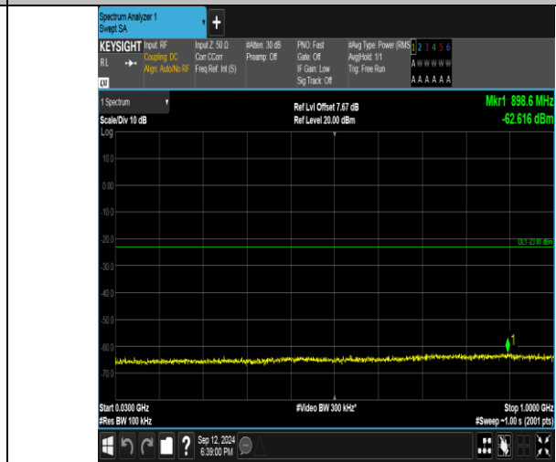
Band4_1.4MHz_16QAM_20393_6RB#0_30~1000_30~1000
