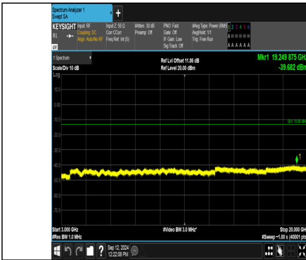
Band2_3MHz_QPSK_19185_15RB#0_3000-20000_3000-20000
