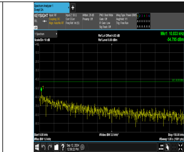
Band2_5MHz_16QAM_18625_25RB#0_0.009-0.15_0.009-0.15
