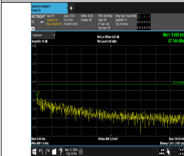
Band2_5MHz_QPSK_18900_25RB#0_0.009~0.15_0.009~0.15
