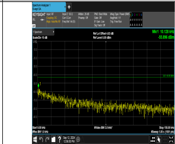
Band2_5MHz_16QAM_18625_1RB#24_0.009~0.15_0.009~0.15
