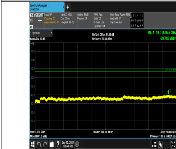
Band2_5MHz_QPSK_19175_1RB#24_3000~20000_3000~20000
