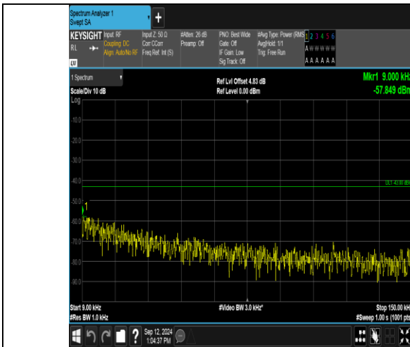
Band2_5MHz_QPSK_19175_1RB#0_0.009~0.15_0.009~0.15
