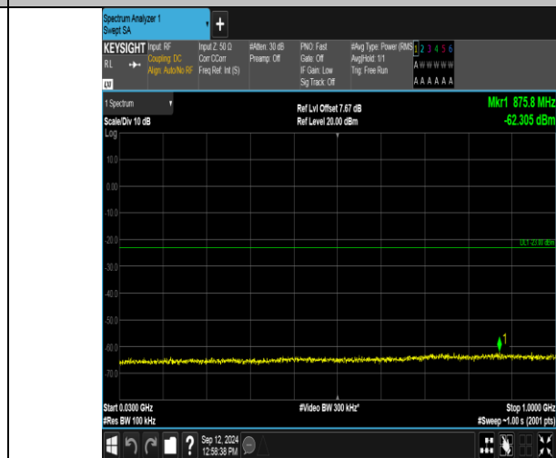
Band2_5MHz_16QAM_18625_25RB#0_30-1000_30-1000
