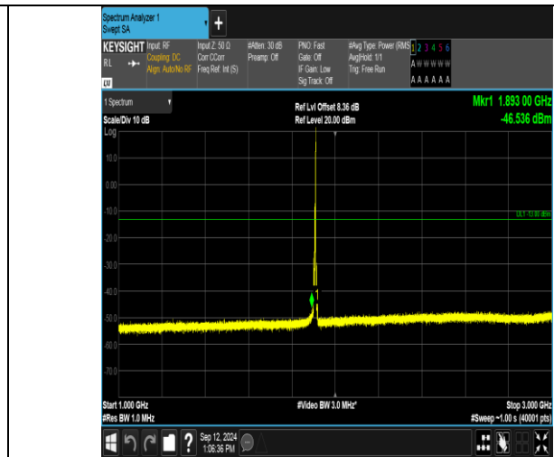
Band2_5MHz_QPSK_19175_1RB#24_1000~3000_1000~3000
