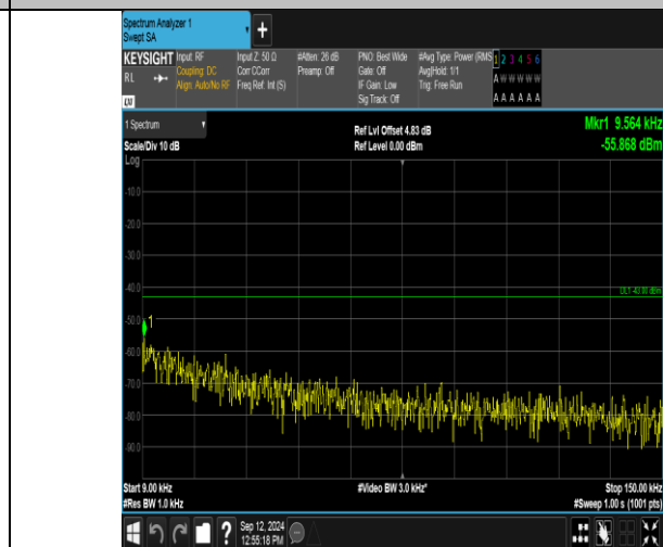
Band2_5MHz_16QAM_18625_1RB#0_0.009-0.15_0.009-0.15
