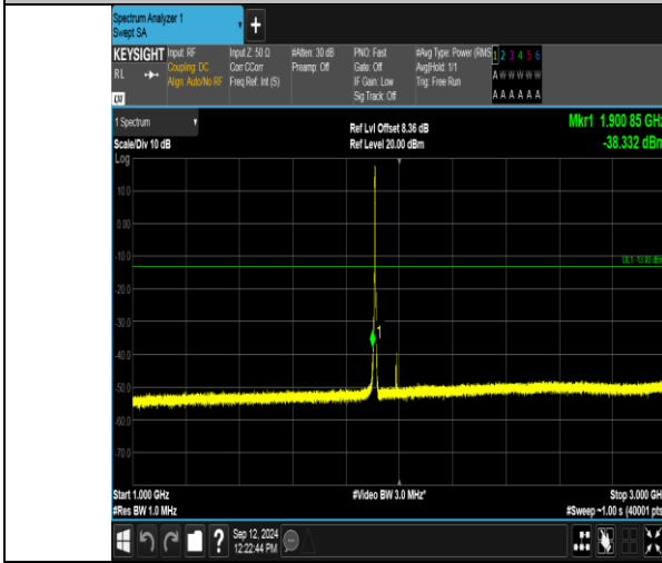
Band2_3MHz_16QAM_19185_15RB#0_1000-3000_1000-3000
