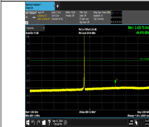
Band2_5MHz_16QAM_19175_1RB#0_1000~3000_1000~3000
