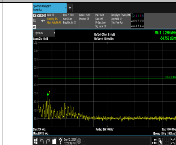
Band2_5MHz_QPSK_18625_1RB#24_0.15~30_0.15~30
