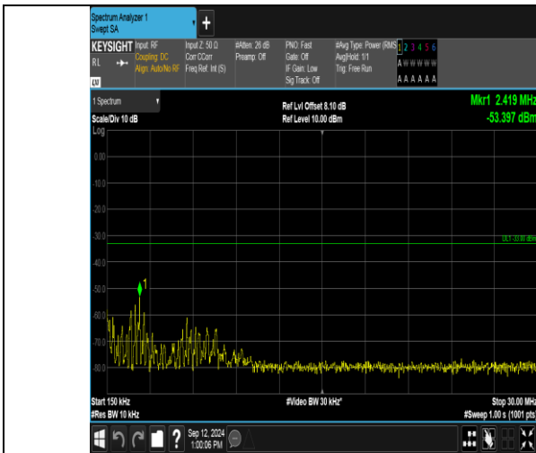
Band2_5MHz_16QAM_18900_1RB#0_0.15~30_0.15~30
