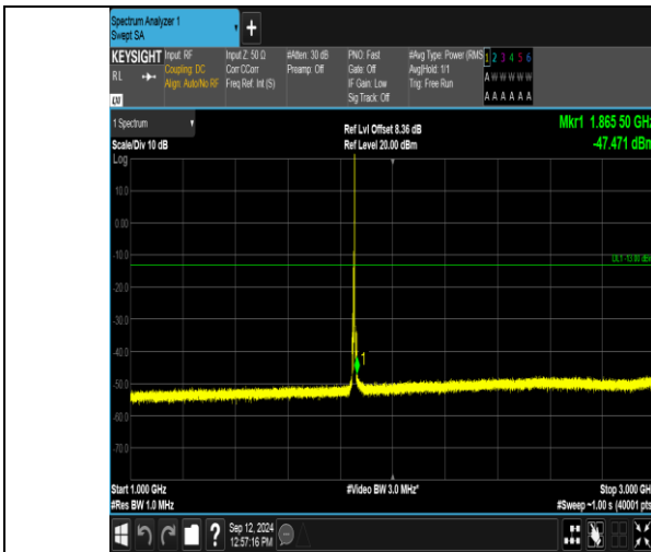
Band2_5MHz_16QAM_18625_1RB#24_1000~3000_1000~3000
