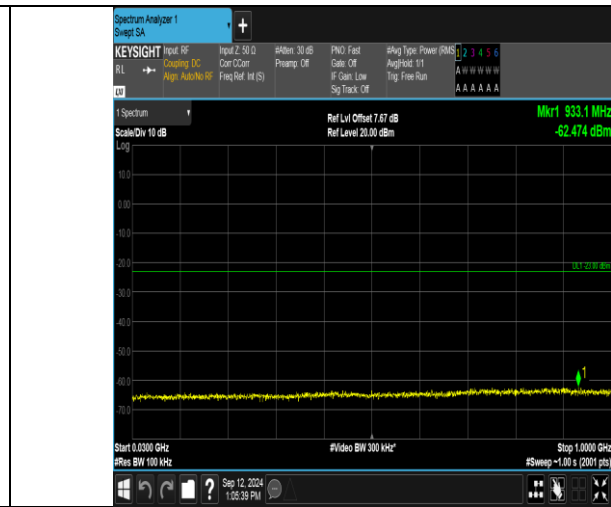
Band2_5MHz_16QAM_19175_1RB#0_30~1000_30~1000
