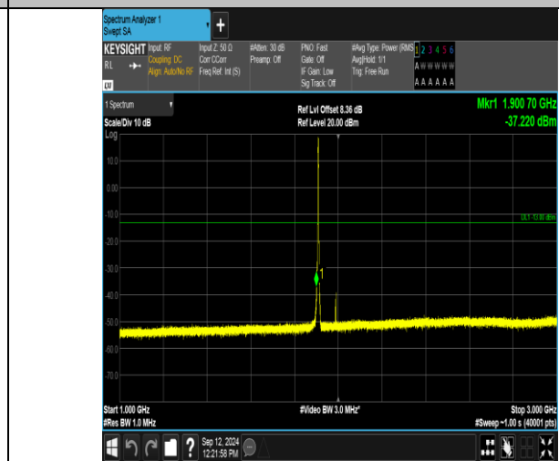
Band2_3MHz_QPSK_19185_15RB#0_1000~3000_1000~3000
