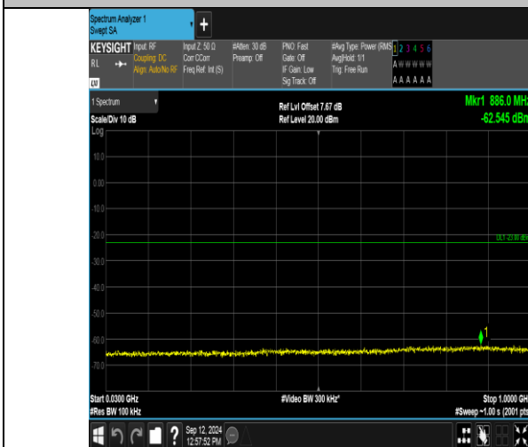
Band2_5MHz_QPSK_18625_25RB#0_30~1000_30~1000
