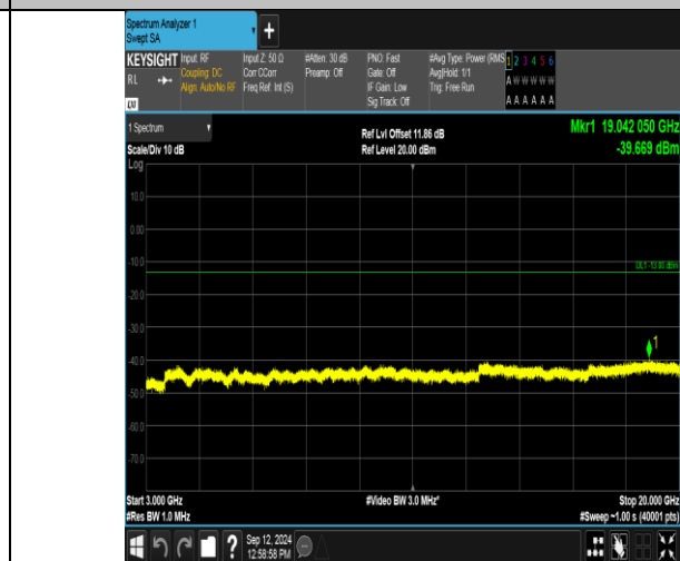
Band2_5MHz_16QAM_18625_25RB#0_3000-20000_3000-20000
