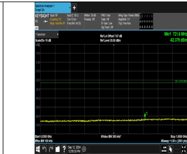
Band2_5MHz_16QAM_18625_1RB#0_30~1000_30~1000
