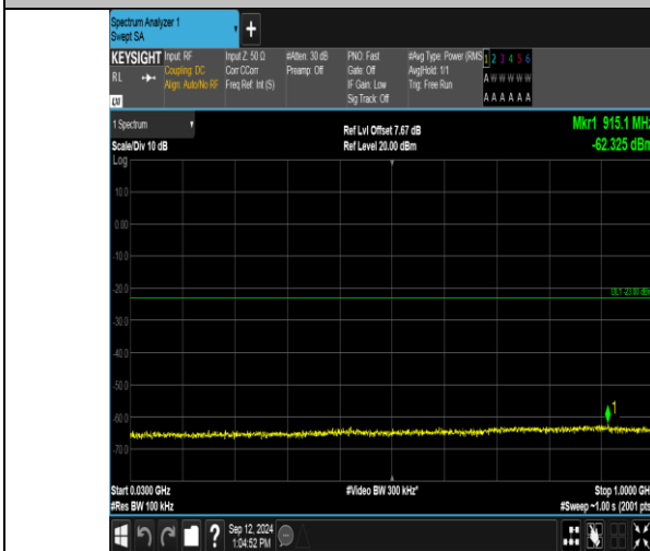
Band2_5MHz_QPSK_19175_1RB#0_30~1000_30~1000
