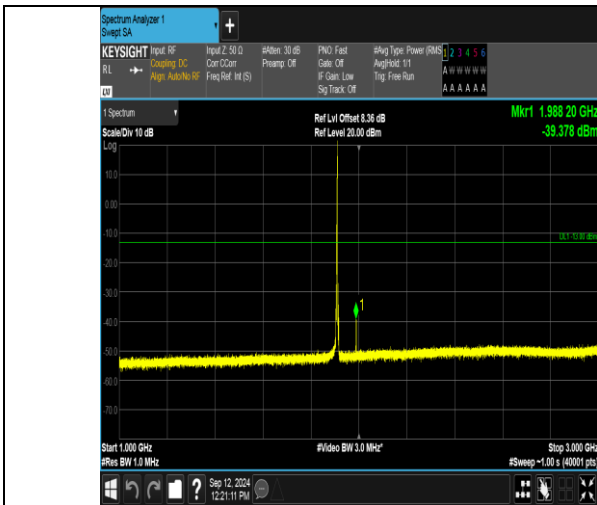
Band2_3MHz_16QAM_19185_1RB#14_1000~3000_1000~3000
