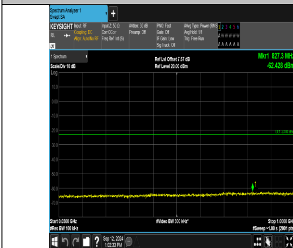
Band2_5MHz_QPSK_18900_25RB#0_30~1000_30~1000
