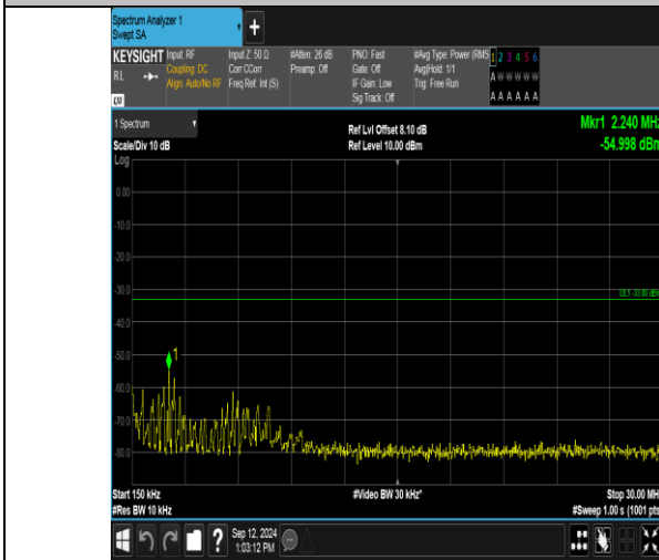
Band2_5MHz_16QAM_18900_25RB#0_0.15~30_0.15~30
