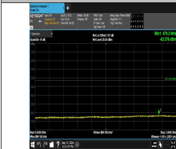
Band2_3MHz_QPSK_19185_15RB#0_30~1000_30~1000
