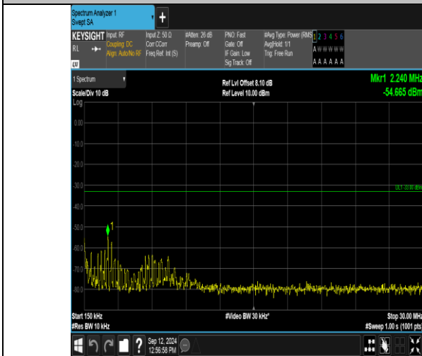
Band2_5MHz_16QAM_18625_1RB#24_0.15~30_0.15~30
