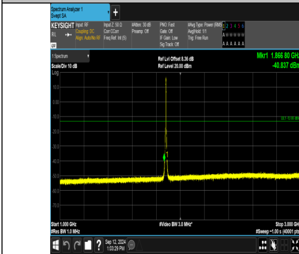
Band2_5MHz_16QAM_18900_25RB#0_1000~3000_1000~3000
