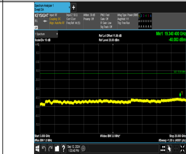
Band2_5MHz_16QAM_18900_25RB#0_3000~20000_3000~20000
