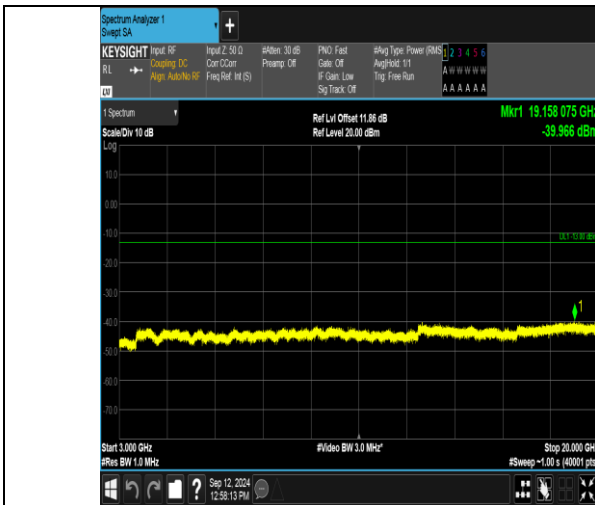
Band2_5MHz_QPSK_18625_25RB#0_3000-20000_3000-20000
