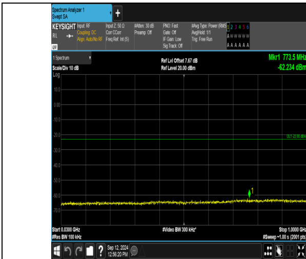
Band2_5MHz_QPSK_18625_1RB#24_30~1000_30~1000
