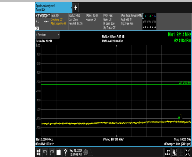
Band2_5MHz_16QAM_18625_1RB#24_30~1000_30~1000
