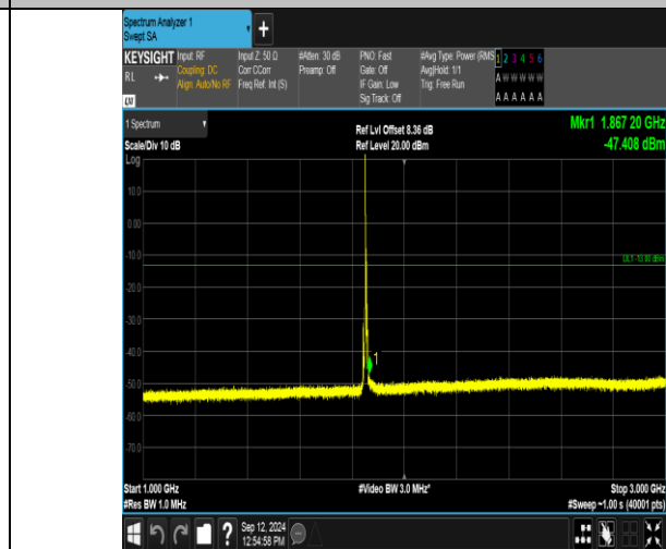
Band2_5MHz_QPSK_18625_1RB#0_1000-3000_1000-3000
