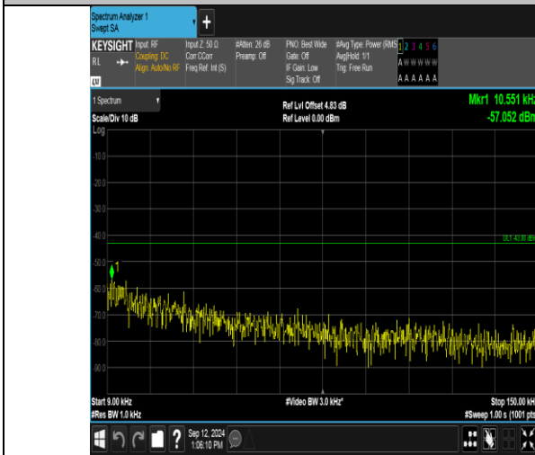
Band2_5MHz_QPSK_19175_1RB#24_0.009~0.15_0.009~0.15
