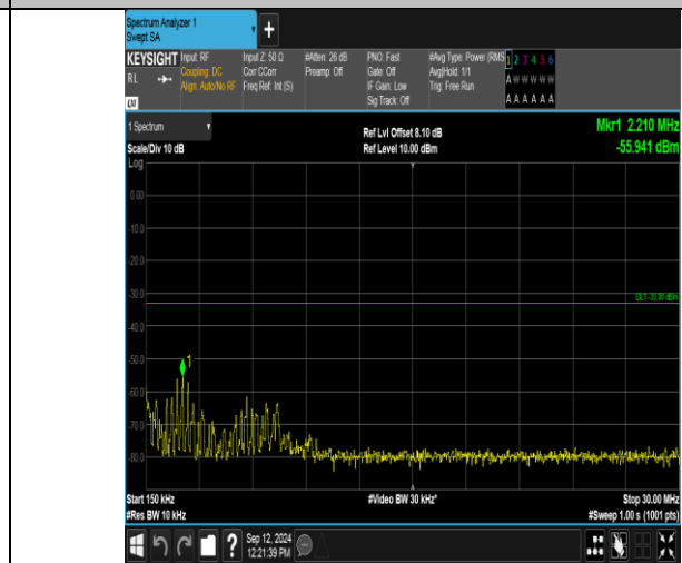
Band2_3MHz_QPSK_19185_15RB#0_0.15~30_0.15~30
