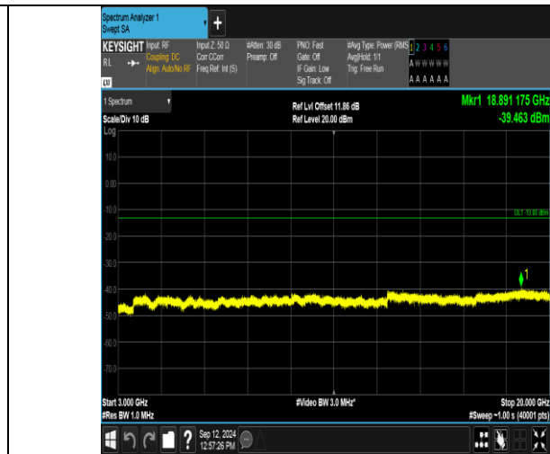
Band2_5MHz_16QAM_18625_1RB#24_3000~20000_3000~20000
