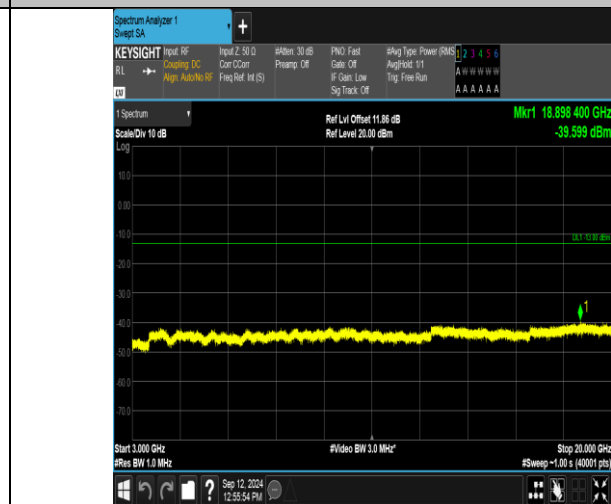
Band2_5MHz_16QAM_18625_1RB#0_3000~20000_3000~20000
