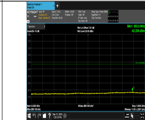
Band2_5MHz_16QAM_18900_25RB#0_30~1000_30~1000
