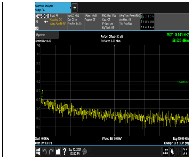
Band2_5MHz_16QAM_18900_25RB#0_0.009~0.15_0.009~0.15
