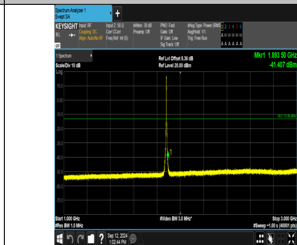
Band2_5MHz_QPSK_18900_25RB#0_1000~3000_1000~3000
