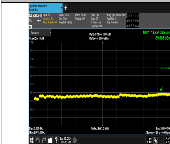
Band2_5MHz_QPSK_19175_1RB#0_3000~20000_3000~20000
