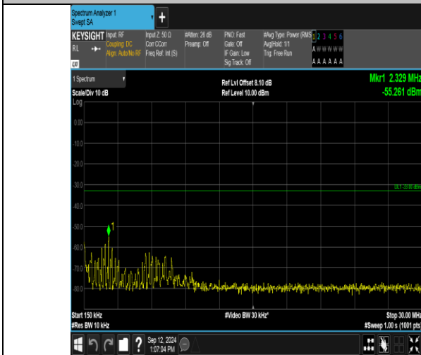
Band2_5MHz_16QAM_19175_1RB#24_0.15~30_0.15~30
