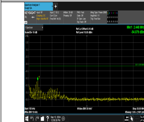
Band2_5MHz_16QAM_18625_25RB#0_0.15-30_0.15-30
