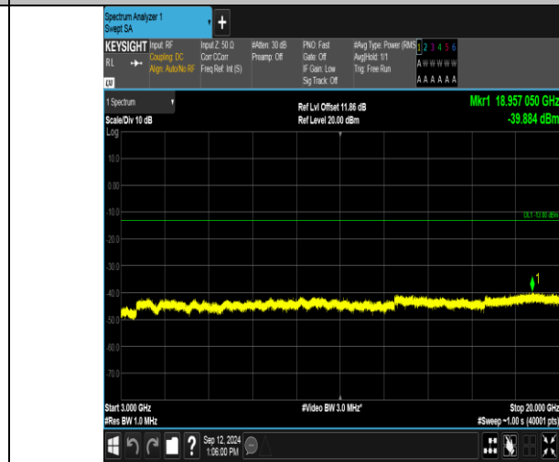
Band2_5MHz_16QAM_19175_1RB#0_3000~20000_3000~20000
