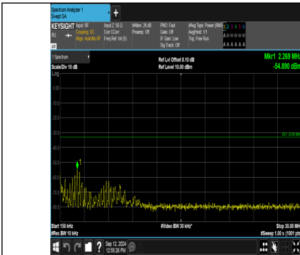
Band2_5MHz_16QAM_18625_1RB#0_0.15~30_0.15~30
