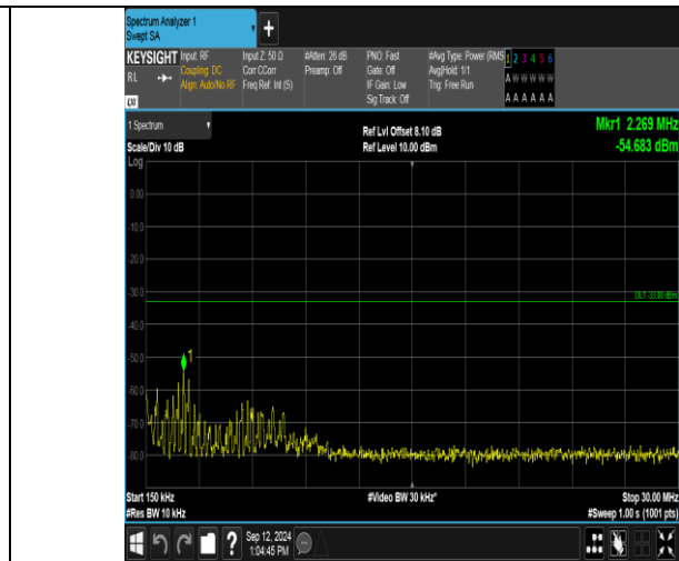
Band2_5MHz_QPSK_19175_1RB#0_0.15~30_0.15~30
