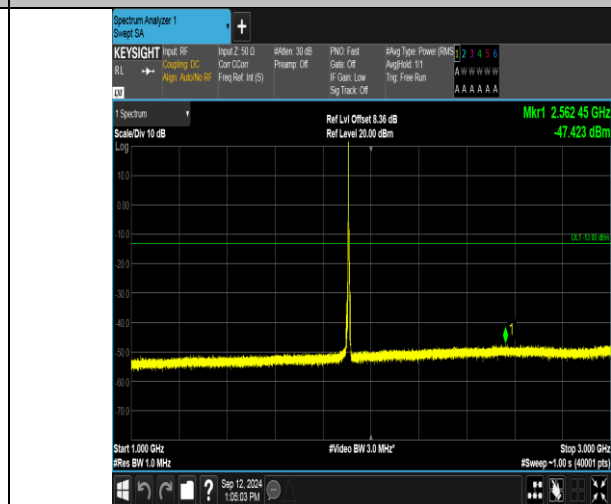
Band2_5MHz_QPSK_19175_1RB#0_1000~3000_1000~3000
