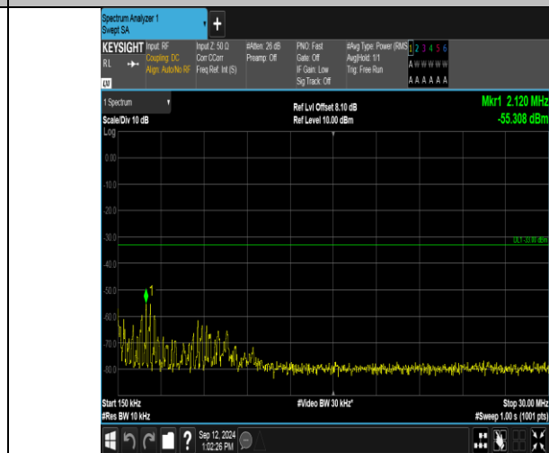
Band2_5MHz_QPSK_18900_25RB#0_0.15~30_0.15~30
