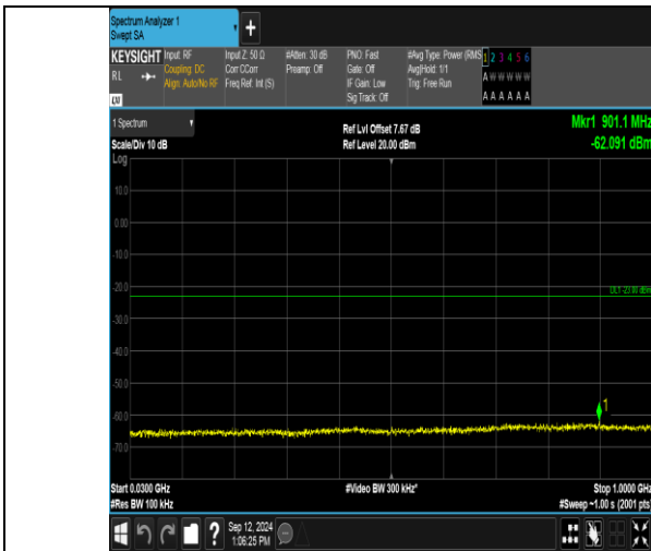
Band2_5MHz_QPSK_19175_1RB#24_30~1000_30~1000
