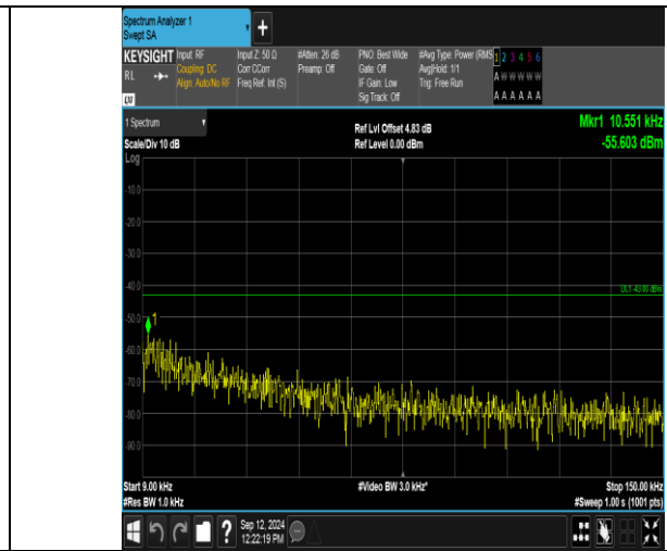
Band2_3MHz_16QAM_19185_15RB#0_0.009-0.15_0.009-0.15
