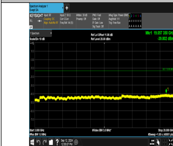
Band2_5MHz_QPSK_18625_1RB#0_3000-20000_3000-20000
