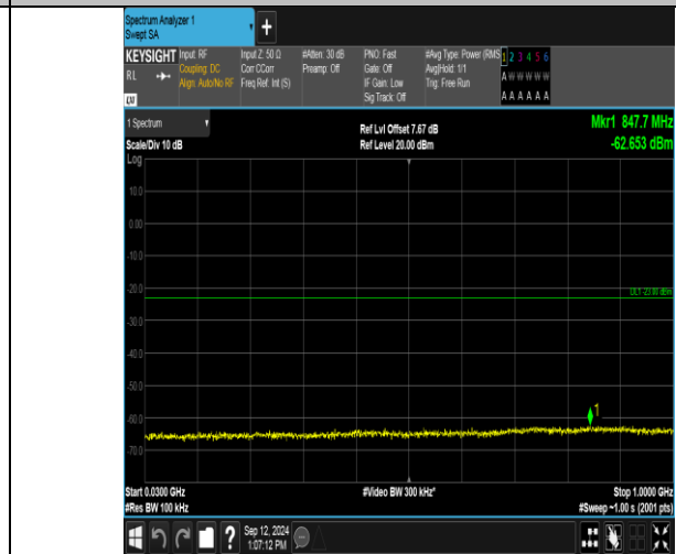
Band2_5MHz_16QAM_19175_1RB#24_30~1000_30~1000
