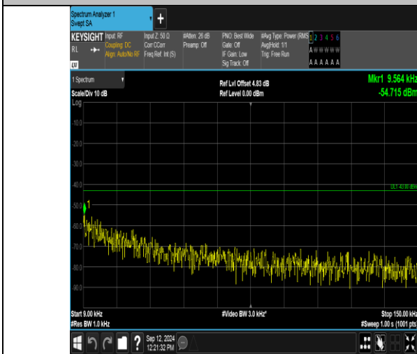
Band2_3MHz_QPSK_19185_15RB#0_0.009~0.15_0.009~0.15
