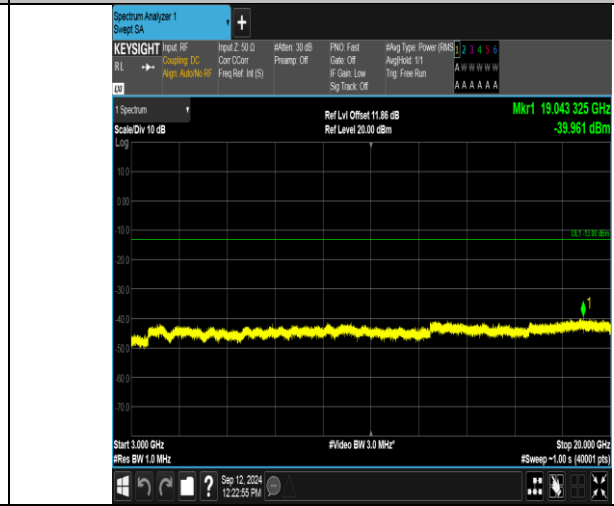
Band2_3MHz_16QAM_19185_15RB#0_3000-20000_3000-20000
