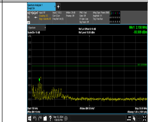
Band2_5MHz_QPSK_18900_1RB#24_0.15~30_0.15~30
