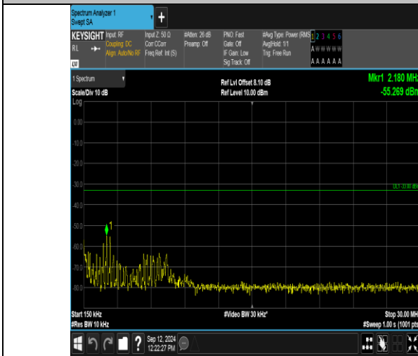
Band2_3MHz_16QAM_19185_15RB#0_0.15-30_0.15-30
