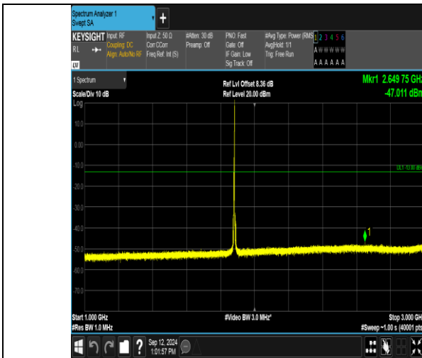
Band2_5MHz_16QAM_18900_1RB#24_1000~3000_1000~3000
