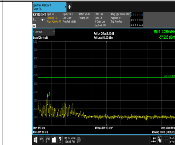
Band2_5MHz_QPSK_19175_1RB#24_0.15~30_0.15~30
