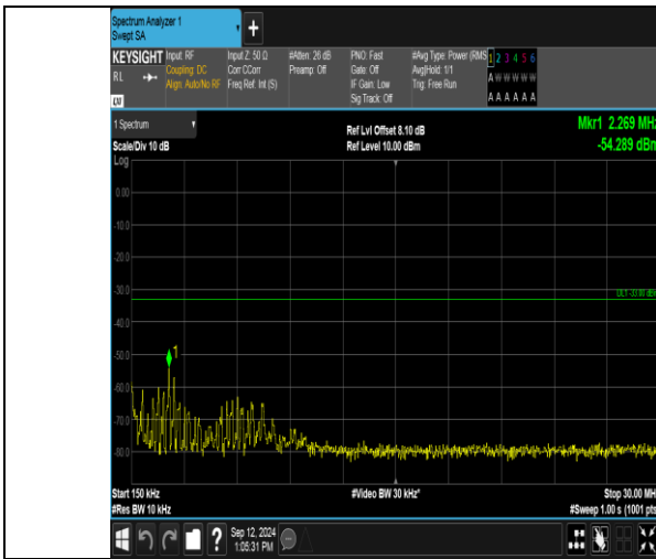
Band2_5MHz_16QAM_19175_1RB#0_0.15~30_0.15~30
