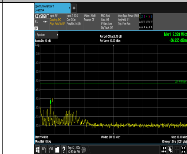
Band2_5MHz_QPSK_18625_25RB#0_0.15~30_0.15~30
