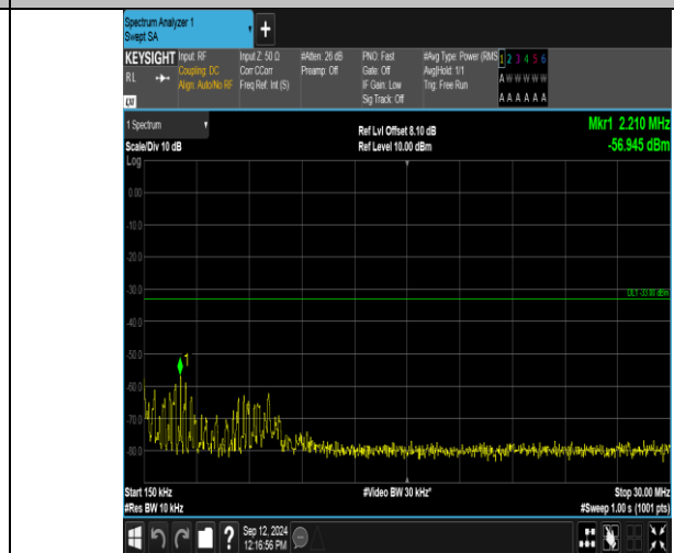
Band2_3MHz_QPSK_18900_15RB#0_0.15~30_0.15~30
