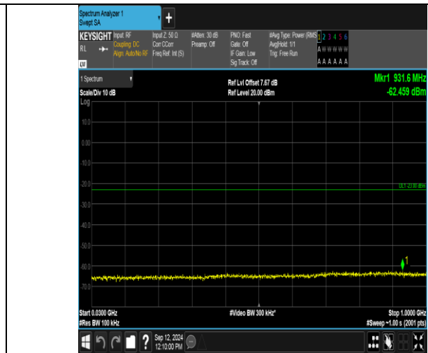
Band2_3MHz_16QAM_18615_1RB#0_30~1000_30~1000
