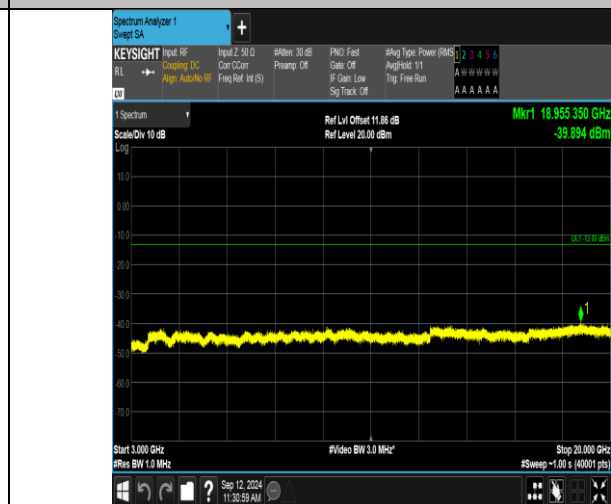
Band2_1.4MHz_16QAM_19193_6RB#0_3000~20000_3000~20000
