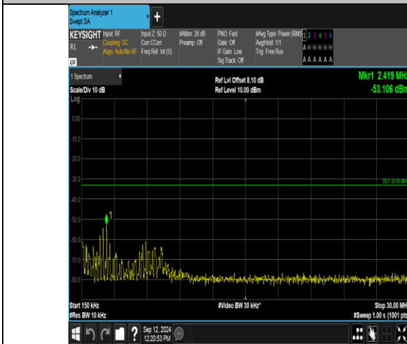
Band2_3MHz_16QAM_19185_1RB#14_0.15~30_0.15~30
