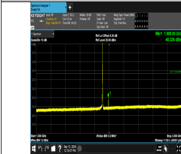
Band2_3MHz_16QAM_19185_1RB#0_1000~3000_1000~3000
