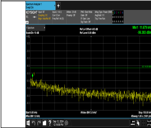
Band2_3MHz_QPSK_19185_1RB#14_0.009~0.15_0.009~0.15
