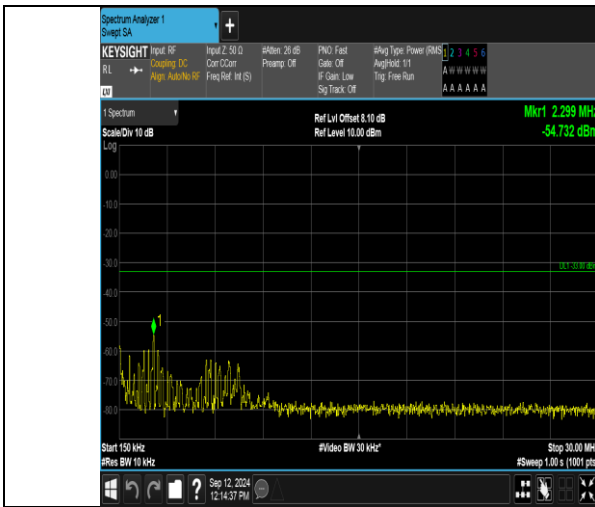
Band2_3MHz_16QAM_18900_1RB#0_0.15~30_0.15~30
