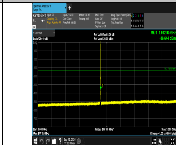
Band2_1.4MHz_QPSK_19193_6RB#0_1000-3000_1000-3000
