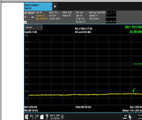
Band2_3MHz_QPSK_18900_15RB#0_30~1000_30~1000
