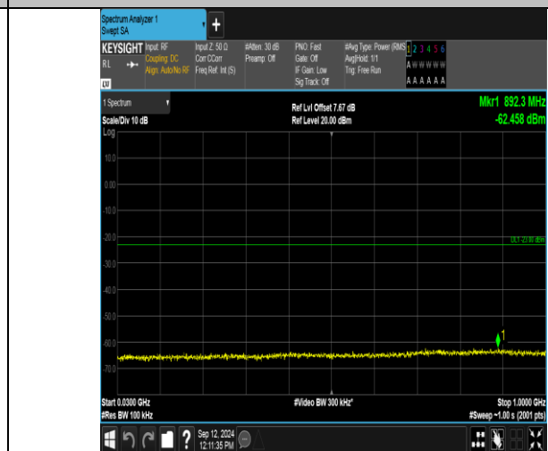
Band2_3MHz_16QAM_18615_1RB#14_30~1000_30~1000
