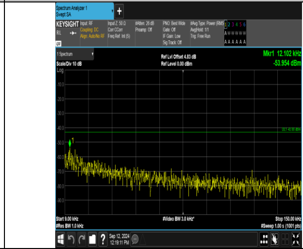
Band2_3MHz_16QAM_19185_1RB#0_0.009~0.15_0.009~0.15
