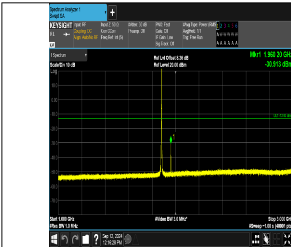
Band2_3MHz_16QAM_18900_1RB#14_1000~3000_1000~3000
