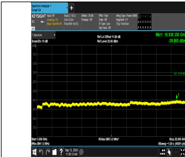
Band2_1.4MHz_QPSK_19193_6RB#0_3000~20000_3000~20000
