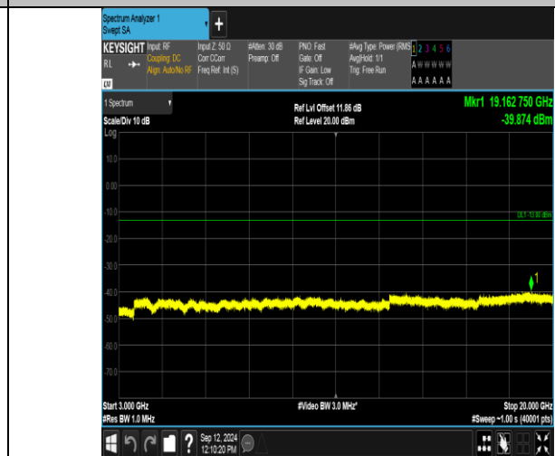
Band2_3MHz_16QAM_18615_1RB#0_3000~20000_3000~20000
