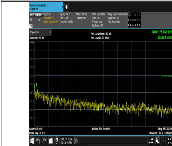
Band2_3MHz_QPSK_18900_1RB#14_0.009~0.15_0.009~0.15
