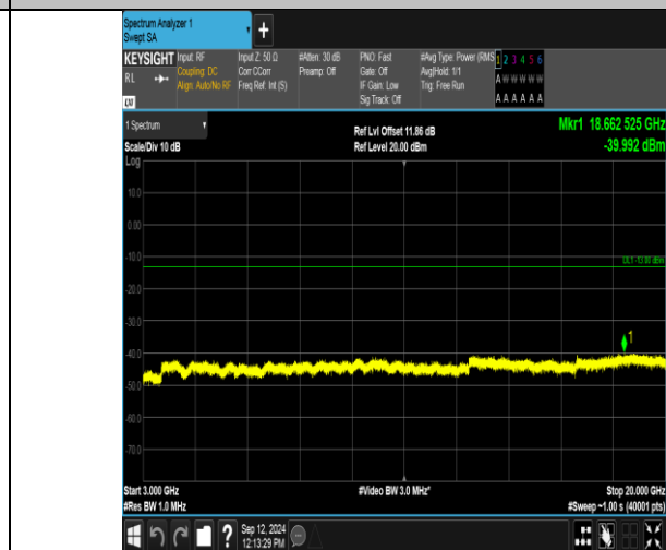
Band2_3MHz_16QAM_18615_15RB#0_3000~20000_3000~20000
