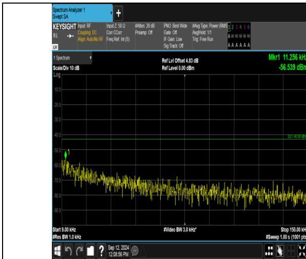
Band2_3MHz_QPSK_18615_1RB#0_0.009~0.15_0.009~0.15
