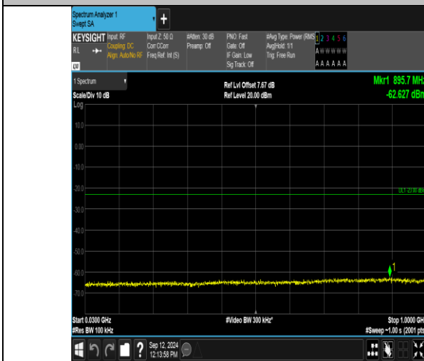
Band2_3MHz_QPSK_18900_1RB#0_30~1000_30~1000
