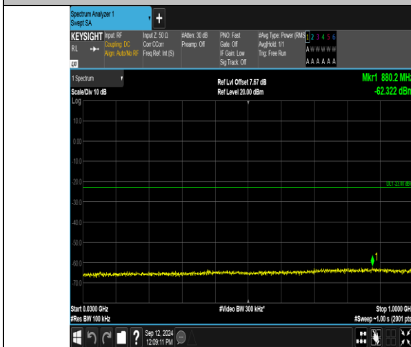
Band2_3MHz_QPSK_18615_1RB#0_30~1000_30~1000
