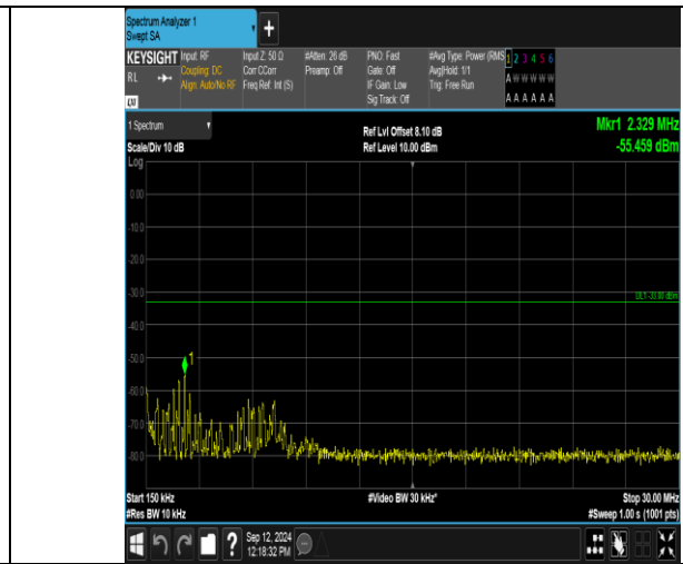
Band2_3MHz_QPSK_19185_1RB#0_0.15~30_0.15~30
