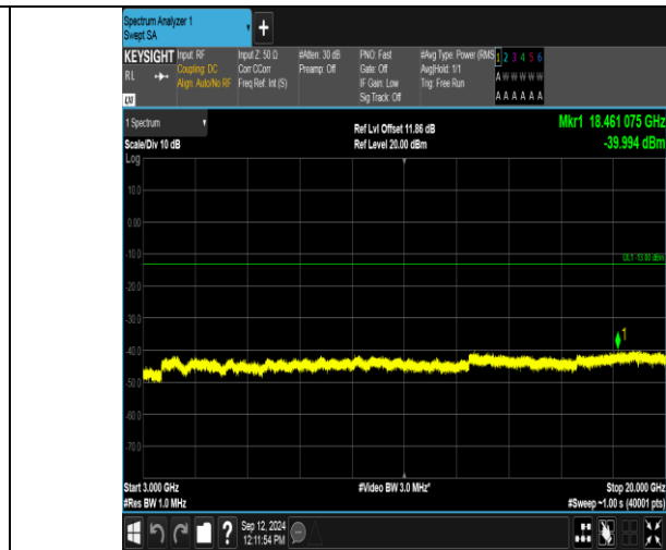
Band2_3MHz_16QAM_18615_1RB#14_3000~20000_3000~20000
