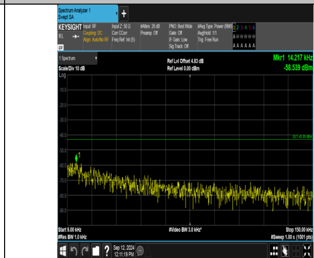
Band2_3MHz_16QAM_18615_1RB#14_0.009~0.15_0.009~0.15
