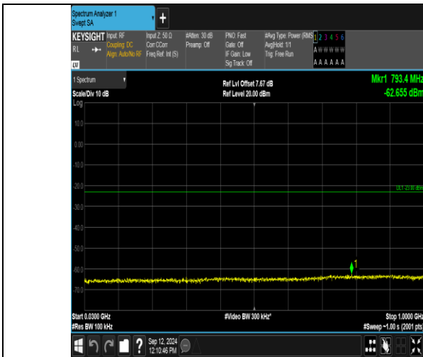
Band2_3MHz_QPSK_18615_1RB#14_30~1000_30~1000
