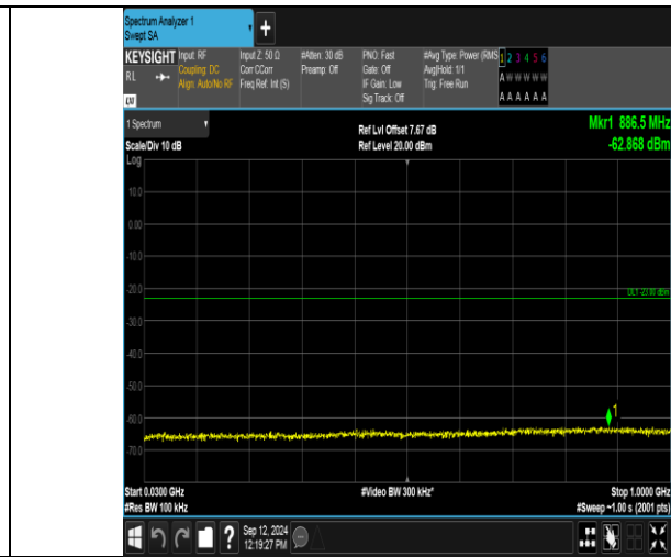
Band2_3MHz_16QAM_19185_1RB#0_30~1000_30~1000
