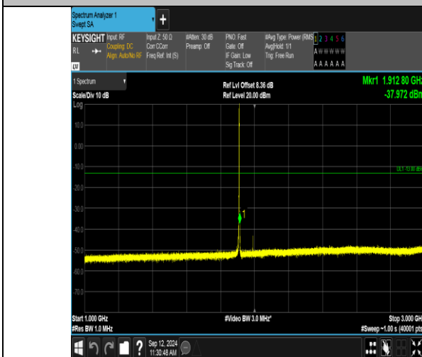
Band2_1.4MHz_16QAM_19193_6RB#0_1000~3000_1000~3000
