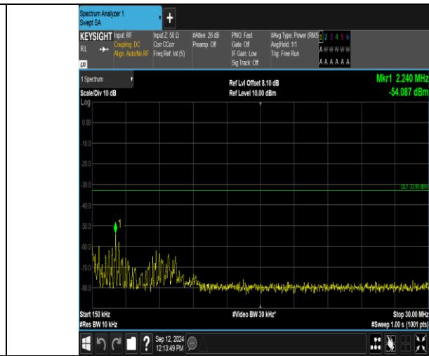
Band2_3MHz_QPSK_18900_1RB#0_0.15~30_0.15~30
