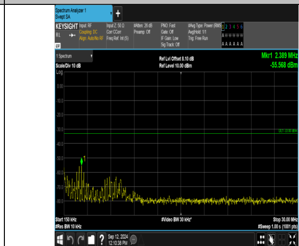
Band2_3MHz_QPSK_18615_1RB#14_0.15~30_0.15~30
