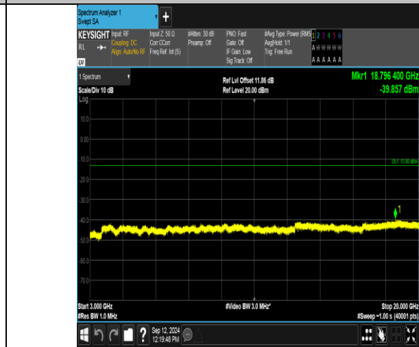
Band2_3MHz_16QAM_19185_1RB#0_3000~20000_3000~20000
