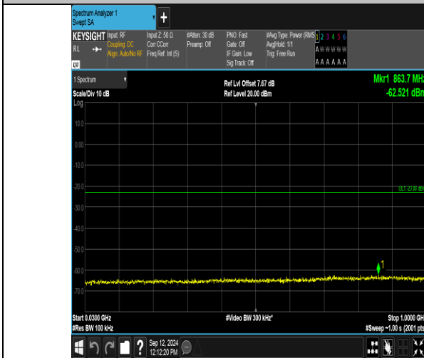
Band2_3MHz_QPSK_18615_15RB#0_30~1000_30~1000
