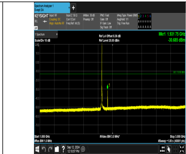
Band2_3MHz_QPSK_18615_1RB#14_1000~3000_1000~3000
