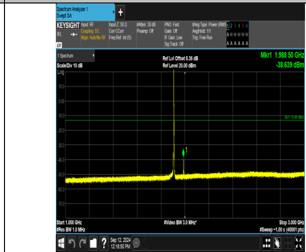
Band2_3MHz_QPSK_19185_1RB#0_1000~3000_1000~3000
