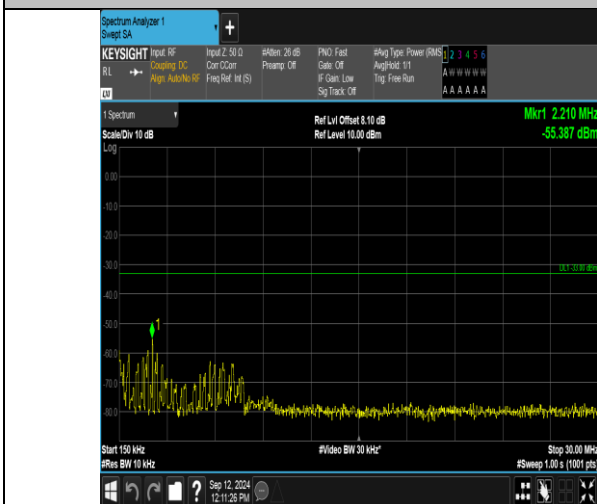
Band2_3MHz_16QAM_18615_1RB#14_0.15~30_0.15~30
