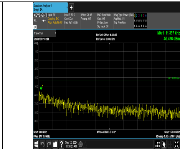
Band2_1.4MHz_16QAM_19193_6RB#0_0.009~0.15_0.009~0.15
