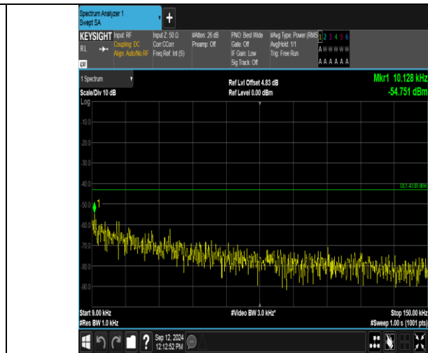
Band2_3MHz_16QAM_18615_15RB#0_0.009~0.15_0.009~0.15
