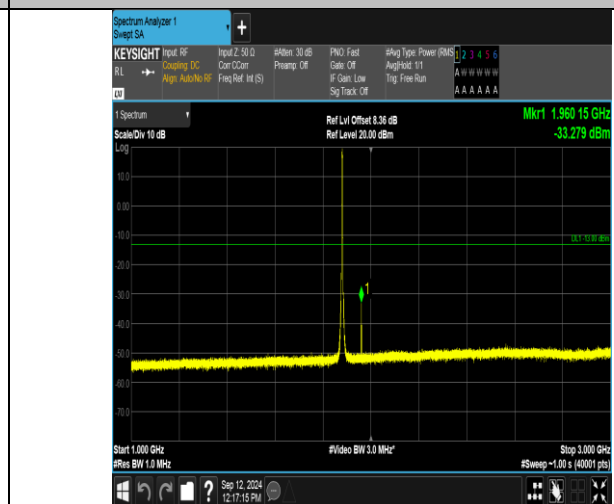
Band2_3MHz_QPSK_18900_15RB#0_1000~3000_1000~3000
