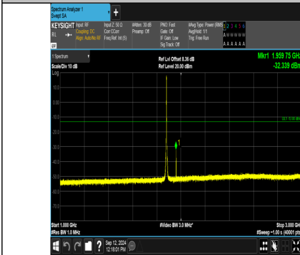
Band2_3MHz_16QAM_18900_15RB#0_1000-3000_1000-3000
