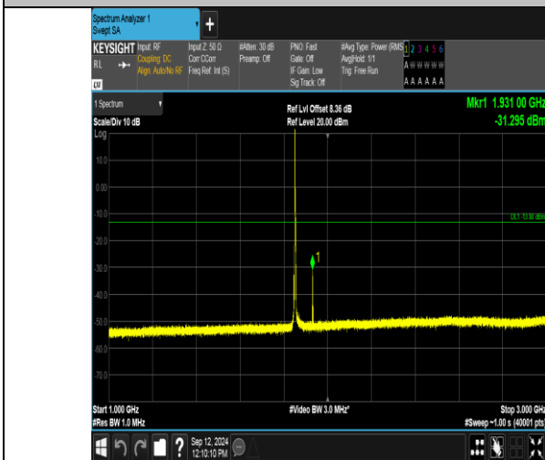
Band2_3MHz_16QAM_18615_1RB#0_1000~3000_1000~3000
