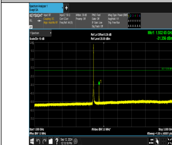
Band2_3MHz_16QAM_18615_15RB#0_1000~3000_1000~3000
