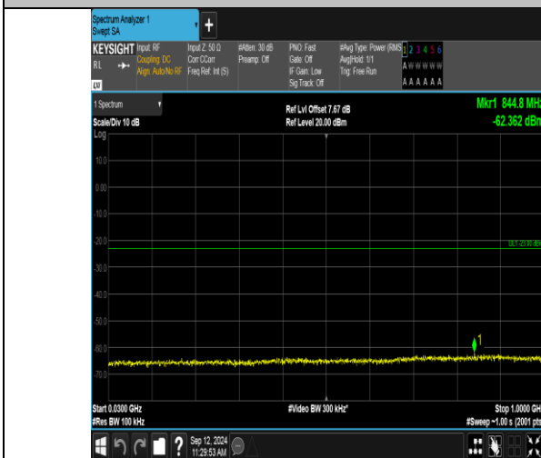
Band2_1.4MHz_QPSK_19193_6RB#0_30-1000_30-1000
