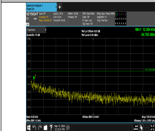
Band2_3MHz_QPSK_18615_1RB#14_0.009~0.15_0.009~0.15
