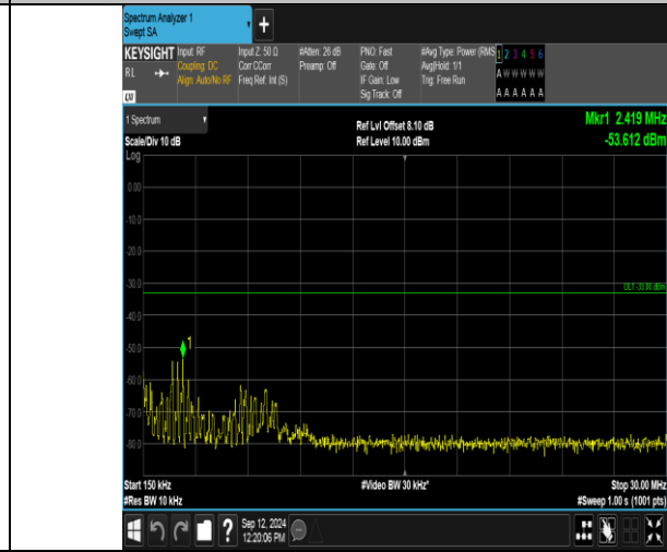
Band2_3MHz_QPSK_19185_1RB#14_0.15~30_0.15~30
