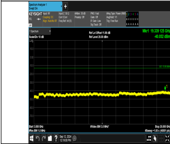
Band2_3MHz_QPSK_19185_1RB#0_3000~20000_3000~20000
