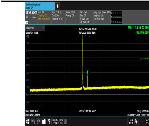
Band2_3MHz_16QAM_18900_1RB#0_1000~3000_1000~3000
