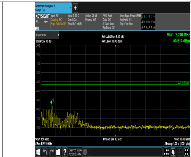
Band2_3MHz_QPSK_18615_1RB#0_0.15~30_0.15~30
