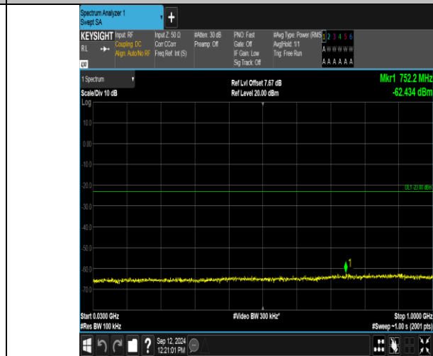
Band2_3MHz_16QAM_19185_1RB#14_30~1000_30~1000
