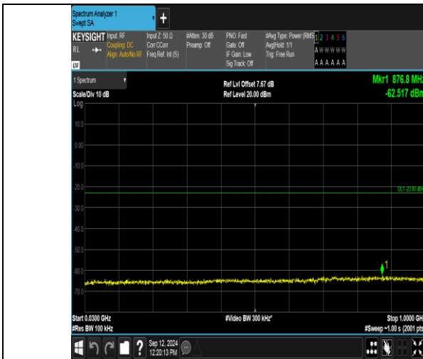
Band2_3MHz_QPSK_19185_1RB#14_30~1000_30~1000
