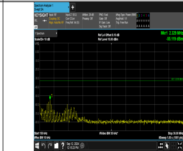
Band2_3MHz_QPSK_18900_1RB#14_0.15~30_0.15~30
