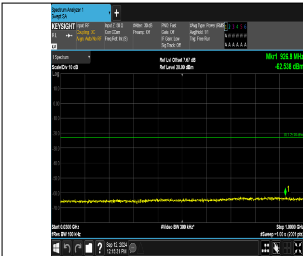
Band2_3MHz_QPSK_18900_1RB#14_30~1000_30~1000
