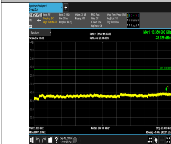
Band2_3MHz_QPSK_18615_1RB#14_3000~20000_3000~20000
