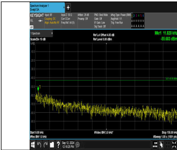
Band2_3MHz_QPSK_19185_1RB#0_0.009~0.15_0.009~0.15
