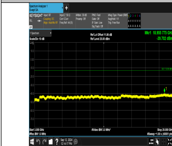
Band2_3MHz_QPSK_18900_1RB#0_3000~20000_3000~20000
