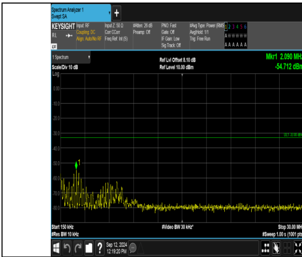
Band2_3MHz_16QAM_19185_1RB#0_0.15~30_0.15~30
