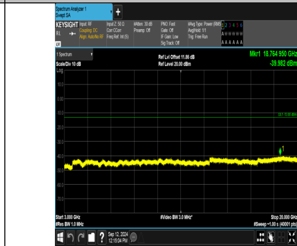
Band2_3MHz_16QAM_18900_1RB#0_3000~20000_3000~20000
