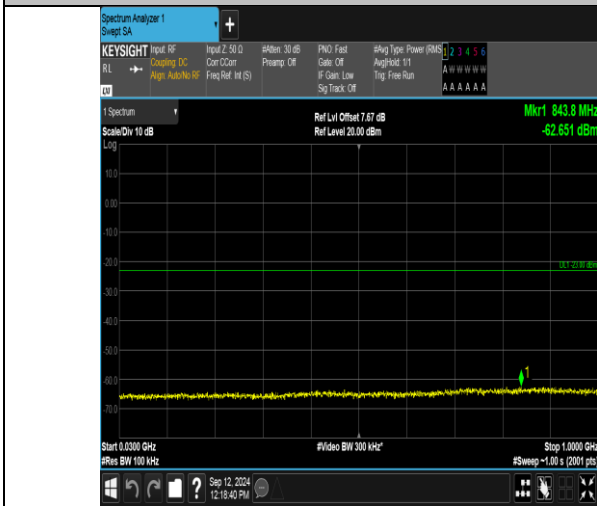
Band2_3MHz_QPSK_19185_1RB#0_30~1000_30~1000
