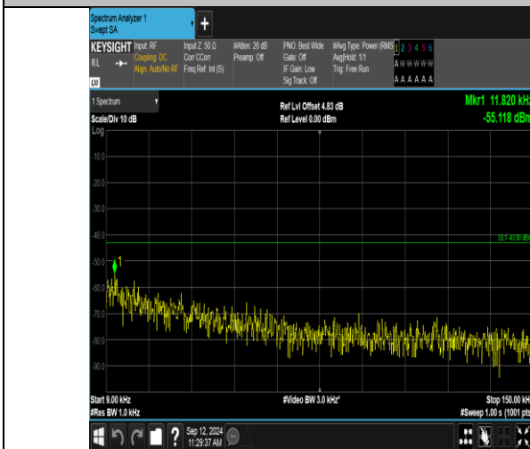
Band2_1.4MHz_QPSK_19193_6RB#0_0.009-0.15_0.009-0.15
