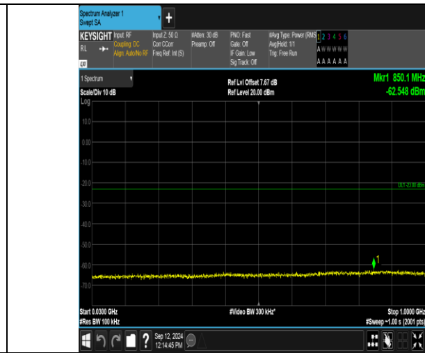
Band2_3MHz_16QAM_18900_1RB#0_30~1000_30~1000
