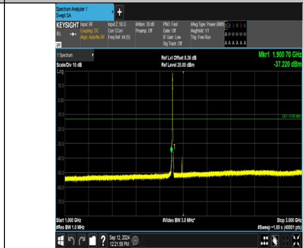
Band2_3MHz_QPSK_19185_15RB#0_1000~3000_1000~3000
