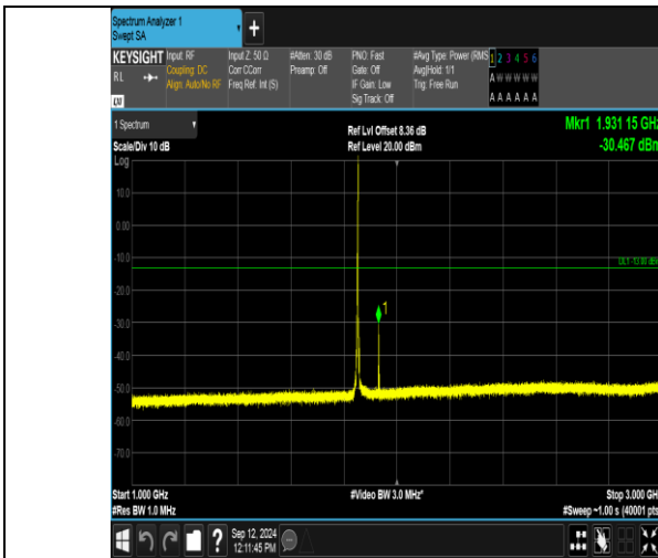
Band2_3MHz_16QAM_18615_1RB#14_1000~3000_1000~3000
