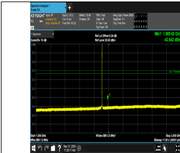
Band2_1.4MHz_16QAM_19193_1RB#5_1000-3000_1000-3000
