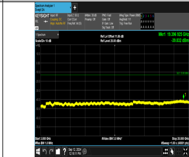
Band2_3MHz_16QAM_18900_15RB#0_3000-20000_3000-20000
