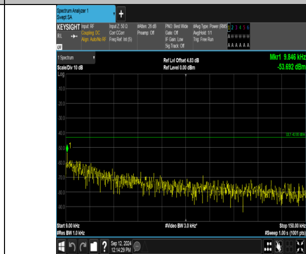
Band2_3MHz_16QAM_18900_1RB#0_0.009~0.15_0.009~0.15
