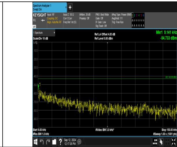
Band2_3MHz_16QAM_18900_15RB#0_0.009-0.15_0.009-0.15
