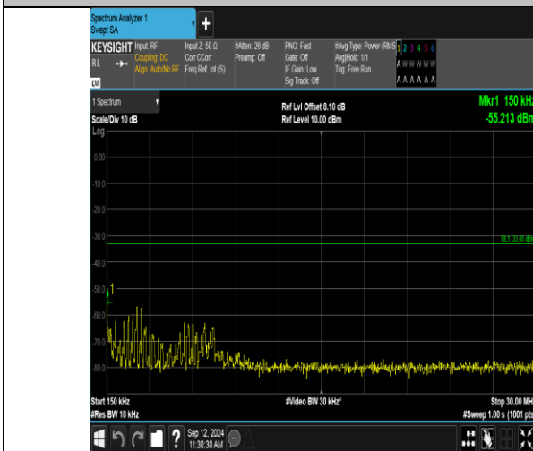
Band2_1.4MHz_16QAM_19193_6RB#0_0.15~30_0.15~30
