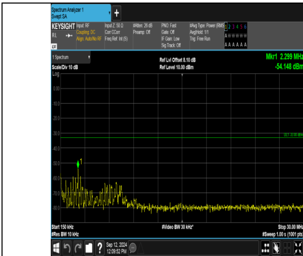
Band2_3MHz_16QAM_18615_1RB#0_0.15~30_0.15~30
