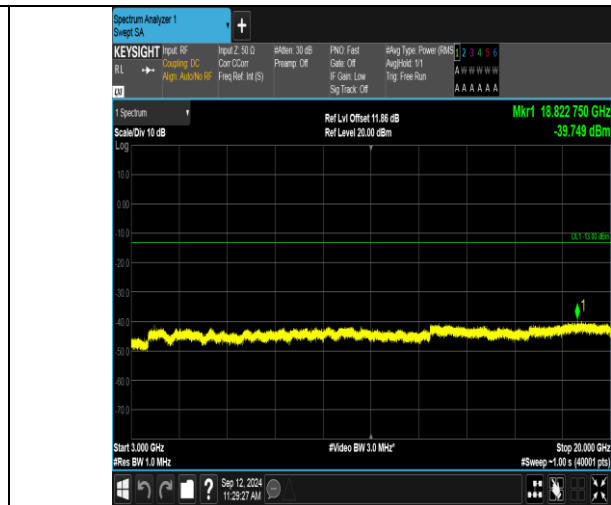
Band2_1.4MHz_16QAM_19193_1RB#5_3000-20000_3000-20000
