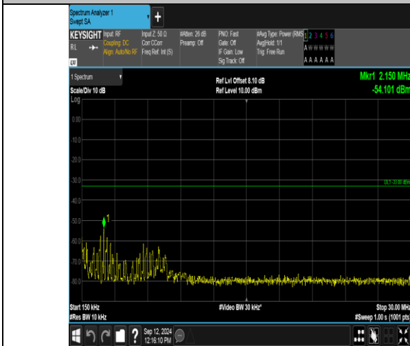
Band2_3MHz_16QAM_18900_1RB#14_0.15~30_0.15~30
