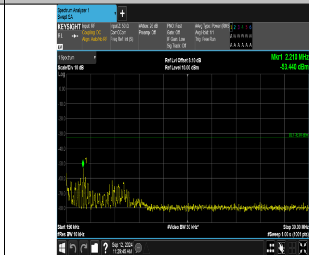
Band2_1.4MHz_QPSK_19193_6RB#0_0.15-30_0.15-30
