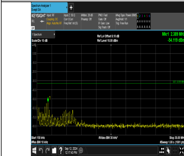
Band2_3MHz_16QAM_18900_15RB#0_0.15-30_0.15-30
