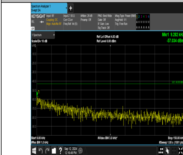
Band2_3MHz_QPSK_18900_15RB#0_0.009~0.15_0.009~0.15
