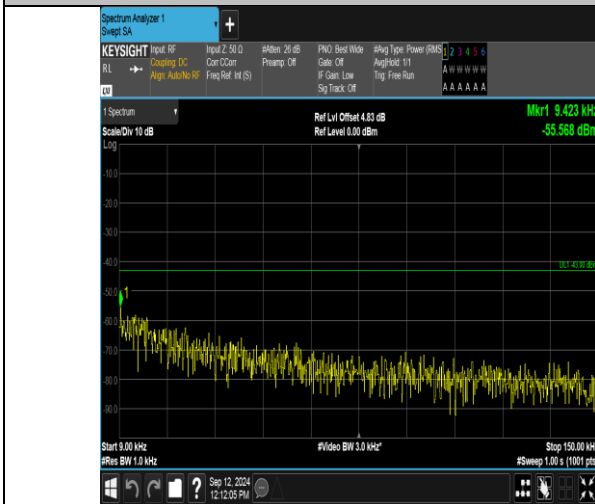
Band2_3MHz_QPSK_18615_15RB#0_0.009~0.15_0.009~0.15
