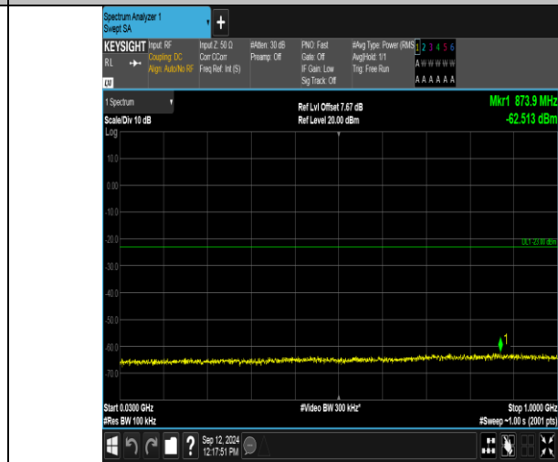
Band2_3MHz_16QAM_18900_15RB#0_30-1000_30-1000
