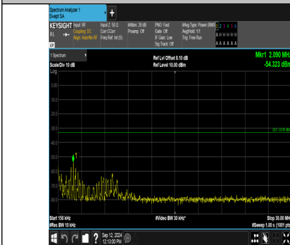
Band2_3MHz_16QAM_18615_15RB#0_0.15~30_0.15~30
