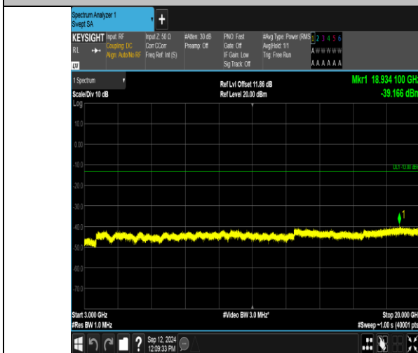
Band2_3MHz_QPSK_18615_1RB#0_3000~20000_3000~20000
