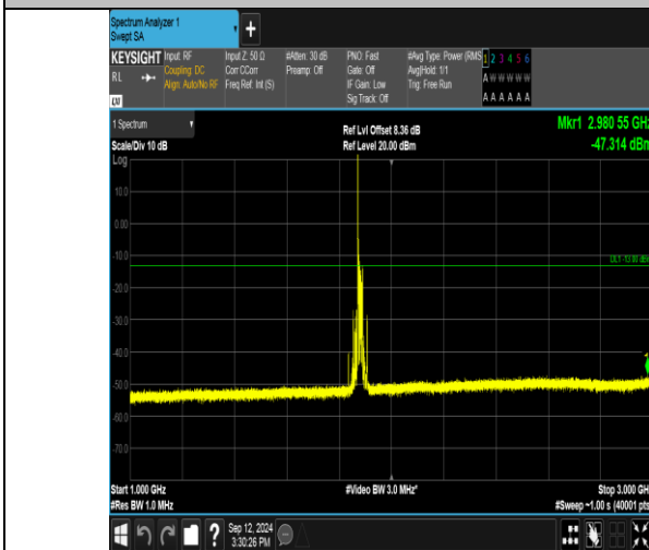
Band_20MHz_16QAM_18900_1RB#0_1000~3000_1000~3000
