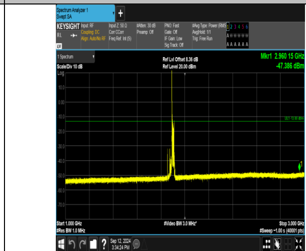
Band2_20MHz_QPSK_19100_1RB#0_1000~3000_1000~3000
