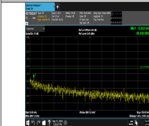
Band_20MHz_QPSK_18900_1RB#99_0.009~0.15_0.009~0.15
