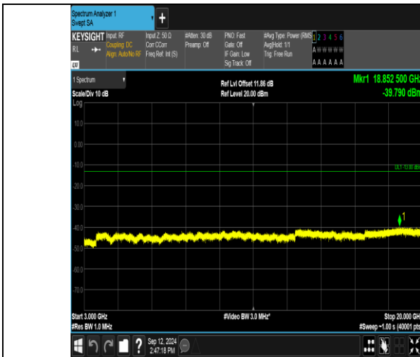
Band2_15MHz_QPSK_19125_75RB#0_3000~20000_3000~20000
