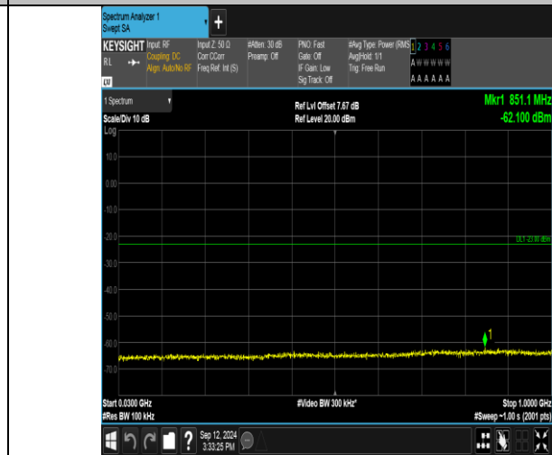
Band2_20MHz_16QAM_18900_100RB#0_30~1000_30~1000
