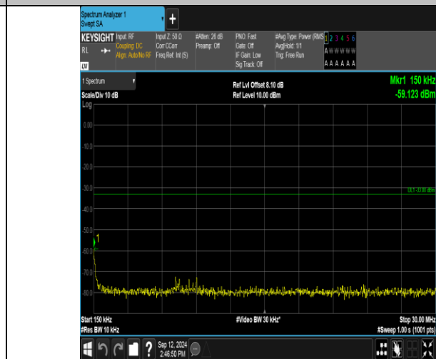
Band2_15MHz_QPSK_19125_75RB#0_0.15-30_0.15-30
