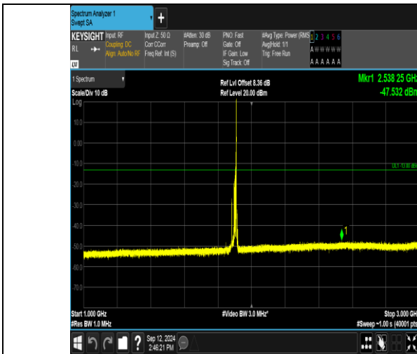
Band2_15MHz_16QAM_19125_1RB#74_1000-3000_1000-3000
