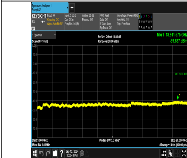
Band2_20MHz_QPSK_18700_1RB#0_3000~20000_3000~20000
