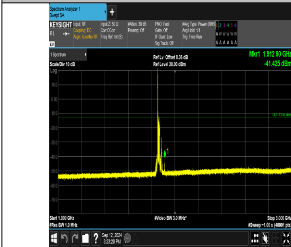
Band_2_20MHz_16QAM_18700_1RB#0_1000~3000_1000~3000
