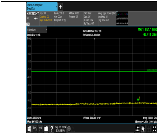
Band2_20MHz_QPSK_19100_1RB#99_30~1000_30~1000
