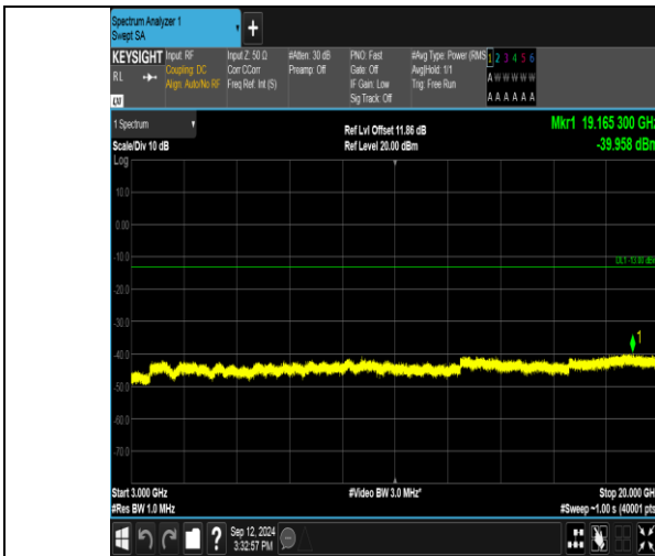
Band2_20MHz_QPSK_18900_100RB#0_3000~20000_3000~20000
