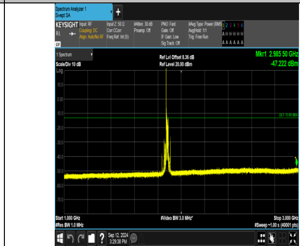
Band2_20MHz_QPSK_18900_1RB#0_1000~3000_1000~3000
