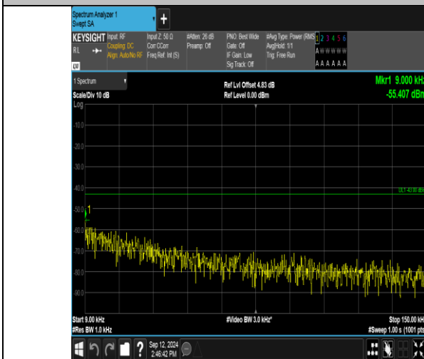
Band2_15MHz_QPSK_19125_75RB#0_0.009-0.15_0.009-0.15
