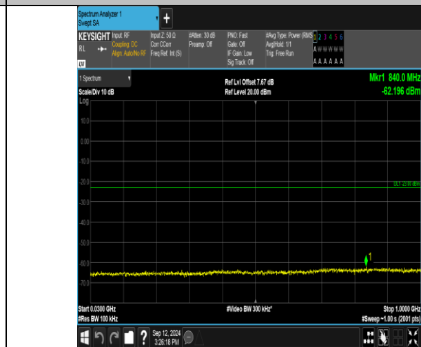
Band2_20MHz_16QAM_18700_100RB#0_30~1000_30~1000
