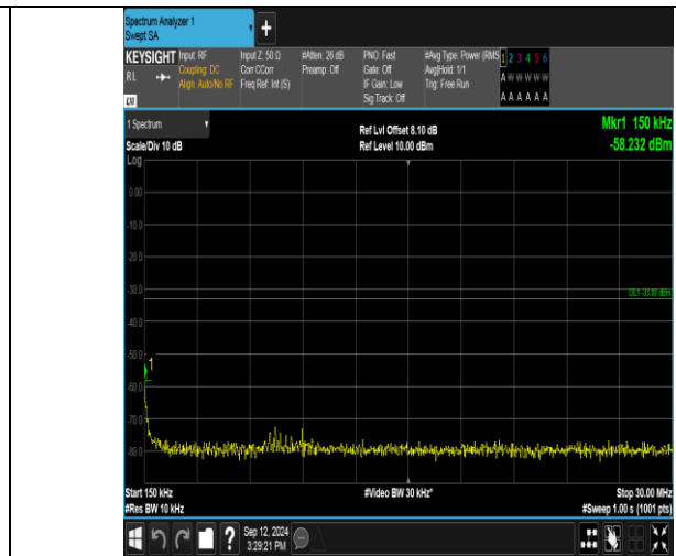
Band2_20MHz_QPSK_18900_1RB#0_0.15~30_0.15~30
