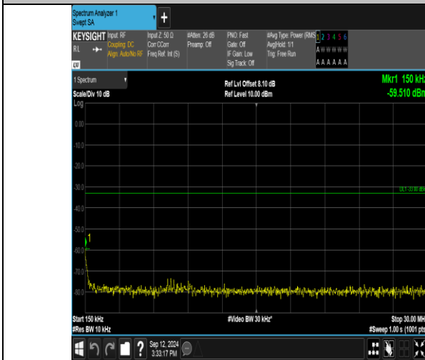
Band2_20MHz_16QAM_18900_100RB#0_0.15~30_0.15~30
