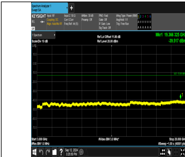
Band2_20MHz_QPSK_18700_100RB#0_3000~20000_3000~20000
