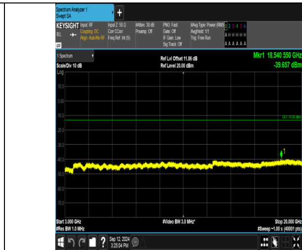
Band2_20MHz_16QAM_18700_1RB#99_3000~20000_3000~20000
