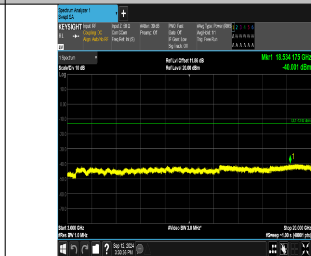
Band2_20MHz_16QAM_18900_1RB#0_3000~20000_3000~20000
