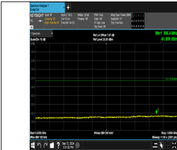
Band2_20MHz_QPSK_18900_1RB#99_30~1000_30~1000
