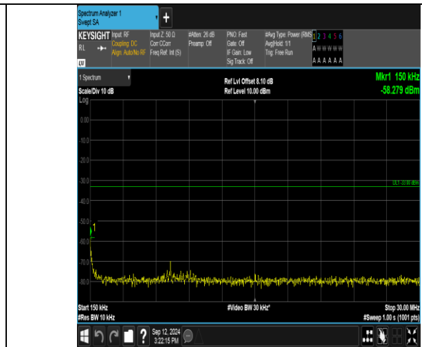
Band2_20MHz_QPSK_18700_1RB#0_0.15~30_0.15~30
