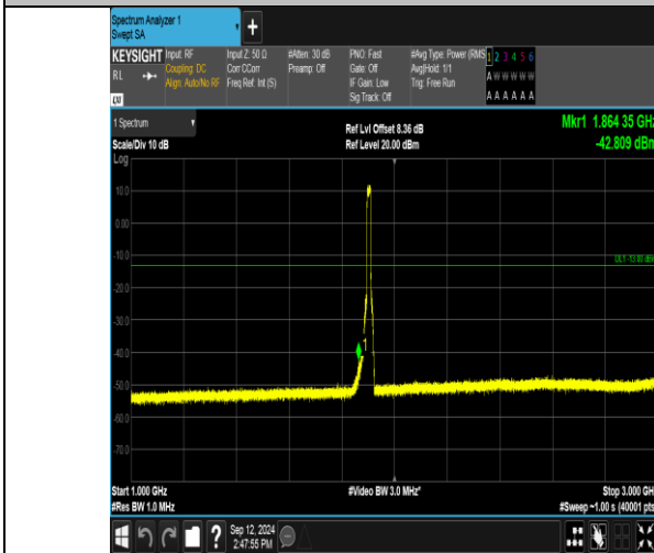
Band2_15MHz_16QAM_19125_75RB#0_1000~3000_1000~3000
