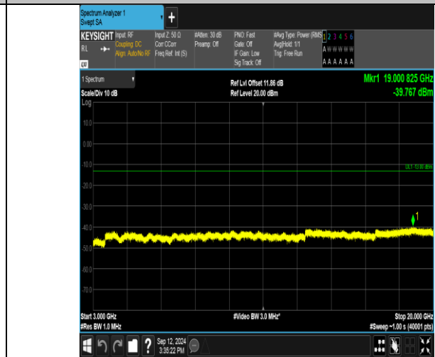
Band2_20MHz_16QAM_19100_1RB#0_3000~20000_3000~20000
