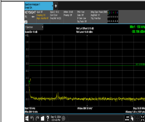
Band2_20MHz_16QAM_18900_1RB#99_0.15~30_0.15~30
