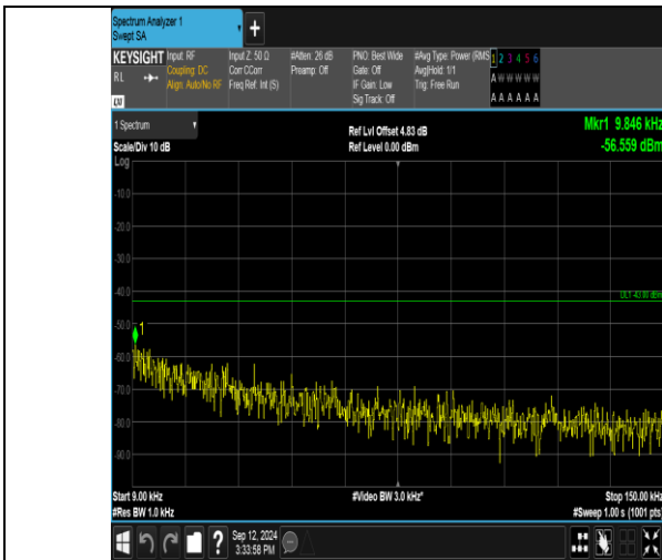
Band2_20MHz_QPSK_19100_1RB#0_0.009~0.15_0.009~0.15
