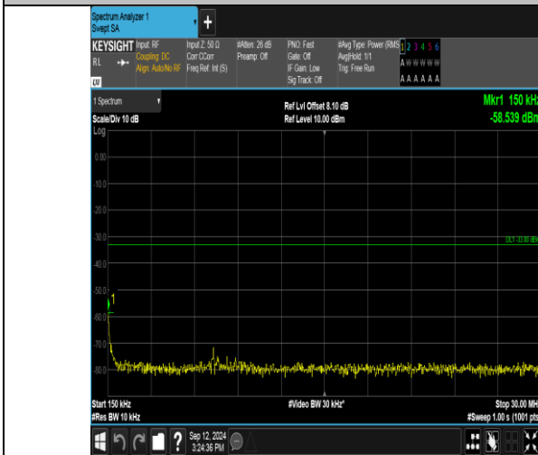
Band2_20MHz_16QAM_18700_1RB#99_0.15~30_0.15~30
