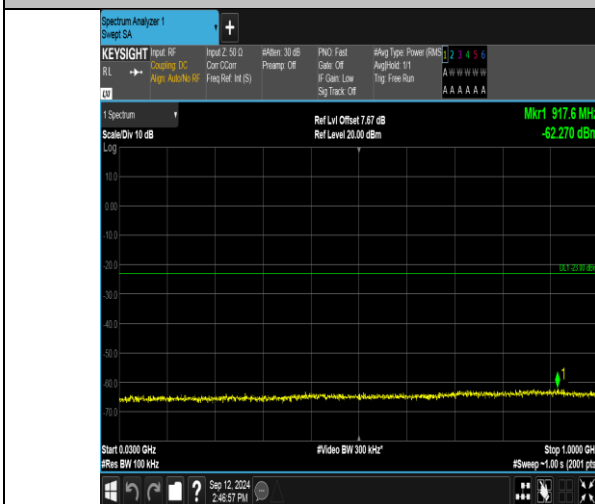
Band2_15MHz_QPSK_19125_75RB#0_30-1000_30-1000
