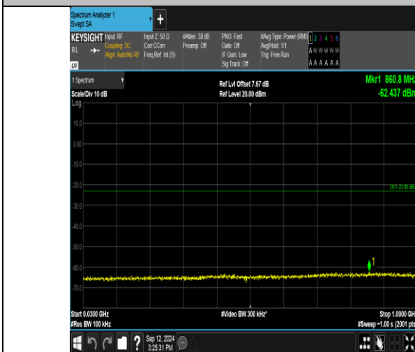
Band2_20MHz_QPSK_18700_100RB#0_30~1000_30~1000
