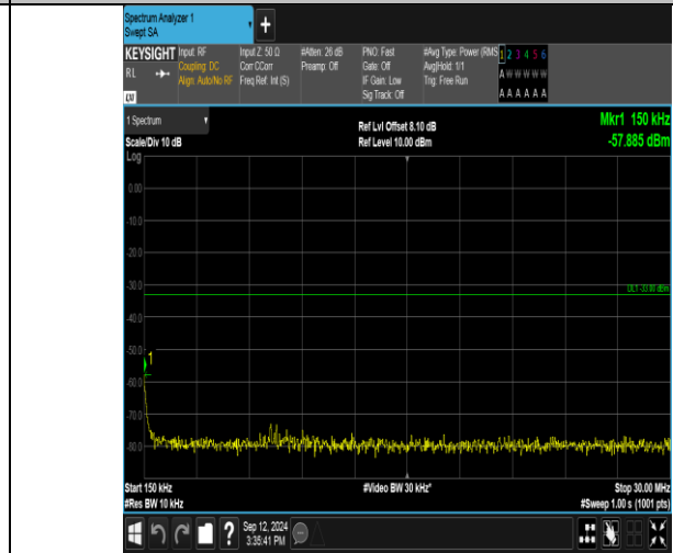
Band_20MHz_QPSK_19100_1RB#99_0.15~30_0.15~30
