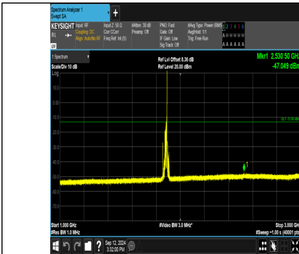
Band2_20MHz_16QAM_18900_1RB#99_1000~3000_1000~3000
