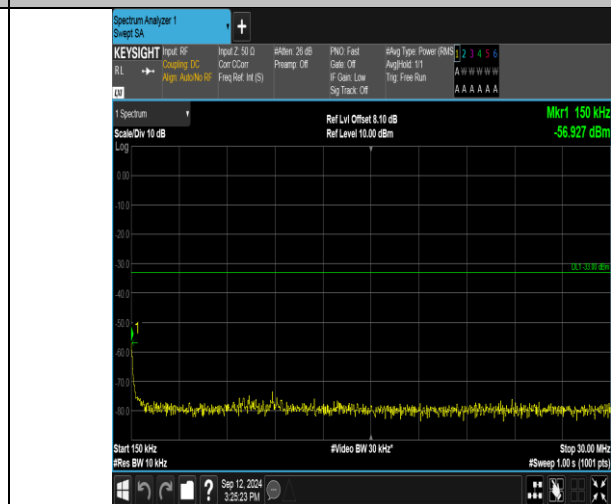
Band2_20MHz_QPSK_18700_100RB#0_0.15~30_0.15~30
