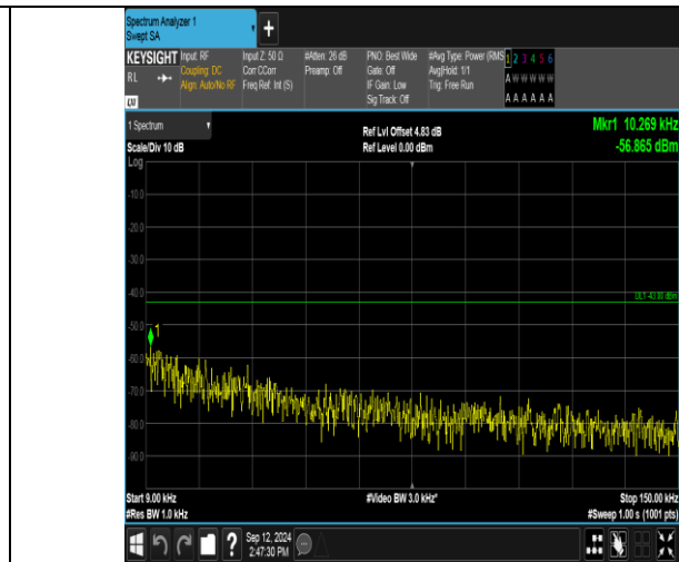
Band2_15MHz_16QAM_19125_75RB#0_0.009~0.15_0.009~0.15
