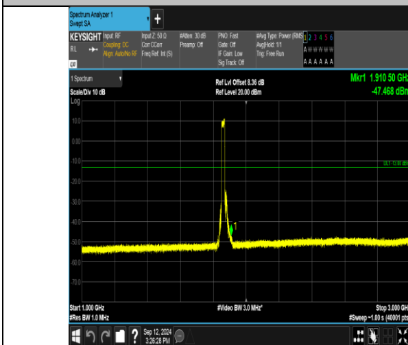
Band2_20MHz_16QAM_18700_100RB#0_1000~3000_1000~3000
