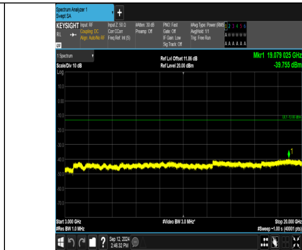
Band2_15MHz_16QAM_19125_1RB#74_3000-20000_3000-20000
