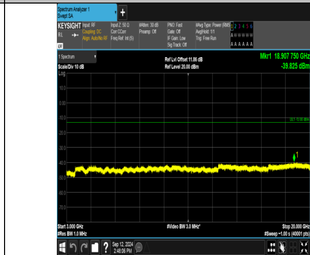
Band2_15MHz_16QAM_19125_75RB#0_3000~20000_3000~20000
