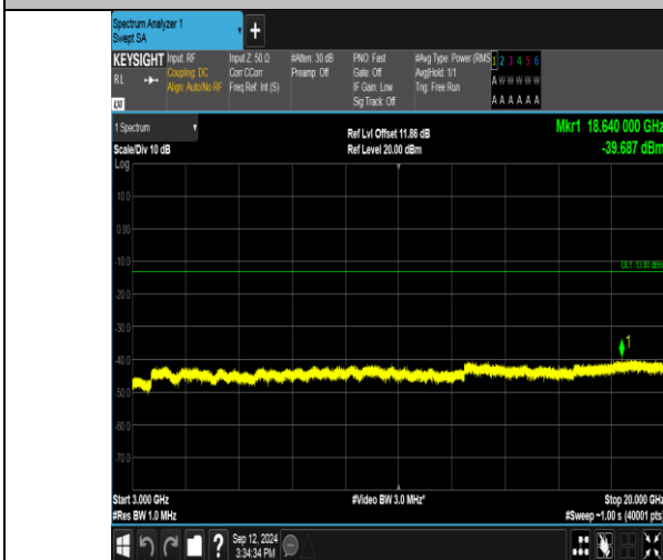
Band2_20MHz_QPSK_19100_1RB#0_3000~20000_3000~20000
