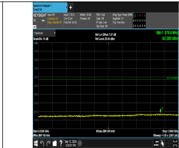
Band2_20MHz_16QAM_19100_1RB#0_30~1000_30~1000
