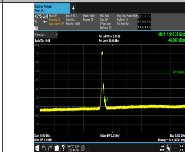
Band2_20MHz_QPSK_18700_100RB#0_1000~3000_1000~3000
