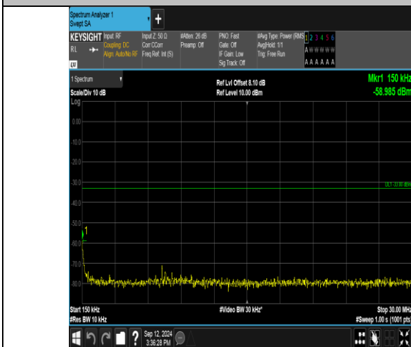
Band2_20MHz_16QAM_19100_1RB#99_0.15~30_0.15~30
