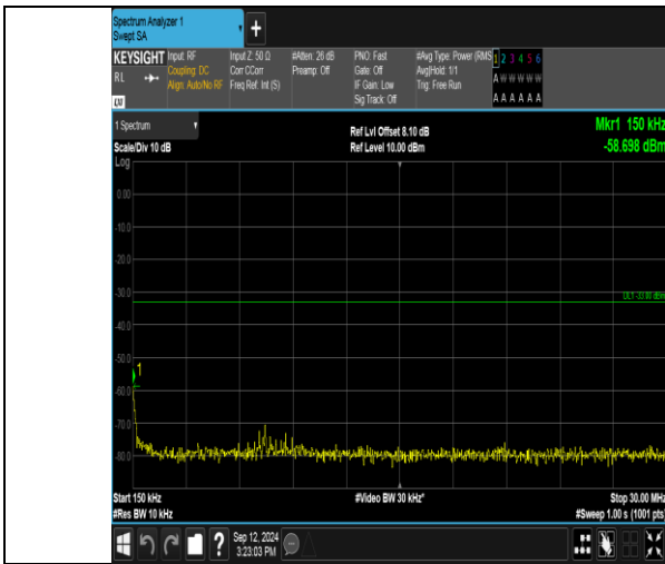
Band_2_20MHz_16QAM_18700_1RB#0_0.15~30_0.15~30
