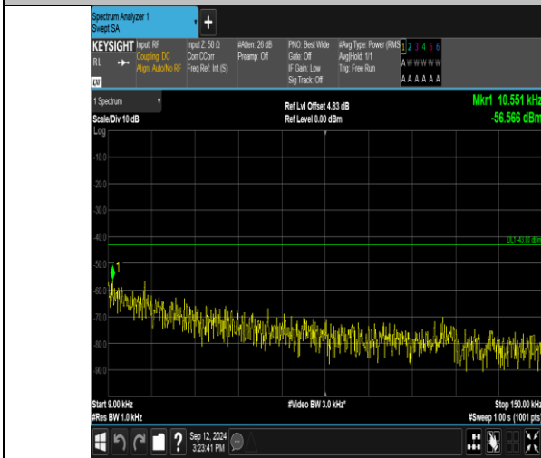
Band_2_20MHz_QPSK_18700_1RB#99_0.009~0.15_0.009~0.15
