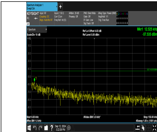
Band2_20MHz_QPSK_18700_1RB#0_0.009~0.15_0.009~0.15
