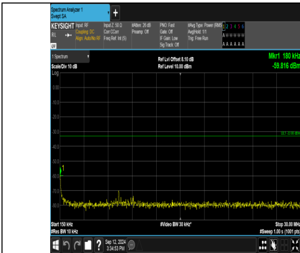
Band_20MHz_16QAM_19100_1RB#0_0.15~30_0.15~30
