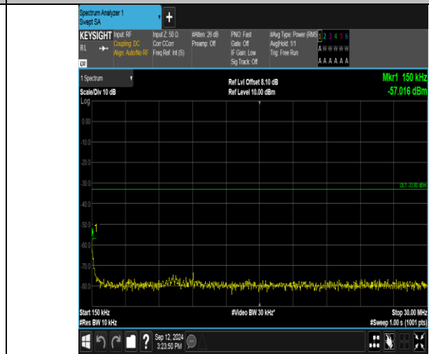
Band_2_20MHz_QPSK_18700_1RB#99_0.15~30_0.15~30
