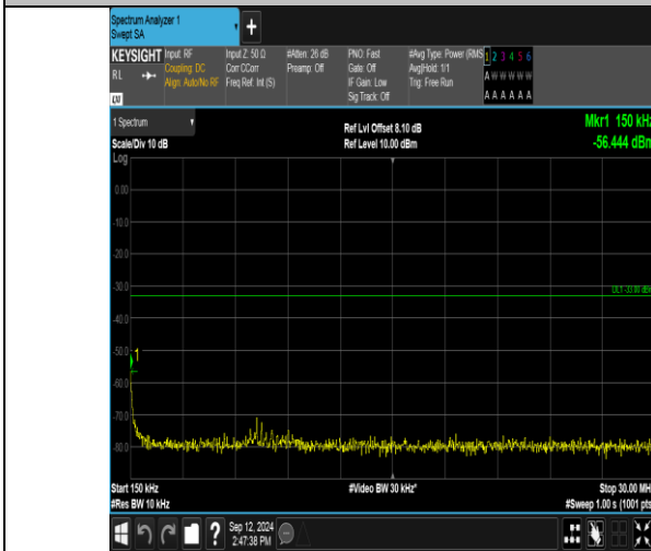
Band2_15MHz_16QAM_19125_75RB#0_0.15~30_0.15~30
