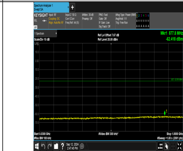
Band2_15MHz_16QAM_19125_75RB#0_30~1000_30~1000
