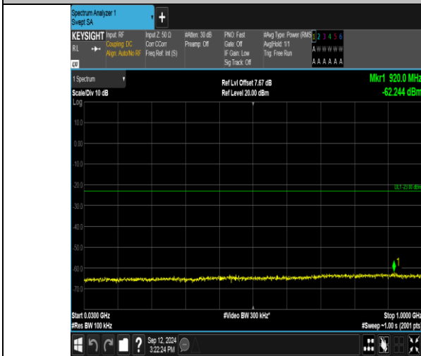
Band2_20MHz_QPSK_18700_1RB#0_30~1000_30~1000
