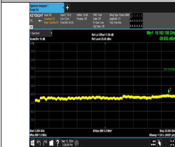
Band2_20MHz_QPSK_19100_1RB#99_3000~20000_3000~20000
