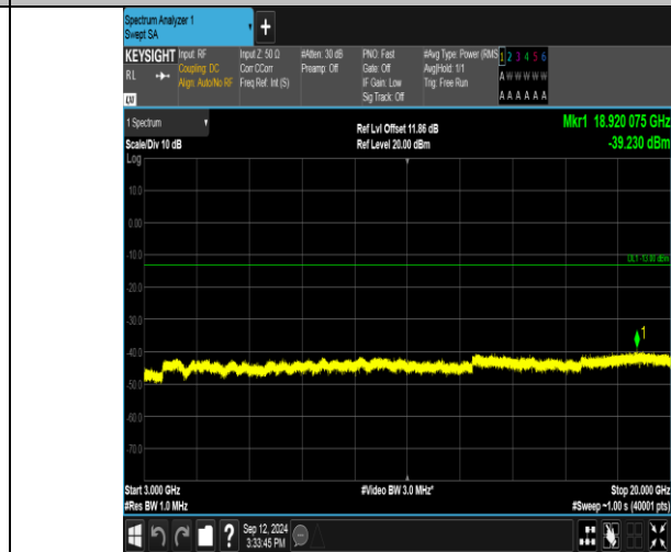
Band2_20MHz_16QAM_18900_100RB#0_3000~20000_3000~20000
