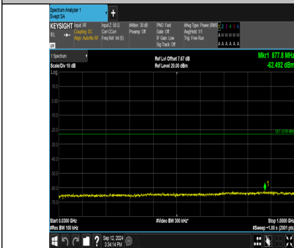
Band2_20MHz_QPSK_19100_1RB#0_30~1000_30~1000
