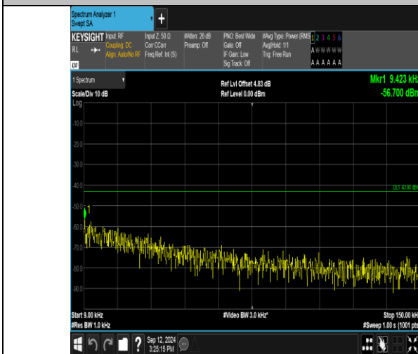
Band2_20MHz_QPSK_18700_100RB#0_0.009~0.15_0.009~0.15
