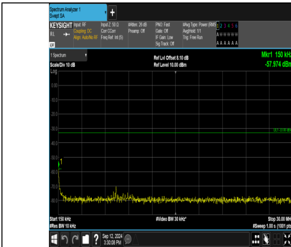
Band_20MHz_16QAM_18900_1RB#0_0.15~30_0.15~30
