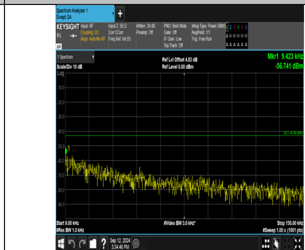
Band2_20MHz_16QAM_19100_1RB#0_0.009~0.15_0.009~0.15
