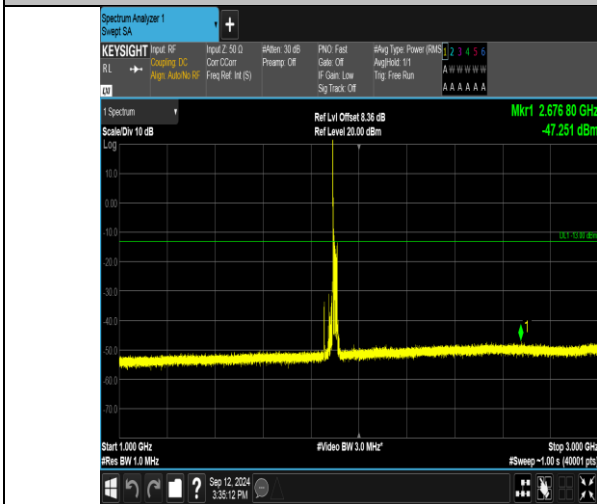
Band_20MHz_16QAM_19100_1RB#0_1000~3000_1000~3000
