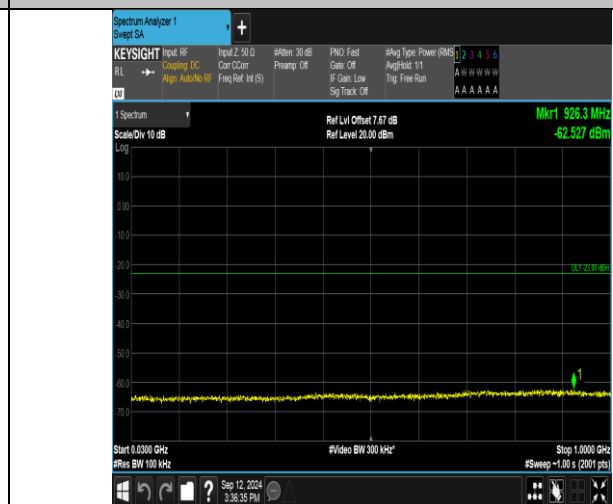
Band2_20MHz_16QAM_19100_1RB#99_30~1000_30~1000
