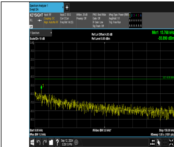
Band2_20MHz_QPSK_18900_1RB#0_0.009~0.15_0.009~0.15
