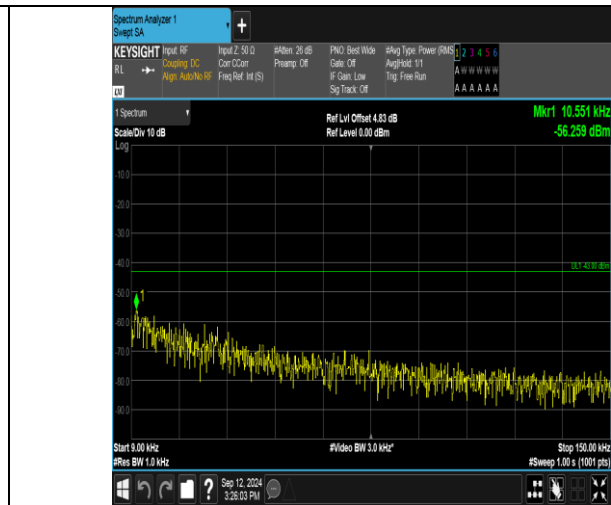
Band2_20MHz_16QAM_18700_100RB#0_0.009~0.15_0.009~0.15
