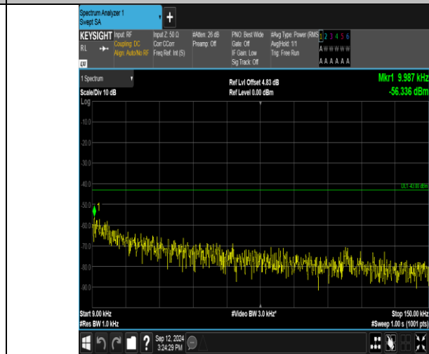
Band2_20MHz_16QAM_18700_1RB#99_0.009~0.15_0.009~0.15
