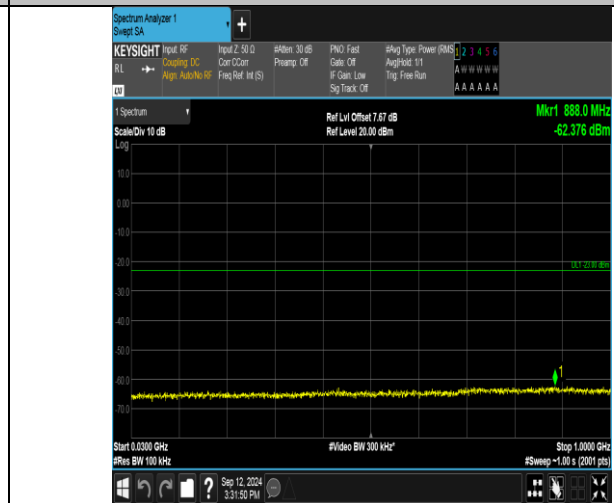
Band2_20MHz_16QAM_18900_1RB#99_30~1000_30~1000
