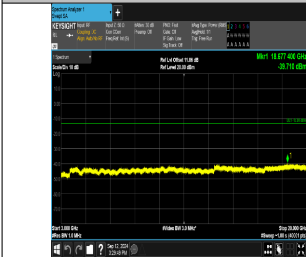
Band2_20MHz_QPSK_18900_1RB#0_3000~20000_3000~20000
