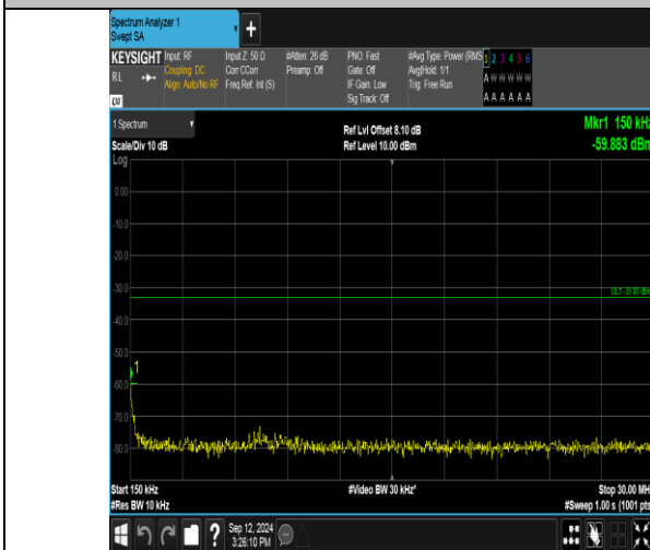
Band2_20MHz_16QAM_18700_100RB#0_0.15~30_0.15~30
