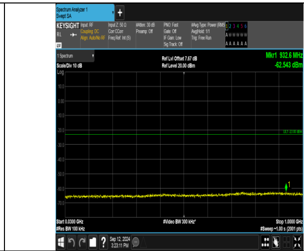
Band2_20MHz_16QAM_18700_1RB#0_30~1000_30~1000
