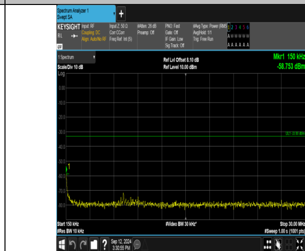
Band_20MHz_QPSK_18900_1RB#99_0.15~30_0.15~30
