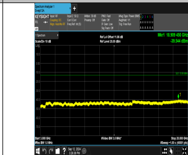
Band2_20MHz_16QAM_18700_100RB#0_3000~20000_3000~20000
