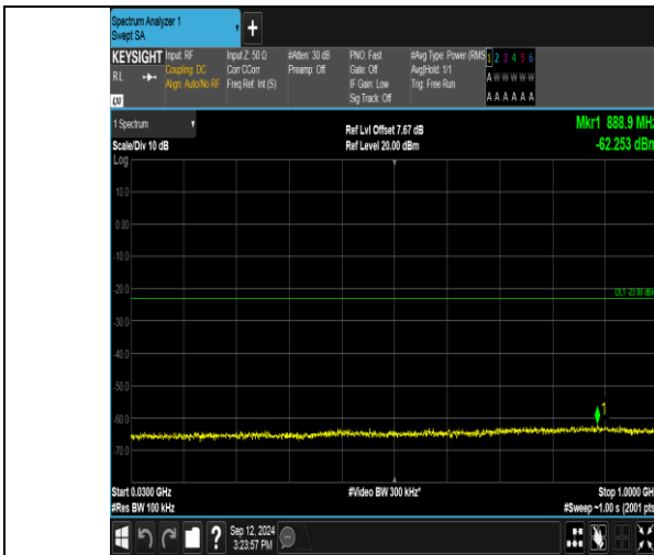
Band2_20MHz_QPSK_18700_1RB#99_30~1000_30~1000
