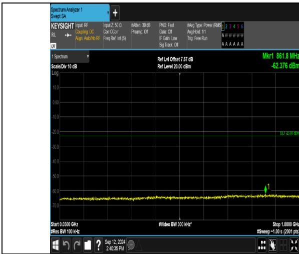
Band2_15MHz_QPSK_18900_1RB#74_30~1000_30~1000
