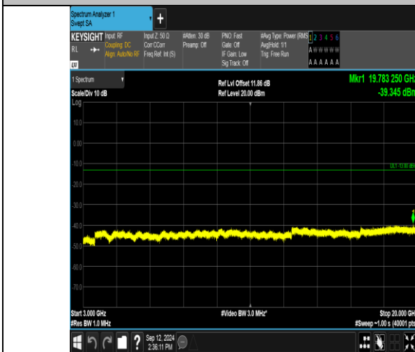
Band2_15MHz_QPSK_18675_1RB#74_3000~20000_3000~20000
