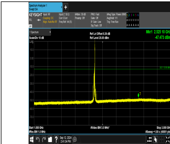
Band2_15MHz_16QAM_18900_1RB#74_1000-3000_1000-3000
