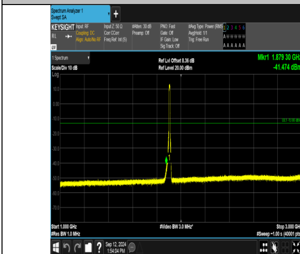
Band2_10MHz_16QAM_19150_50RB#0_1000~3000_1000~3000
