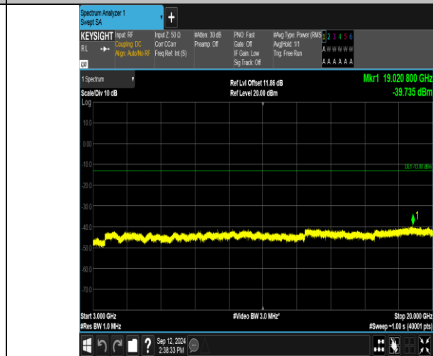
Band2_15MHz_16QAM_18675_75RB#0_3000~20000_3000~20000
