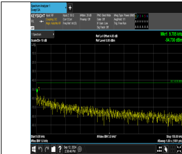
Band2_15MHz_QPSK_18900_1RB#0_0.009~0.15_0.009~0.15
