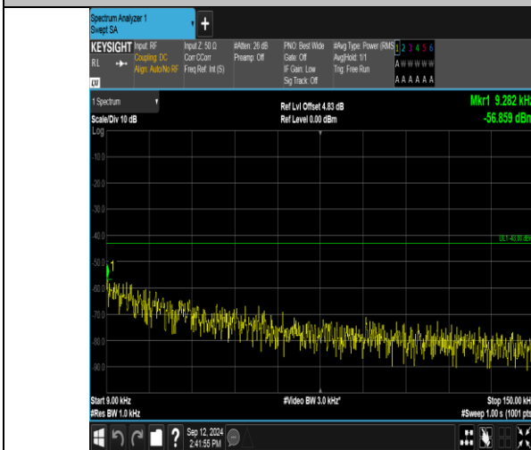
Band2_15MHz_QPSK_18900_75RB#0_0.009-0.15_0.009-0.15
