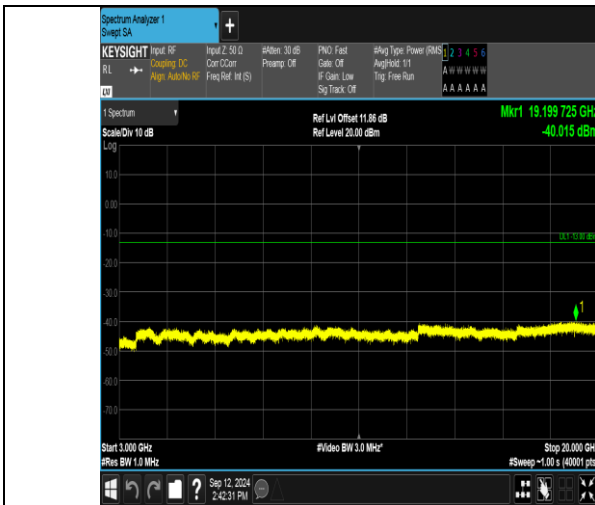
Band2_15MHz_QPSK_18900_75RB#0_3000~20000_3000~20000
