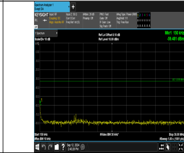
Band2_15MHz_QPSK_18900_1RB#74_0.15~30_0.15~30
