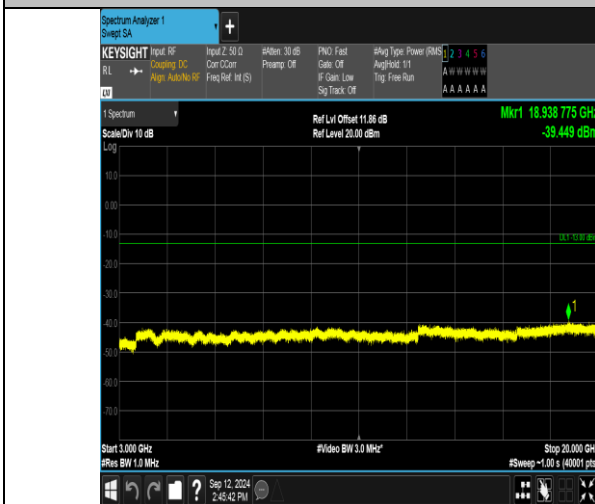
Band2_15MHz_QPSK_19125_1RB#74_3000~20000_3000~20000
