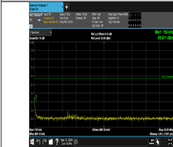
Band2_15MHz_16QAM_18900_1RB#74_0.15~30_0.15~30
