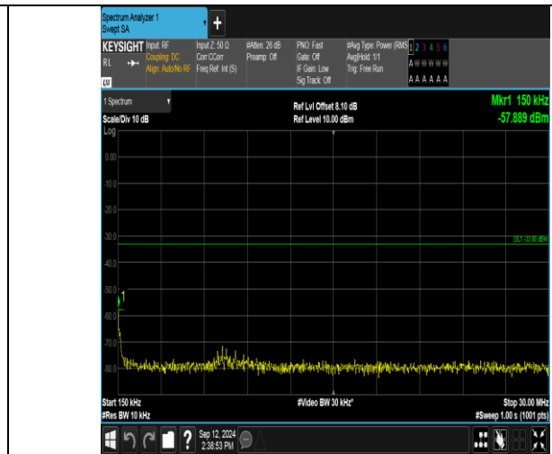
Band2_15MHz_QPSK_18900_1RB#0_0.15~30_0.15~30
