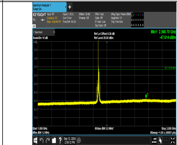
Band2_15MHz_QPSK_18900_1RB#0_1000~3000_1000~3000
