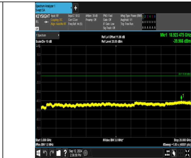
Band2_15MHz_16QAM_18675_1RB#74_3000-20000_3000-20000
