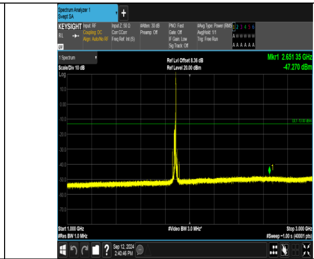
Band2_15MHz_QPSK_18900_1RB#74_1000~3000_1000~3000
