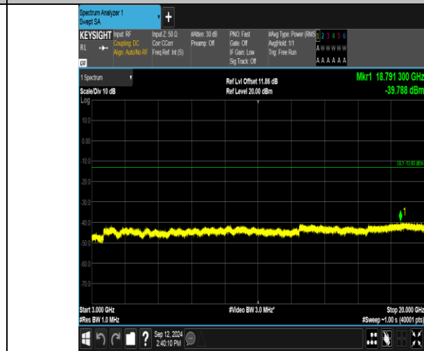
Band2_15MHz_16QAM_18900_1RB#0_3000~20000_3000~20000
