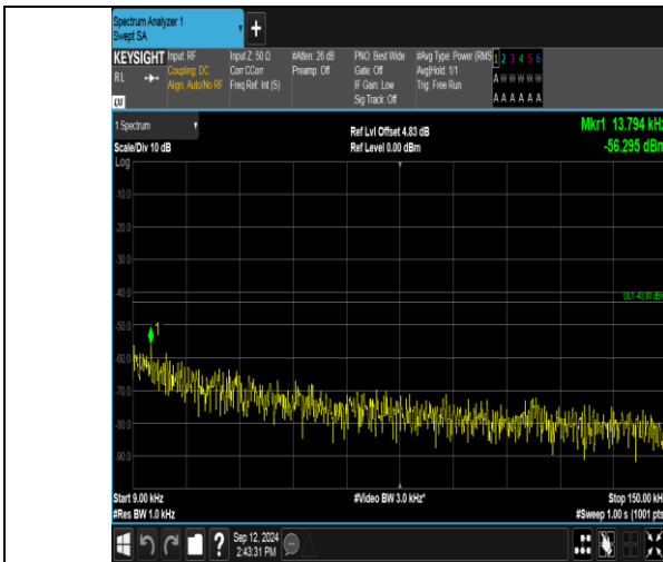
Band2_15MHz_QPSK_19125_1RB#0_0.009~0.15_0.009~0.15
