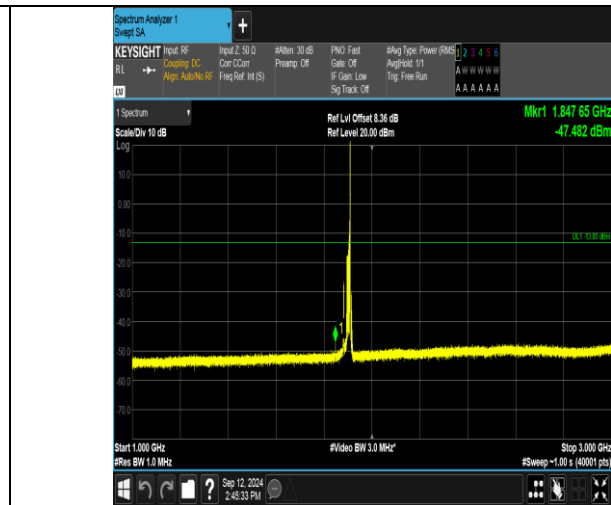
Band2_15MHz_QPSK_19125_1RB#74_1000~3000_1000~3000
