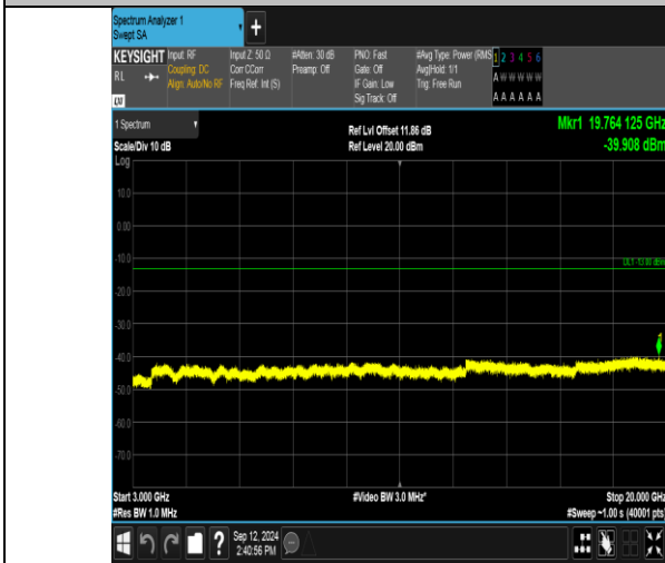
Band2_15MHz_QPSK_18900_1RB#74_3000~20000_3000~20000
