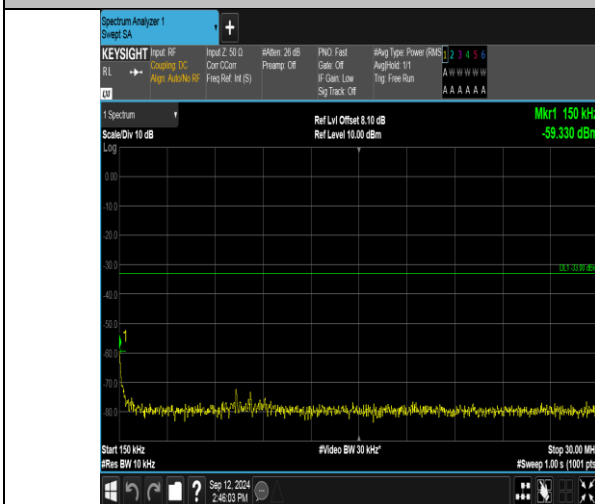
Band2_15MHz_16QAM_19125_1RB#74_0.15~30_0.15~30
