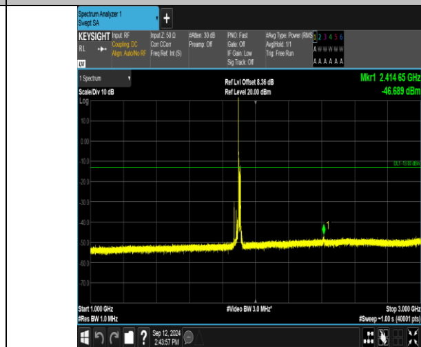
Band2_15MHz_QPSK_19125_1RB#0_1000~3000_1000~3000
