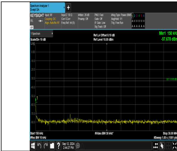
Band2_15MHz_16QAM_19125_1RB#0_0.15~30_0.15~30
