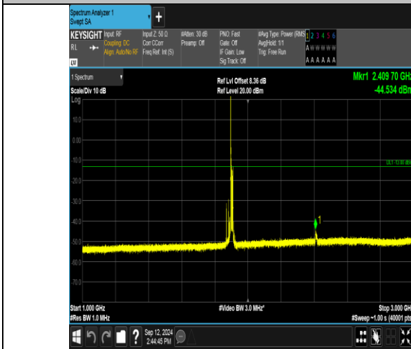
Band2_15MHz_16QAM_19125_1RB#0_1000~3000_1000~3000
