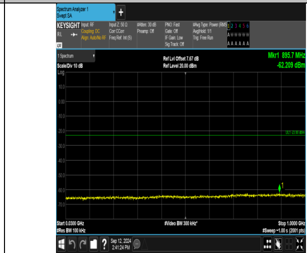
Band2_15MHz_16QAM_18900_1RB#74_30~1000_30~1000
