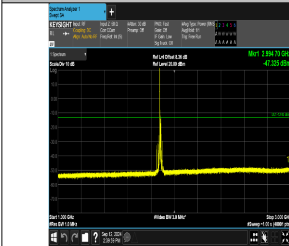
Band2_15MHz_16QAM_18900_1RB#0_1000~3000_1000~3000
