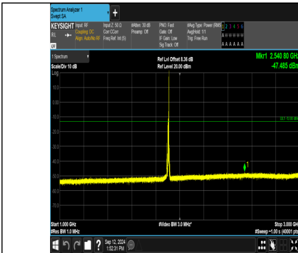
Band2_10MHz_16QAM_19150_1RB#49_1000~3000_1000~3000
