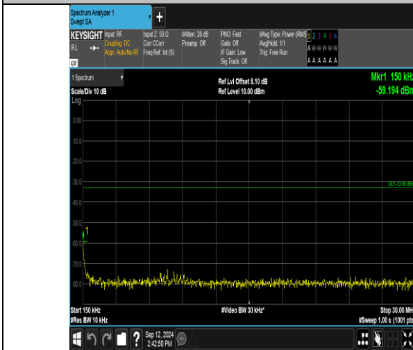
Band2_15MHz_16QAM_18900_75RB#0_0.15~30_0.15~30
