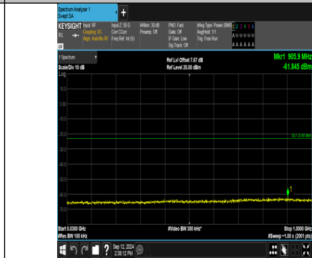
Band2_15MHz_16QAM_18675_75RB#0_30~1000_30~1000
