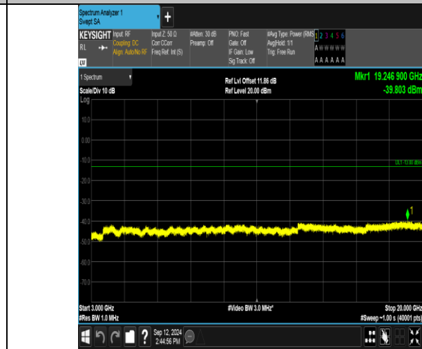
Band2_15MHz_16QAM_19125_1RB#0_3000~20000_3000~20000
