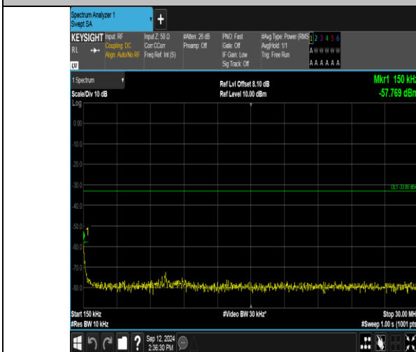
Band2_15MHz_16QAM_18675_1RB#74_0.15~30_0.15~30
