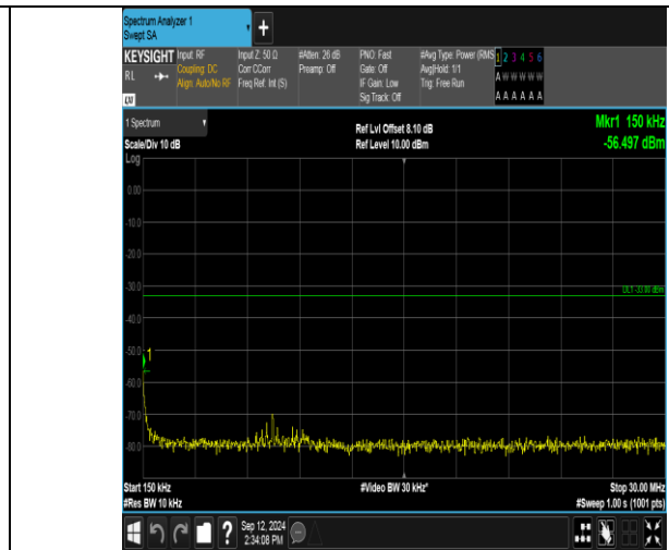
Band2_15MHz_QPSK_18675_1RB#0_0.15~30_0.15~30
