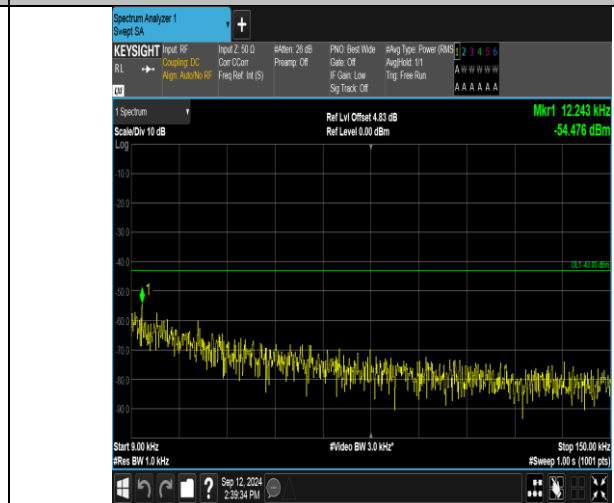
Band2_15MHz_16QAM_18900_1RB#0_0.009~0.15_0.009~0.15
