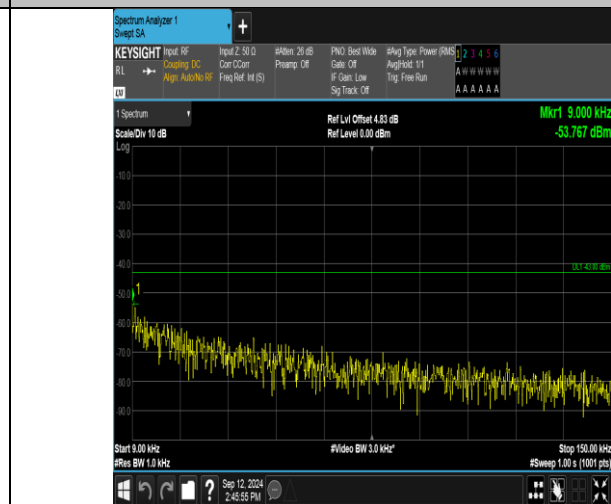
Band2_15MHz_16QAM_19125_1RB#74_0.009~0.15_0.009~0.15
