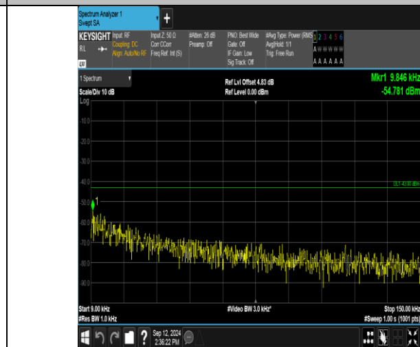
Band2_15MHz_16QAM_18675_1RB#74_0.009~0.15_0.009~0.15
