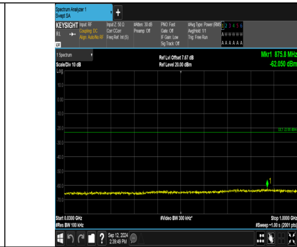
Band2_15MHz_16QAM_18900_1RB#0_30~1000_30~1000
