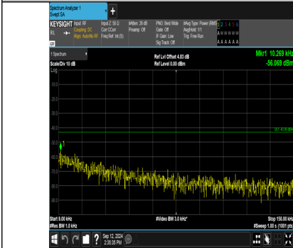
Band2_15MHz_QPSK_18675_1RB#74_0.009~0.15_0.009~0.15
