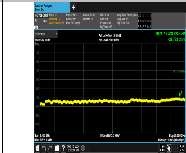
Band2_15MHz_16QAM_18675_1RB#0_3000~20000_3000~20000
