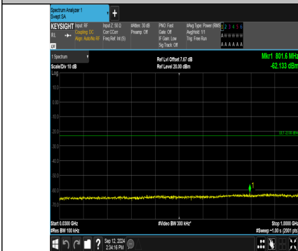
Band2_15MHz_QPSK_18675_1RB#0_30~1000_30~1000
