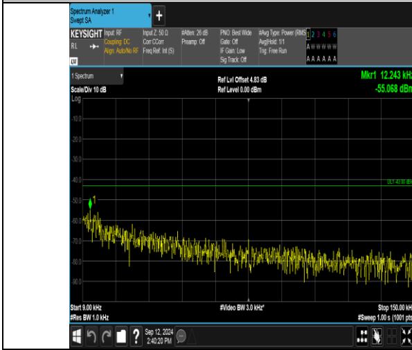
Band2_15MHz_QPSK_18900_1RB#74_0.009~0.15_0.009~0.15
