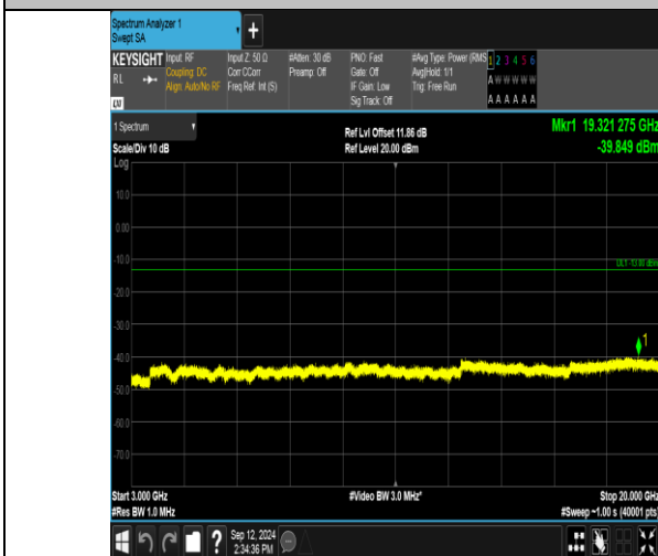
Band2_15MHz_QPSK_18675_1RB#0_3000~20000_3000~20000
