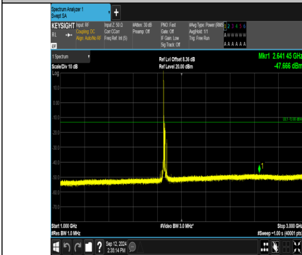
Band2_15MHz_16QAM_18675_1RB#0_1000~3000_1000~3000
