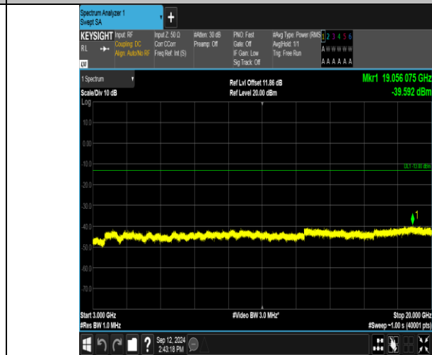
Band2_15MHz_16QAM_18900_75RB#0_3000~20000_3000~20000
