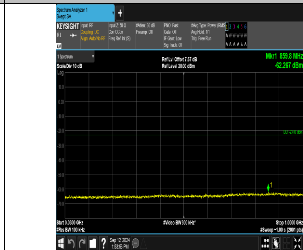
Band2_10MHz_16QAM_19150_50RB#0_30~1000_30~1000
