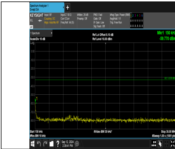
Band2_15MHz_16QAM_18900_1RB#0_0.15~30_0.15~30
