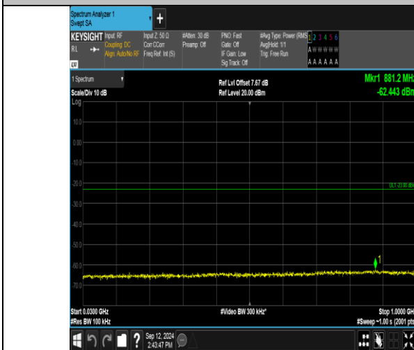
Band2_15MHz_QPSK_19125_1RB#0_30~1000_30~1000
