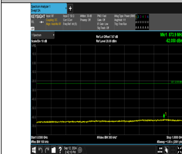
Band2_15MHz_QPSK_18900_75RB#0_30-1000_30-1000
