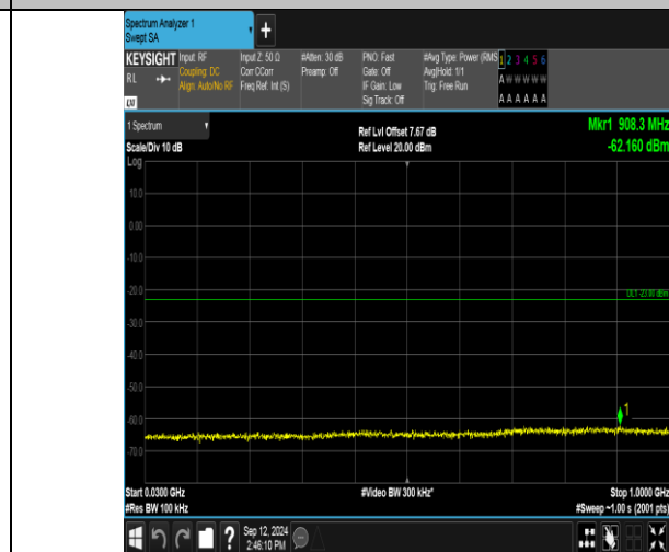
Band2_15MHz_16QAM_19125_1RB#74_30~1000_30~1000
