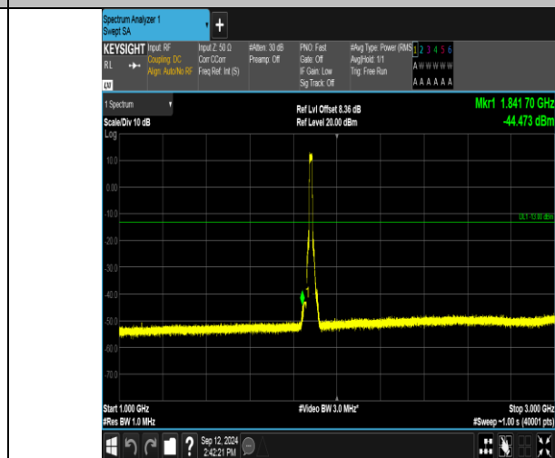
Band2_15MHz_QPSK_18900_75RB#0_1000-3000_1000-3000
