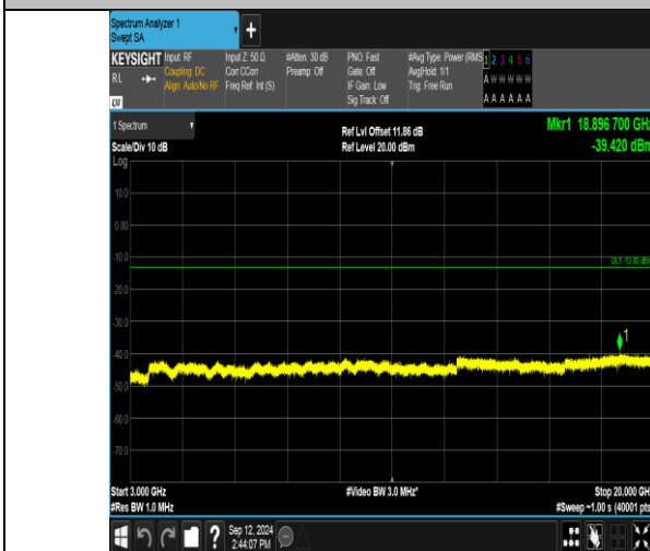
Band2_15MHz_QPSK_19125_1RB#0_3000~20000_3000~20000
