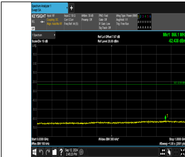
Band2_15MHz_QPSK_19125_1RB#74_30~1000_30~1000
