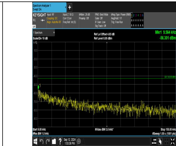
Band2_10MHz_16QAM_19150_50RB#0_0.009~0.15_0.009~0.15
