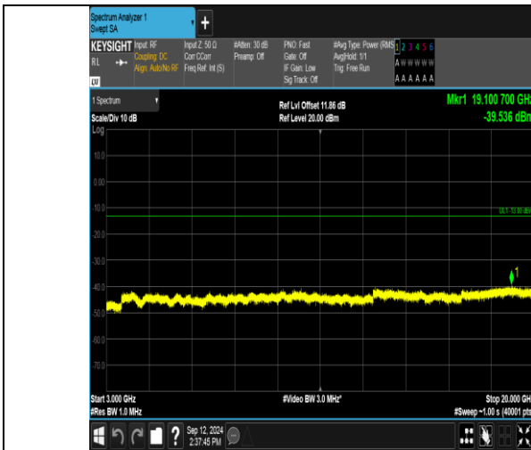
Band2_15MHz_QPSK_18675_75RB#0_3000~20000_3000~20000
