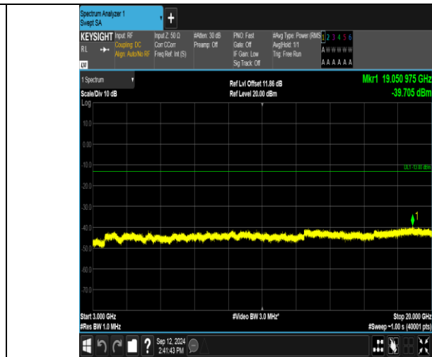
Band2_15MHz_16QAM_18900_1RB#74_3000-20000_3000-20000
