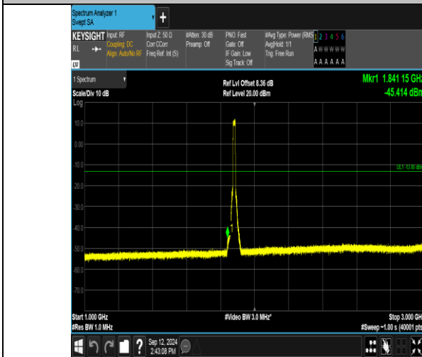
Band2_15MHz_16QAM_18900_75RB#0_1000~3000_1000~3000
