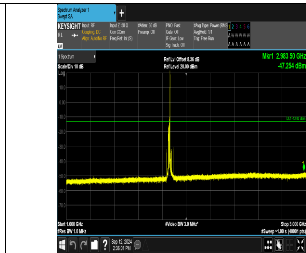
Band2_15MHz_QPSK_18675_1RB#74_1000~3000_1000~3000
