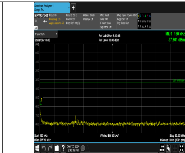
Band2_15MHz_QPSK_19125_1RB#0_0.15~30_0.15~30
