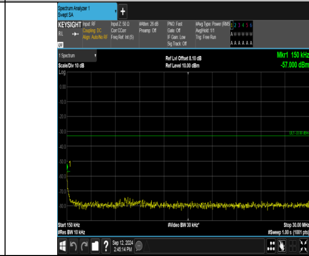
Band2_15MHz_QPSK_19125_1RB#74_0.15~30_0.15~30
