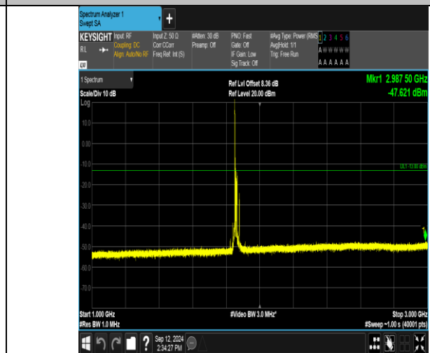
Band2_15MHz_QPSK_18675_1RB#0_1000~3000_1000~3000
