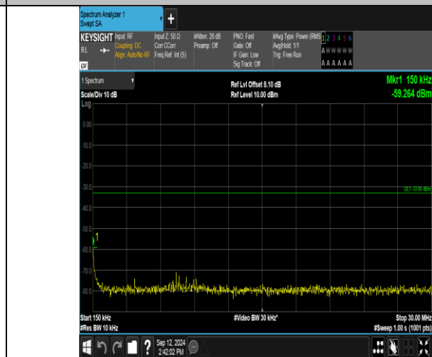
Band2_15MHz_QPSK_18900_75RB#0_0.15-30_0.15-30
