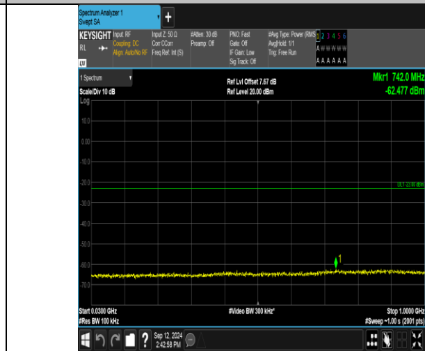
Band2_15MHz_16QAM_18900_75RB#0_30~1000_30~1000
