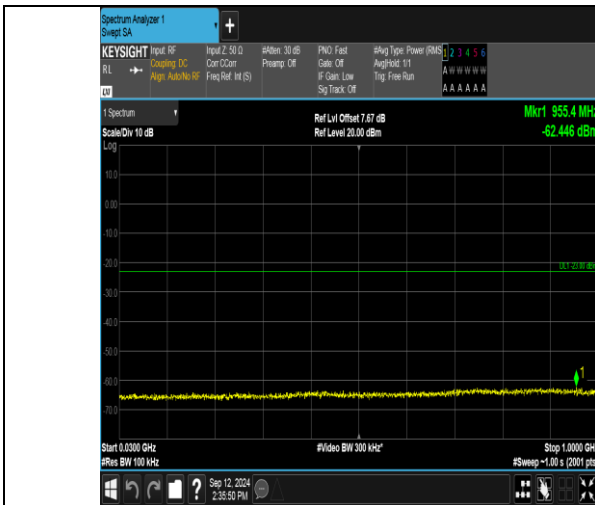
Band2_15MHz_QPSK_18675_1RB#74_30~1000_30~1000
