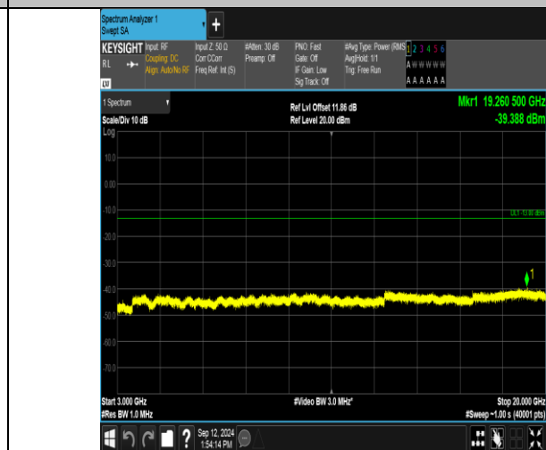
Band2_10MHz_16QAM_19150_50RB#0_3000~20000_3000~20000
