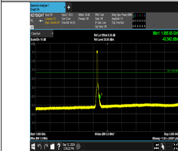
Band2_15MHz_16QAM_18675_75RB#0_1000~3000_1000~3000
