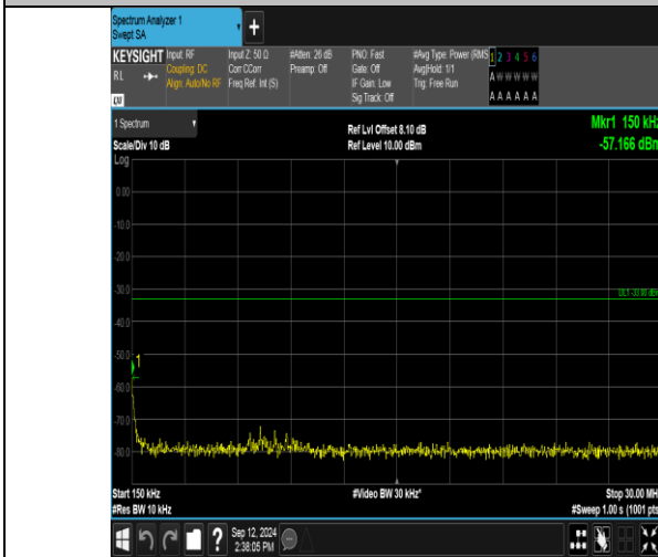
Band2_15MHz_16QAM_18675_75RB#0_0.15~30_0.15~30
