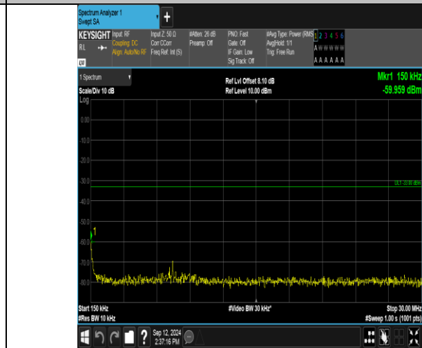
Band2_15MHz_QPSK_18675_75RB#0_0.15-30_0.15-30
