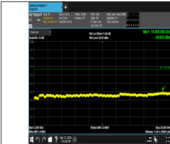
Band2_10MHz_QPSK_19150_50RB#0_3000~20000_3000~20000
