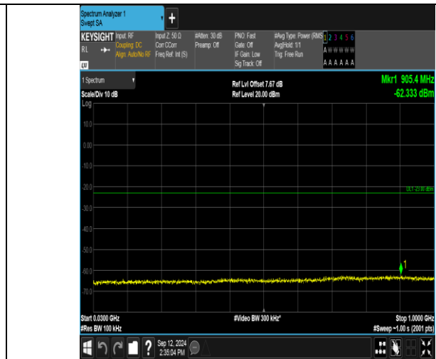
Band2_15MHz_16QAM_18675_1RB#0_30~1000_30~1000
