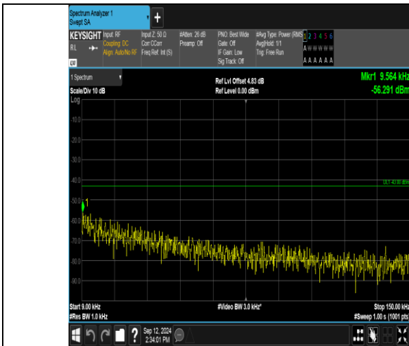
Band2_15MHz_QPSK_18675_1RB#0_0.009~0.15_0.009~0.15
