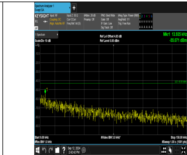
Band2_15MHz_16QAM_18900_75RB#0_0.009~0.15_0.009~0.15
