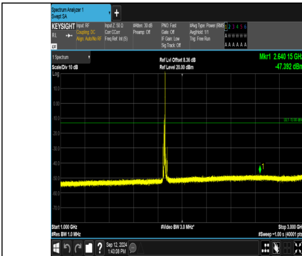
Band2_10MHz_16QAM_18650_1RB#49_1000-3000_1000-3000
