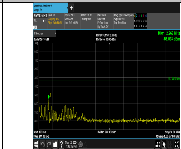
Band2_10MHz_QPSK_18900_50RB#0_0.15~30_0.15~30
