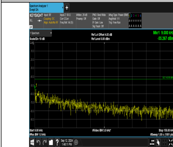
Band2_10MHz_QPSK_18900_50RB#0_0.009~0.15_0.009~0.15
