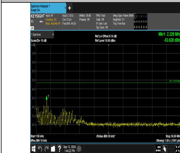
Band2_10MHz_16QAM_18650_50RB#0_0.15~30_0.15~30
