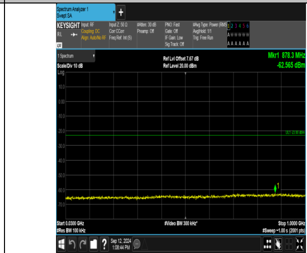
Band2_5MHz_16QAM_19175_25RB#0_30~1000_30~1000
