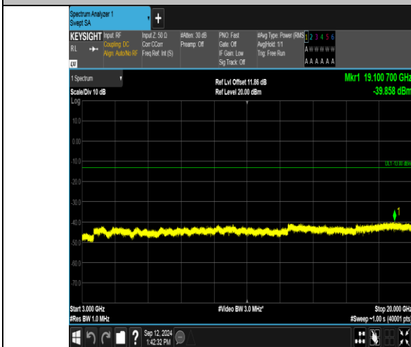
Band2_10MHz_QPSK_18650_1RB#49_3000~20000_3000~20000
