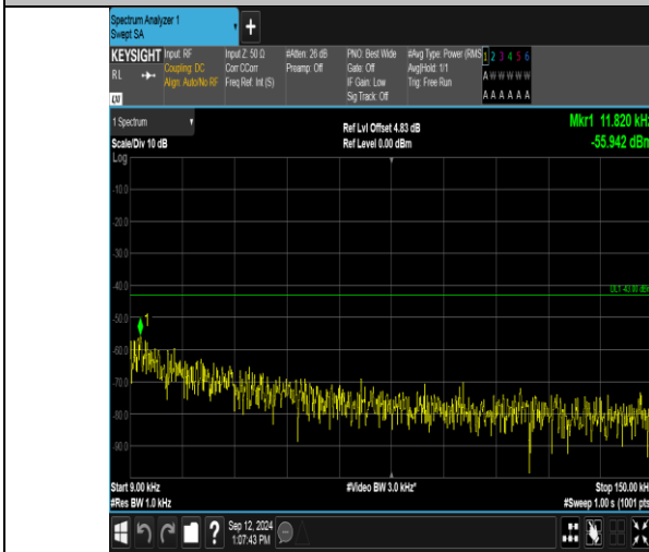
Band2_5MHz_QPSK_19175_25RB#0_0.009~0.15_0.009~0.15
