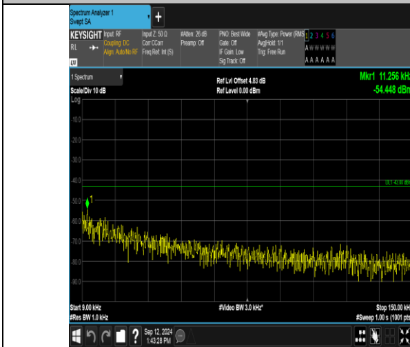
Band2_10MHz_QPSK_18650_50RB#0_0.009-0.15_0.009-0.15
