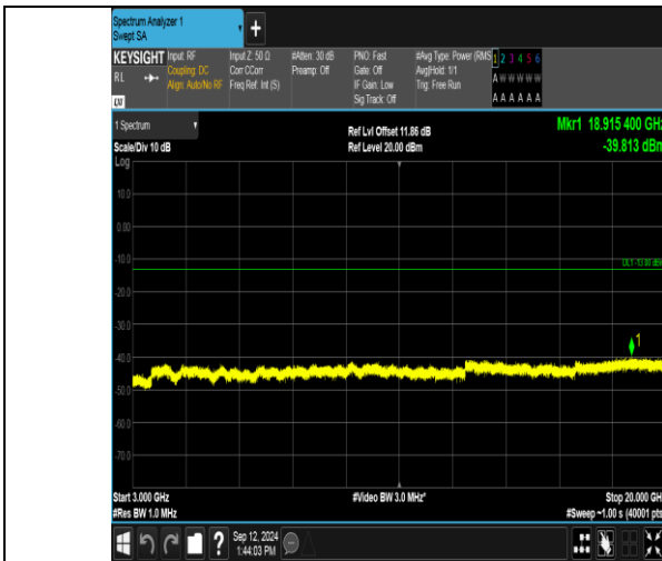
Band2_10MHz_QPSK_18650_50RB#0_3000~20000_3000~20000
