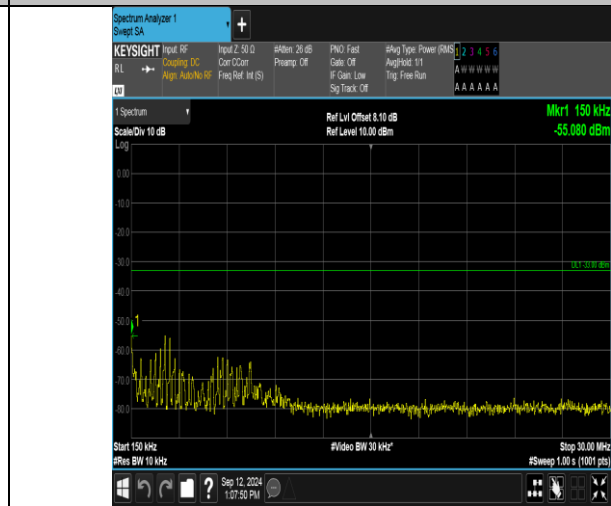
Band2_5MHz_QPSK_19175_25RB#0_0.15~30_0.15~30
