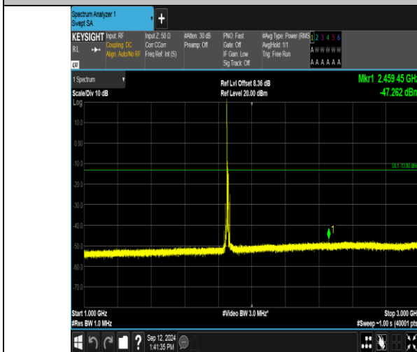
Band_2_10MHz_16QAM_18650_1RB#0_1000~3000_1000~3000
