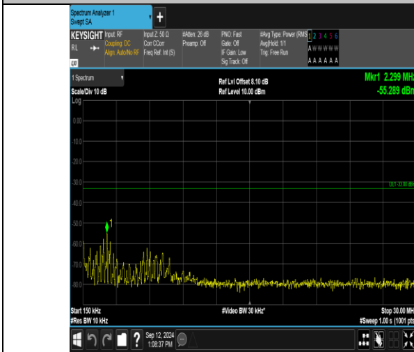
Band2_5MHz_16QAM_19175_25RB#0_0.15~30_0.15~30
