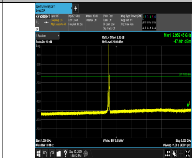
Band2_10MHz_QPSK_19150_1RB#0_1000~3000_1000~3000
