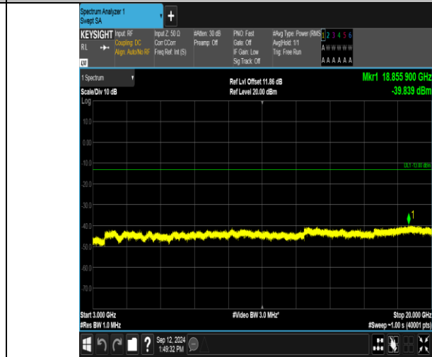
Band2_10MHz_16QAM_18900_50RB#0_3000~20000_3000~20000
