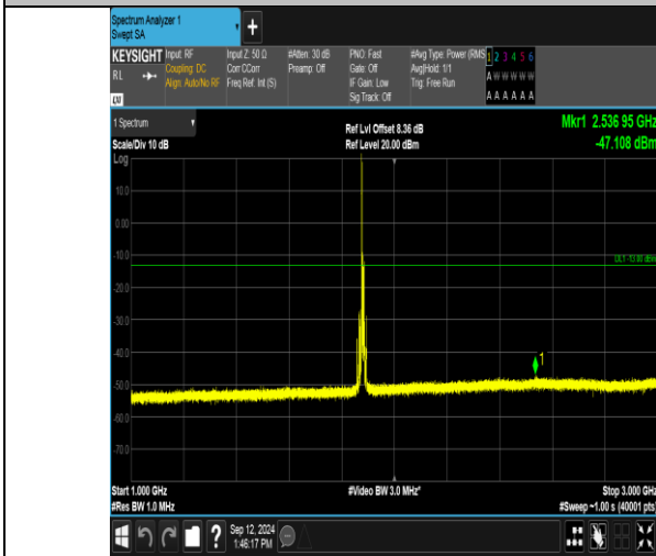
Band_2_10MHz_16QAM_18900_1RB#0_1000~3000_1000~3000
