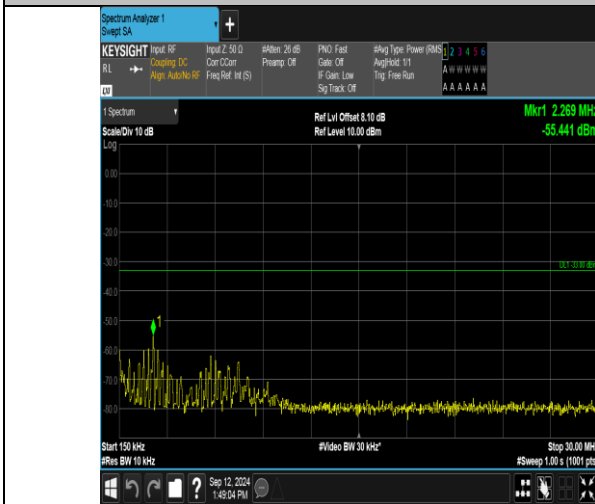
Band2_10MHz_16QAM_18900_50RB#0_0.15~30_0.15~30
