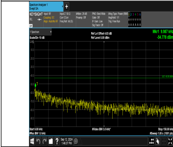
Band_2_10MHz_QPSK_18900_1RB#49_0.009~0.15_0.009~0.15
