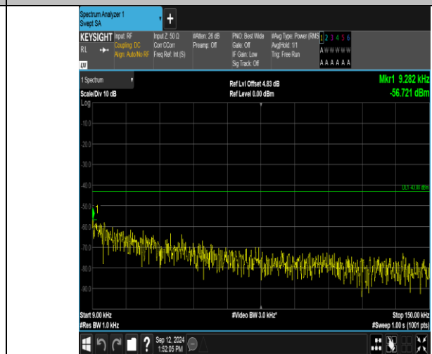
Band2_10MHz_16QAM_19150_1RB#49_0.009~0.15_0.009~0.15
