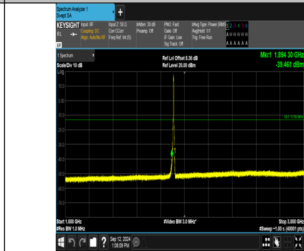
Band2_5MHz_QPSK_19175_25RB#0_1000~3000_1000~3000
