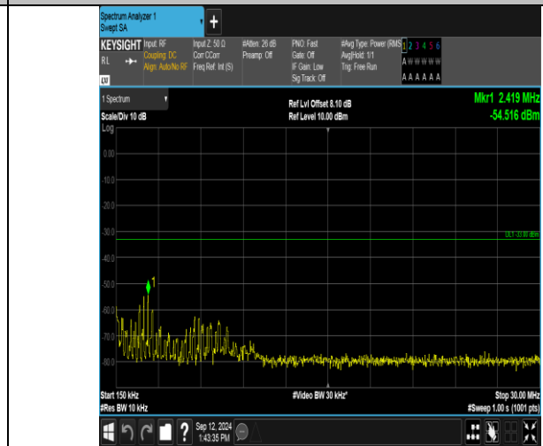
Band2_10MHz_QPSK_18650_50RB#0_0.15-30_0.15-30
