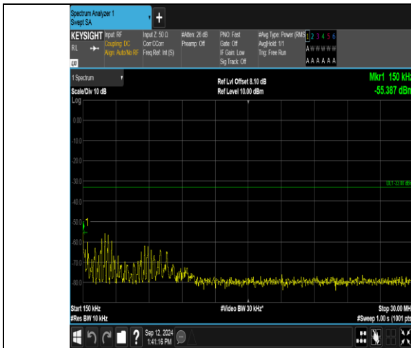
Band_2_10MHz_16QAM_18650_1RB#0_0.15~30_0.15~30
