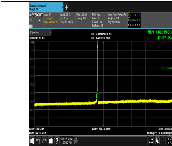
Band2_5MHz_16QAM_19175_1RB#24_1000~3000_1000~3000
