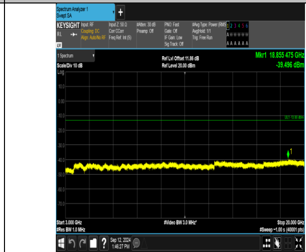
Band_2_10MHz_16QAM_18900_1RB#0_3000~20000_3000~20000
