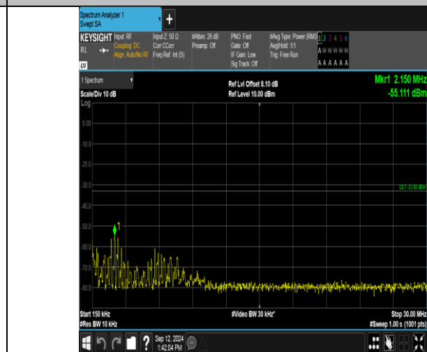
Band_2_10MHz_QPSK_18650_1RB#49_0.15~30_0.15~30
