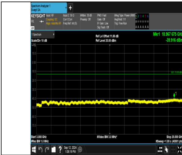
Band2_5MHz_QPSK_19175_25RB#0_3000~20000_3000~20000
