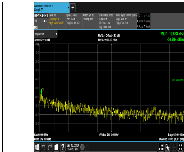
Band2_10MHz_16QAM_18900_50RB#0_0.009~0.15_0.009~0.15
