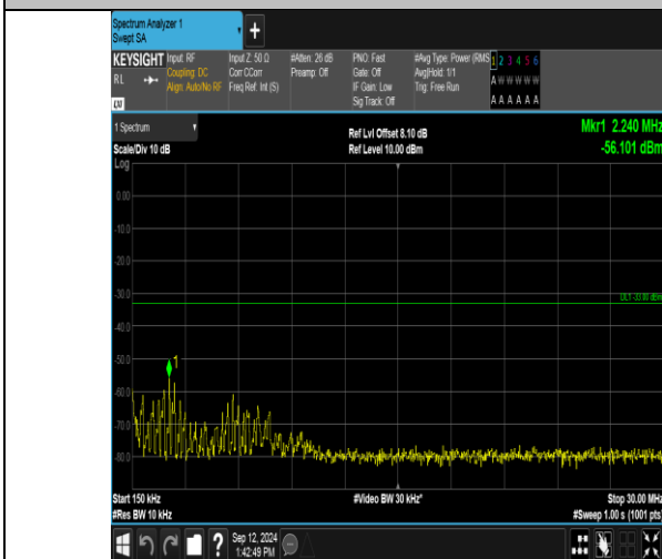
Band2_10MHz_16QAM_18650_1RB#49_0.15~30_0.15~30
