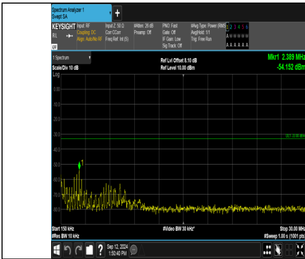
Band_2_10MHz_16QAM_19150_1RB#0_0.15~30_0.15~30
