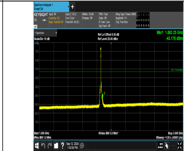
Band2_10MHz_QPSK_18650_50RB#0_1000-3000_1000-3000
