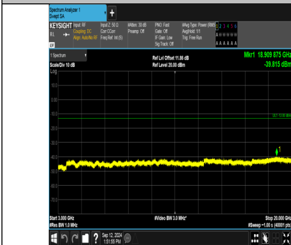
Band2_10MHz_QPSK_19150_1RB#49_3000~20000_3000~20000
