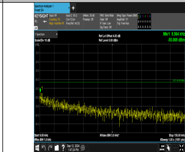
Band2_10MHz_16QAM_18900_1RB#49_0.009~0.15_0.009~0.15
