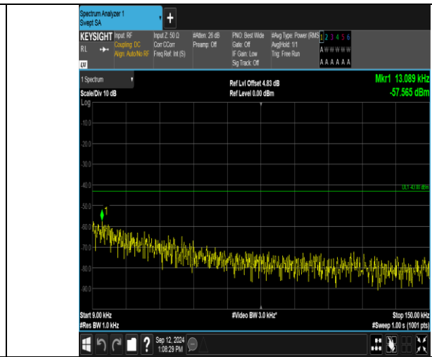
Band2_5MHz_16QAM_19175_25RB#0_0.009~0.15_0.009~0.15
