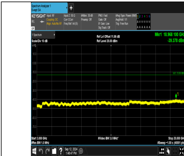
Band2_10MHz_QPSK_18900_50RB#0_3000~20000_3000~20000
