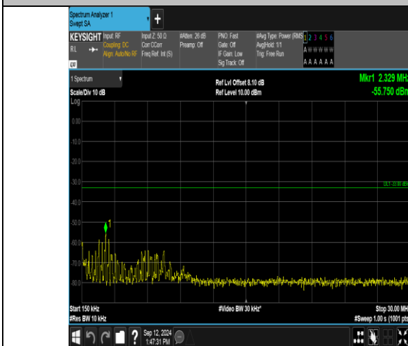
Band2_10MHz_16QAM_18900_1RB#49_0.15~30_0.15~30
