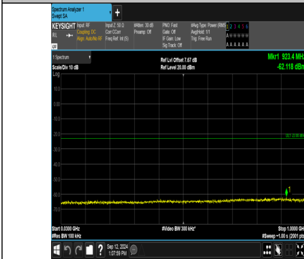
Band2_5MHz_QPSK_19175_25RB#0_30~1000_30~1000
