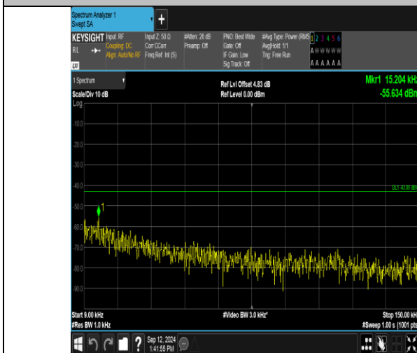
Band_2_10MHz_QPSK_18650_1RB#49_0.009~0.15_0.009~0.15
