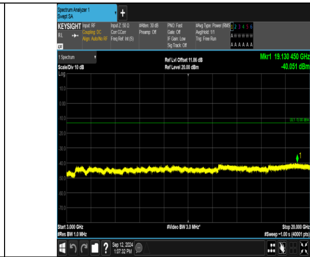
Band2_5MHz_16QAM_19175_1RB#24_3000~20000_3000~20000
