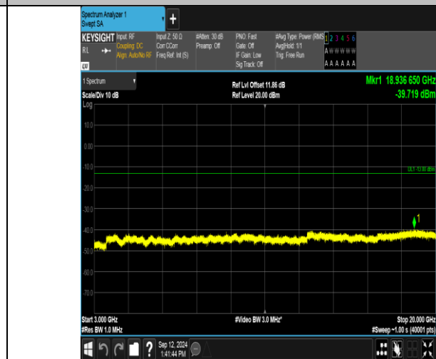
Band_2_10MHz_16QAM_18650_1RB#0_3000~20000_3000~20000
