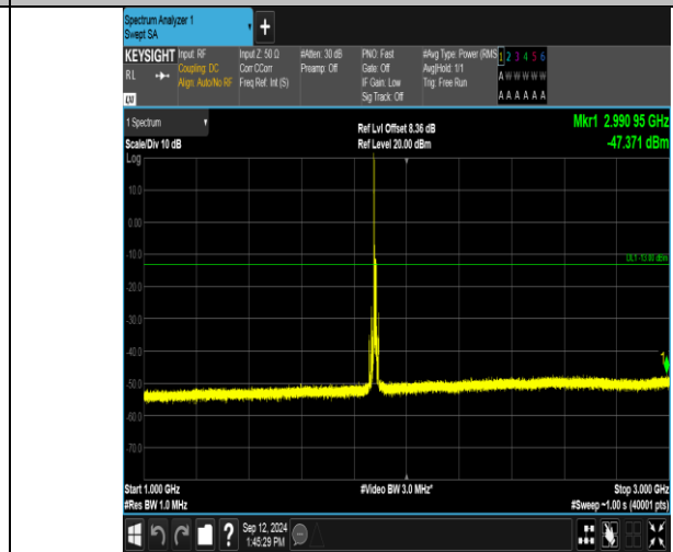
Band2_10MHz_QPSK_18900_1RB#0_1000~3000_1000~3000
