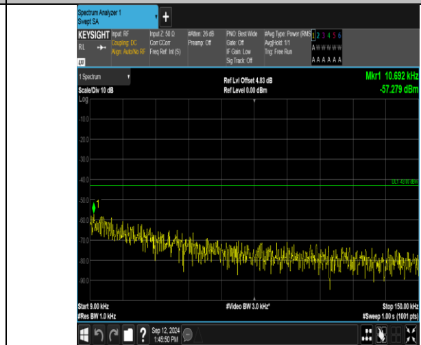
Band2_10MHz_16QAM_18900_1RB#0_0.009~0.15_0.009~0.15
