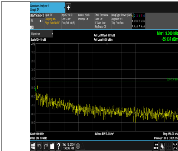
Band2_10MHz_QPSK_19150_1RB#0_0.009~0.15_0.009~0.15
