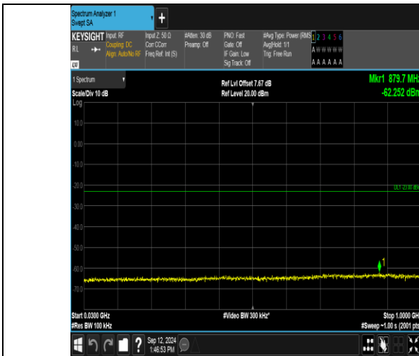
Band2_10MHz_QPSK_18900_1RB#49_30~1000_30~1000
