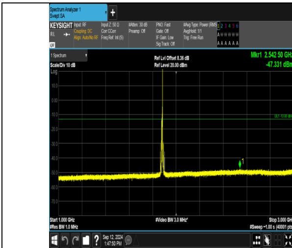
Band2_10MHz_16QAM_18900_1RB#49_1000~3000_1000~3000
