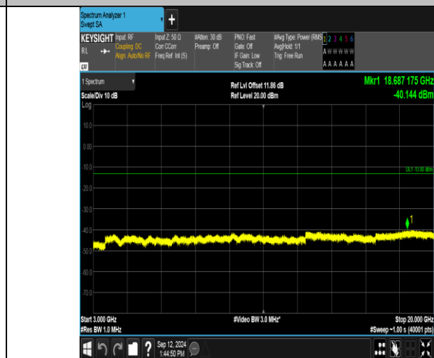
Band2_10MHz_16QAM_18650_50RB#0_3000~20000_3000~20000
