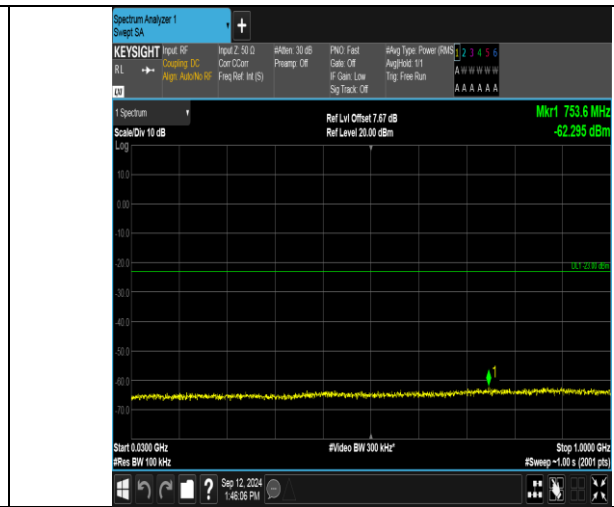
Band_2_10MHz_16QAM_18900_1RB#0_30~1000_30~1000
