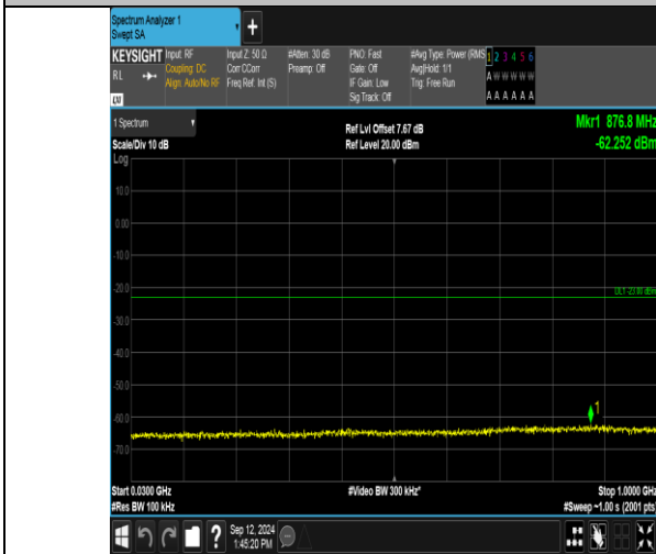
Band2_10MHz_QPSK_18900_1RB#0_30~1000_30~1000
