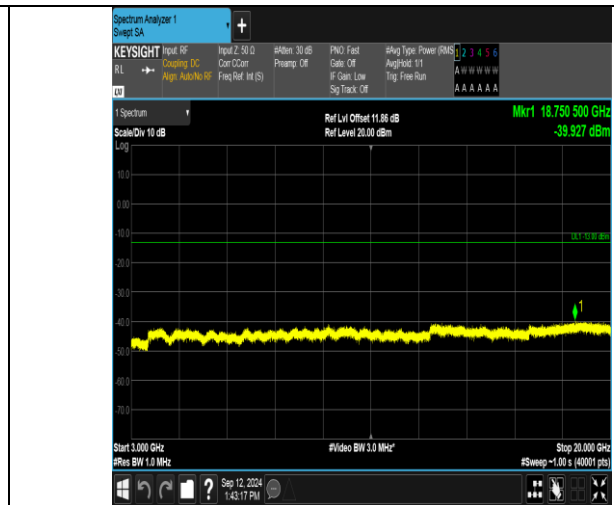
Band2_10MHz_16QAM_18650_1RB#49_3000-20000_3000-20000
