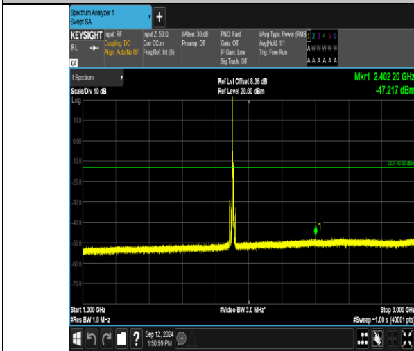
Band_2_10MHz_16QAM_19150_1RB#0_1000~3000_1000~3000
