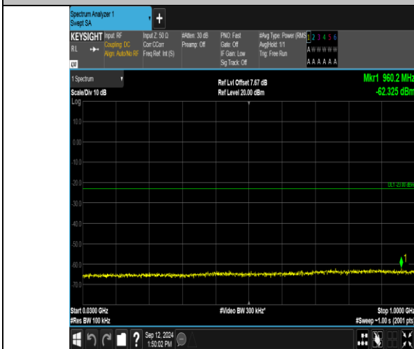
Band_10MHz_QPSK_19150_1RB#0_30~1000_30~1000
