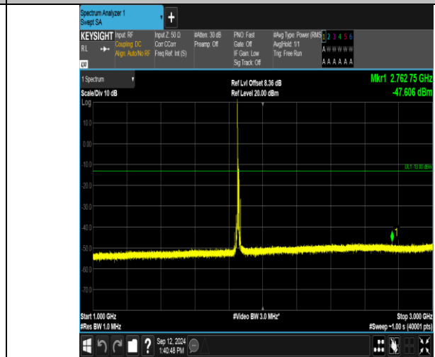
Band2_10MHz_QPSK_18650_1RB#0_1000~3000_1000~3000
