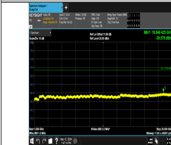
Band2_10MHz_QPSK_18900_1RB#49_3000~20000_3000~20000
