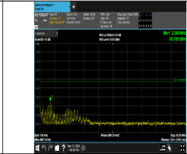
Band_2_10MHz_QPSK_18900_1RB#49_0.15~30_0.15~30
