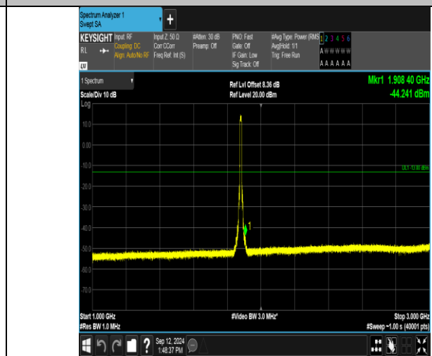
Band2_10MHz_QPSK_18900_50RB#0_1000~3000_1000~3000
