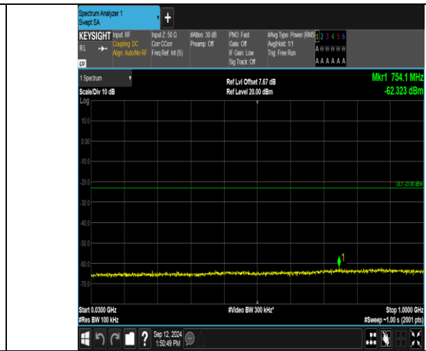
Band2_10MHz_16QAM_19150_1RB#0_30~1000_30~1000
