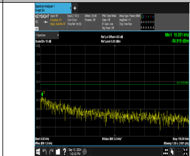
Band2_10MHz_16QAM_18650_1RB#49_0.009~0.15_0.009~0.15
