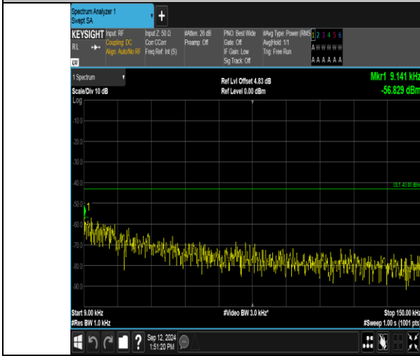
Band_2_10MHz_QPSK_19150_1RB#49_0.009~0.15_0.009~0.15
