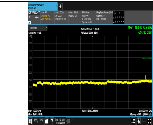
Band2_10MHz_16QAM_18900_1RB#49_3000~20000_3000~20000
