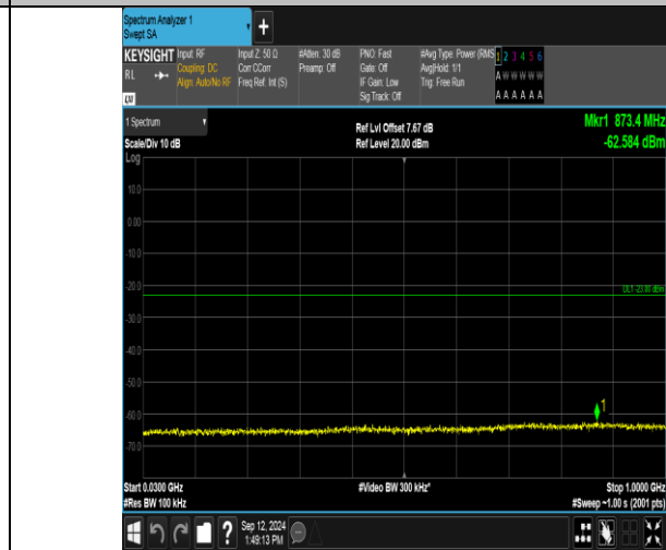
Band2_10MHz_16QAM_18900_50RB#0_30~1000_30~1000
