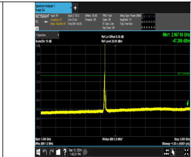
Band2_10MHz_QPSK_18650_1RB#49_1000~3000_1000~3000
