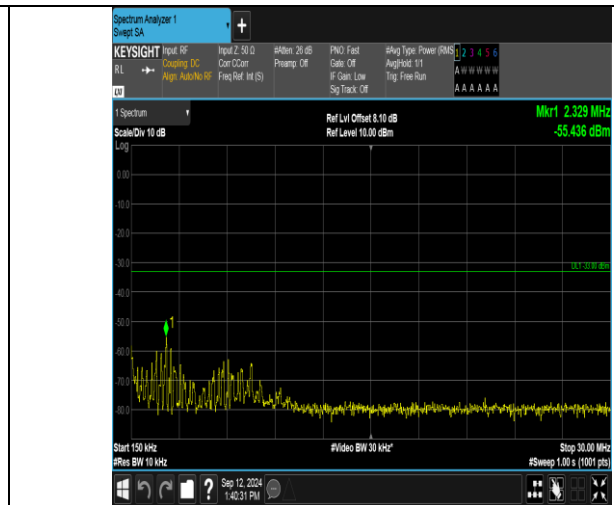
Band2_10MHz_QPSK_18650_1RB#0_0.15~30_0.15~30
