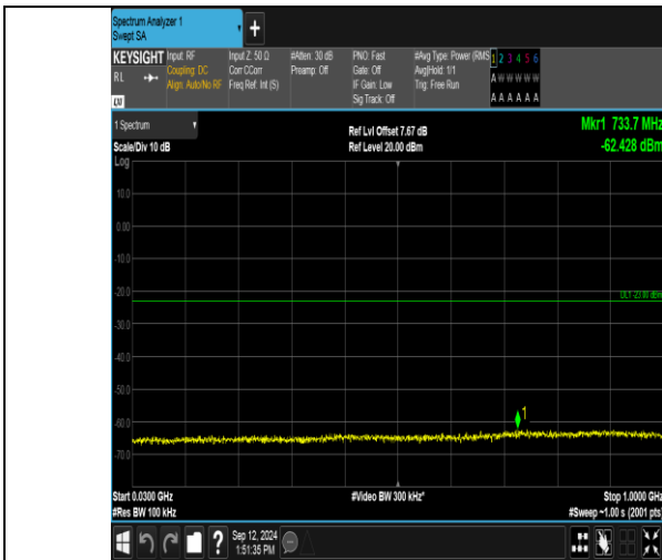
Band2_10MHz_QPSK_19150_1RB#49_30~1000_30~1000
