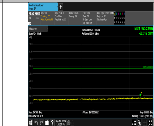
Band2_10MHz_16QAM_18650_1RB#49_30~1000_30~1000
