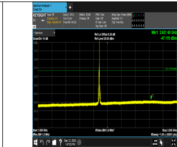
Band2_10MHz_QPSK_18900_1RB#49_1000~3000_1000~3000
