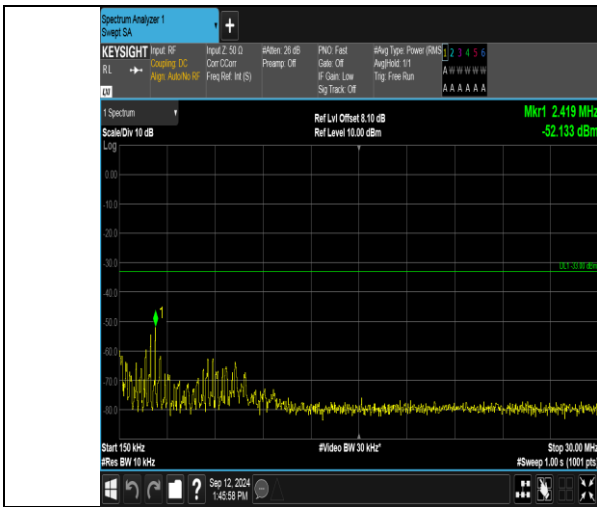
Band_2_10MHz_16QAM_18900_1RB#0_0.15~30_0.15~30
