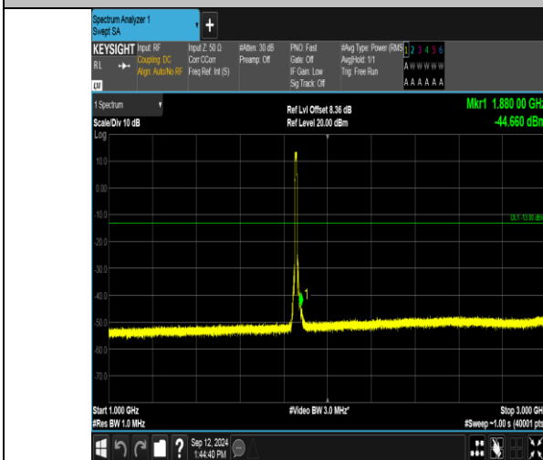
Band2_10MHz_16QAM_18650_50RB#0_1000~3000_1000~3000
