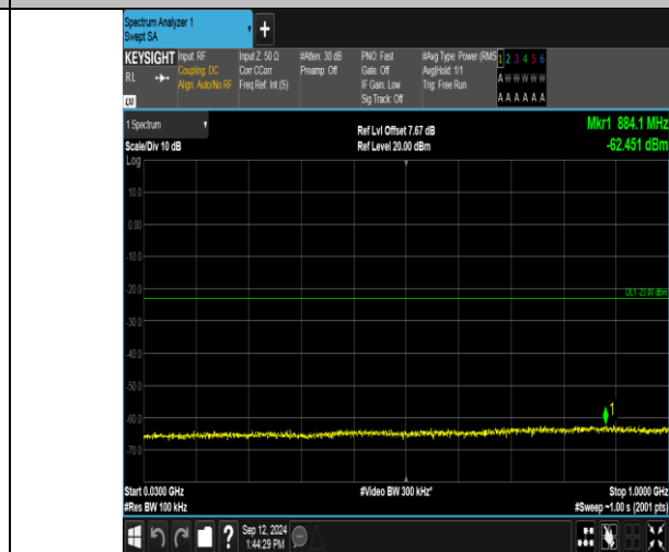
Band2_10MHz_16QAM_18650_50RB#0_30~1000_30~1000
