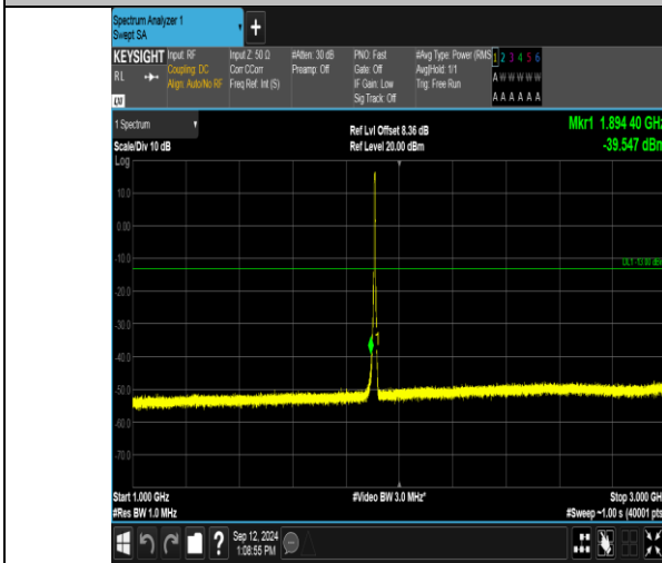
Band2_5MHz_16QAM_19175_25RB#0_1000~3000_1000~3000
