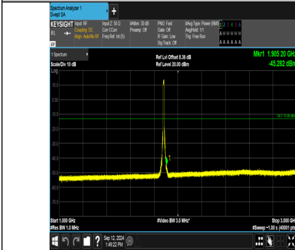
Band2_10MHz_16QAM_18900_50RB#0_1000~3000_1000~3000
