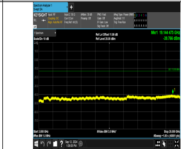
Band2_5MHz_16QAM_19175_25RB#0_3000~20000_3000~20000
