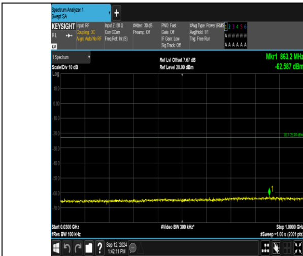
Band2_10MHz_QPSK_18650_1RB#49_30~1000_30~1000
