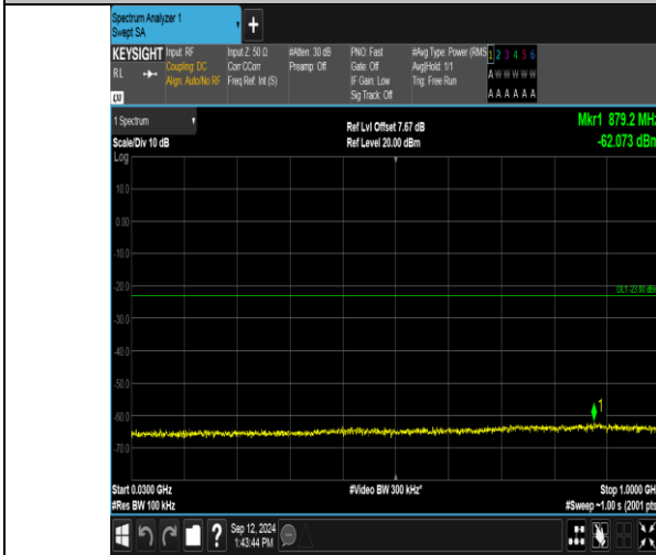
Band2_10MHz_QPSK_18650_50RB#0_30-1000_30-1000
