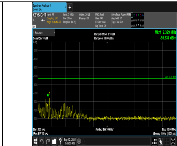
Band2_10MHz_QPSK_19150_1RB#0_0.15~30_0.15~30
