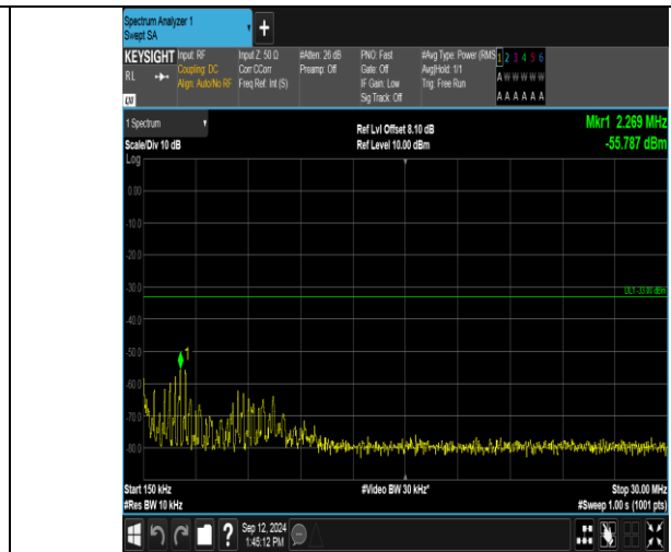
Band2_10MHz_QPSK_18900_1RB#0_0.15~30_0.15~30
