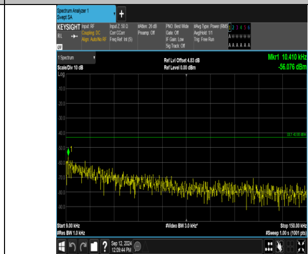
Band2_3MHz_16QAM_18615_1RB#0_0.009~0.15_0.009~0.15
