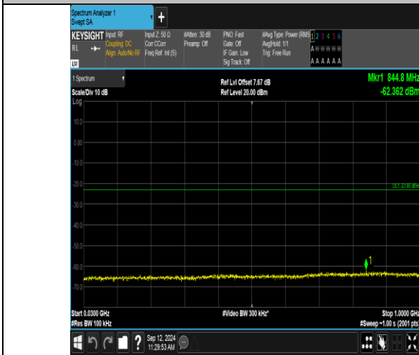
Band2_1.4MHz_QPSK_19193_6RB#0_30-1000_30-1000
