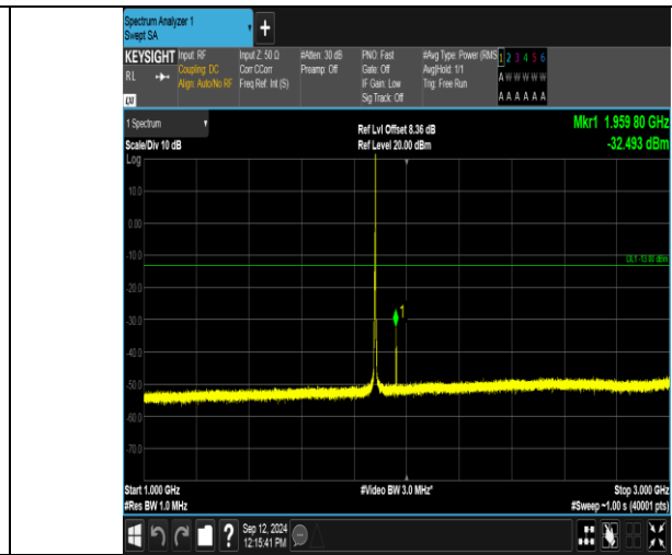
Band2_3MHz_QPSK_18900_1RB#14_1000~3000_1000~3000
