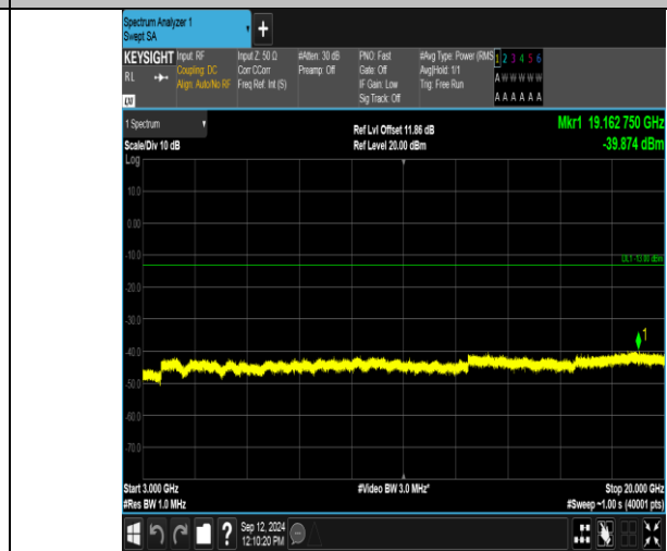
Band2_3MHz_16QAM_18615_1RB#0_3000~20000_3000~20000
