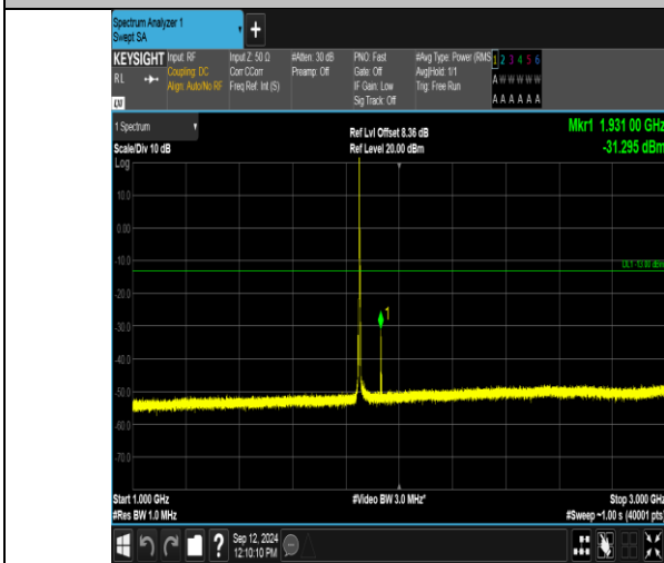
Band2_3MHz_16QAM_18615_1RB#0_1000~3000_1000~3000
