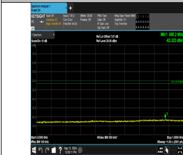
Band2_3MHz_QPSK_18615_1RB#0_30~1000_30~1000
