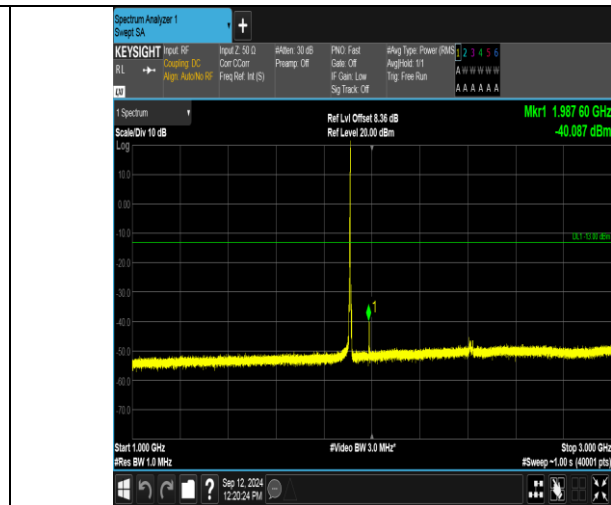
Band2_3MHz_QPSK_19185_1RB#14_1000~3000_1000~3000
