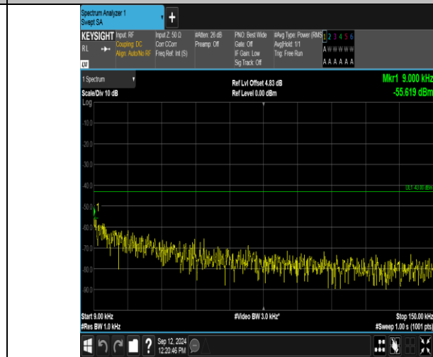
Band2_3MHz_16QAM_19185_1RB#14_0.009~0.15_0.009~0.15
