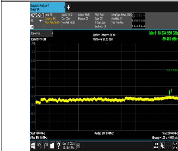
Band2_3MHz_QPSK_18900_1RB#14_3000~20000_3000~20000
