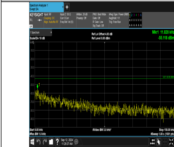
Band2_1.4MHz_QPSK_19193_6RB#0_0.009-0.15_0.009-0.15
