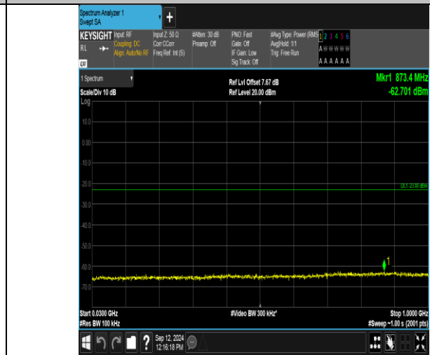
Band2_3MHz_16QAM_18900_1RB#14_30~1000_30~1000
