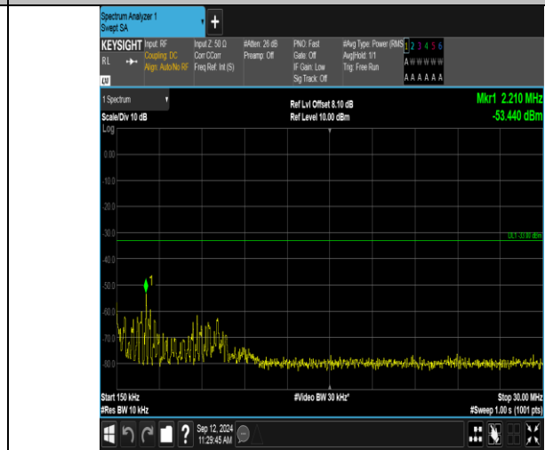
Band2_1.4MHz_QPSK_19193_6RB#0_0.15-30_0.15-30
