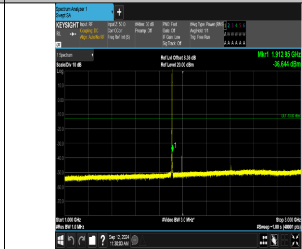
Band2_1.4MHz_QPSK_19193_6RB#0_1000-3000_1000-3000
