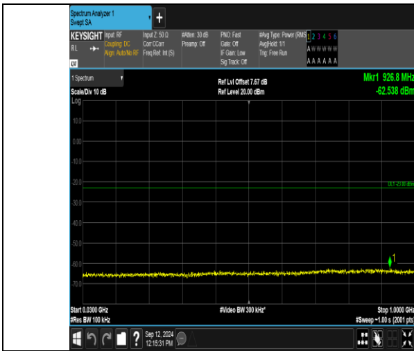
Band2_3MHz_QPSK_18900_1RB#14_30~1000_30~1000
