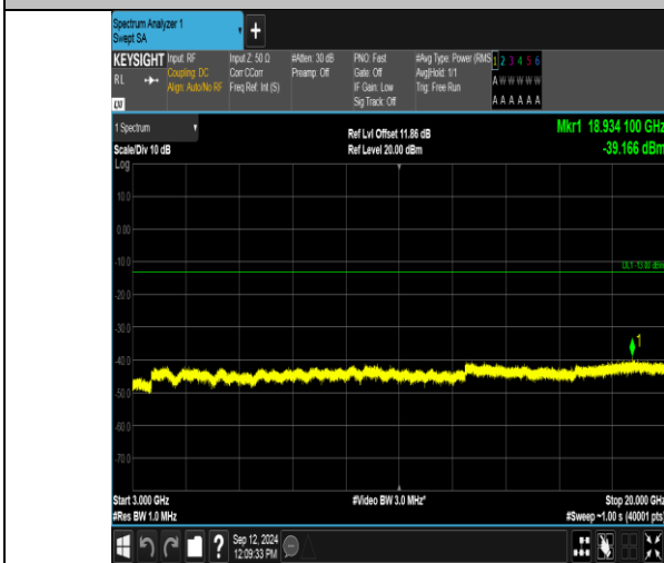
Band2_3MHz_QPSK_18615_1RB#0_3000~20000_3000~20000
