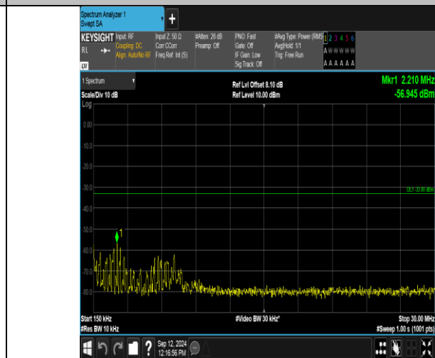
Band2_3MHz_QPSK_18900_15RB#0_0.15~30_0.15~30
