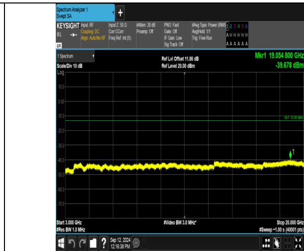
Band2_3MHz_16QAM_18900_1RB#14_3000~20000_3000~20000
