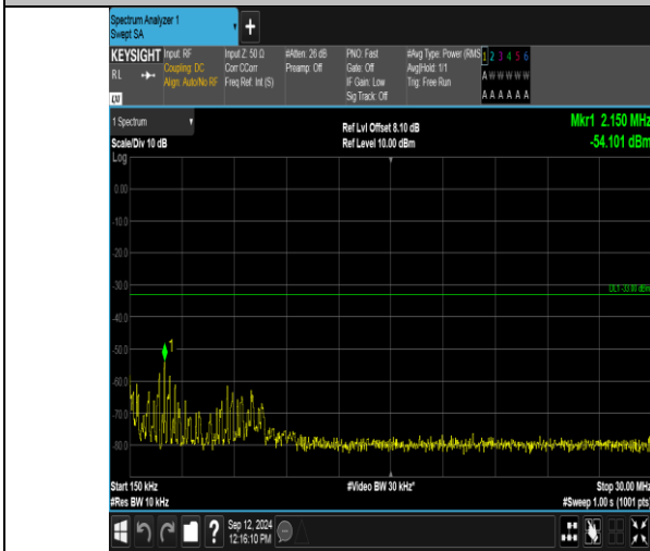
Band2_3MHz_16QAM_18900_1RB#14_0.15~30_0.15~30
