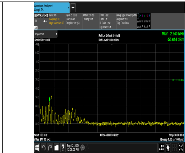
Band2_3MHz_QPSK_18615_1RB#0_0.15~30_0.15~30
