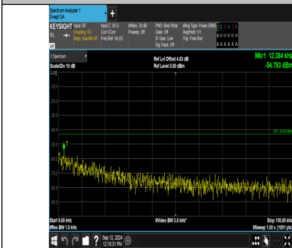
Band2_3MHz_QPSK_18615_1RB#14_0.009~0.15_0.009~0.15
