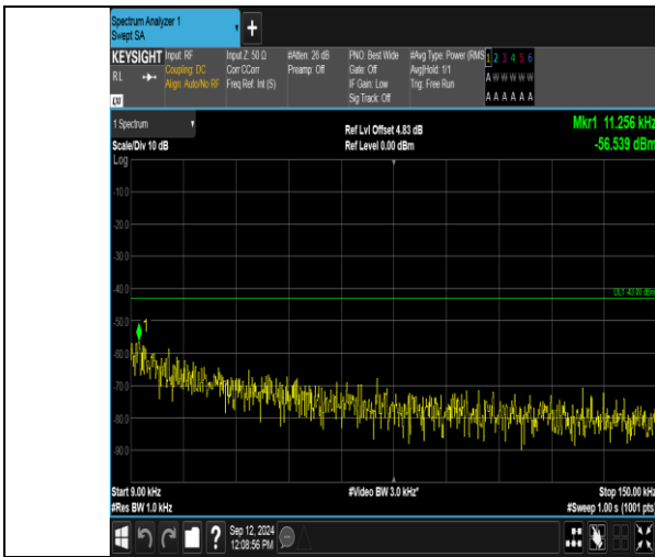
Band2_3MHz_QPSK_18615_1RB#0_0.009~0.15_0.009~0.15
