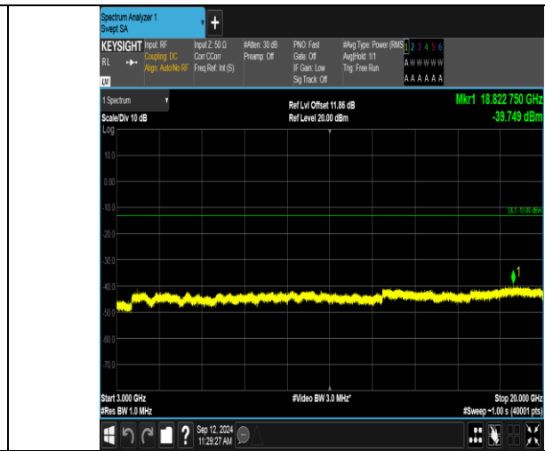
Band2_1.4MHz_16QAM_19193_1RB#5_3000-20000_3000-20000
