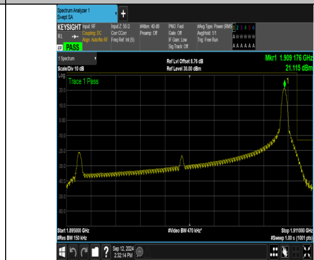
Band2_15MHz_16QAM_19125_1RB#74
