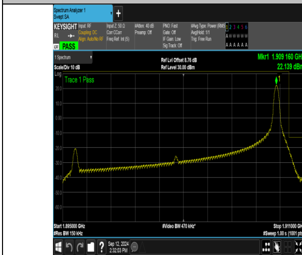
Band2_15MHz_QPSK_19125_1RB#74
