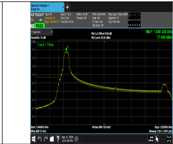
Band2_5MHz_16QAM_18625_1RB#0
