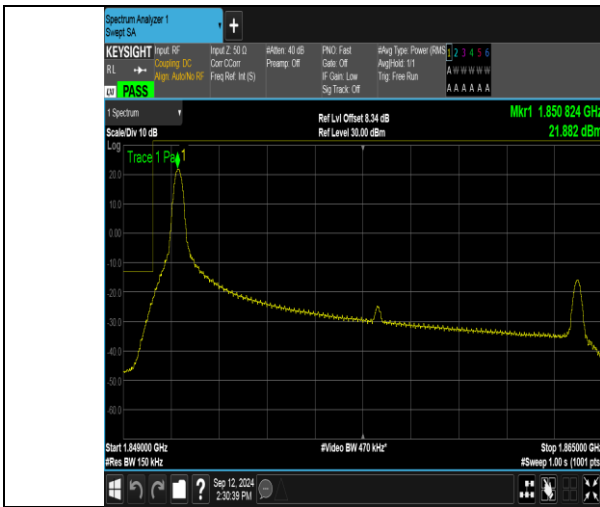
Band2_15MHz_QPSK_18675_1RB#0
