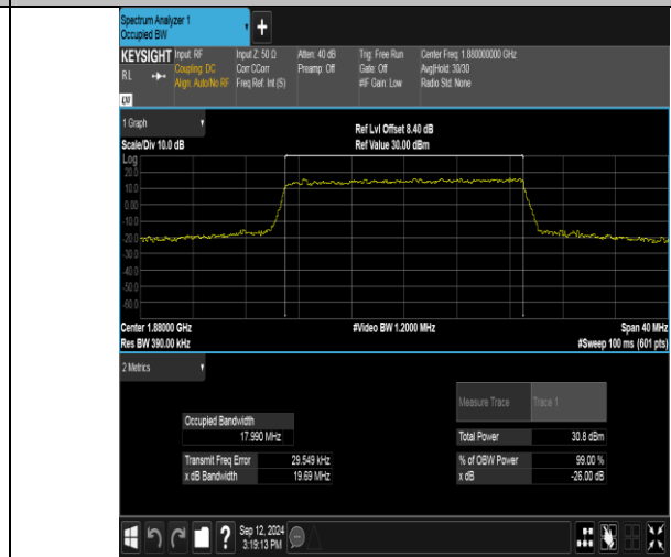
Band2-20MHz-16QAM-18900-100RB#0-PASS
