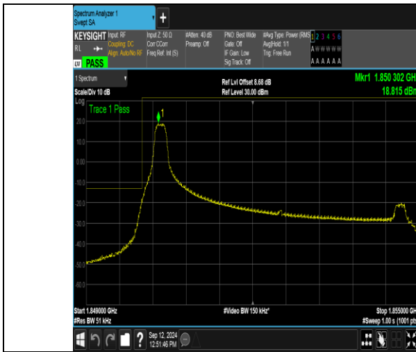
Band2_5MHz_QPSK_18625_1RB#0
