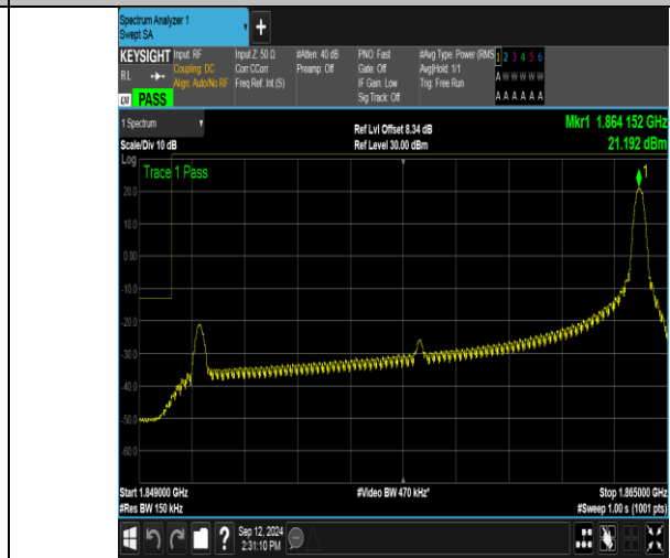
Band2_15MHz_16QAM_18675_1RB#74
