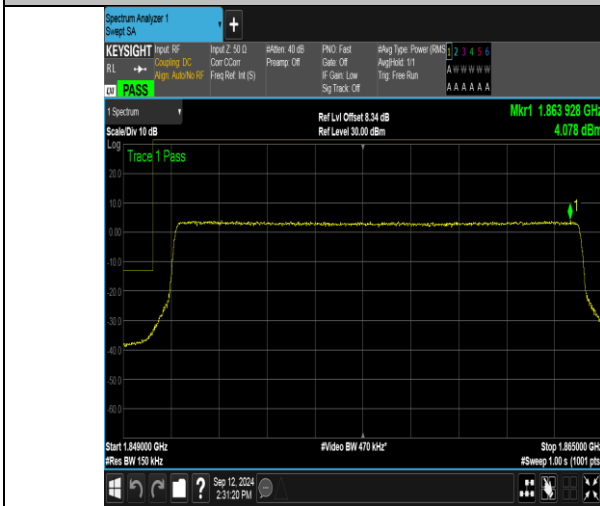
Band2_15MHz_QPSK_18675_75RB#0
