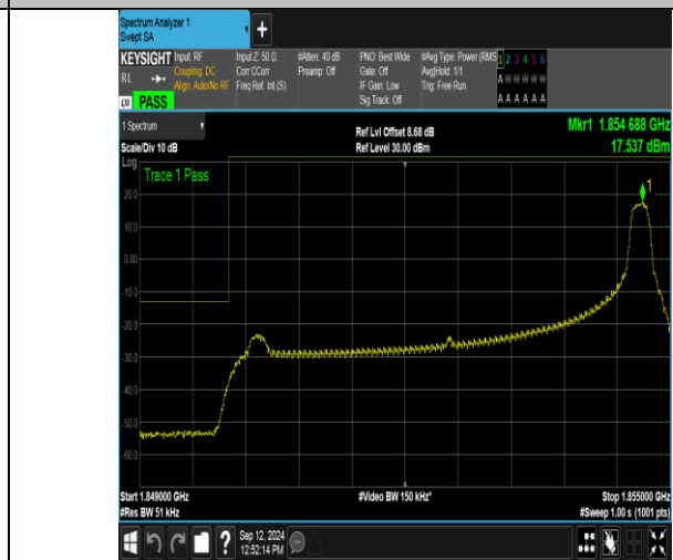
Band2_5MHz_16QAM_18625_1RB#24
