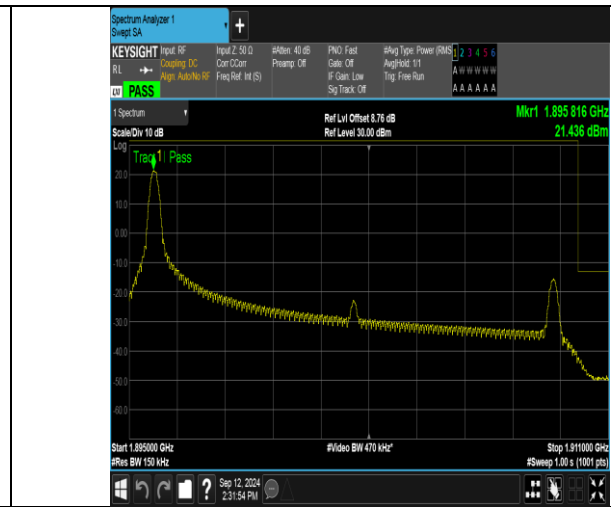
Band2_15MHz_16QAM_19125_1RB#0
