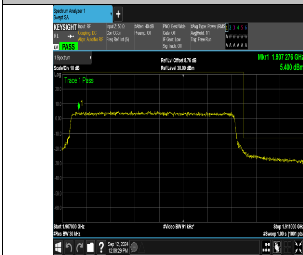
Band2_3MHz_QPSK_19185_15RB#0
