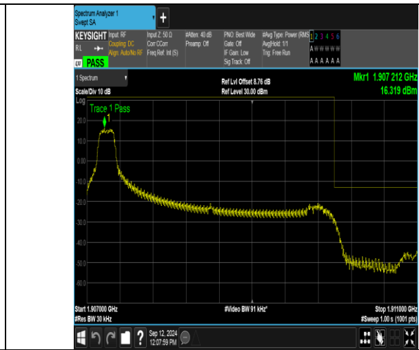
Band2_3MHz_16QAM_19185_1RB#0
