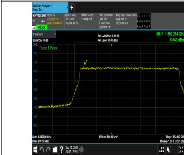
Band2_3MHz_QPSK_18615_15RB#0
