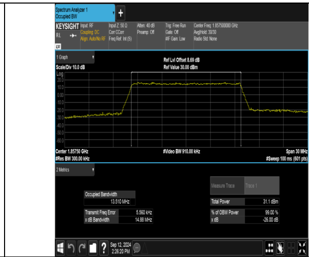
Band2-15MHz-16QAM-18675-75RB#0-PASS
