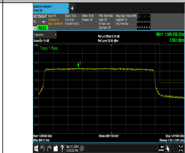
Band2_5MHz_16QAM_19175_25RB#0
