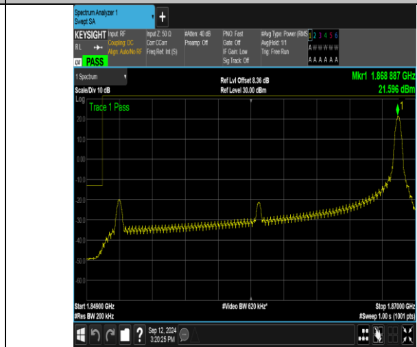
Band2_20MHz_16QAM_18700_1RB#99
