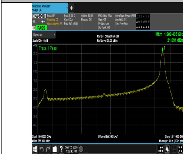
Band2_10MHz_QPSK_19150_1RB#49
