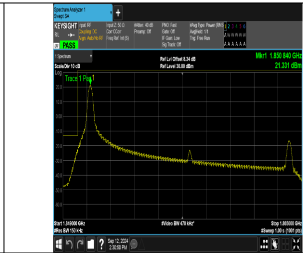
Band2_15MHz_16QAM_18675_1RB#0
