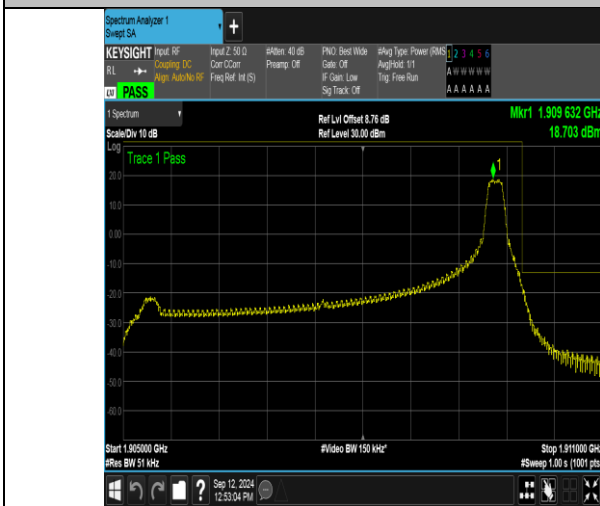
Band2_5MHz_QPSK_19175_1RB#24
