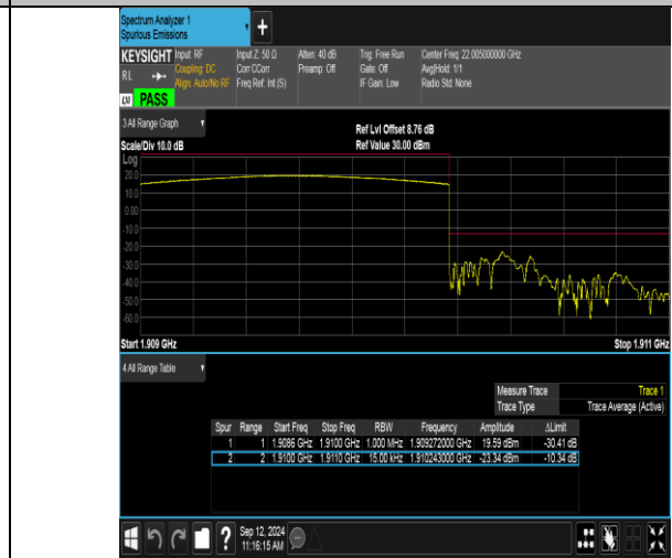
Band2_1.4MHz_16QAM_19193_6RB#0
