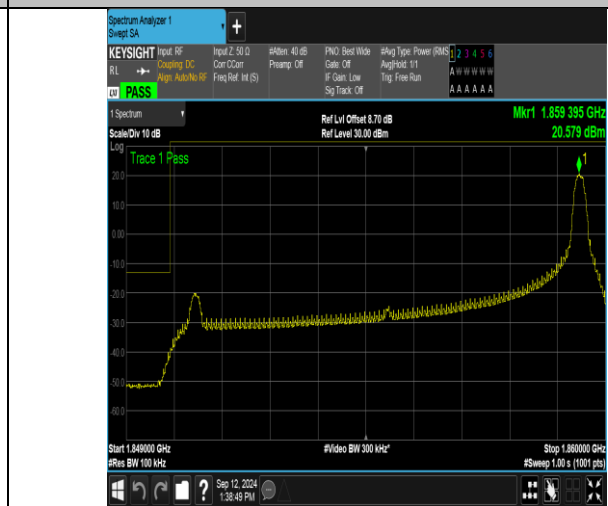
Band2_10MHz_16QAM_18650_1RB#49
