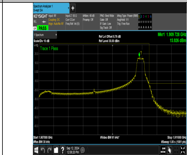
Band2_3MHz_16QAM_19185_1RB#14
