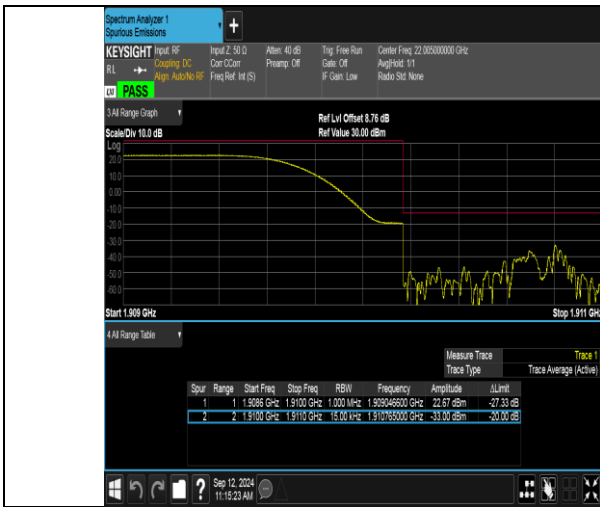
Band2_1.4MHz_QPSK_19193_1RB#0
