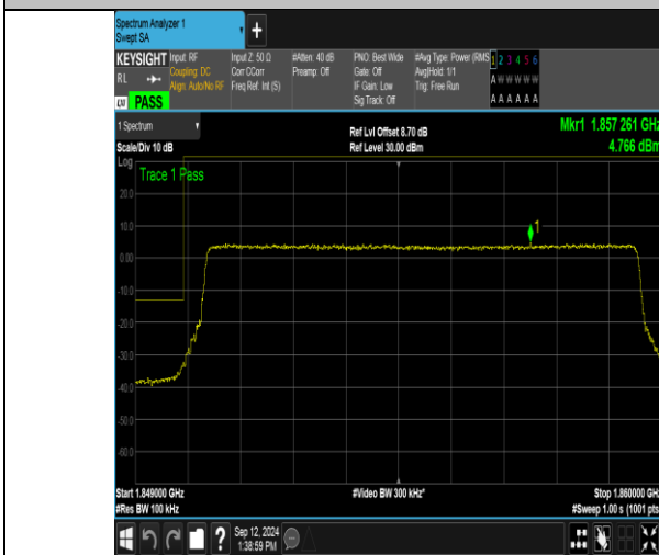
Band2_10MHz_QPSK_18650_50RB#0
