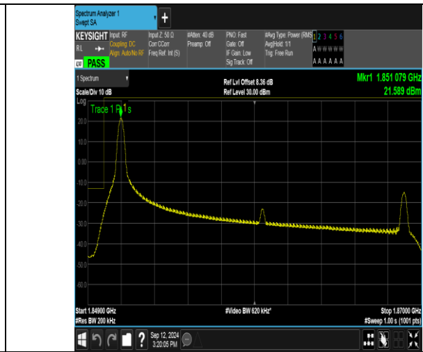
Band2_20MHz_16QAM_18700_1RB#0
