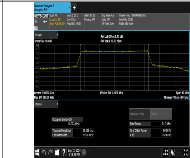
Band2-20MHz-16QAM-19100-100RB#0-PASS
