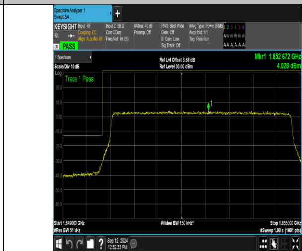
Band2_5MHz_16QAM_18625_25RB#0
