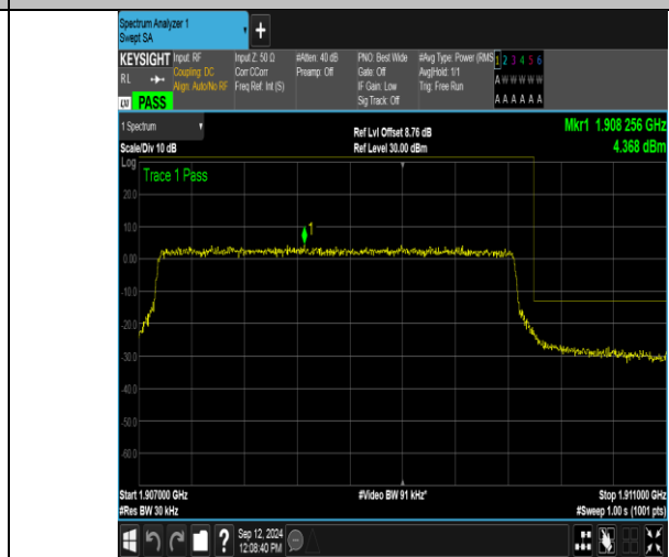
Band2_3MHz_16QAM_19185_15RB#0
