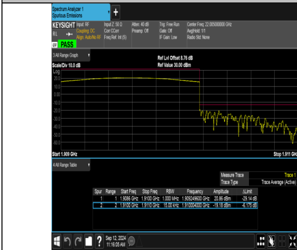
Band2_1.4MHz_QPSK_19193_6RB#0
