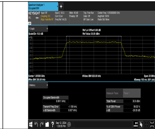
Band2-10MHz-16QAM-18650-50RB#0-PASS
