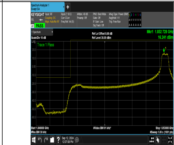
Band2_3MHz_16QAM_18615_1RB#14
