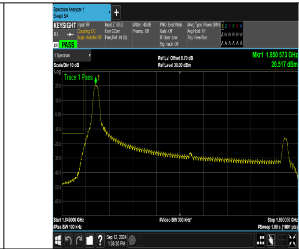
Band2_10MHz_16QAM_18650_1RB#0
