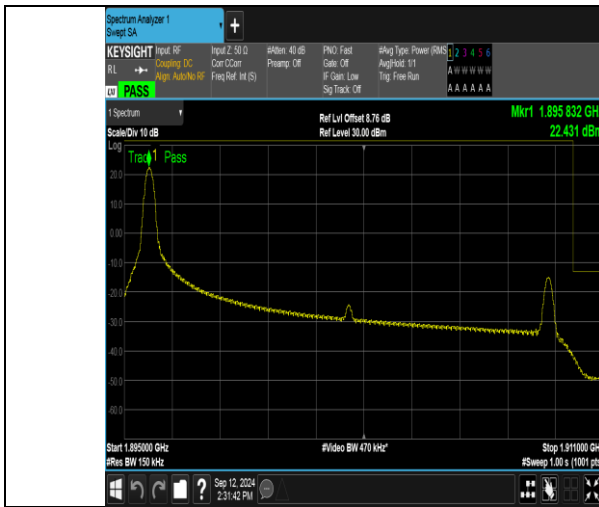
Band2_15MHz_QPSK_19125_1RB#0
