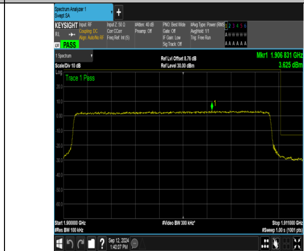
Band2_10MHz_16QAM_19150_50RB#0
