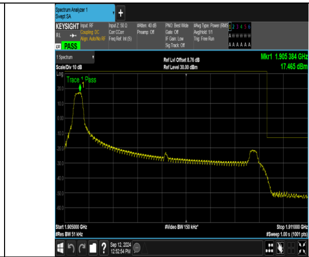
Band2_5MHz_16QAM_19175_1RB#0
