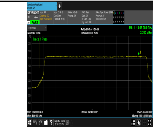
Band2_15MHz_16QAM_18675_75RB#0
