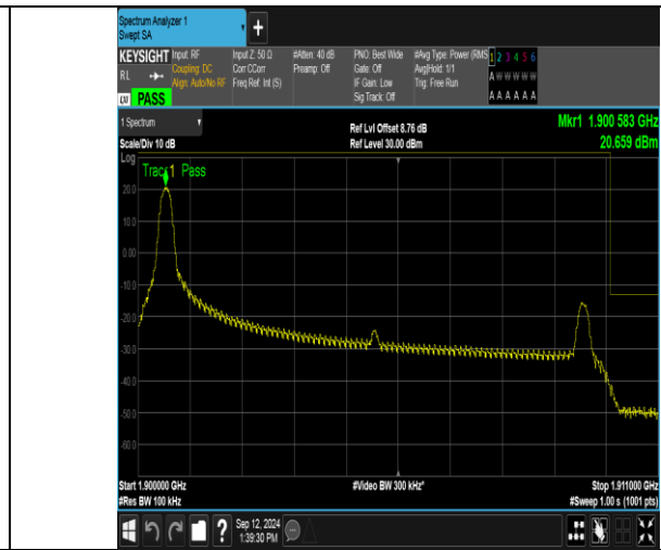
Band2_10MHz_16QAM_19150_1RB#0
