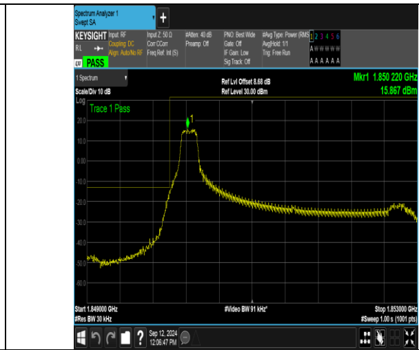
Band2_3MHz_16QAM_18615_1RB#0
