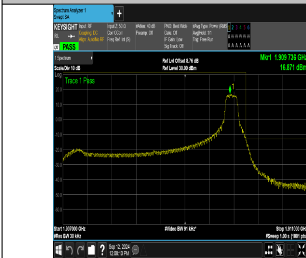
Band2_3MHz_QPSK_19185_1RB#14
