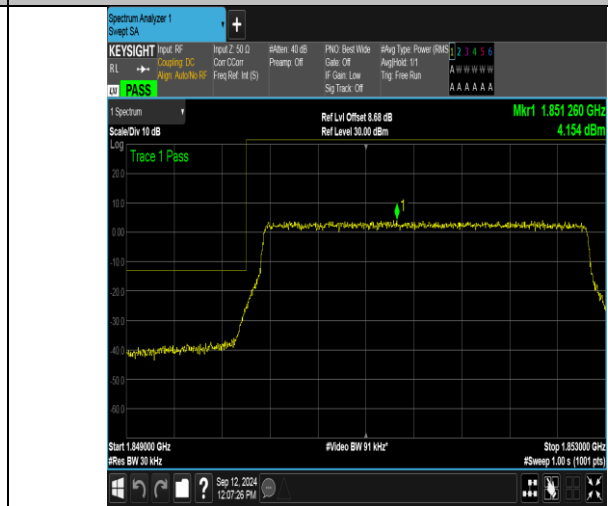
Band2_3MHz_16QAM_18615_15RB#0
