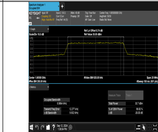
Band2-10MHz-16QAM-19150-50RB#0-PASS
