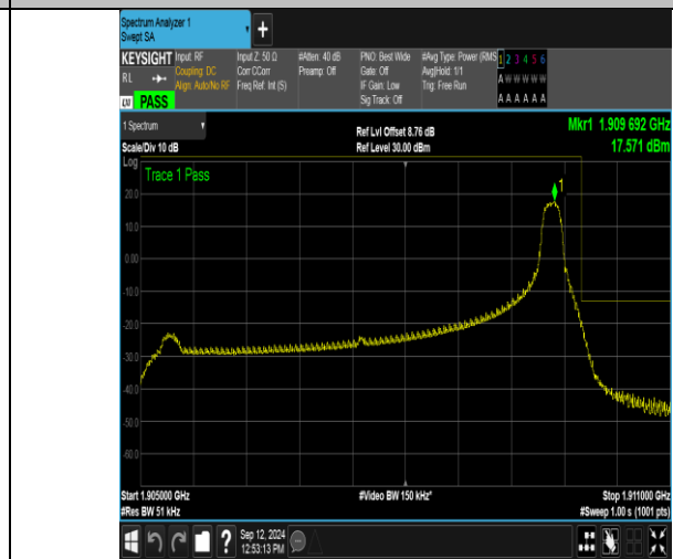
Band2_5MHz_16QAM_19175_1RB#24
