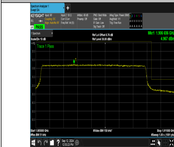
Band2_5MHz_QPSK_19175_25RB#0
