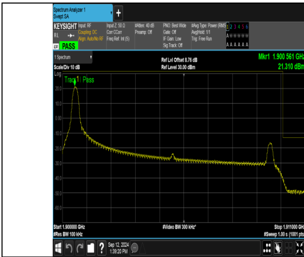
Band2_10MHz_QPSK_19150_1RB#0
