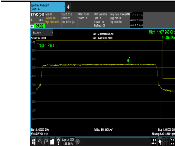
Band2_10MHz_QPSK_19150_50RB#0
