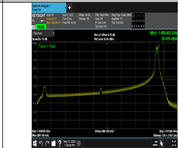
Band2_10MHz_16QAM_19150_1RB#49
