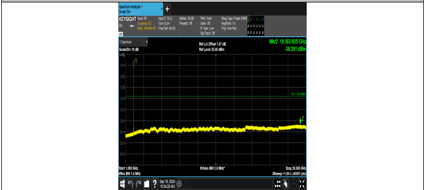
Band2-9262-3-1000~20000MHz-PASS
