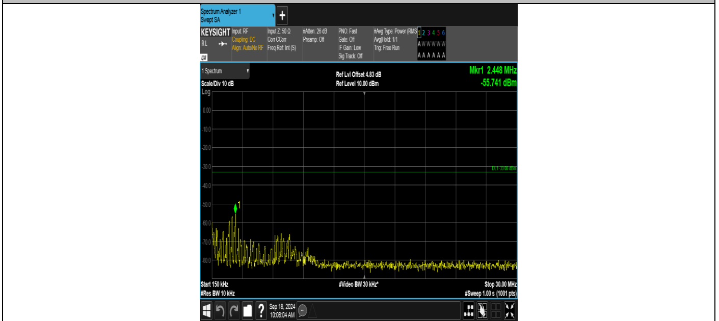
Band2-9538-4-0.15~30MHz-PASS
