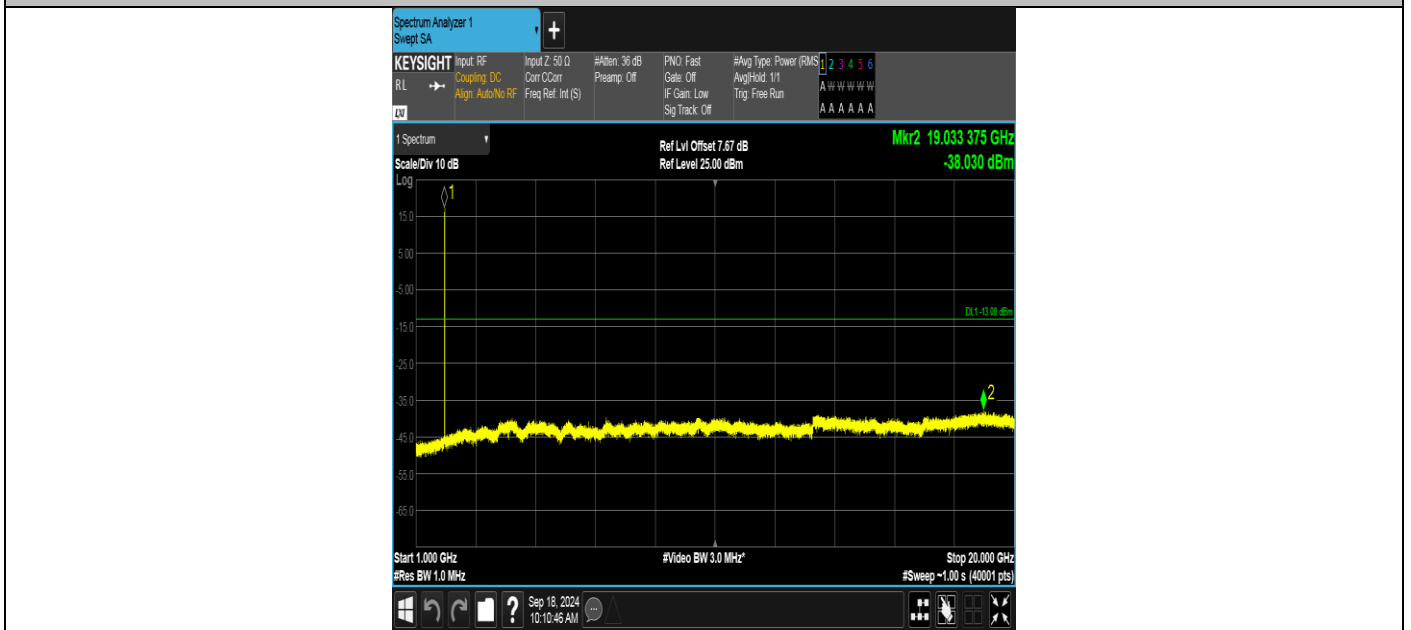
Band2-9538-5-1000~20000MHz-PASS
