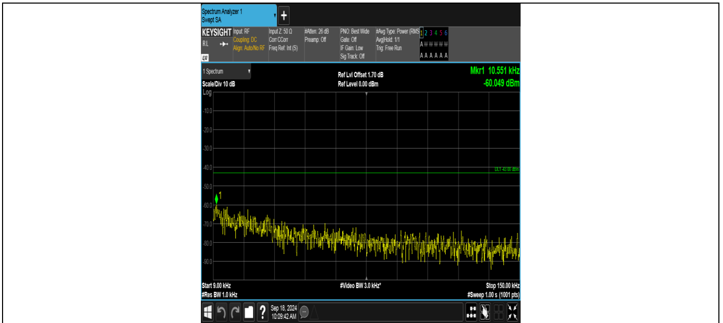
Band2-9400-5-0.009~0.15MHz-PASS
