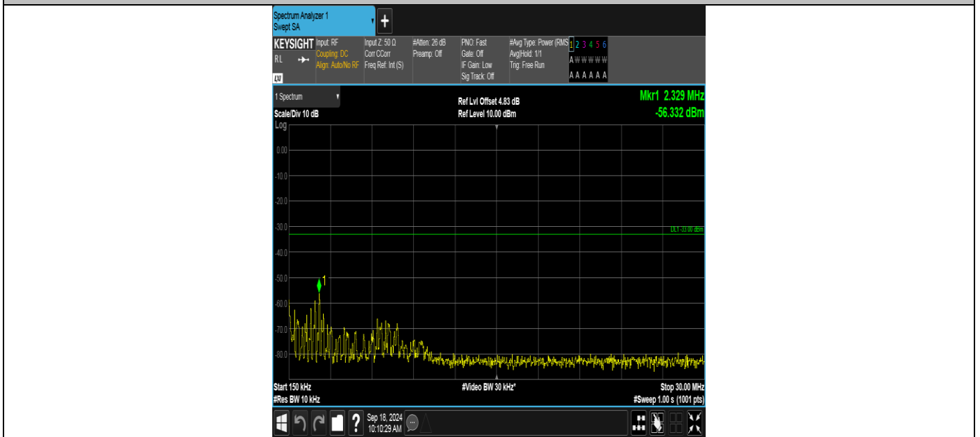
Band2-9538-5-0.15~30MHz-PASS
