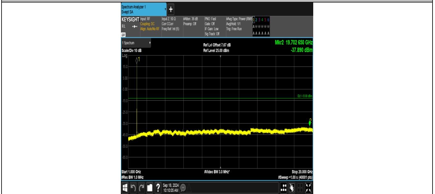
Band2-9400-5-1000~20000MHz-PASS
