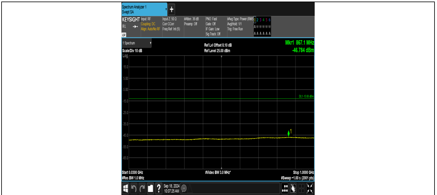
Band2-9400-4-30~1000MHz-PASS
