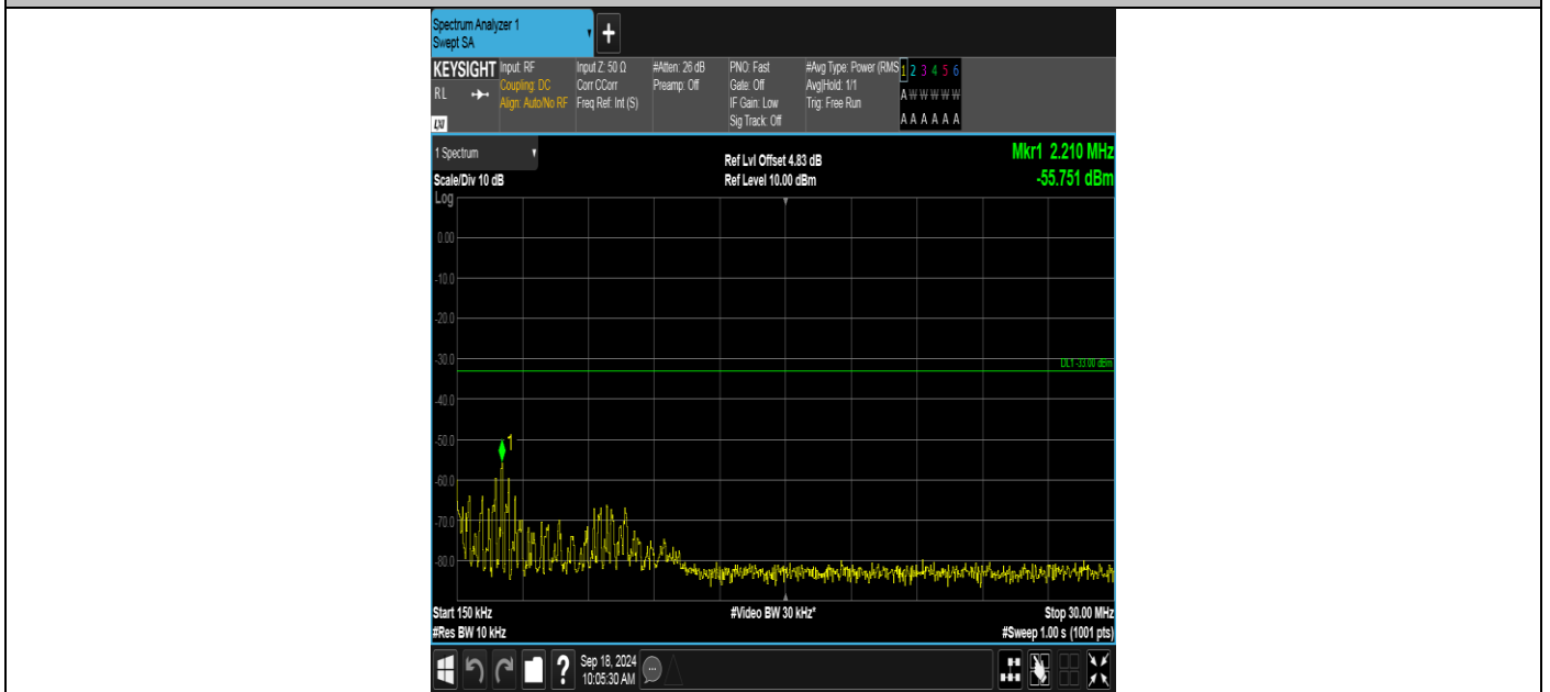
Band2-9538-3-0.15~30MHz-PASS
