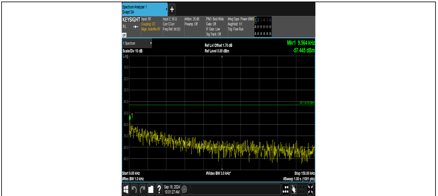
Band2-9262-2-0.009~0.15MHz-PASS
