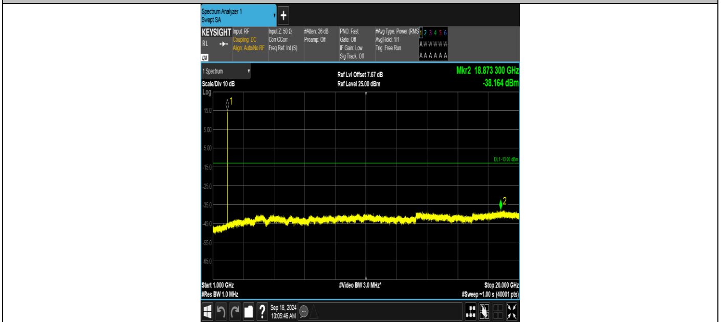
Band2-9538-3-1000~20000MHz-PASS
