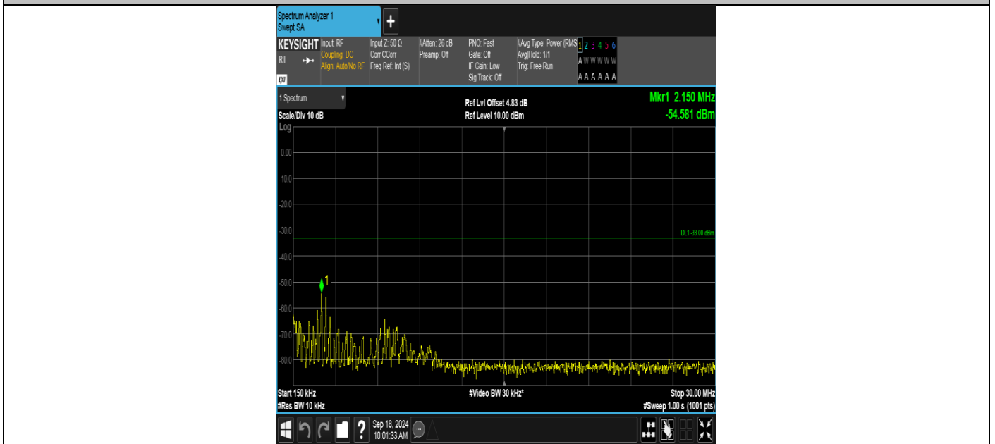
Band2-9262-2-0.15~30MHz-PASS
