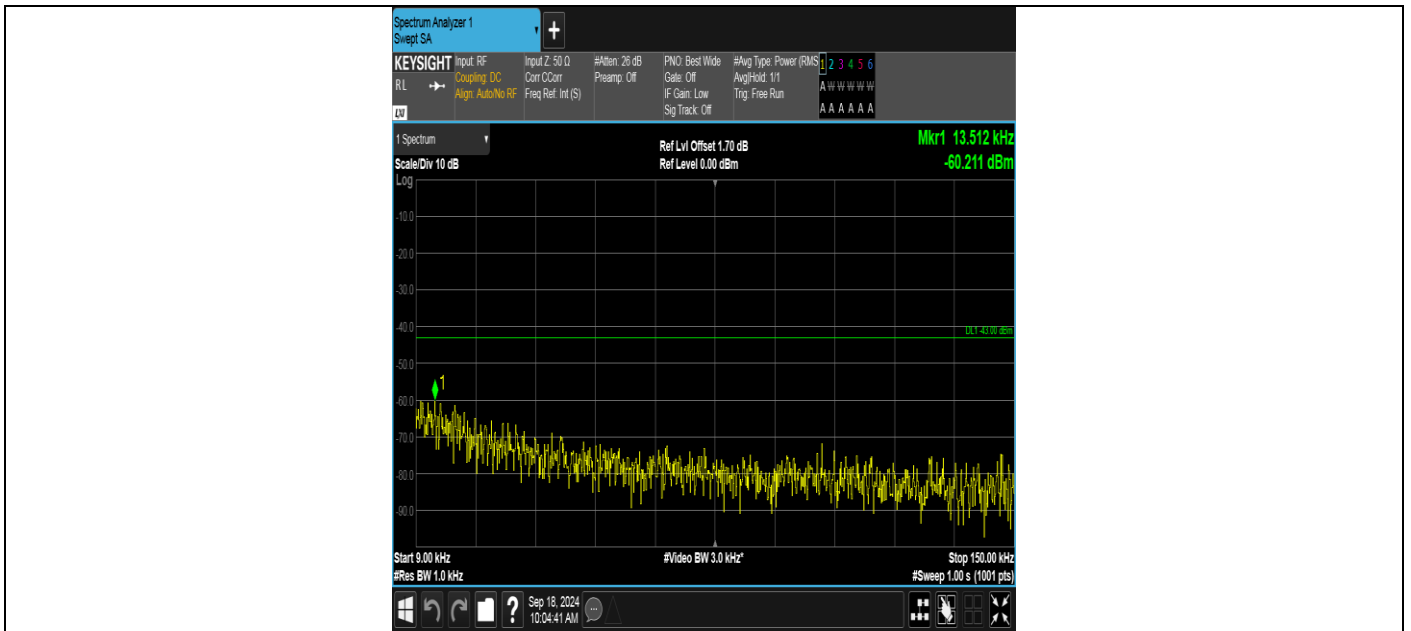
Band2-9400-3-0.009~0.15MHz-PASS
