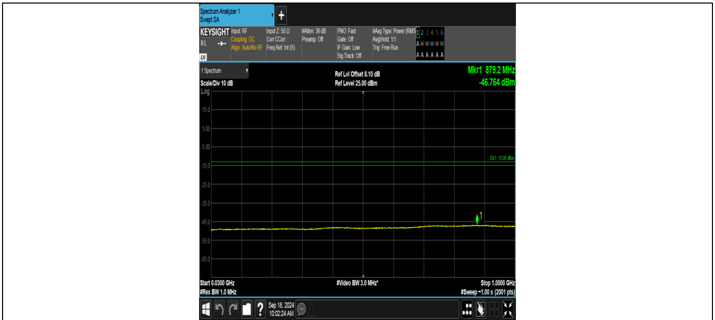
Band2-9400-2-30~1000MHz-PASS
