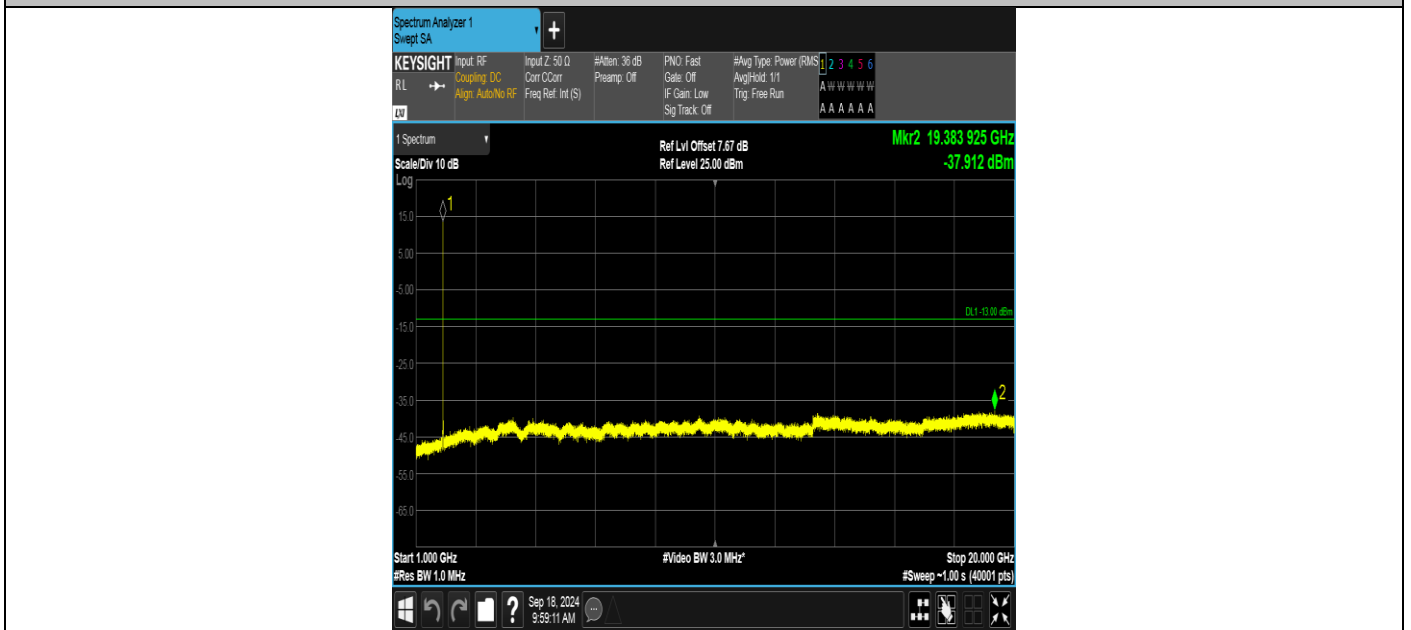
Band2-9262-1-1000~20000MHz-PASS
