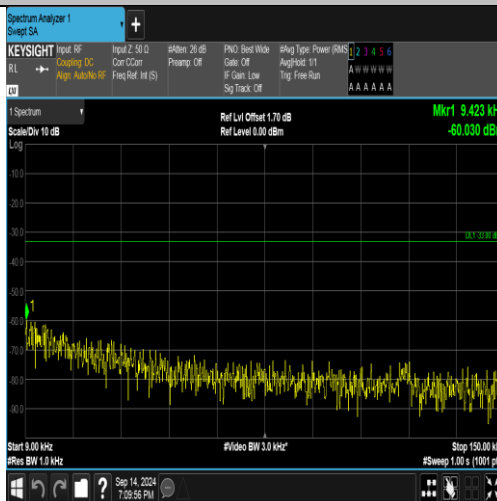
Band5-4233-4-0.009~0.15MHz-PASS
