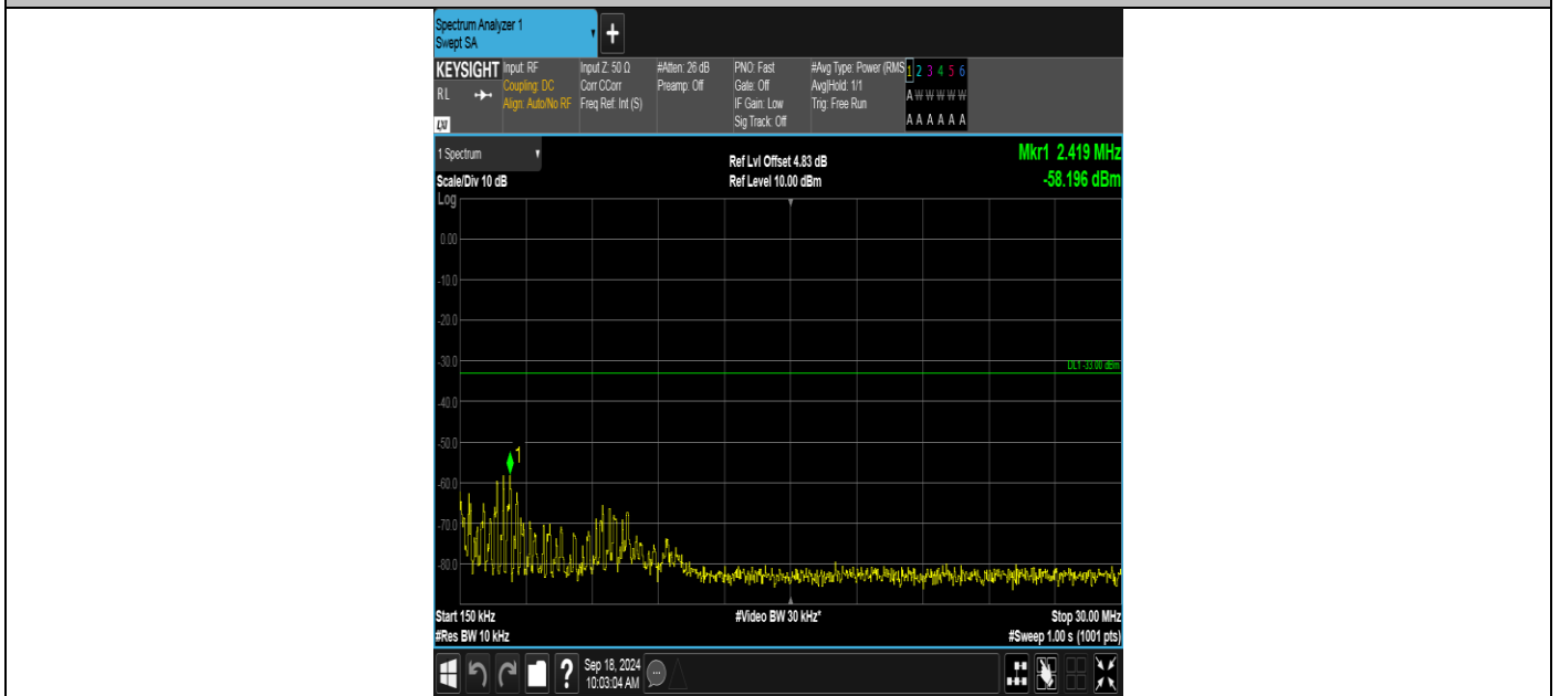
Band2-9538-2-0.15~30MHz-PASS
