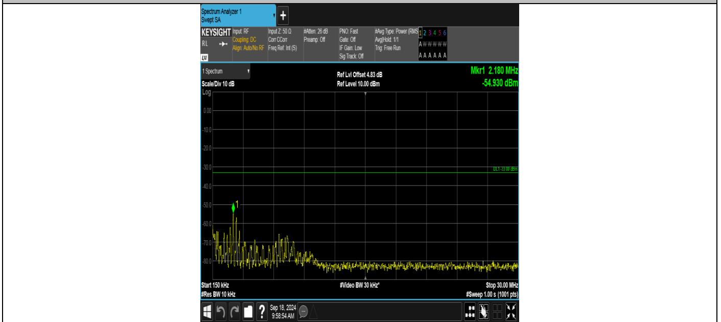
Band2-9262-1-0.15~30MHz-PASS
