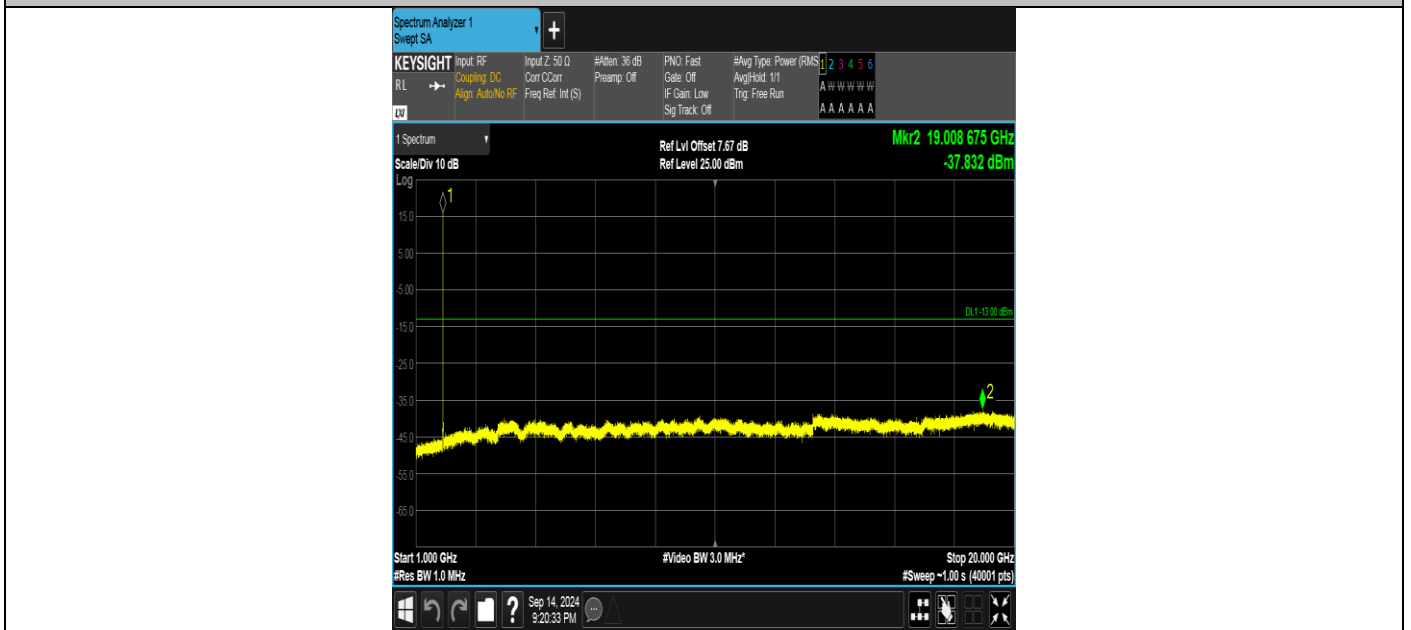
Band2-9262-3-1000~20000MHz-PASS
