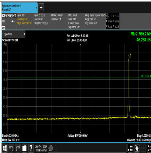
Band5-4182-2-30~1000MHz-PASS
