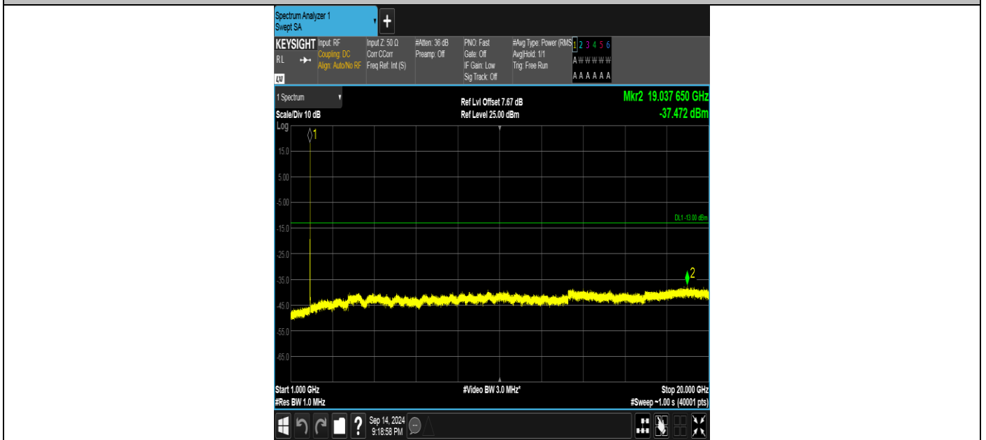
Band2-9400-2-1000~20000MHz-PASS
