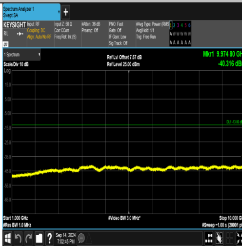
Band5-4182-1-1000~10000MHz-PASS
