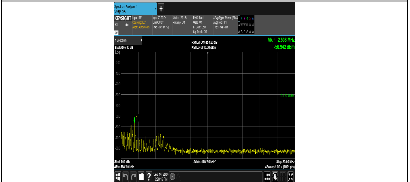
Band2-9262-3-0.15~30MHz-PASS
