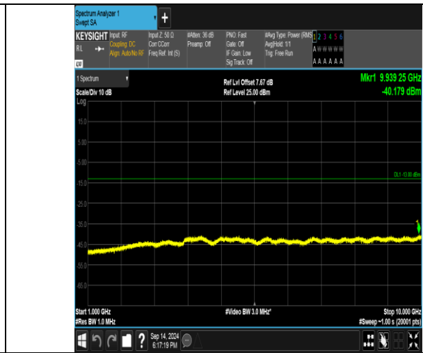
Band5-4182-1000~10000MHz-PASS
