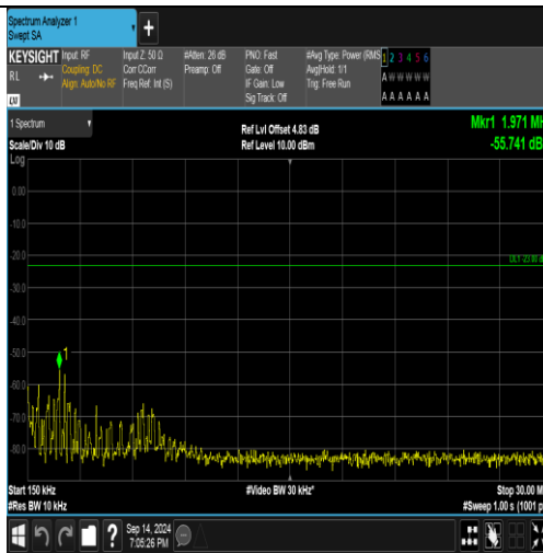
Band5-4233-2-0.15~30MHz-PASS
