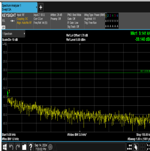
Band5-4233-1-0.009~0.15MHz-PASS
