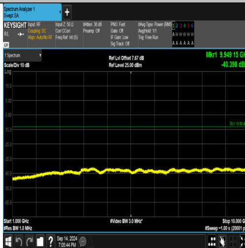
Band5-4233-2-1000~10000MHz-PASS
