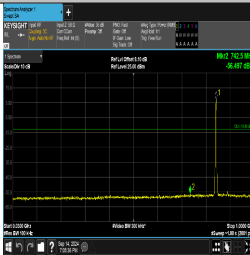
Band5-4233-2-30~1000MHz-PASS
