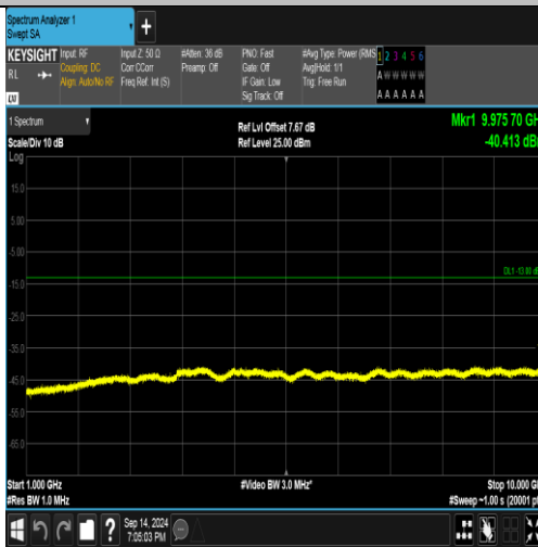
Band5-4182-2-1000~10000MHz-PASS
