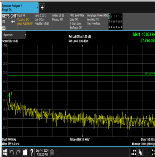
Band5-4233-2-0.009~0.15MHz-PASS
