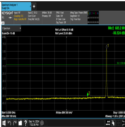
Band5-4182-1-30~1000MHz-PASS
