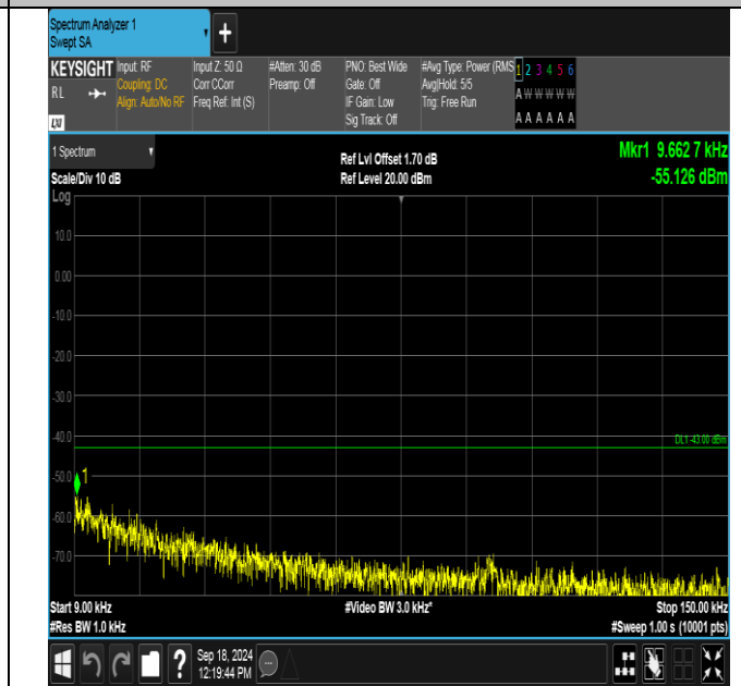
GPRS1900-512-0-0.009~0.15MHz-PASS
