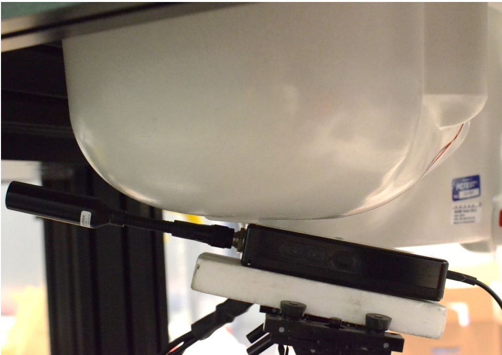
SAR Test Setup Photo 2: Head, Right Tilt, 0 mm
