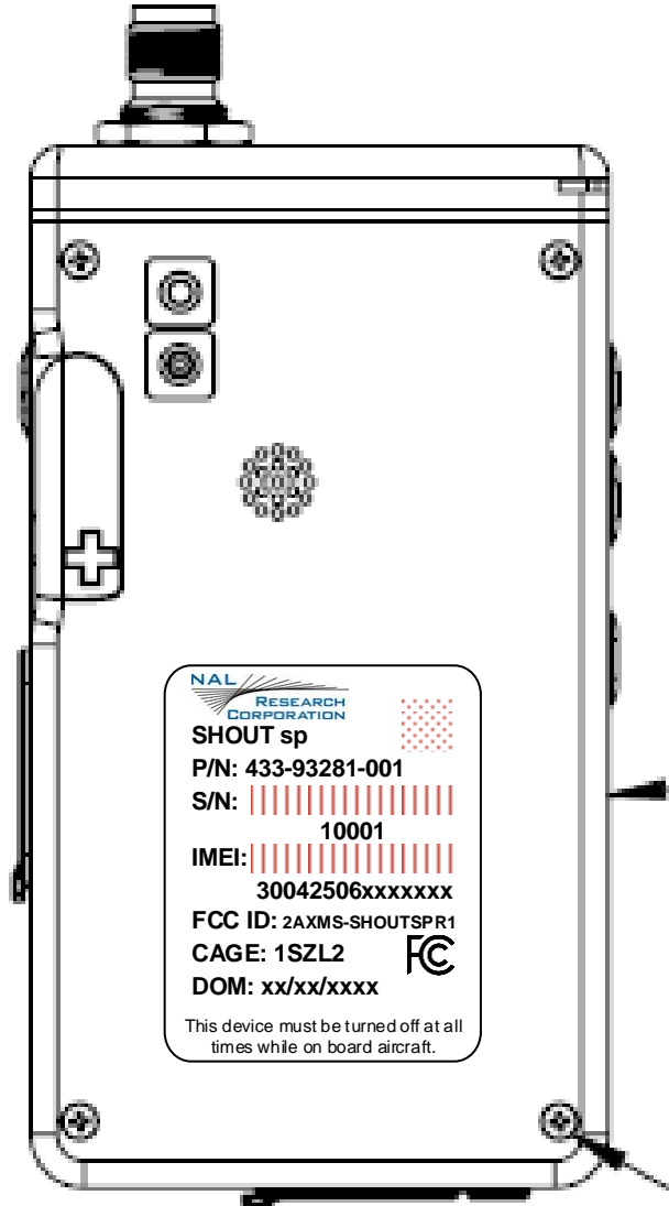
NAL SHOUT sp with Proposed FCC ID Label and Location
