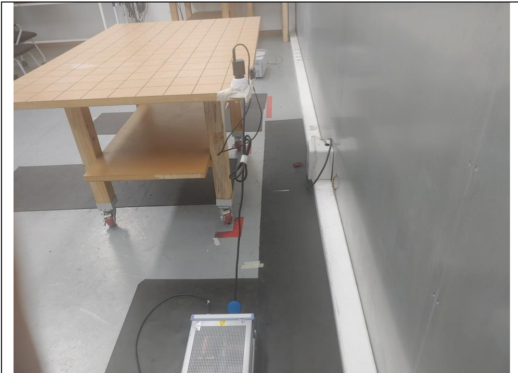
Conducted Emission
