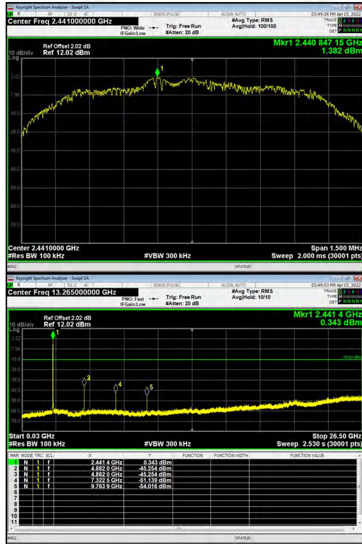
30MHz~26.5GHz
