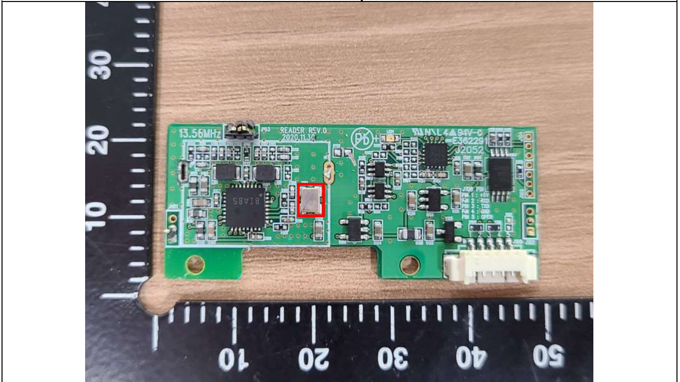
Shield Can opened
