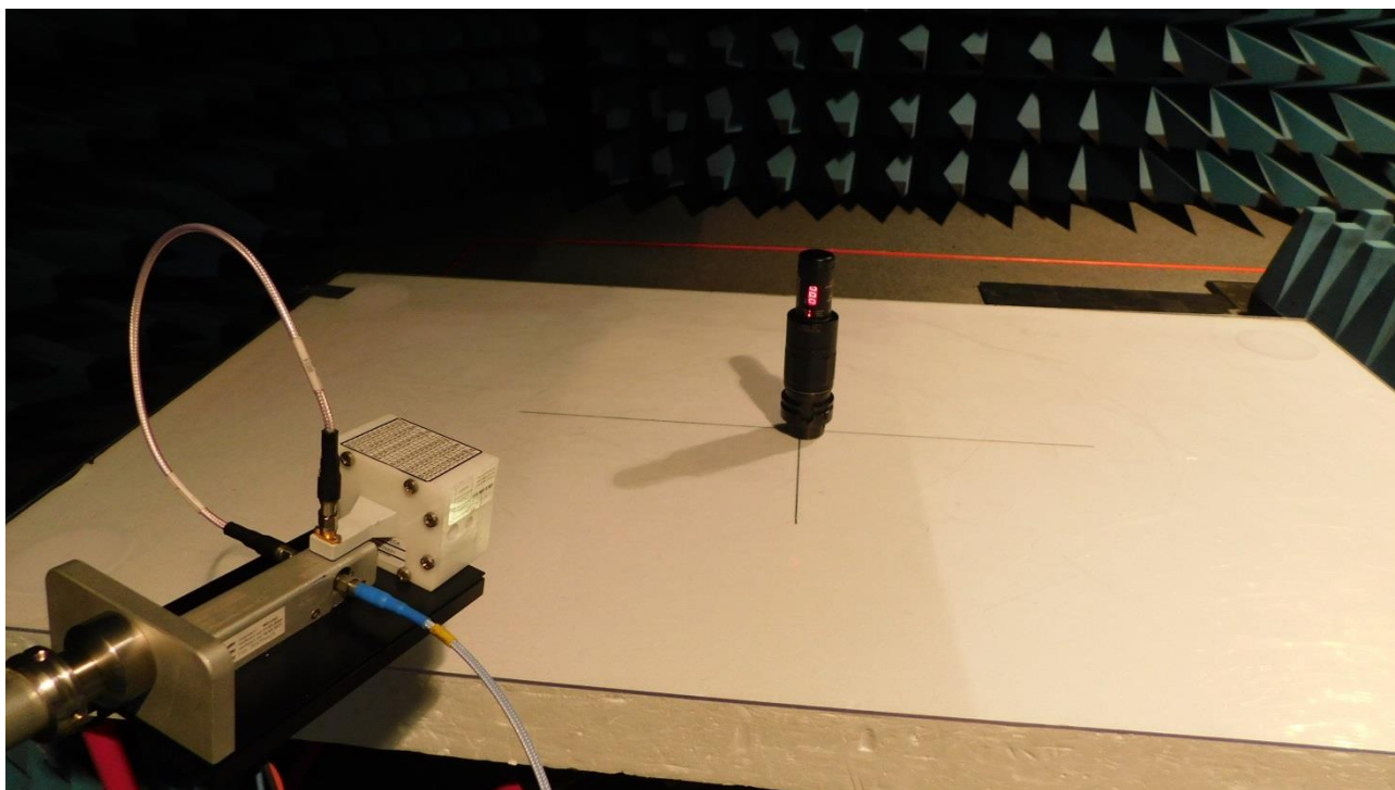
Picture 7: AC, exploratory measurement 17 GHz – 25 GHz (front view)
