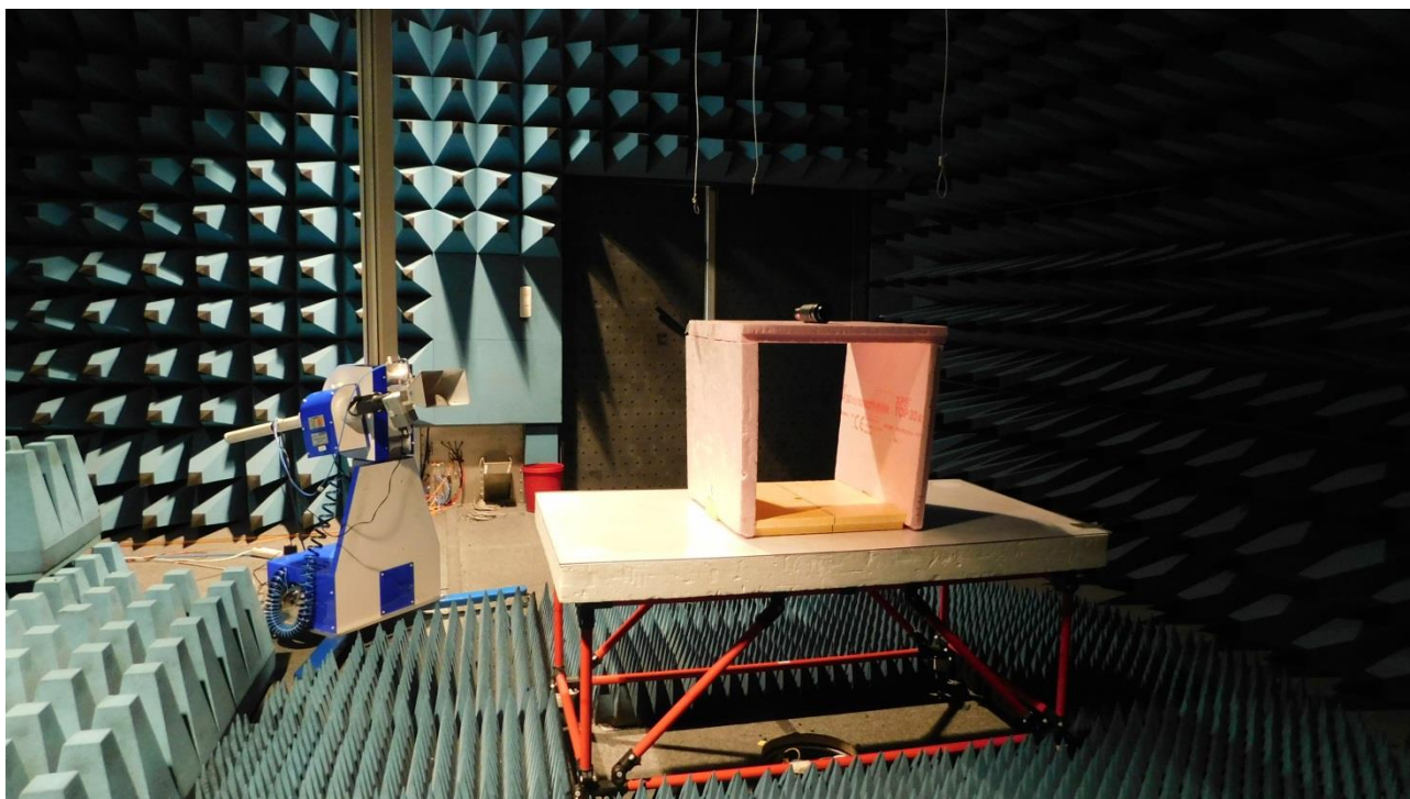
Picture 9: AC, field strength and bandwidths measurements (rear view)
