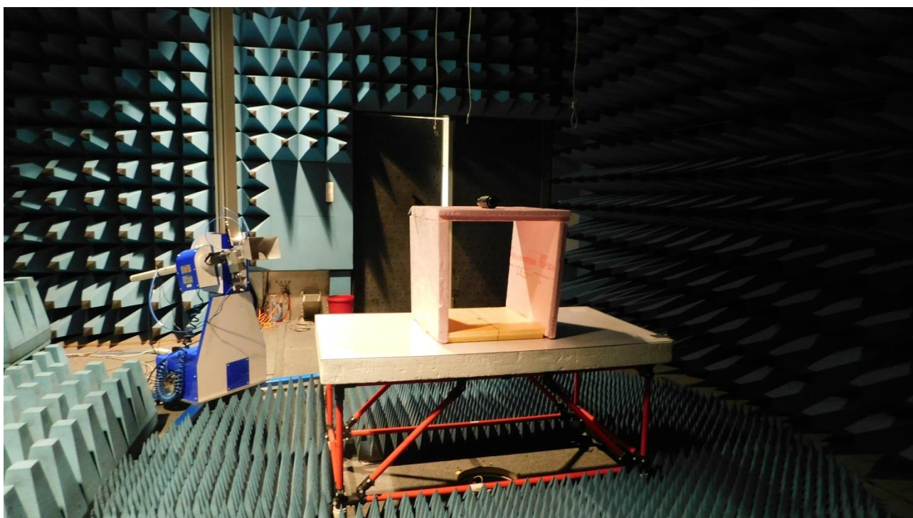
Picture 6: AC, radiated emission test 1 GHz – 17 GHz (rear view)
