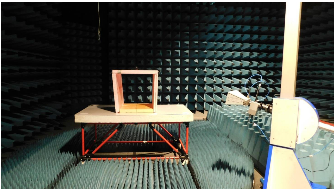
Picture 5: AC, radiated emission test 1 GHz – 17 GHz (front view)
