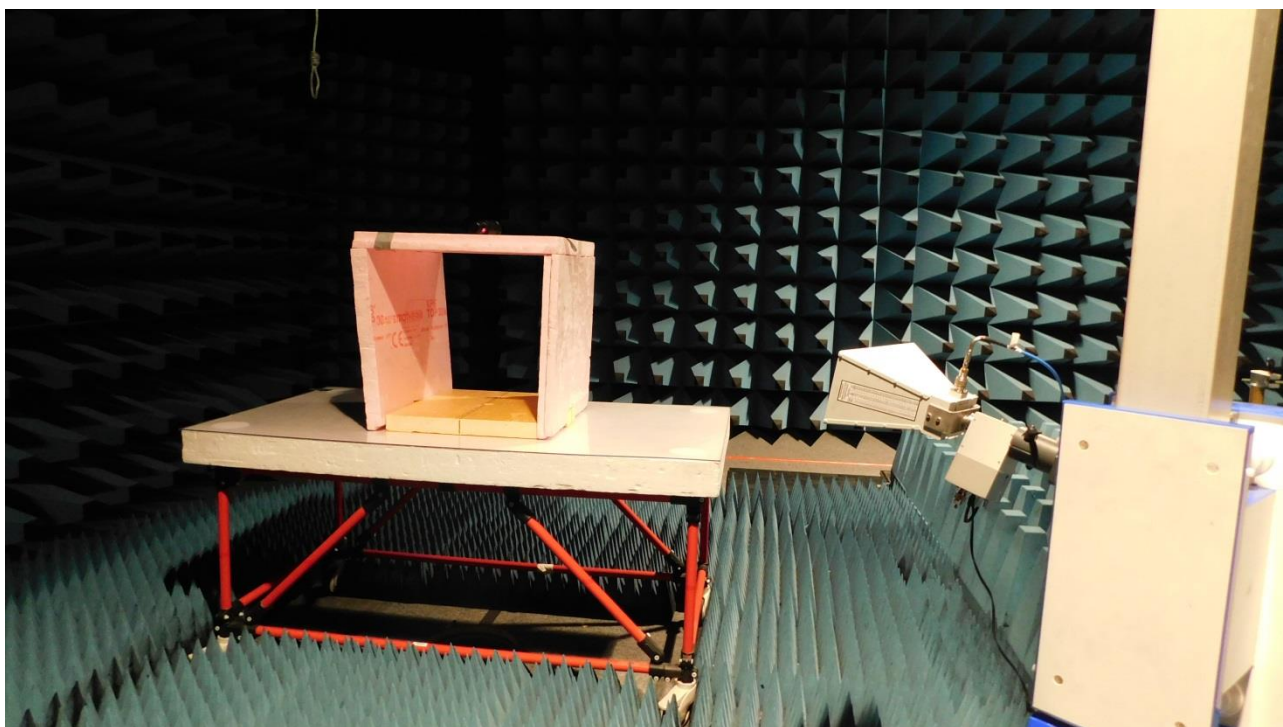
Picture 8: AC, field strength and bandwidths measurements (front view)
