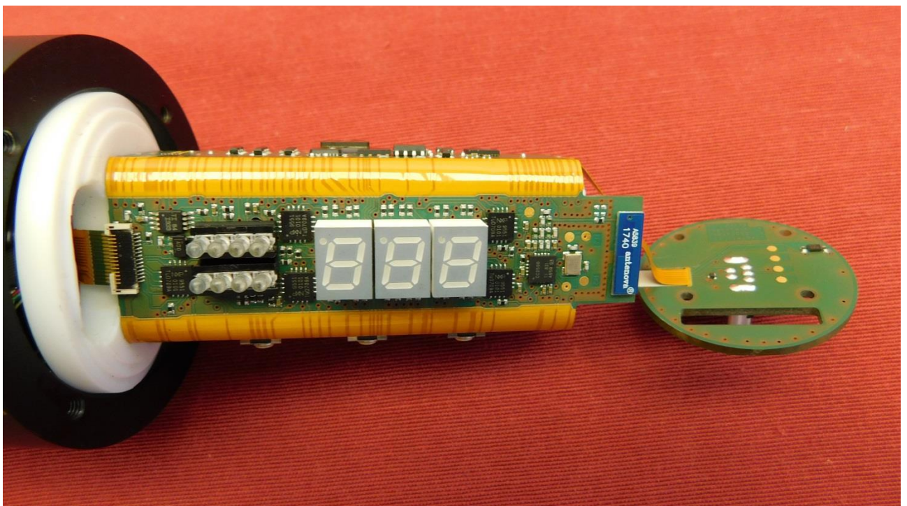
Picture 6: EUT with RF module - detailed view, without housing
