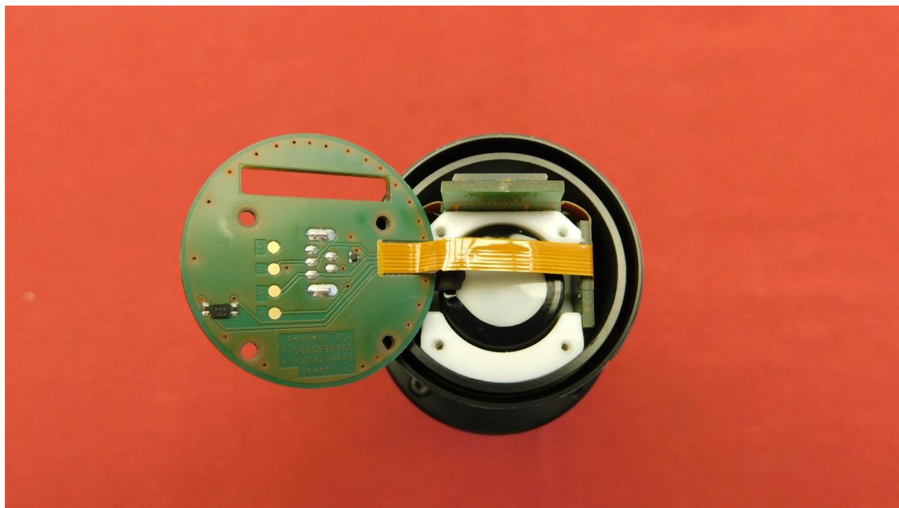
Picture 3: EUT - top view, without board
