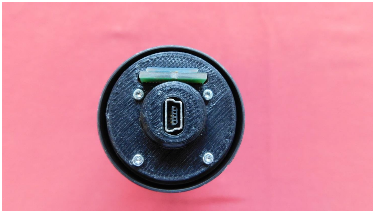
Picture 5: EUT without cap - detailed view
