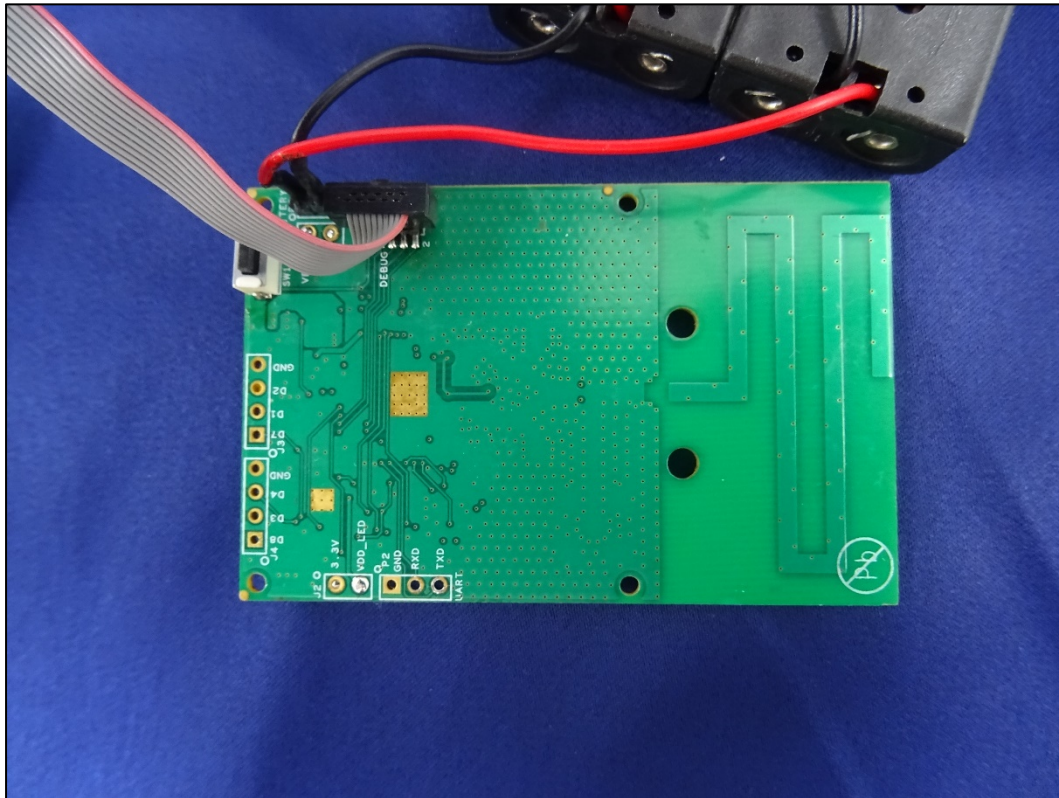
Photo 4: EUT Conducted sample Rear view
