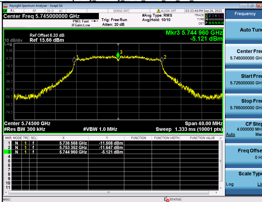
Frequency Stability NVNT ANT2 802.11a 5745
