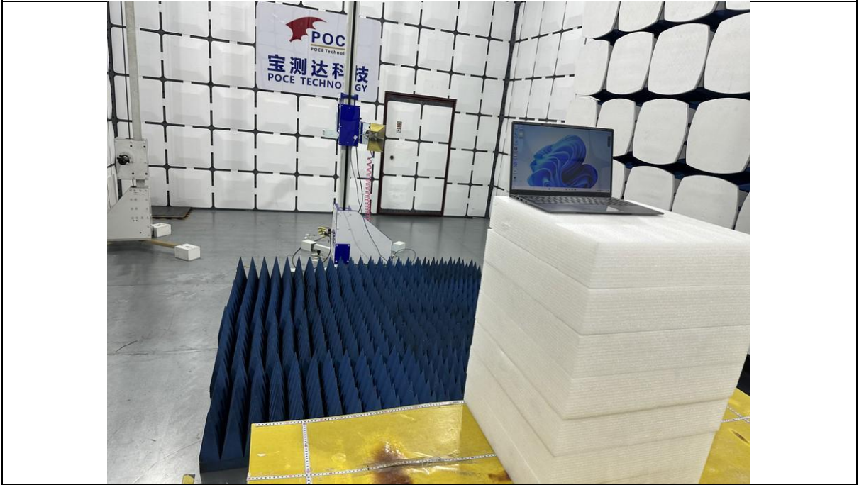
Emissions in frequency bands (above 1GHz)
