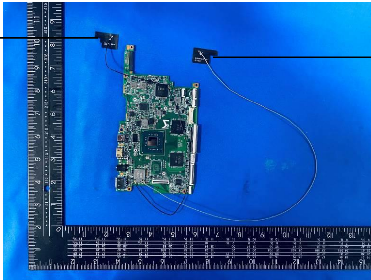
2.4G WIFI Diversity PIFA antenna
