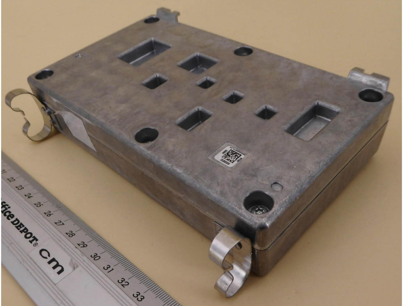
Host – 3D view 2
