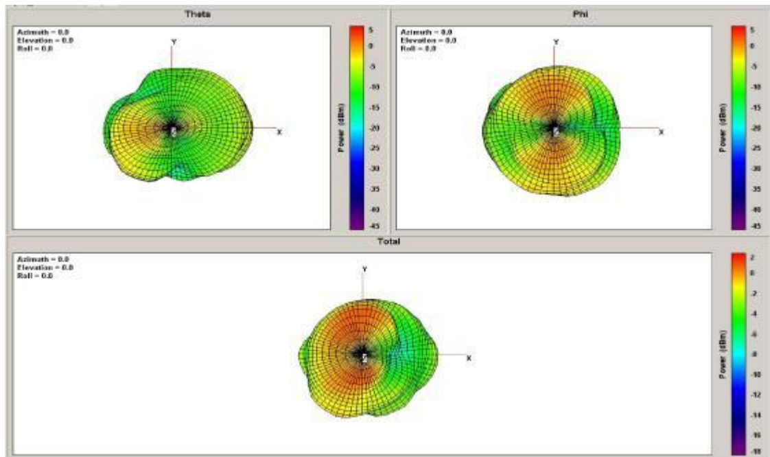
Antenna gain and 3D pattern
