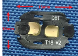
Antenna Type:FPCB Antenna
