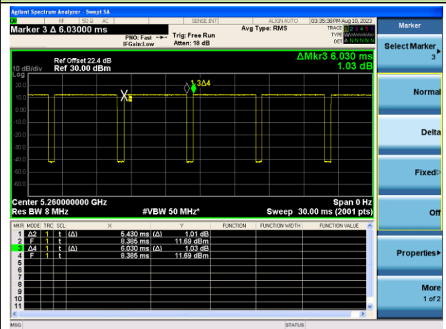
802.11ax-HE80 (T = 5.445ms)
