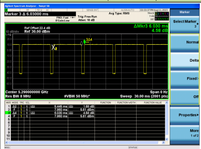
802.11ax-HE80 (T = 5.445ms)
