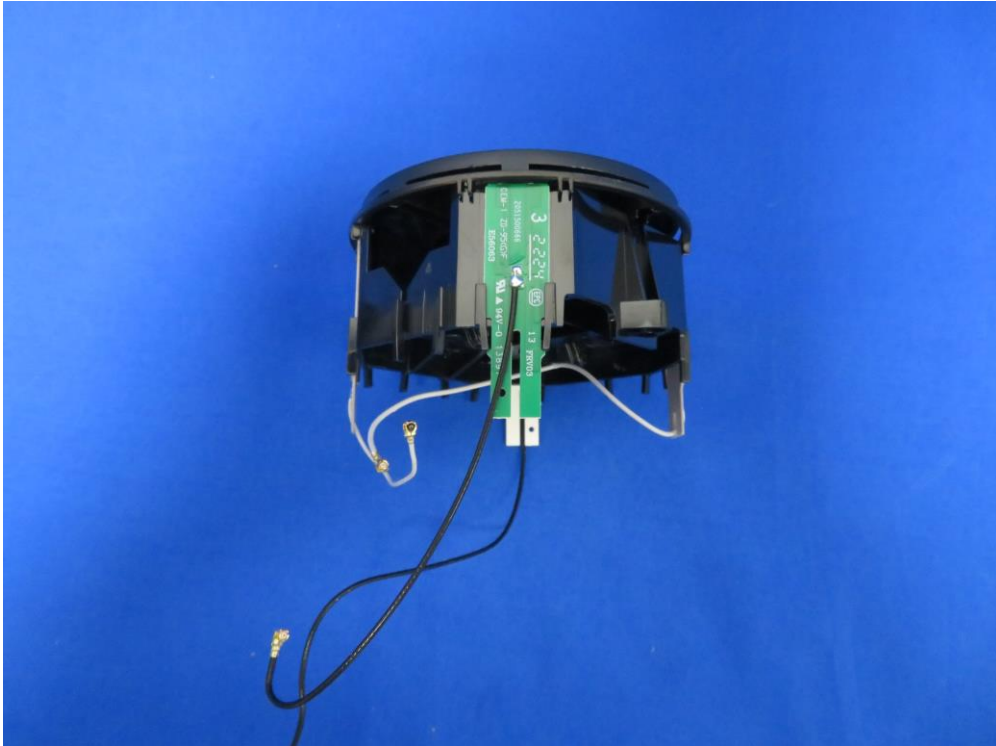
(21) EUT Photo (Wi-Fi 2.4G & 5G Antenna)
