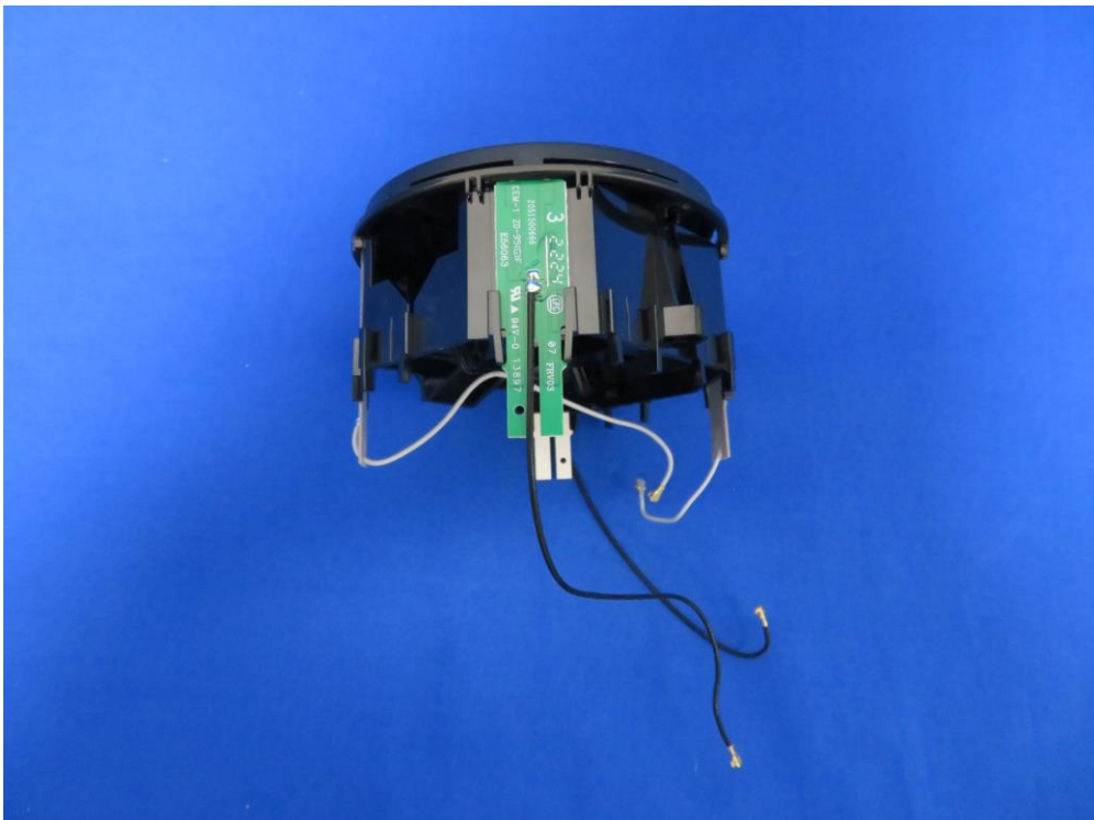
(22) EUT Photo (Wi-Fi 2.4G & 5G Antenna)
