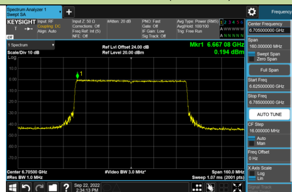
Channel 151 (6705MHz)
