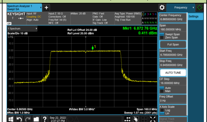
Channel 183 (6865MHz)
