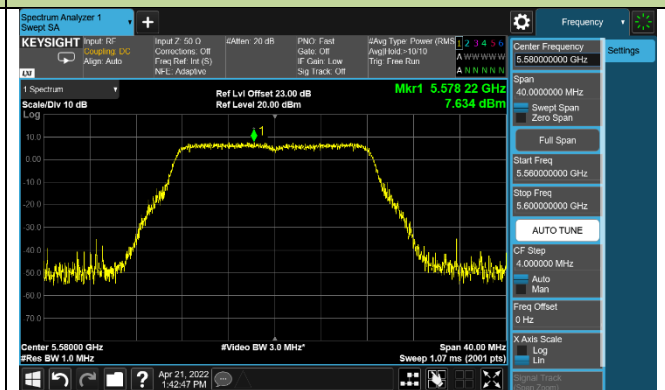
Channel 116 (5580MHz)
