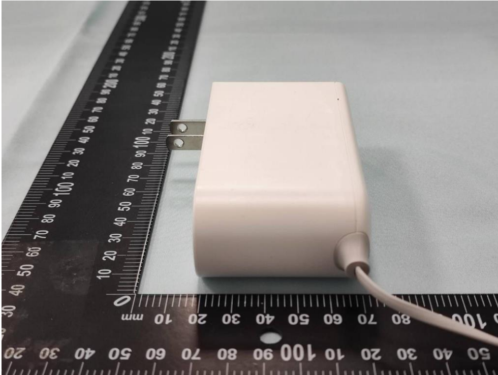
(12) EUT Photo_T120150-2B4
