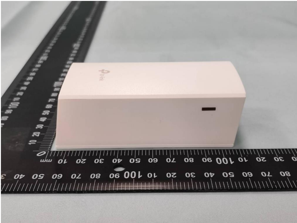
(20) EUT Photo_T480050-2-PoE
