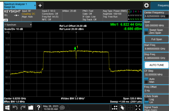
Channel 175 (6825MHz)
